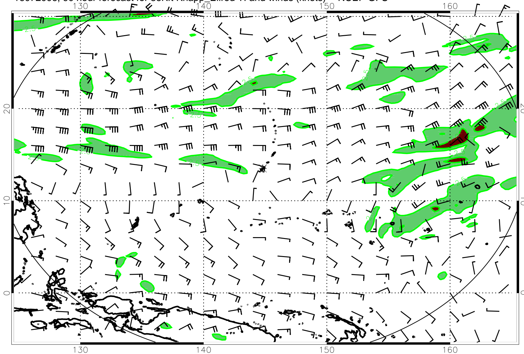
16072006, 90 hour forecast for 36Kft Knapp_Ellrod TI and winds (knots) -- NCEP GFS
