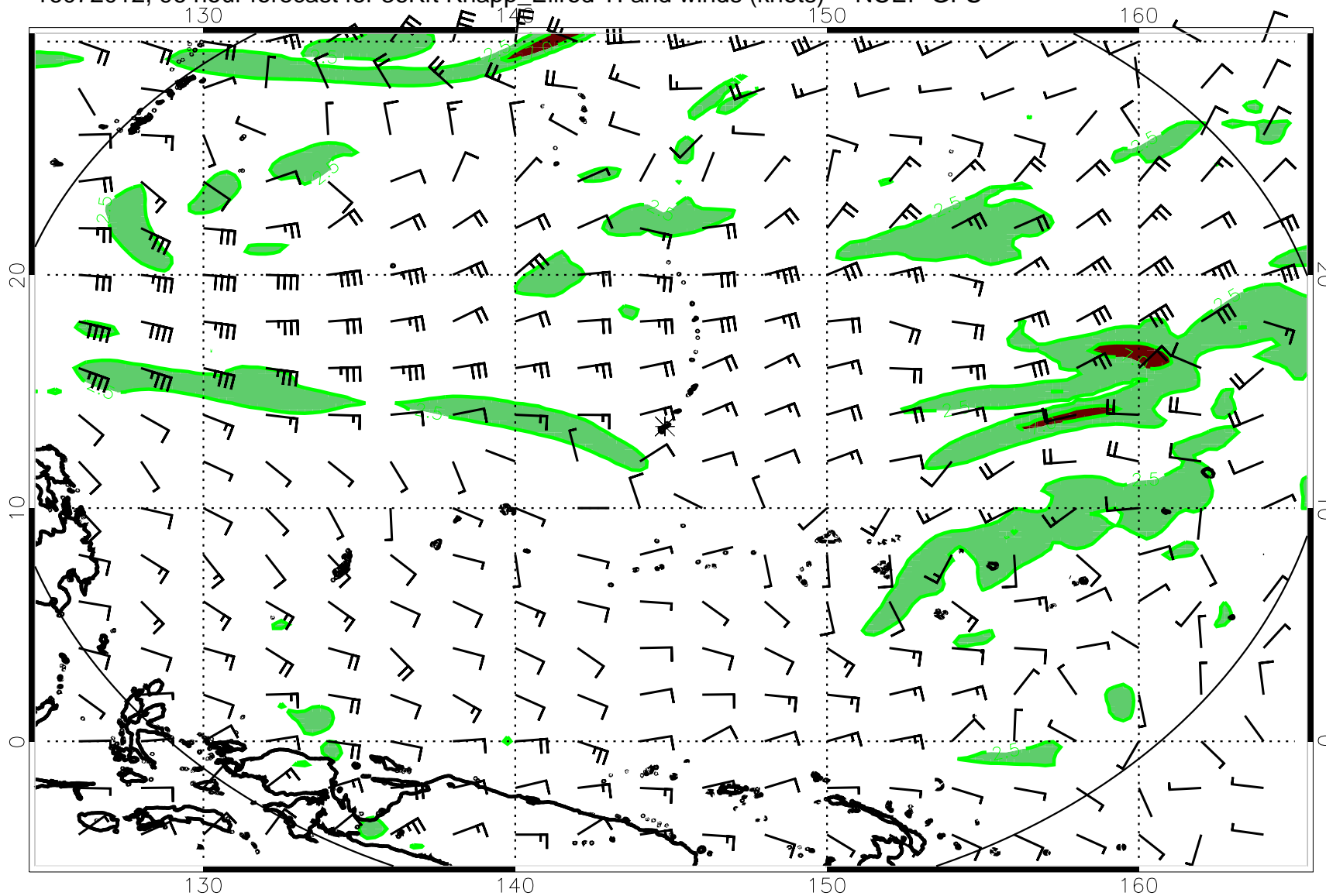
16072012, 96 hour forecast for 36Kft Knapp Ellrod TI and winds (knots) -- NCEP GFS
