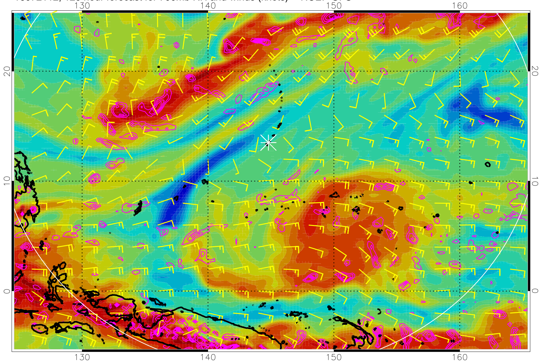
16072112, 120 hour forecast for 700mb RH and winds (knots) -- NCEP GFS
