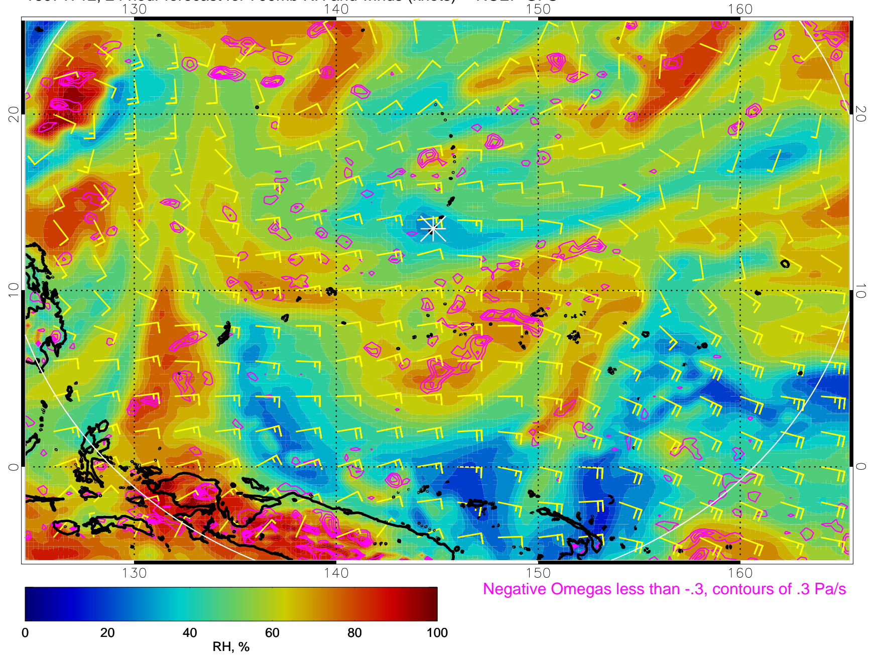
16071712, 24 hour forecast for 700mb RH and winds (knots) -- NCEP GFS
