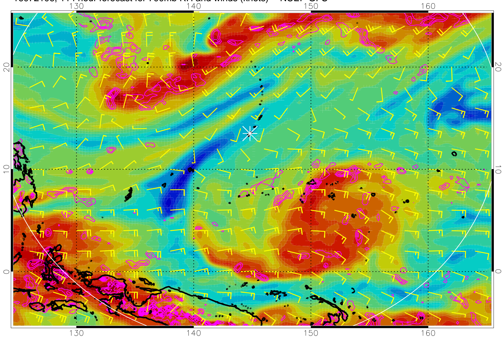
16072106, 114 hour forecast for 700mb RH and winds (knots) -- NCEP GFS
