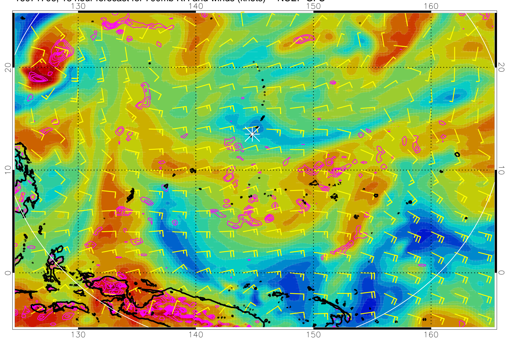
16071706, 18 hour forecast for 700mb RH and winds (knots) -- NCEP GFS
