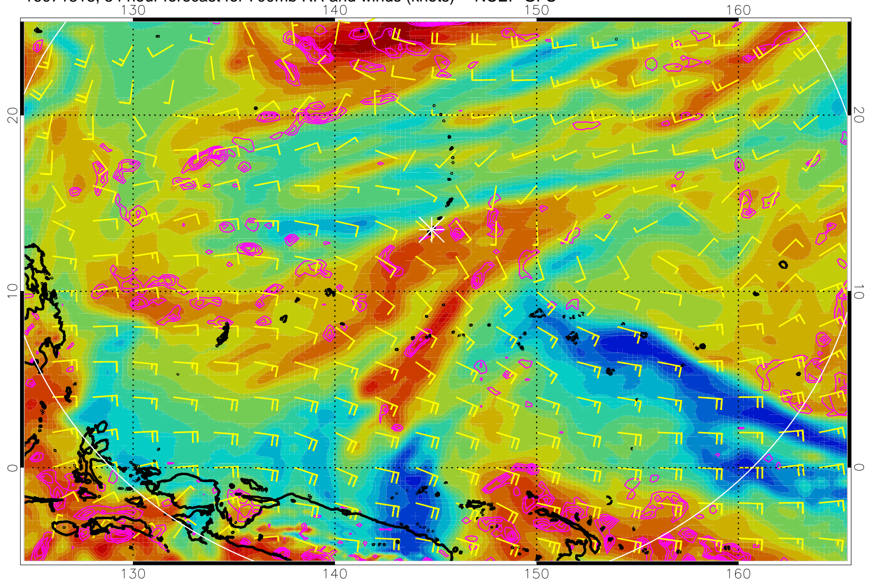
16071818, 54 hour forecast for 700mb RH and winds (knots) -- NCEP GFS
