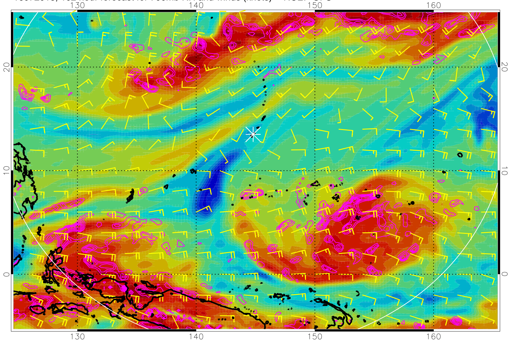
16072018, 102 hour forecast for 700mb RH and winds (knots) -- NCEP GFS
