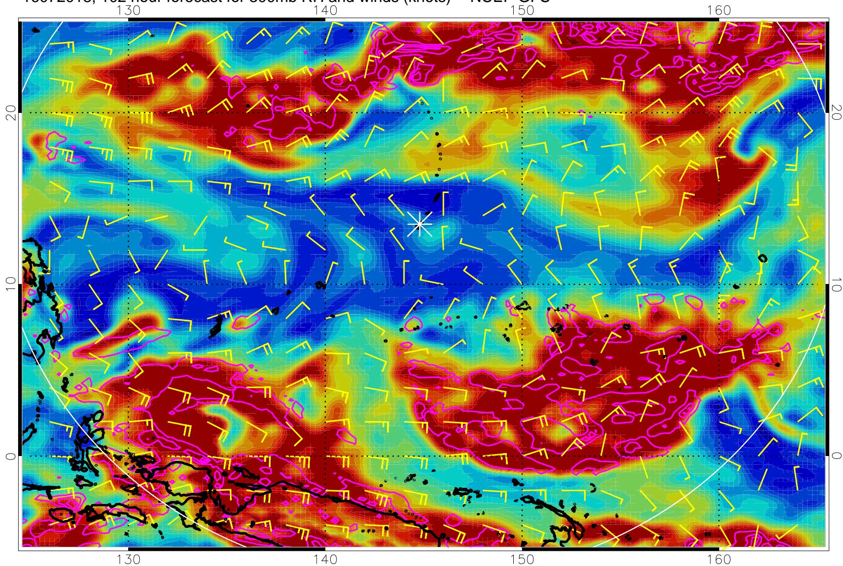
16072018, 102 hour forecast for 300mb RH and winds (knots) -- NCEP GFS
