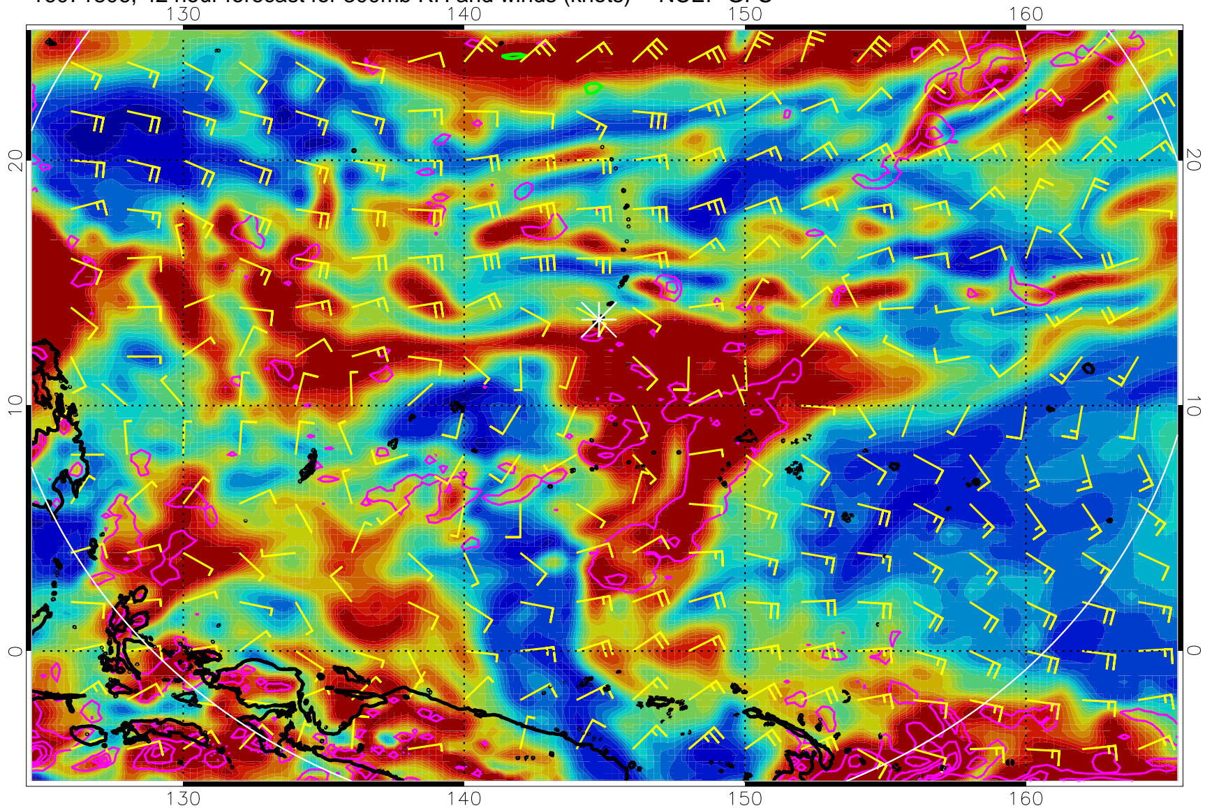
16071806, 42 hour forecast for 300mb RH and winds (knots) -- NCEP GFS
