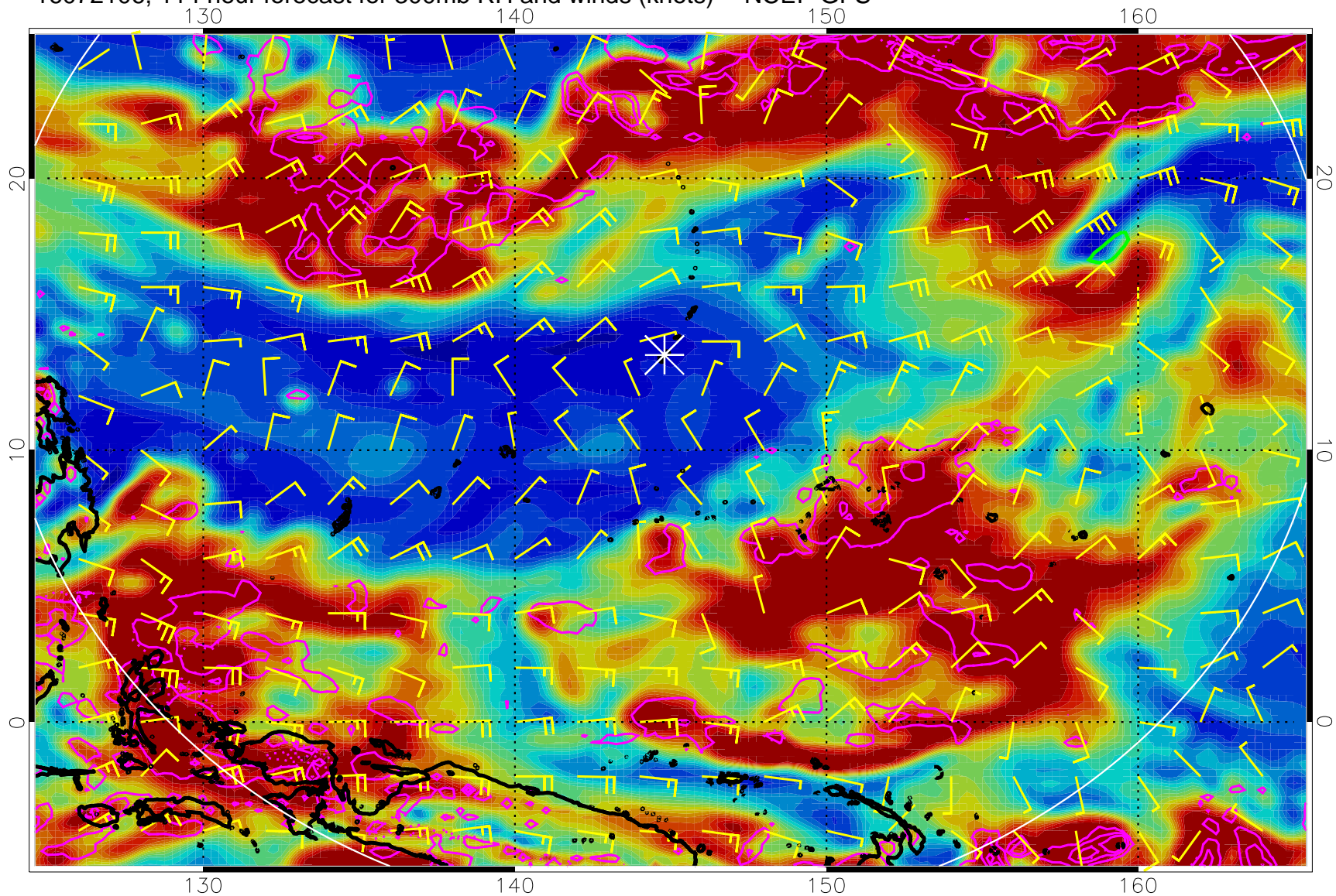
16072106, 114 hour forecast for 300mb RH and winds (knots) -- NCEP GFS
