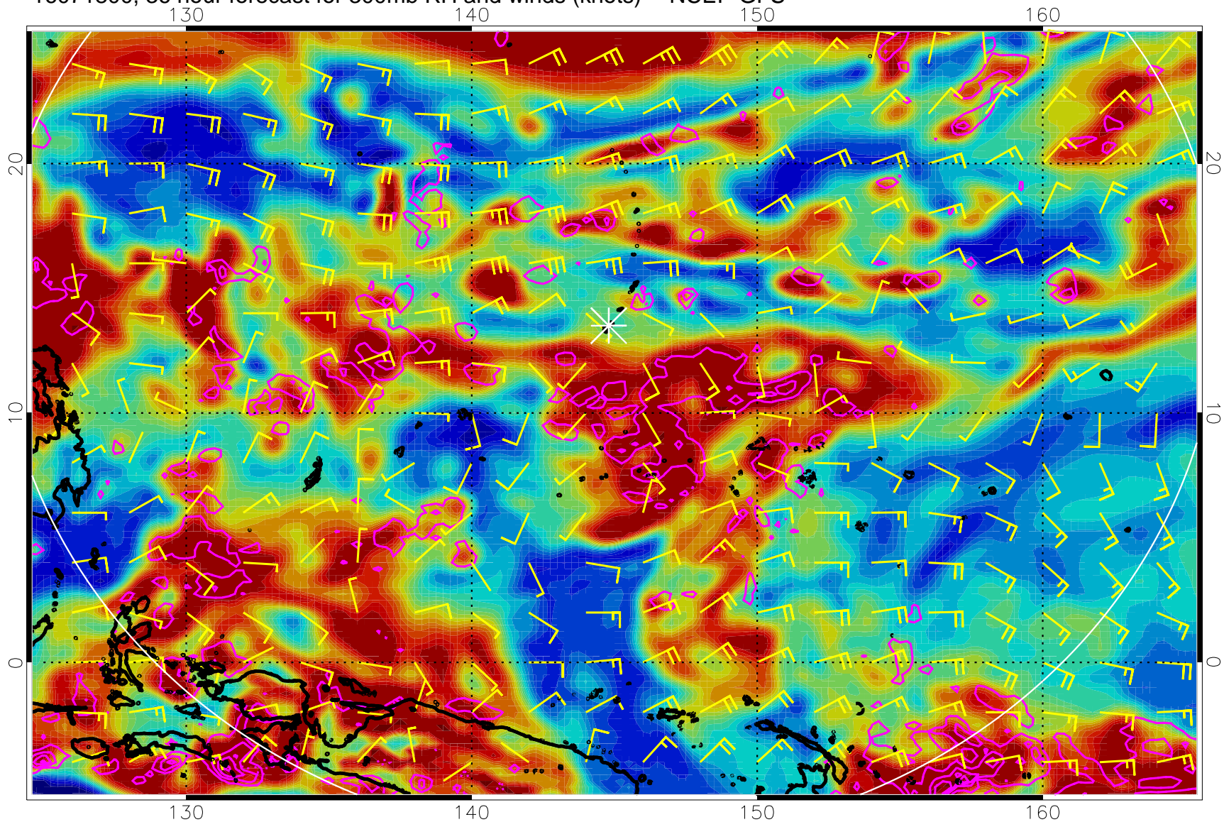
16071800, 36 hour forecast for 300mb RH and winds (knots) -- NCEP GFS
