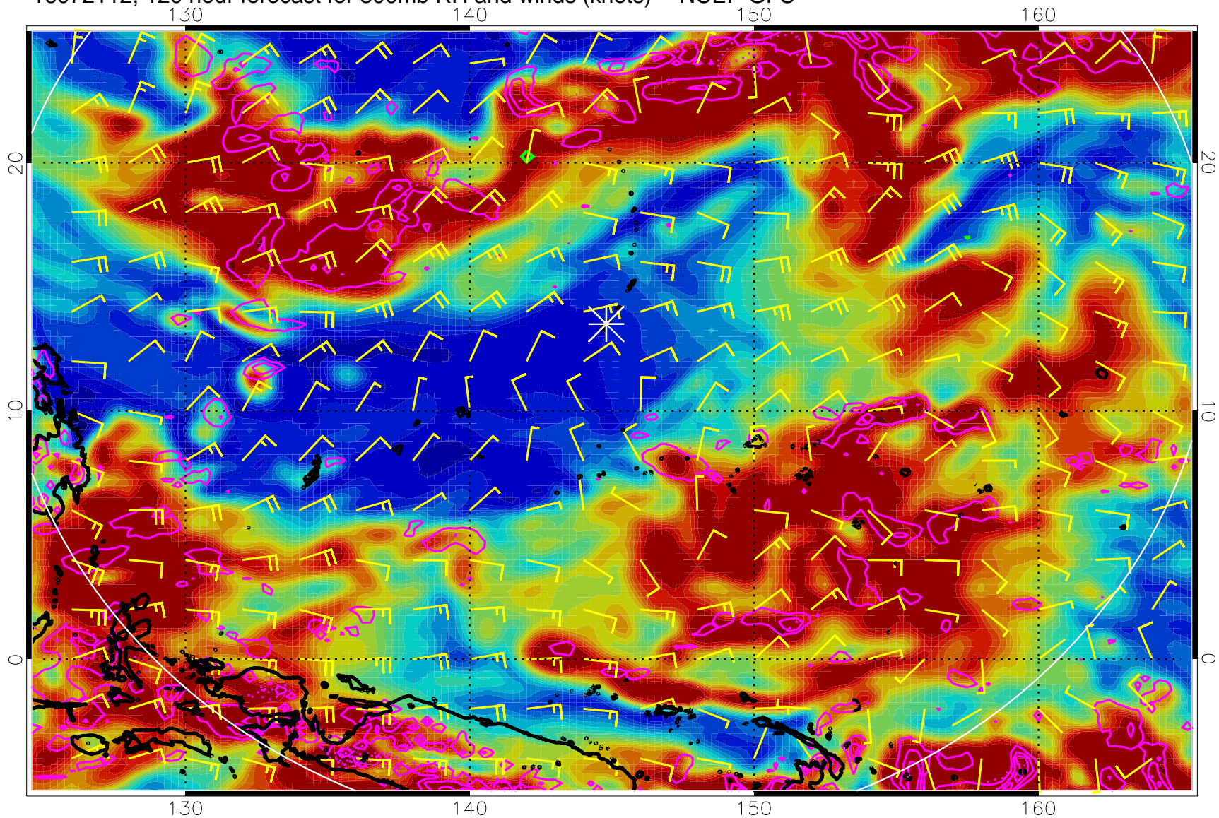
16072112, 120 hour forecast for 300mb RH and winds (knots) -- NCEP GFS
