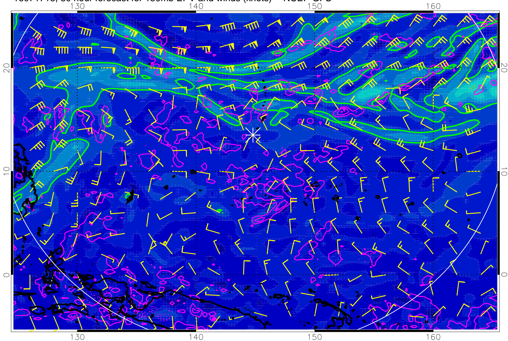
16071718, 30 hour forecast for 150mb EPV and winds (knots) -- NCEP GFS
