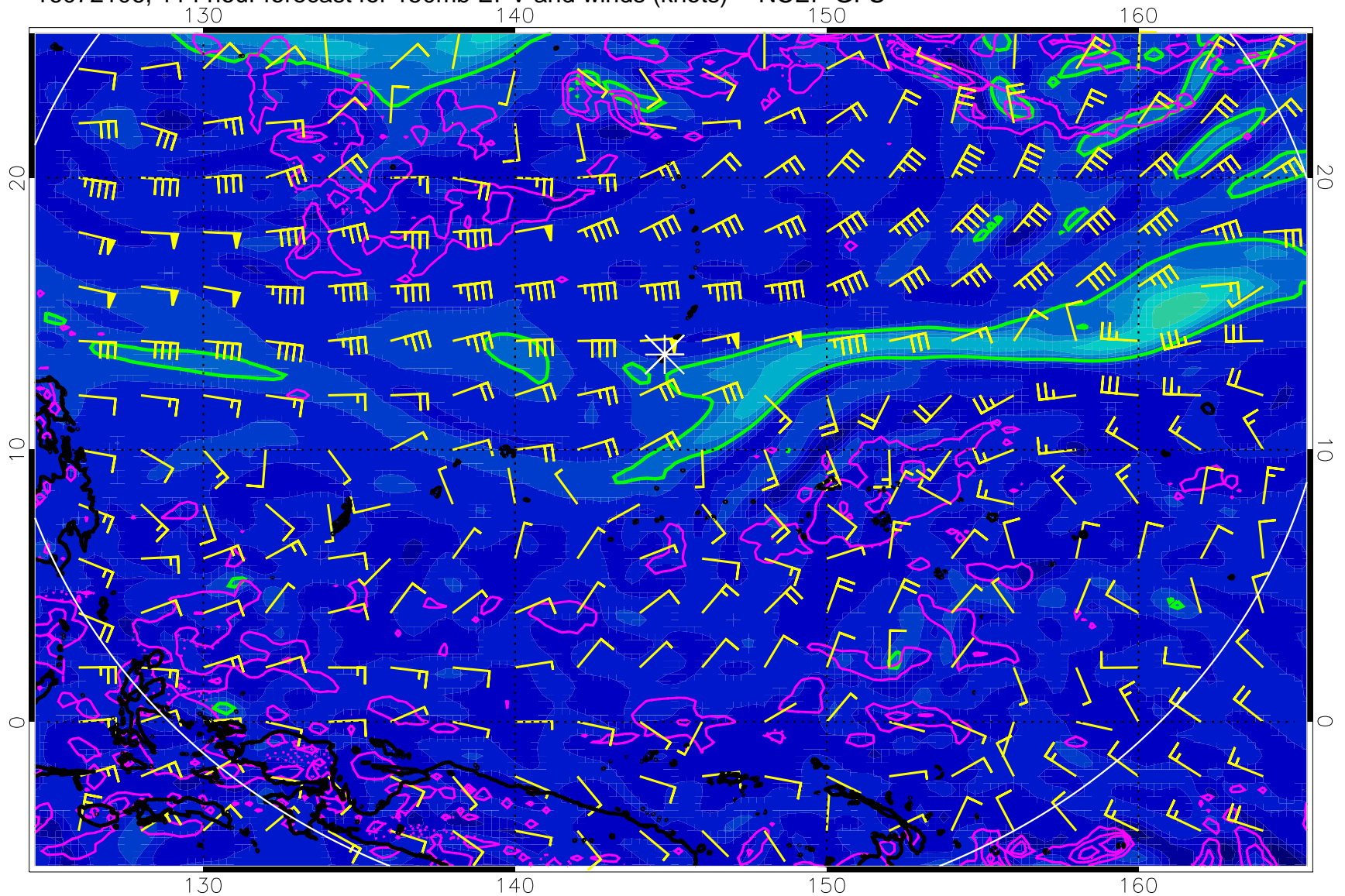
16072106, 114 hour forecast for 150mb EPV and winds (knots) -- NCEP GFS
