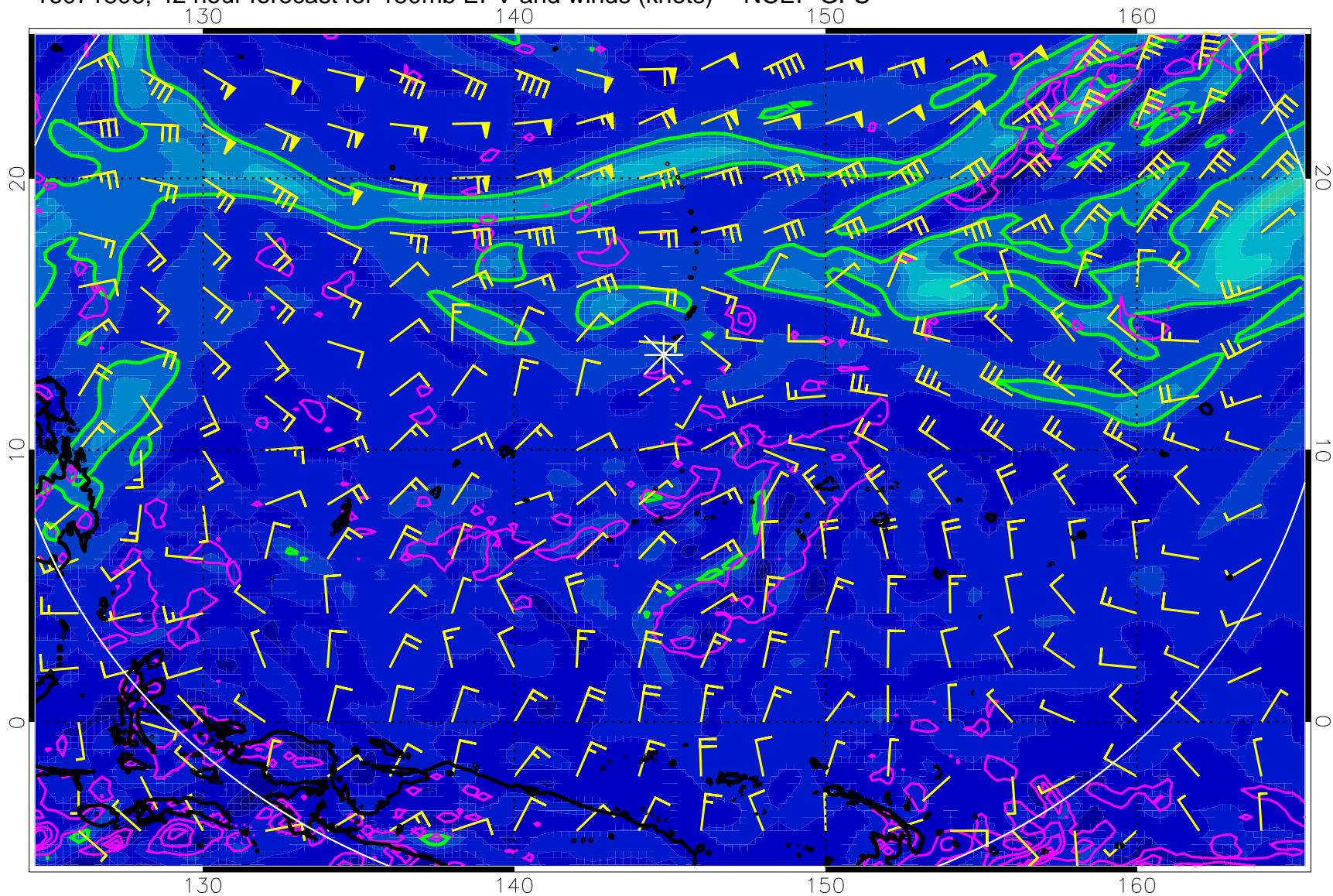
16071806, 42 hour forecast for 150mb EPV and winds (knots) -- NCEP GFS
