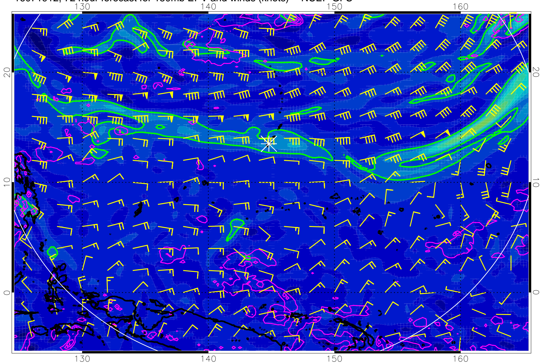
16071912, 72 hour forecast for 150mb EPV and winds (knots) -- NCEP GFS
