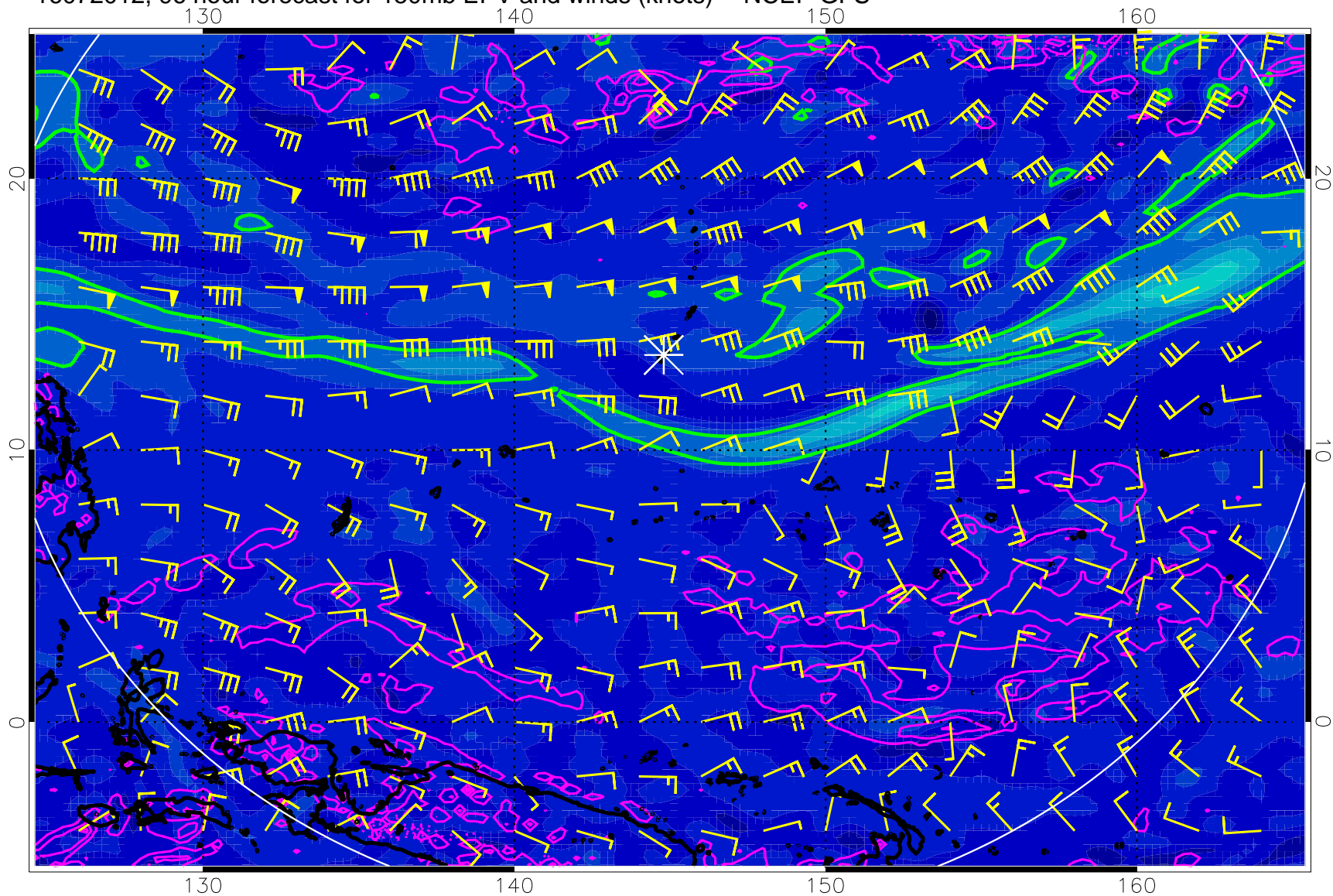
16072012, 96 hour forecast for 150mb EPV and winds (knots) -- NCEP GFS
