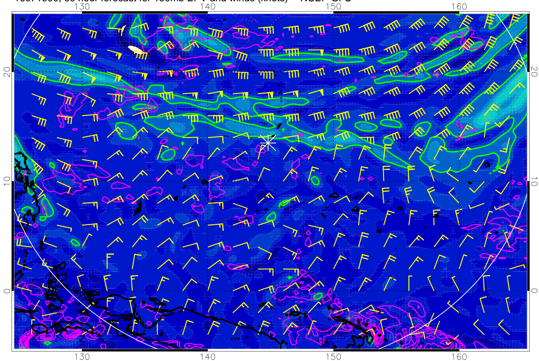
16071900, 60 hour forecast for 150mb EPV and winds (knots) -- NCEP GFS
