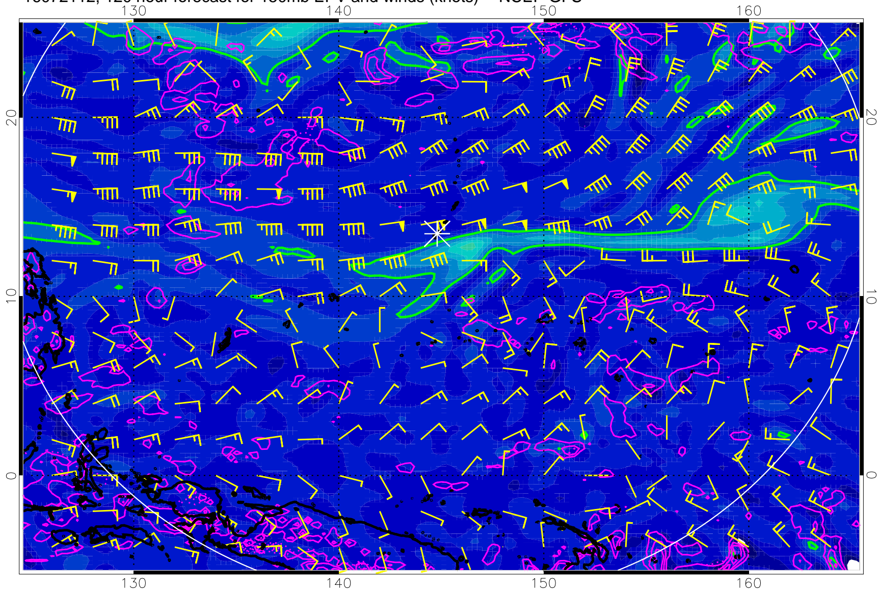
16072112, 120 hour forecast for 150mb EPV and winds (knots) -- NCEP GFS
