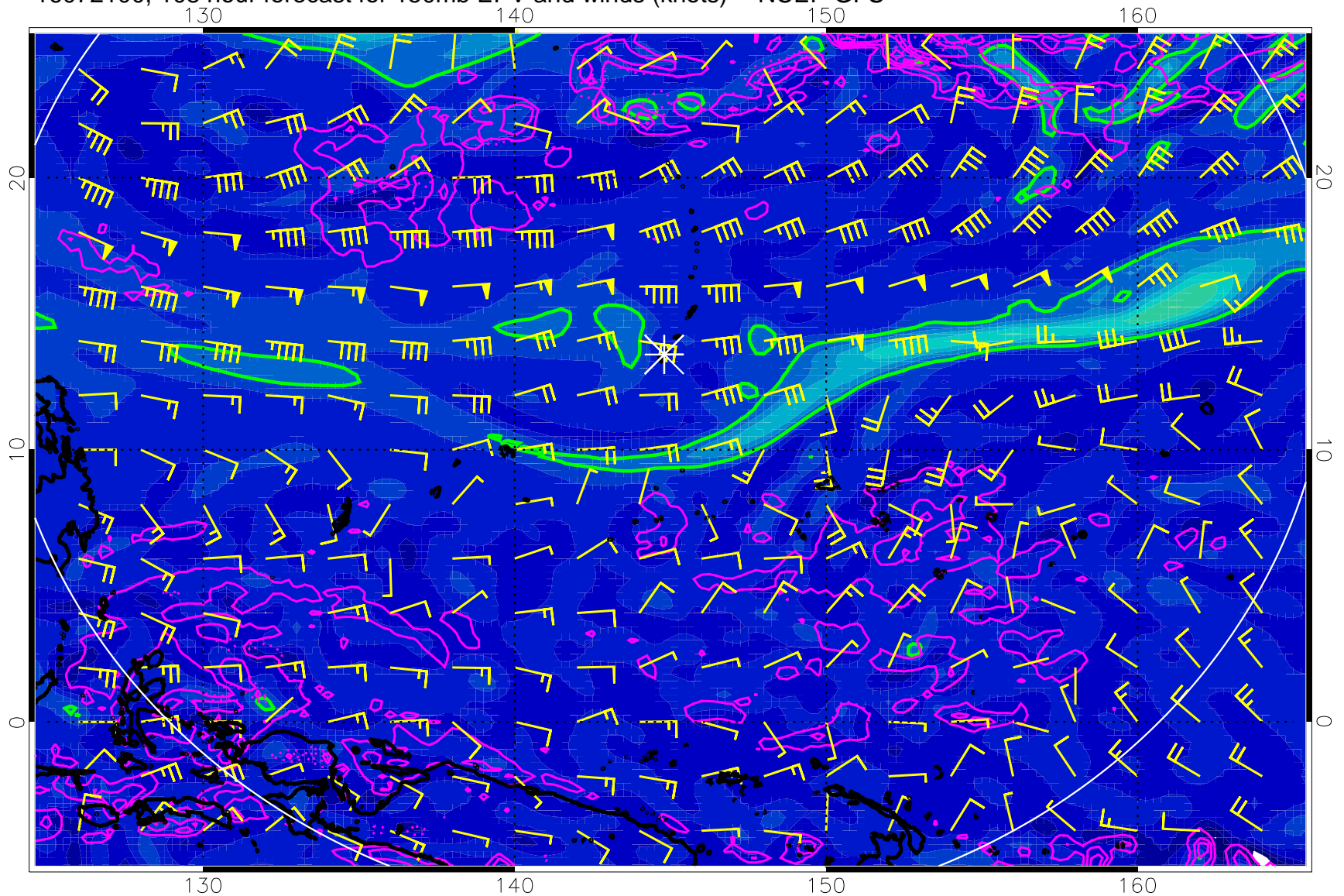
16072100, 108 hour forecast for 150mb EPV and winds (knots) -- NCEP GFS
