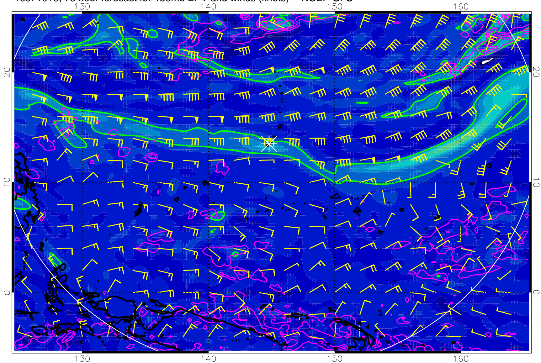
16071918, 78 hour forecast for 150mb EPV and winds (knots) -- NCEP GFS
