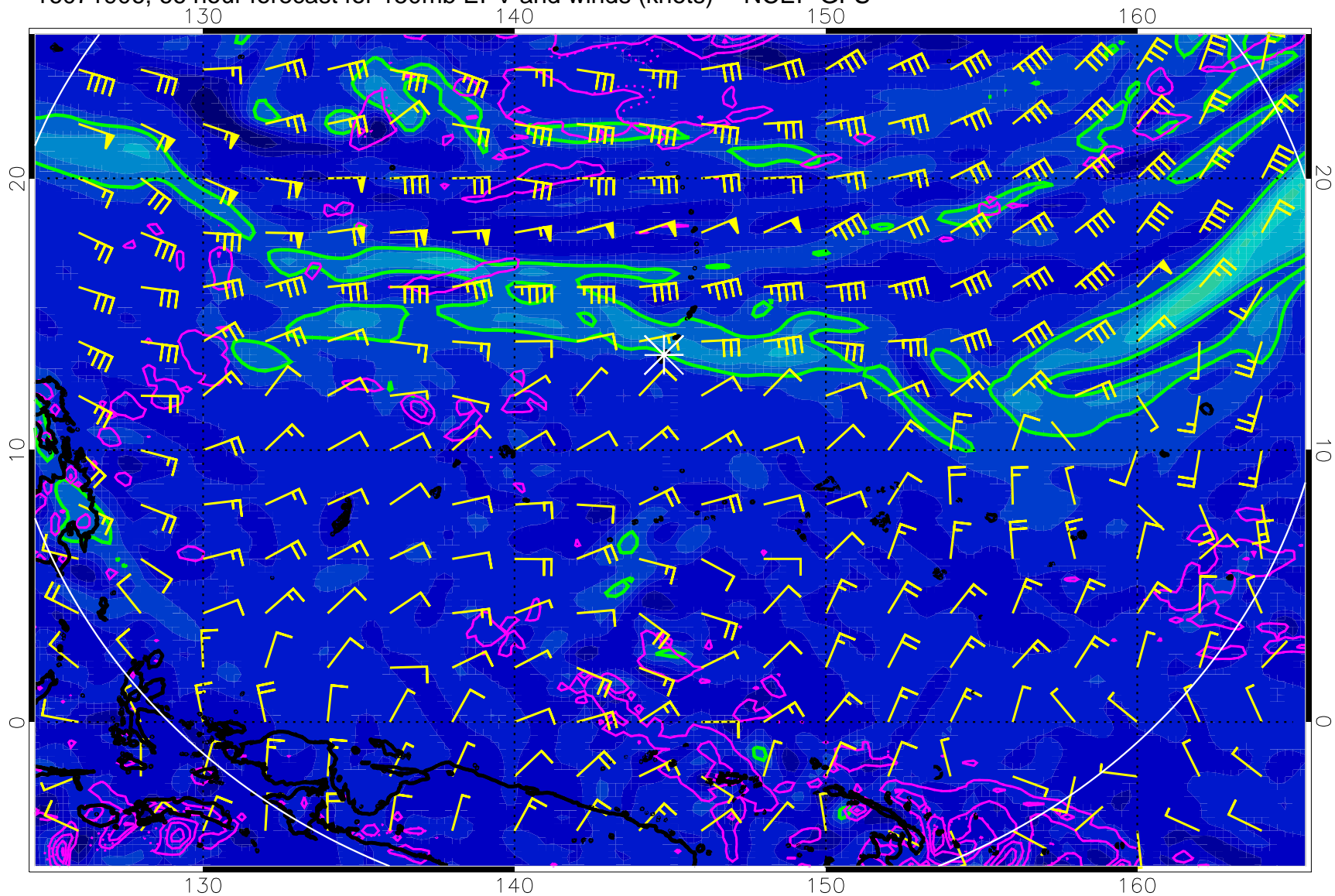
16071906, 66 hour forecast for 150mb EPV and winds (knots) -- NCEP GFS
