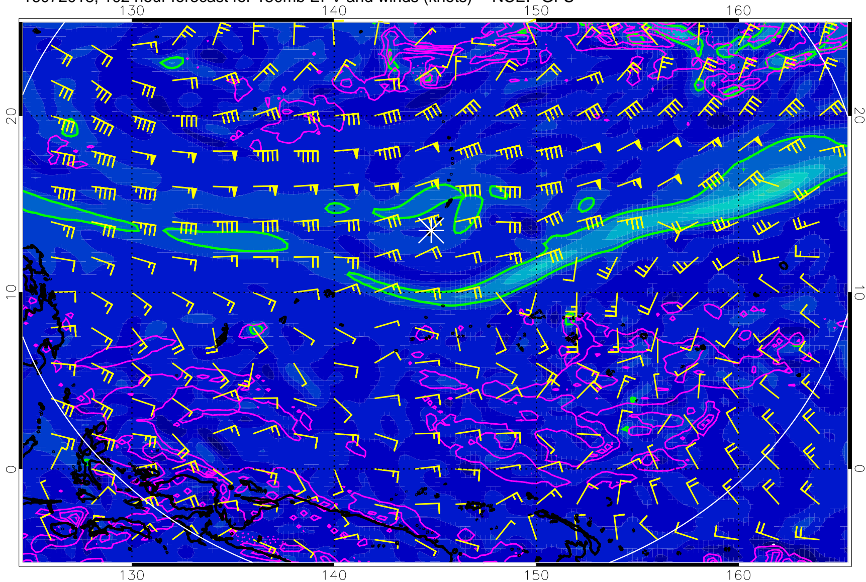
16072018, 102 hour forecast for 150mb EPV and winds (knots) -- NCEP GFS
