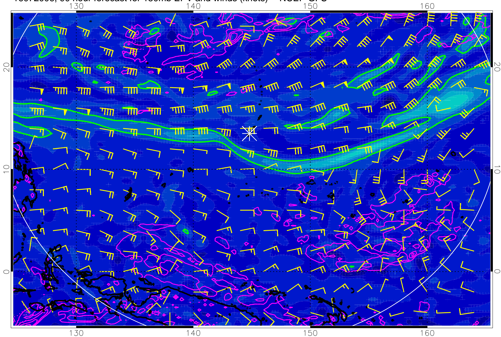
16072006, 90 hour forecast for 150mb EPV and winds (knots) -- NCEP GFS
