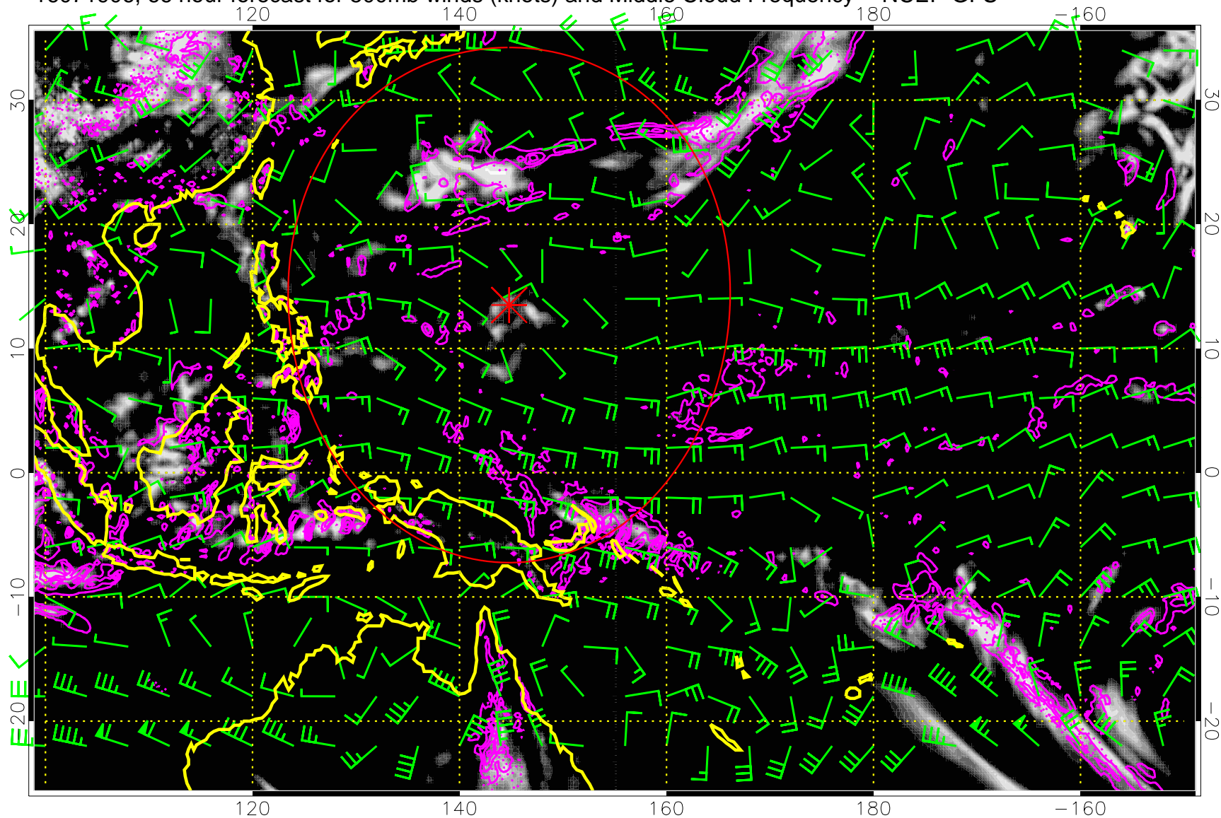
16071906, 66 hour forecast for 500mb winds (knots) and Middle Cloud Frequency -- NCEP GFS
