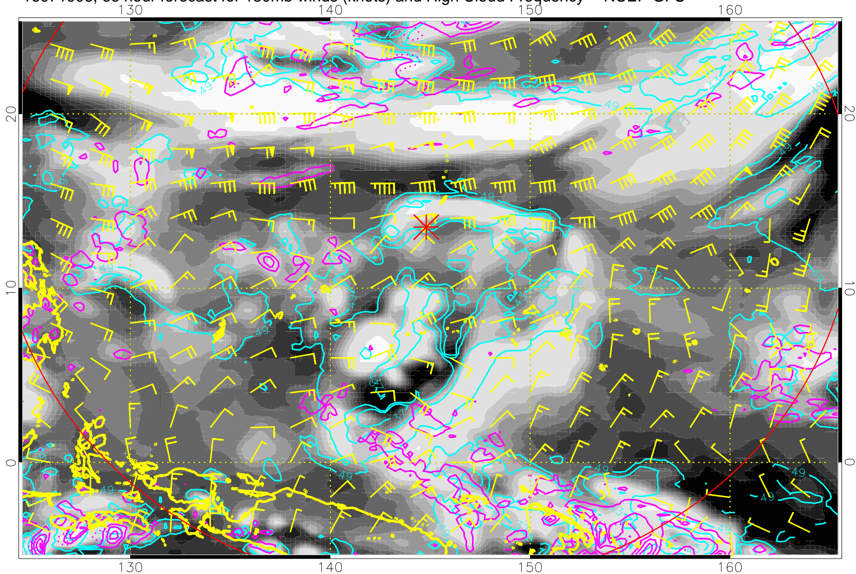
16071906, 66 hour forecast for 150mb winds (knots) and High Cloud Frequency -- NCEP GFS
