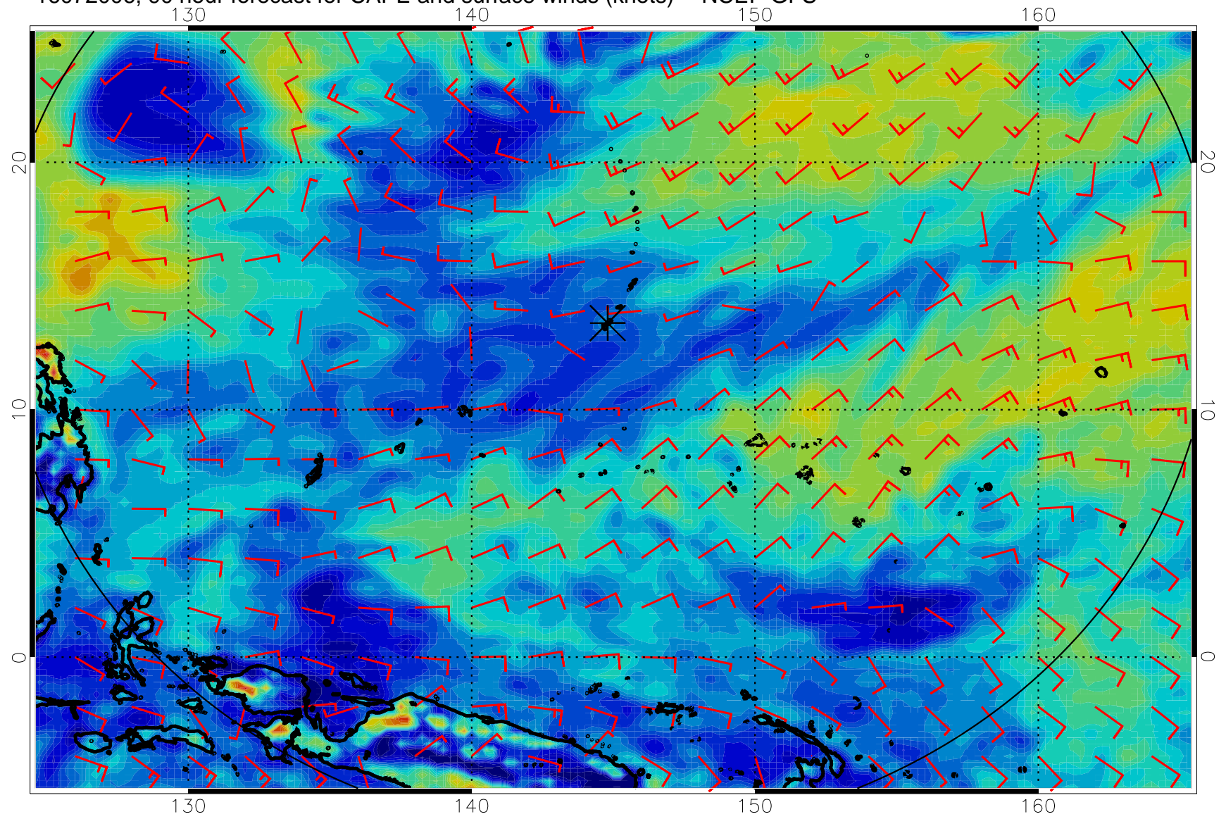
16072006, 90 hour forecast for CAPE and surface winds (knots) -- NCEP GFS
