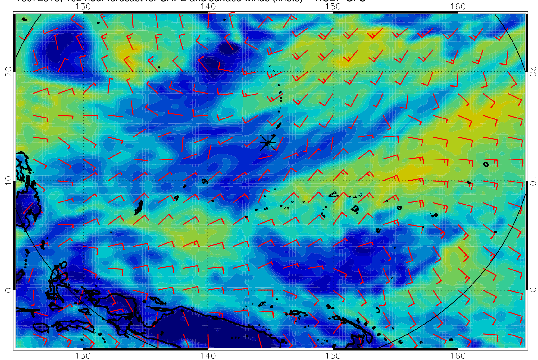
16072018, 102 hour forecast for CAPE and surface winds (knots) -- NCEP GFS
