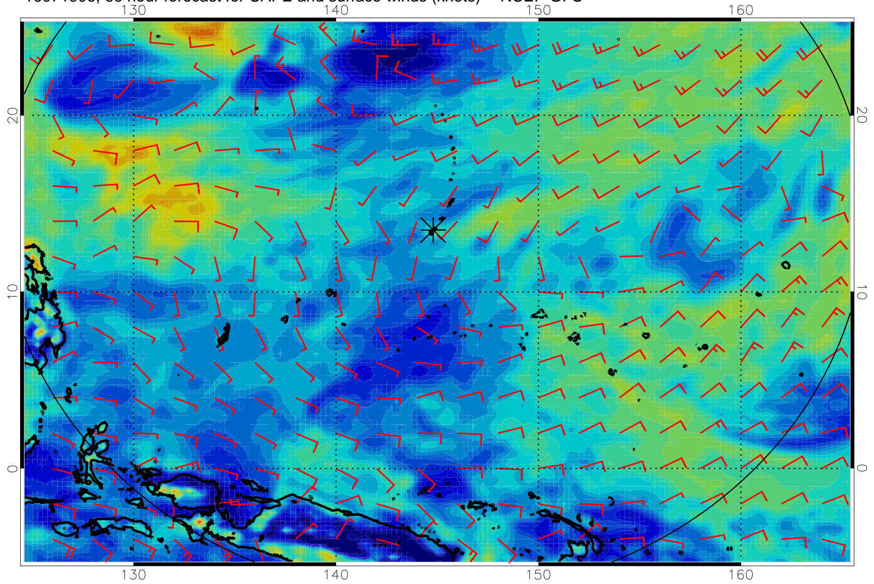
16071906, 66 hour forecast for CAPE and surface winds (knots) -- NCEP GFS
