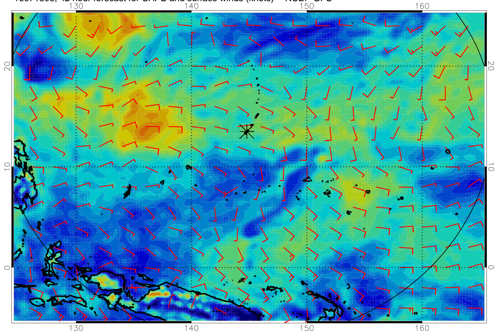
16071806, 42 hour forecast for CAPE and surface winds (knots) -- NCEP GFS
