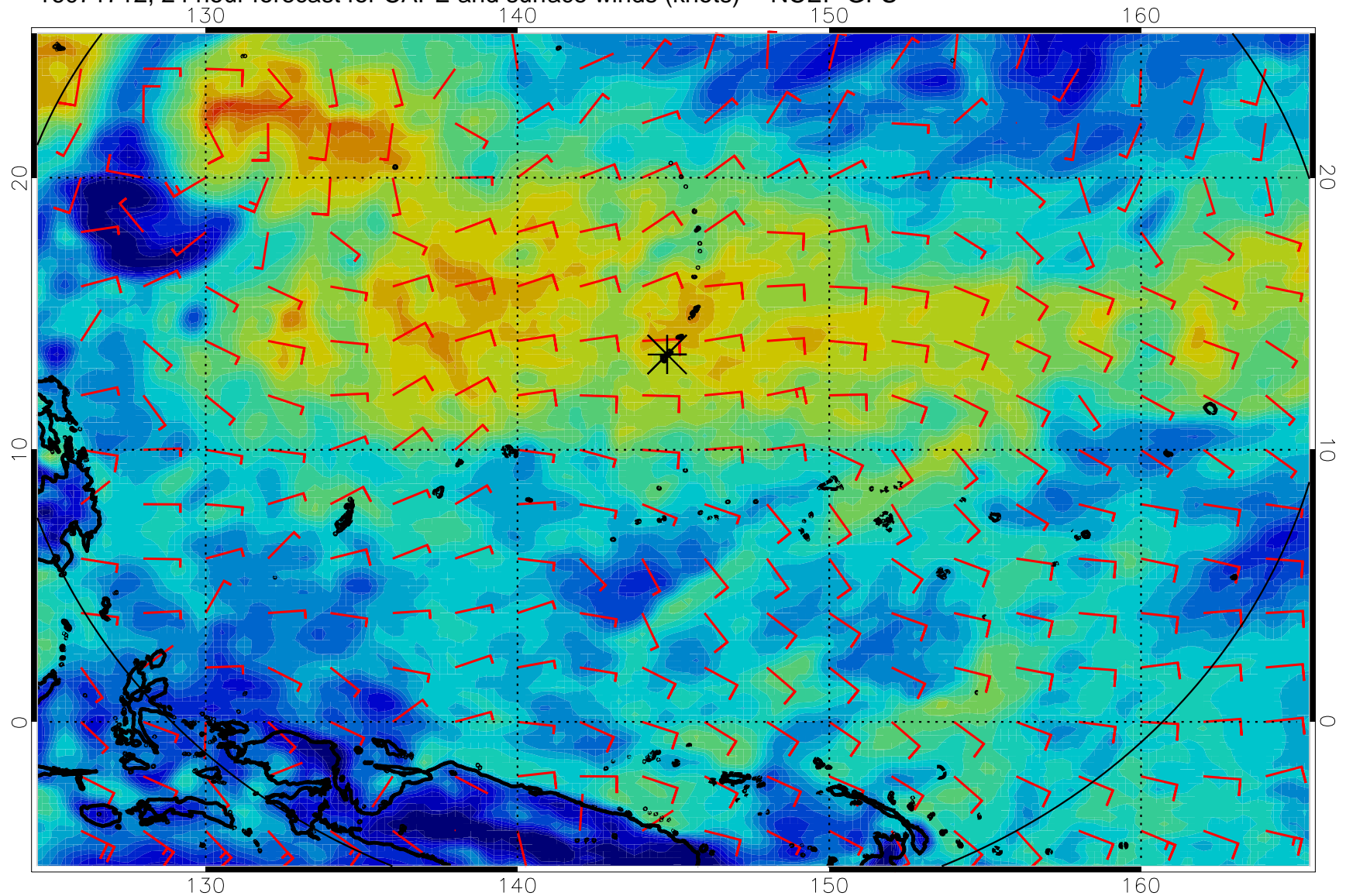
16071712, 24 hour forecast for CAPE and surface winds (knots) -- NCEP GFS
