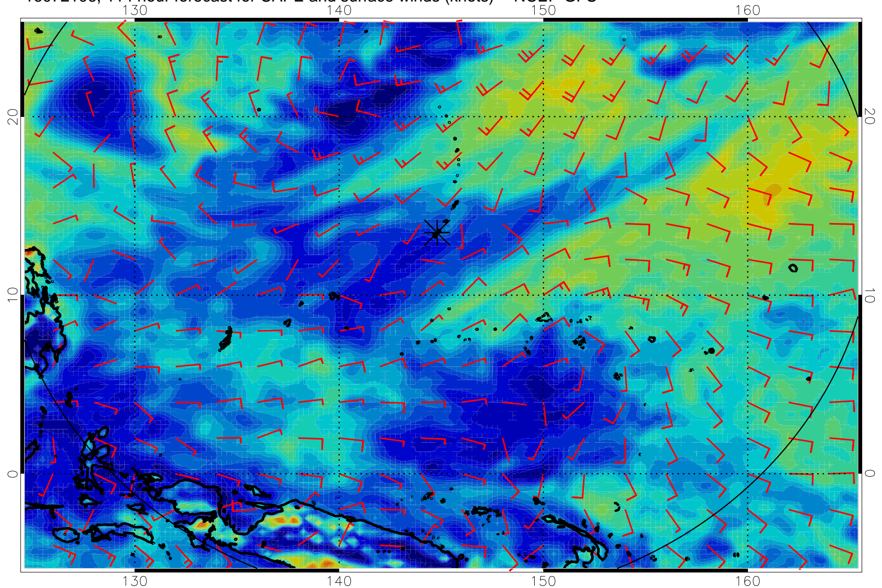
16072106, 114 hour forecast for CAPE and surface winds (knots) -- NCEP GFS
