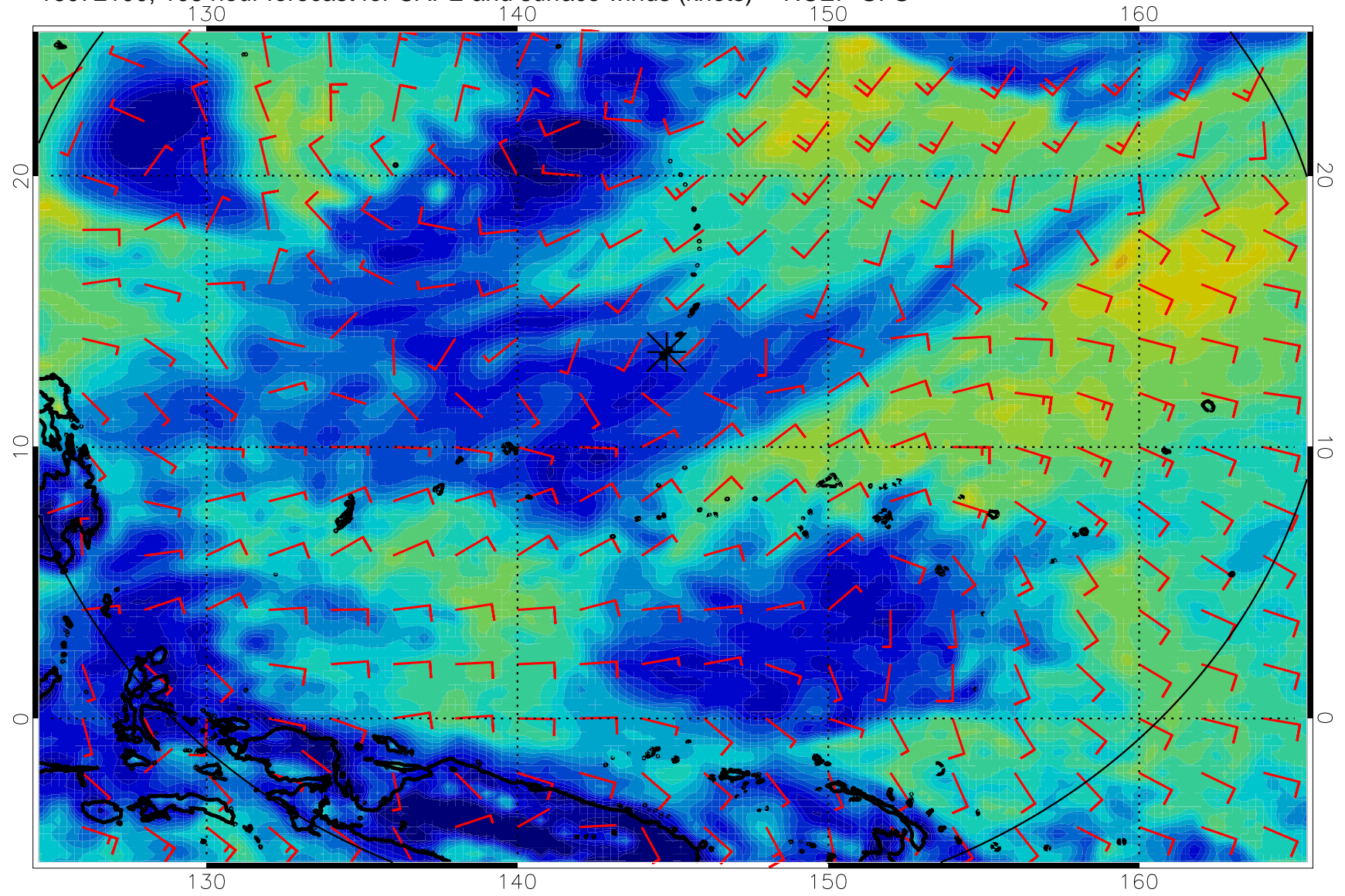
16072100, 108 hour forecast for CAPE and surface winds (knots) -- NCEP GFS
