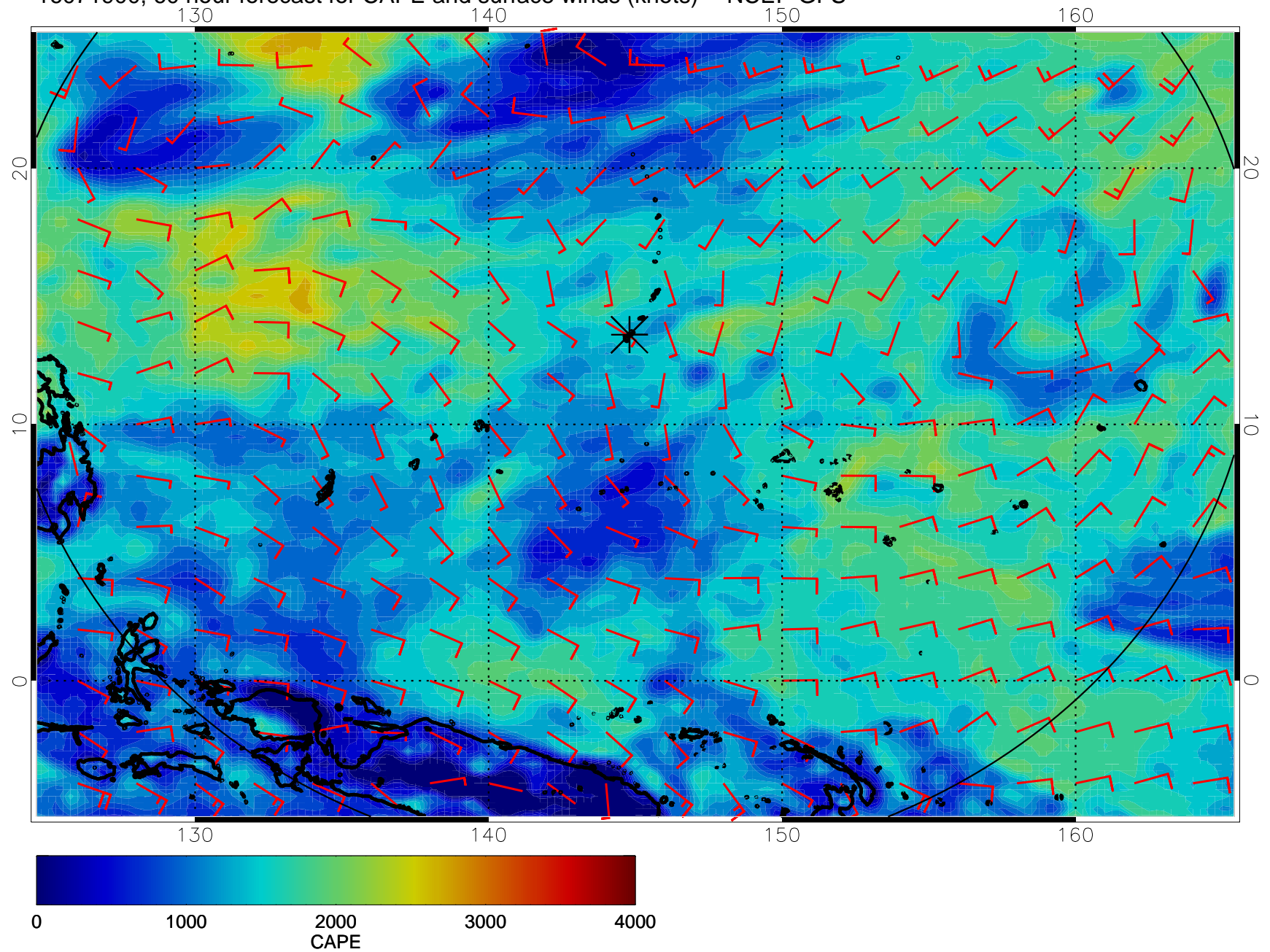
16071900, 60 hour forecast for CAPE and surface winds (knots) -- NCEP GFS
