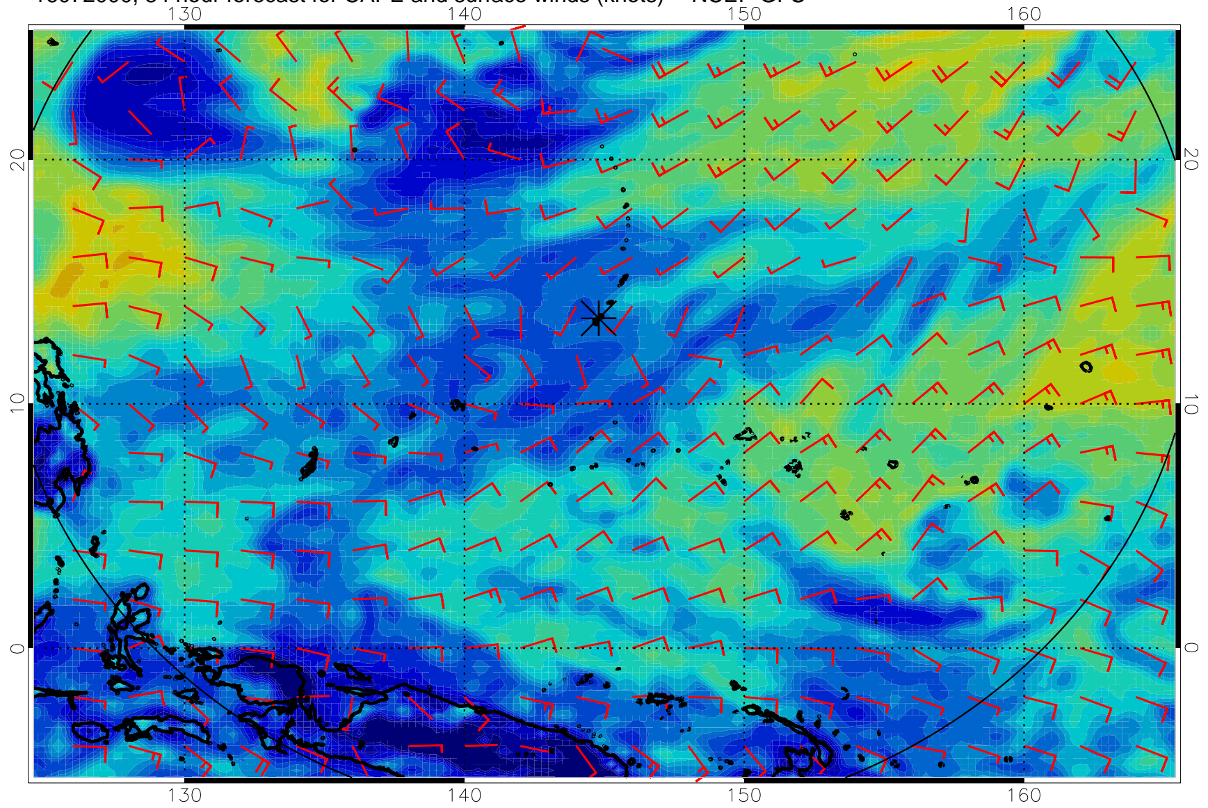
16072000, 84 hour forecast for CAPE and surface winds (knots) -- NCEP GFS
