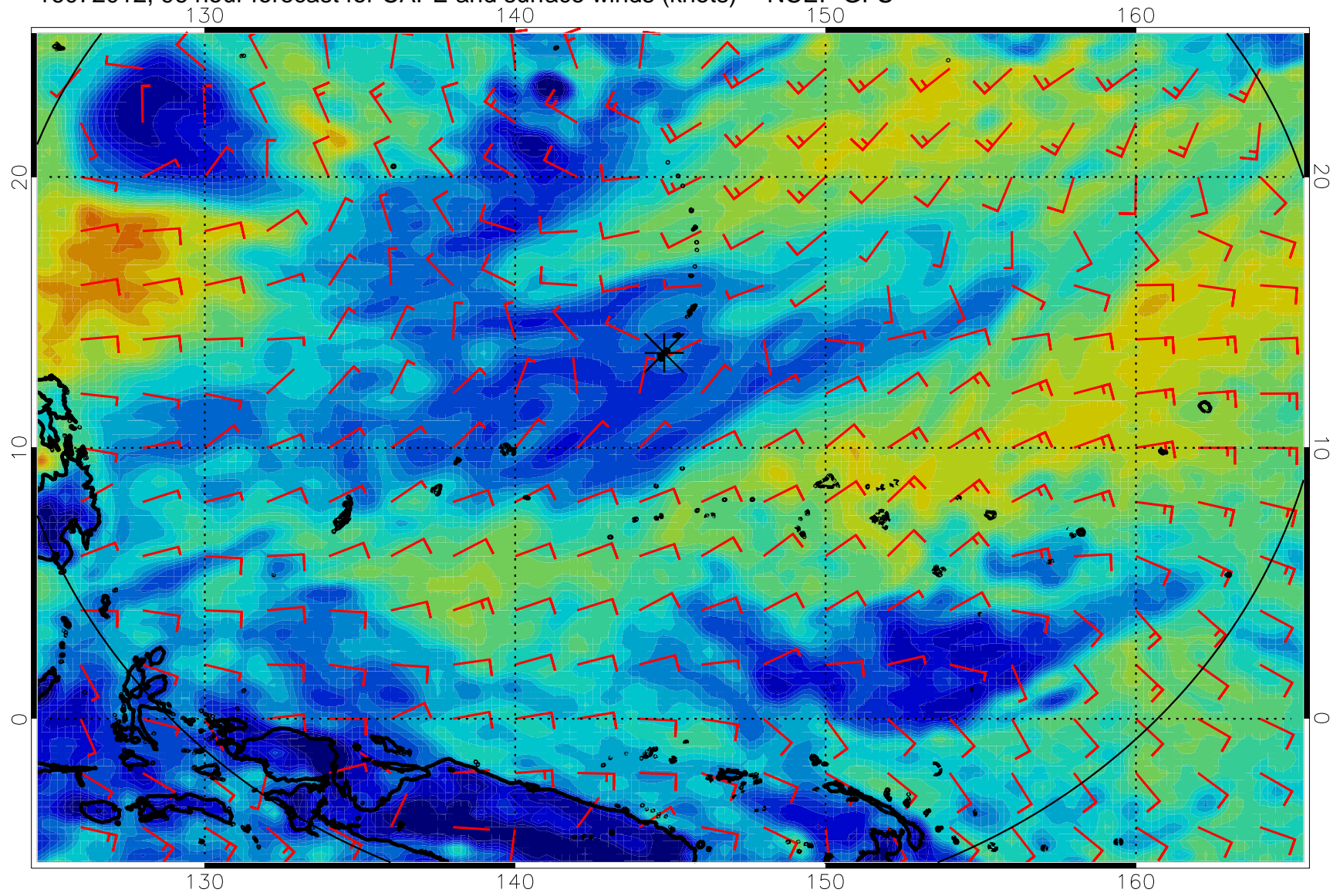
16072012, 96 hour forecast for CAPE and surface winds (knots) -- NCEP GFS
