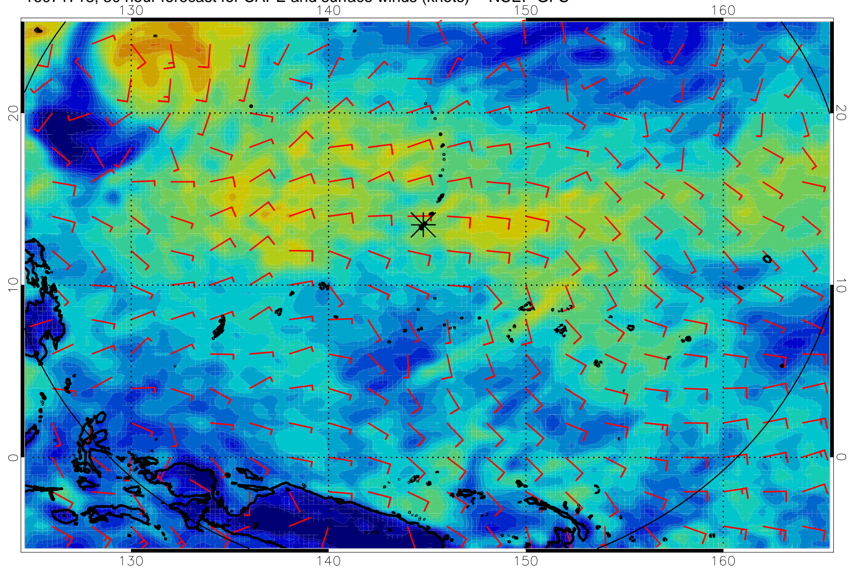
16071718, 30 hour forecast for CAPE and surface winds (knots) -- NCEP GFS
