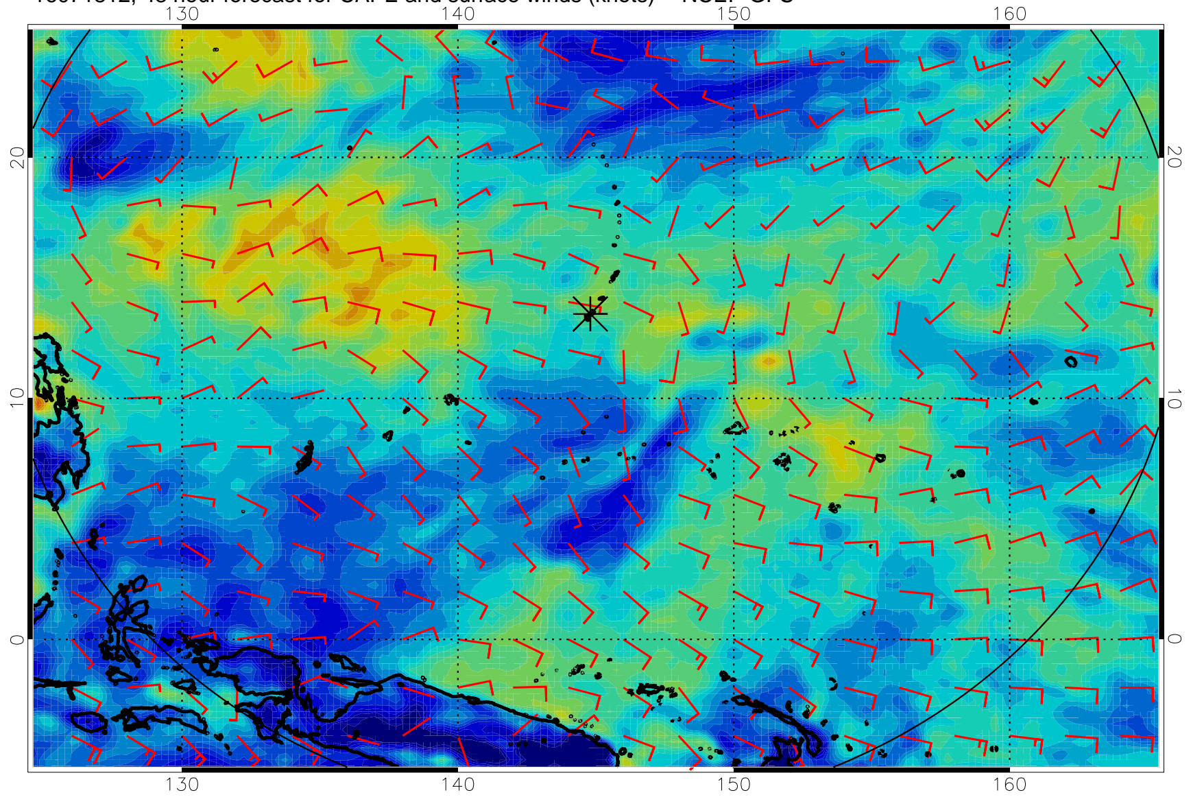
16071812, 48 hour forecast for CAPE and surface winds (knots) -- NCEP GFS
