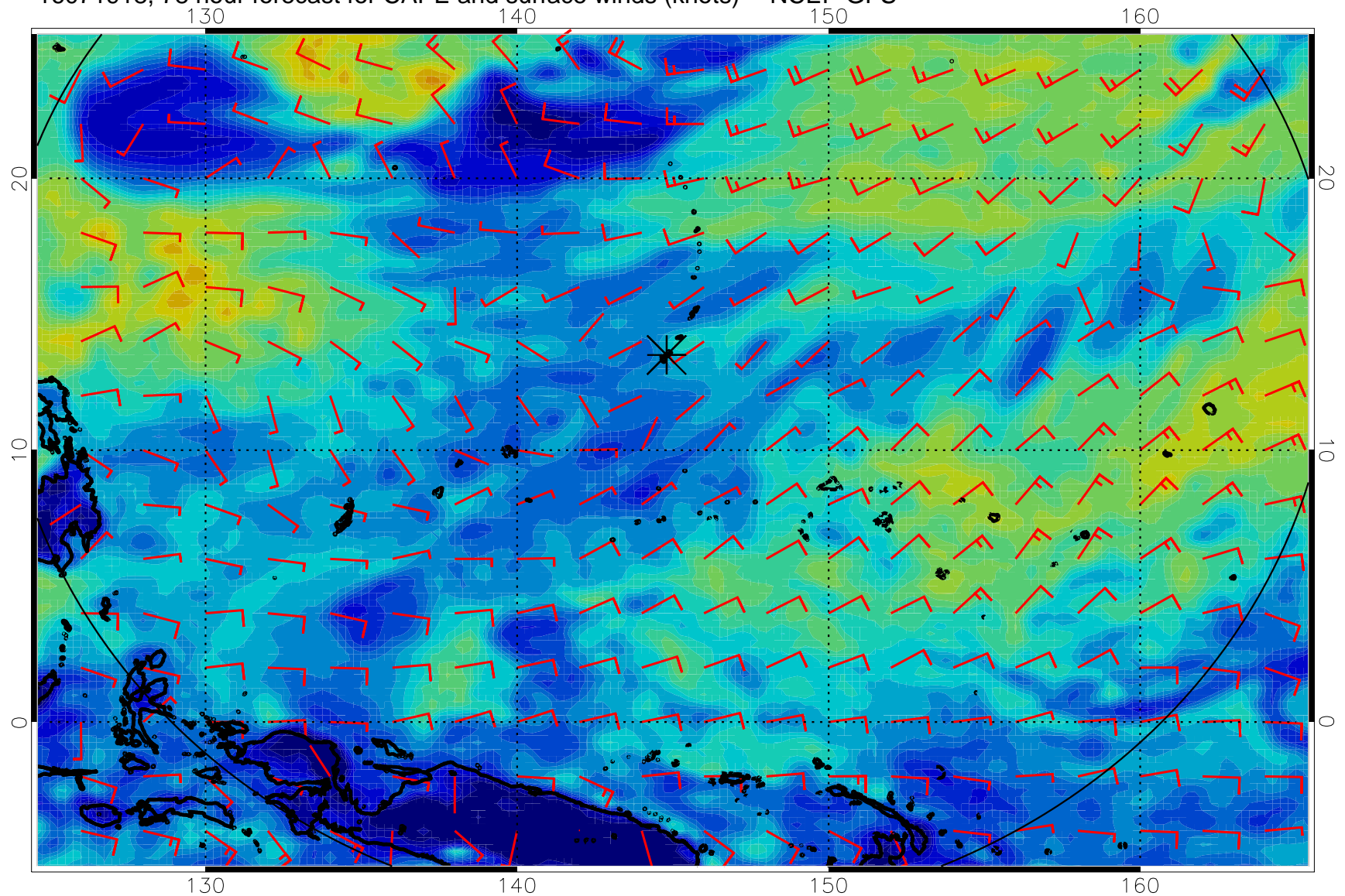
16071918, 78 hour forecast for CAPE and surface winds (knots) -- NCEP GFS
