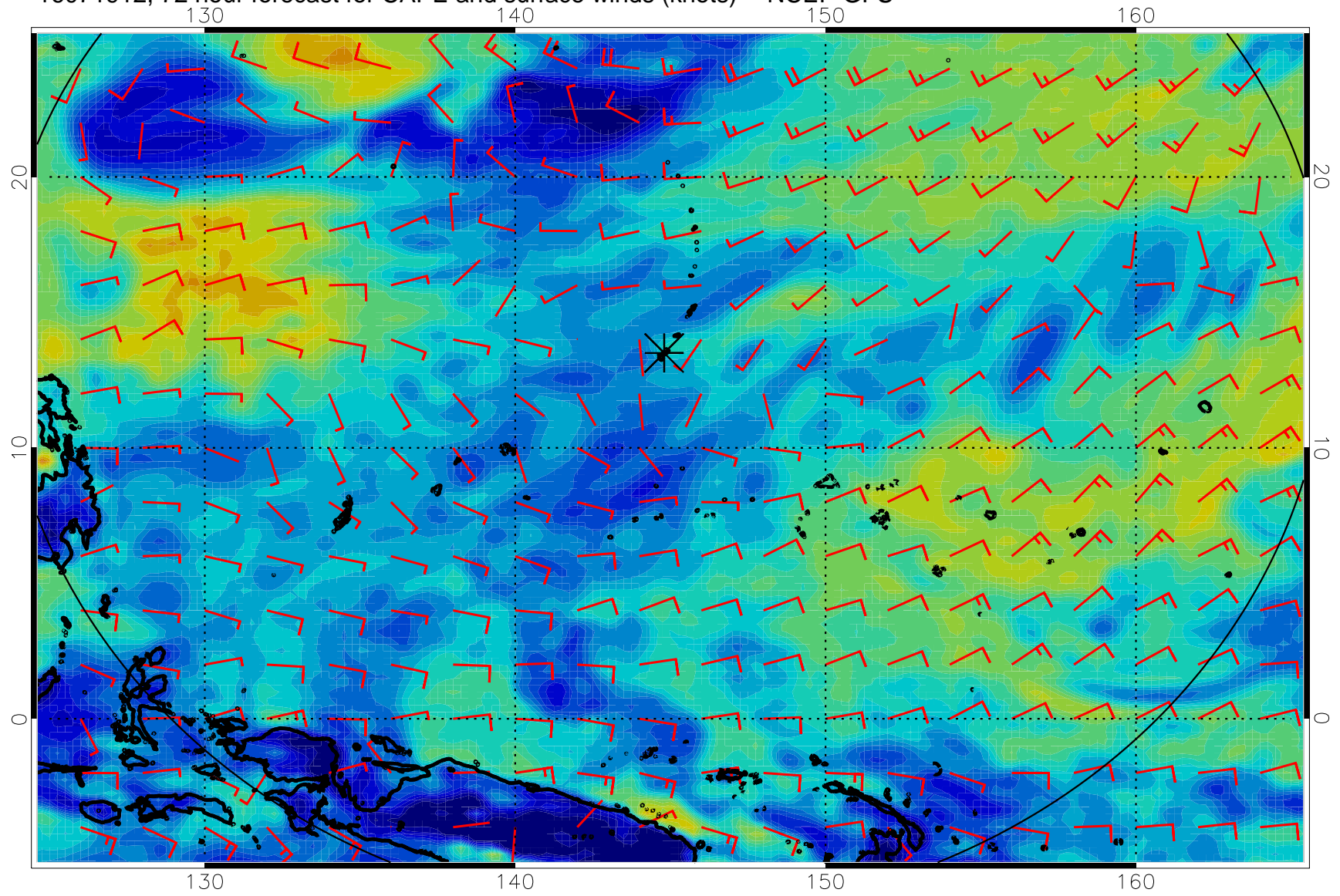
16071912, 72 hour forecast for CAPE and surface winds (knots) -- NCEP GFS
