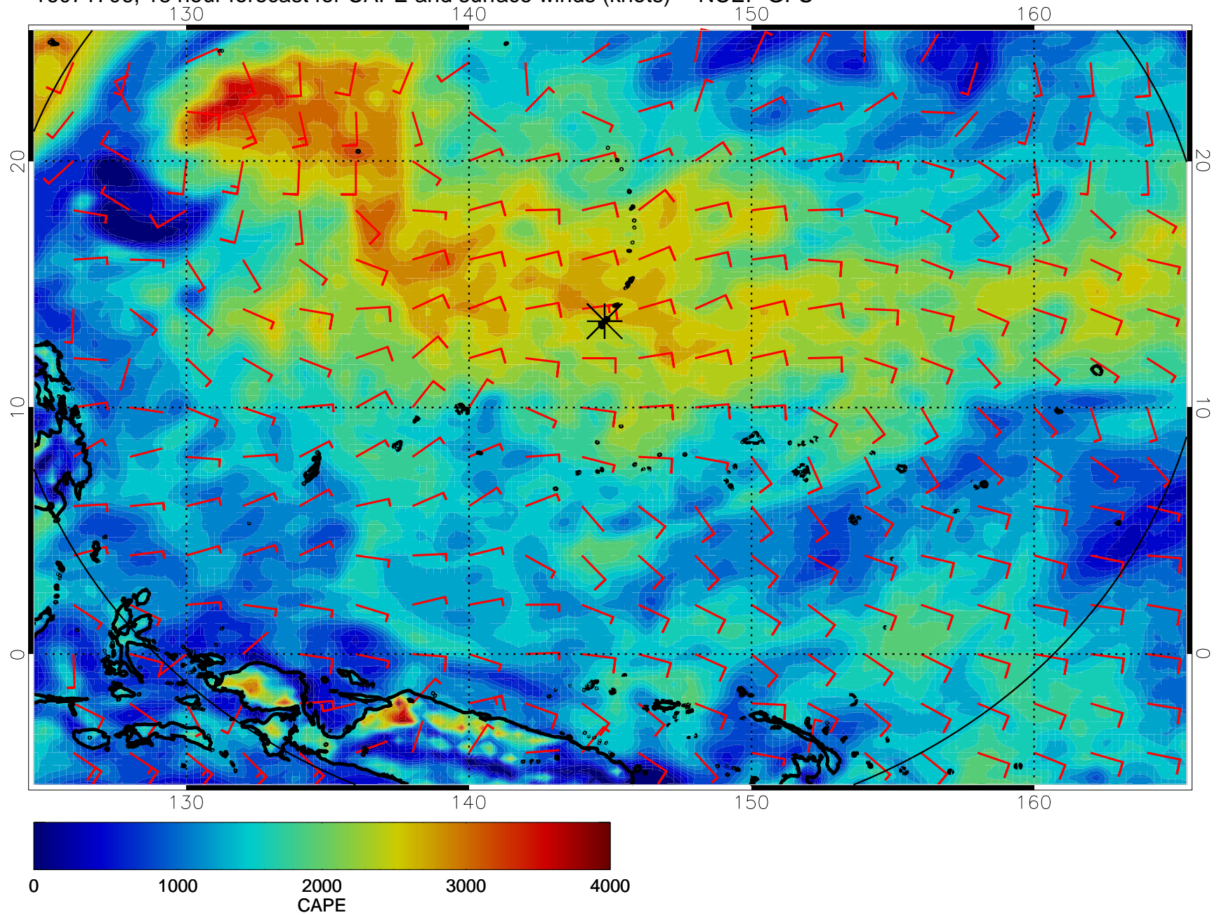
16071706, 18 hour forecast for CAPE and surface winds (knots) -- NCEP GFS
