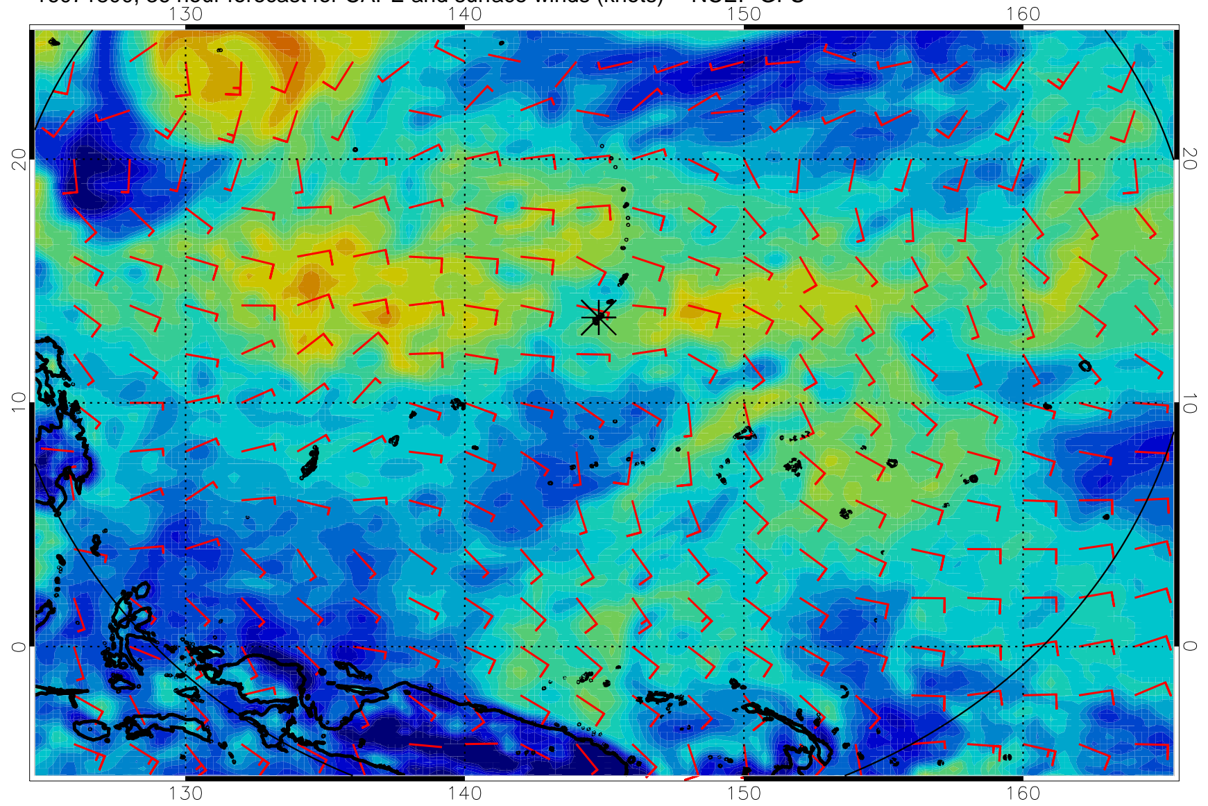
16071800, 36 hour forecast for CAPE and surface winds (knots) -- NCEP GFS
