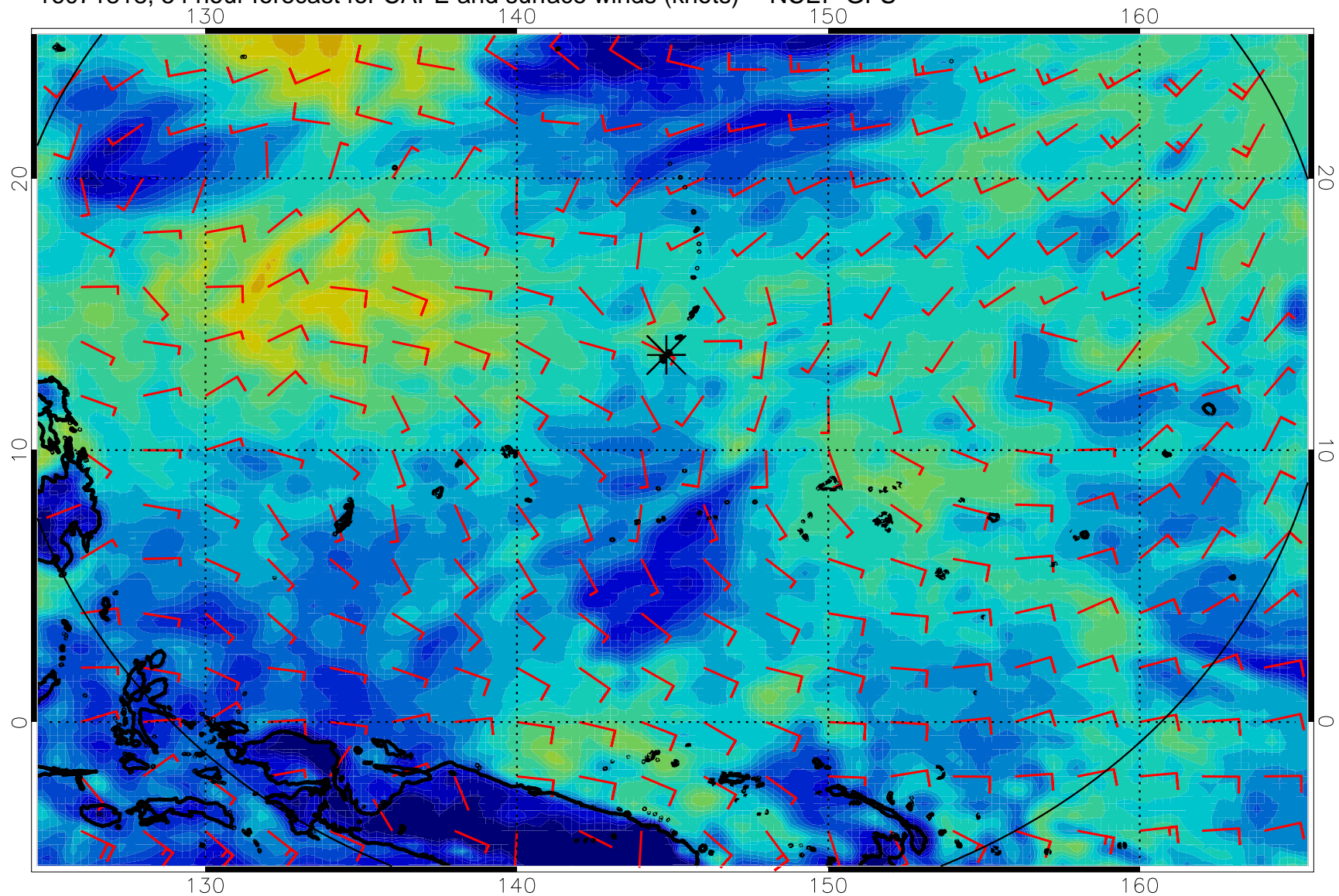
16071818, 54 hour forecast for CAPE and surface winds (knots) -- NCEP GFS
