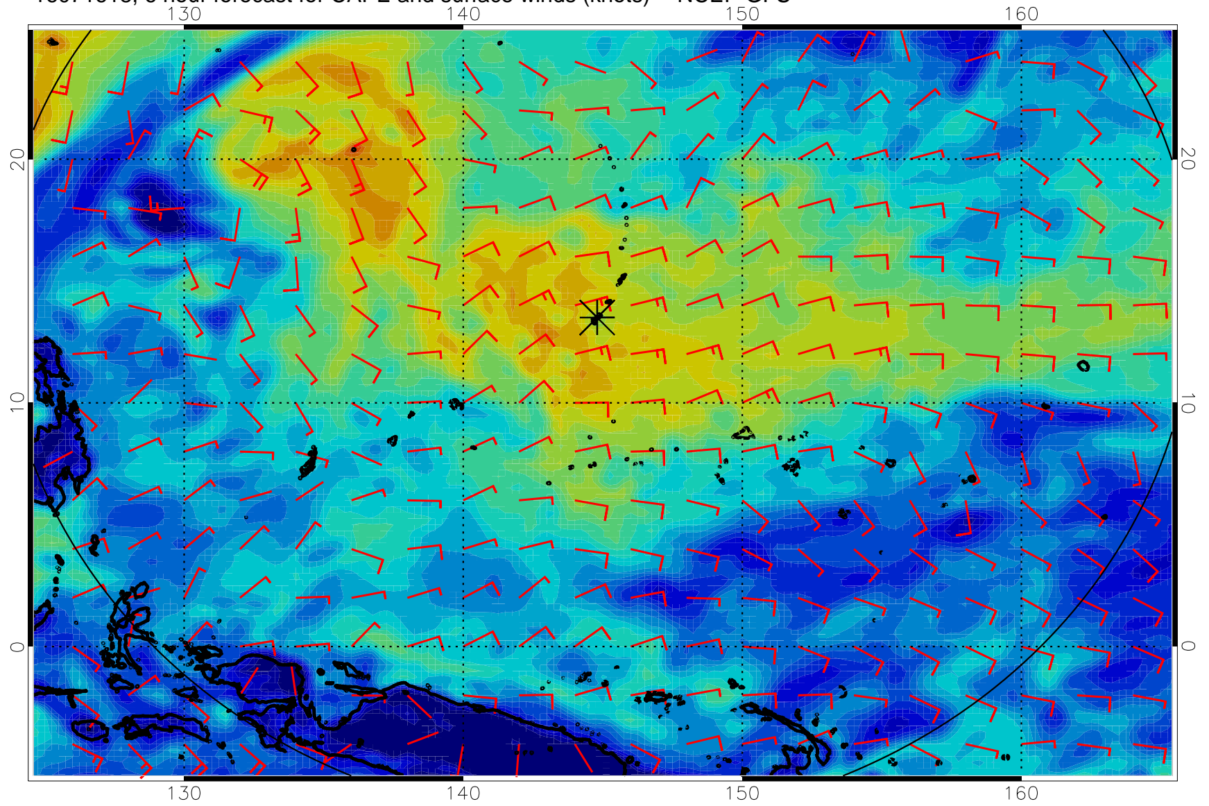
16071618, 6 hour forecast for CAPE and surface winds (knots) -- NCEP GFS
