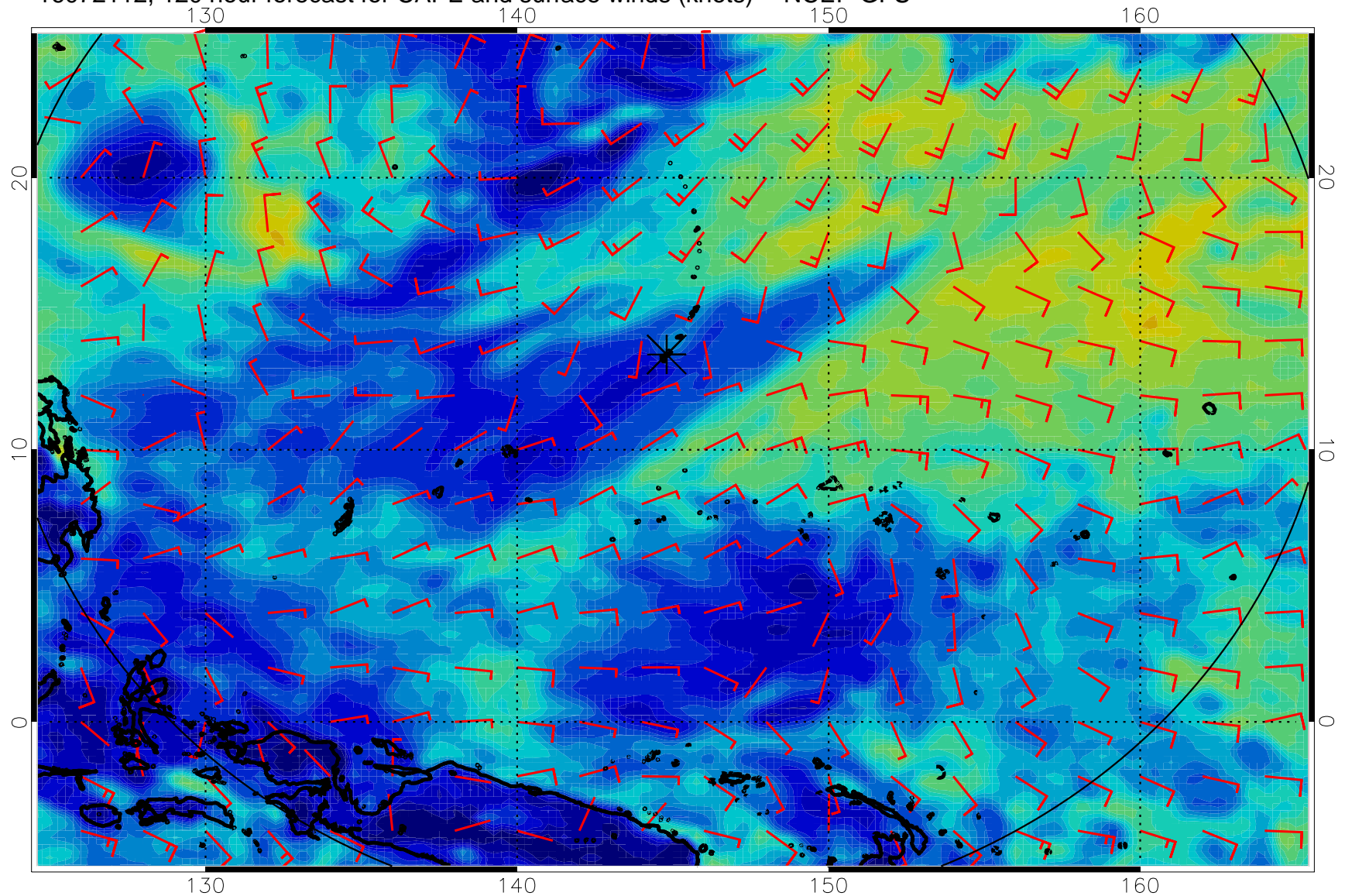
16072112, 120 hour forecast for CAPE and surface winds (knots) -- NCEP GFS
