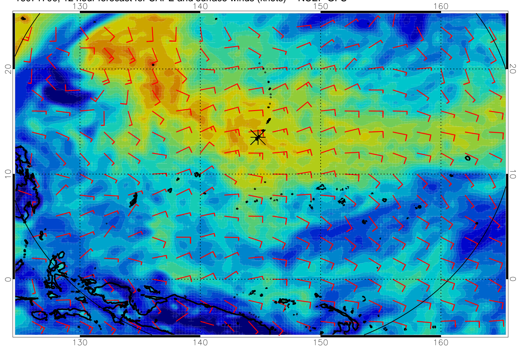
16071700, 12 hour forecast for CAPE and surface winds (knots) -- NCEP GFS
