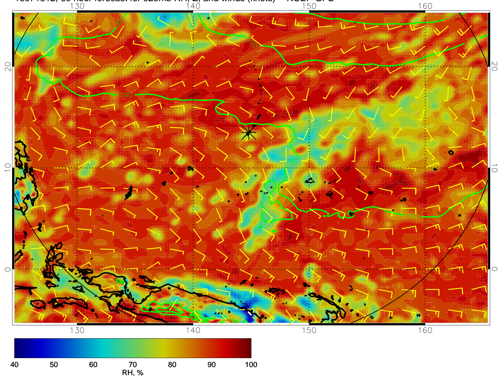
16071812, 60 hour forecast for 925mb RH, Z, and winds (knots) -- NCEP GFS
