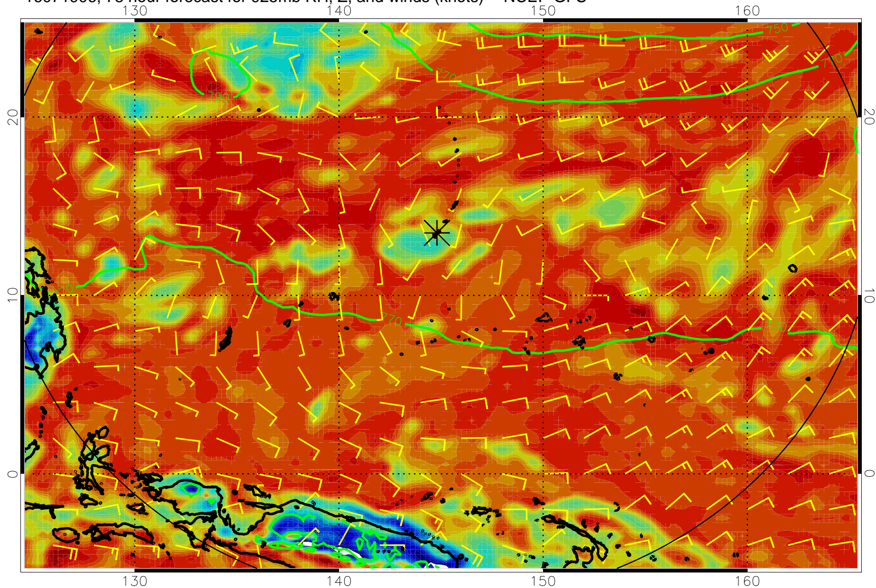
16071906, 78 hour forecast for 925mb RH, Z, and winds (knots) -- NCEP GFS
