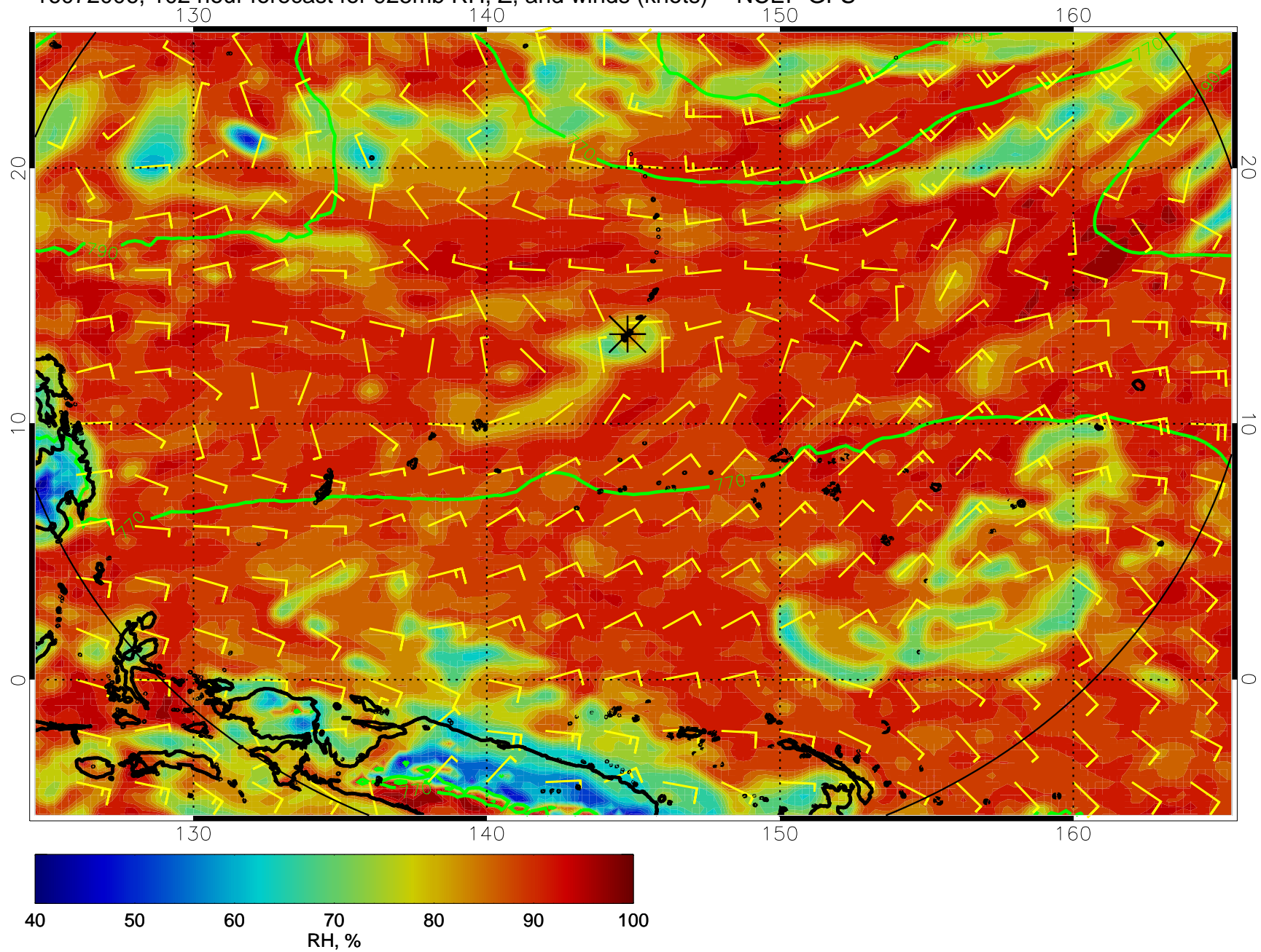
16072006, 102 hour forecast for 925mb RH, Z, and winds (knots) -- NCEP GFS
