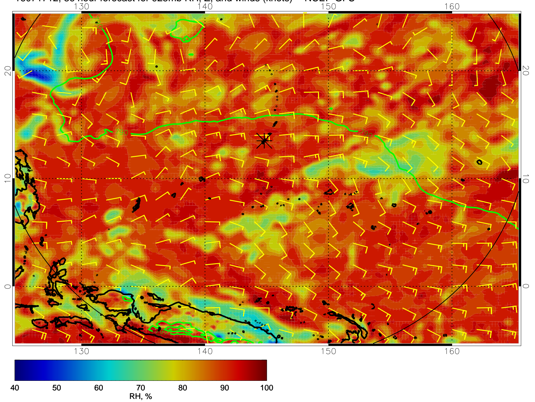
16071712, 36 hour forecast for 925mb RH, Z, and winds (knots) -- NCEP GFS
