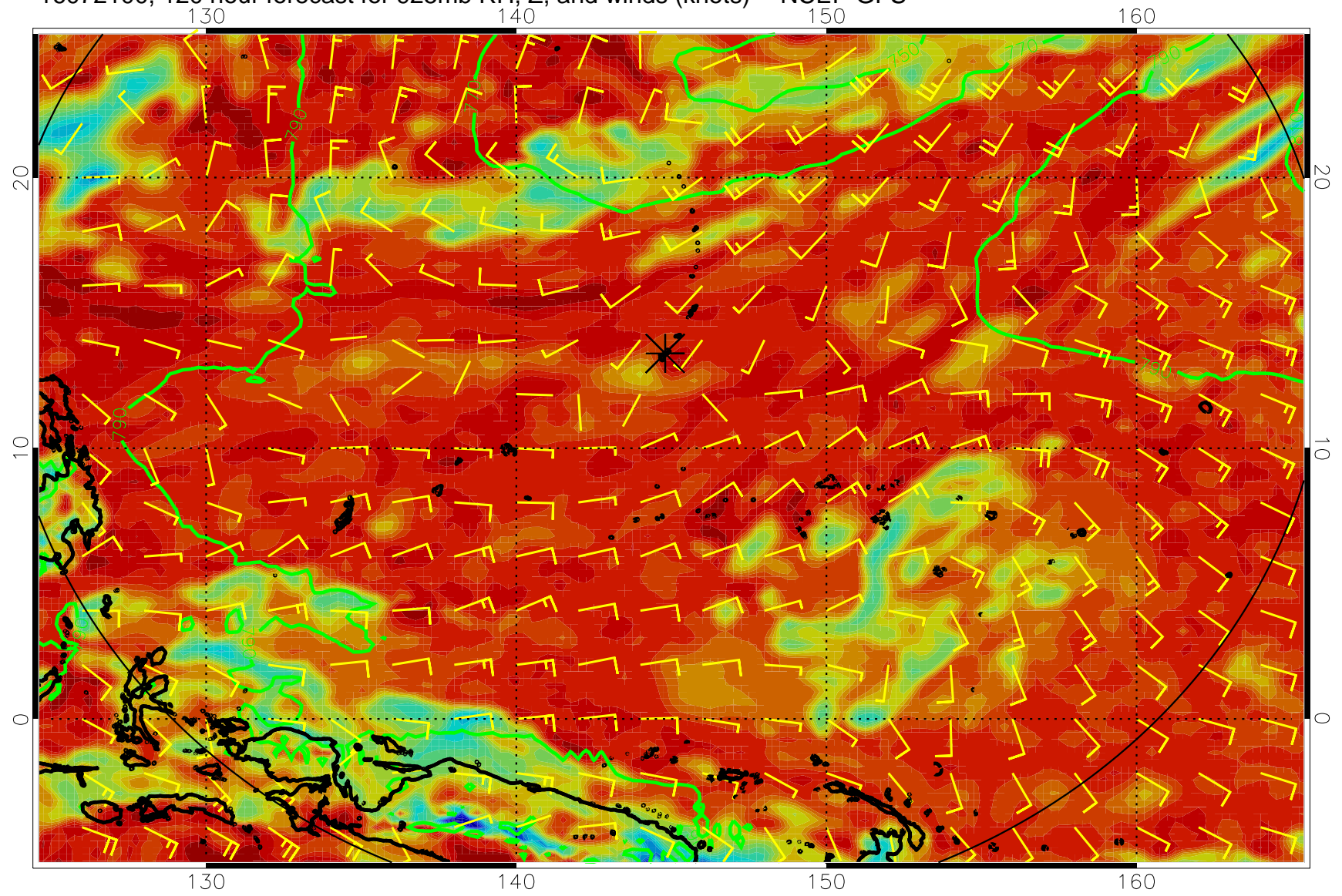
16072100, 120 hour forecast for 925mb RH, Z, and winds (knots) -- NCEP GFS
