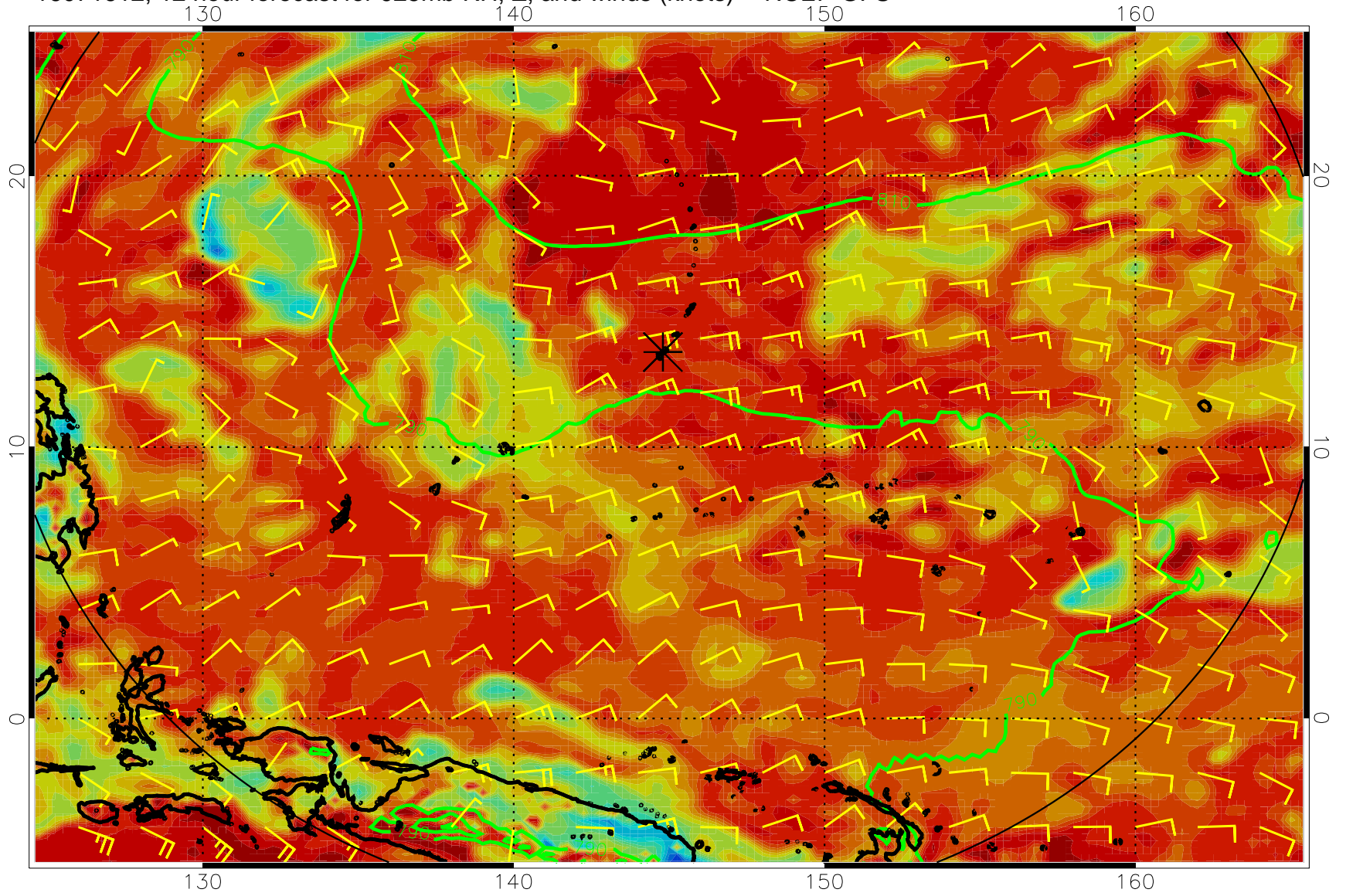
16071612, 12 hour forecast for 925mb RH, Z, and winds (knots) -- NCEP GFS
