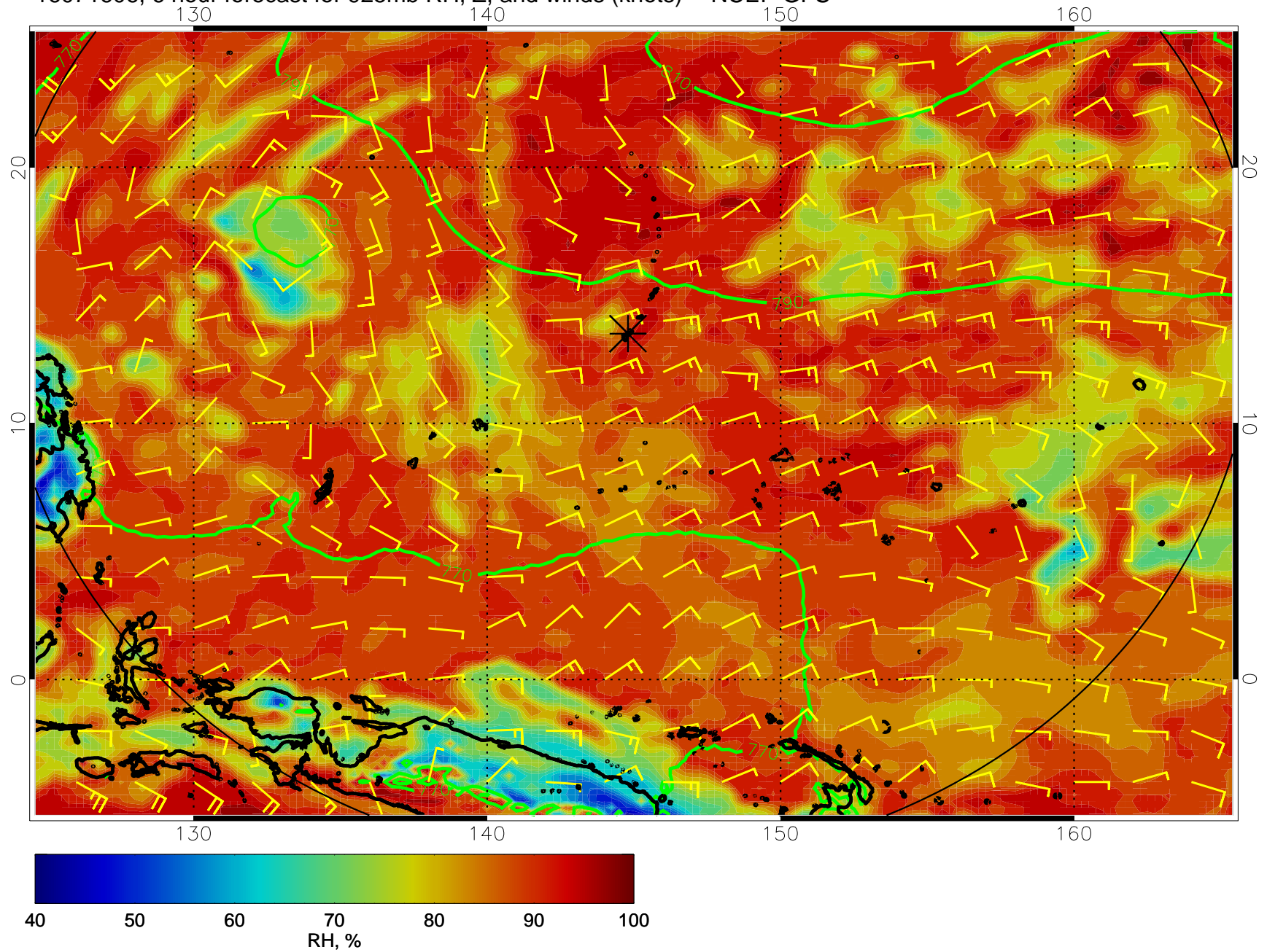
16071606, 6 hour forecast for 925mb RH, Z, and winds (knots) -- NCEP GFS
