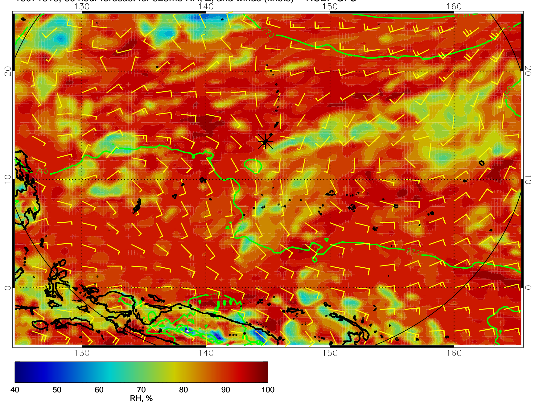
16071818, 66 hour forecast for 925mb RH, Z, and winds (knots) -- NCEP GFS
