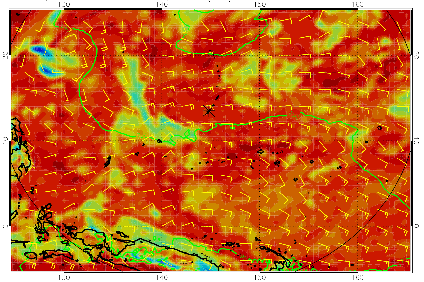
16071700, 24 hour forecast for 925mb RH, Z, and winds (knots) -- NCEP GFS
