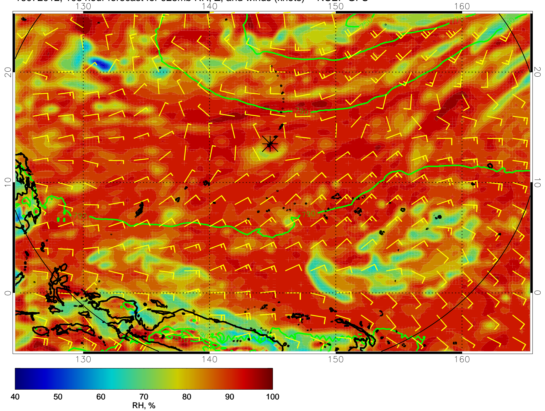
16072012, 108 hour forecast for 925mb RH, Z, and winds (knots) -- NCEP GFS
