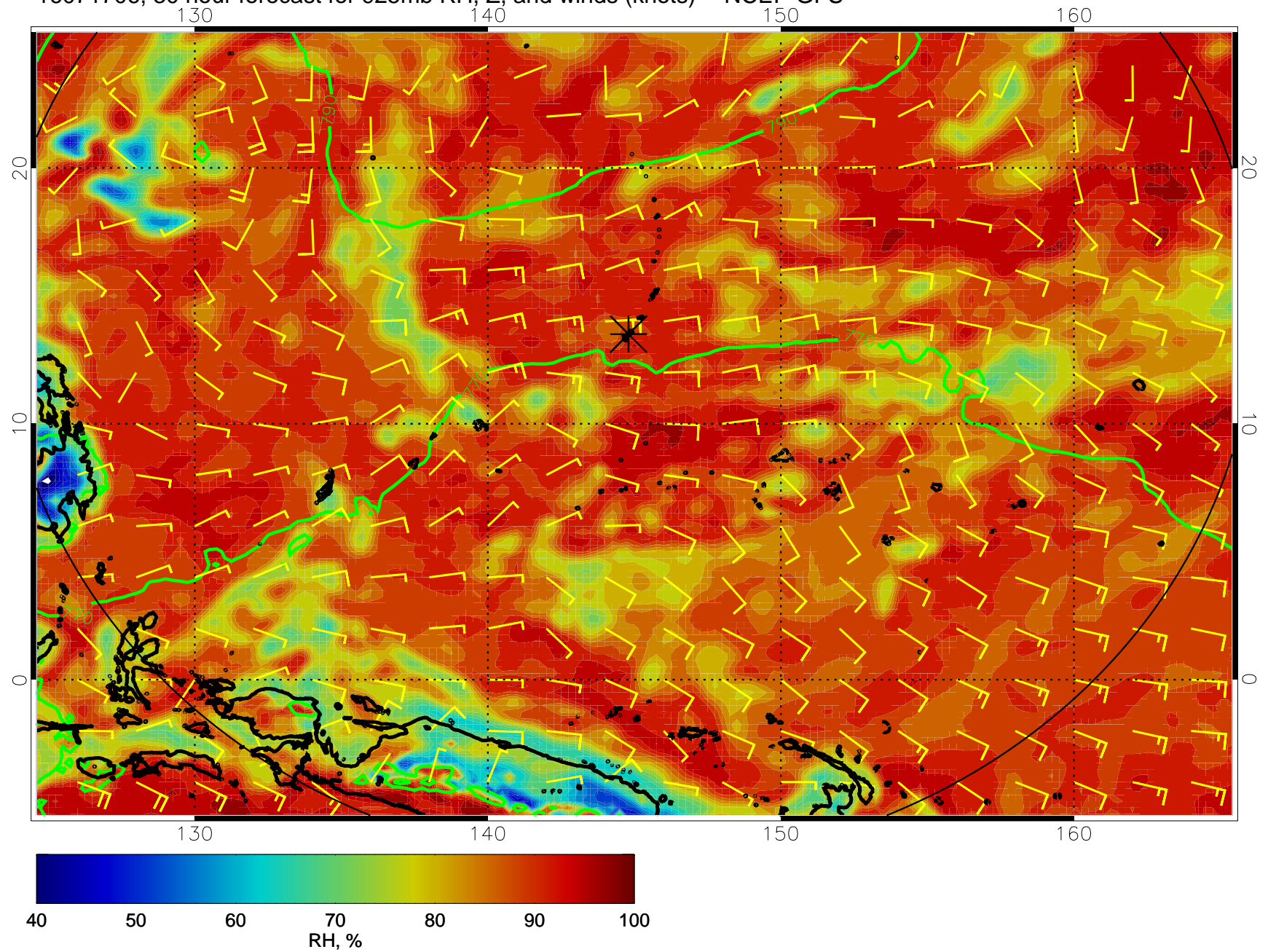
16071706, 30 hour forecast for 925mb RH, Z, and winds (knots) -- NCEP GFS
