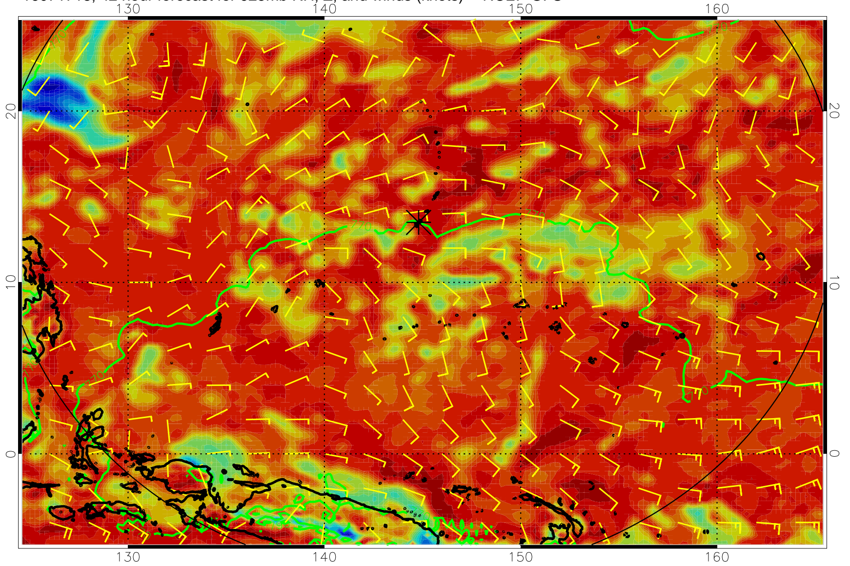
16071718, 42 hour forecast for 925mb RH, Z, and winds (knots) -- NCEP GFS
