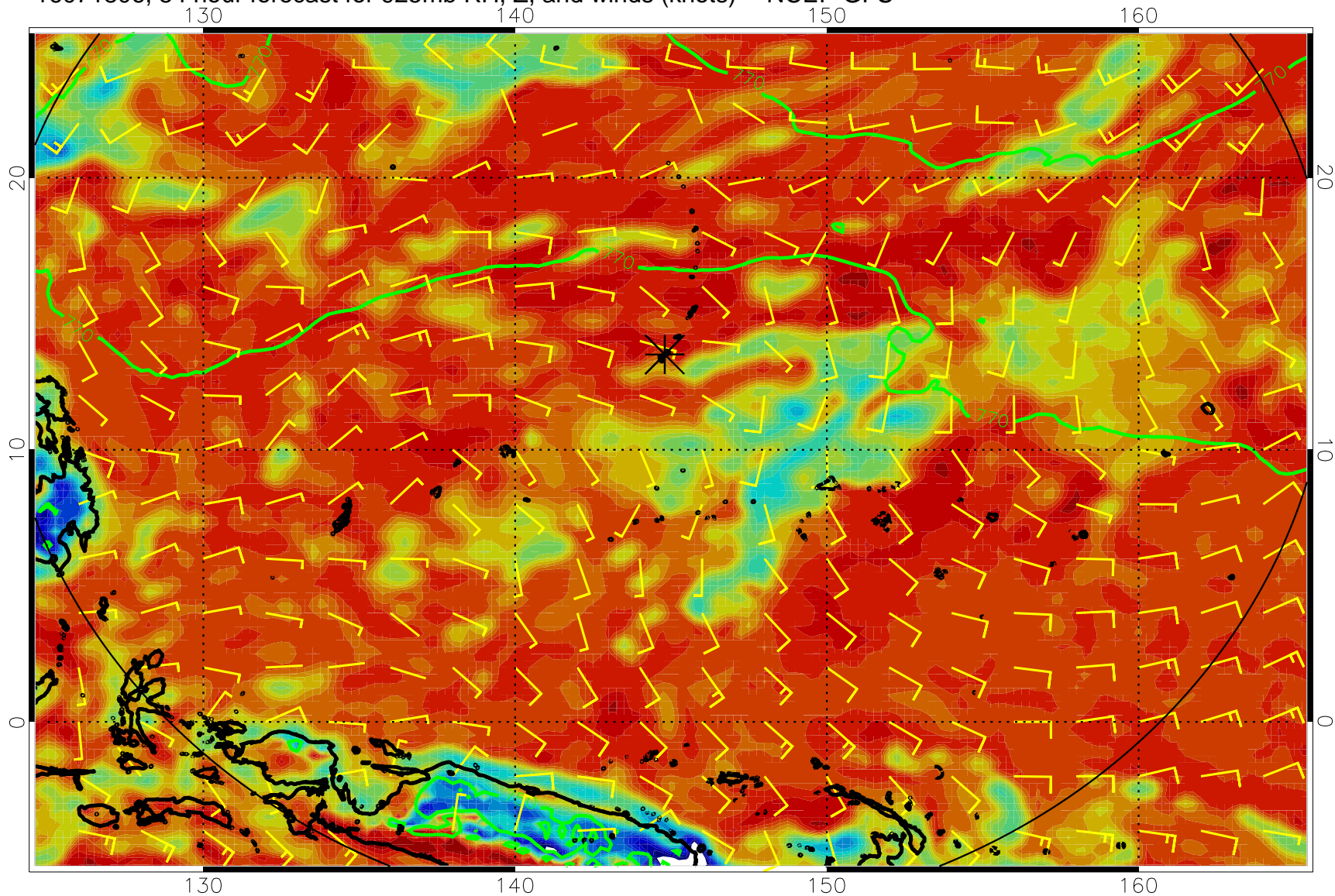
16071806, 54 hour forecast for 925mb RH, Z, and winds (knots) -- NCEP GFS
