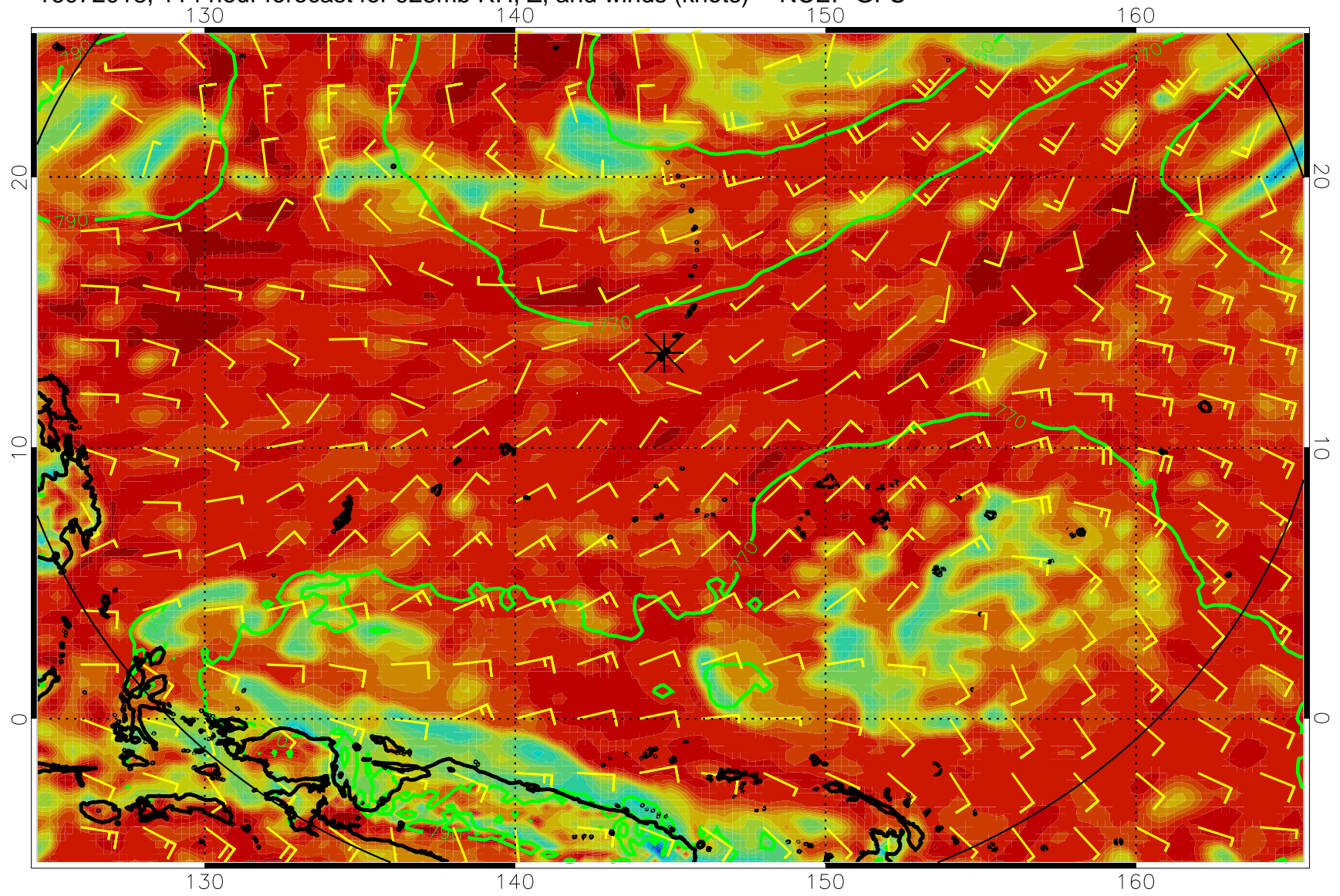
16072018, 114 hour forecast for 925mb RH, Z, and winds (knots) -- NCEP GFS
