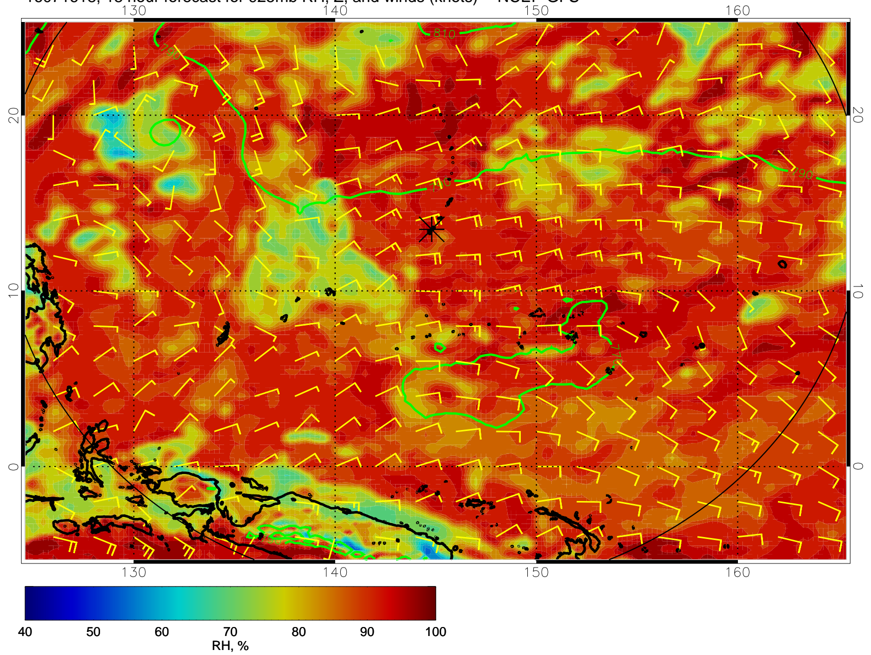
16071618, 18 hour forecast for 925mb RH, Z, and winds (knots) -- NCEP GFS
