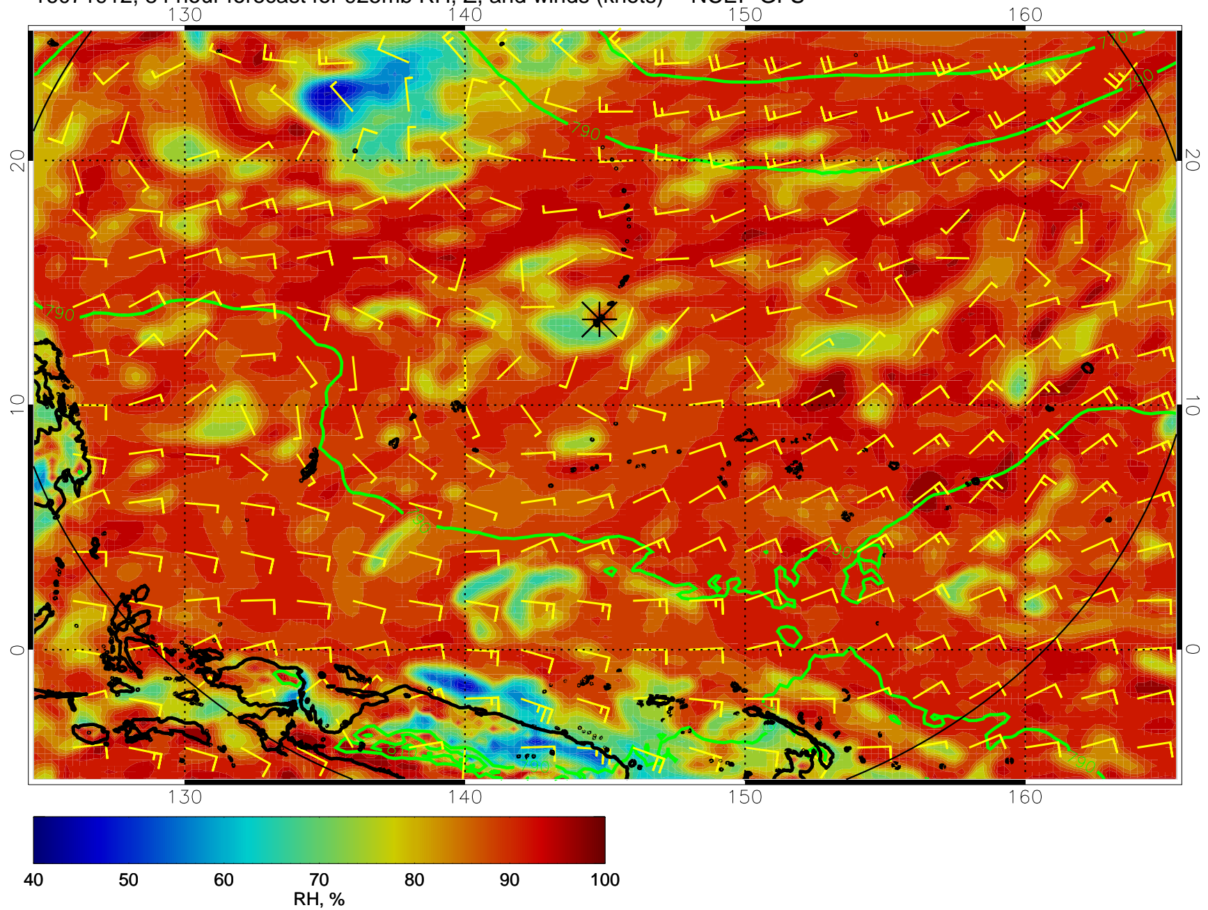
16071912, 84 hour forecast for 925mb RH, Z, and winds (knots) -- NCEP GFS
