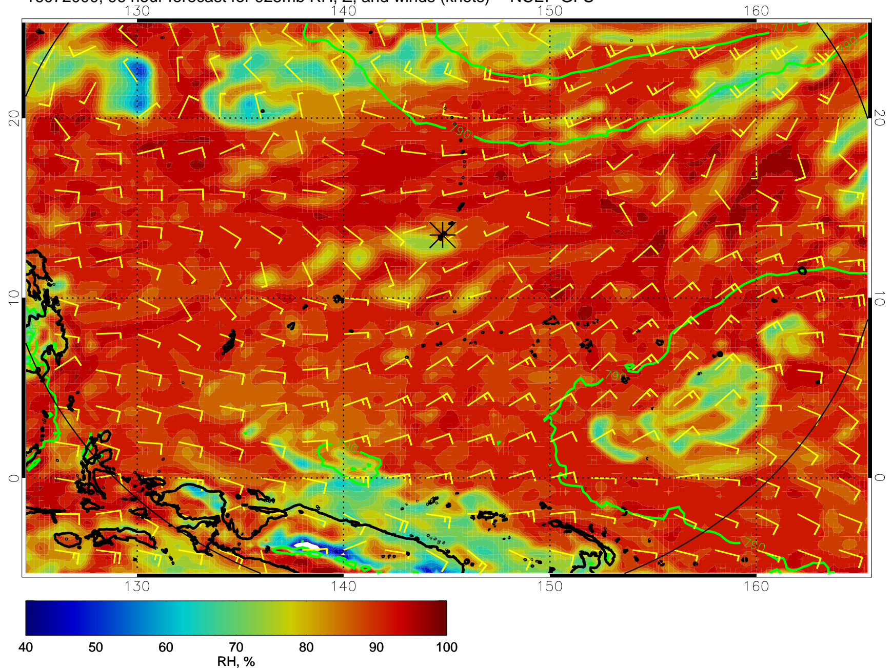
16072000, 96 hour forecast for 925mb RH, Z, and winds (knots) -- NCEP GFS
