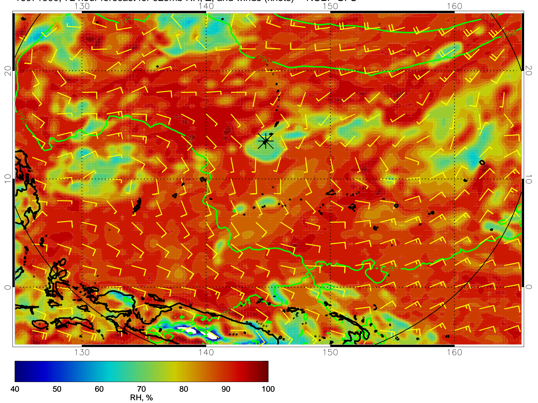
16071900, 72 hour forecast for 925mb RH, Z, and winds (knots) -- NCEP GFS
