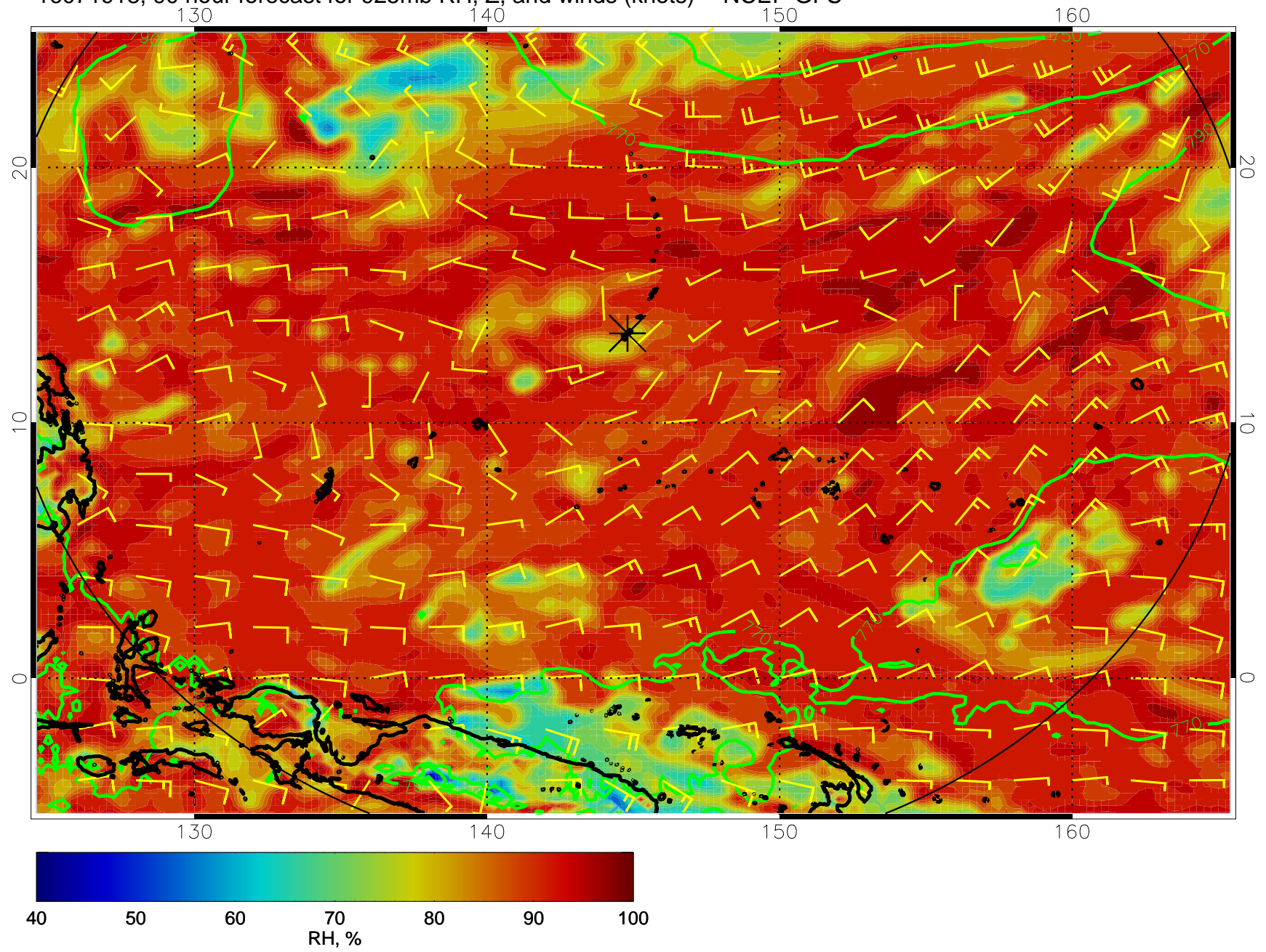
16071918, 90 hour forecast for 925mb RH, Z, and winds (knots) -- NCEP GFS
