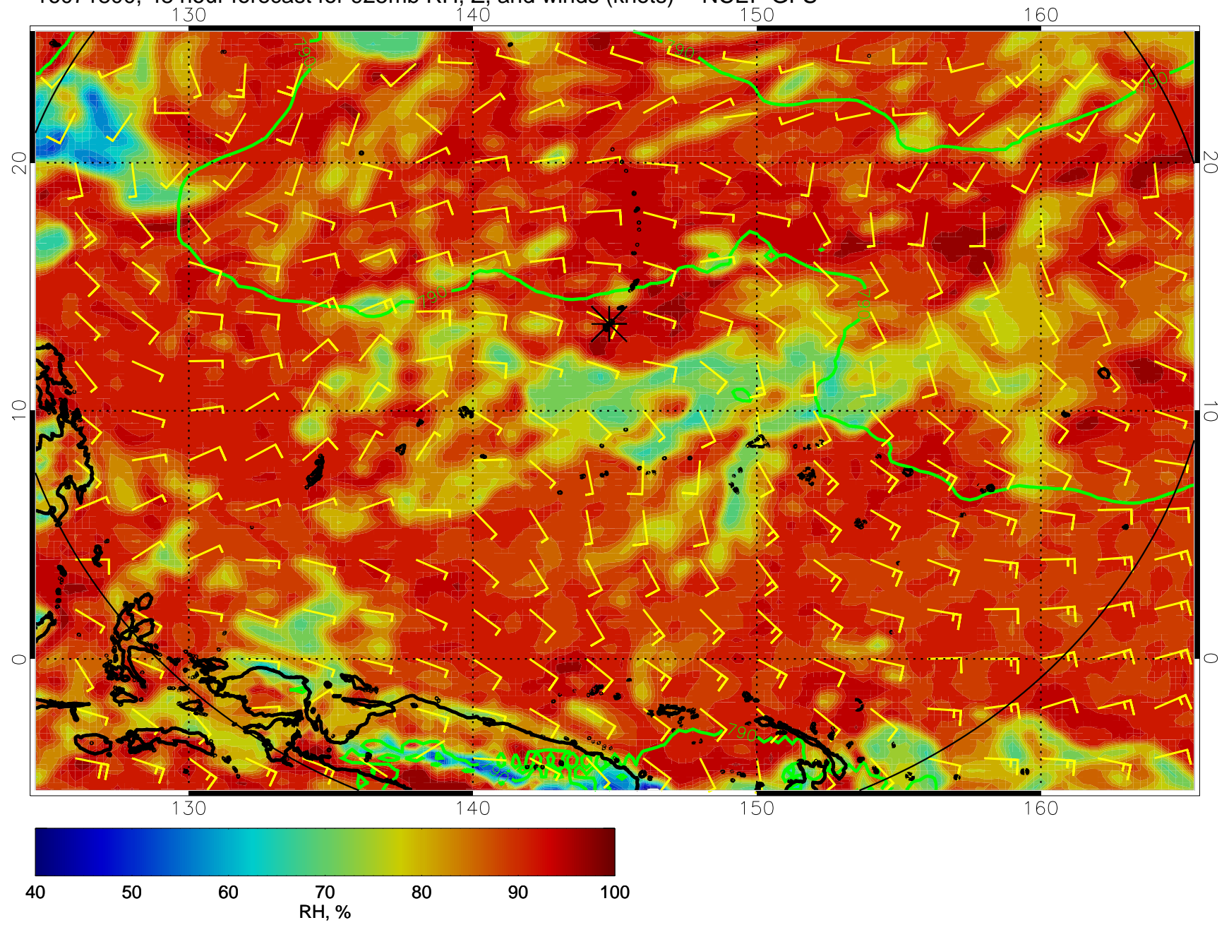
16071800, 48 hour forecast for 925mb RH, Z, and winds (knots) -- NCEP GFS
