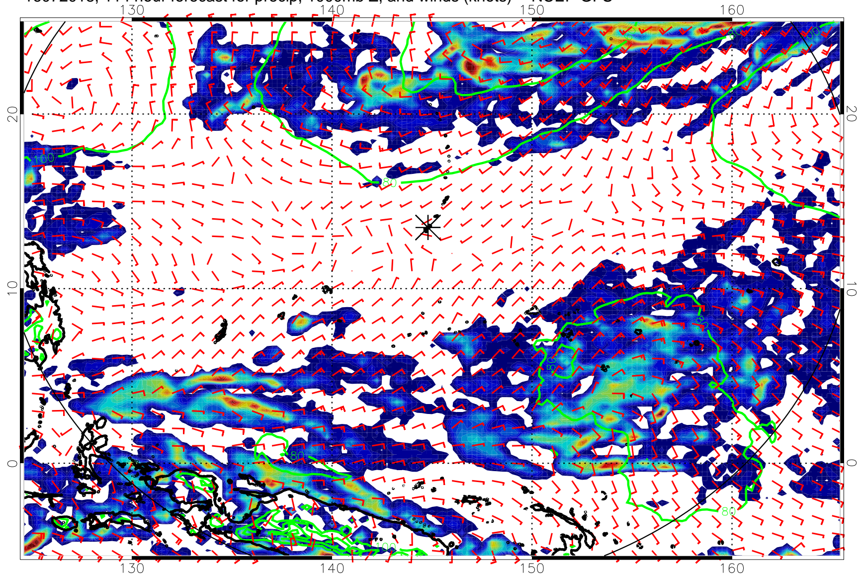
16072018, 114 hour forecast for precip, 1000mb Z, and winds (knots) -- NCEP GFS
