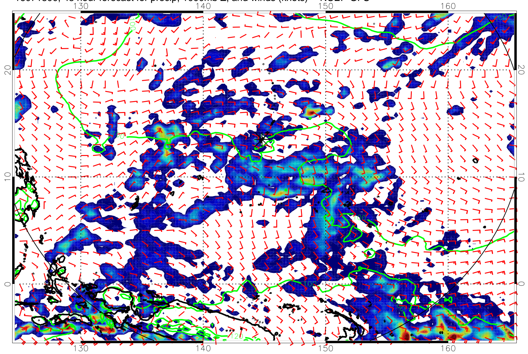
16071800, 48 hour forecast for precip, 1000mb Z, and winds (knots) -- NCEP GFS
