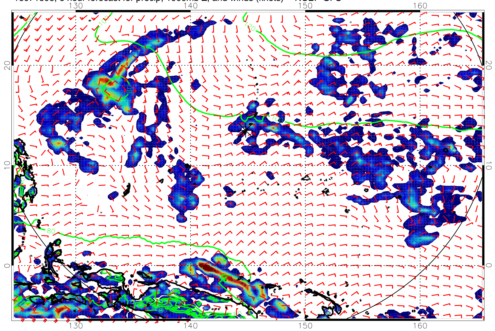
16071606, 6 hour forecast for precip, 1000mb Z, and winds (knots) -- NCEP GFS
