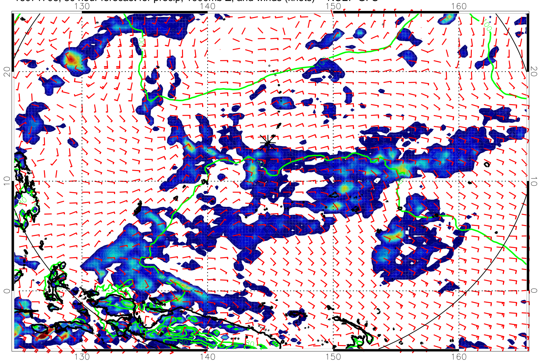
16071706, 30 hour forecast for precip, 1000mb Z, and winds (knots) -- NCEP GFS
