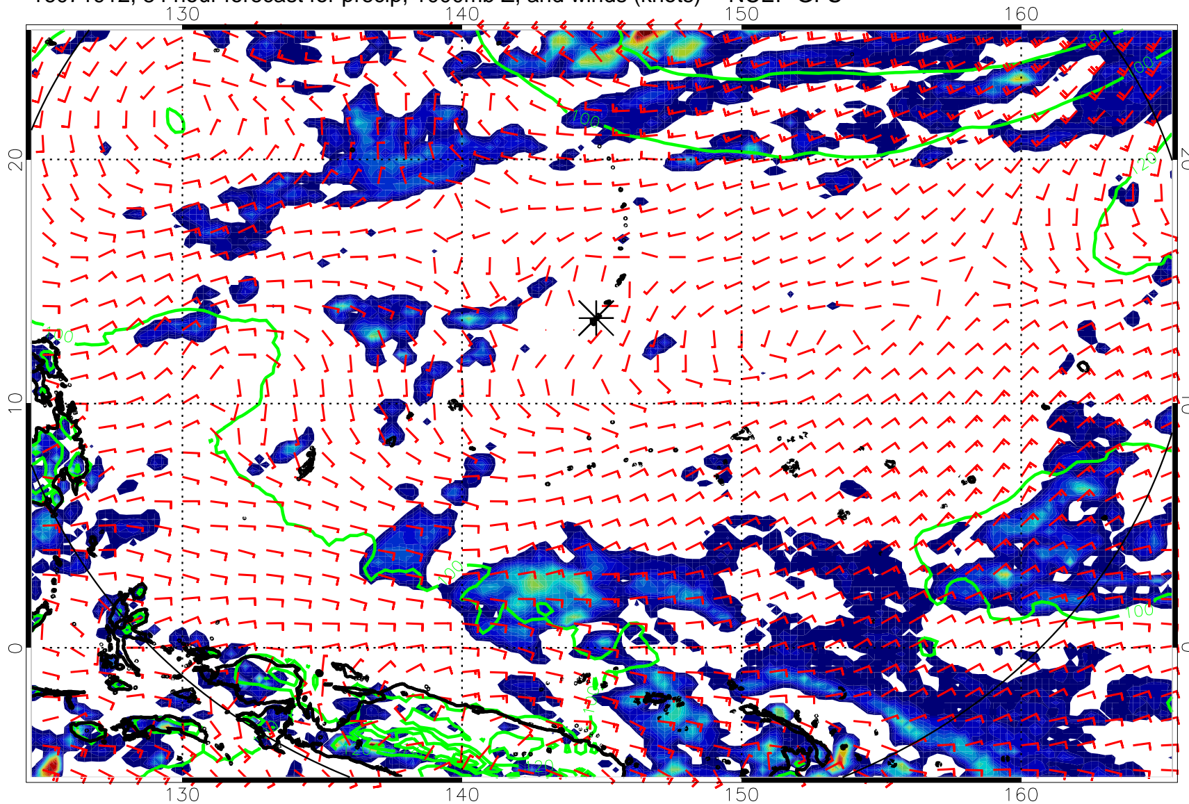
16071912, 84 hour forecast for precip, 1000mb Z, and winds (knots) -- NCEP GFS
