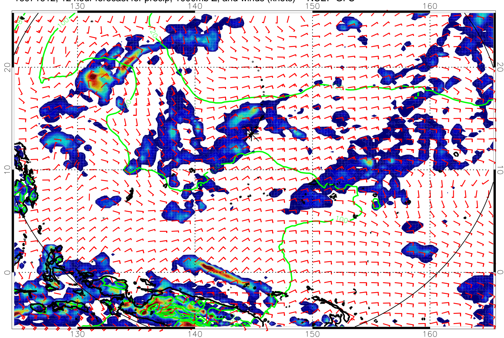
16071612, 12 hour forecast for precip, 1000mb Z, and winds (knots) -- NCEP GFS
