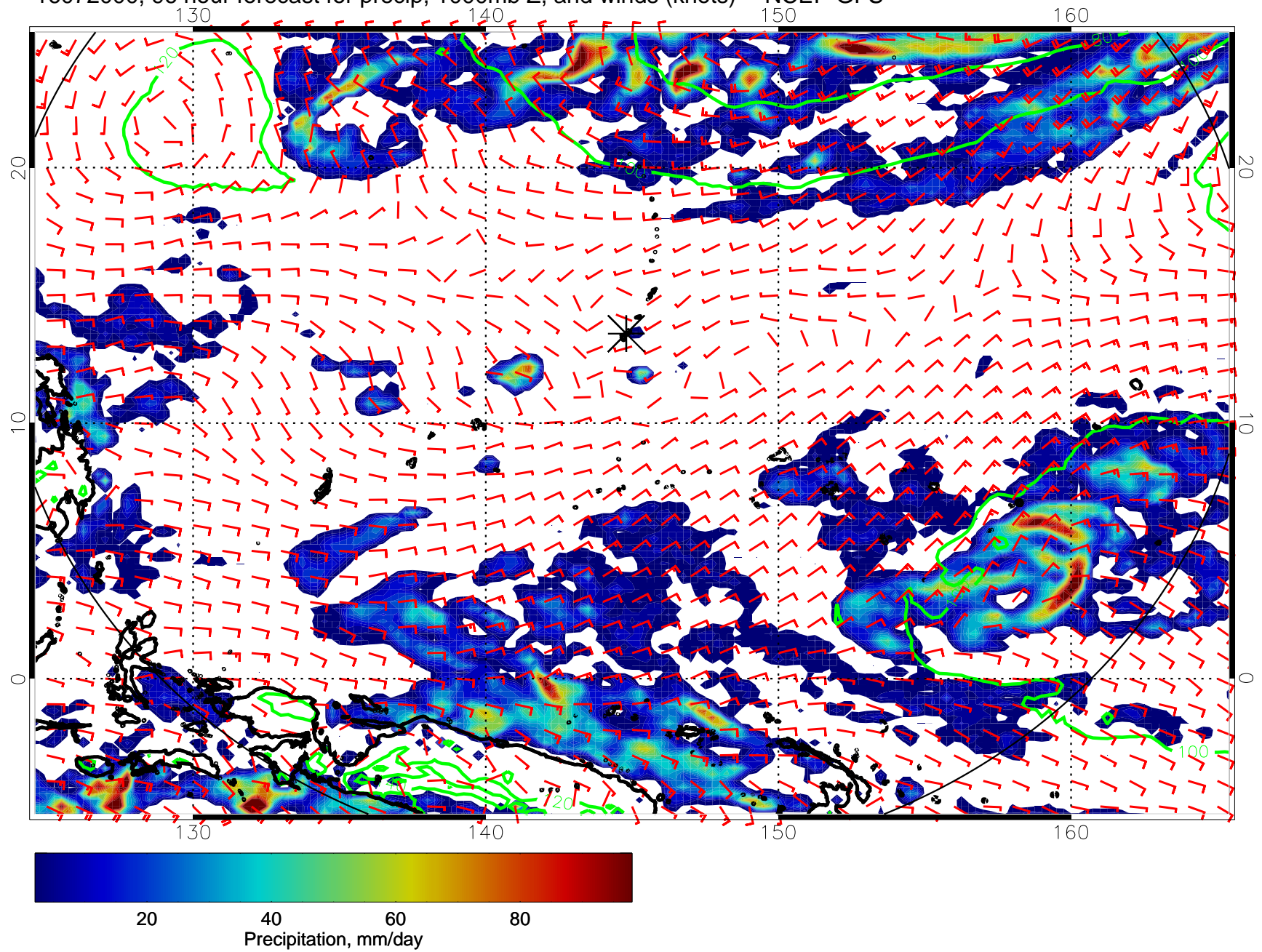
16072000, 96 hour forecast for precip, 1000mb Z, and winds (knots) -- NCEP GFS
