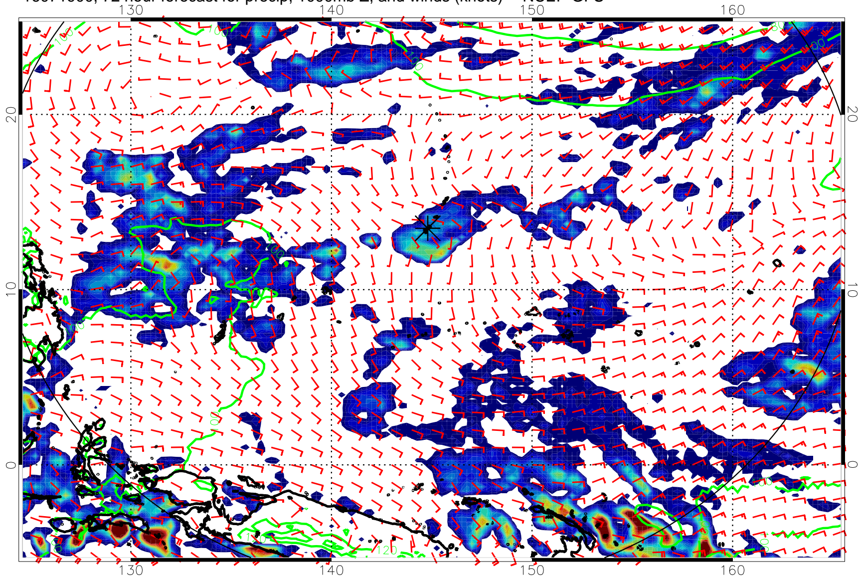
16071900, 72 hour forecast for precip, 1000mb Z, and winds (knots) -- NCEP GFS
