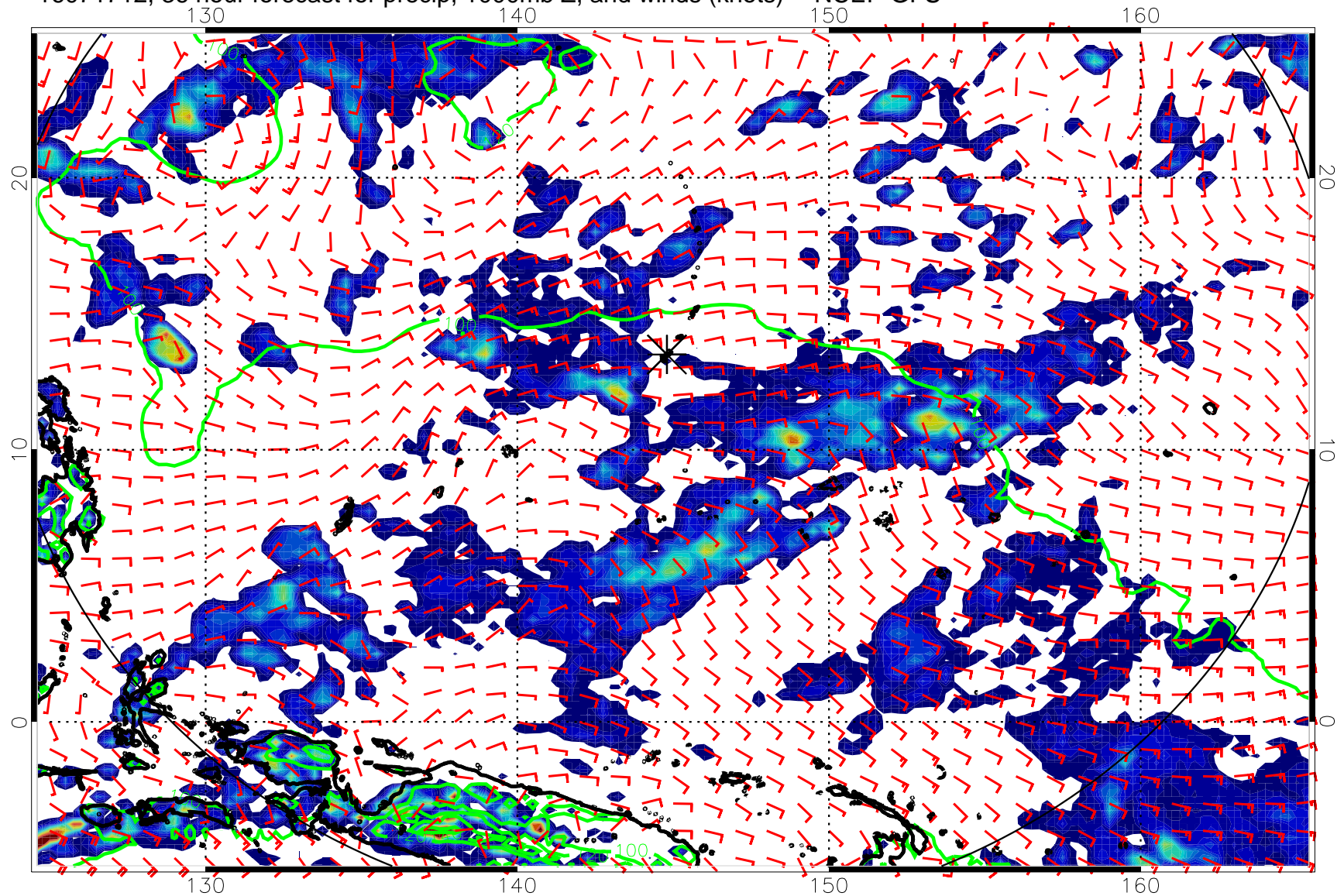
16071712, 36 hour forecast for precip, 1000mb Z, and winds (knots) -- NCEP GFS
