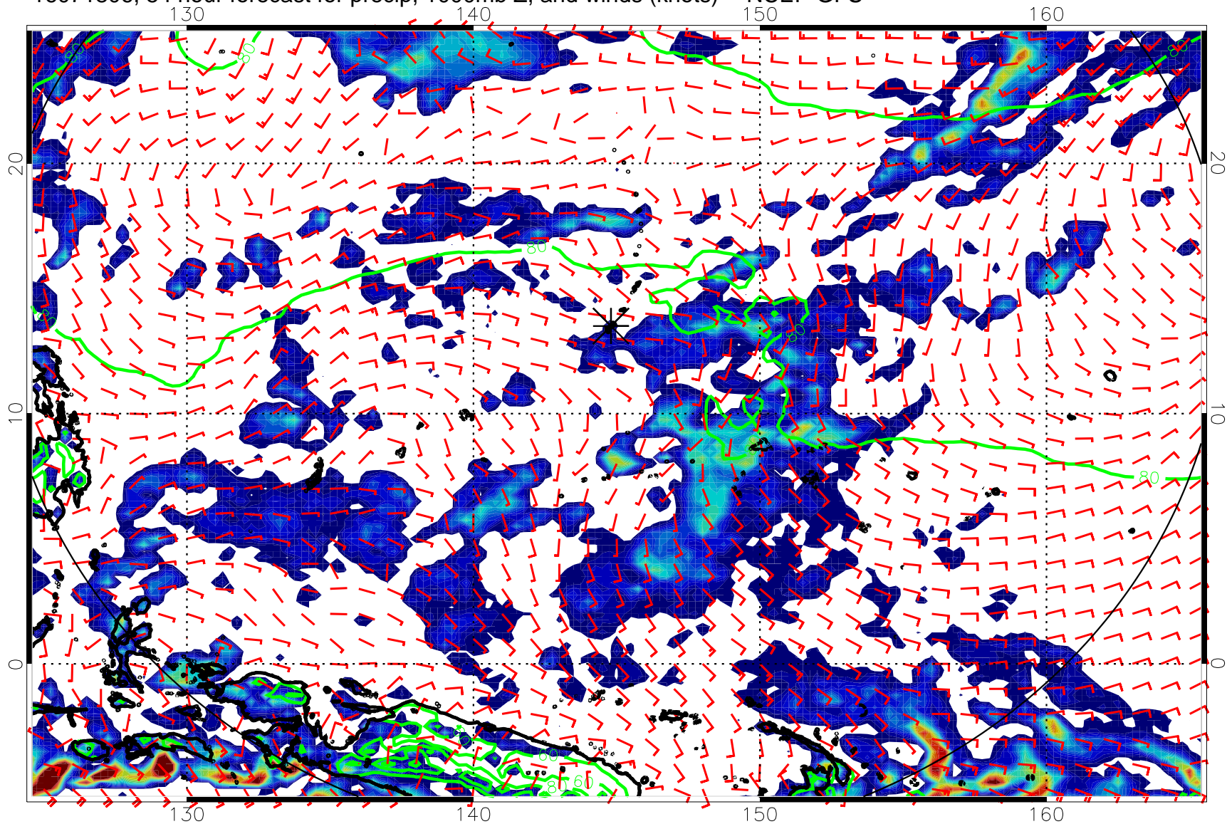
16071806, 54 hour forecast for precip, 1000mb Z, and winds (knots) -- NCEP GFS
