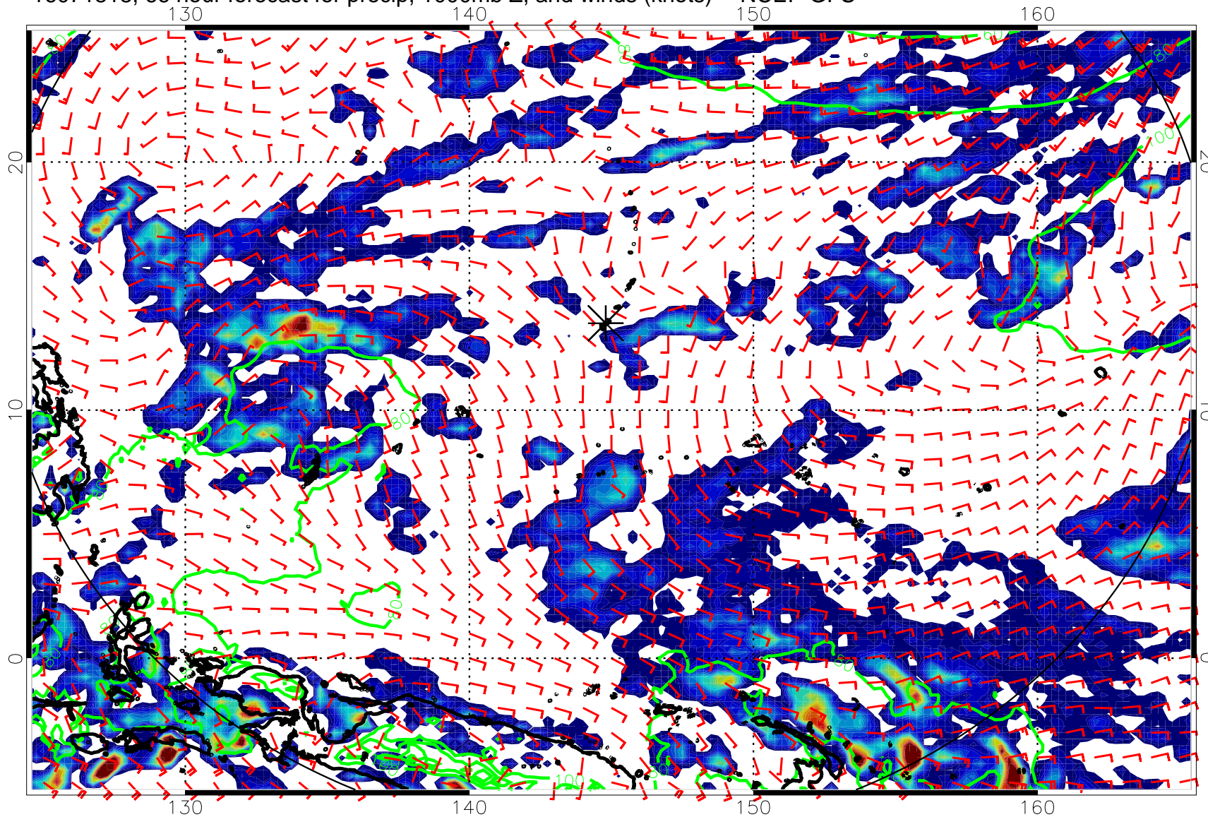
16071818, 66 hour forecast for precip, 1000mb Z, and winds (knots) -- NCEP GFS
