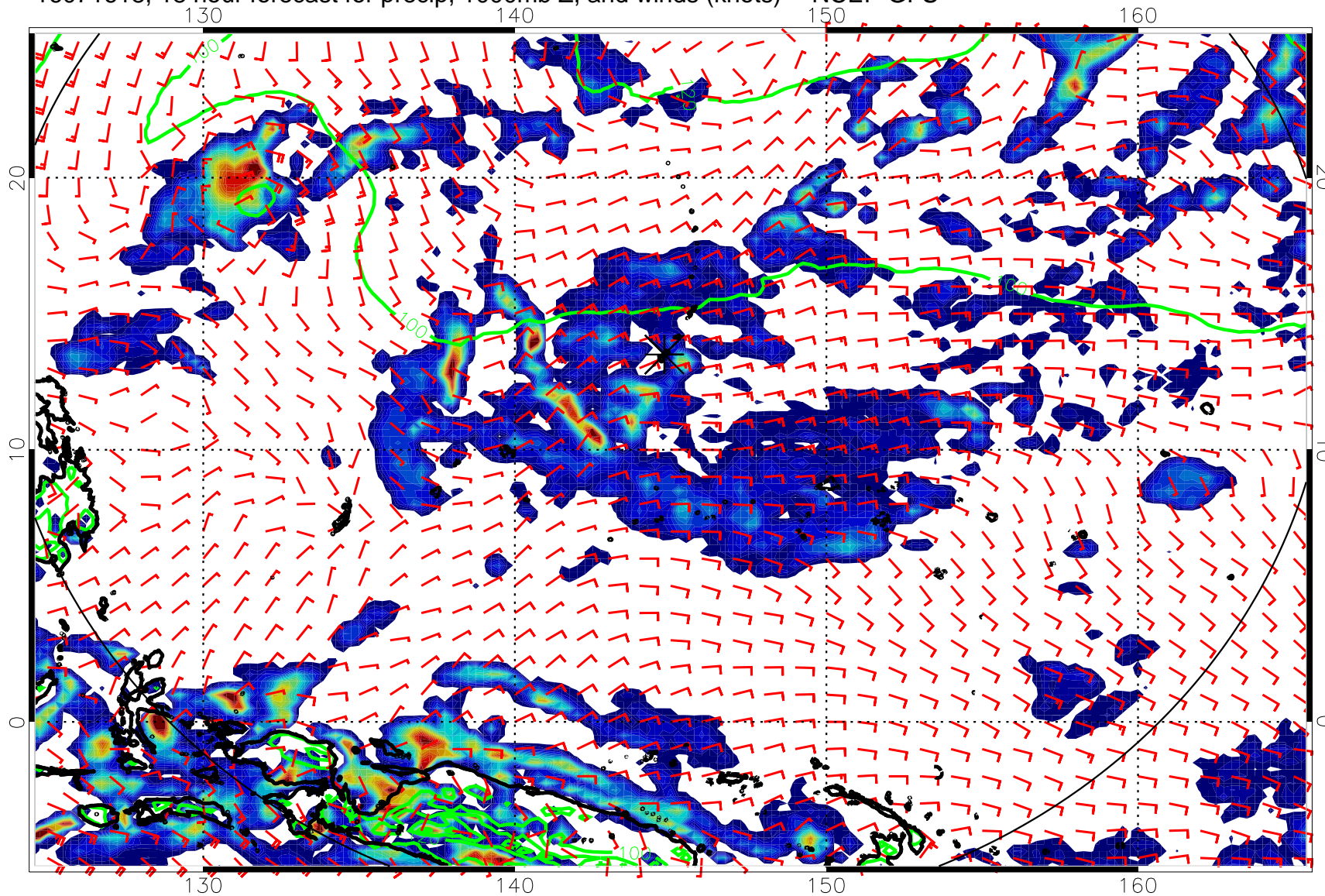
16071618, 18 hour forecast for precip, 1000mb Z, and winds (knots) -- NCEP GFS
