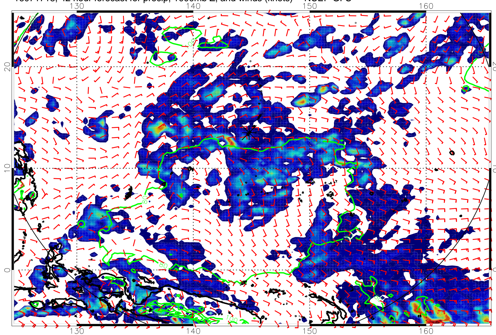
16071718, 42 hour forecast for precip, 1000mb Z, and winds (knots) -- NCEP GFS
