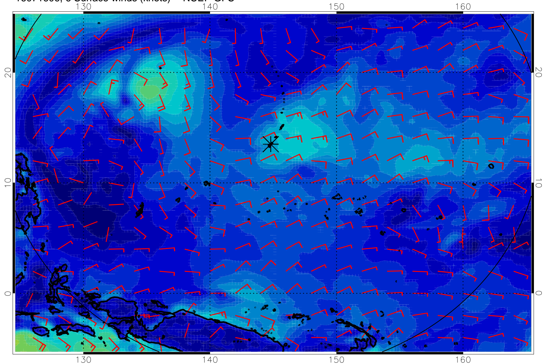
16071606, 6 Surface winds (knots) -- NCEP GFS
