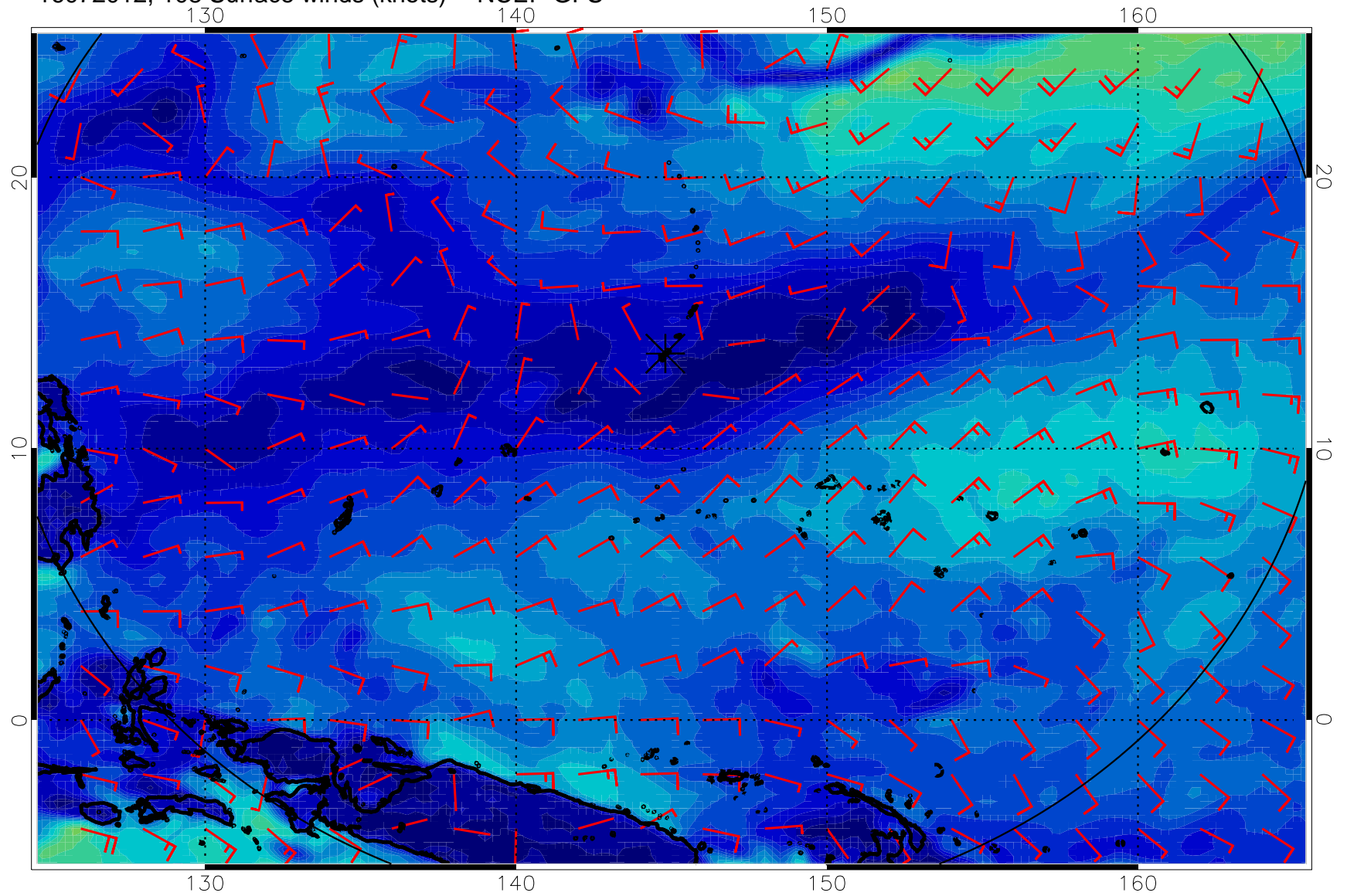
16072012, 108 Surface winds (knots) -- NCEP GFS
