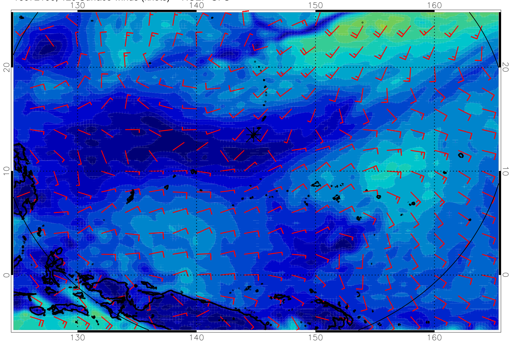
16072100, 120 Surface winds (knots) -- NCEP GFS
