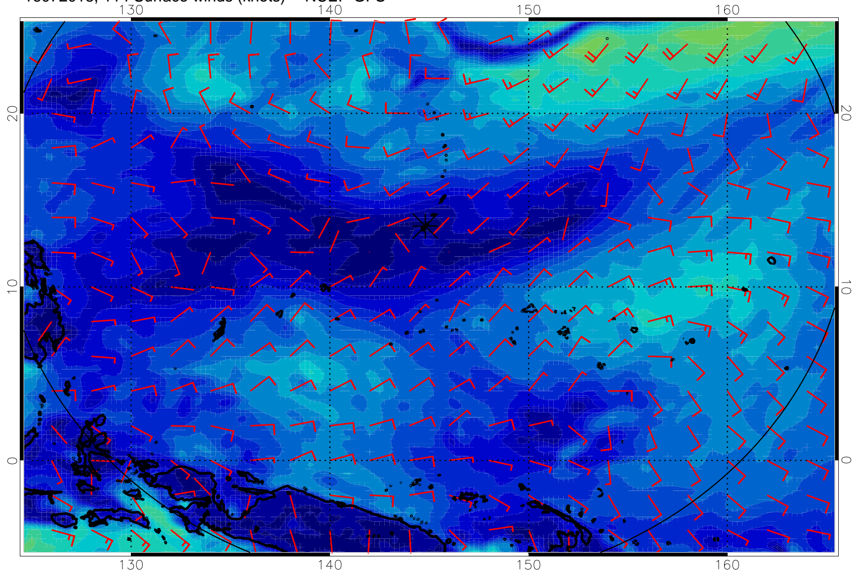
16072018, 114 Surface winds (knots) -- NCEP GFS
