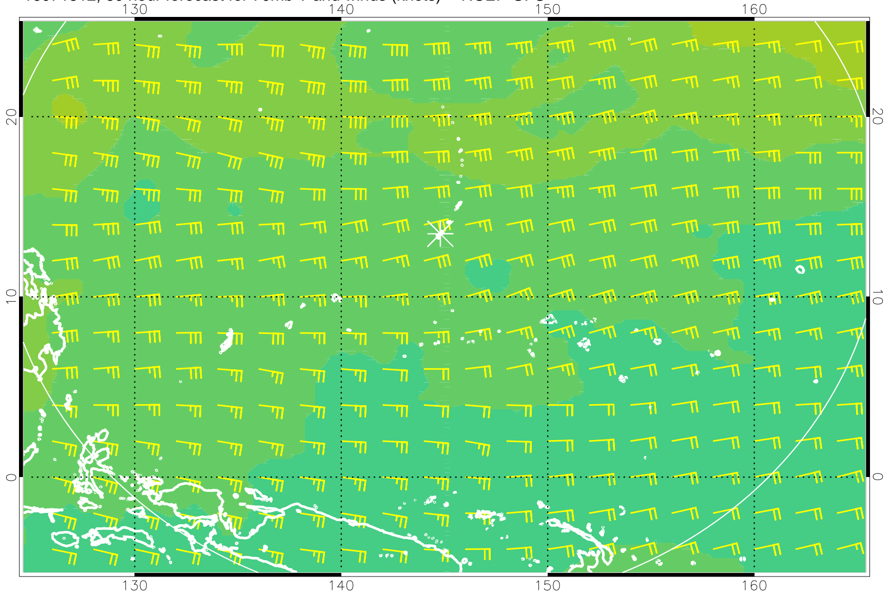
16071812, 60 hour forecast for 70mb T and winds (knots) -- NCEP GFS
