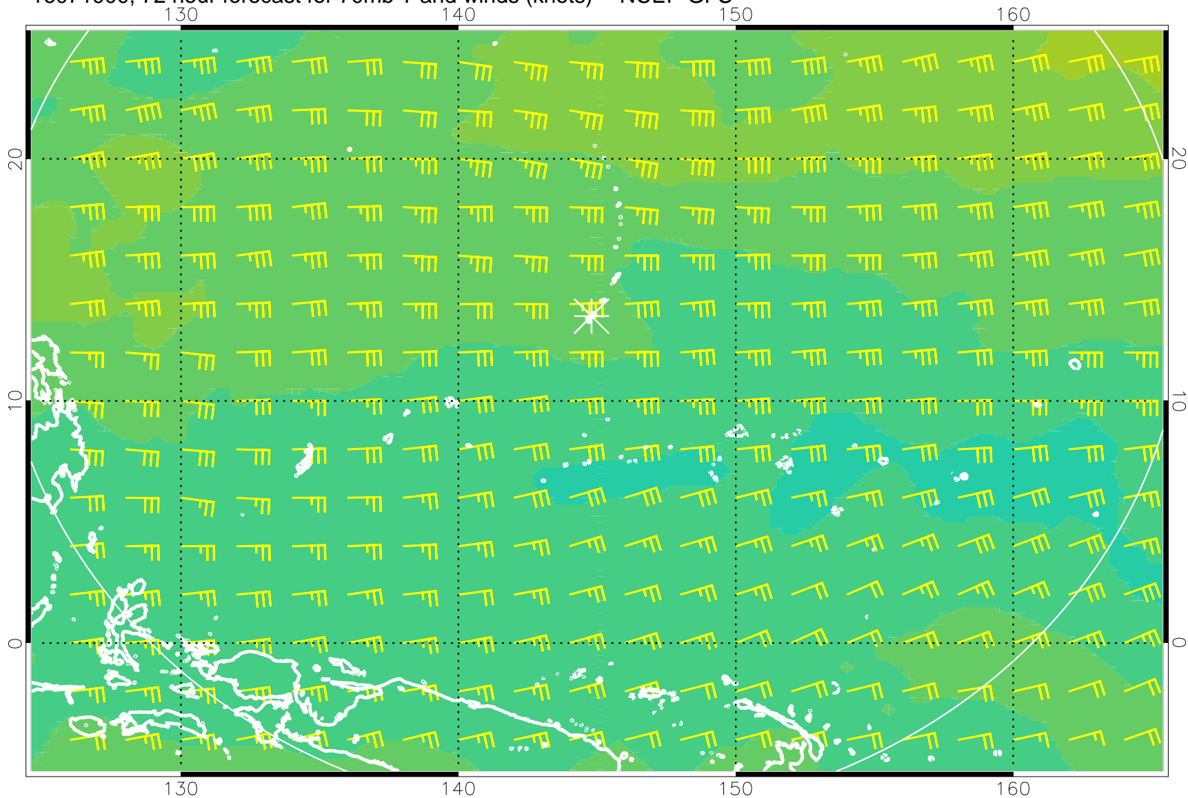
16071900, 72 hour forecast for 70mb T and winds (knots) -- NCEP GFS
