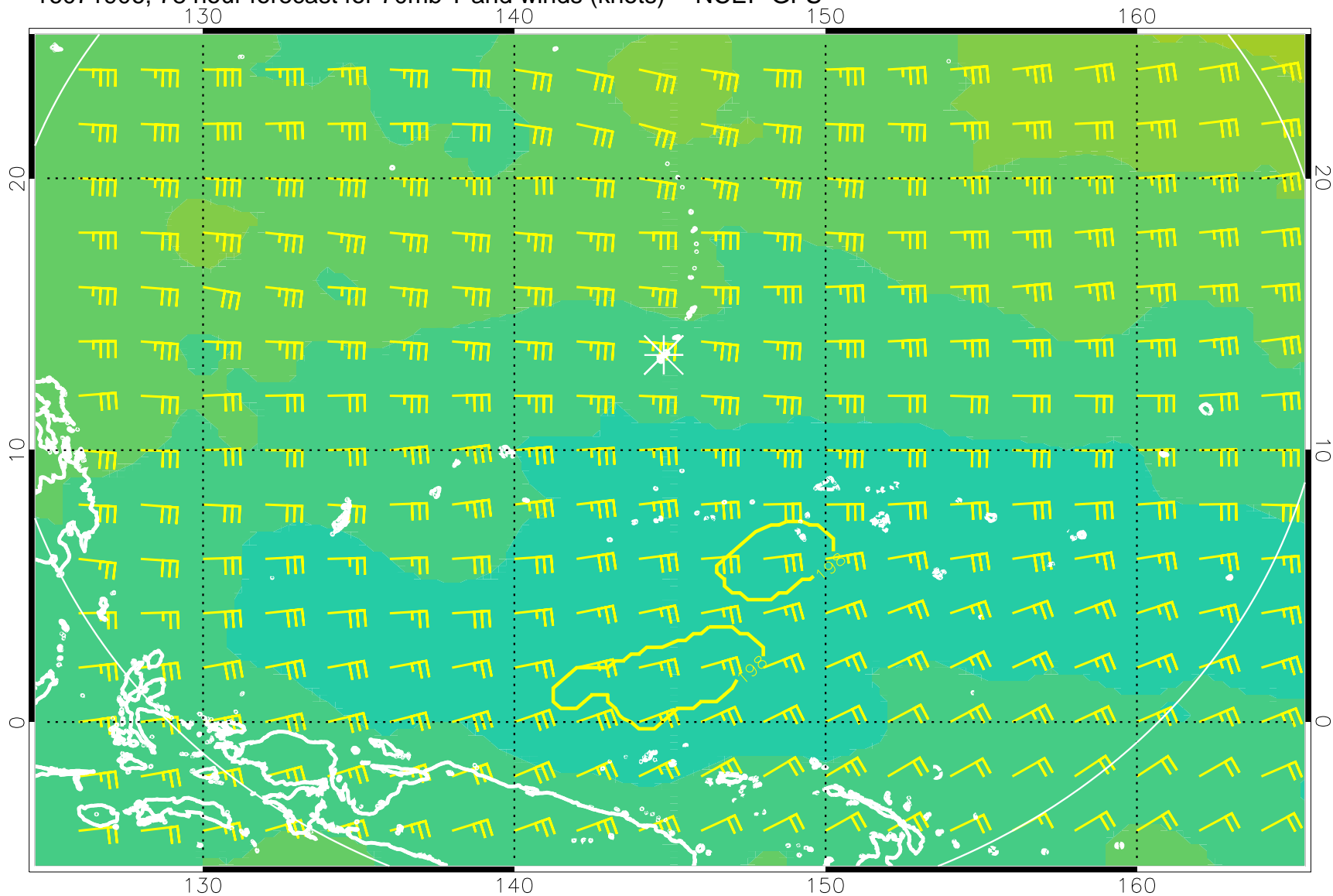
16071906, 78 hour forecast for 70mb T and winds (knots) -- NCEP GFS
