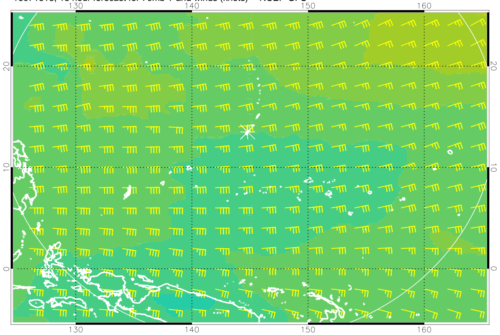
16071618, 18 hour forecast for 70mb T and winds (knots) -- NCEP GFS
