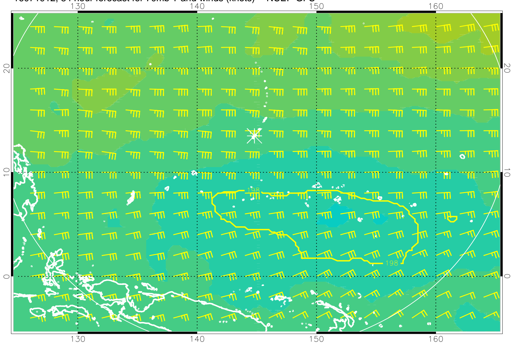
16071912, 84 hour forecast for 70mb T and winds (knots) -- NCEP GFS
