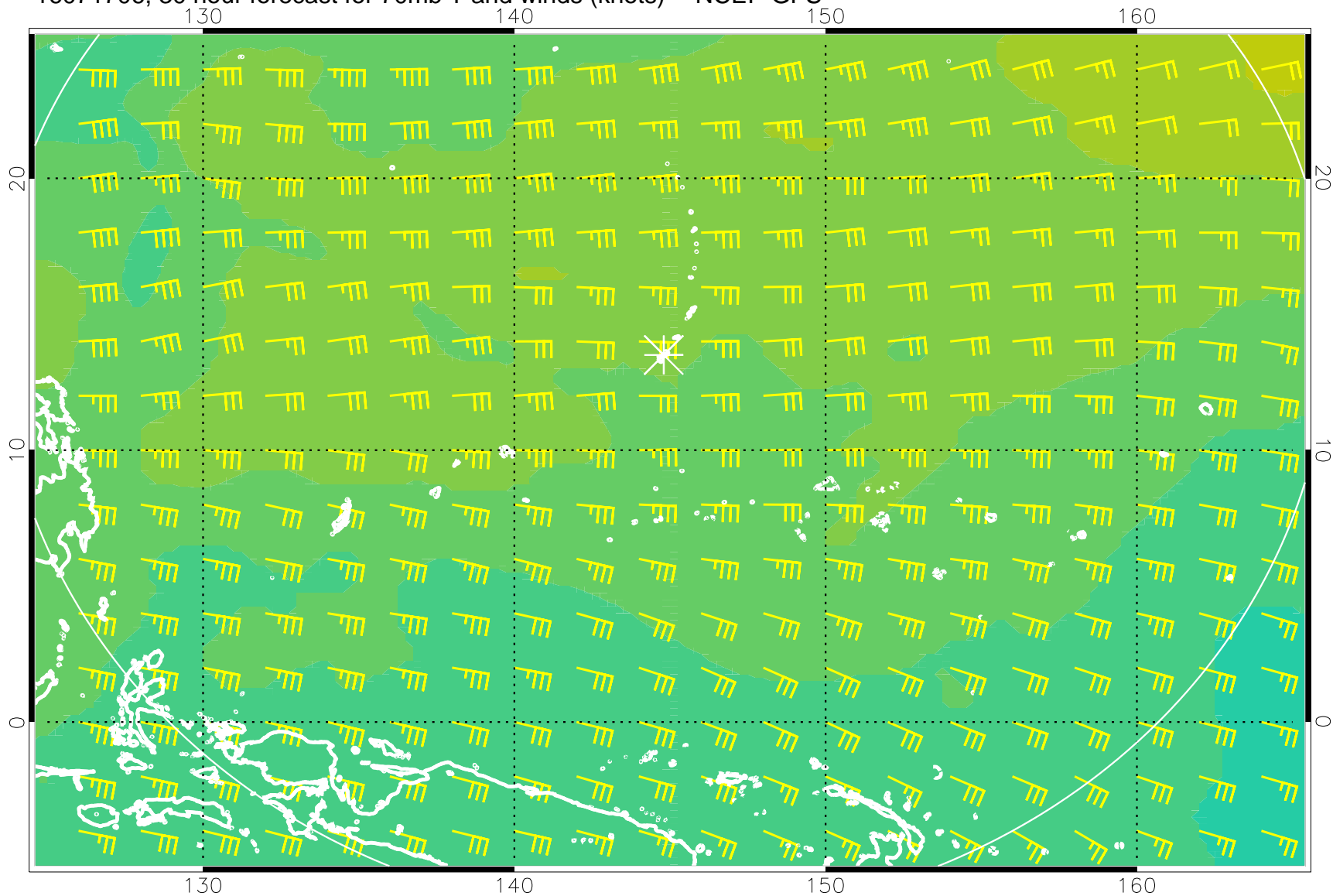
16071706, 30 hour forecast for 70mb T and winds (knots) -- NCEP GFS
