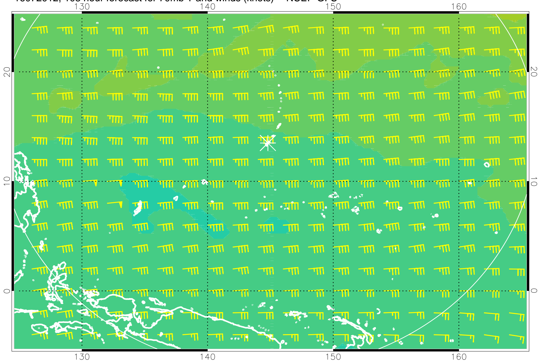
16072012, 108 hour forecast for 70mb T and winds (knots) -- NCEP GFS
