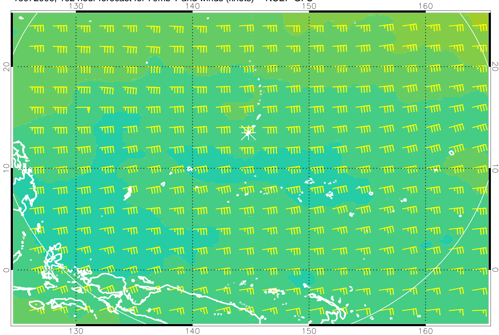
16072006, 102 hour forecast for 70mb T and winds (knots) -- NCEP GFS
