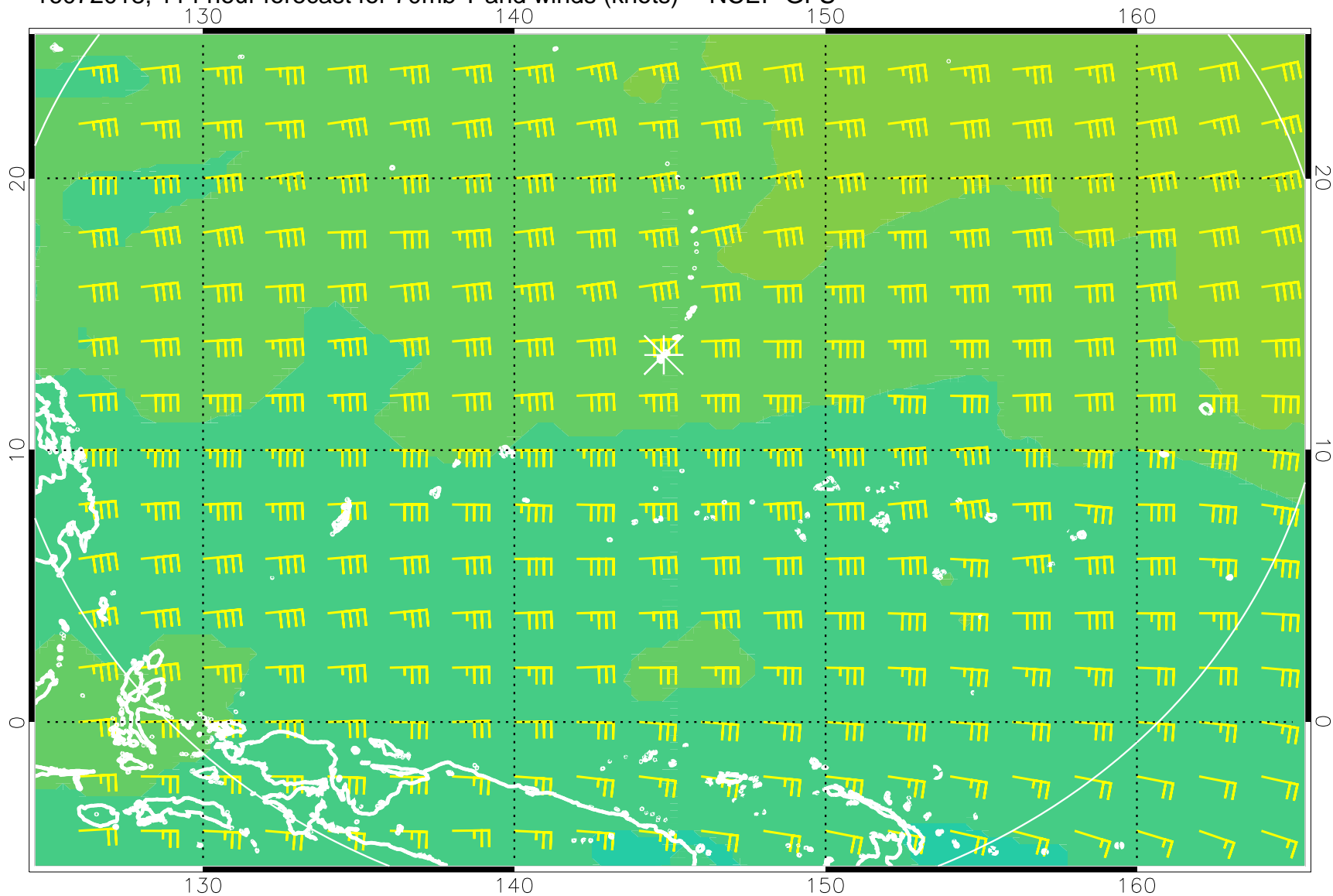
16072018, 114 hour forecast for 70mb T and winds (knots) -- NCEP GFS
