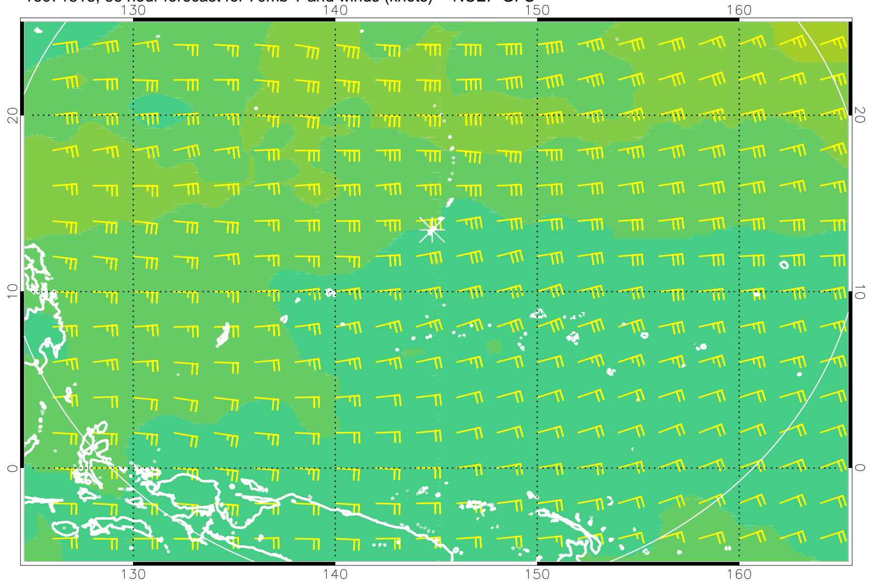
16071818, 66 hour forecast for 70mb T and winds (knots) -- NCEP GFS
