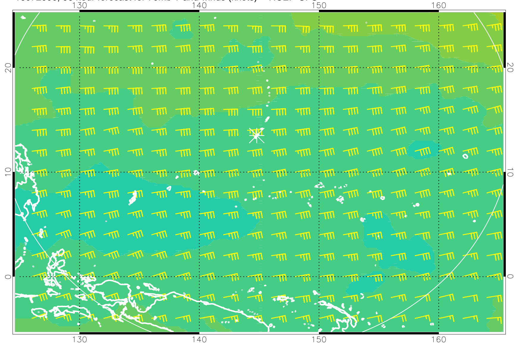
16072000, 96 hour forecast for 70mb T and winds (knots) -- NCEP GFS
