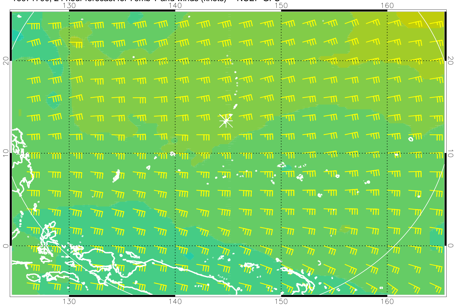
16071700, 24 hour forecast for 70mb T and winds (knots) -- NCEP GFS
