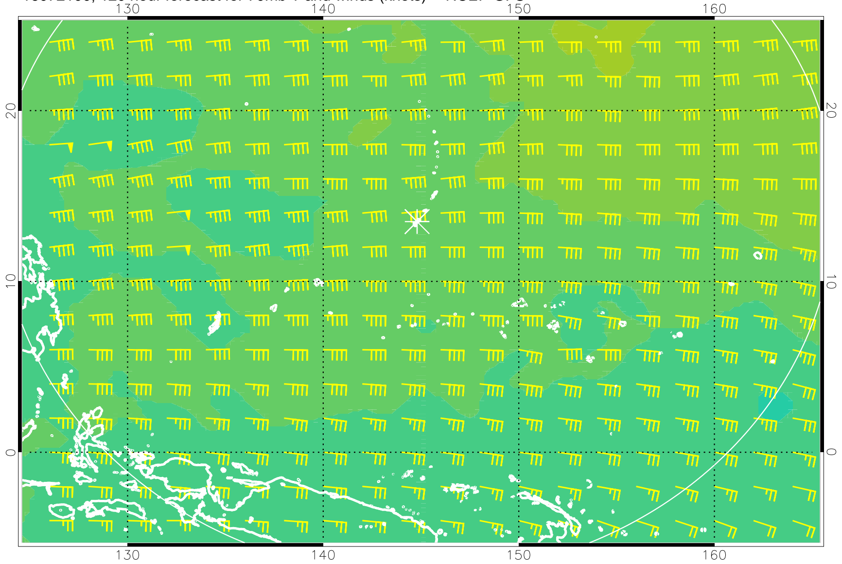
16072100, 120 hour forecast for 70mb T and winds (knots) -- NCEP GFS
