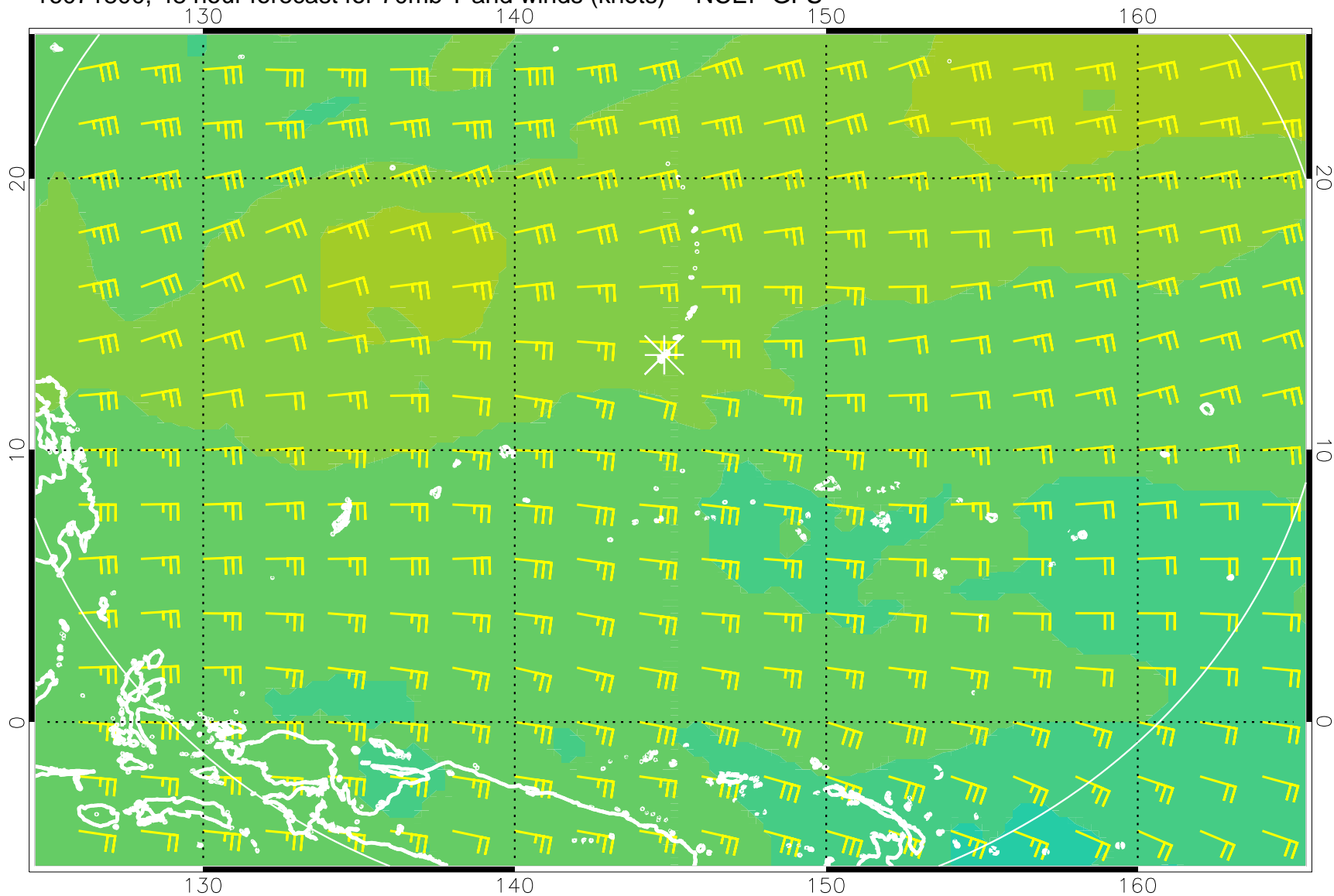
16071800, 48 hour forecast for 70mb T and winds (knots) -- NCEP GFS
