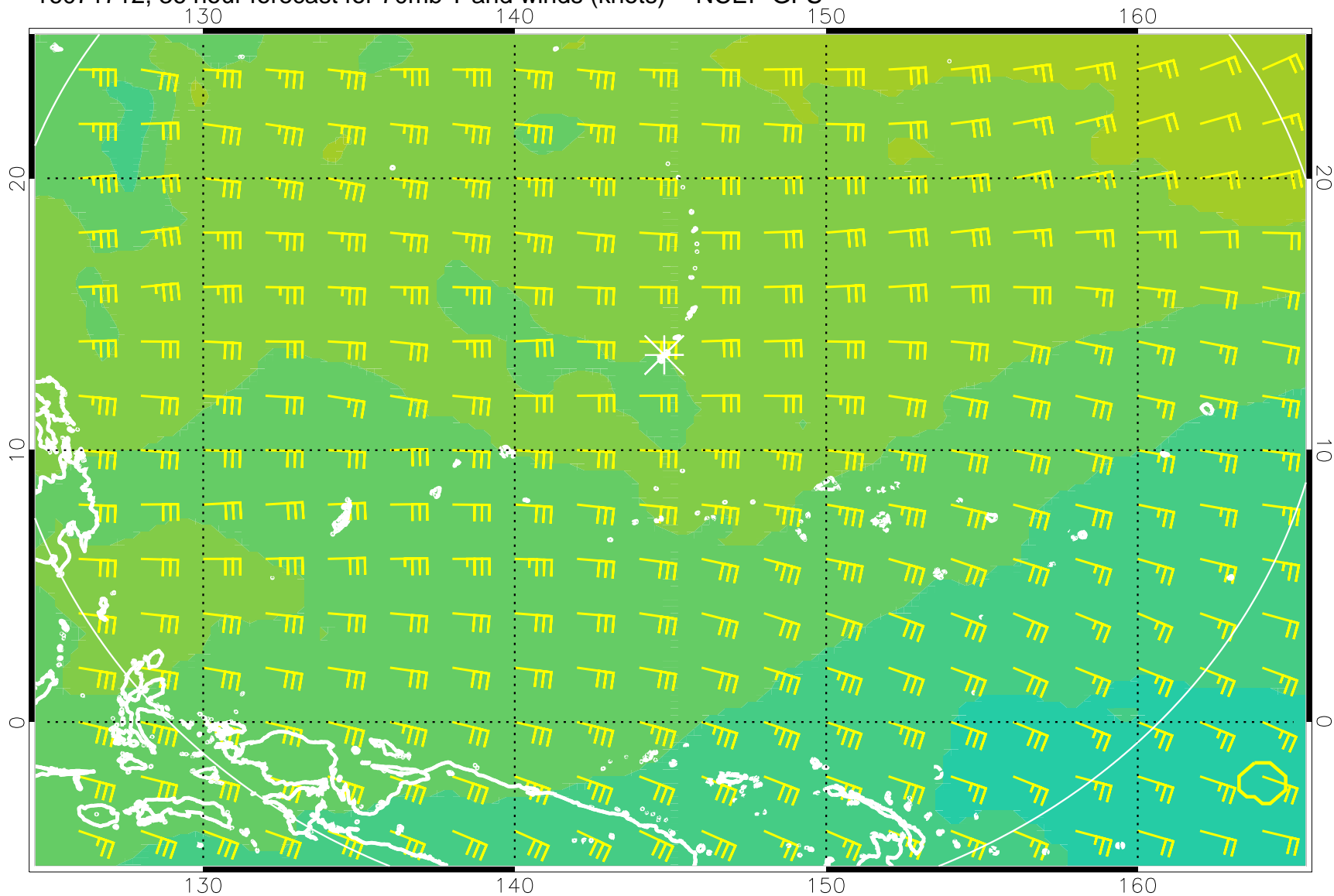
16071712, 36 hour forecast for 70mb T and winds (knots) -- NCEP GFS
