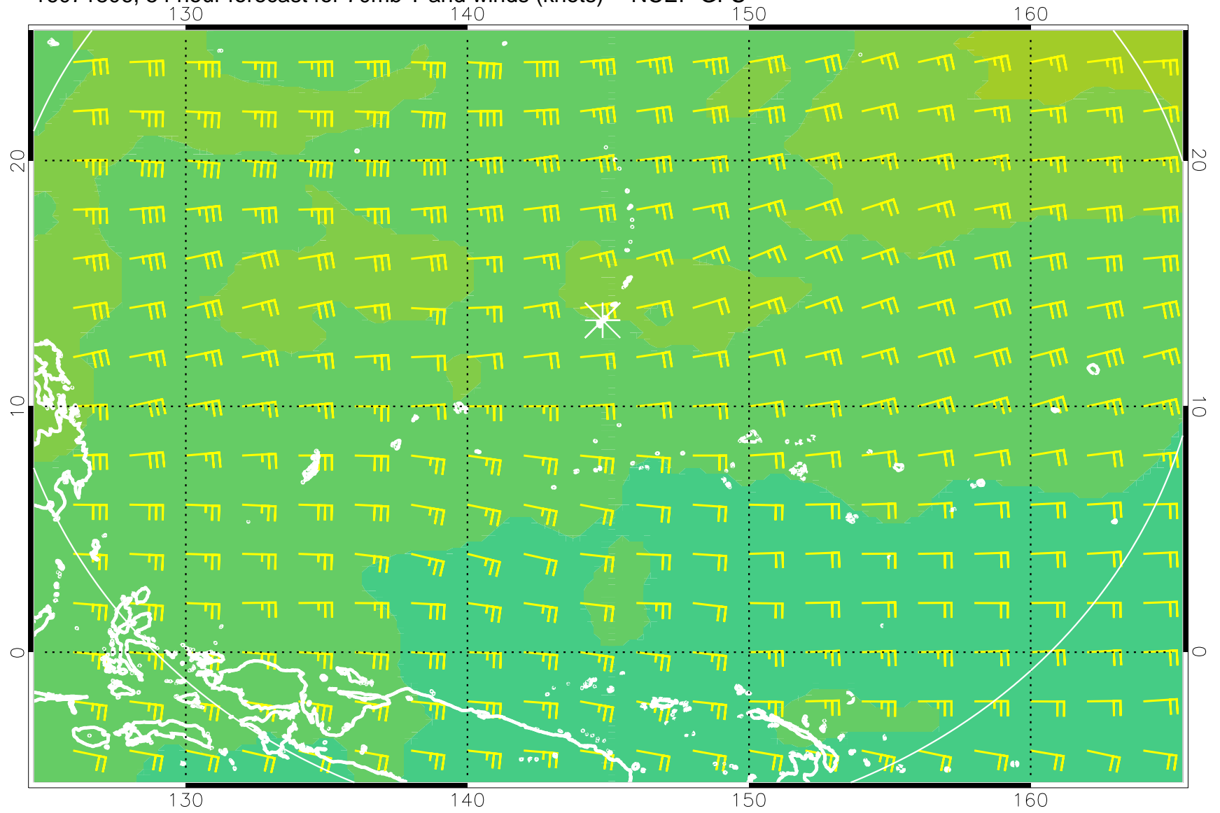
16071806, 54 hour forecast for 70mb T and winds (knots) -- NCEP GFS
