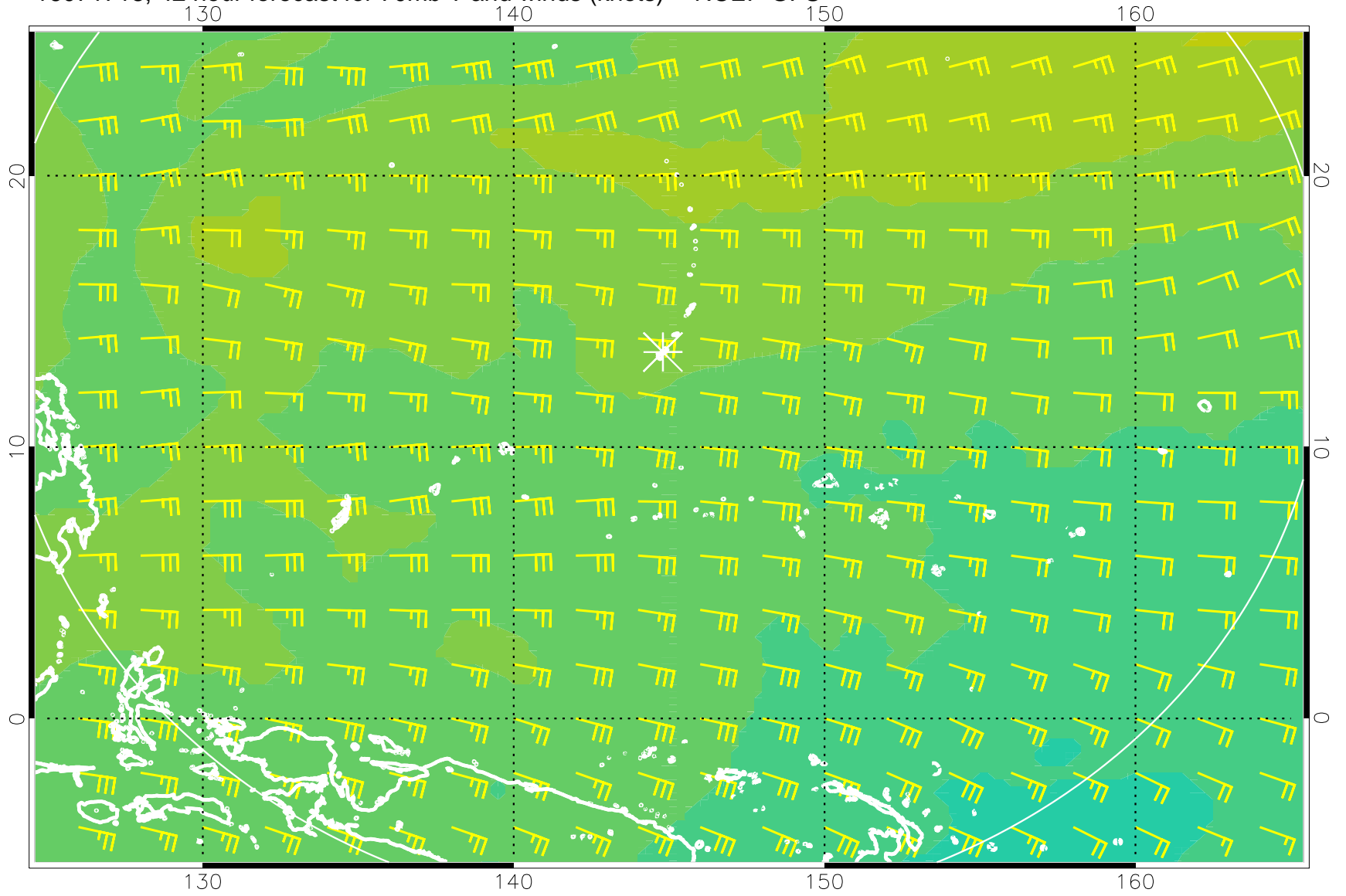
16071718, 42 hour forecast for 70mb T and winds (knots) -- NCEP GFS
