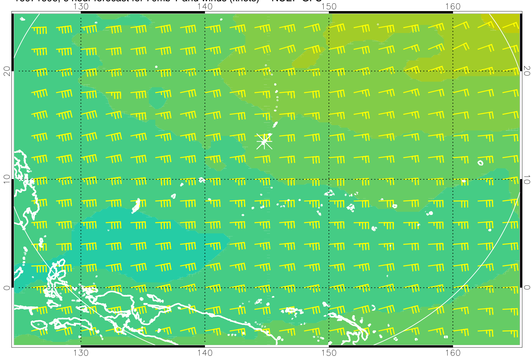
16071606, 6 hour forecast for 70mb T and winds (knots) -- NCEP GFS
