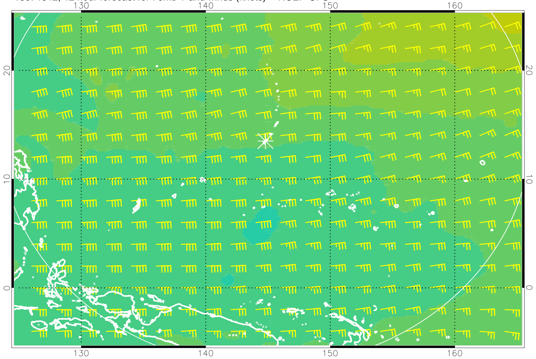
16071612, 12 hour forecast for 70mb T and winds (knots) -- NCEP GFS
