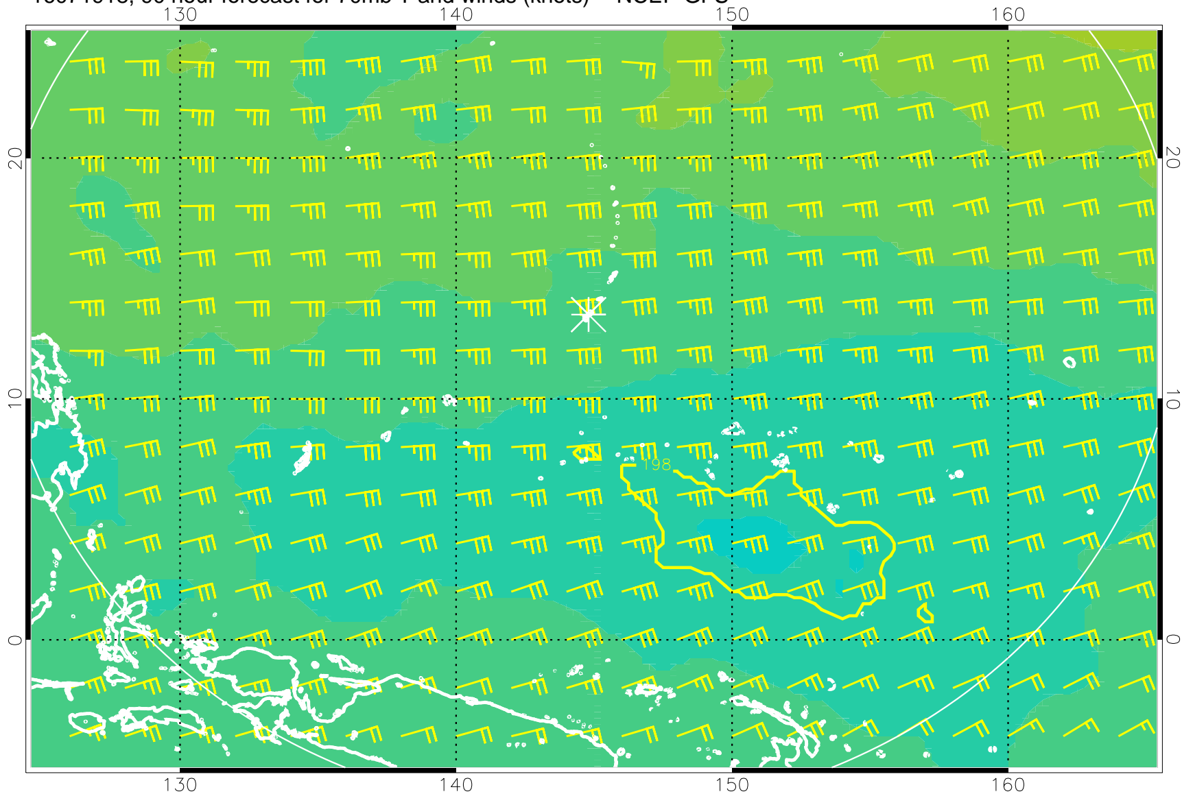
16071918, 90 hour forecast for 70mb T and winds (knots) -- NCEP GFS
