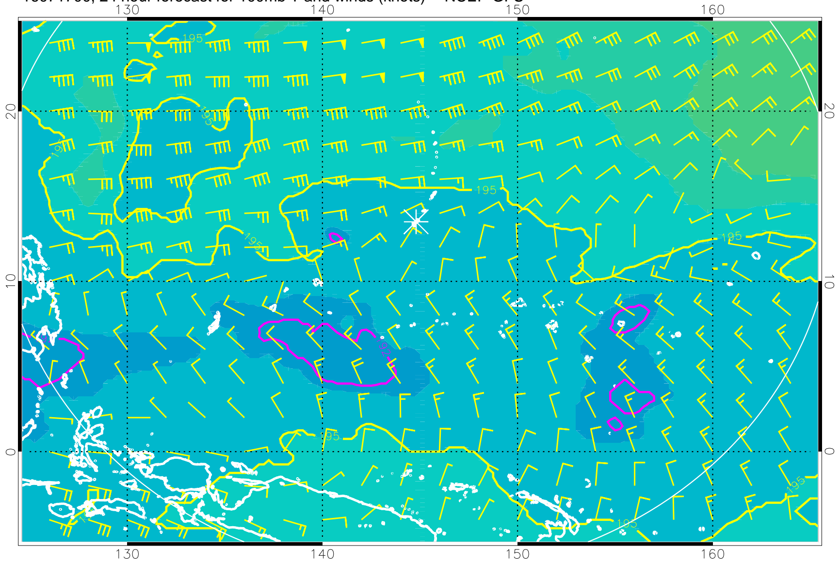
16071700, 24 hour forecast for 100mb T and winds (knots) -- NCEP GFS
