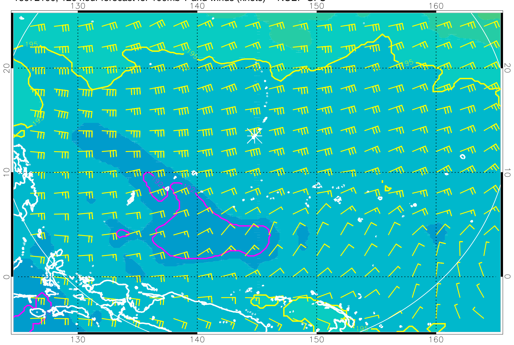
16072100, 120 hour forecast for 100mb T and winds (knots) -- NCEP GFS
