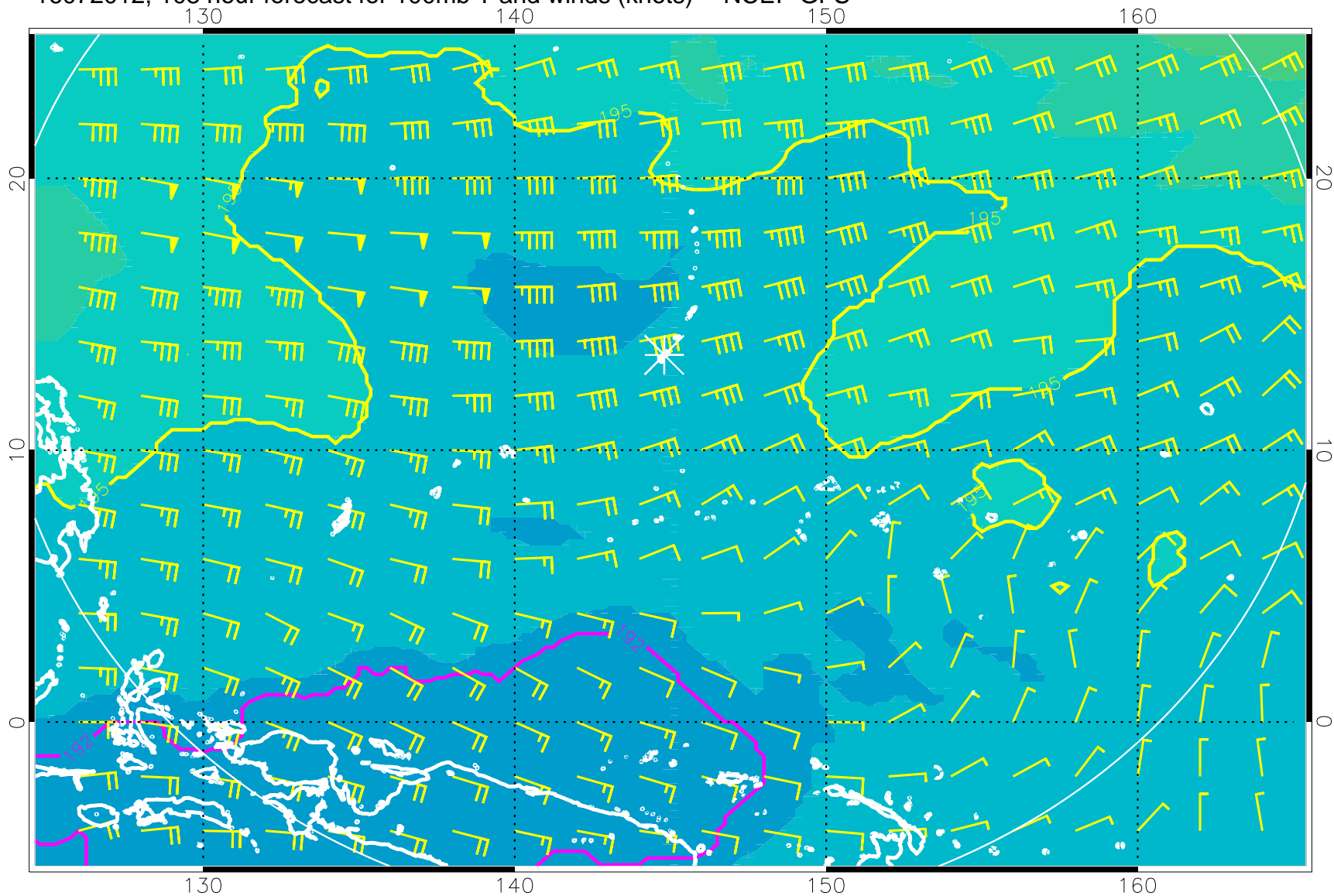
16072012, 108 hour forecast for 100mb T and winds (knots) -- NCEP GFS
