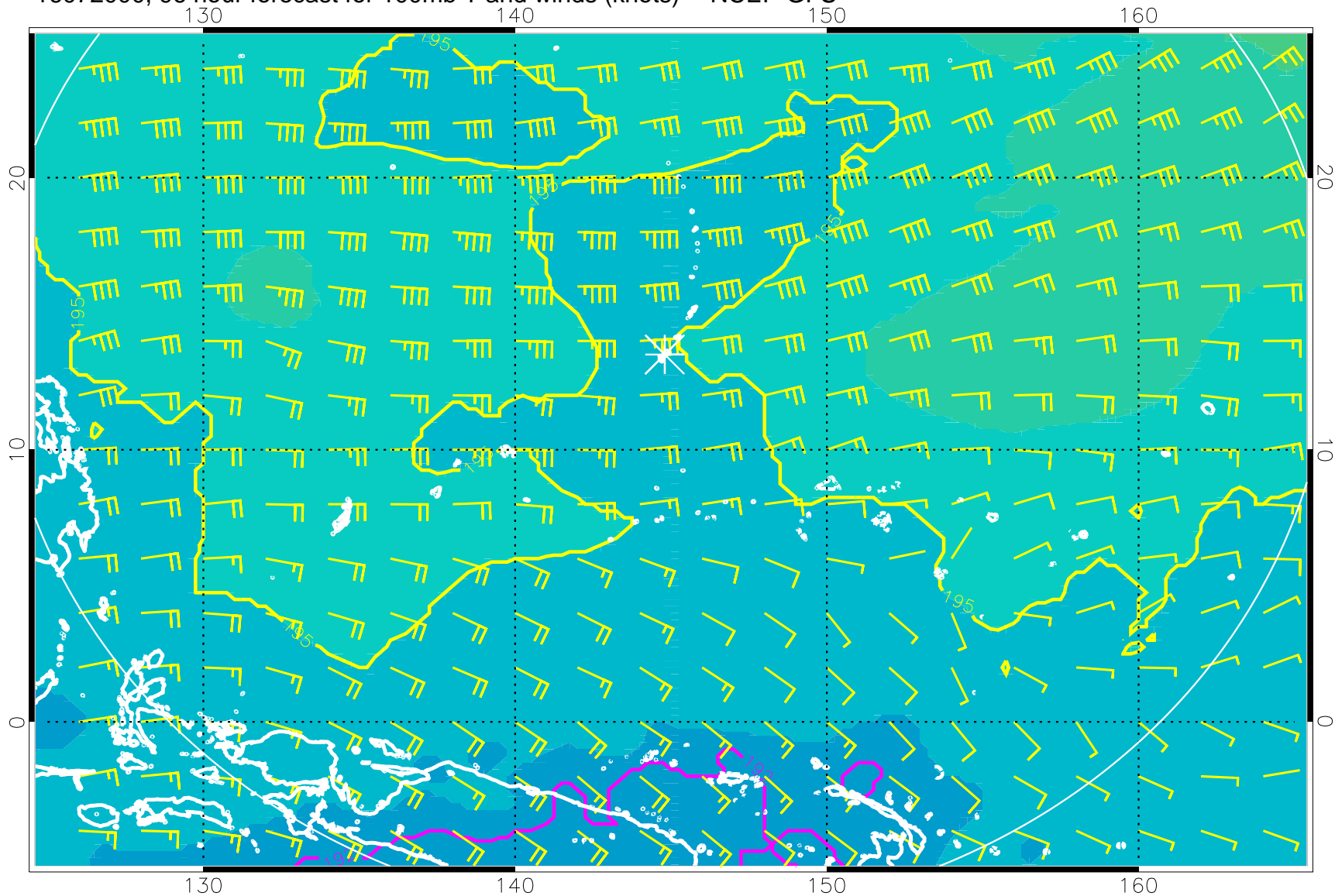
16072000, 96 hour forecast for 100mb T and winds (knots) -- NCEP GFS
