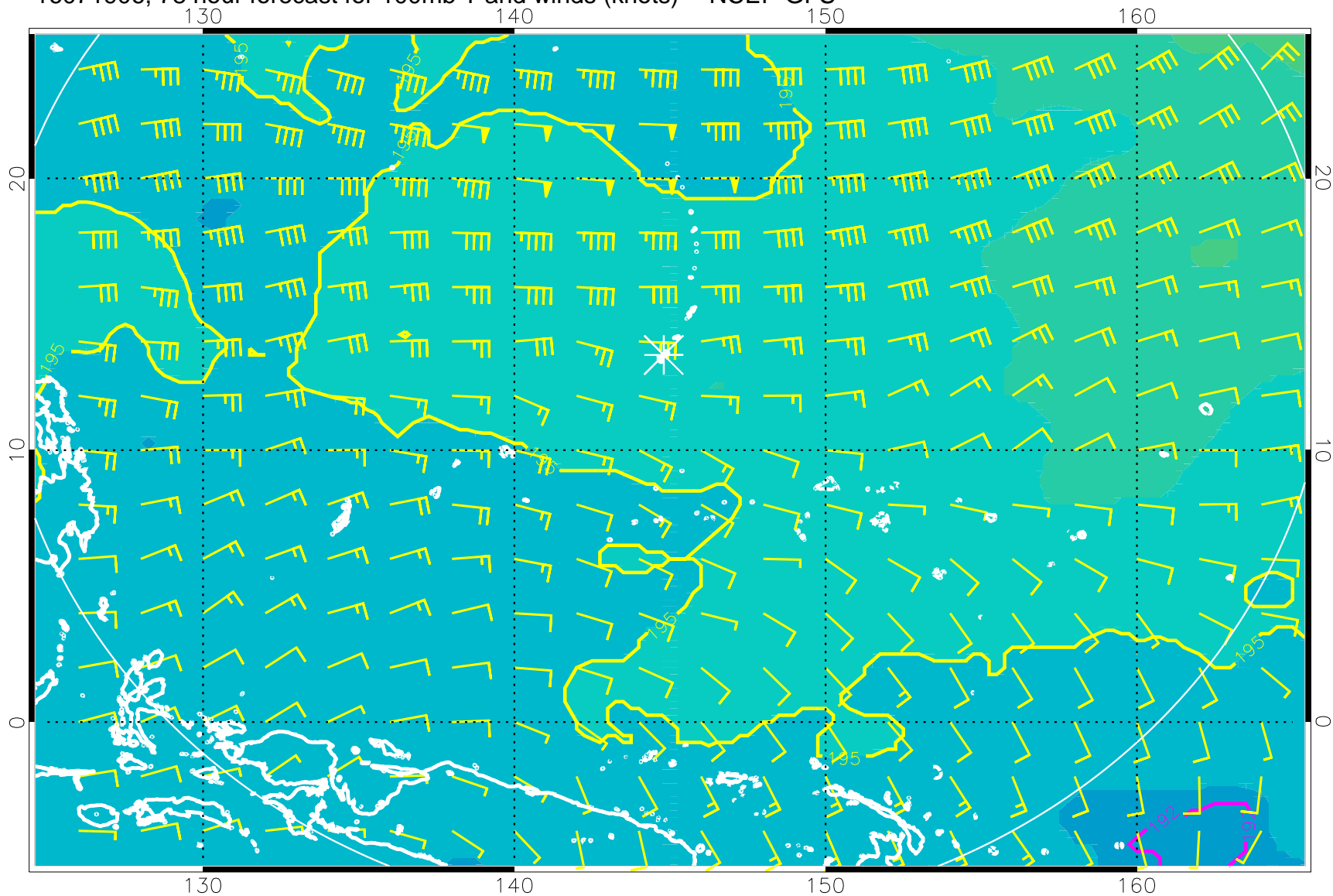
16071906, 78 hour forecast for 100mb T and winds (knots) -- NCEP GFS
