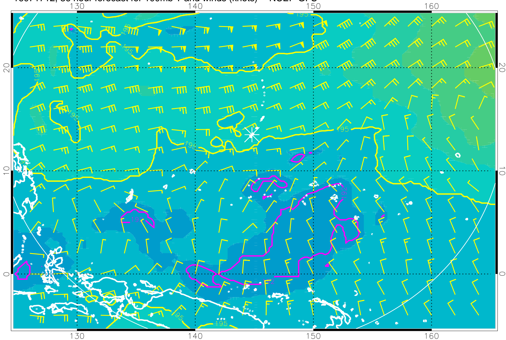
16071712, 36 hour forecast for 100mb T and winds (knots) -- NCEP GFS
