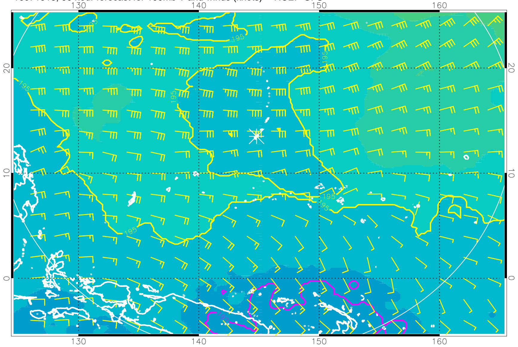
16071918, 90 hour forecast for 100mb T and winds (knots) -- NCEP GFS
