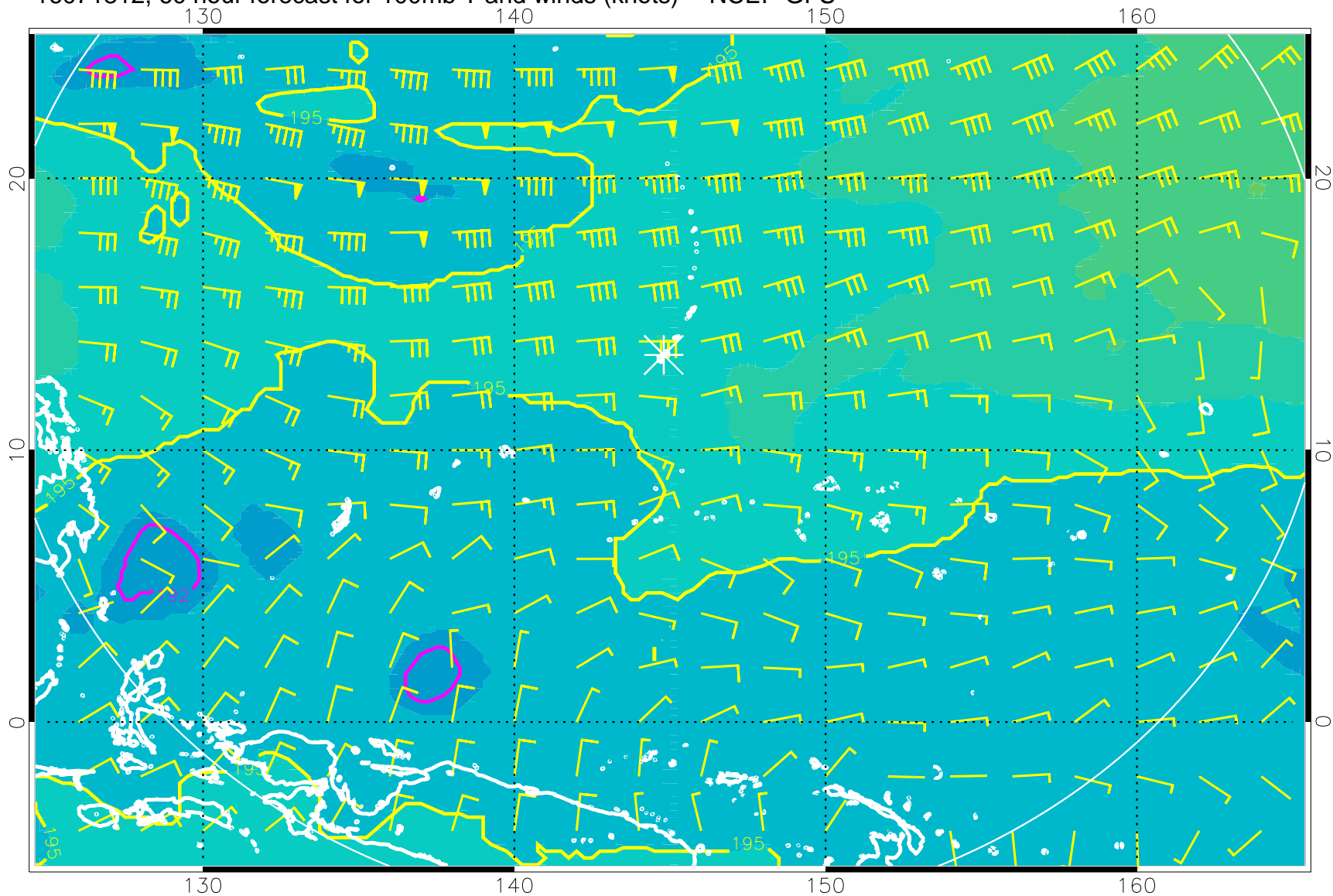
16071812, 60 hour forecast for 100mb T and winds (knots) -- NCEP GFS
