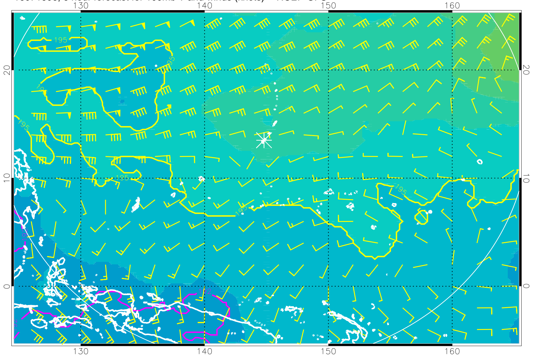
16071606, 6 hour forecast for 100mb T and winds (knots) -- NCEP GFS
