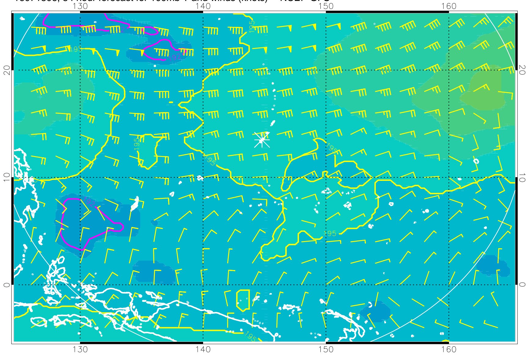
16071806, 54 hour forecast for 100mb T and winds (knots) -- NCEP GFS
