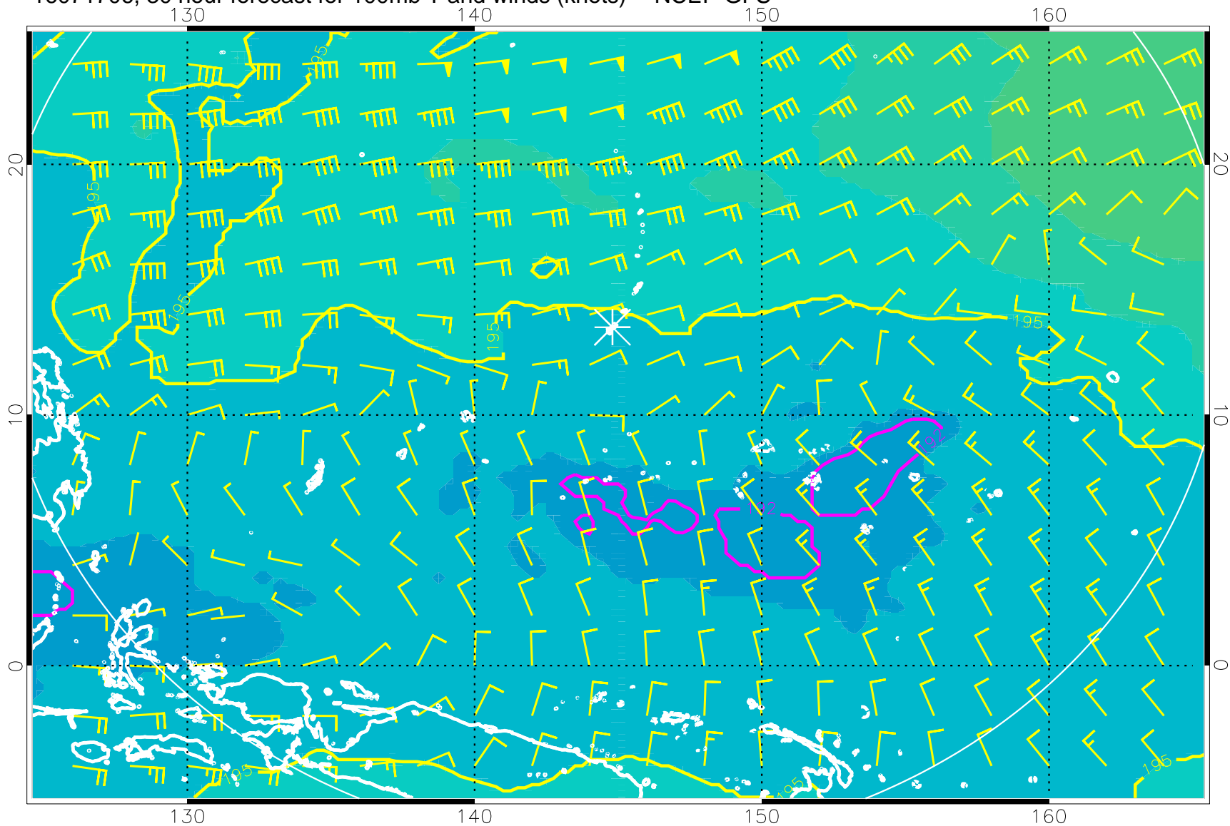
16071706, 30 hour forecast for 100mb T and winds (knots) -- NCEP GFS
