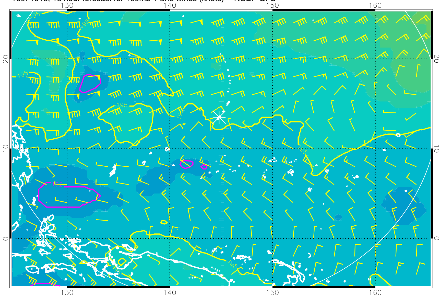
16071618, 18 hour forecast for 100mb T and winds (knots) -- NCEP GFS
