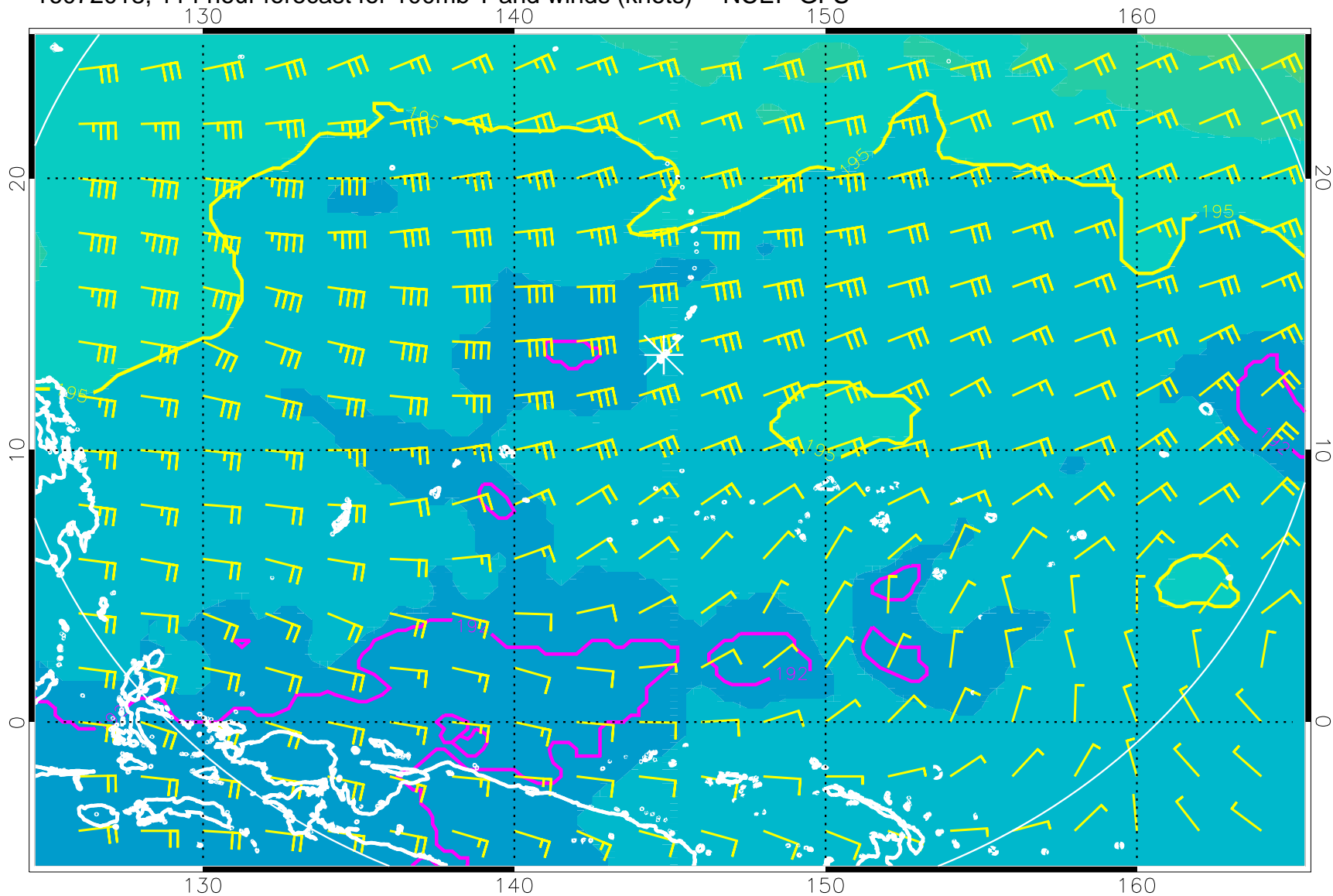
16072018, 114 hour forecast for 100mb T and winds (knots) -- NCEP GFS
