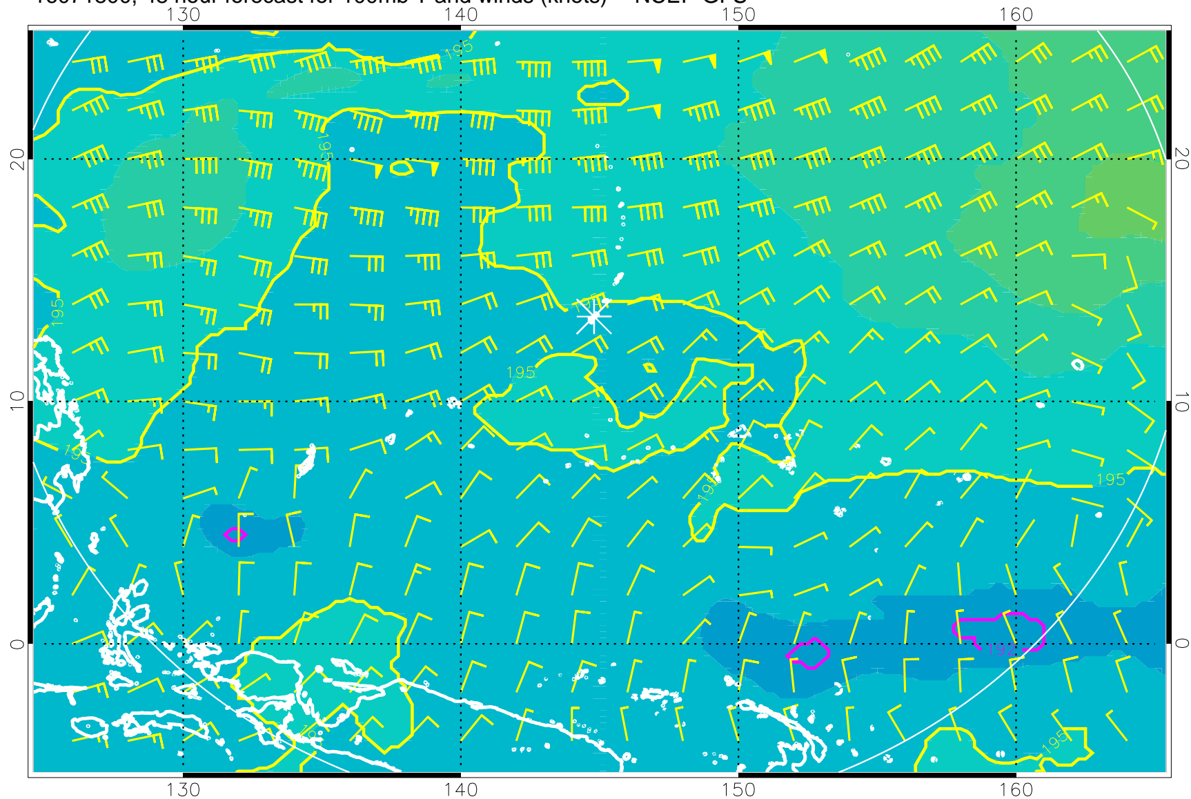
16071800, 48 hour forecast for 100mb T and winds (knots) -- NCEP GFS
