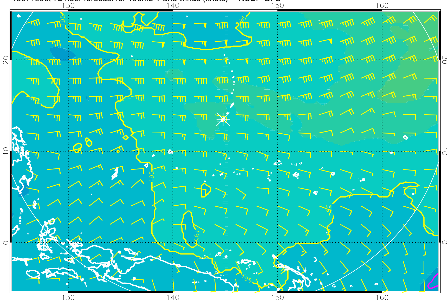
16071900, 72 hour forecast for 100mb T and winds (knots) -- NCEP GFS
