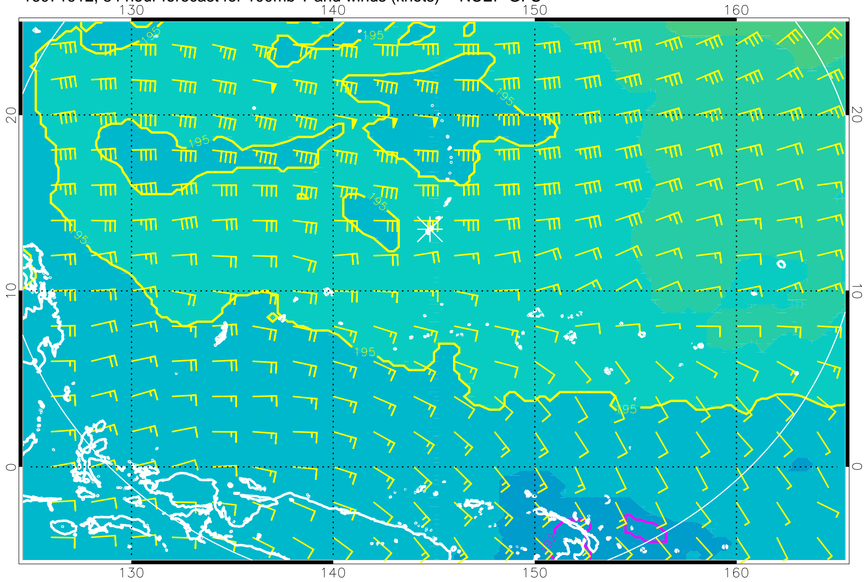
16071912, 84 hour forecast for 100mb T and winds (knots) -- NCEP GFS
