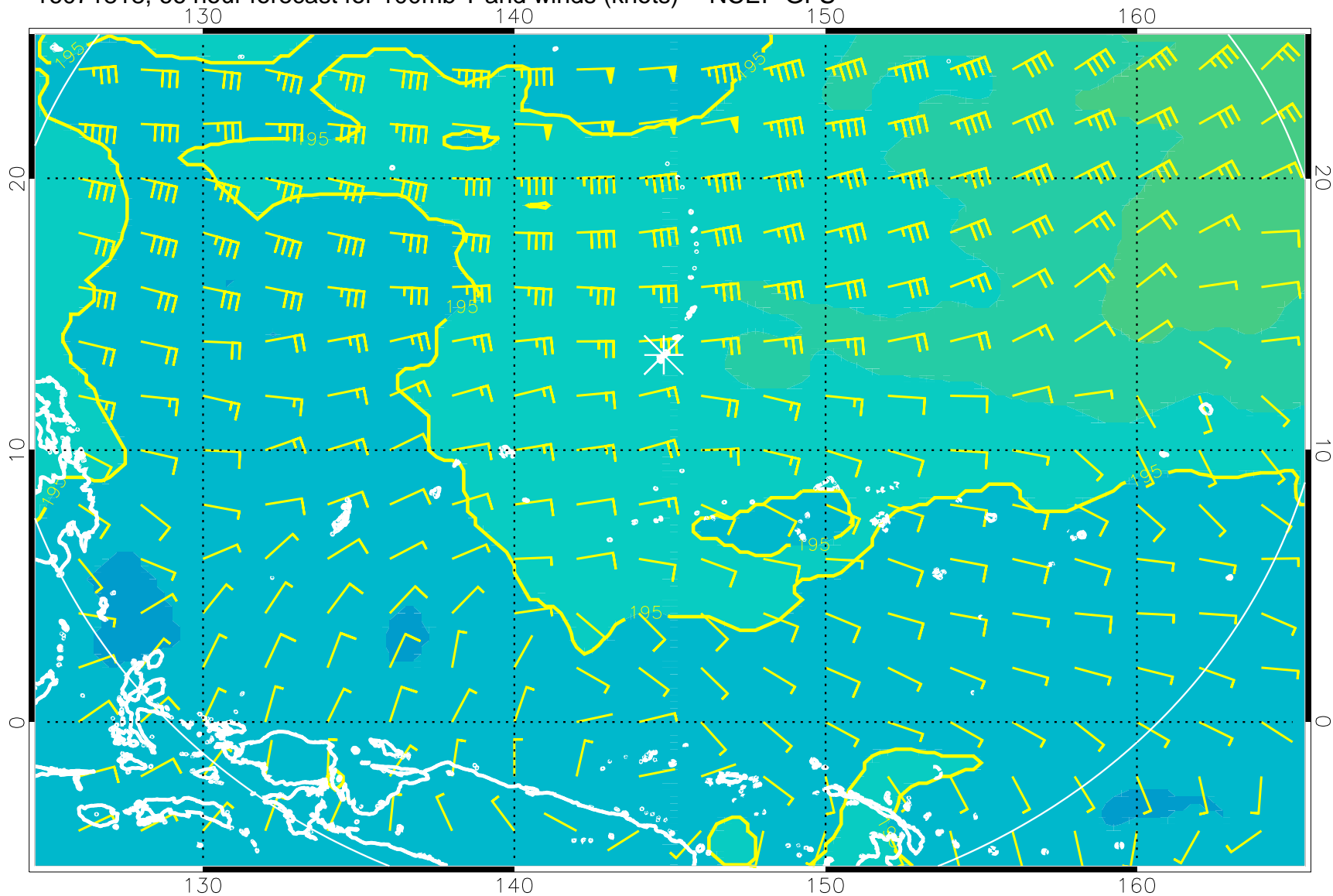
16071818, 66 hour forecast for 100mb T and winds (knots) -- NCEP GFS
