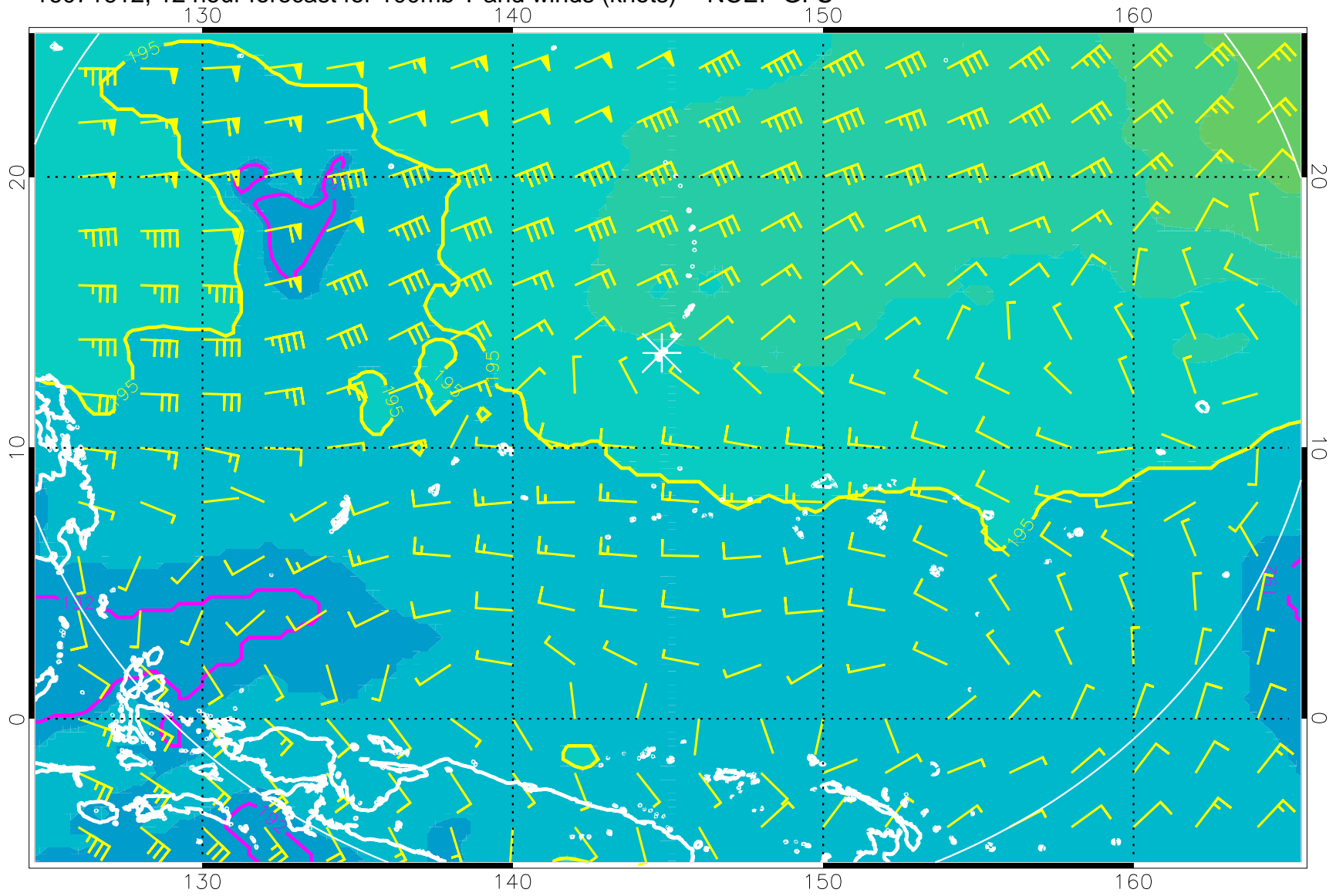
16071612, 12 hour forecast for 100mb T and winds (knots) -- NCEP GFS
