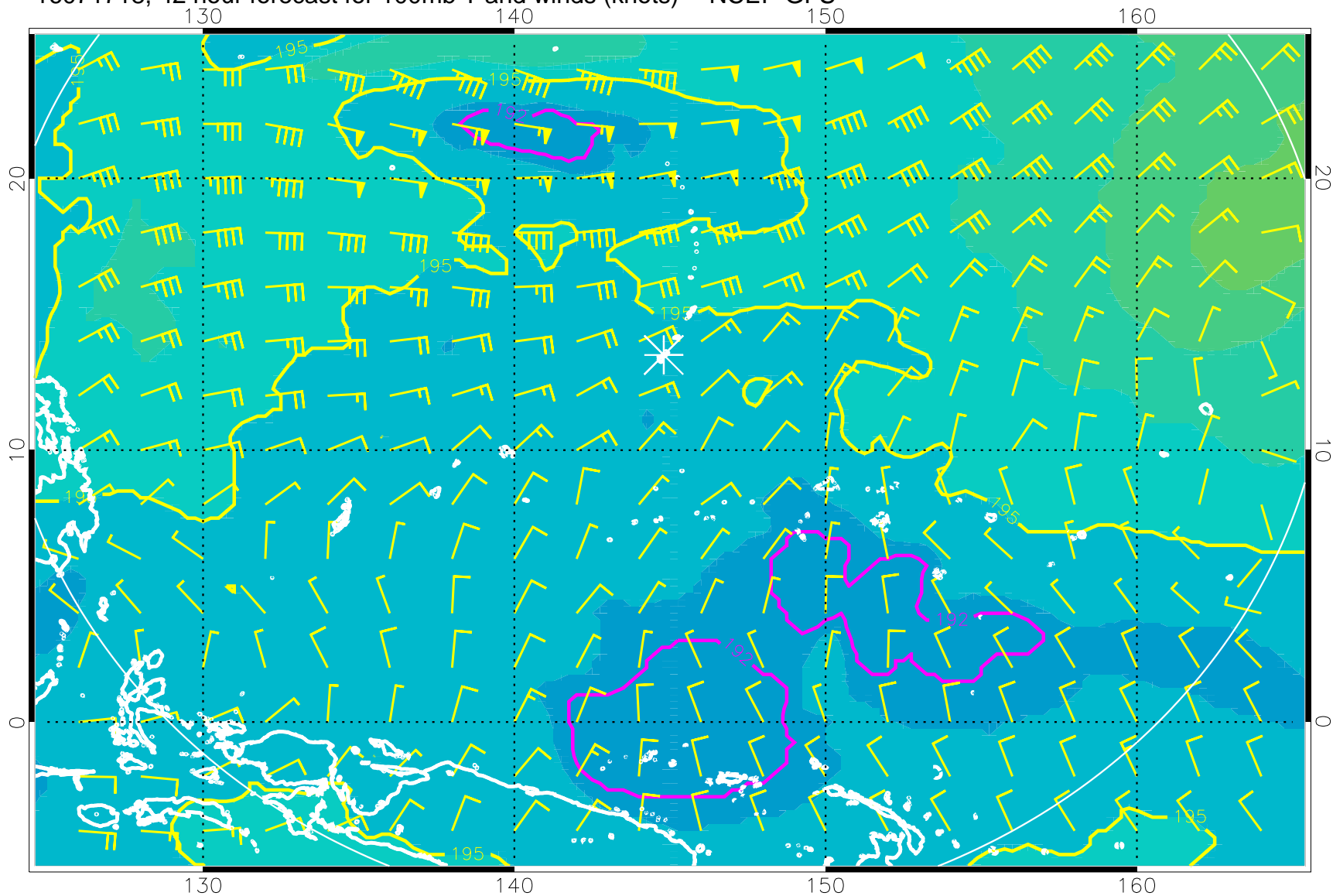
16071718, 42 hour forecast for 100mb T and winds (knots) -- NCEP GFS
