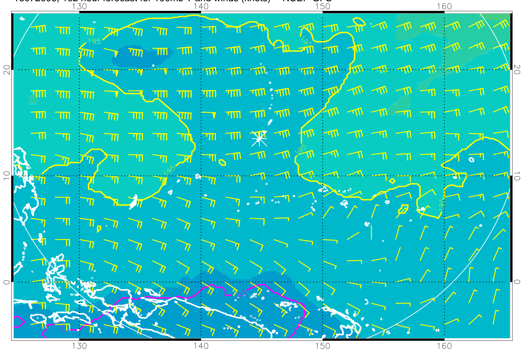
16072006, 102 hour forecast for 100mb T and winds (knots) -- NCEP GFS
