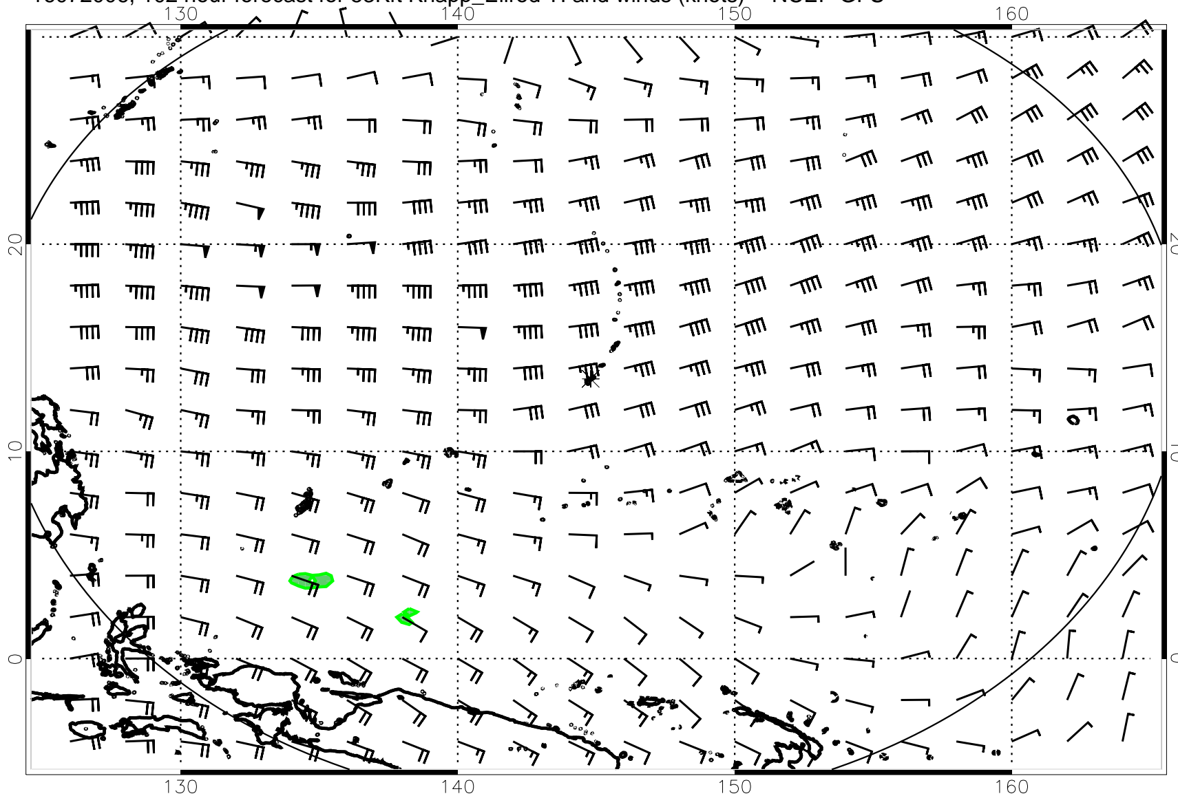
16072006, 102 hour forecast for 53Kft Knapp_Ellrod TI and winds (knots) -- NCEP GFS
