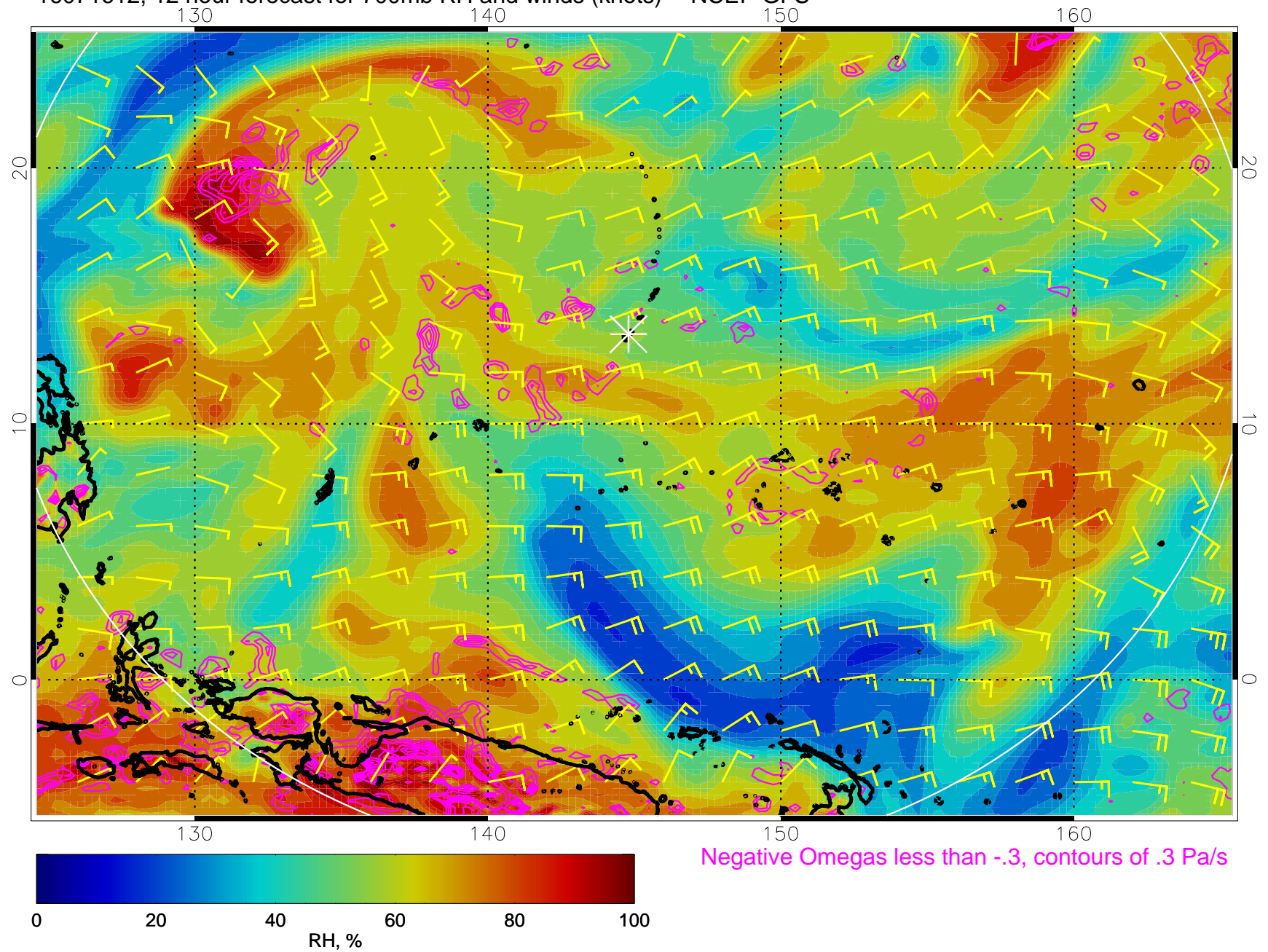
16071612, 12 hour forecast for 700mb RH and winds (knots) -- NCEP GFS
