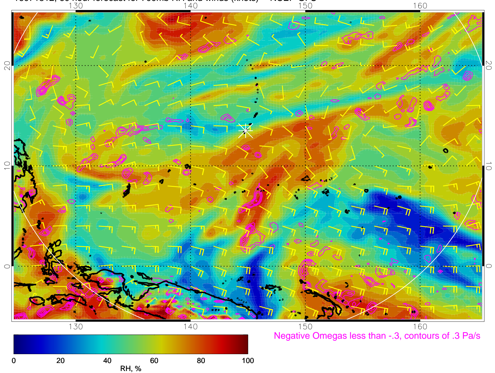
16071812, 60 hour forecast for 700mb RH and winds (knots) -- NCEP GFS
