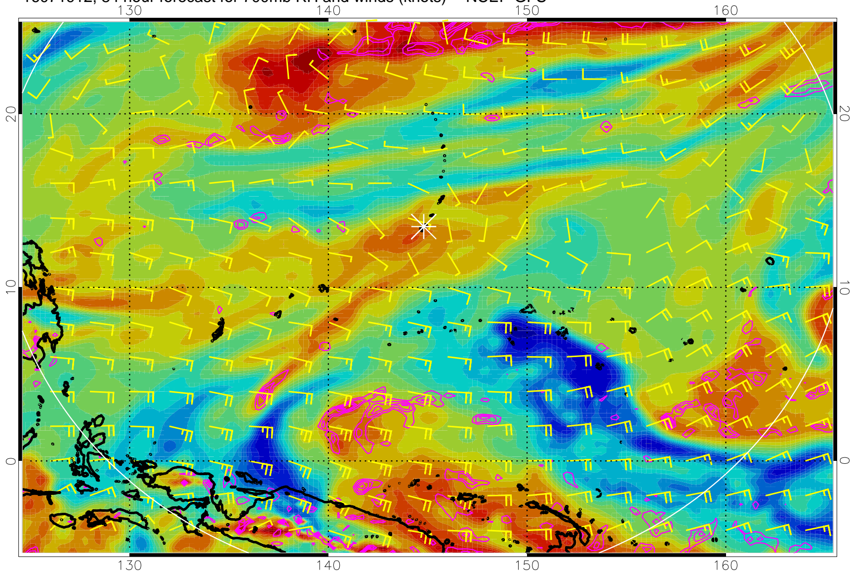
16071912, 84 hour forecast for 700mb RH and winds (knots) -- NCEP GFS
