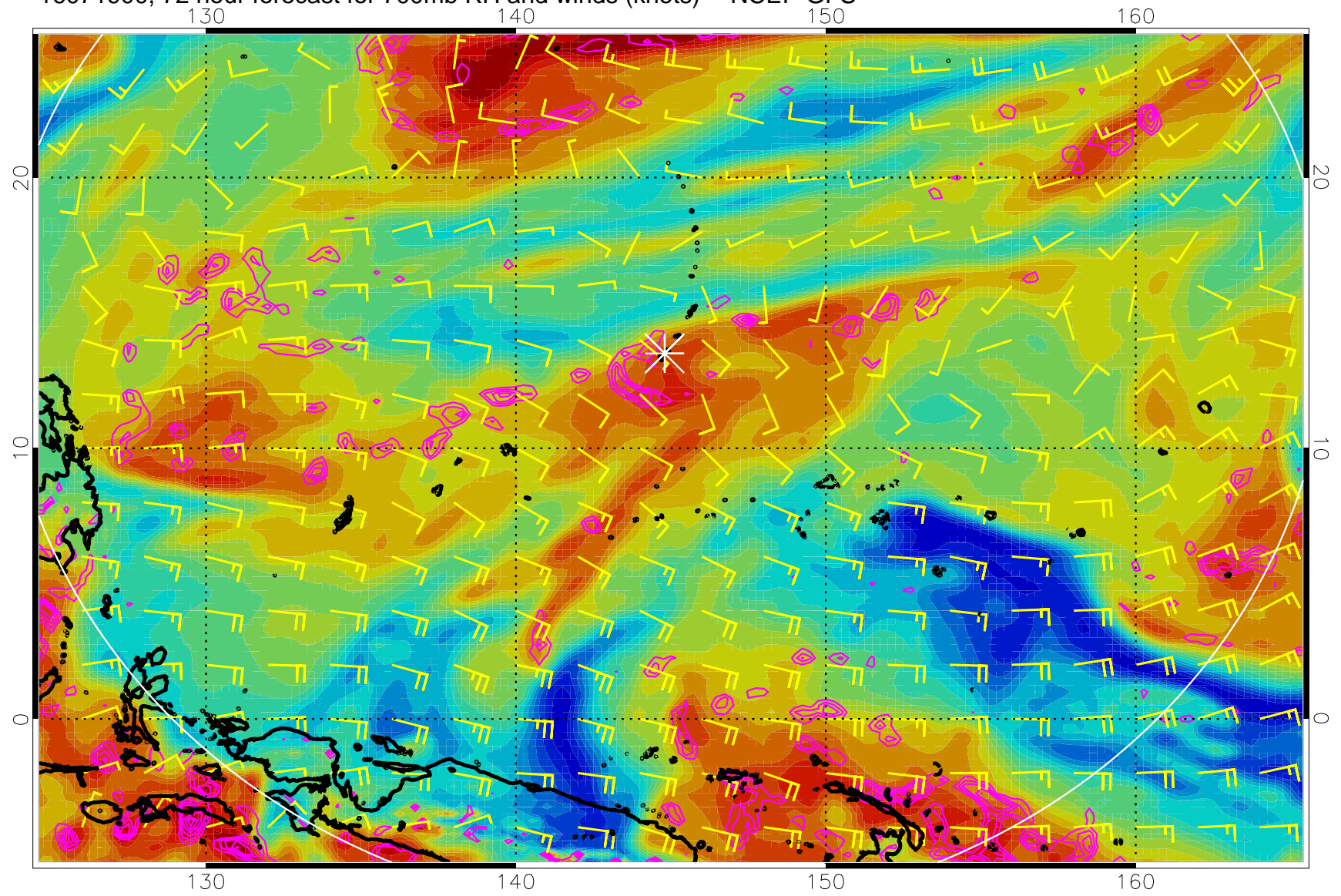
16071900, 72 hour forecast for 700mb RH and winds (knots) -- NCEP GFS
