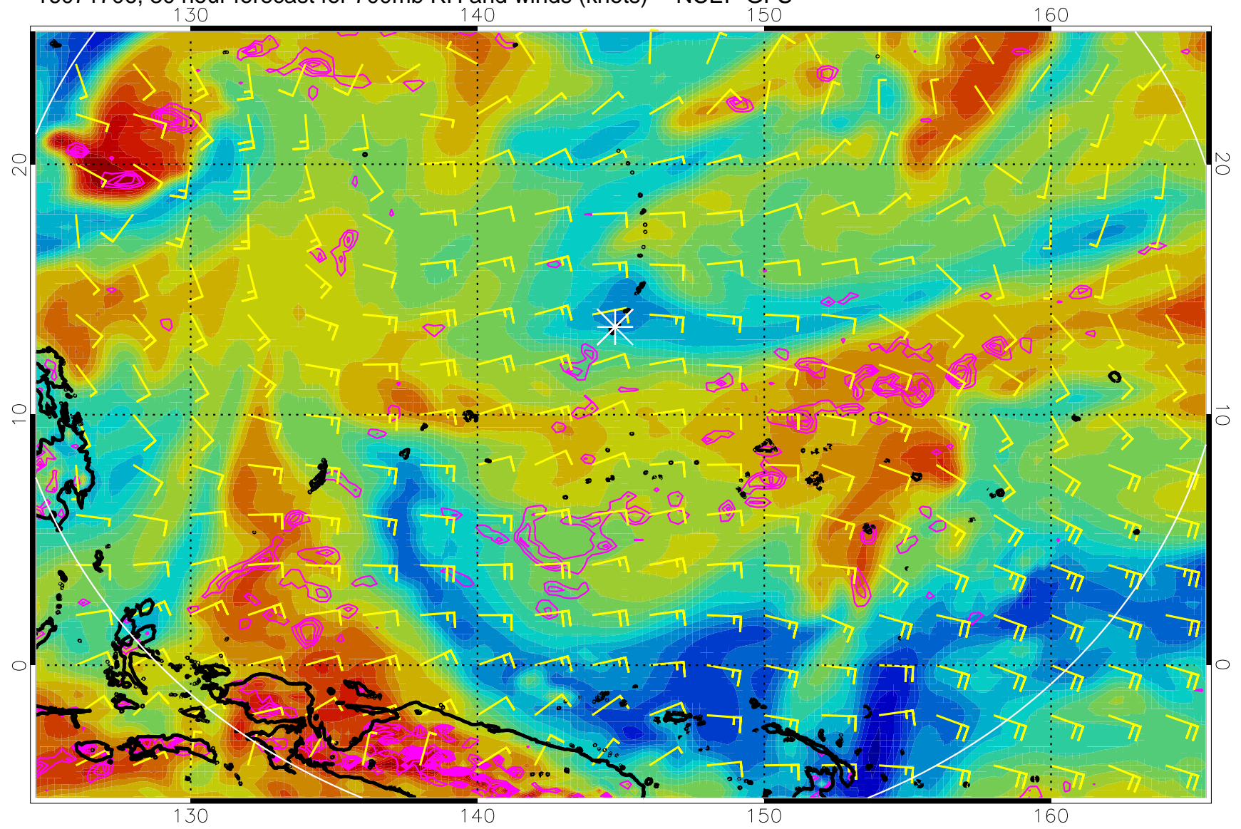
16071706, 30 hour forecast for 700mb RH and winds (knots) -- NCEP GFS
