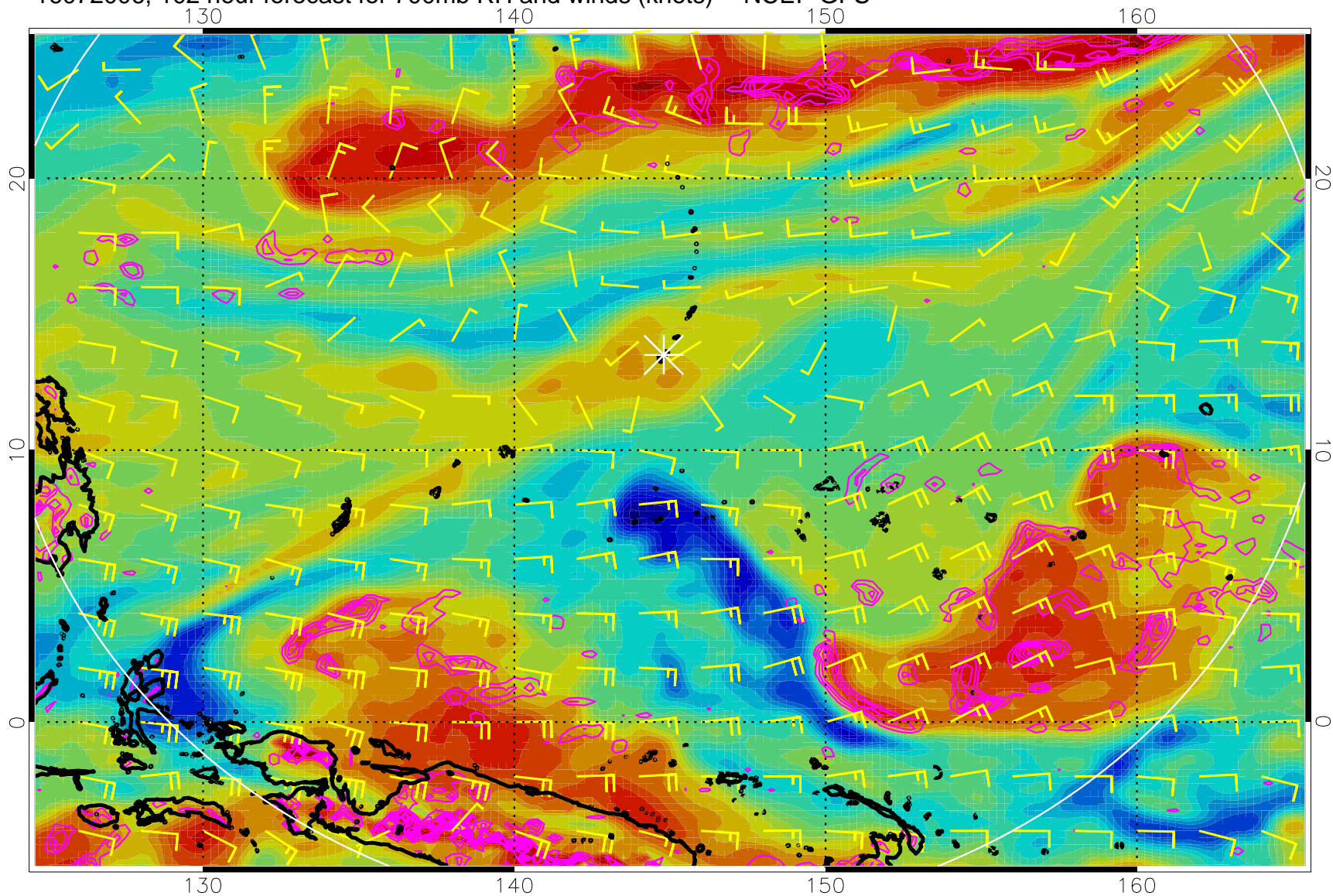
16072006, 102 hour forecast for 700mb RH and winds (knots) -- NCEP GFS
