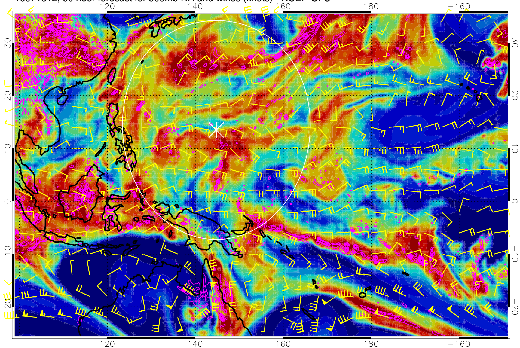
16071812, 60 hour forecast for 500mb RH and winds (knots) - NCEP GFS
