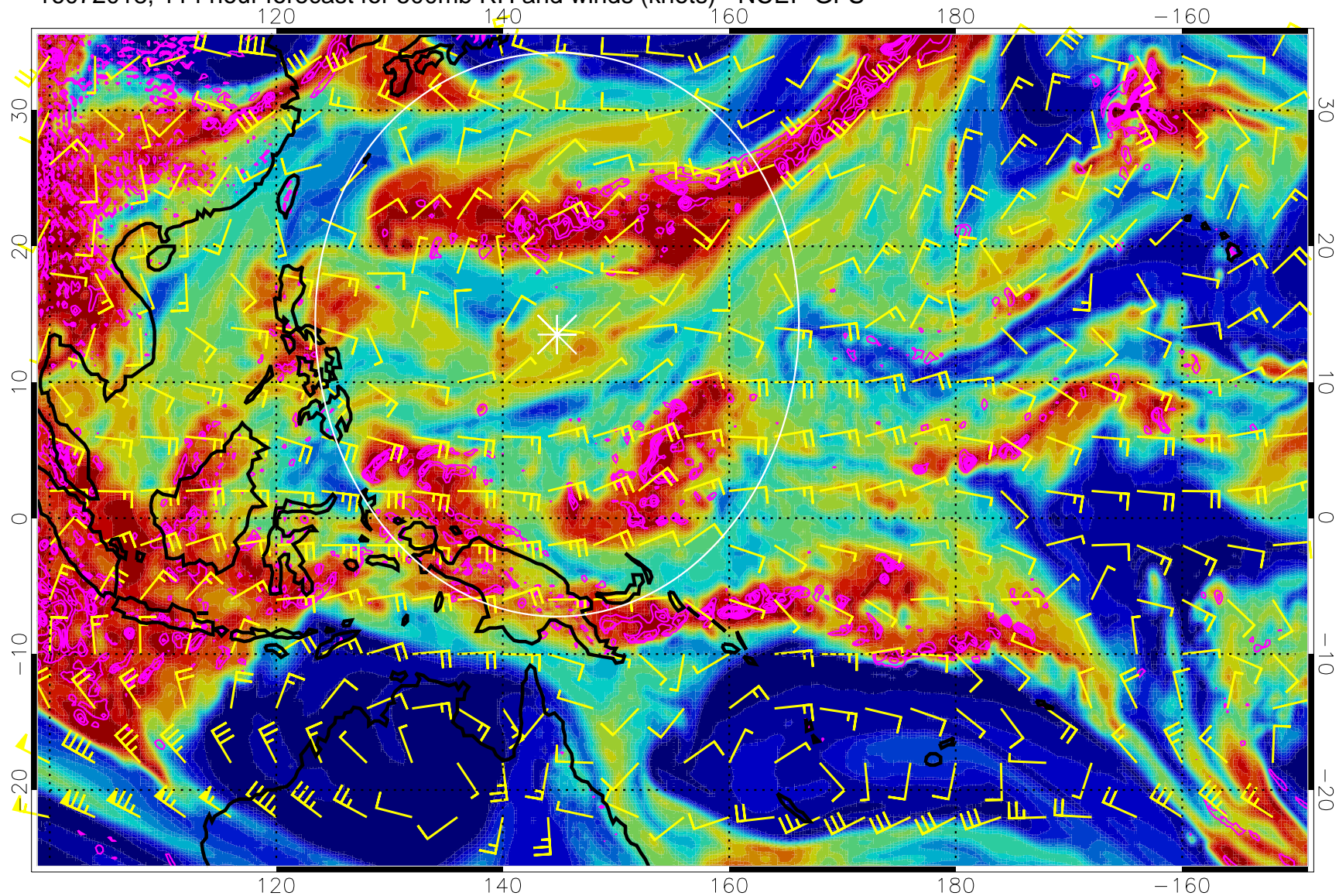
16072018, 114 hour forecast for 500mb RH and winds (knots) - NCEP GFS
