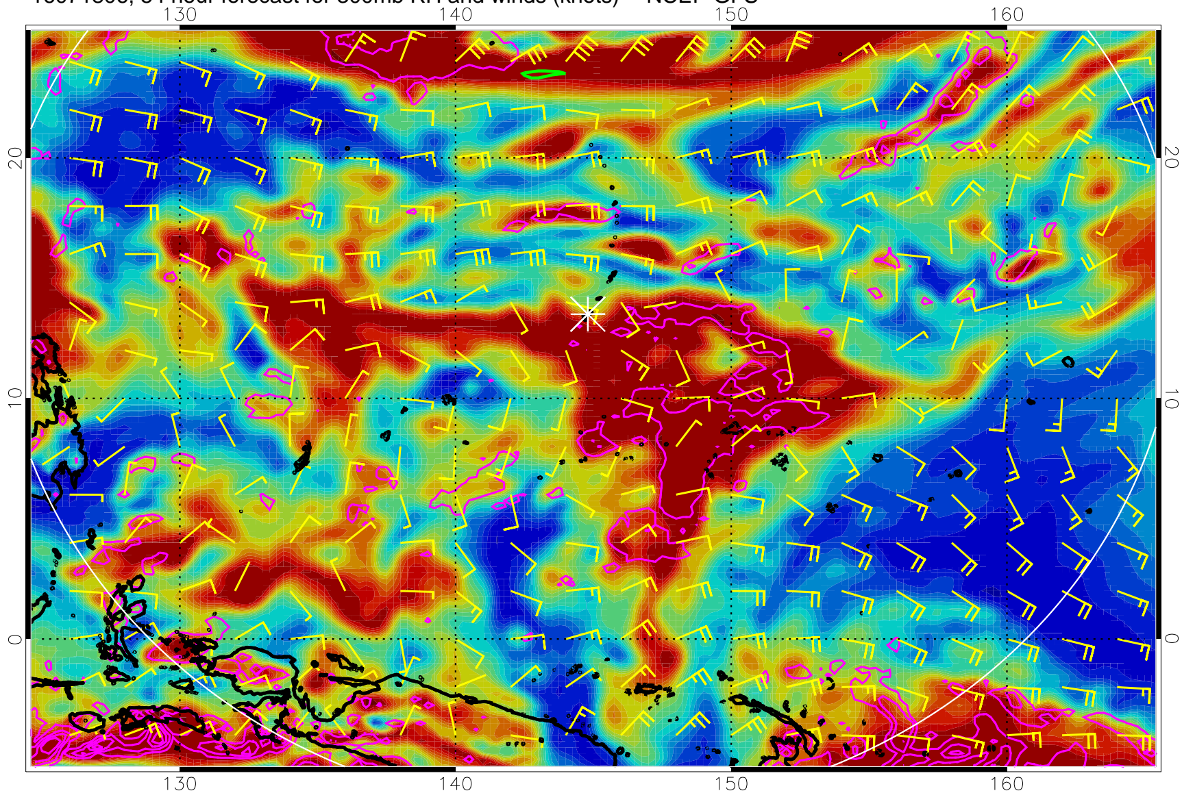
16071806, 54 hour forecast for 300mb RH and winds (knots) -- NCEP GFS
