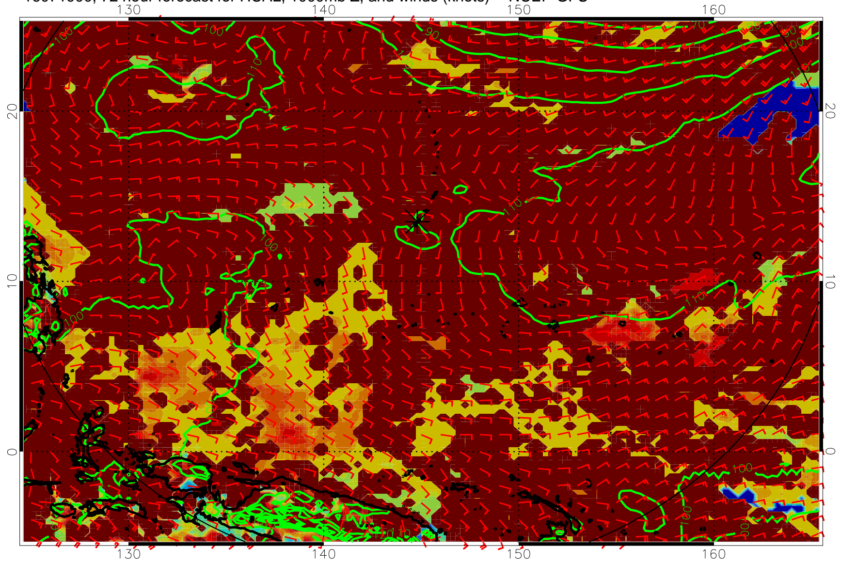
16071900, 72 hour forecast for HCAL, 1000mb Z, and winds (knots) -- NCEP GFS
