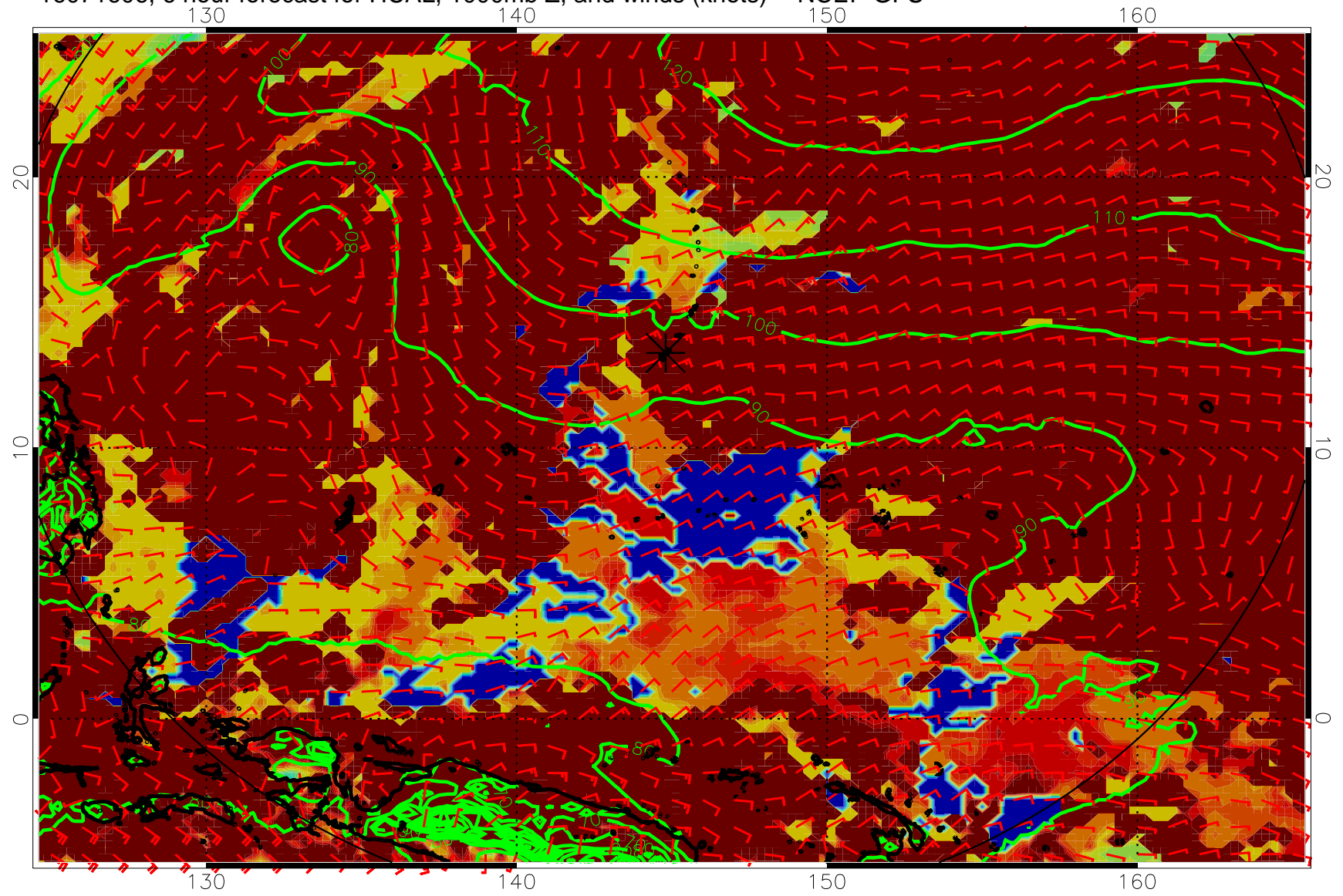
16071606, 6 hour forecast for HCAL, 1000mb Z, and winds (knots) -- NCEP GFS
