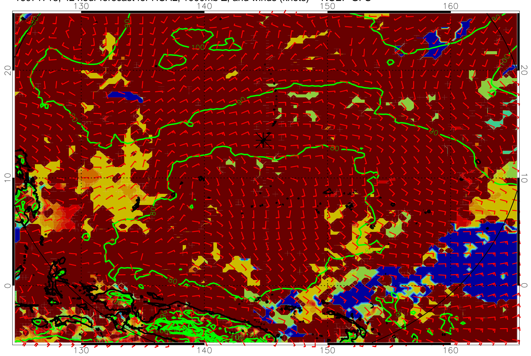
16071718, 42 hour forecast for HCAL, 1000mb Z, and winds (knots) -- NCEP GFS
