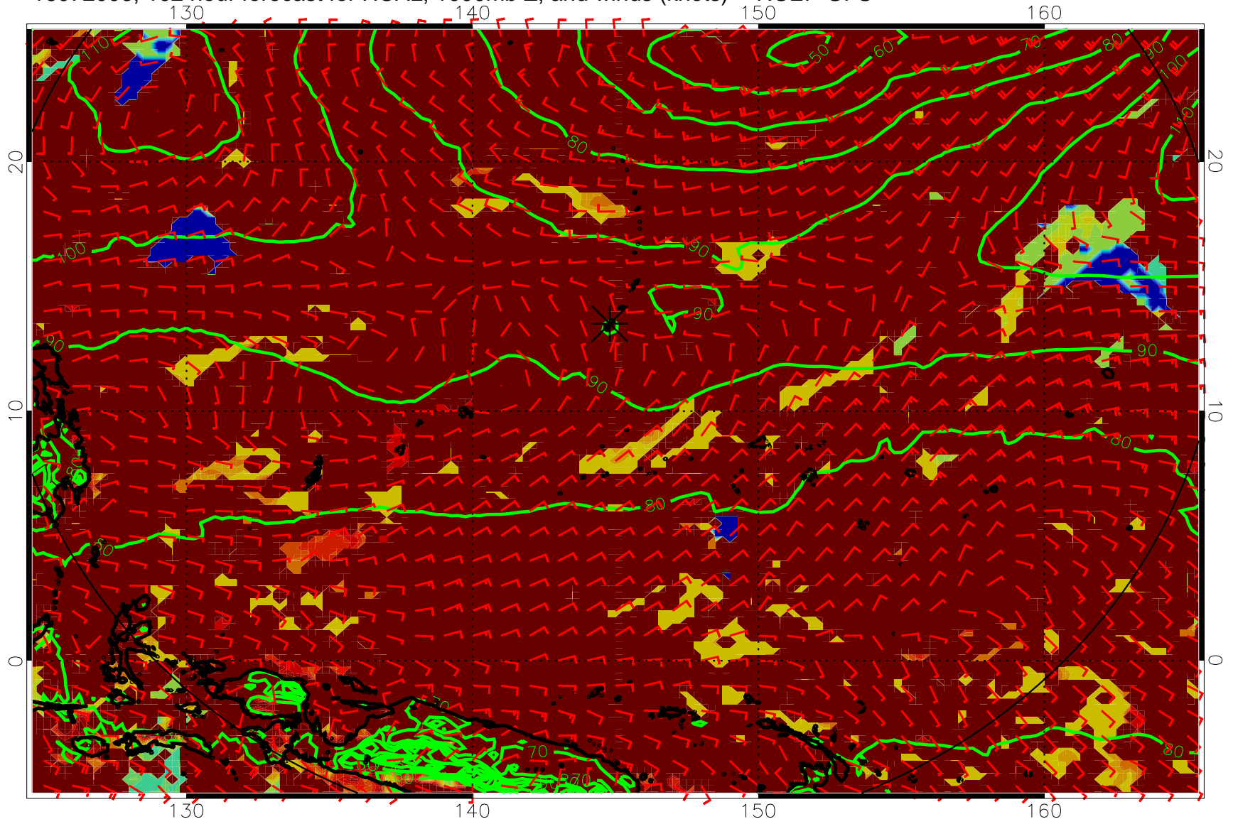
16072006, 102 hour forecast for HCAL, 1000mb Z, and winds (knots) -- NCEP GFS
