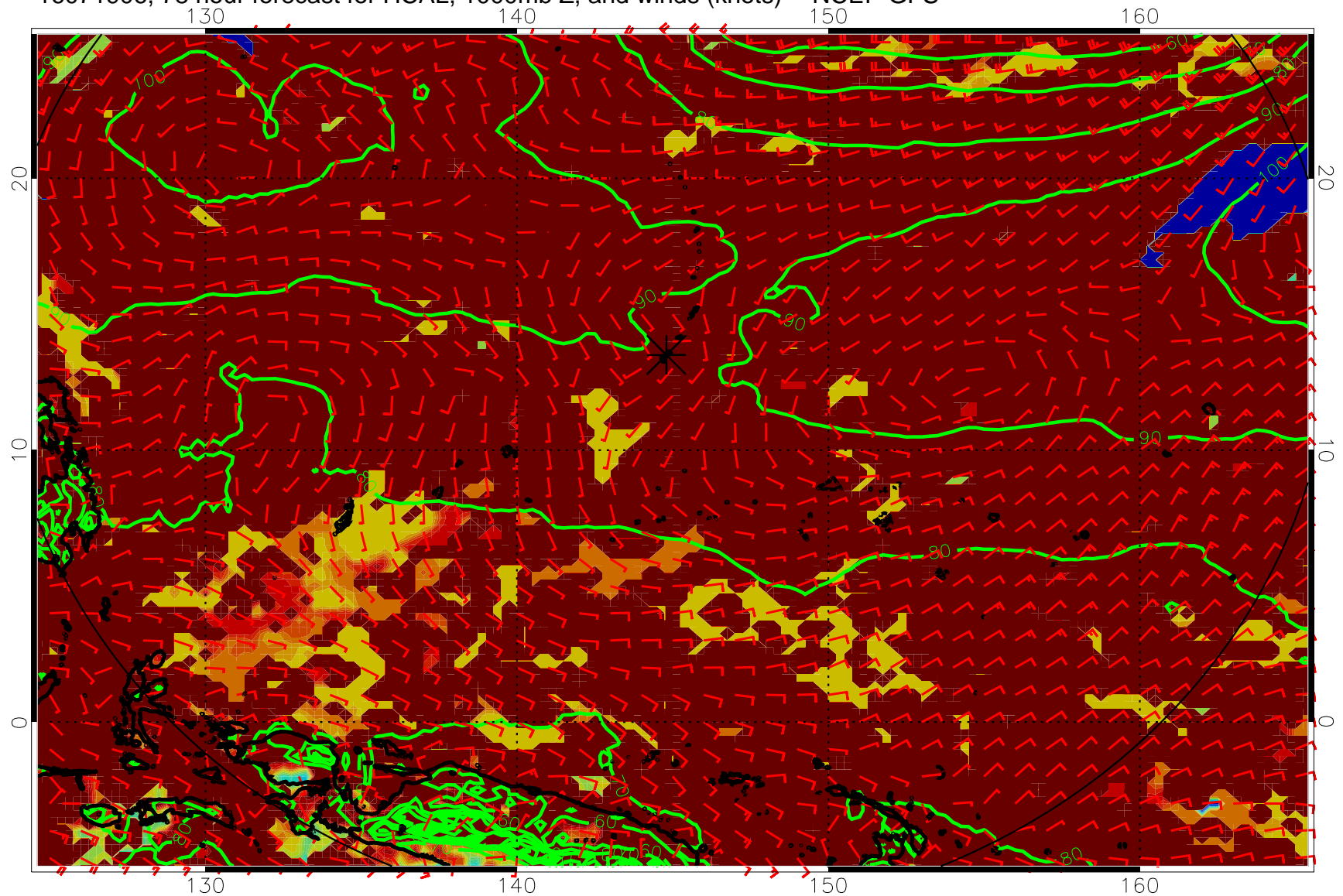
16071906, 78 hour forecast for HCAL, 1000mb Z, and winds (knots) -- NCEP GFS
