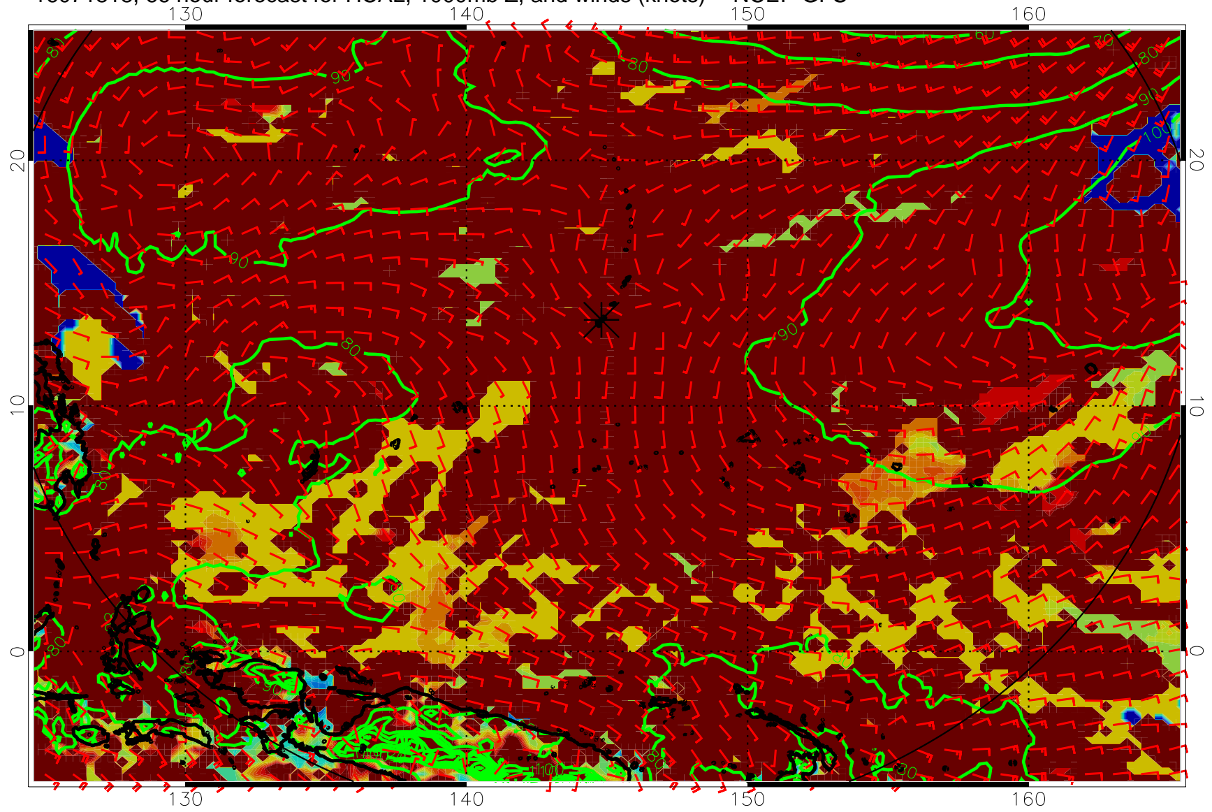
16071818, 66 hour forecast for HCAL, 1000mb Z, and winds (knots) -- NCEP GFS
