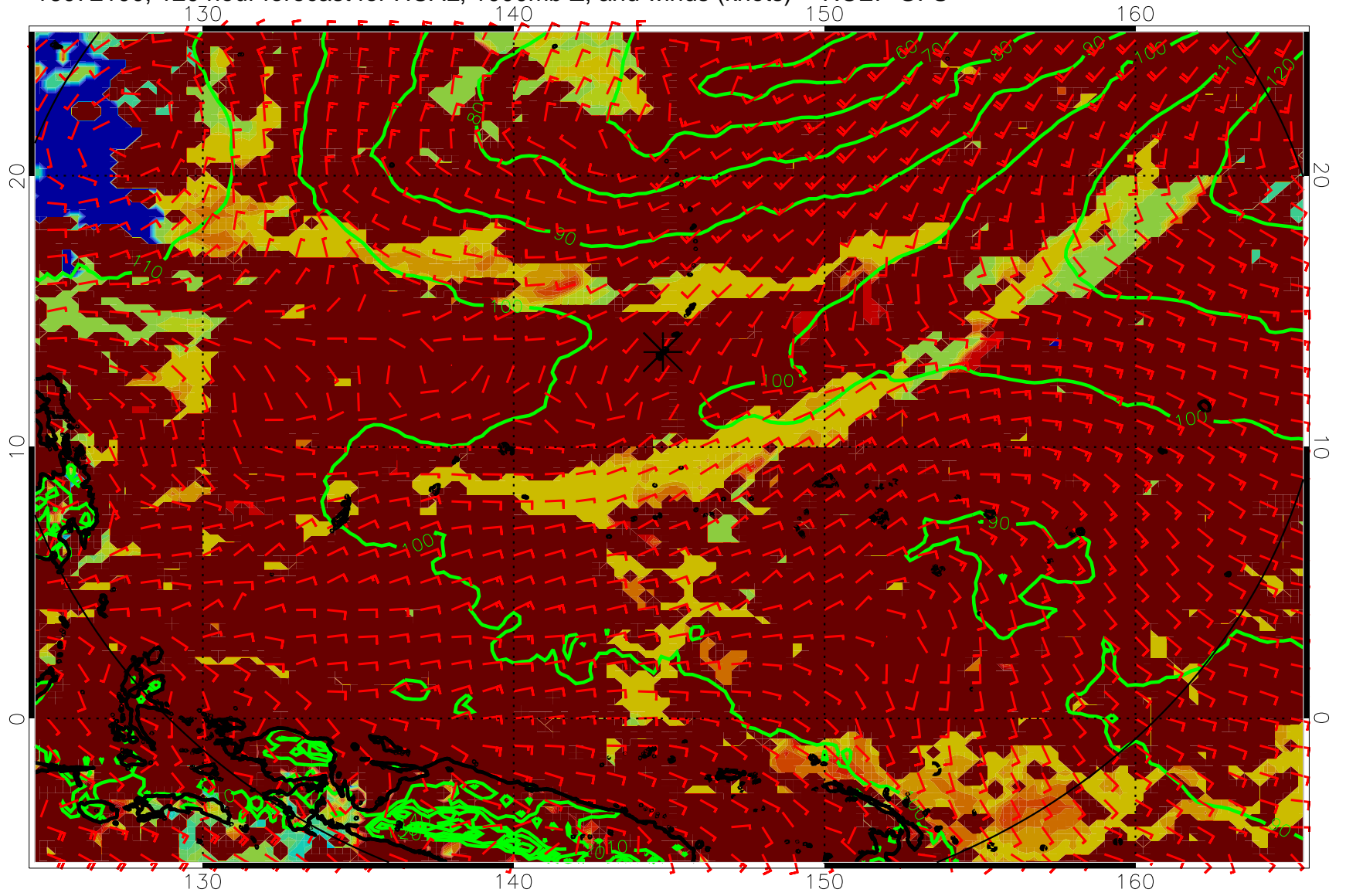
16072100, 120 hour forecast for HCAL, 1000mb Z, and winds (knots) -- NCEP GFS
