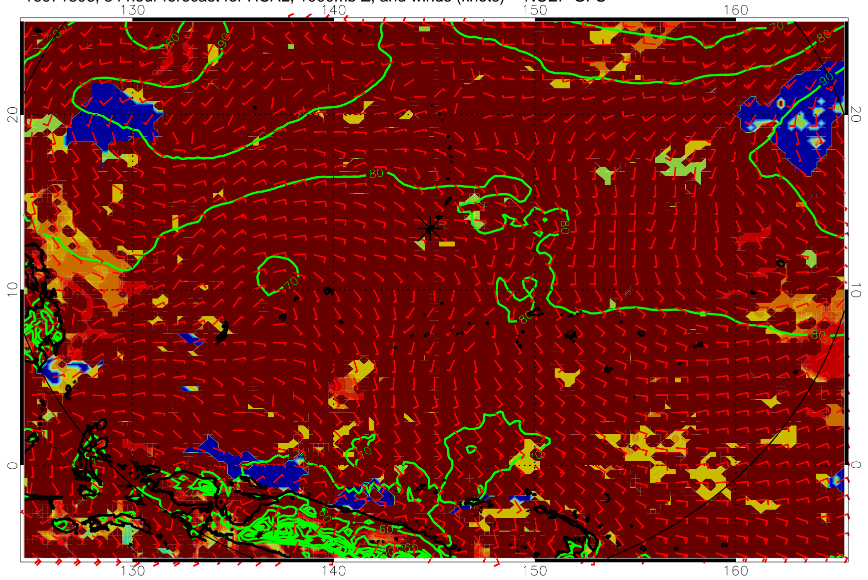
16071806, 54 hour forecast for HCAL, 1000mb Z, and winds (knots) -- NCEP GFS
