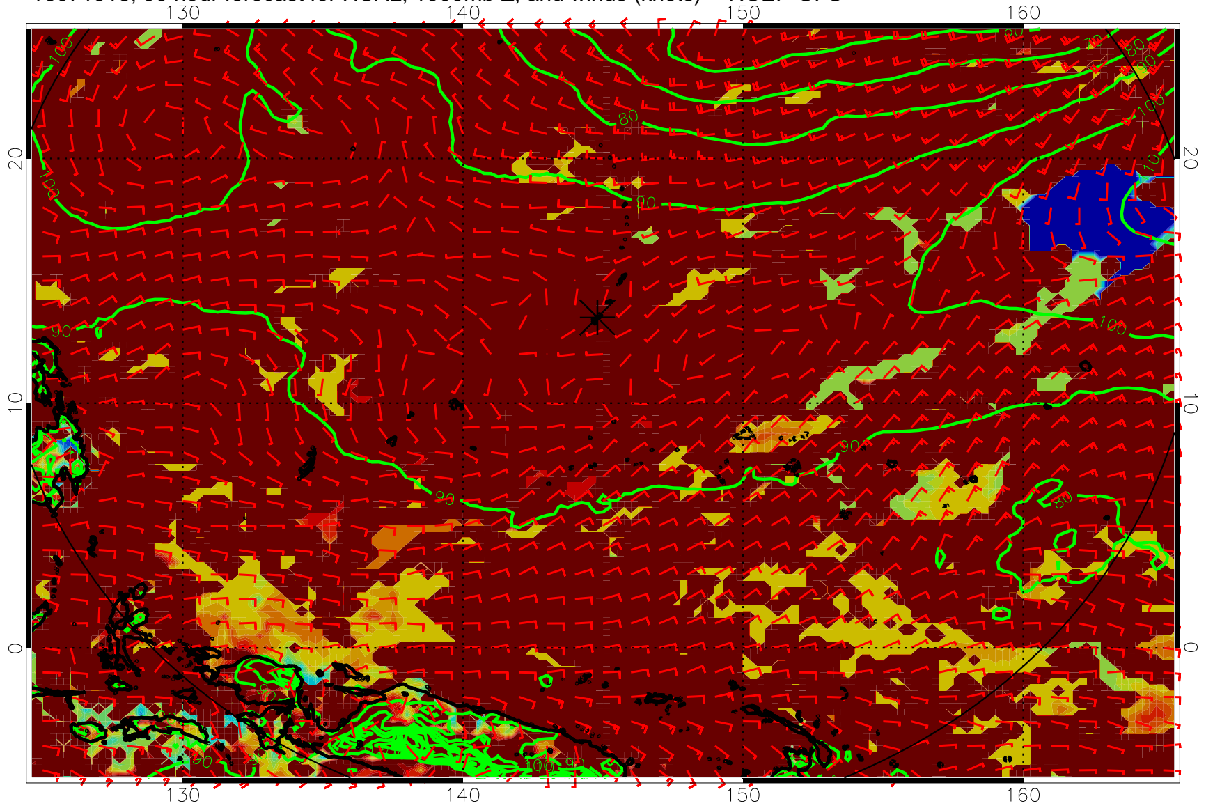
16071918, 90 hour forecast for HCAL, 1000mb Z, and winds (knots) -- NCEP GFS
