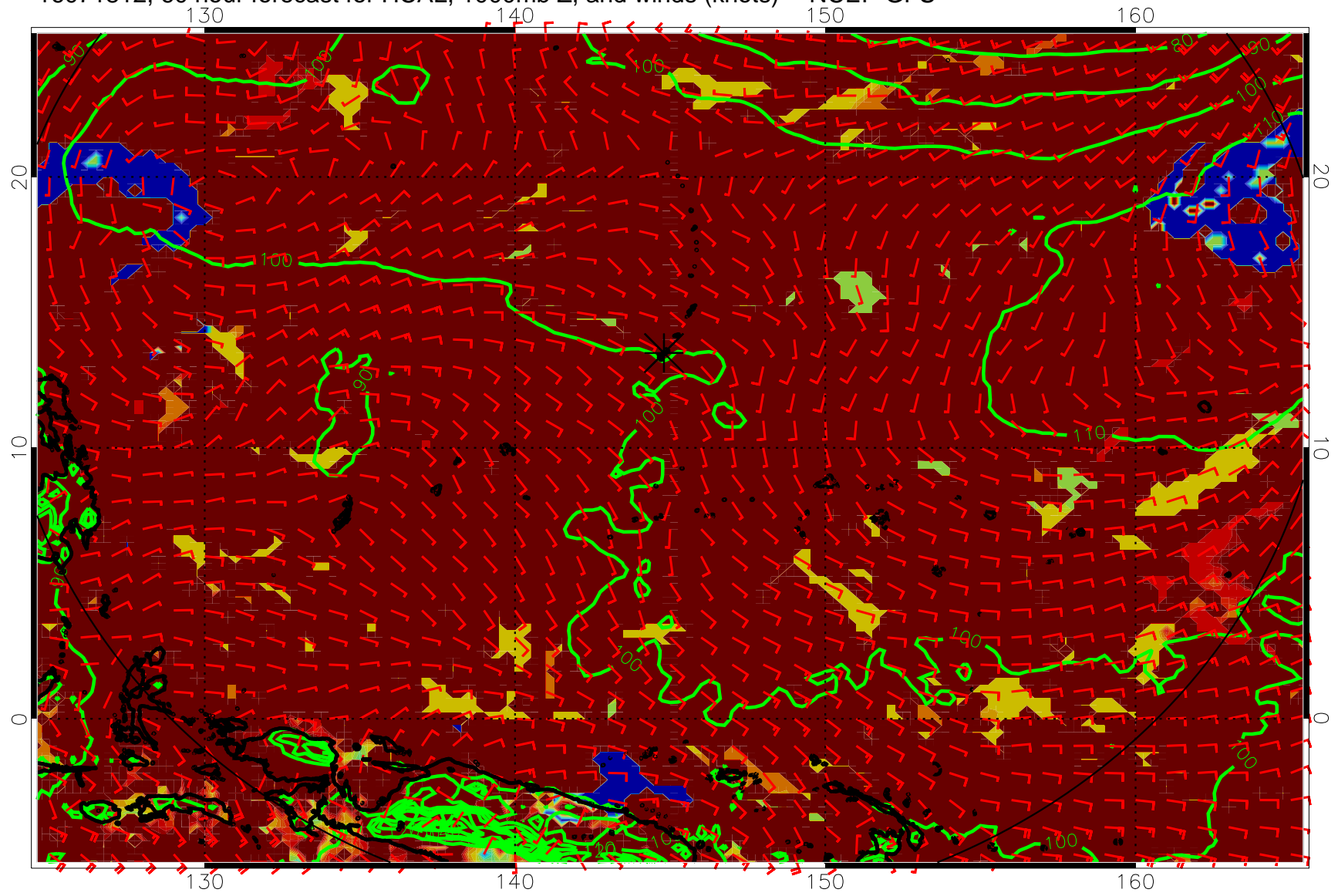
16071812, 60 hour forecast for HCAL, 1000mb Z, and winds (knots) -- NCEP GFS
