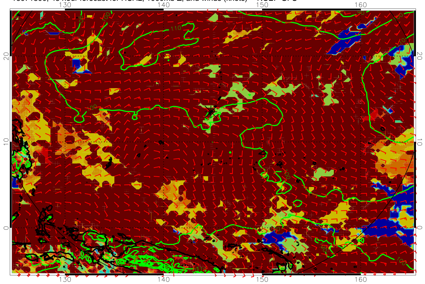
16071800, 48 hour forecast for HCAL, 1000mb Z, and winds (knots) -- NCEP GFS
