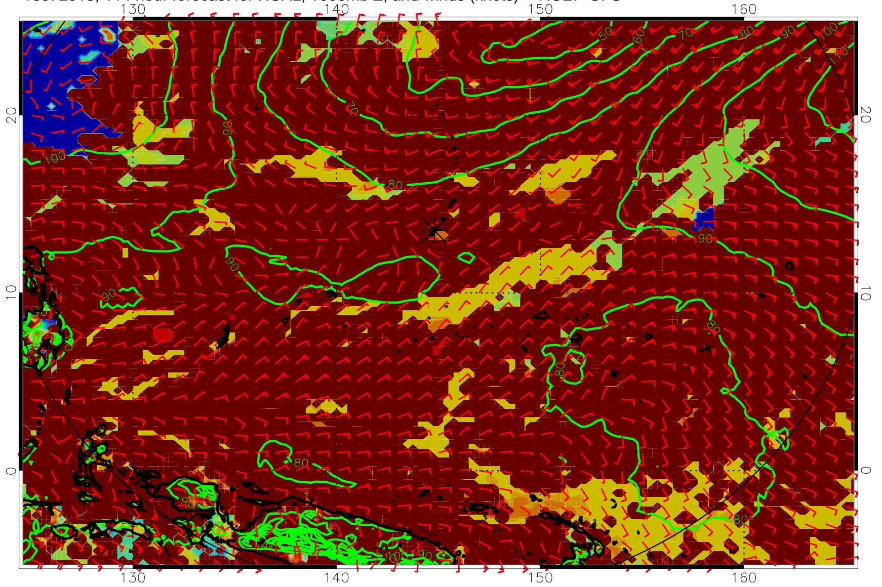
16072018, 114 hour forecast for HCAL, 1000mb Z, and winds (knots) -- NCEP GFS
