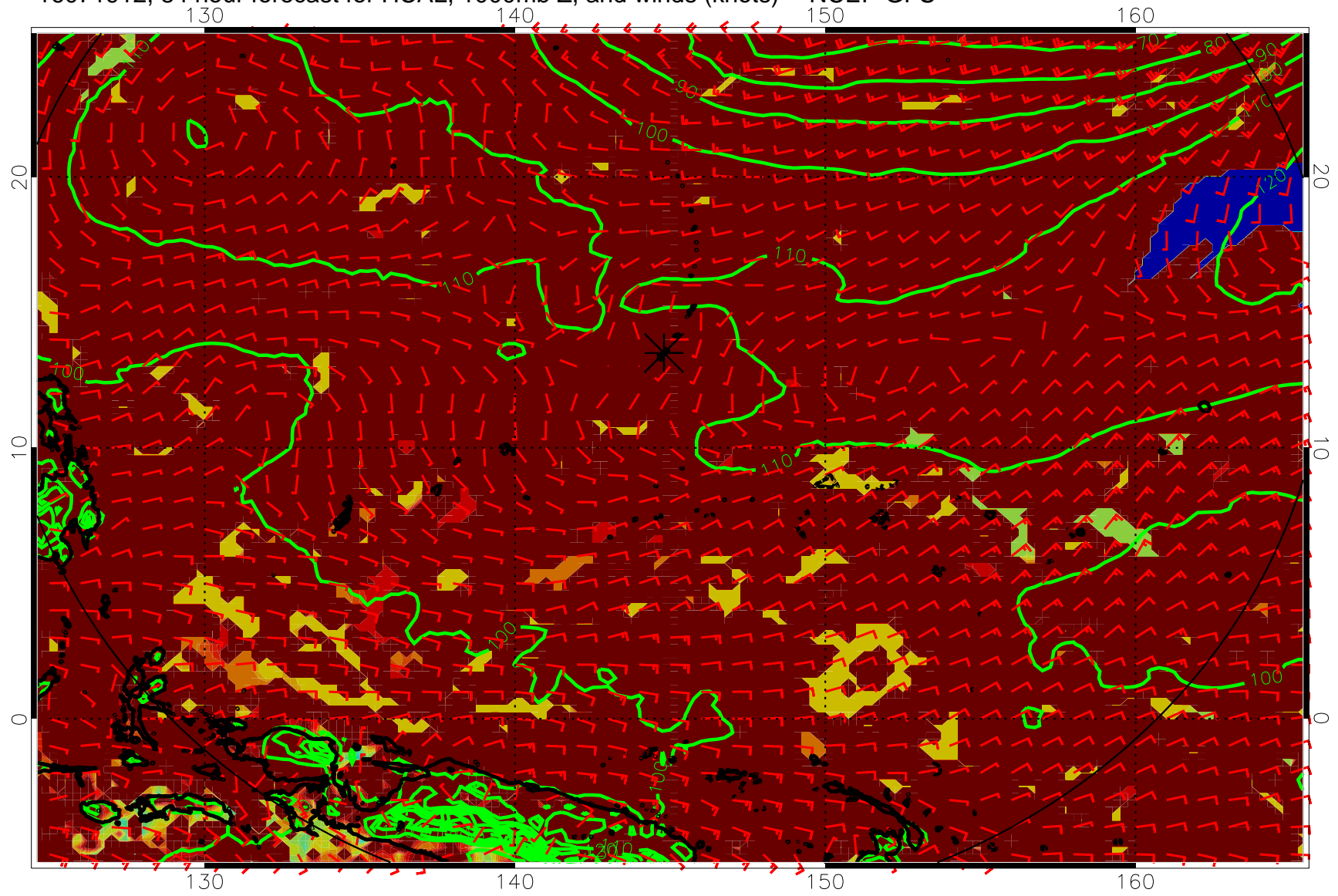
16071912, 84 hour forecast for HCAL, 1000mb Z, and winds (knots) -- NCEP GFS
