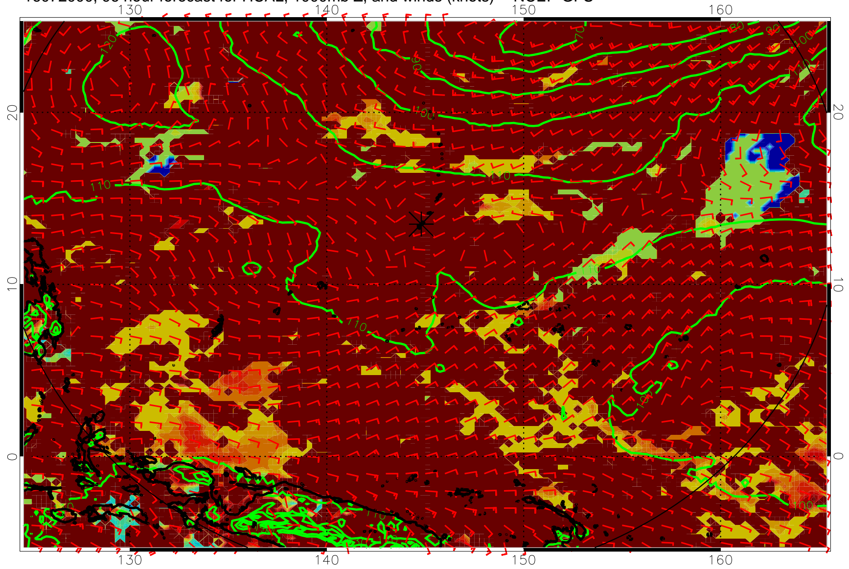
16072000, 96 hour forecast for HCAL, 1000mb Z, and winds (knots) -- NCEP GFS
