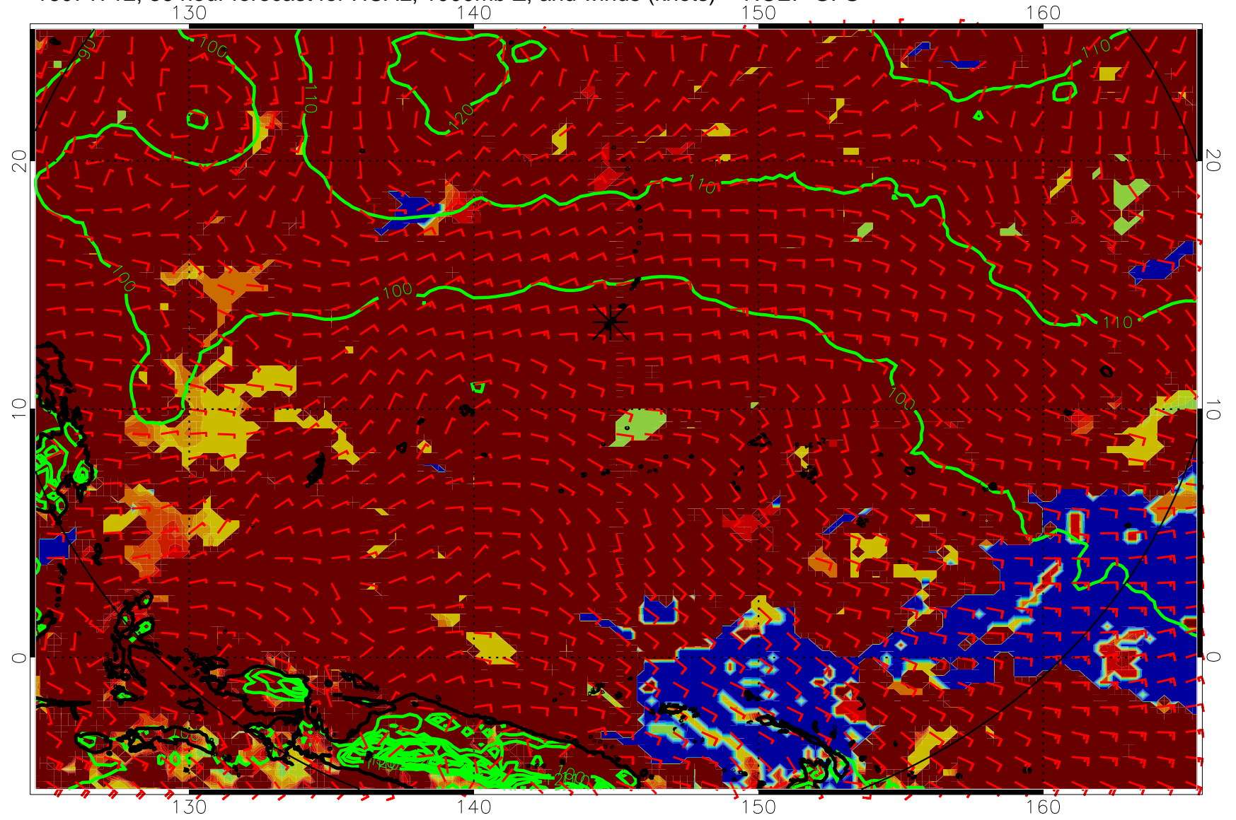
16071712, 36 hour forecast for HCAL, 1000mb Z, and winds (knots) -- NCEP GFS
