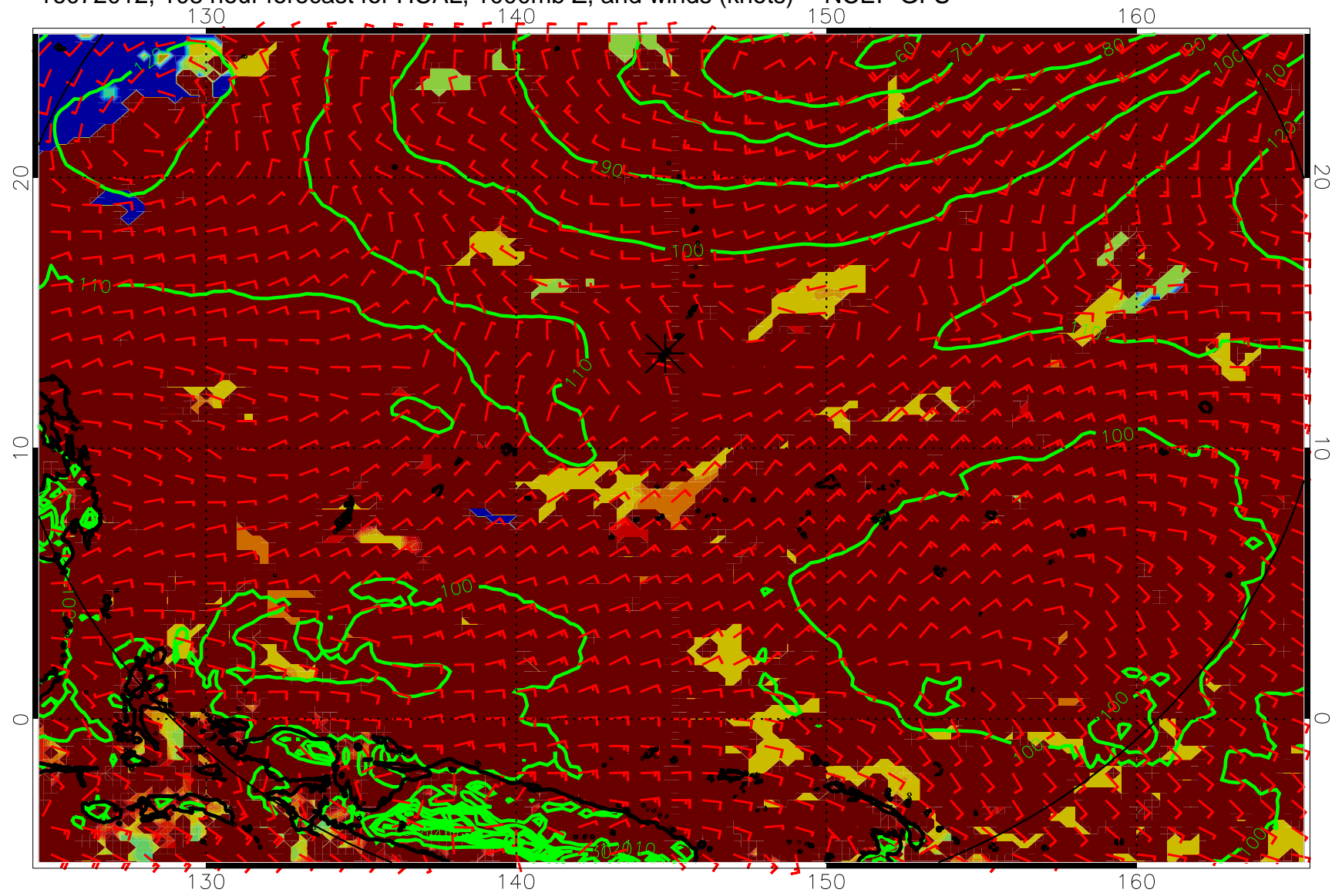
16072012, 108 hour forecast for HCAL, 1000mb Z, and winds (knots) -- NCEP GFS
