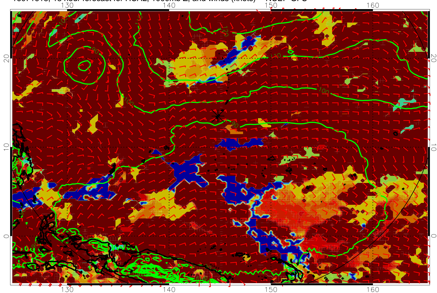
16071618, 18 hour forecast for HCAL, 1000mb Z, and winds (knots) -- NCEP GFS
