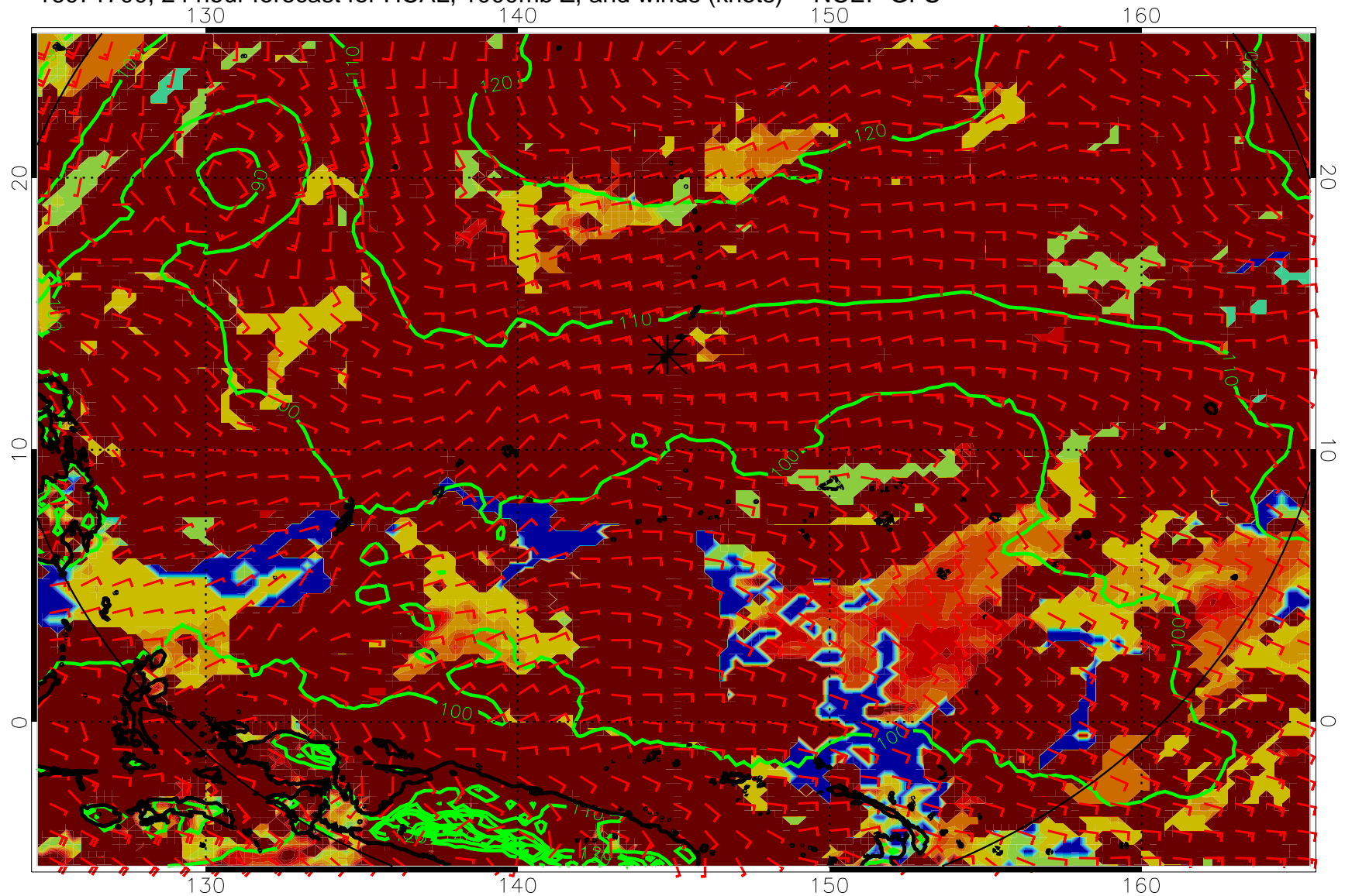
16071700, 24 hour forecast for HCAL, 1000mb Z, and winds (knots) -- NCEP GFS
