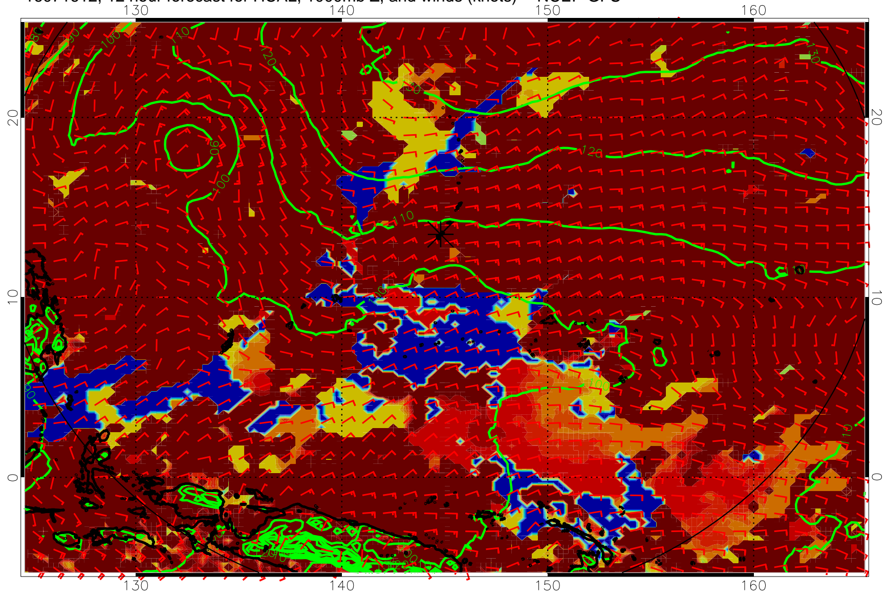
16071612, 12 hour forecast for HCAL, 1000mb Z, and winds (knots) -- NCEP GFS
