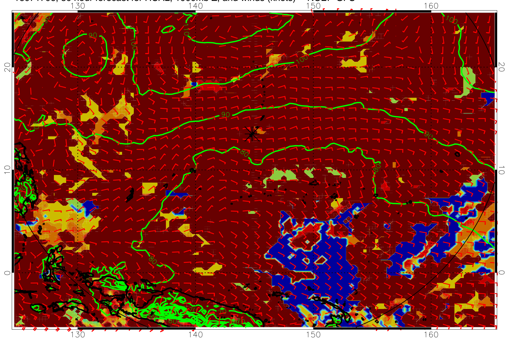
16071706, 30 hour forecast for HCAL, 1000mb Z, and winds (knots) -- NCEP GFS
