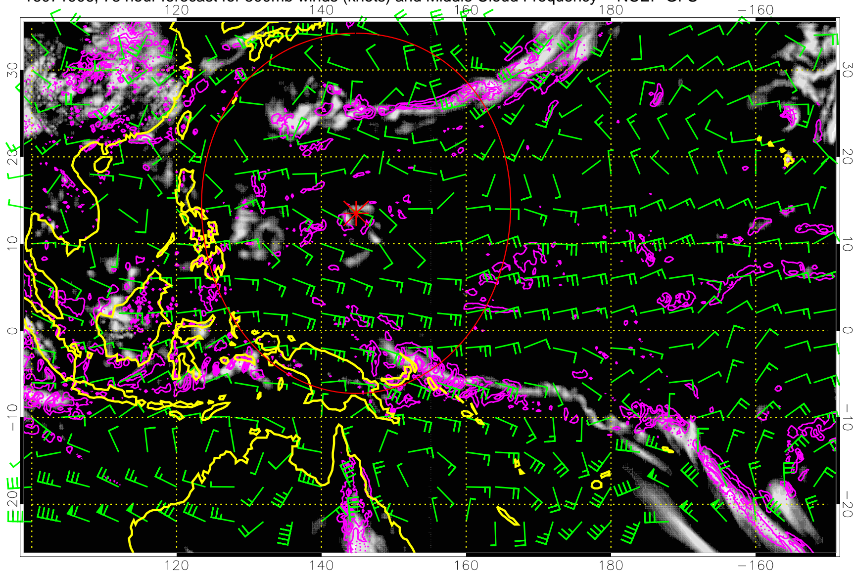
16071906, 78 hour forecast for 500mb winds (knots) and Middle Cloud Frequency -- NCEP GFS
