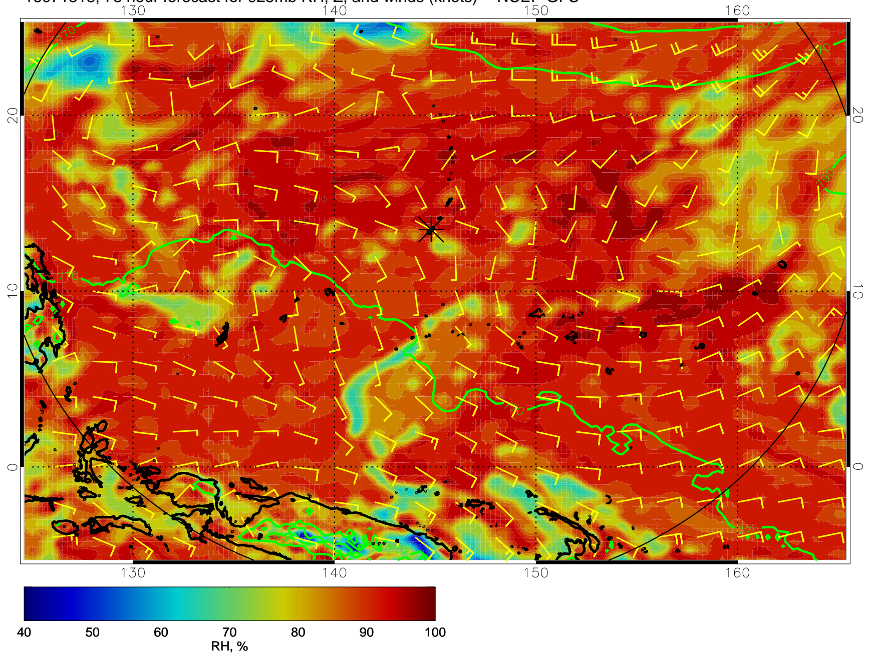
16071818, 78 hour forecast for 925mb RH, Z, and winds (knots) -- NCEP GFS
