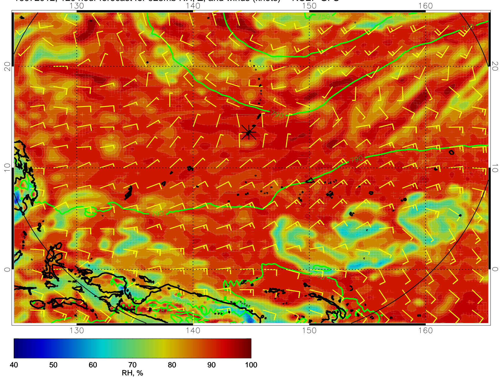
16072012, 120 hour forecast for 925mb RH, Z, and winds (knots) -- NCEP GFS
