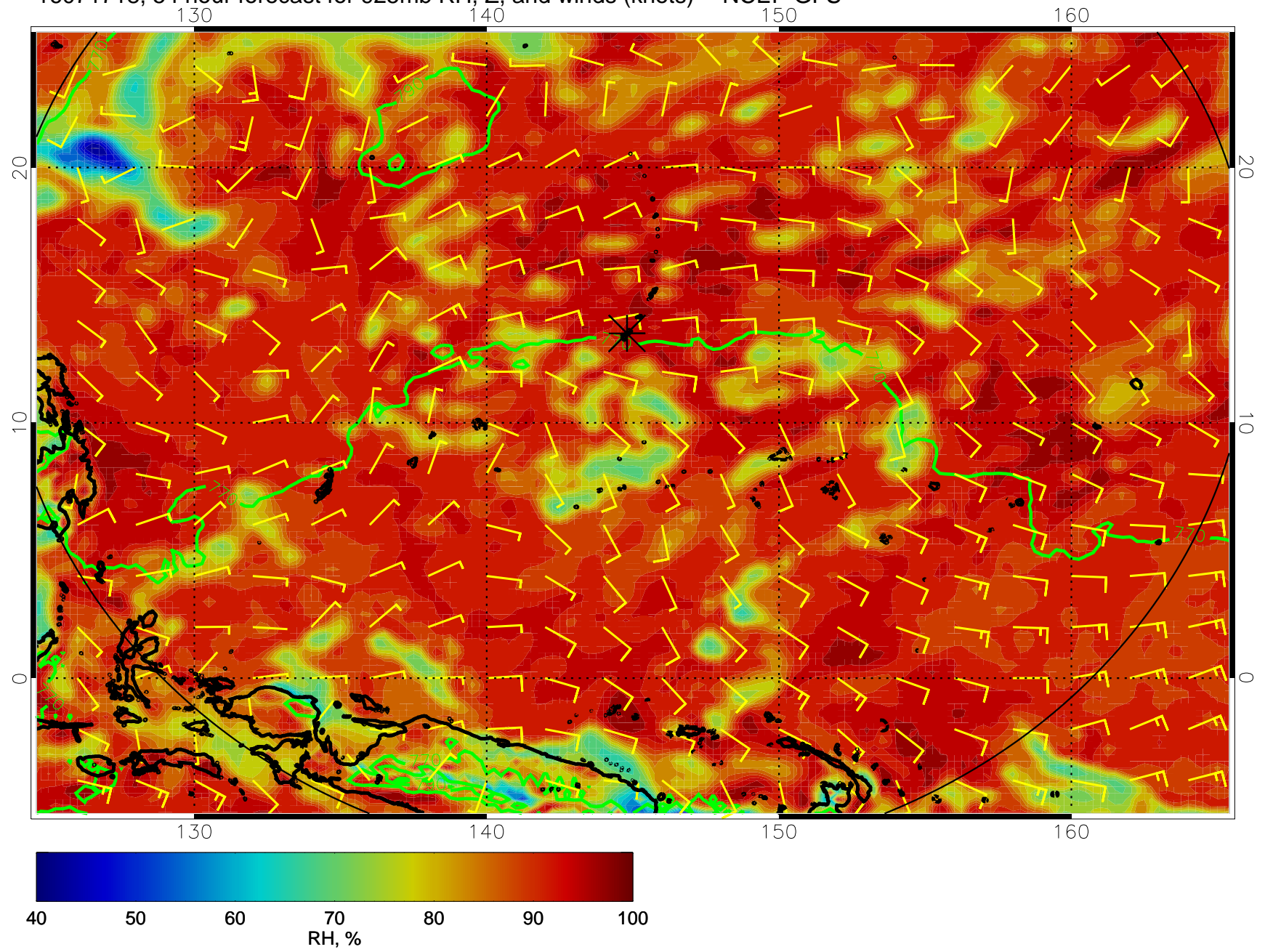
16071718, 54 hour forecast for 925mb RH, Z, and winds (knots) -- NCEP GFS
