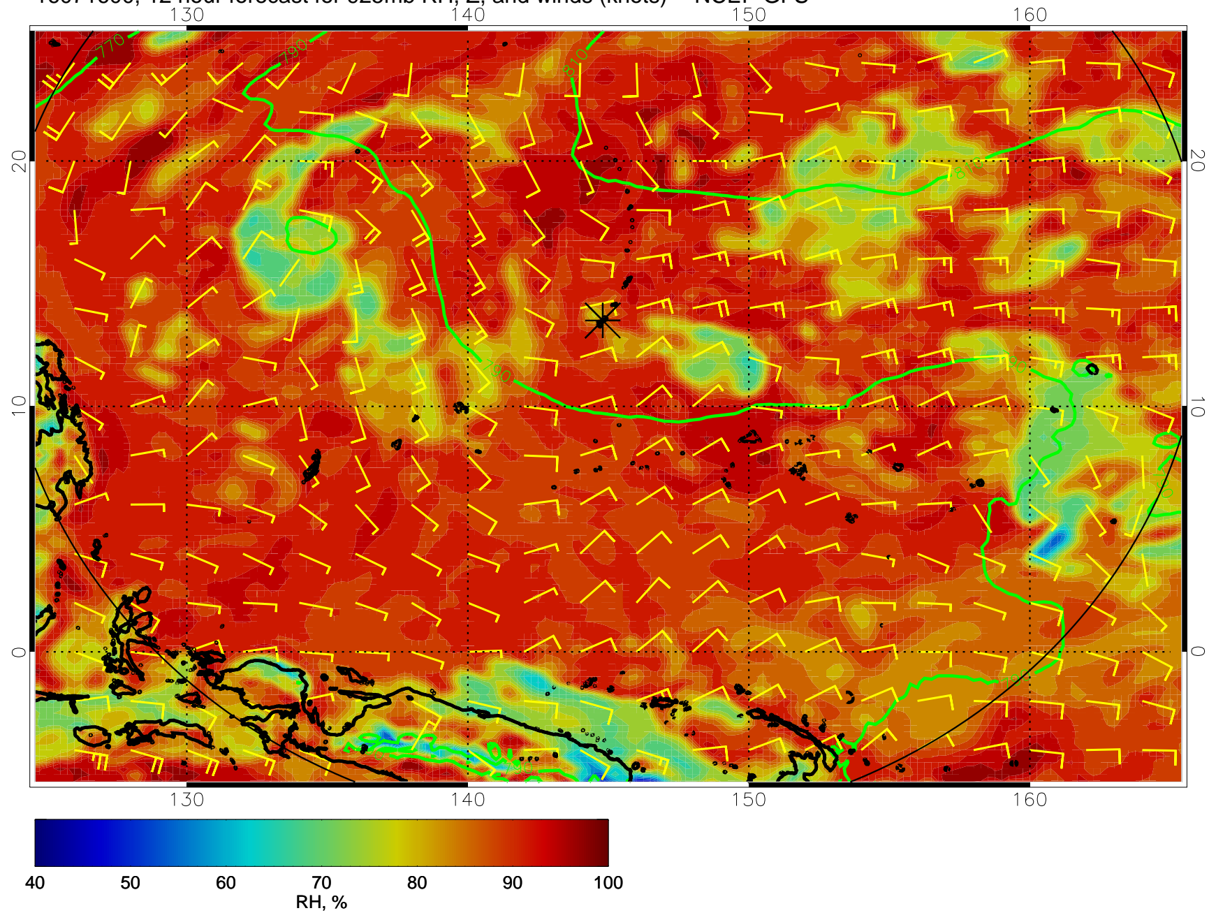
16071600, 12 hour forecast for 925mb RH, Z, and winds (knots) -- NCEP GFS
