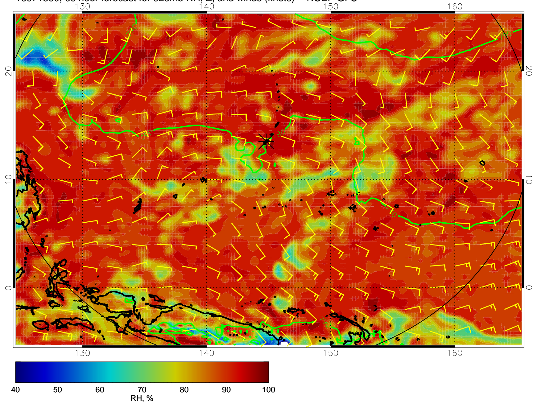
16071800, 60 hour forecast for 925mb RH, Z, and winds (knots) -- NCEP GFS
