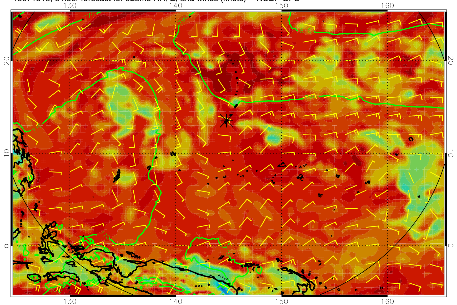
16071518, 6 hour forecast for 925mb RH, Z, and winds (knots) -- NCEP GFS
