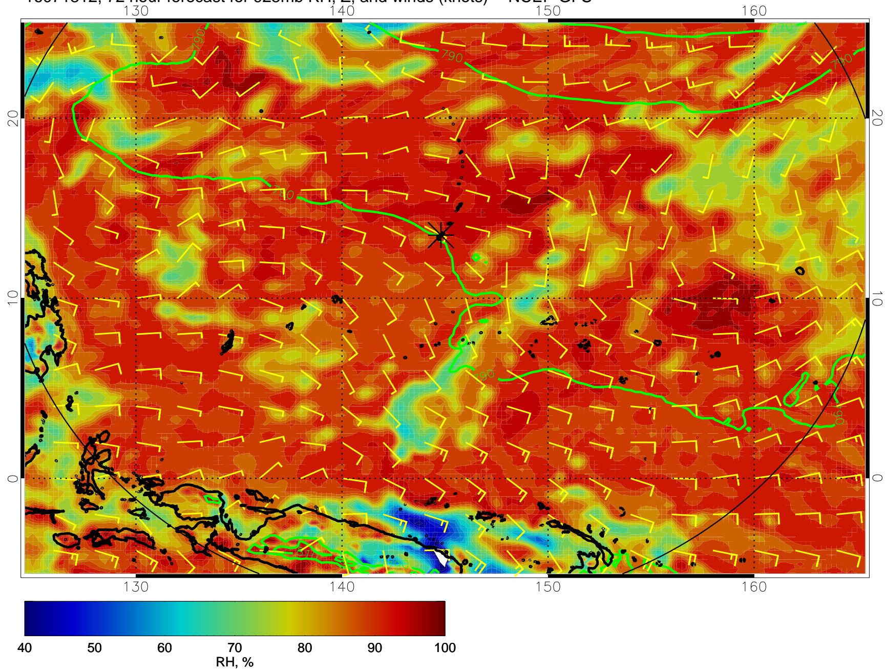
16071812, 72 hour forecast for 925mb RH, Z, and winds (knots) -- NCEP GFS
