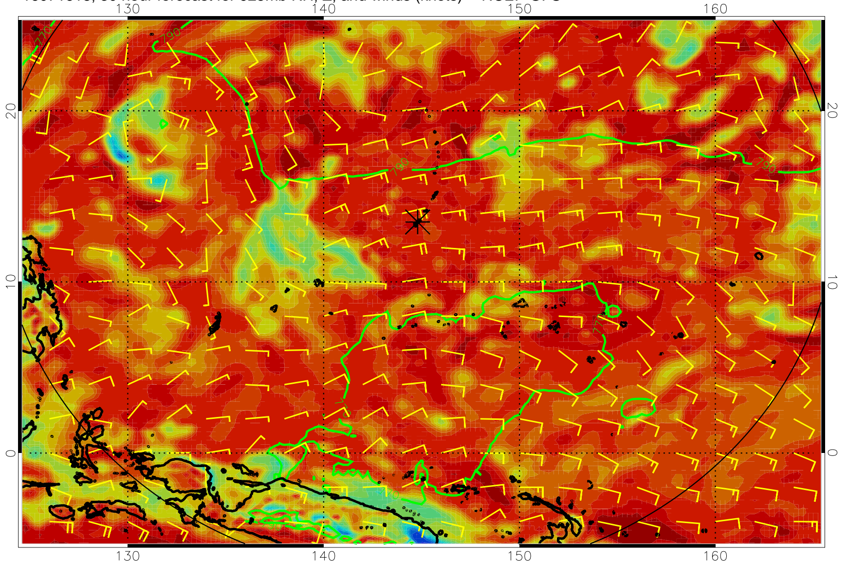
16071618, 30 hour forecast for 925mb RH, Z, and winds (knots) -- NCEP GFS
