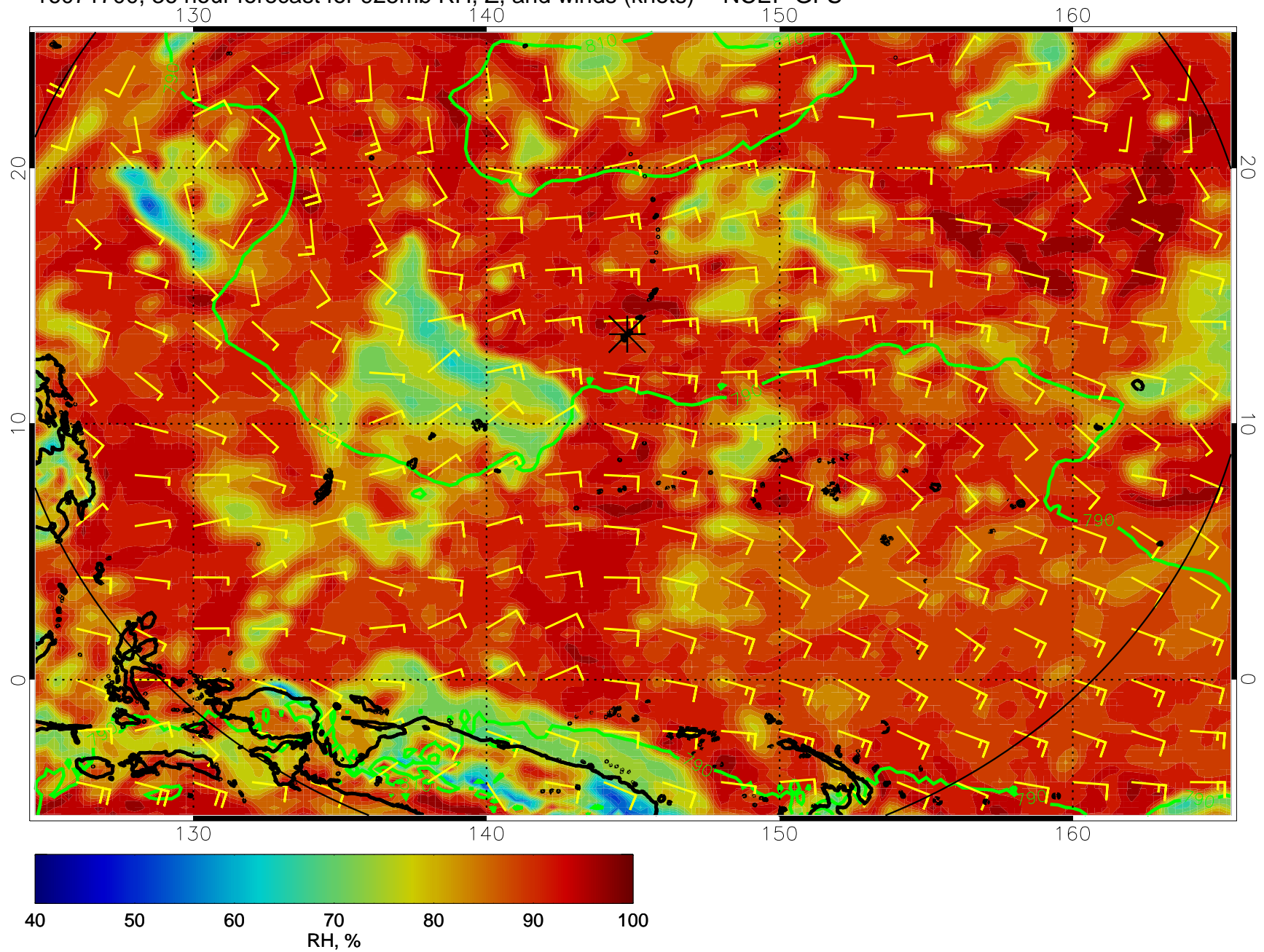
16071700, 36 hour forecast for 925mb RH, Z, and winds (knots) -- NCEP GFS
