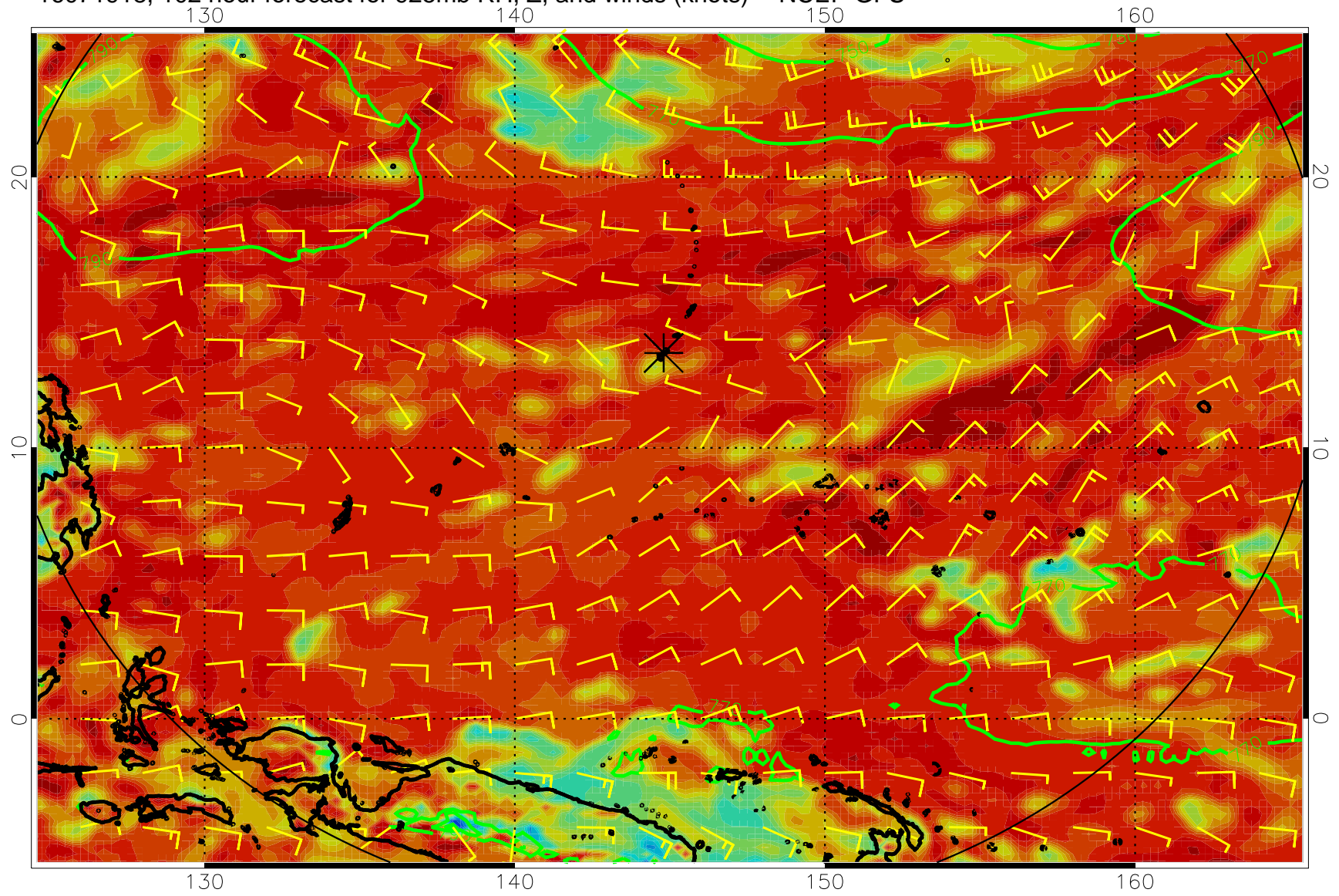
16071918, 102 hour forecast for 925mb RH, Z, and winds (knots) -- NCEP GFS
