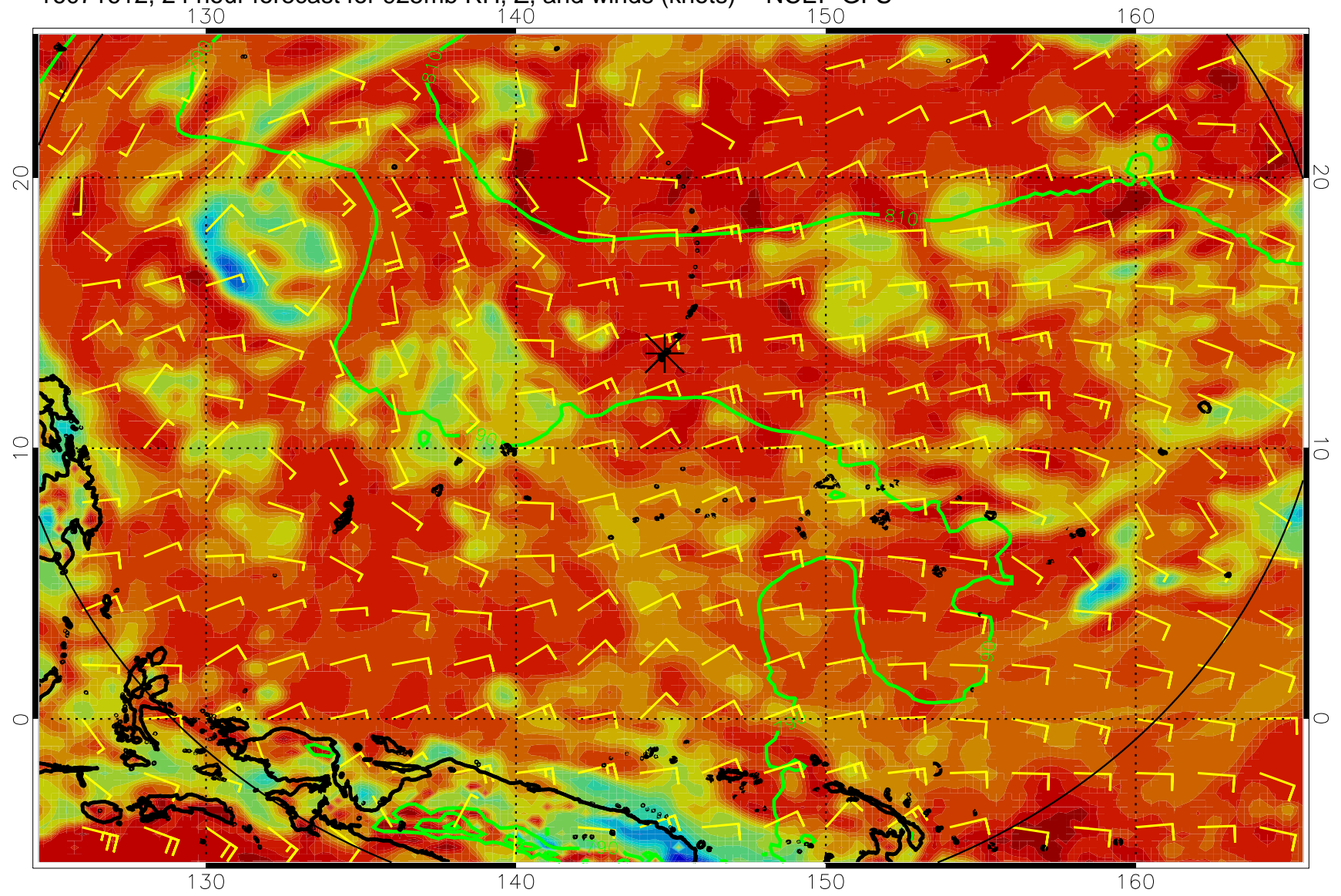
16071612, 24 hour forecast for 925mb RH, Z, and winds (knots) -- NCEP GFS
