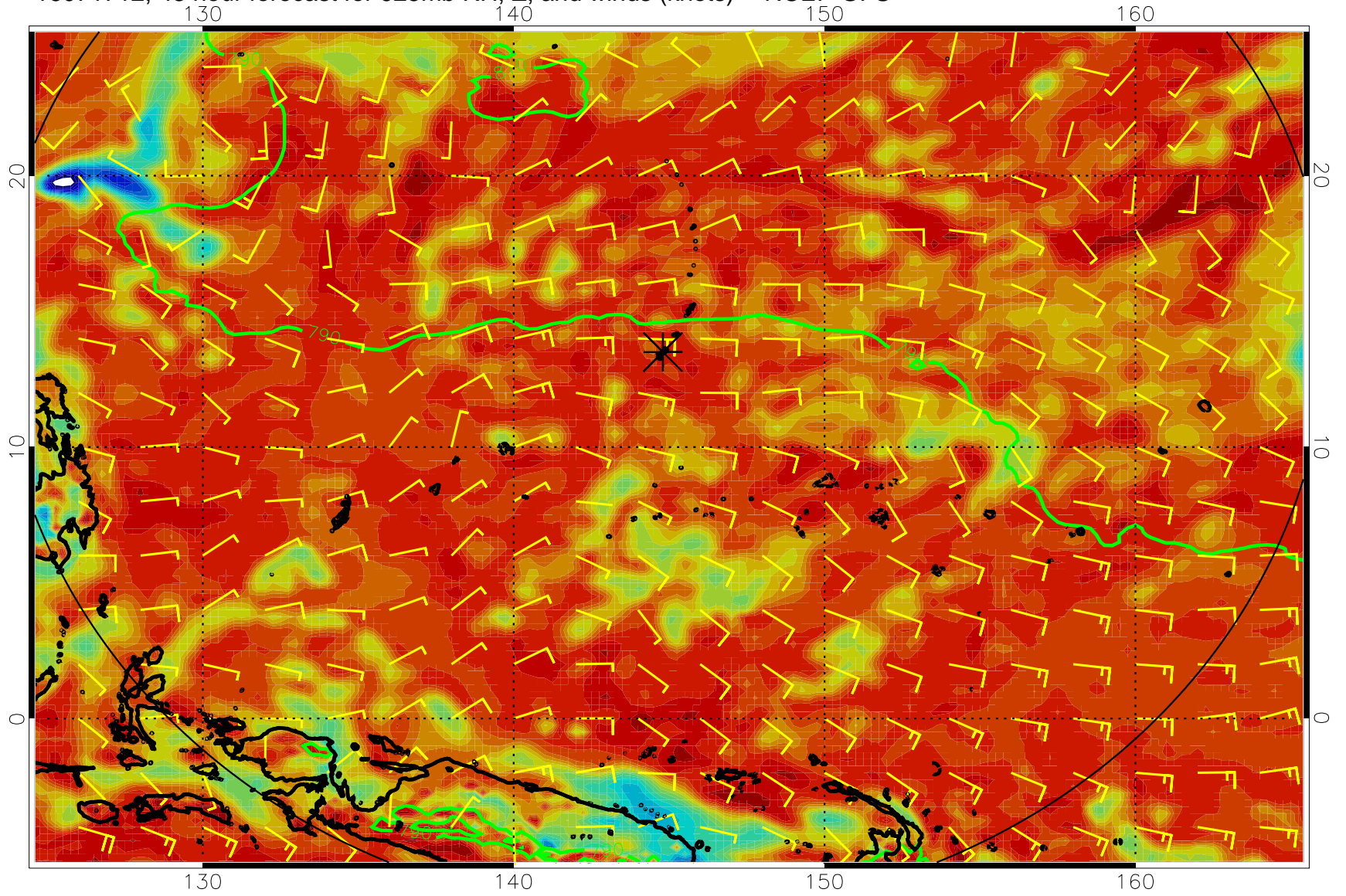
16071712, 48 hour forecast for 925mb RH, Z, and winds (knots) -- NCEP GFS
