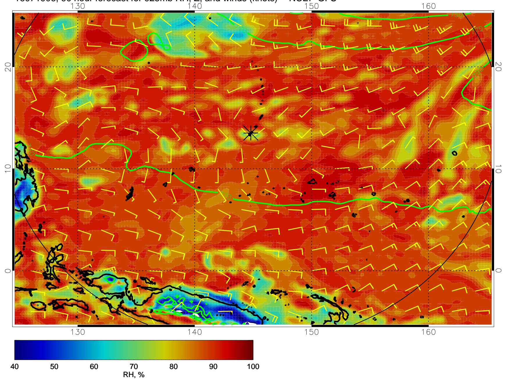
16071906, 90 hour forecast for 925mb RH, Z, and winds (knots) -- NCEP GFS
