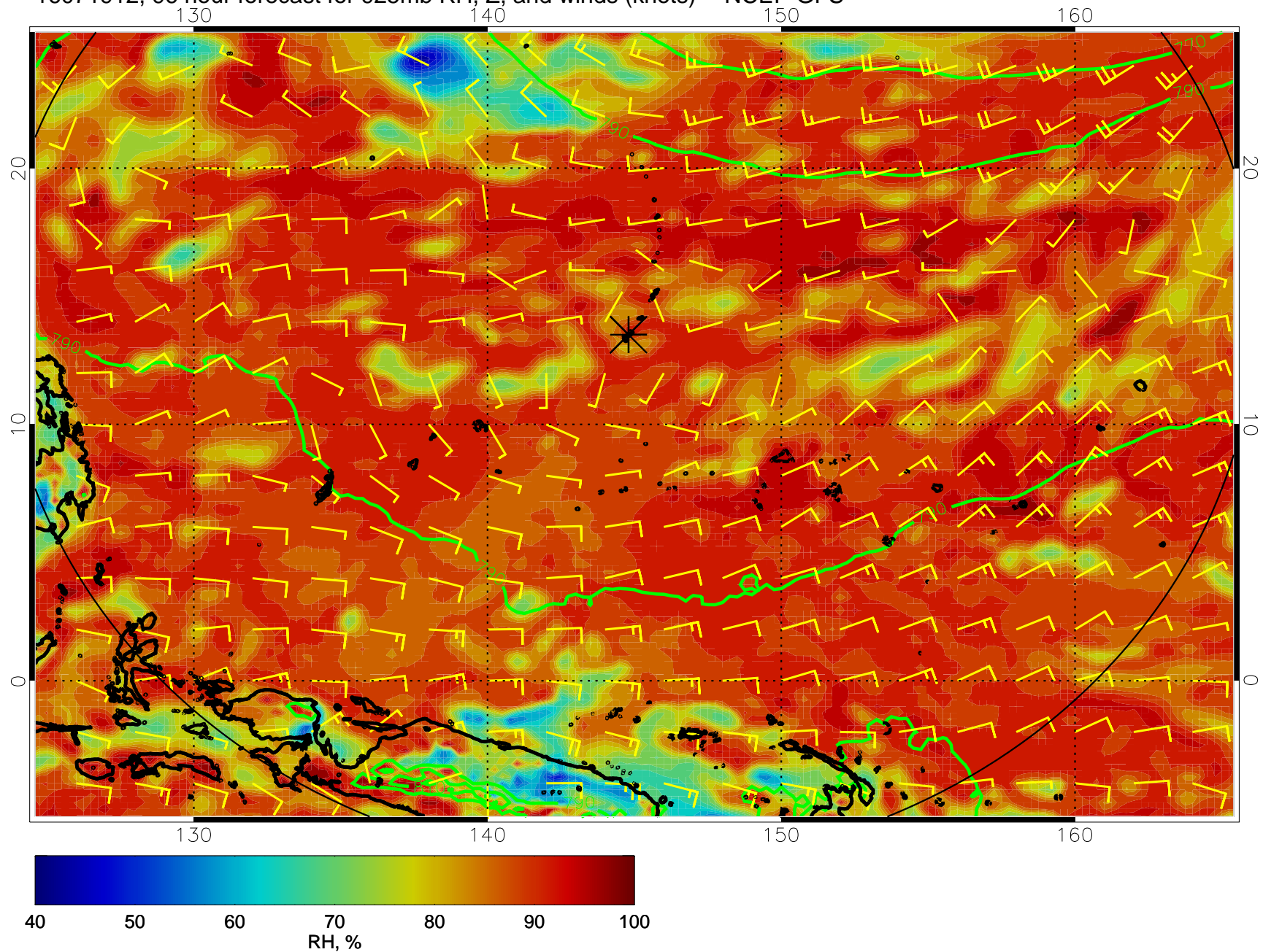
16071912, 96 hour forecast for 925mb RH, Z, and winds (knots) -- NCEP GFS
