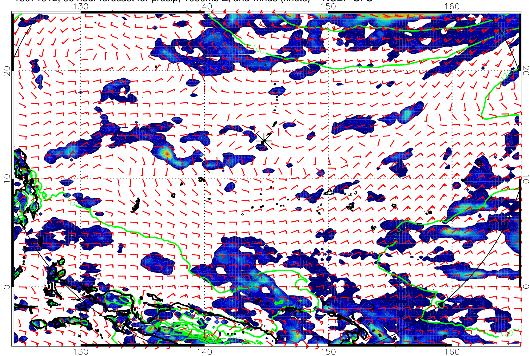
16071912, 96 hour forecast for precip, 1000mb Z, and winds (knots) -- NCEP GFS
