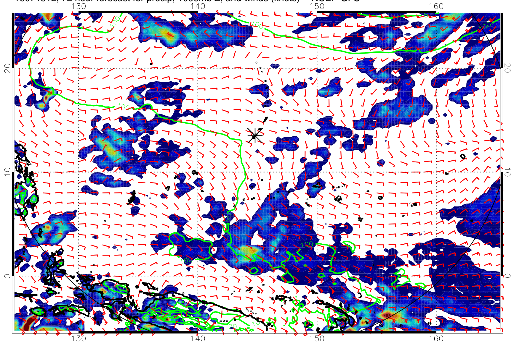
16071812, 72 hour forecast for precip, 1000mb Z, and winds (knots) -- NCEP GFS
