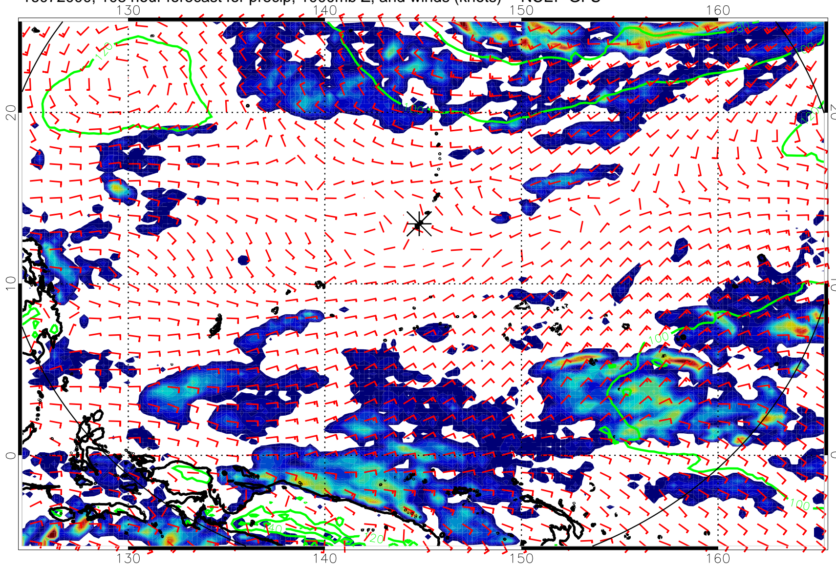
16072000, 108 hour forecast for precip, 1000mb Z, and winds (knots) -- NCEP GFS
