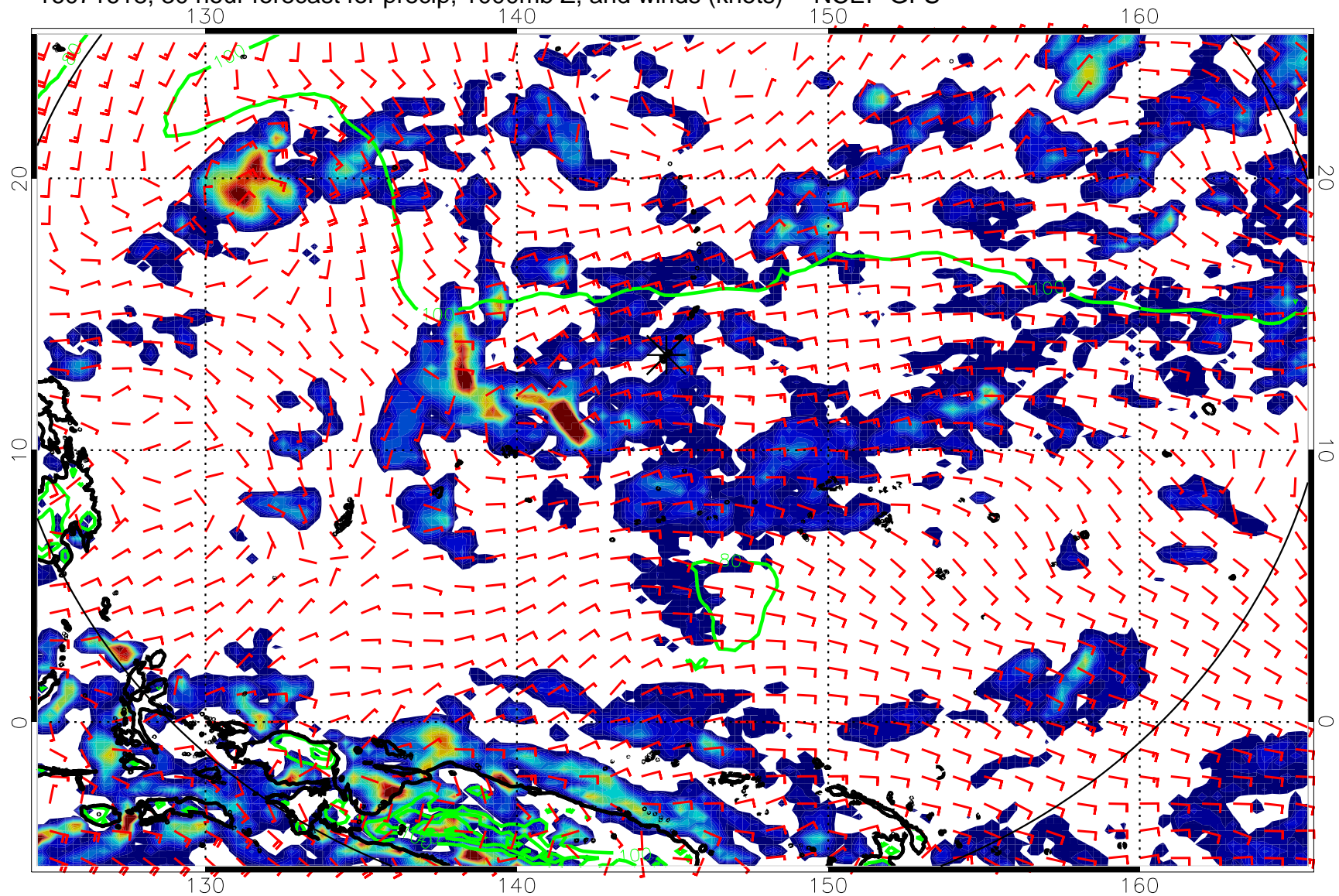
16071618, 30 hour forecast for precip, 1000mb Z, and winds (knots) -- NCEP GFS
