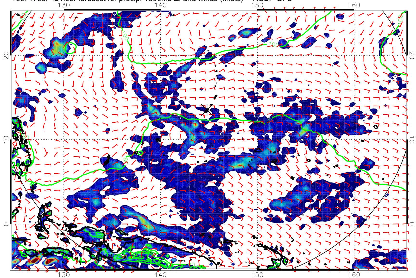
16071706, 42 hour forecast for precip, 1000mb Z, and winds (knots) -- NCEP GFS
