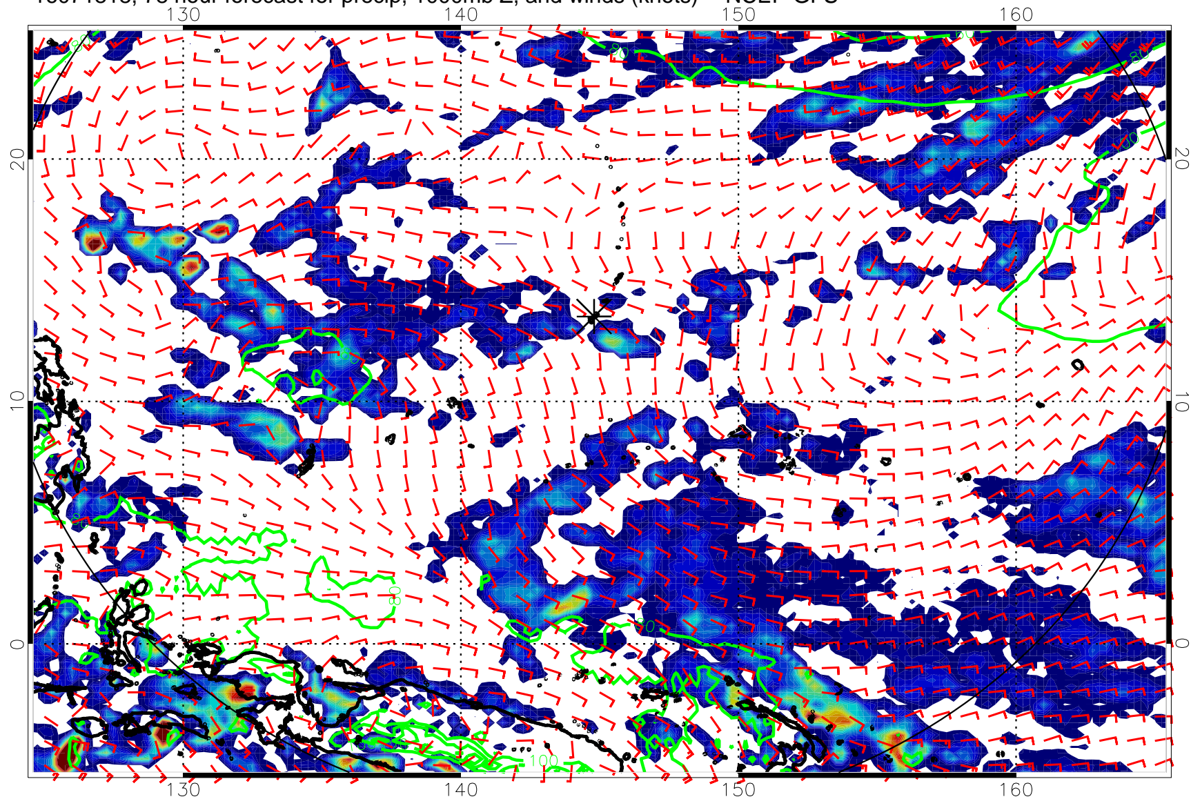
16071818, 78 hour forecast for precip, 1000mb Z, and winds (knots) -- NCEP GFS
