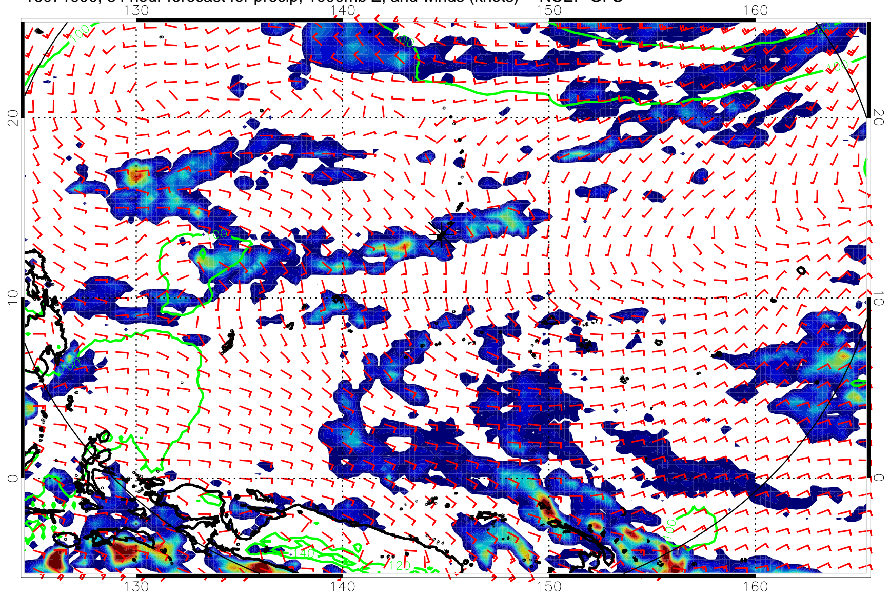
16071900, 84 hour forecast for precip, 1000mb Z, and winds (knots) -- NCEP GFS
