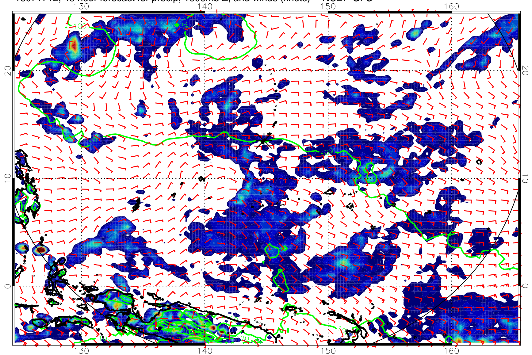
16071712, 48 hour forecast for precip, 1000mb Z, and winds (knots) -- NCEP GFS
