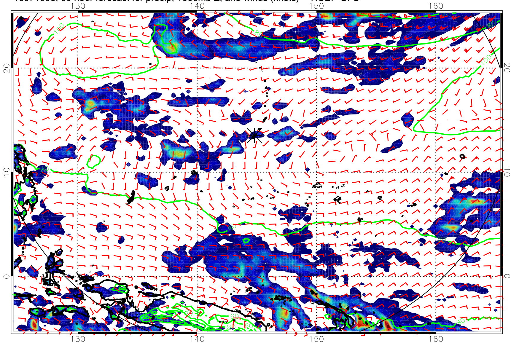
16071906, 90 hour forecast for precip, 1000mb Z, and winds (knots) -- NCEP GFS
