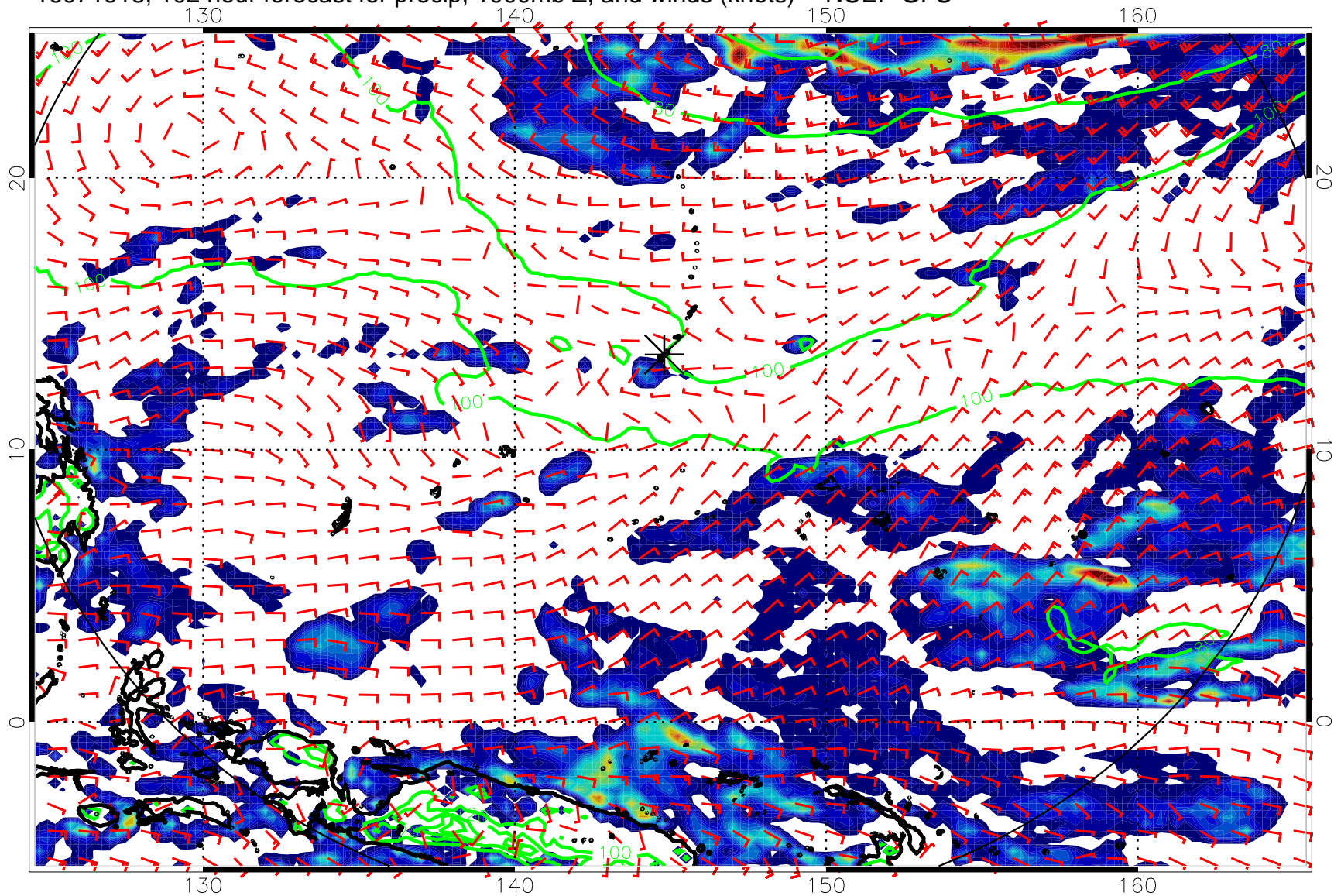
16071918, 102 hour forecast for precip, 1000mb Z, and winds (knots) -- NCEP GFS
