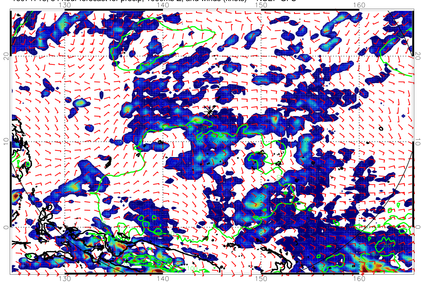
16071718, 54 hour forecast for precip, 1000mb Z, and winds (knots) -- NCEP GFS
