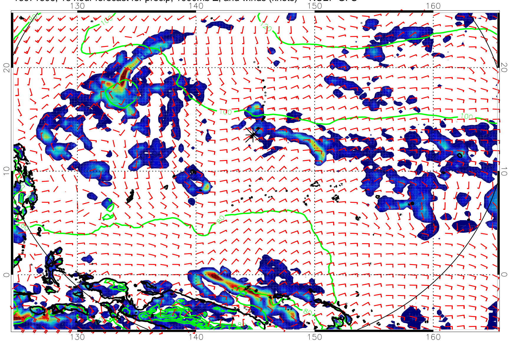
16071606, 18 hour forecast for precip, 1000mb Z, and winds (knots) -- NCEP GFS
