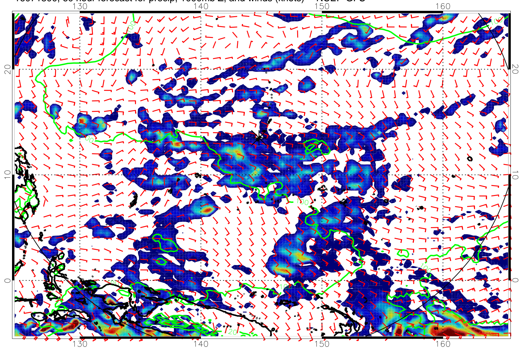
16071800, 60 hour forecast for precip, 1000mb Z, and winds (knots) -- NCEP GFS
