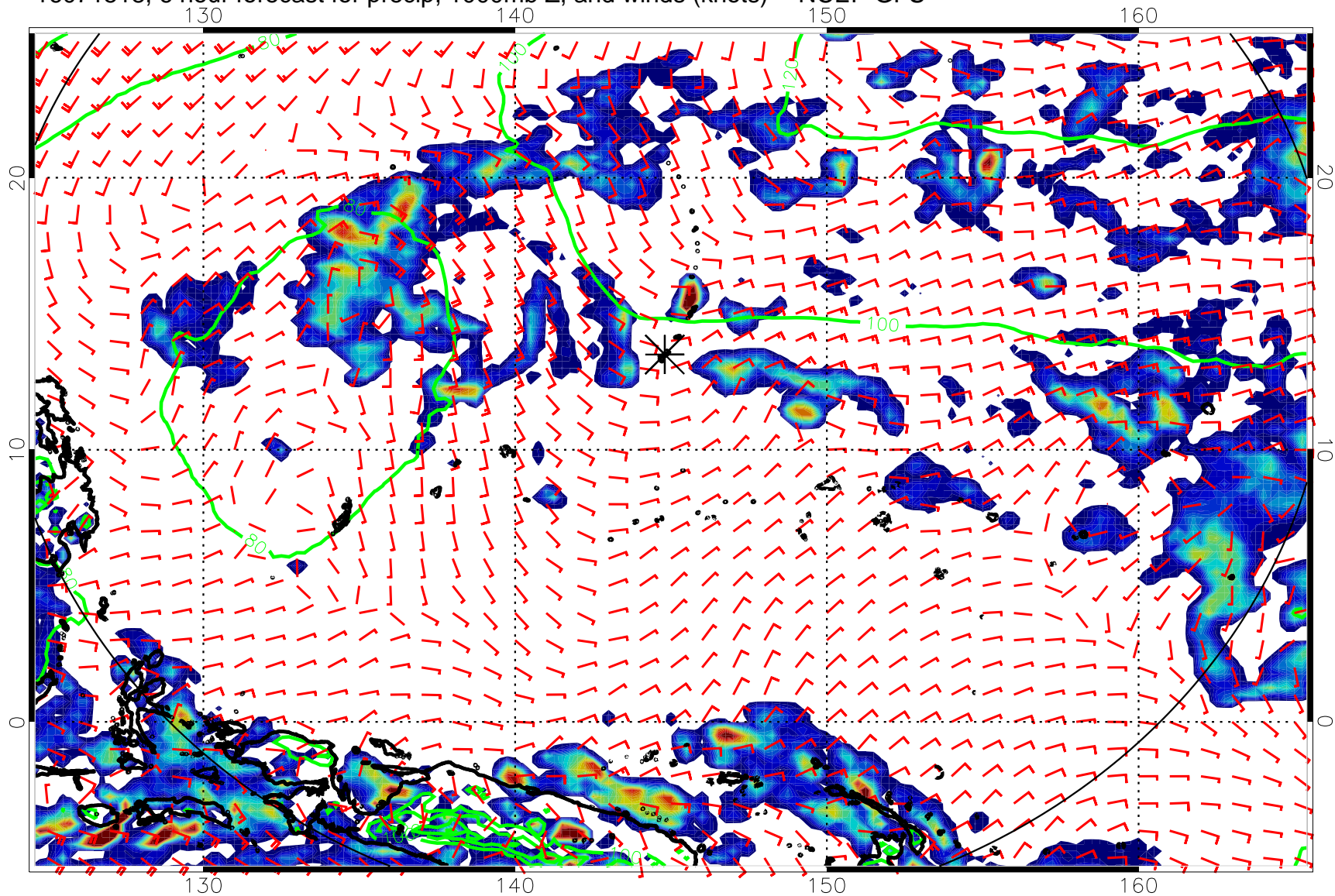
16071518, 6 hour forecast for precip, 1000mb Z, and winds (knots) -- NCEP GFS
