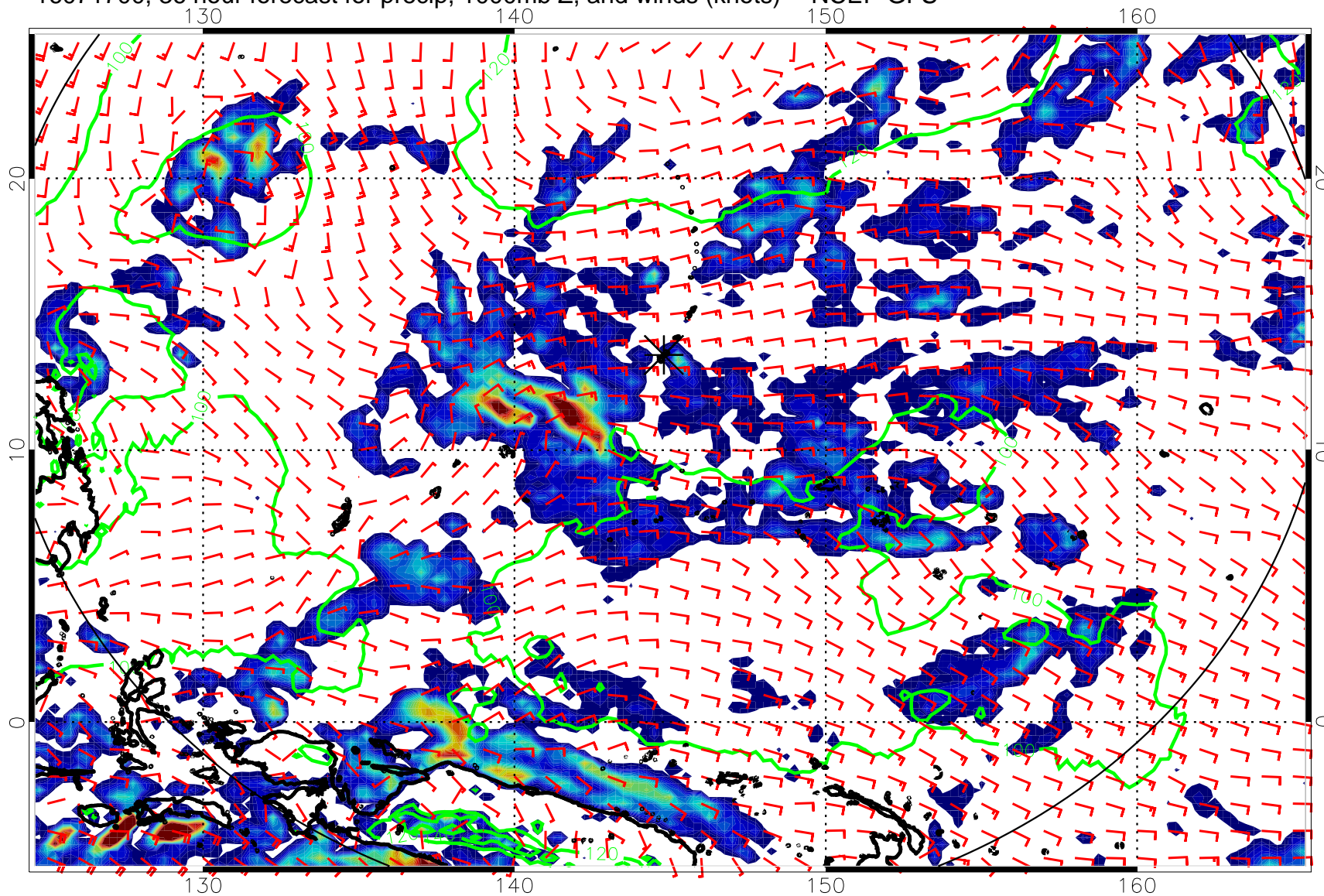
16071700, 36 hour forecast for precip, 1000mb Z, and winds (knots) -- NCEP GFS
