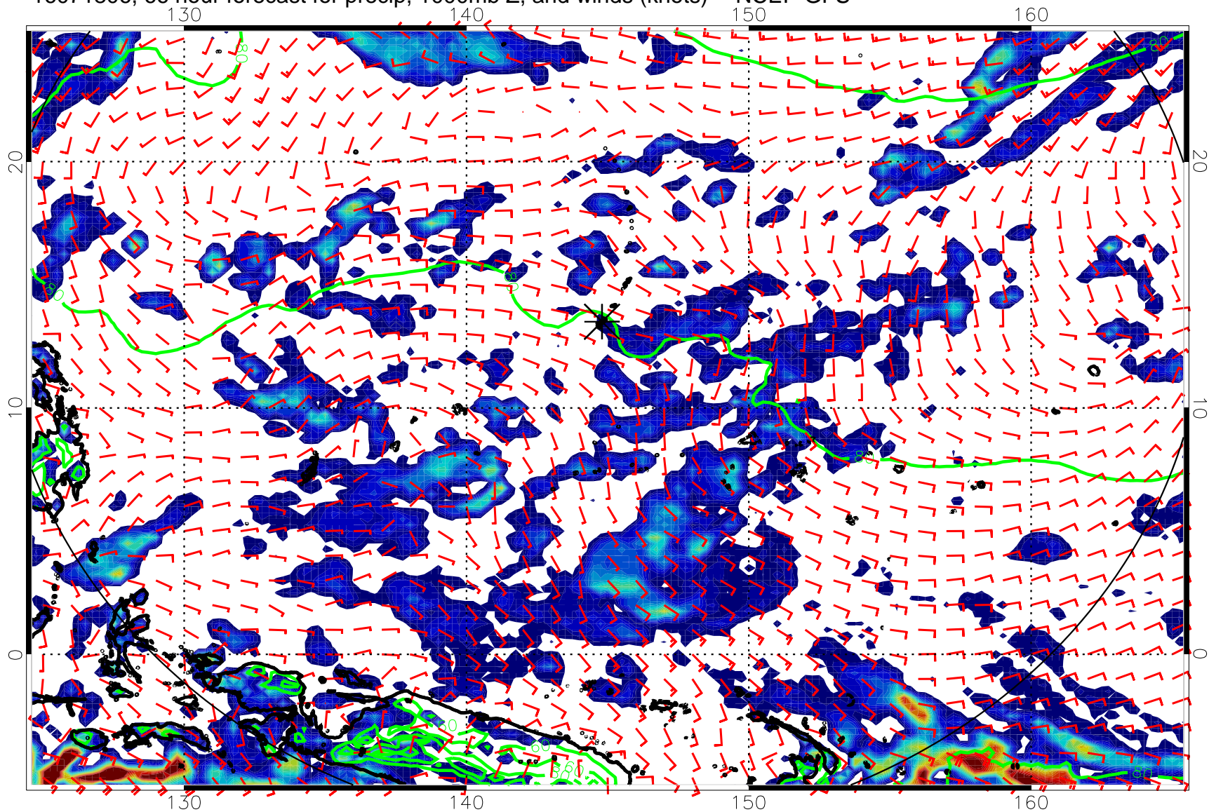
16071806, 66 hour forecast for precip, 1000mb Z, and winds (knots) -- NCEP GFS
