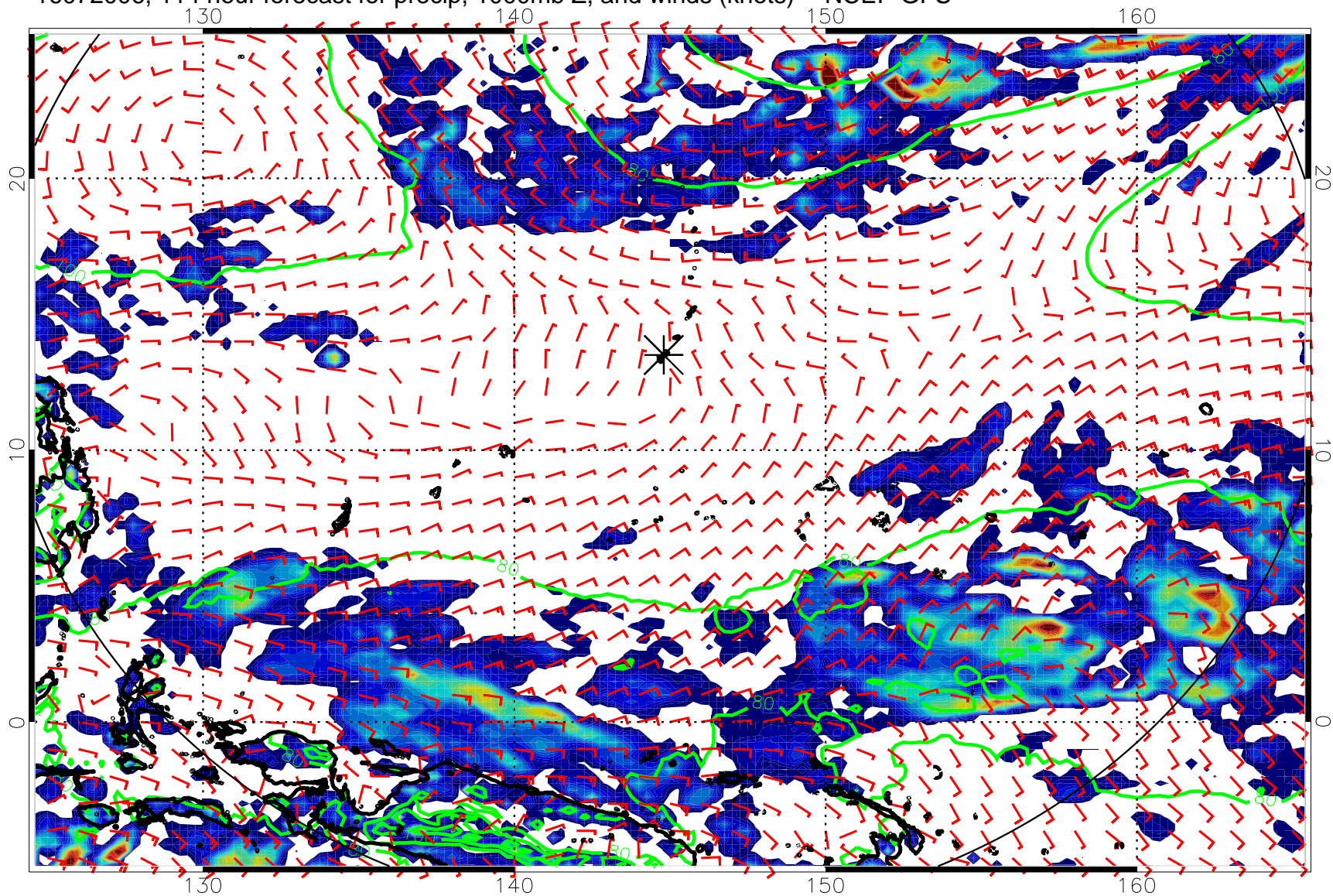
16072006, 114 hour forecast for precip, 1000mb Z, and winds (knots) -- NCEP GFS
