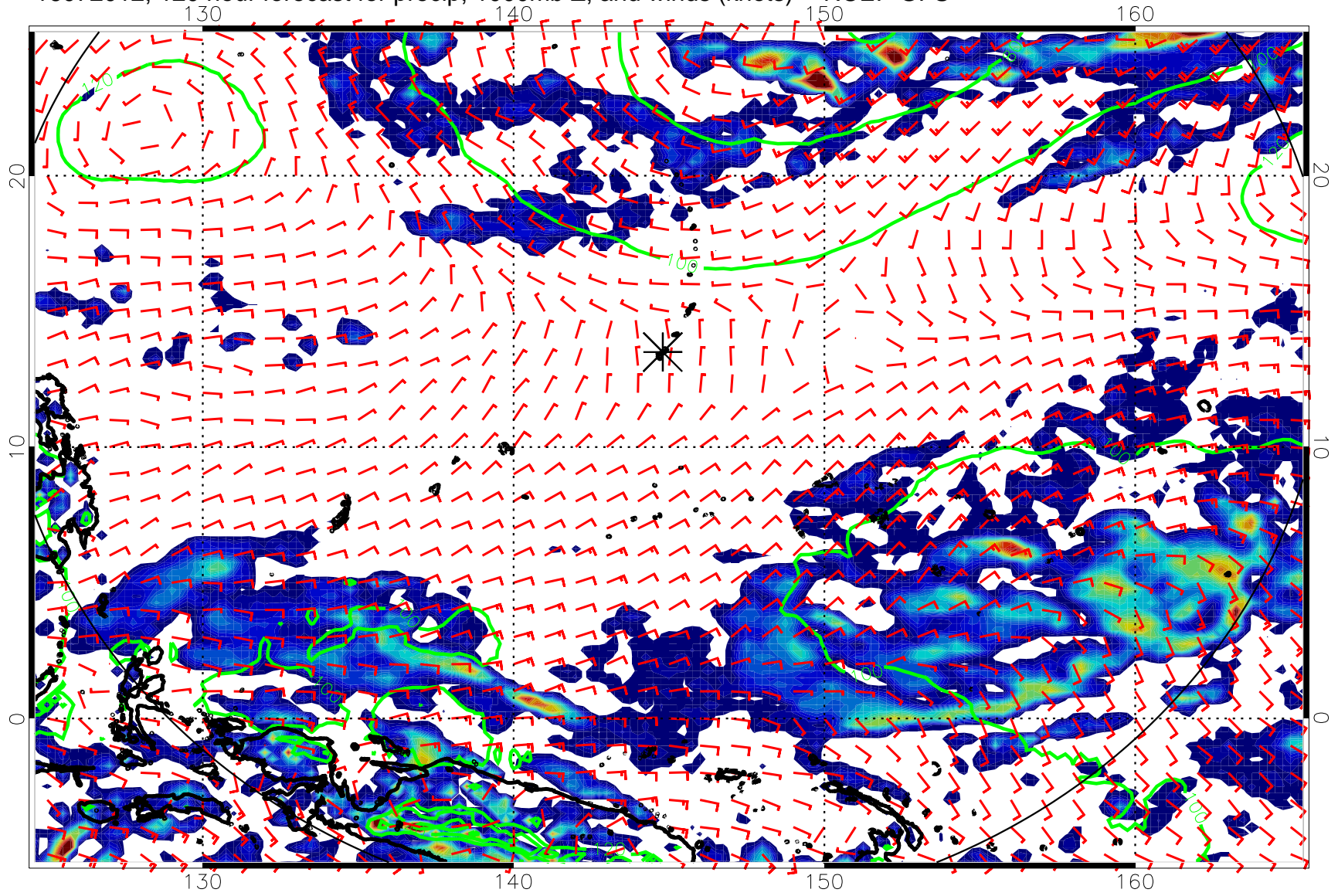
16072012, 120 hour forecast for precip, 1000mb Z, and winds (knots) -- NCEP GFS
