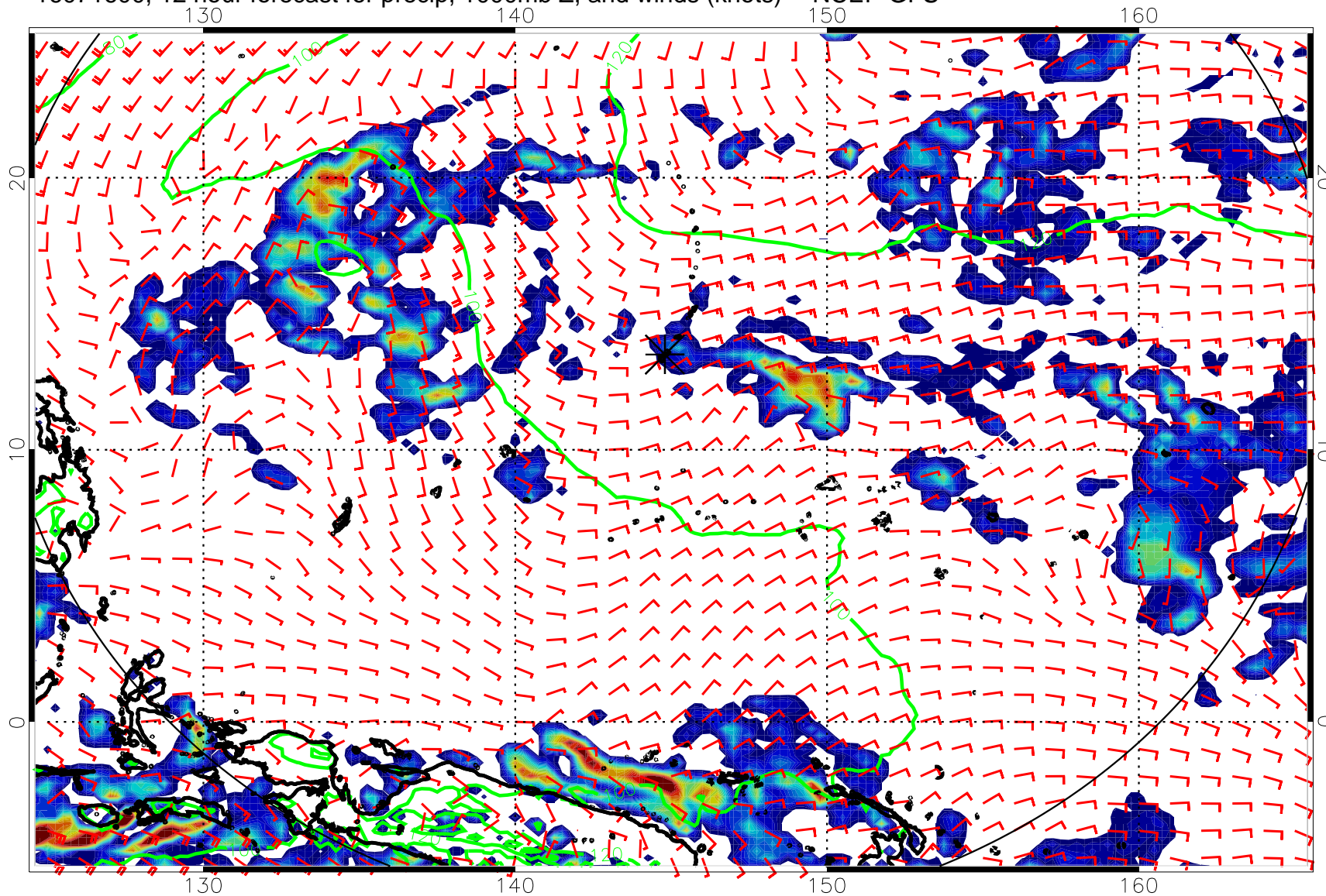
16071600, 12 hour forecast for precip, 1000mb Z, and winds (knots) -- NCEP GFS
