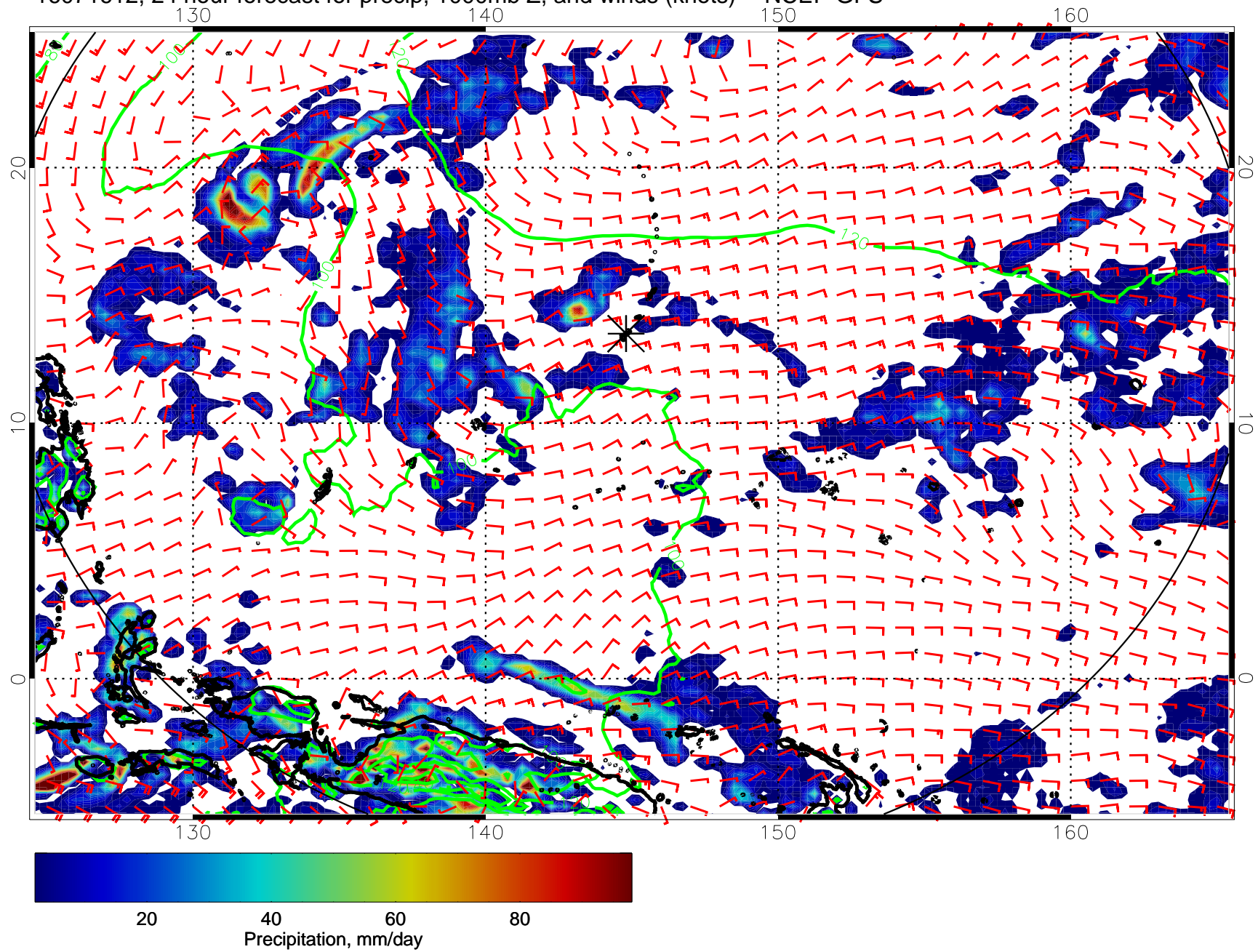
16071612, 24 hour forecast for precip, 1000mb Z, and winds (knots) -- NCEP GFS
