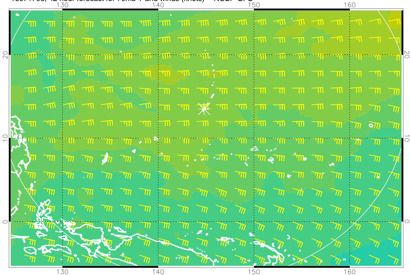
16071706, 42 hour forecast for 70mb T and winds (knots) -- NCEP GFS
