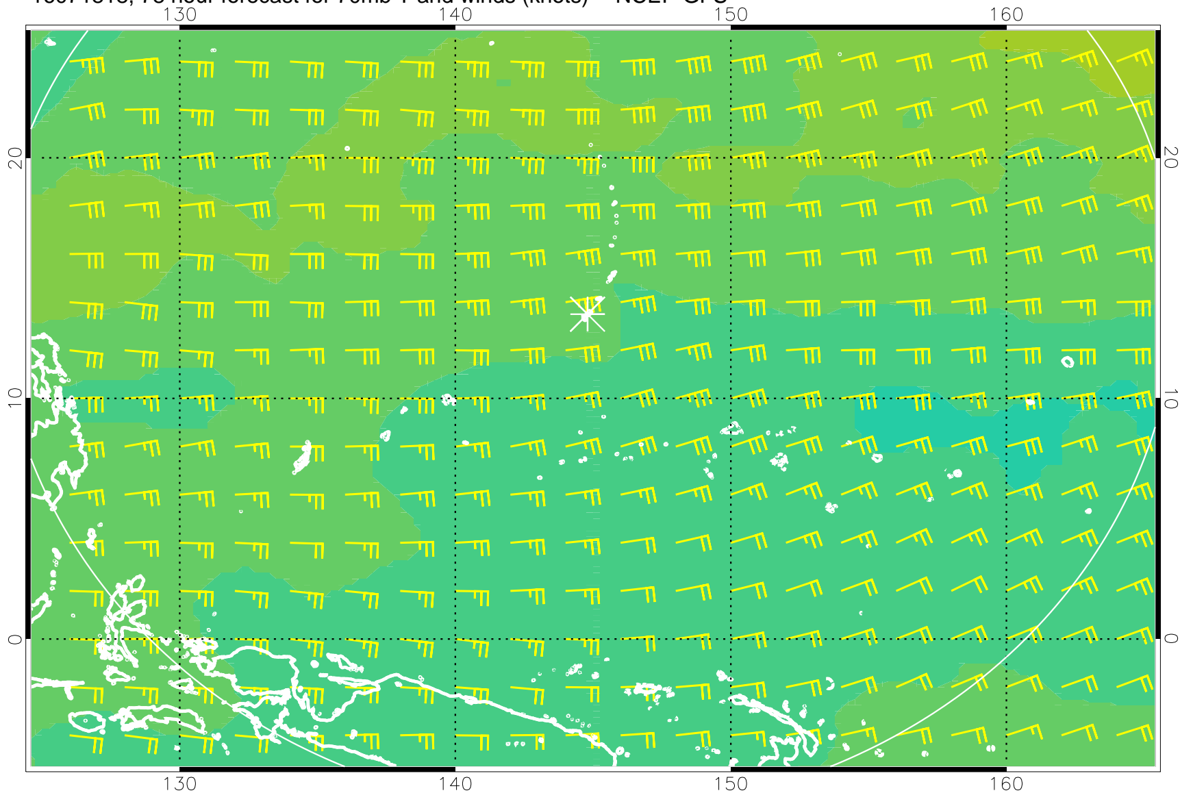
16071818, 78 hour forecast for 70mb T and winds (knots) -- NCEP GFS
