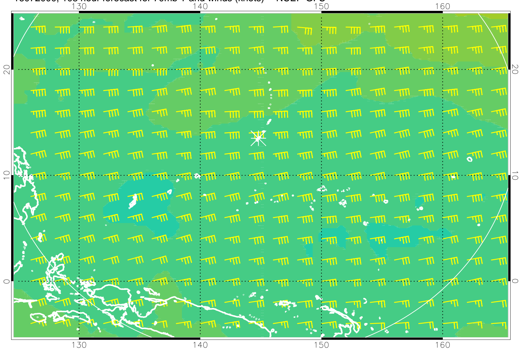
16072000, 108 hour forecast for 70mb T and winds (knots) -- NCEP GFS
