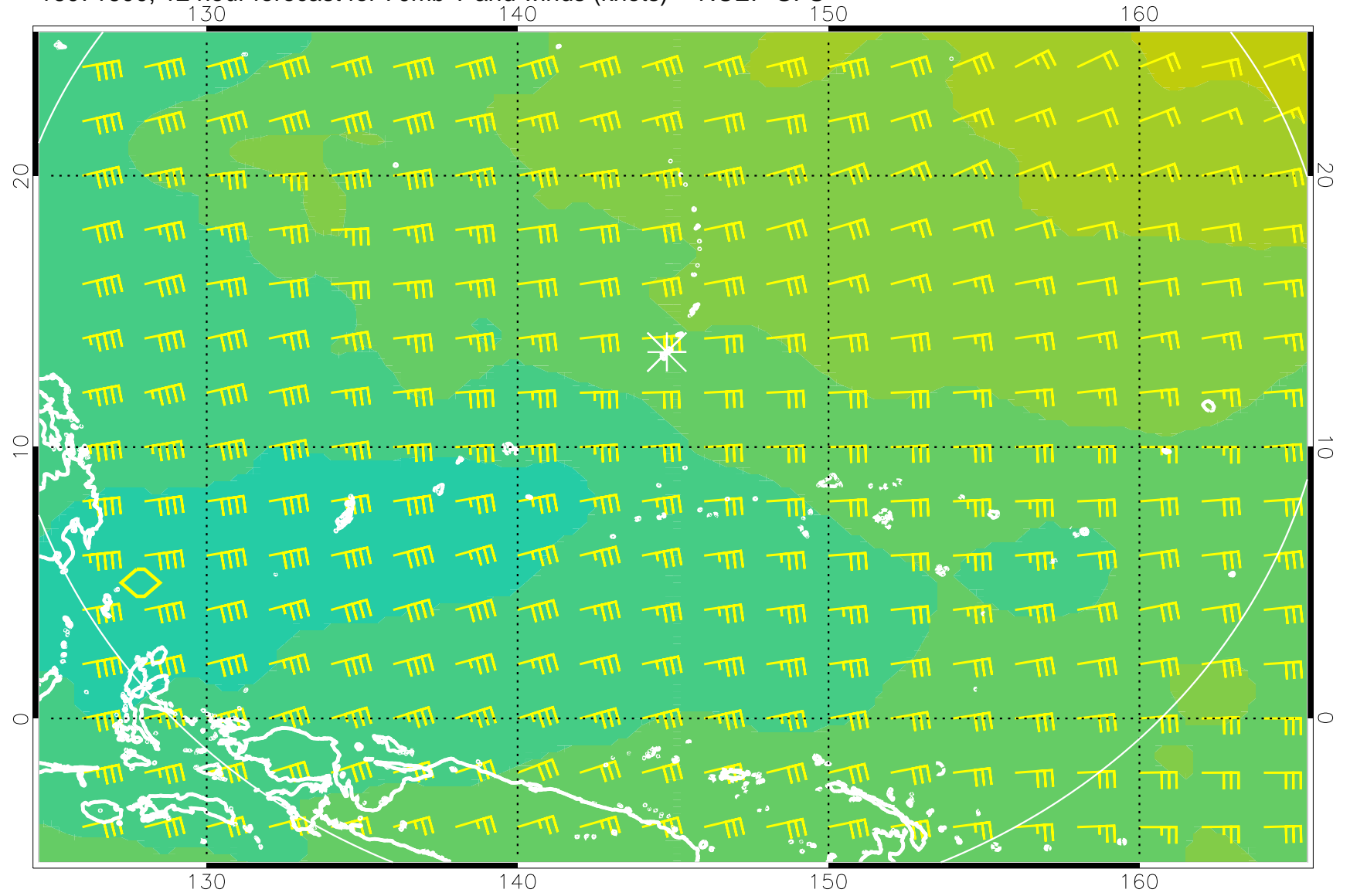
16071600, 12 hour forecast for 70mb T and winds (knots) -- NCEP GFS
