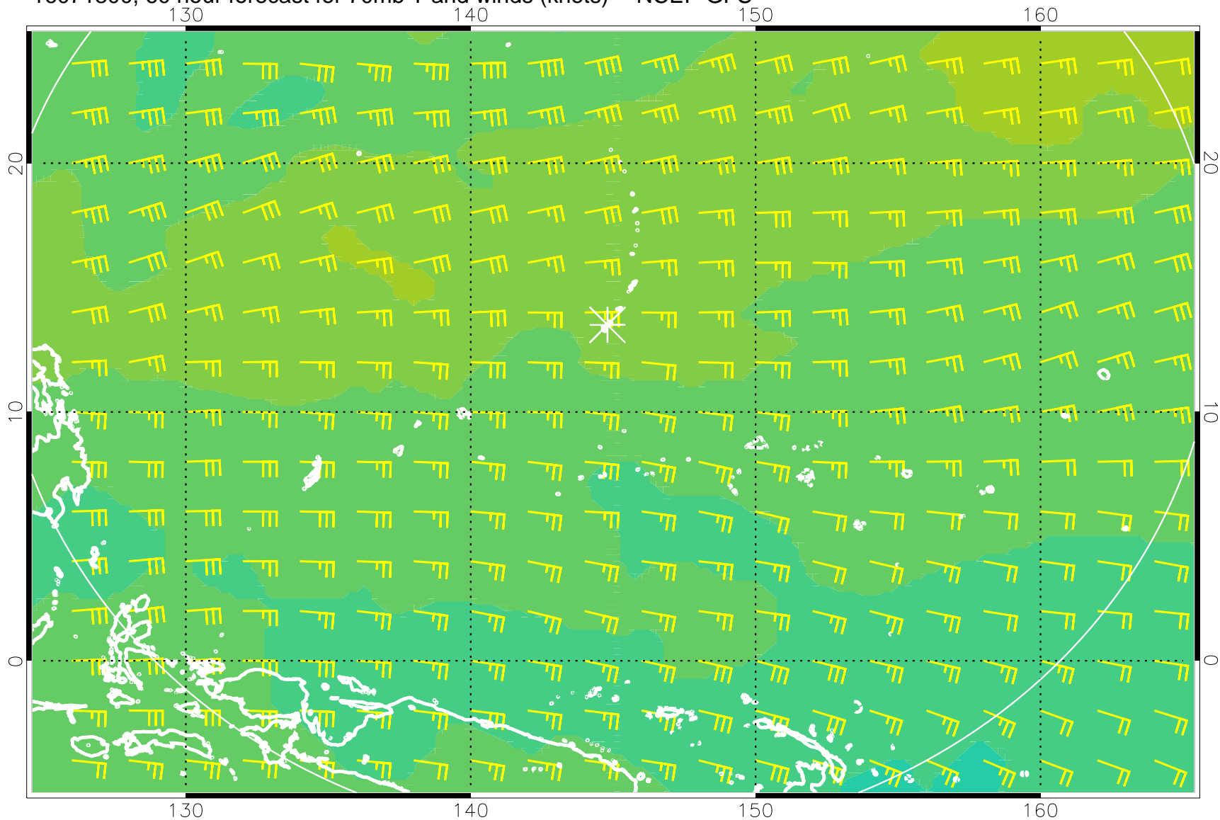
16071800, 60 hour forecast for 70mb T and winds (knots) -- NCEP GFS
