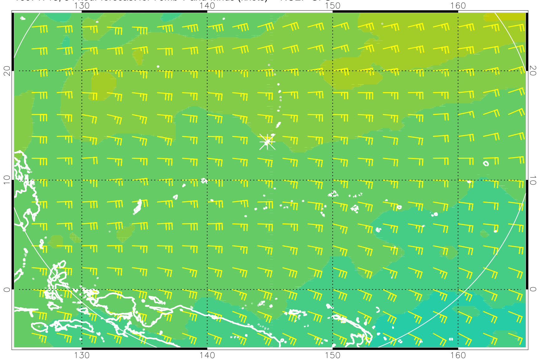
16071718, 54 hour forecast for 70mb T and winds (knots) -- NCEP GFS
