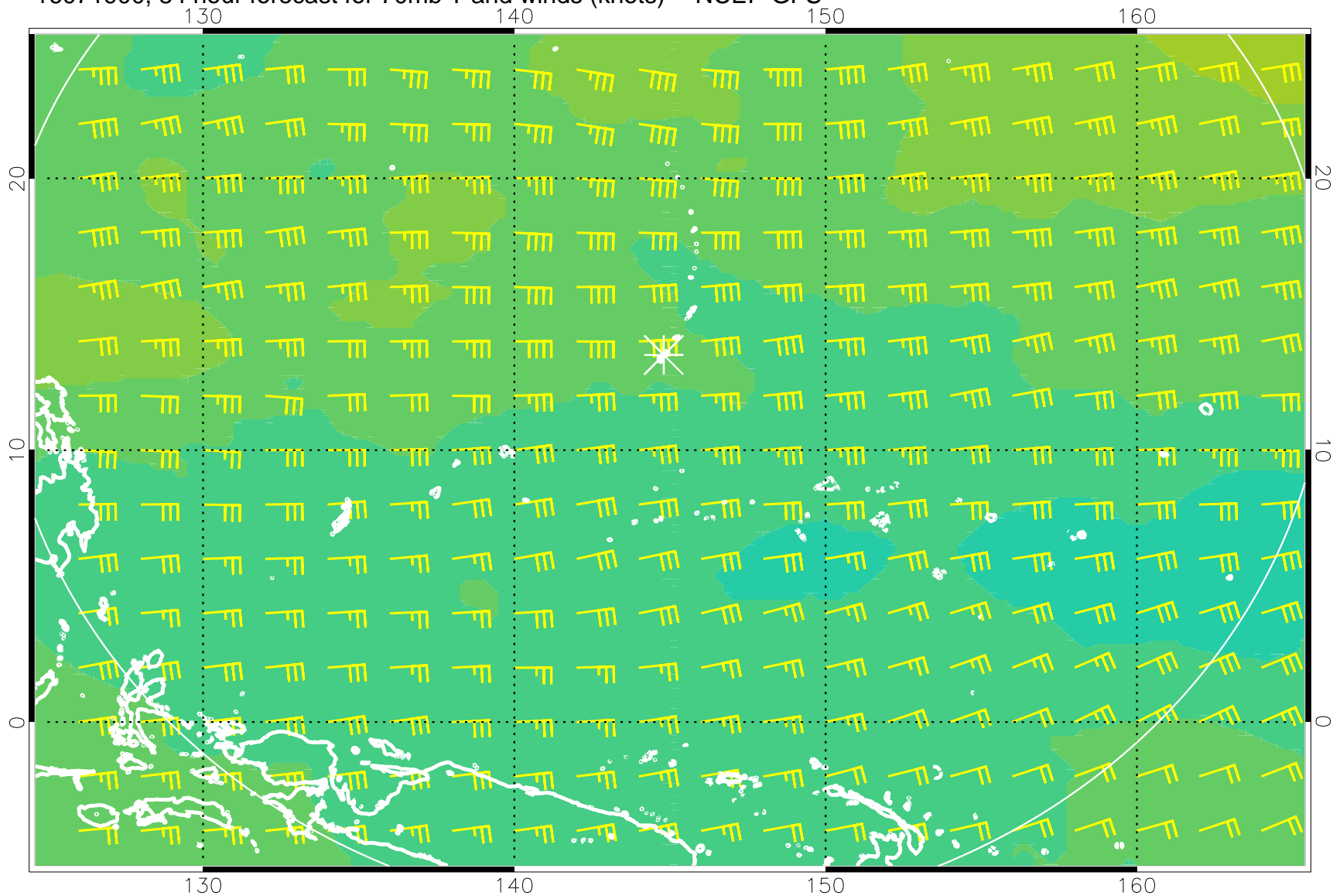
16071900, 84 hour forecast for 70mb T and winds (knots) -- NCEP GFS
