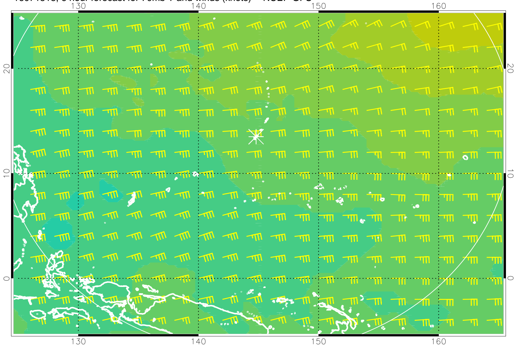
16071518, 6 hour forecast for 70mb T and winds (knots) -- NCEP GFS
