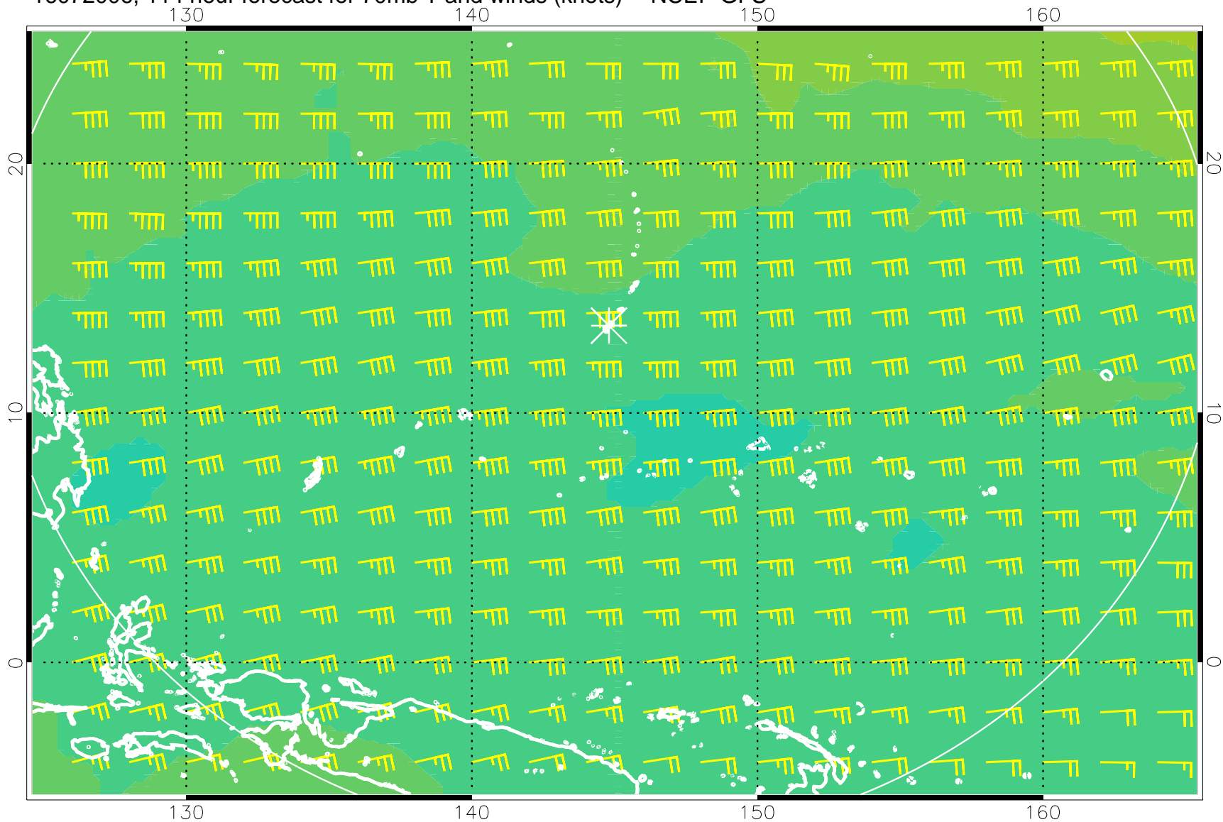
16072006, 114 hour forecast for 70mb T and winds (knots) -- NCEP GFS
