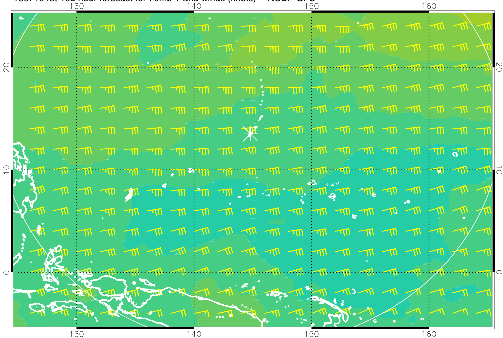
16071918, 102 hour forecast for 70mb T and winds (knots) -- NCEP GFS
