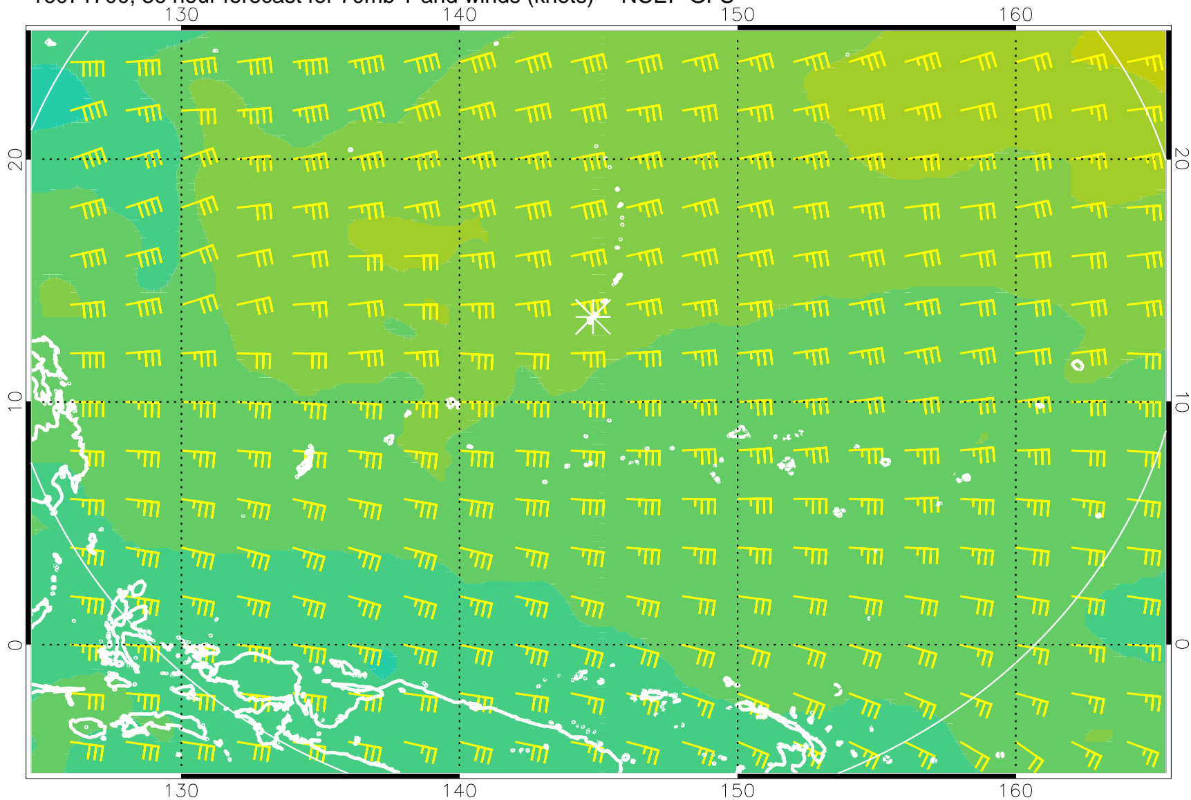
16071700, 36 hour forecast for 70mb T and winds (knots) -- NCEP GFS
