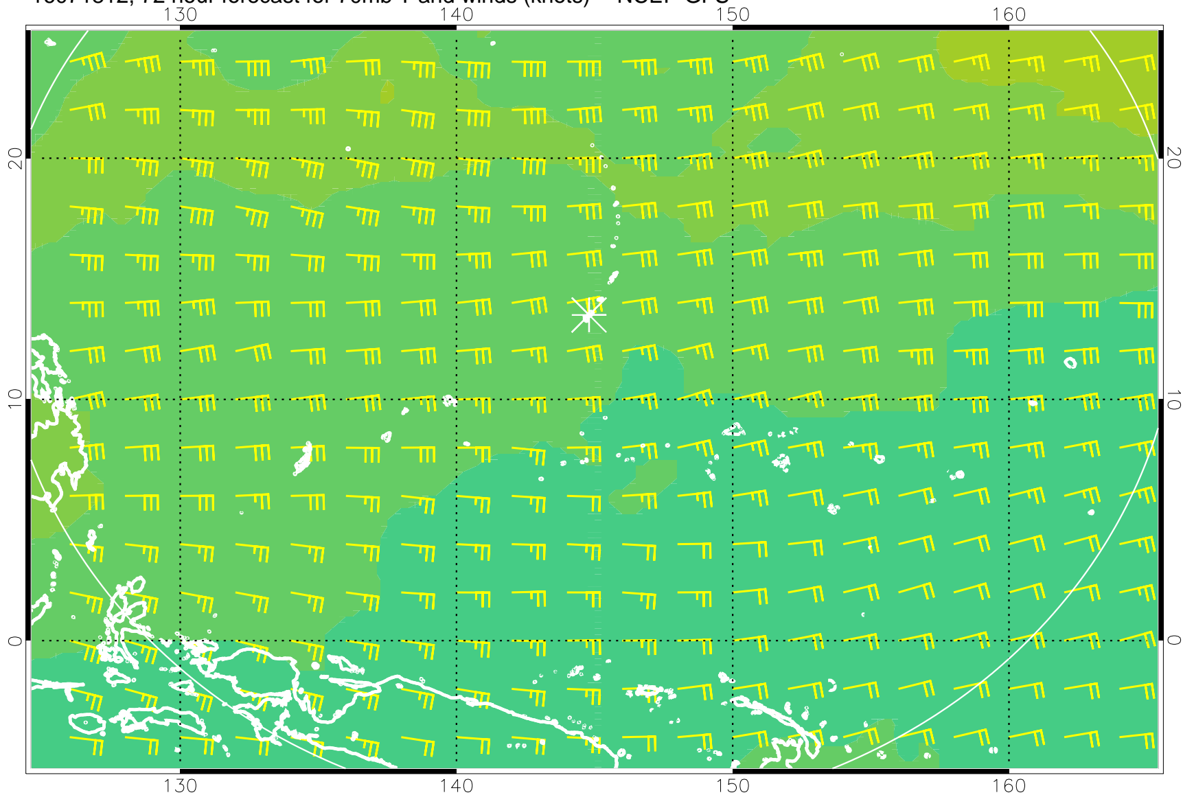
16071812, 72 hour forecast for 70mb T and winds (knots) -- NCEP GFS
