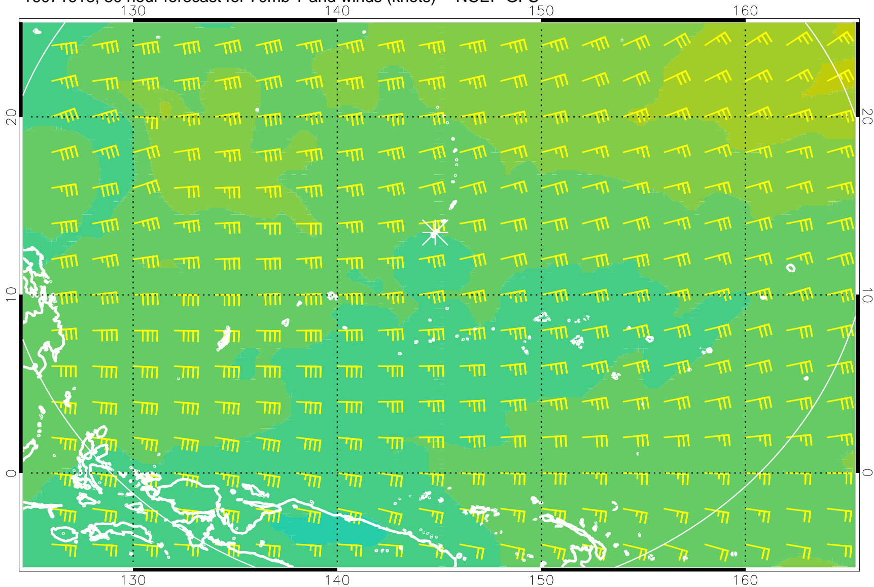
16071618, 30 hour forecast for 70mb T and winds (knots) -- NCEP GFS
