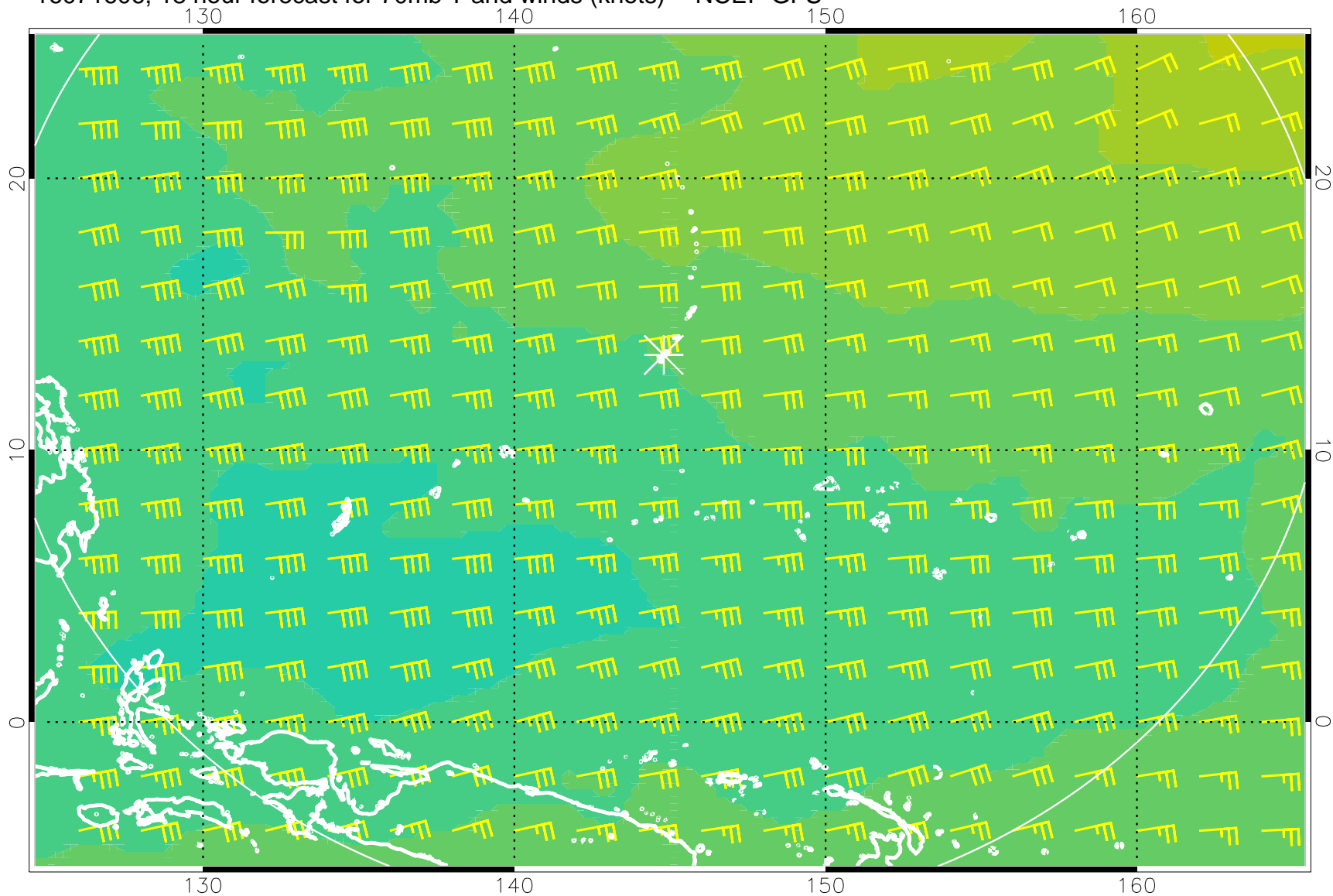
16071606, 18 hour forecast for 70mb T and winds (knots) -- NCEP GFS
