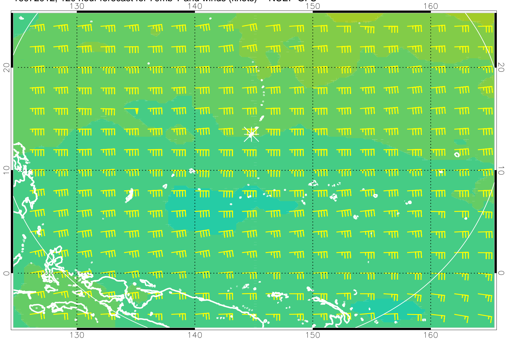
16072012, 120 hour forecast for 70mb T and winds (knots) -- NCEP GFS
