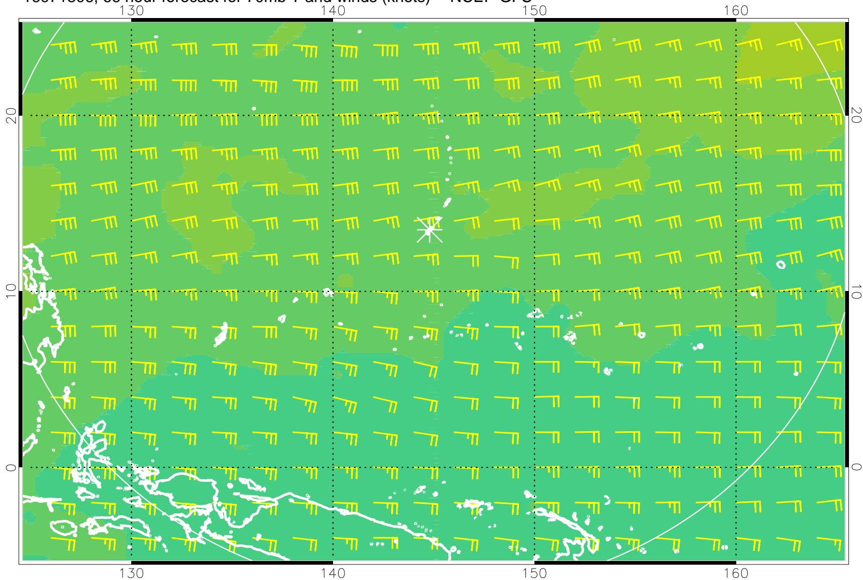
16071806, 66 hour forecast for 70mb T and winds (knots) -- NCEP GFS
