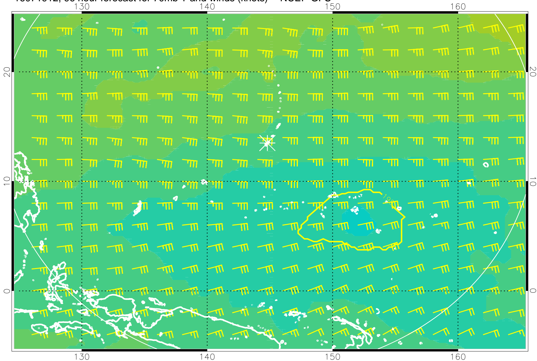
16071912, 96 hour forecast for 70mb T and winds (knots) -- NCEP GFS
