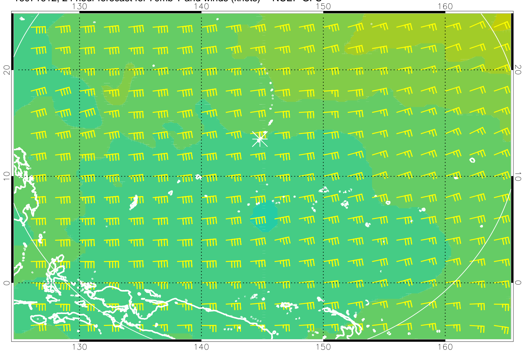
16071612, 24 hour forecast for 70mb T and winds (knots) -- NCEP GFS
