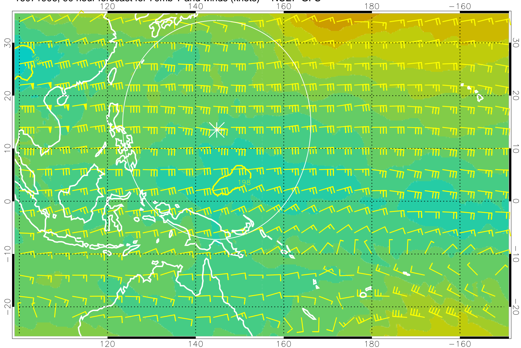
16071906, 90 hour forecast for 70mb T and winds (knots) -- NCEP GFS
