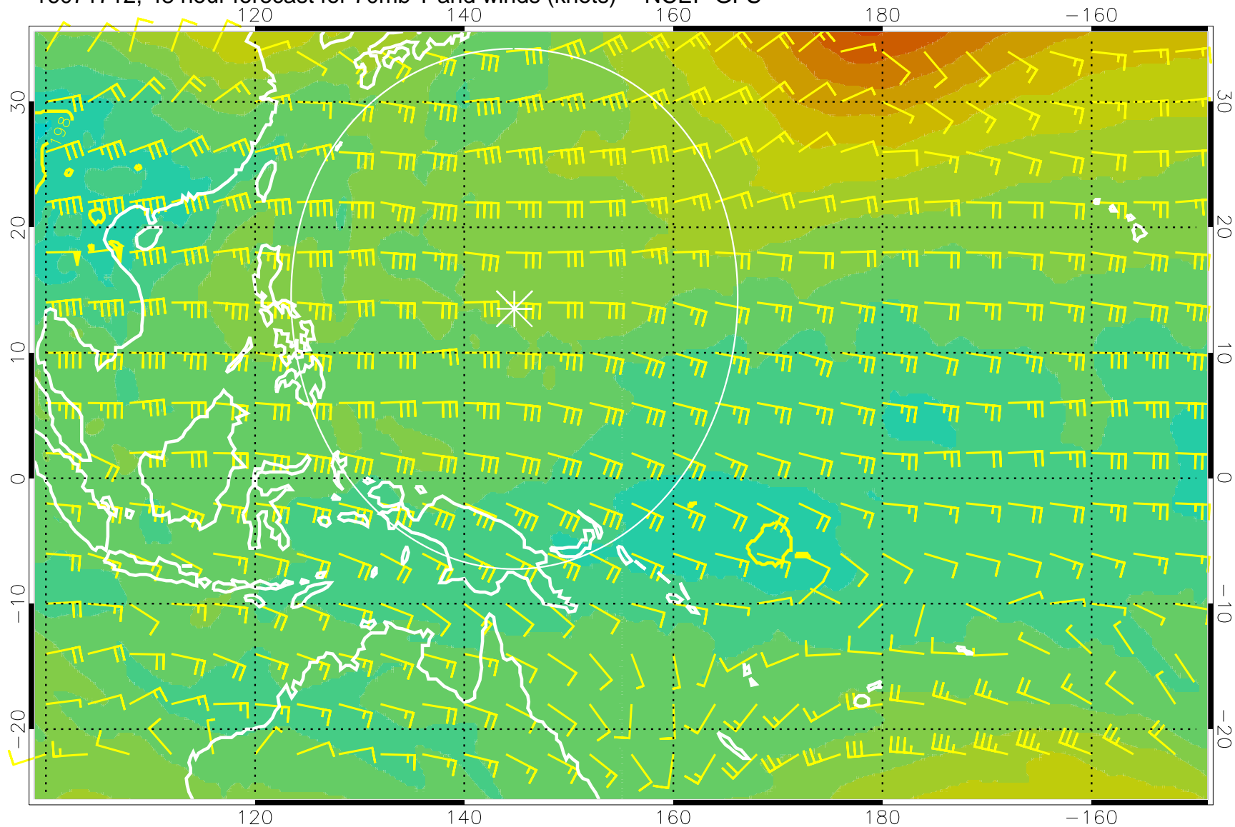
16071712, 48 hour forecast for 70mb T and winds (knots) -- NCEP GFS
