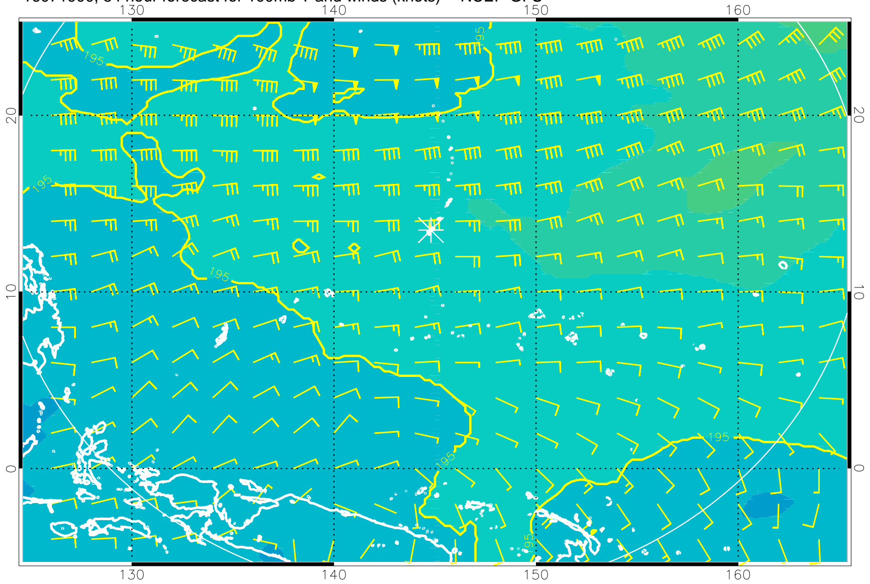
16071900, 84 hour forecast for 100mb T and winds (knots) -- NCEP GFS
