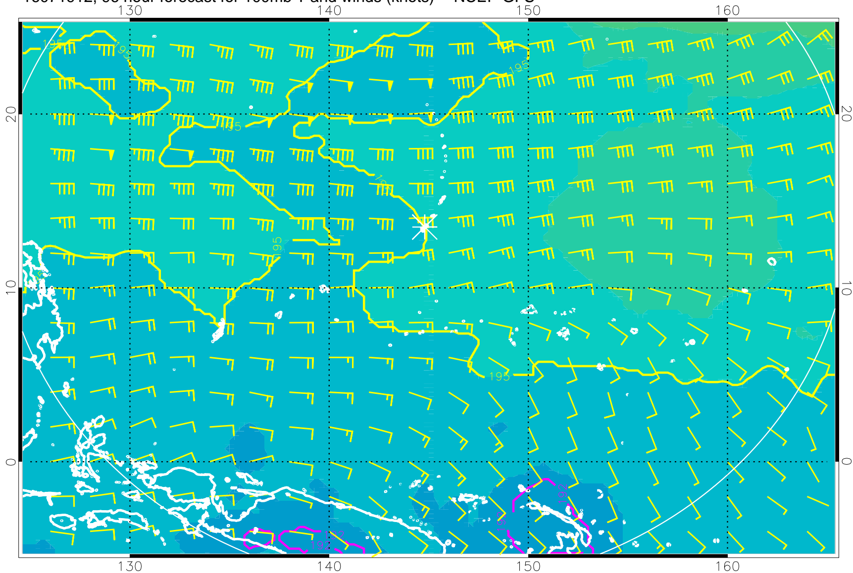
16071912, 96 hour forecast for 100mb T and winds (knots) -- NCEP GFS
