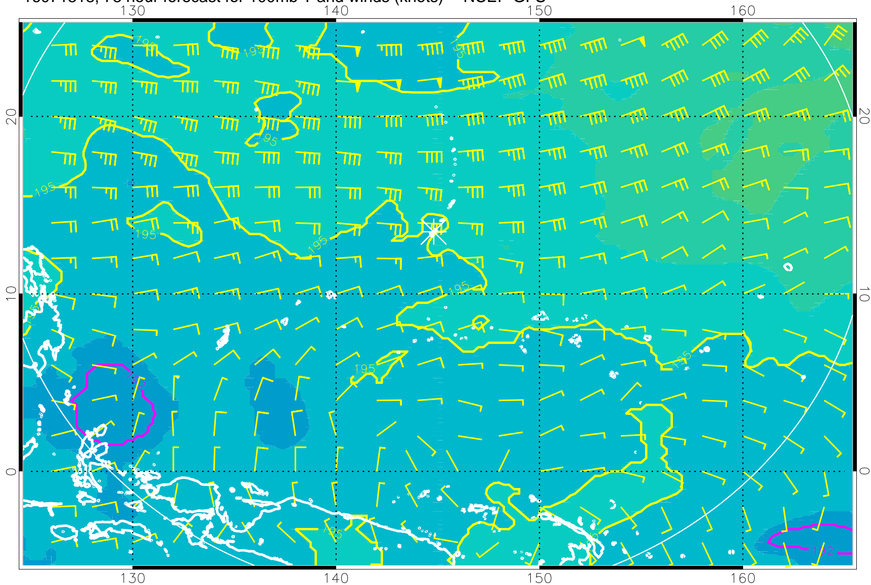
16071818, 78 hour forecast for 100mb T and winds (knots) -- NCEP GFS
