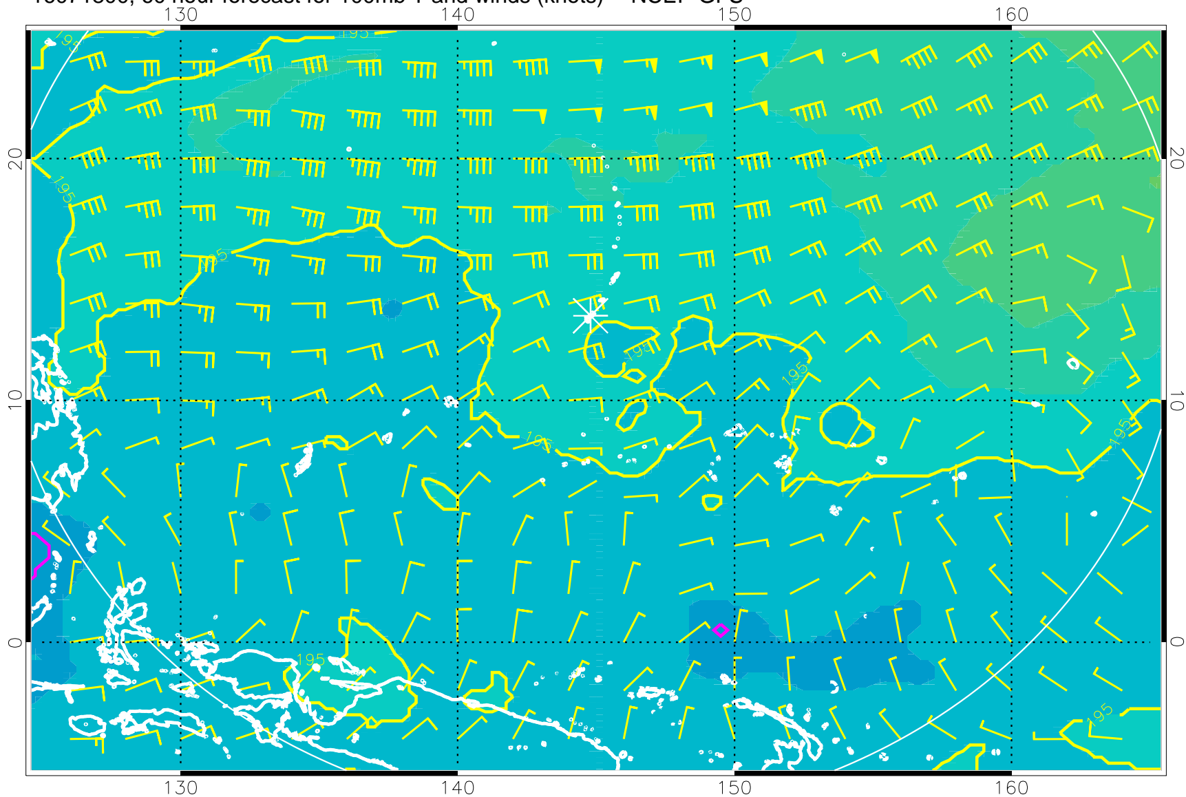
16071800, 60 hour forecast for 100mb T and winds (knots) -- NCEP GFS
