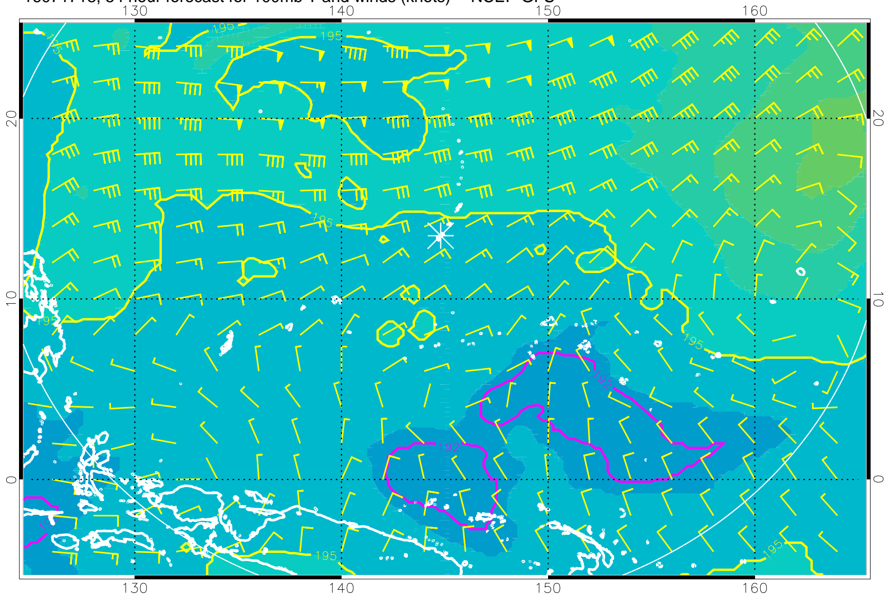
16071718, 54 hour forecast for 100mb T and winds (knots) -- NCEP GFS
