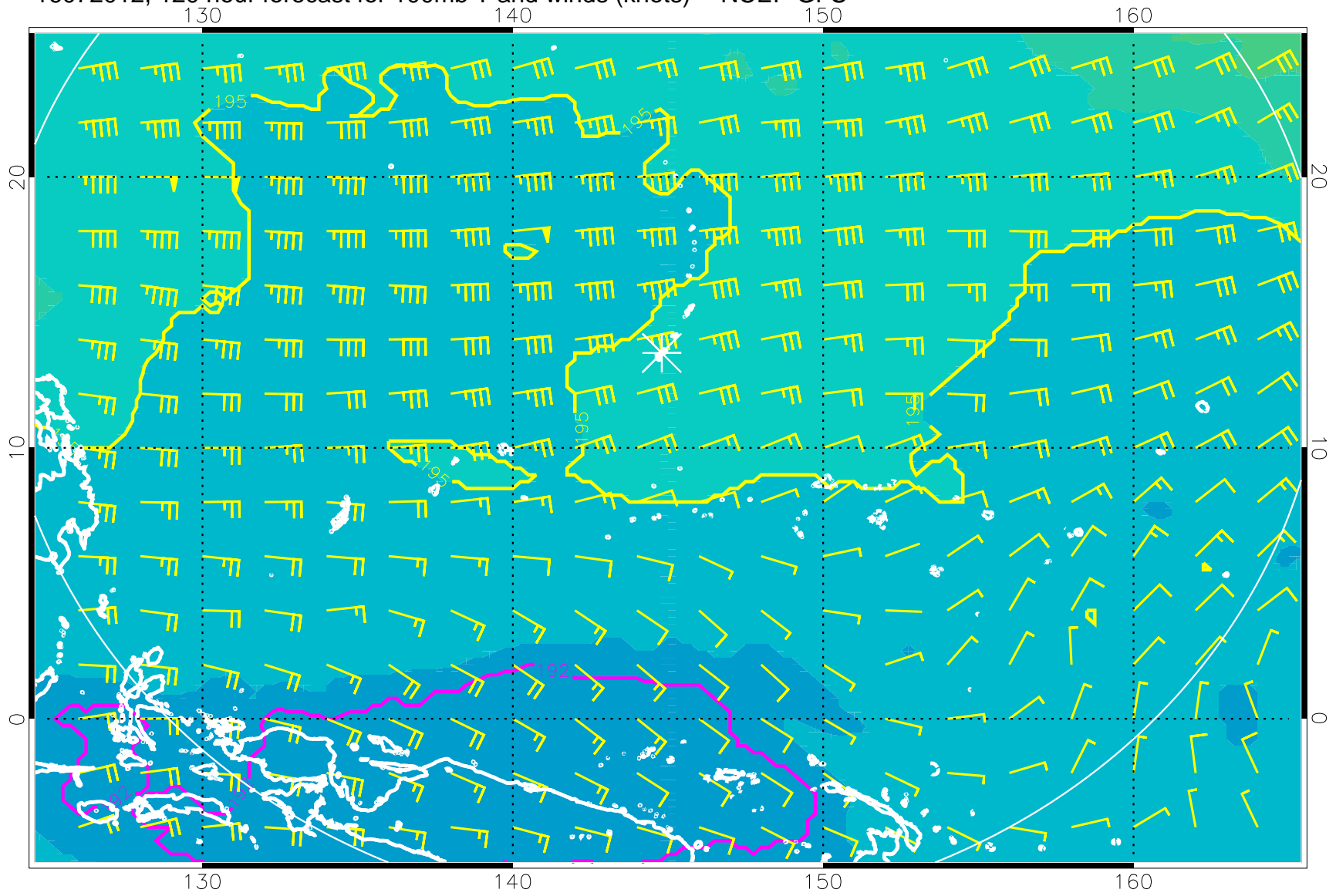
16072012, 120 hour forecast for 100mb T and winds (knots) -- NCEP GFS
