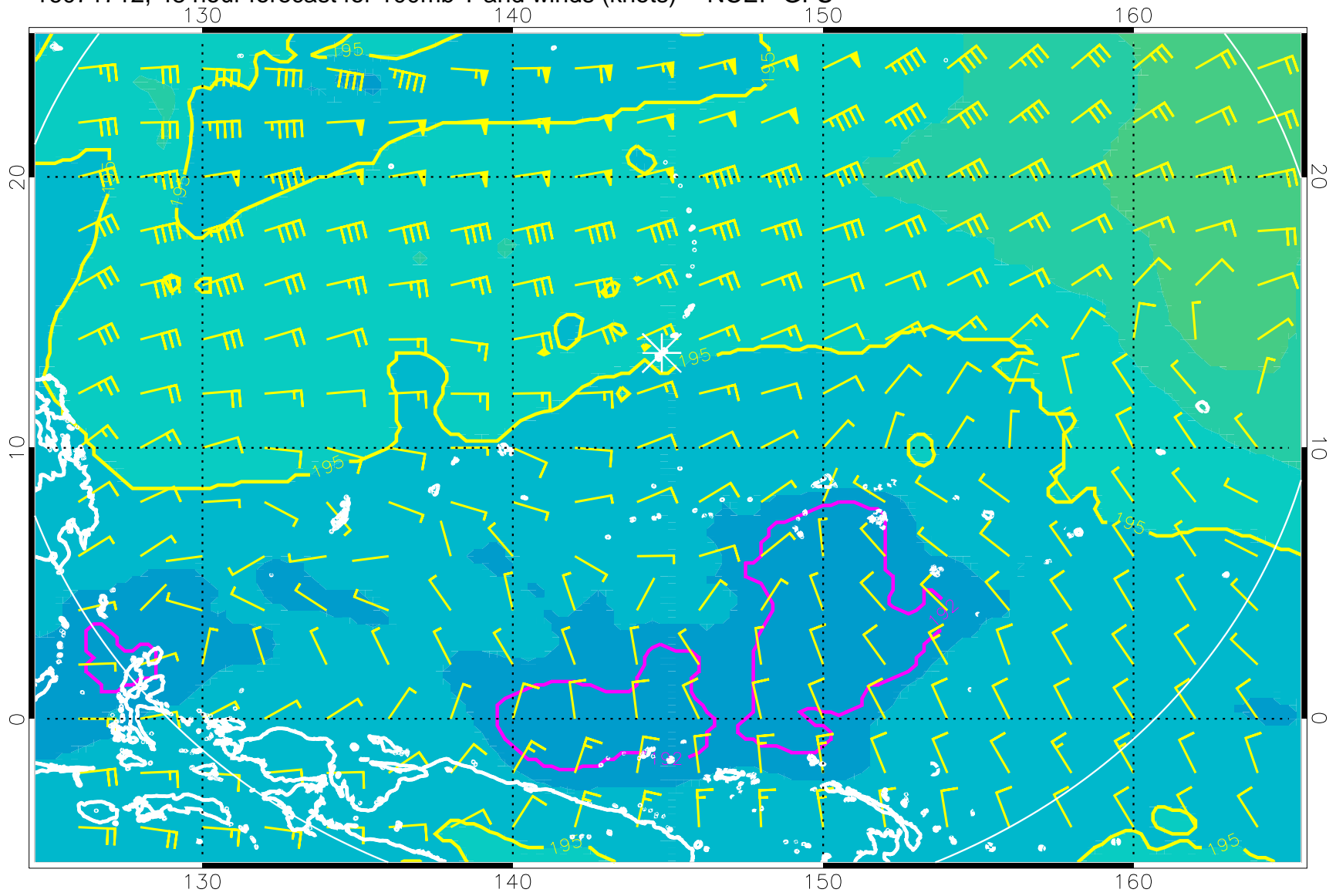
16071712, 48 hour forecast for 100mb T and winds (knots) -- NCEP GFS
