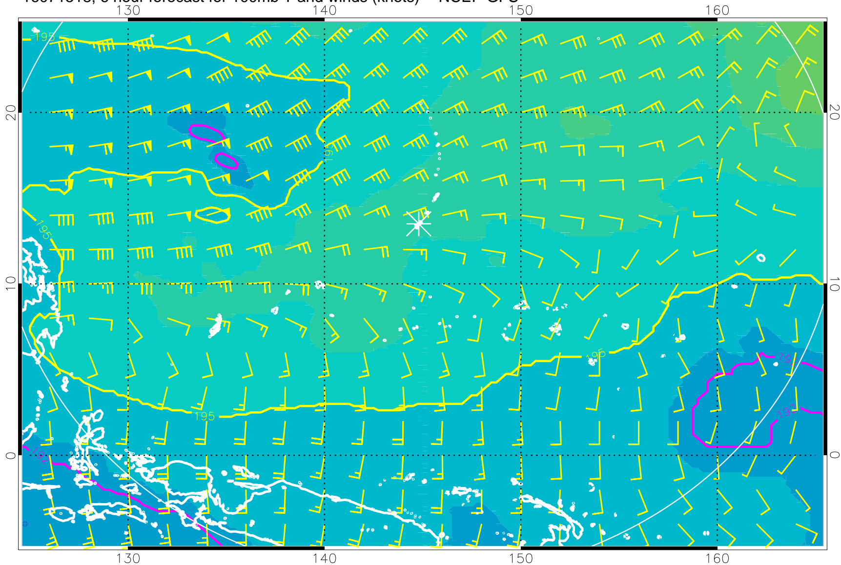
16071518, 6 hour forecast for 100mb T and winds (knots) -- NCEP GFS
