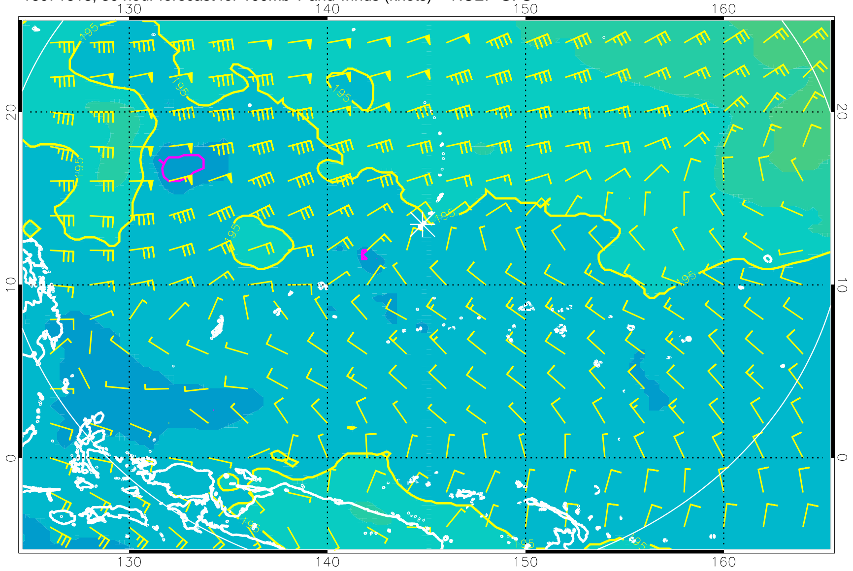
16071618, 30 hour forecast for 100mb T and winds (knots) -- NCEP GFS
