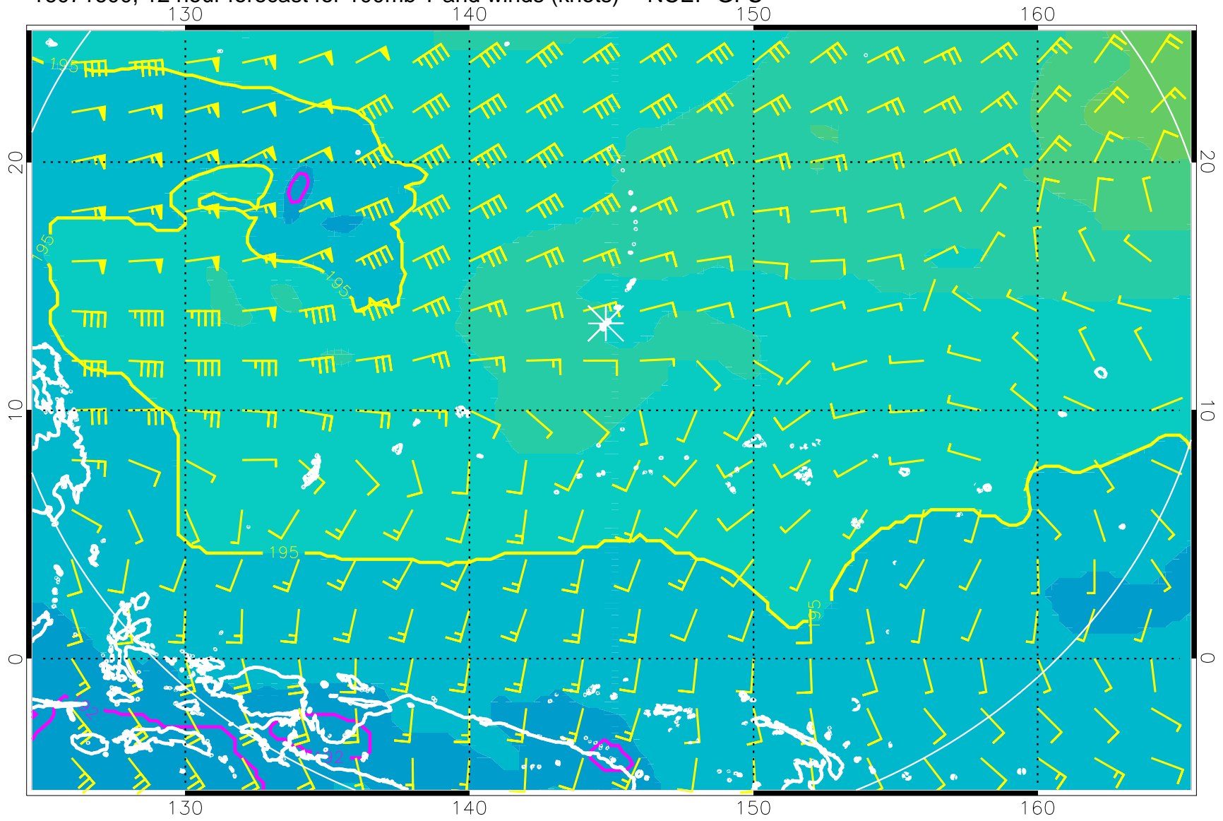
16071600, 12 hour forecast for 100mb T and winds (knots) -- NCEP GFS
