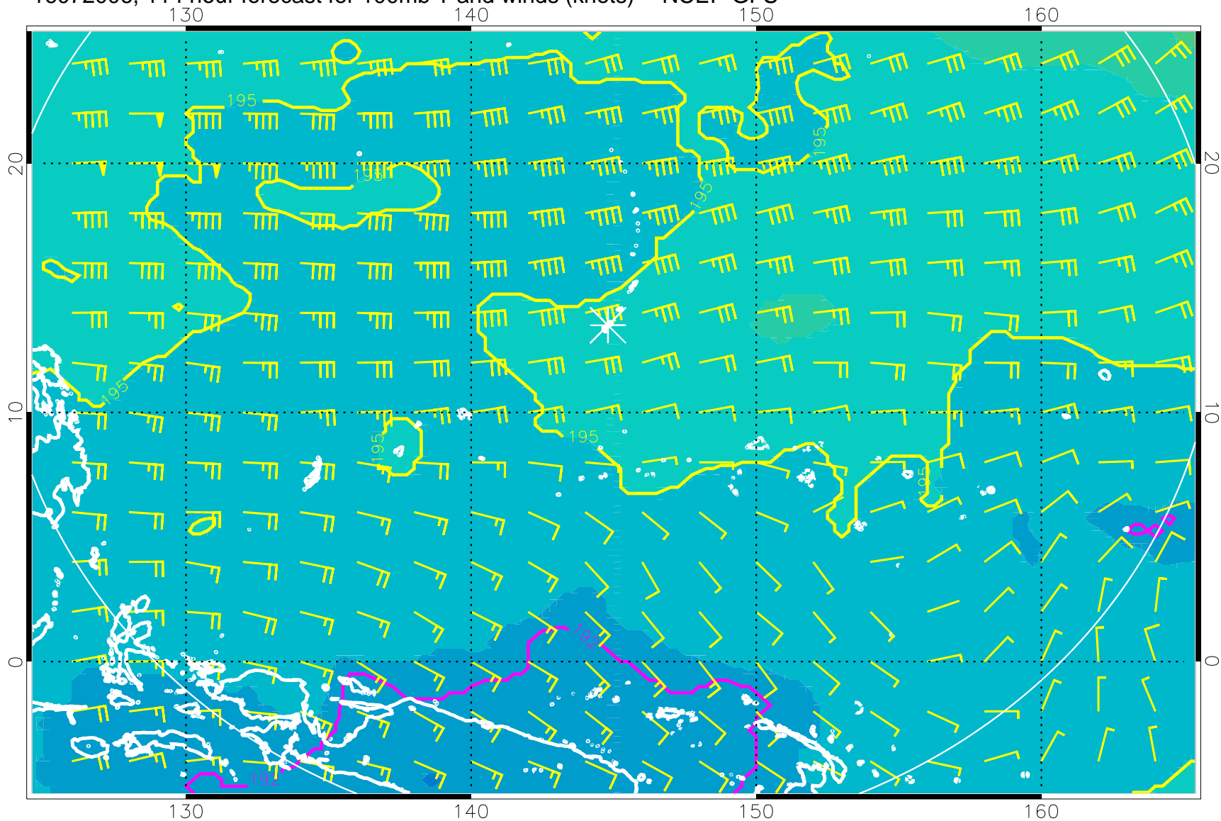
16072006, 114 hour forecast for 100mb T and winds (knots) -- NCEP GFS
