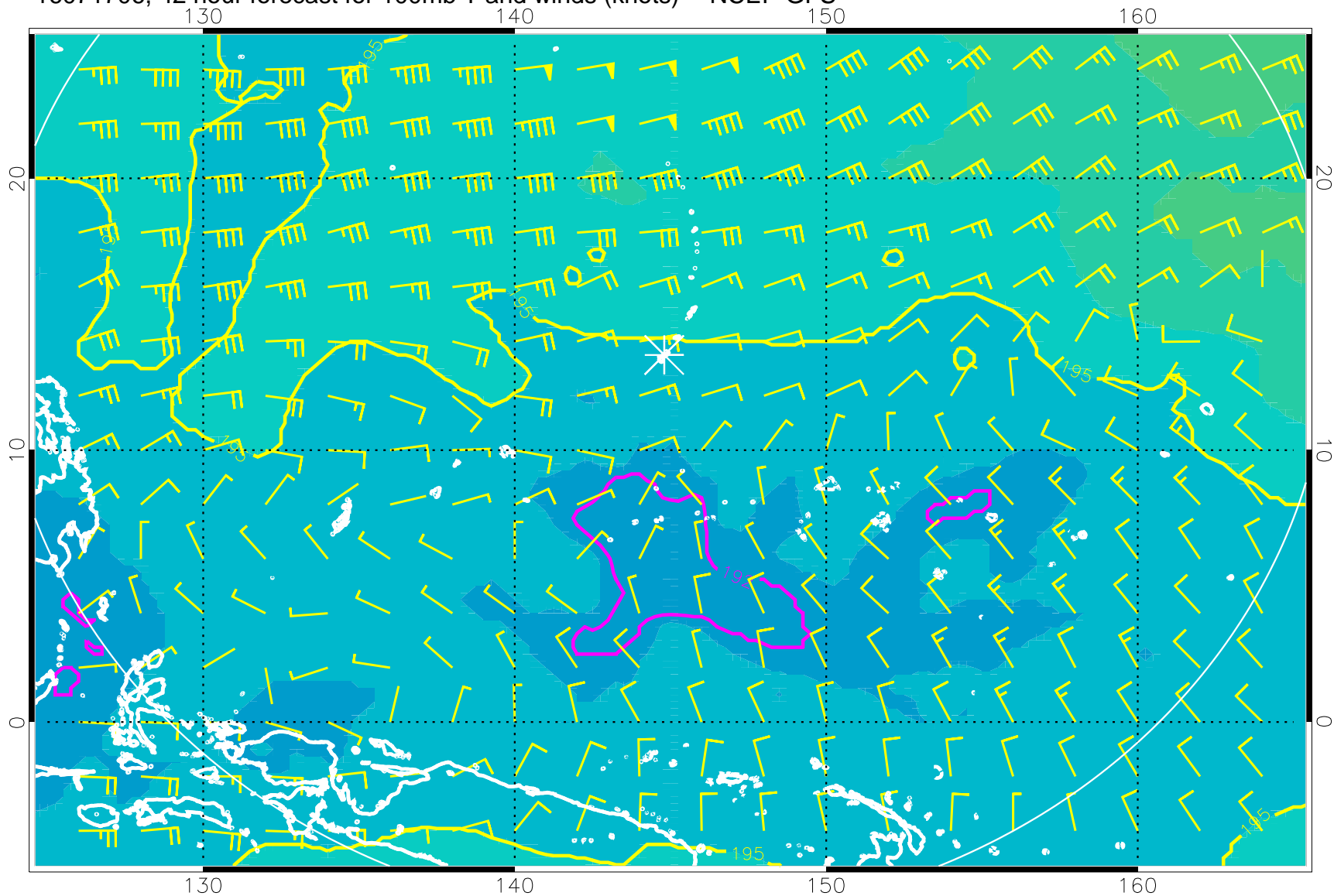
16071706, 42 hour forecast for 100mb T and winds (knots) -- NCEP GFS
