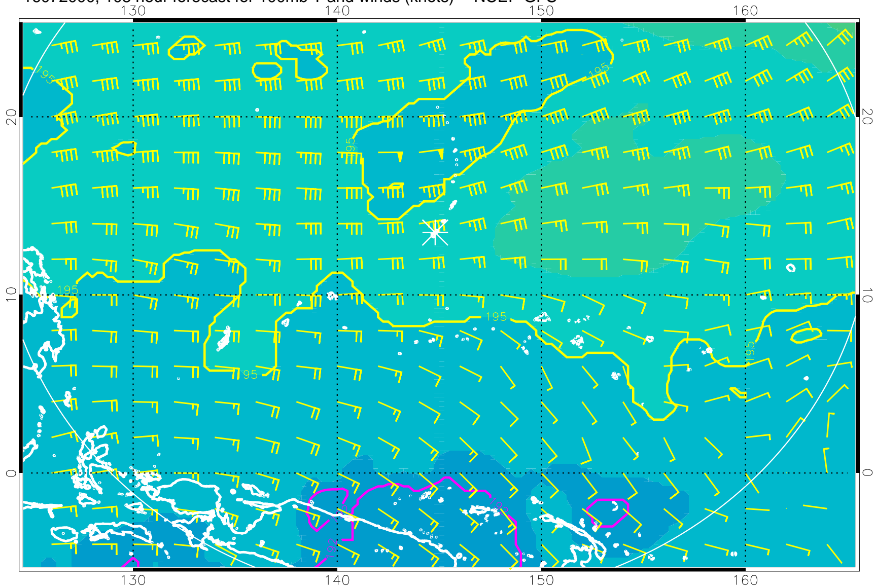
16072000, 108 hour forecast for 100mb T and winds (knots) -- NCEP GFS
