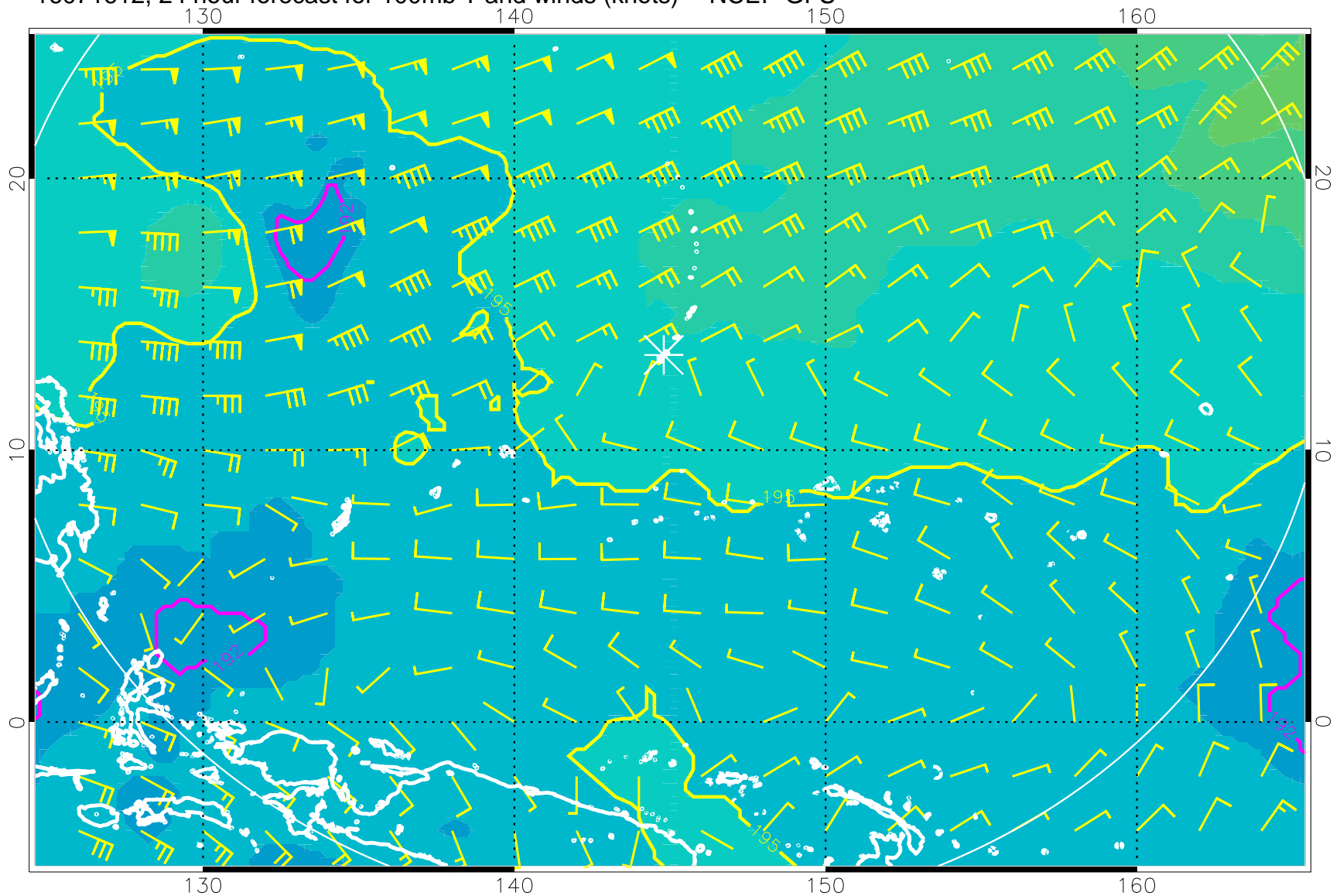
16071612, 24 hour forecast for 100mb T and winds (knots) -- NCEP GFS
