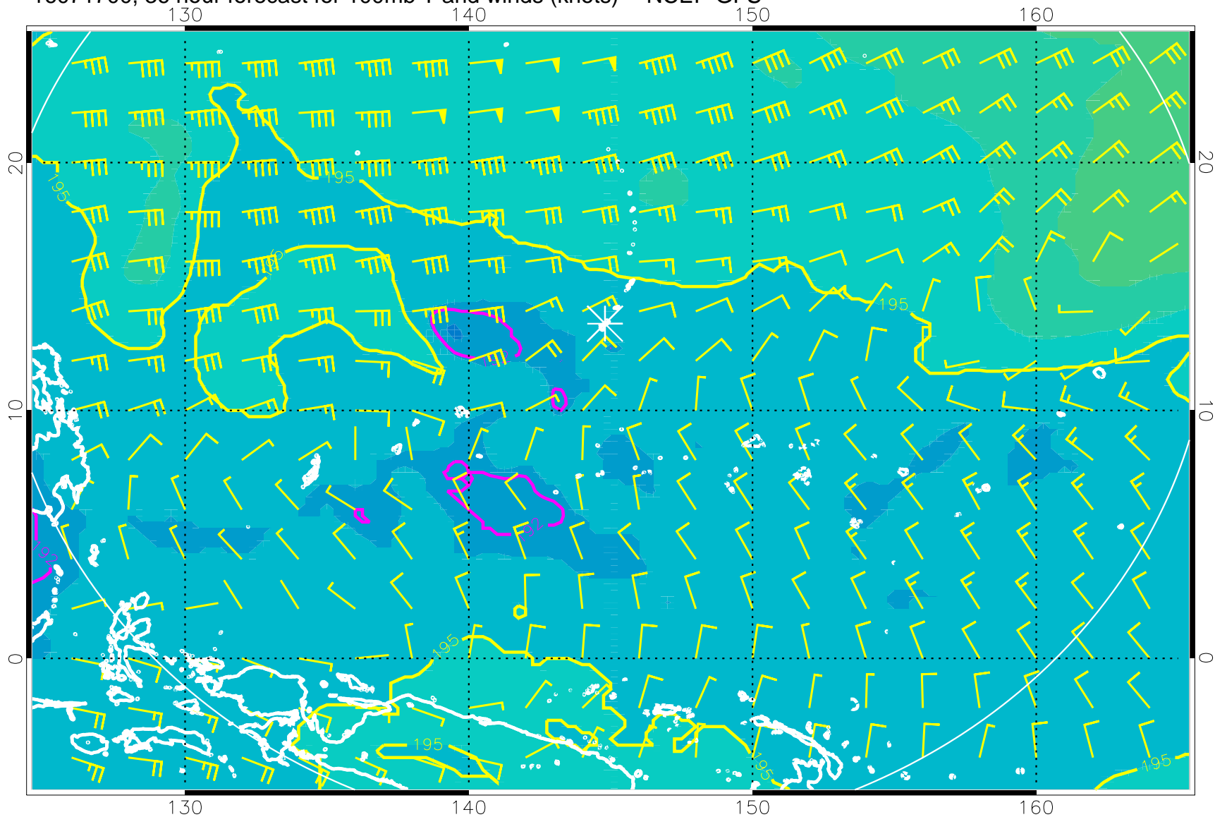
16071700, 36 hour forecast for 100mb T and winds (knots) -- NCEP GFS
