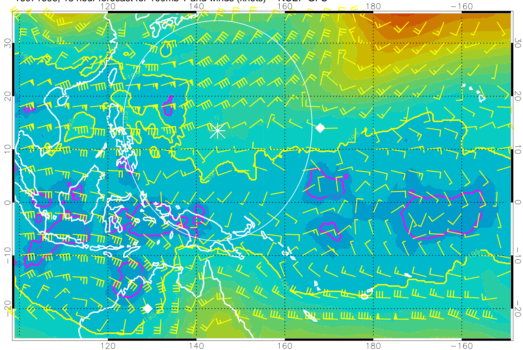
16071606, 18 hour forecast for 100mb T and winds (knots) -- NCEP GFS
