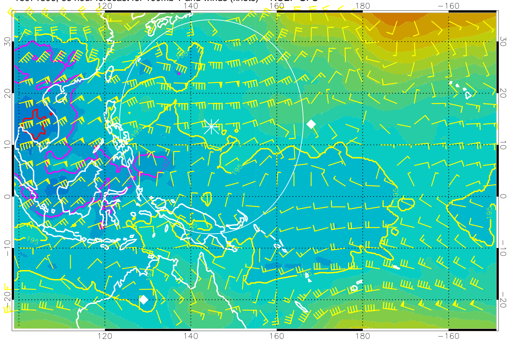
16071806, 66 hour forecast for 100mb T and winds (knots) -- NCEP GFS
