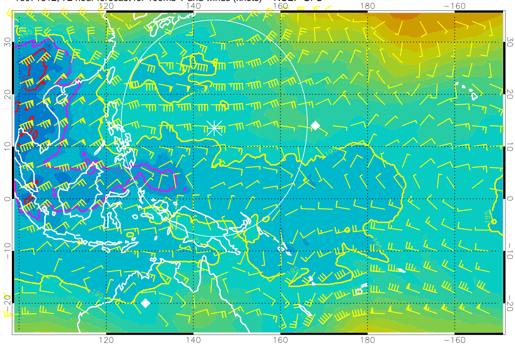
16071812, 72 hour forecast for 100mb T and winds (knots) -- NCEP GFS
