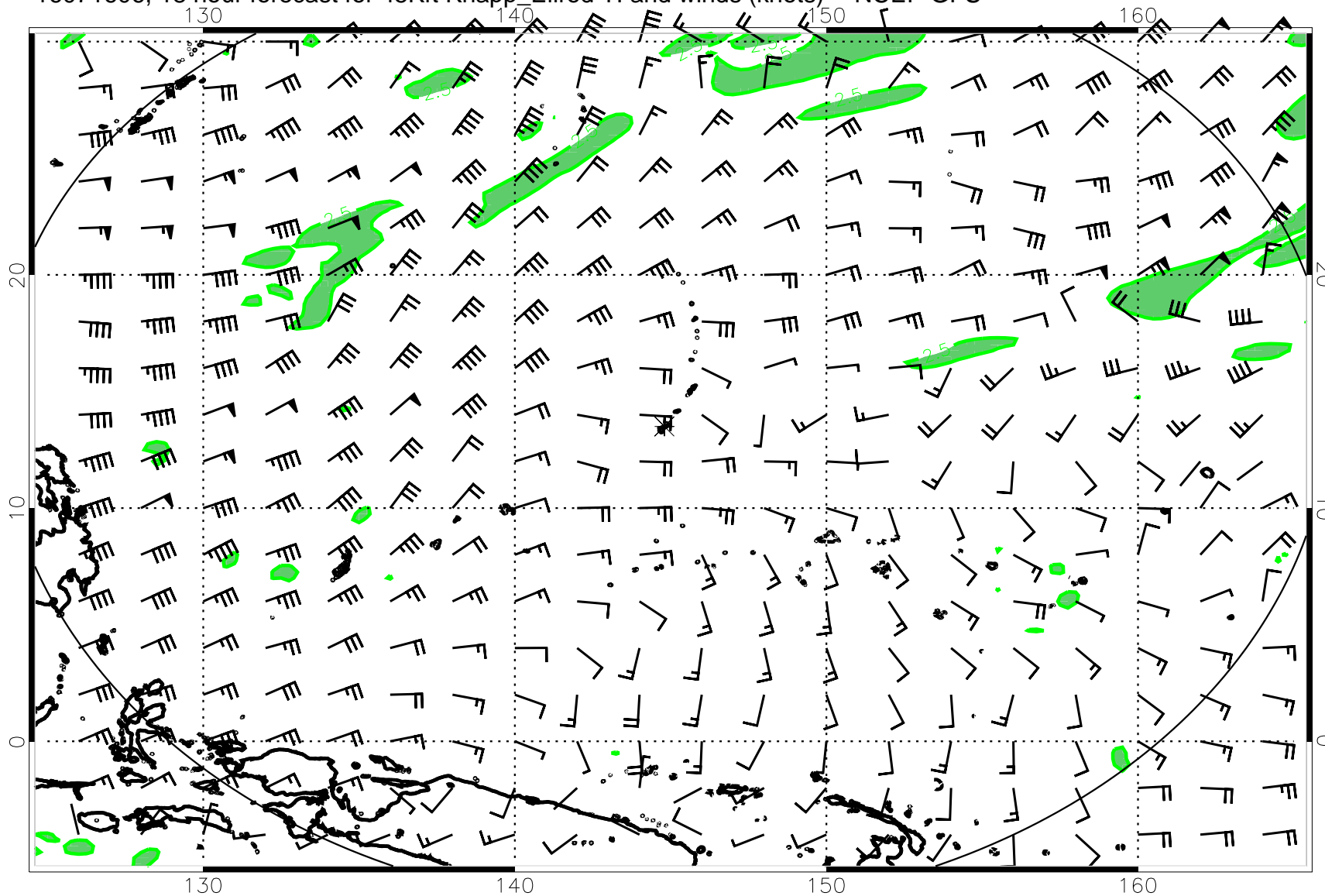
16071606, 18 hour forecast for 45Kft Knapp_Ellrod TI and winds (knots) -- NCEP GFS
