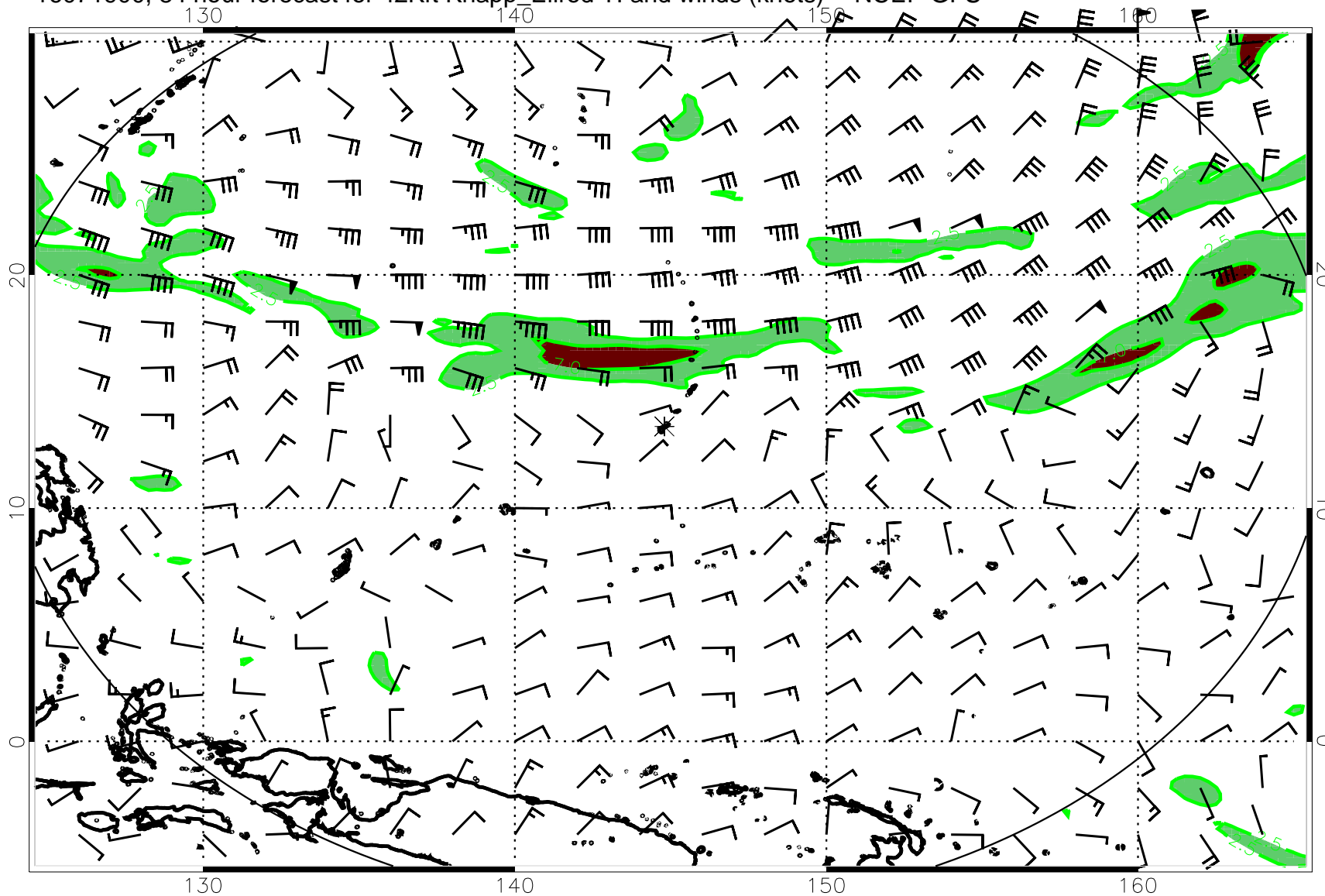
16071900, 84 hour forecast for 42Kft Knapp_Ellrod TI and winds (knots) -- NCEP GFS
