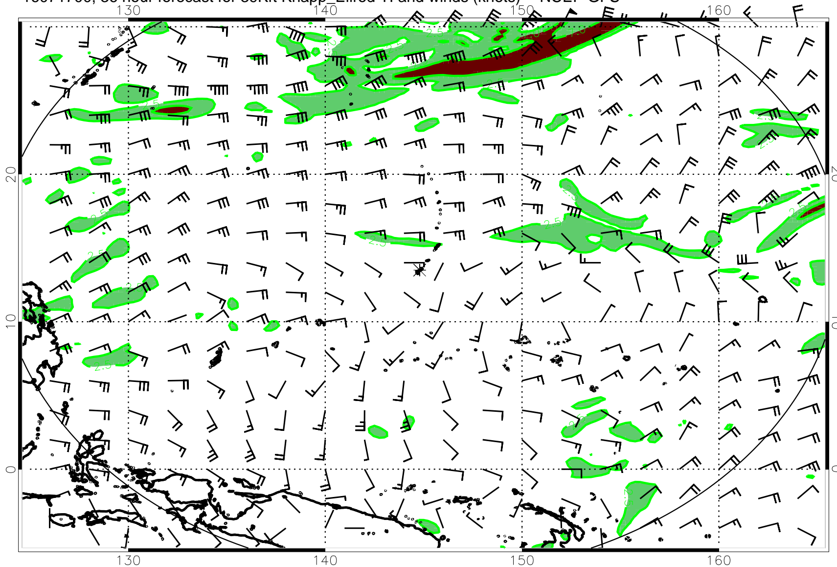
16071700, 36 hour forecast for 39Kft Knapp_Ellrod TI and winds (knots) -- NCEP GFS
