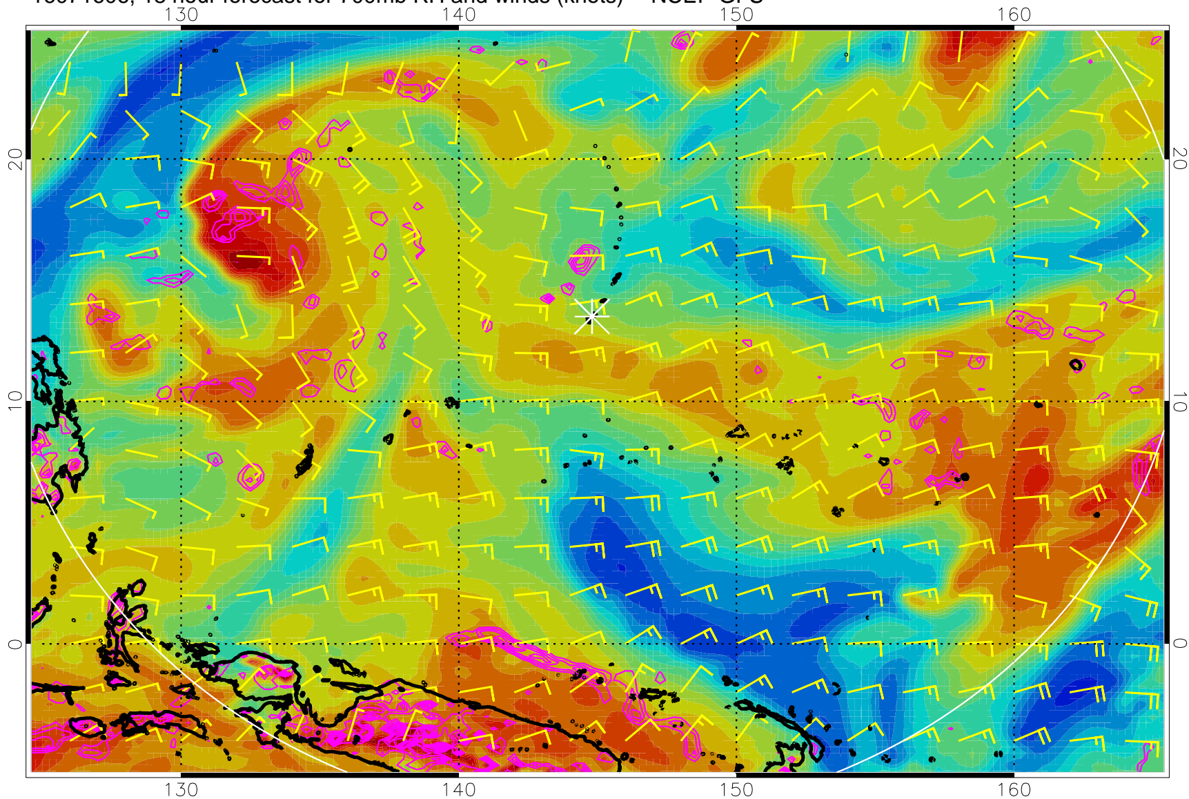
16071606, 18 hour forecast for 700mb RH and winds (knots) -- NCEP GFS
