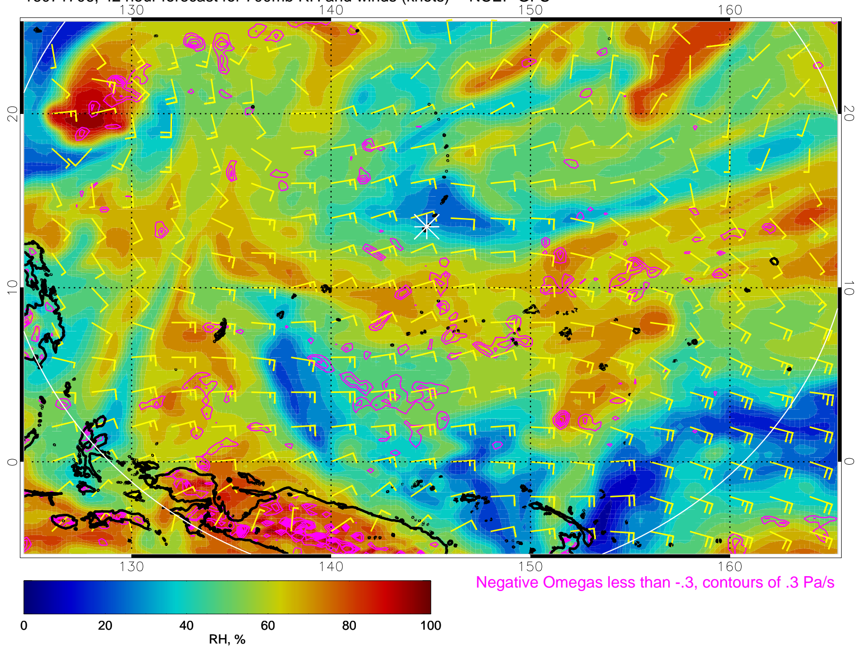
16071706, 42 hour forecast for 700mb RH and winds (knots) -- NCEP GFS
