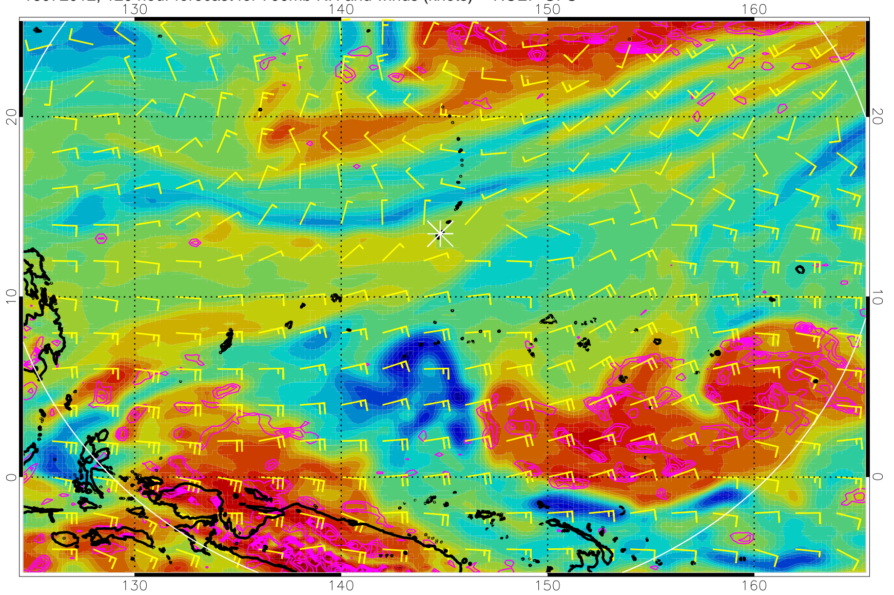
16072012, 120 hour forecast for 700mb RH and winds (knots) -- NCEP GFS
