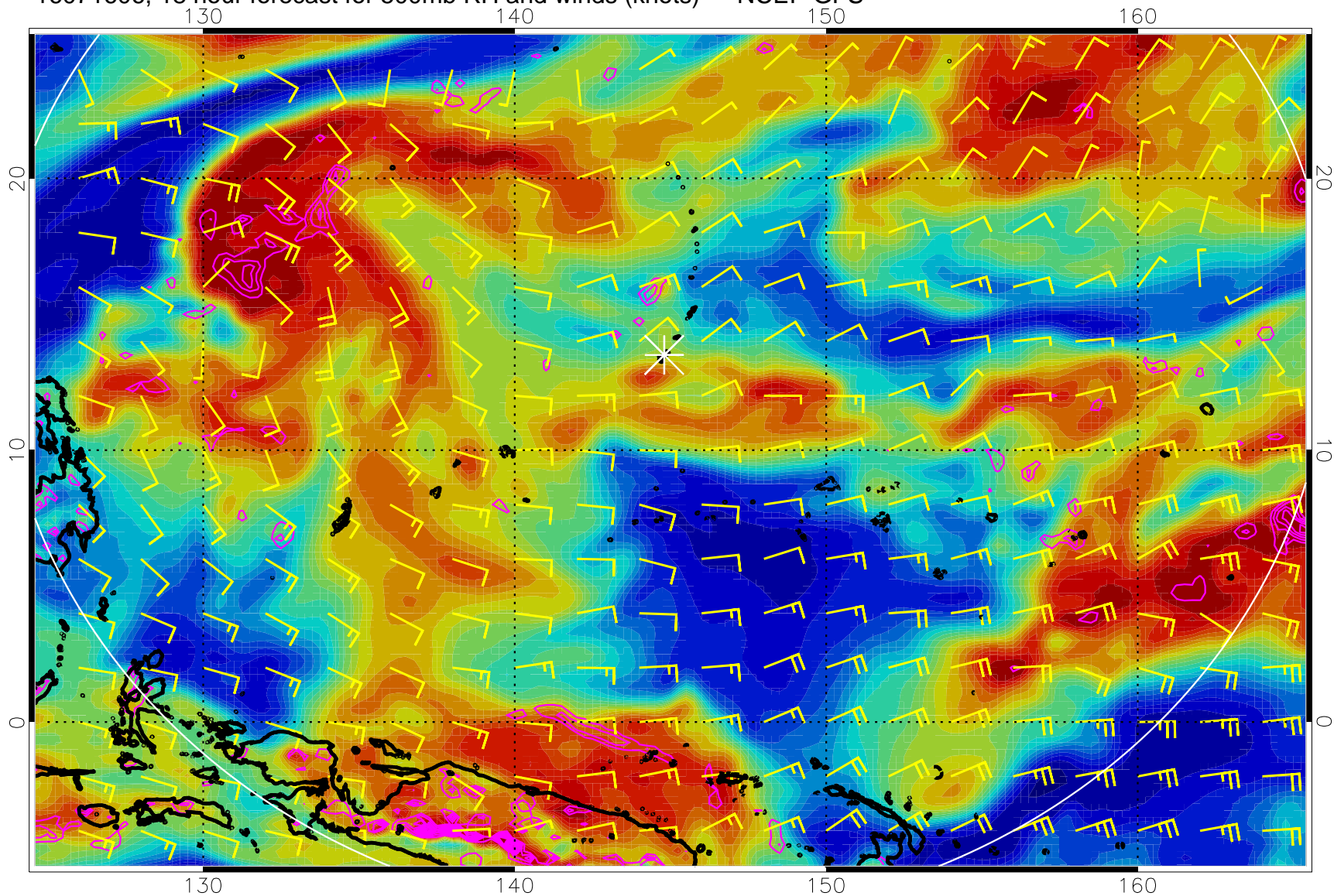
16071606, 18 hour forecast for 500mb RH and winds (knots) -- NCEP GFS
