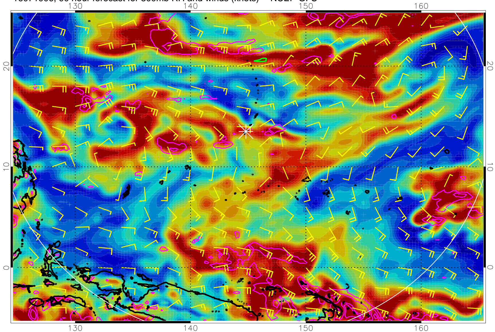
16071906, 90 hour forecast for 300mb RH and winds (knots) -- NCEP GFS
