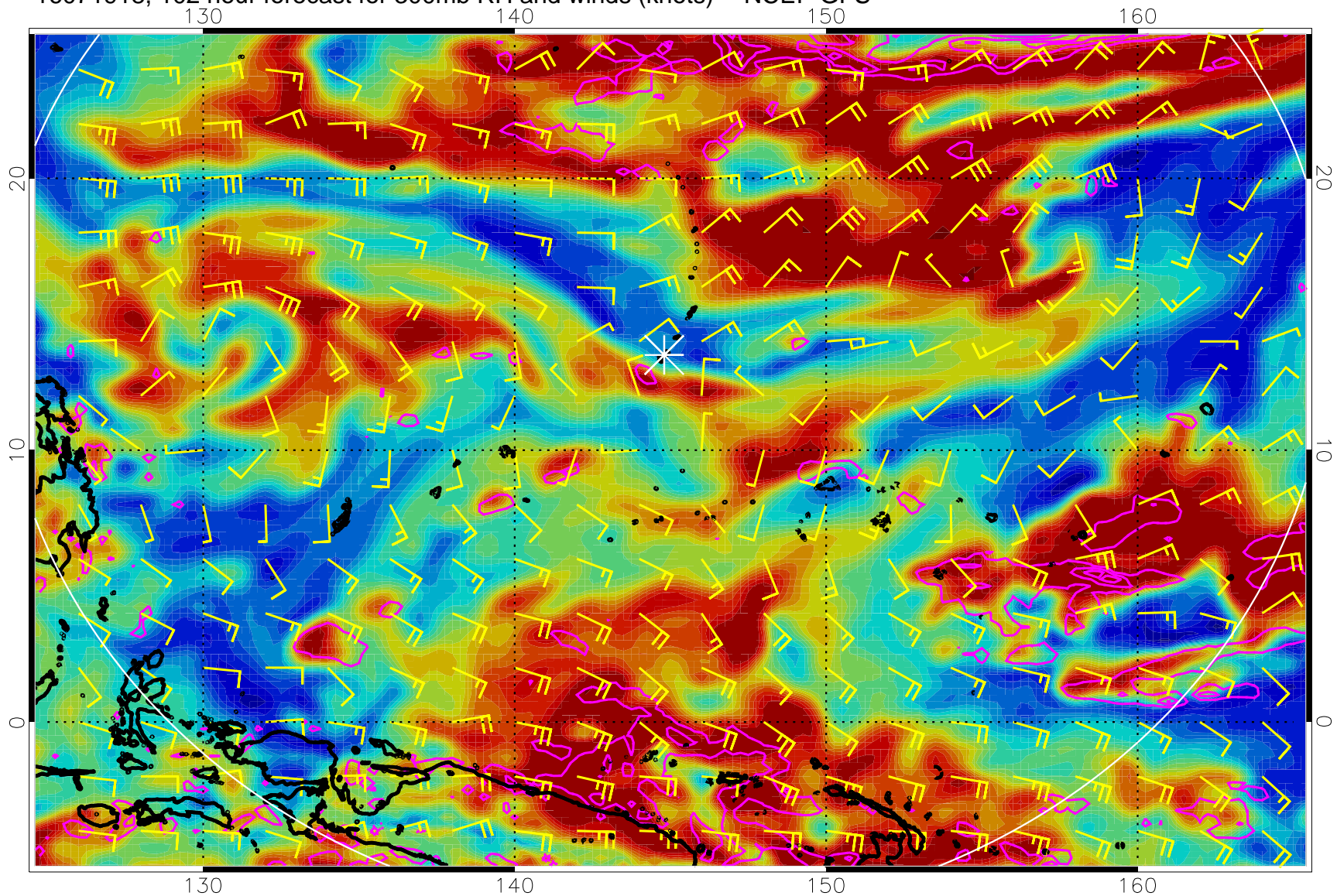
16071918, 102 hour forecast for 300mb RH and winds (knots) -- NCEP GFS
