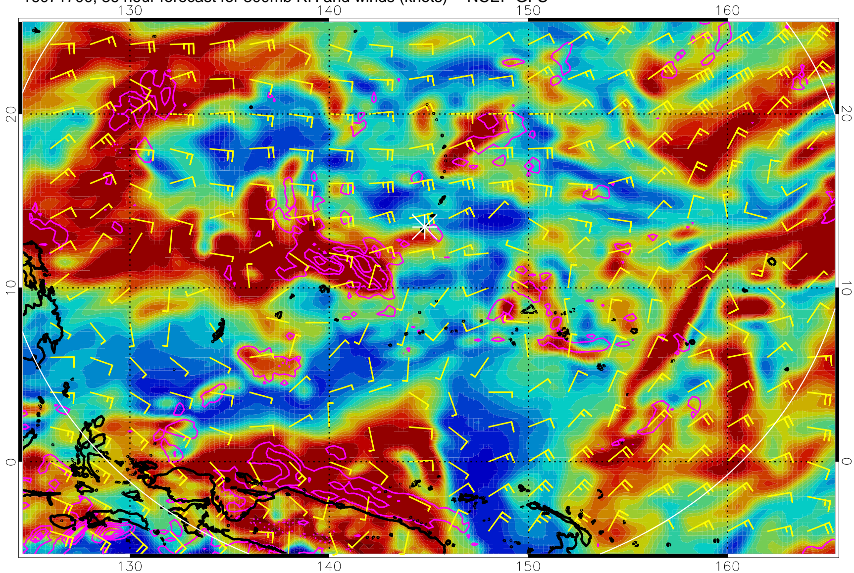
16071700, 36 hour forecast for 300mb RH and winds (knots) -- NCEP GFS
