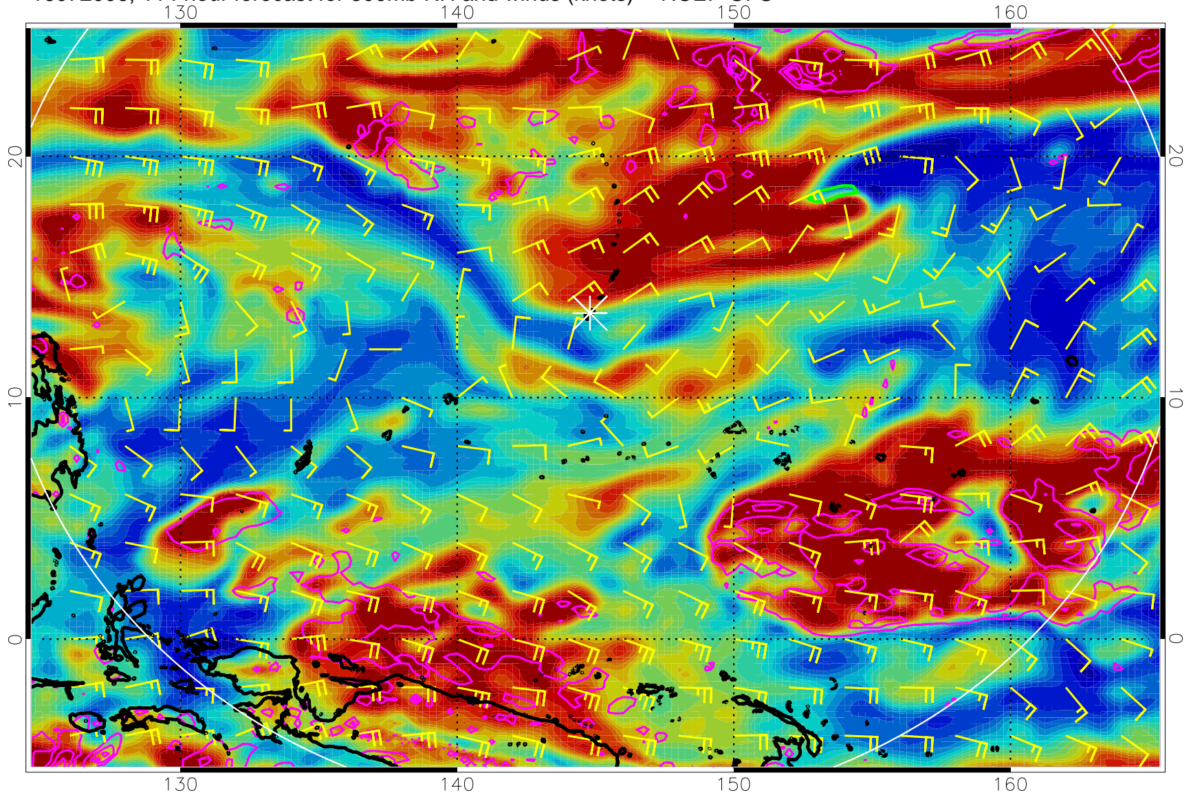
16072006, 114 hour forecast for 300mb RH and winds (knots) -- NCEP GFS
