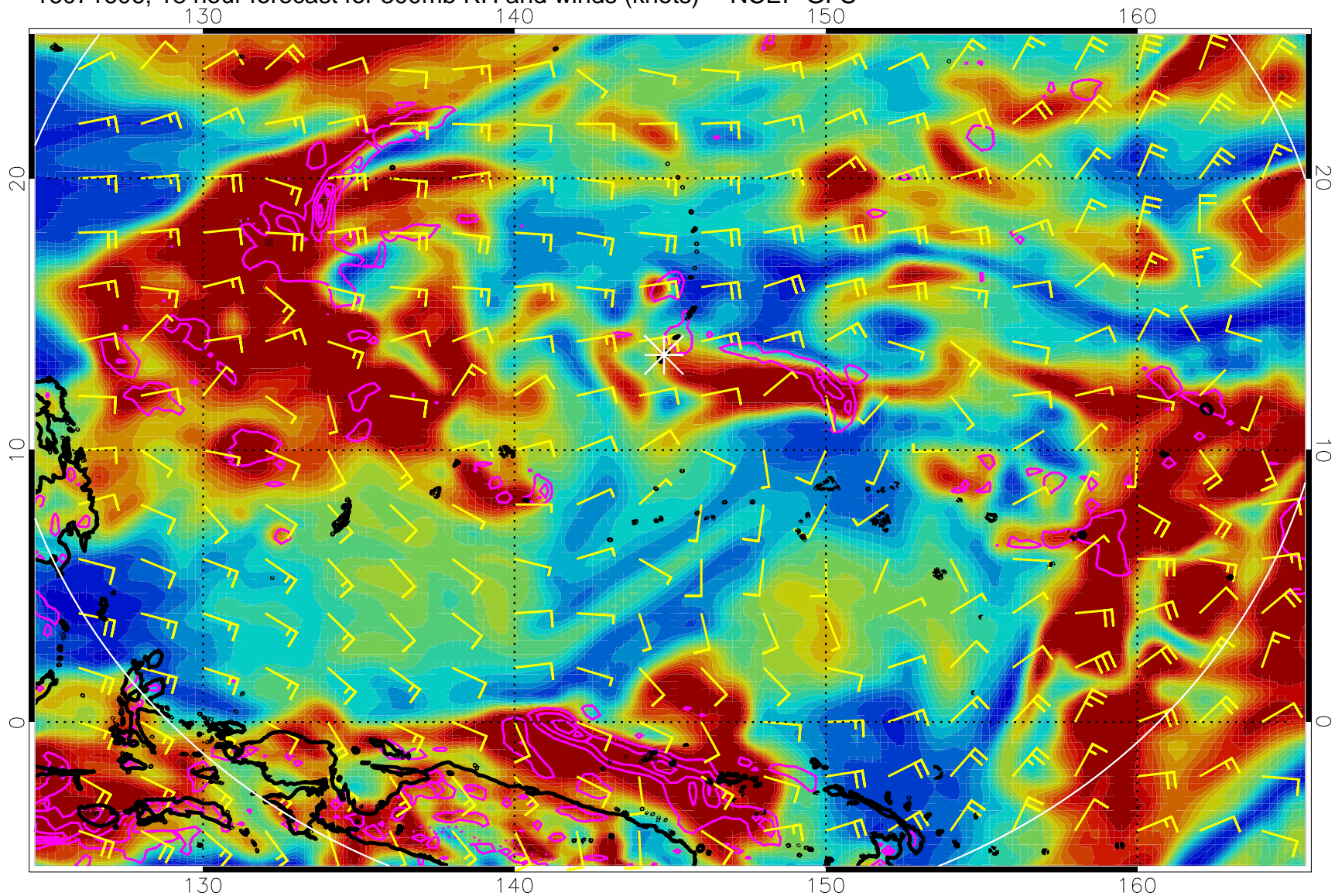
16071606, 18 hour forecast for 300mb RH and winds (knots) -- NCEP GFS
