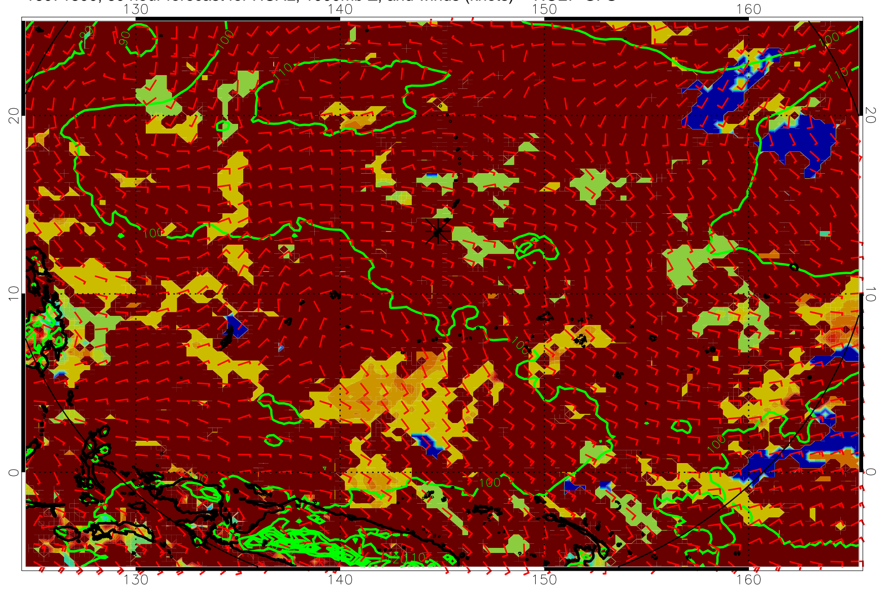
16071800, 60 hour forecast for HCAL, 1000mb Z, and winds (knots) -- NCEP GFS
