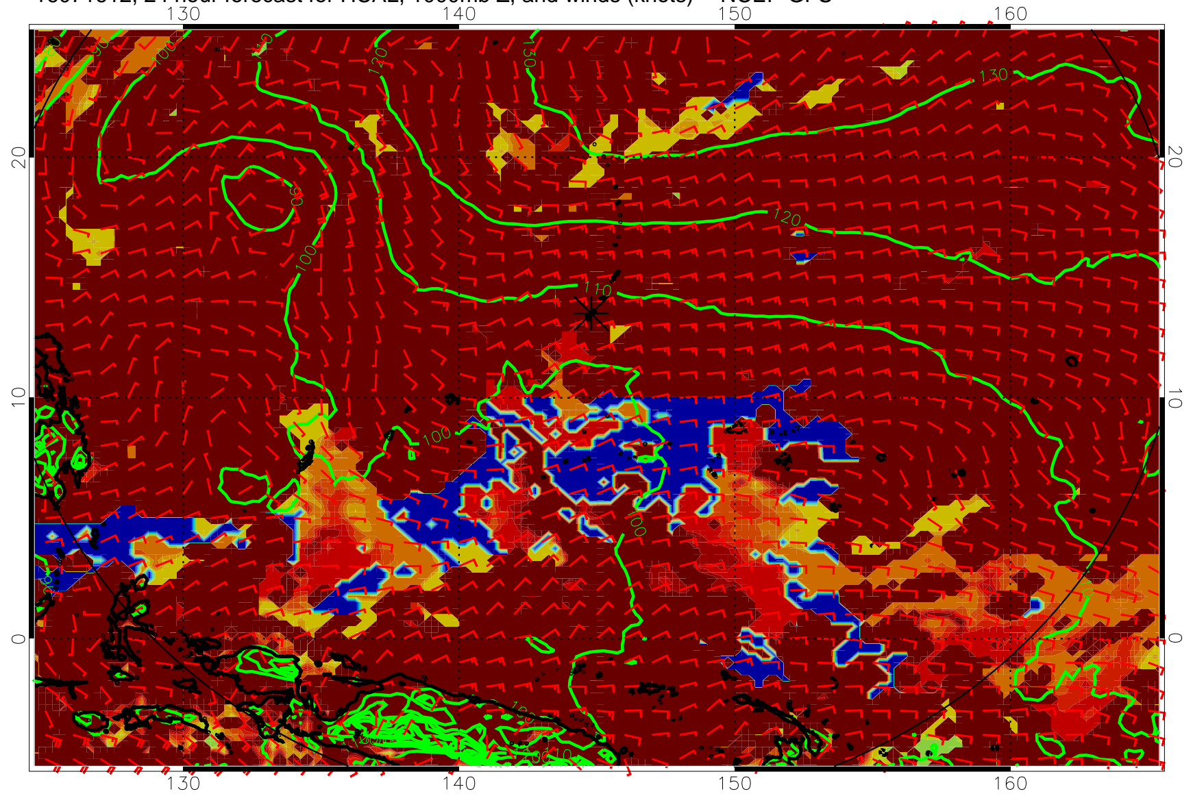
16071612, 24 hour forecast for HCAL, 1000mb Z, and winds (knots) -- NCEP GFS
