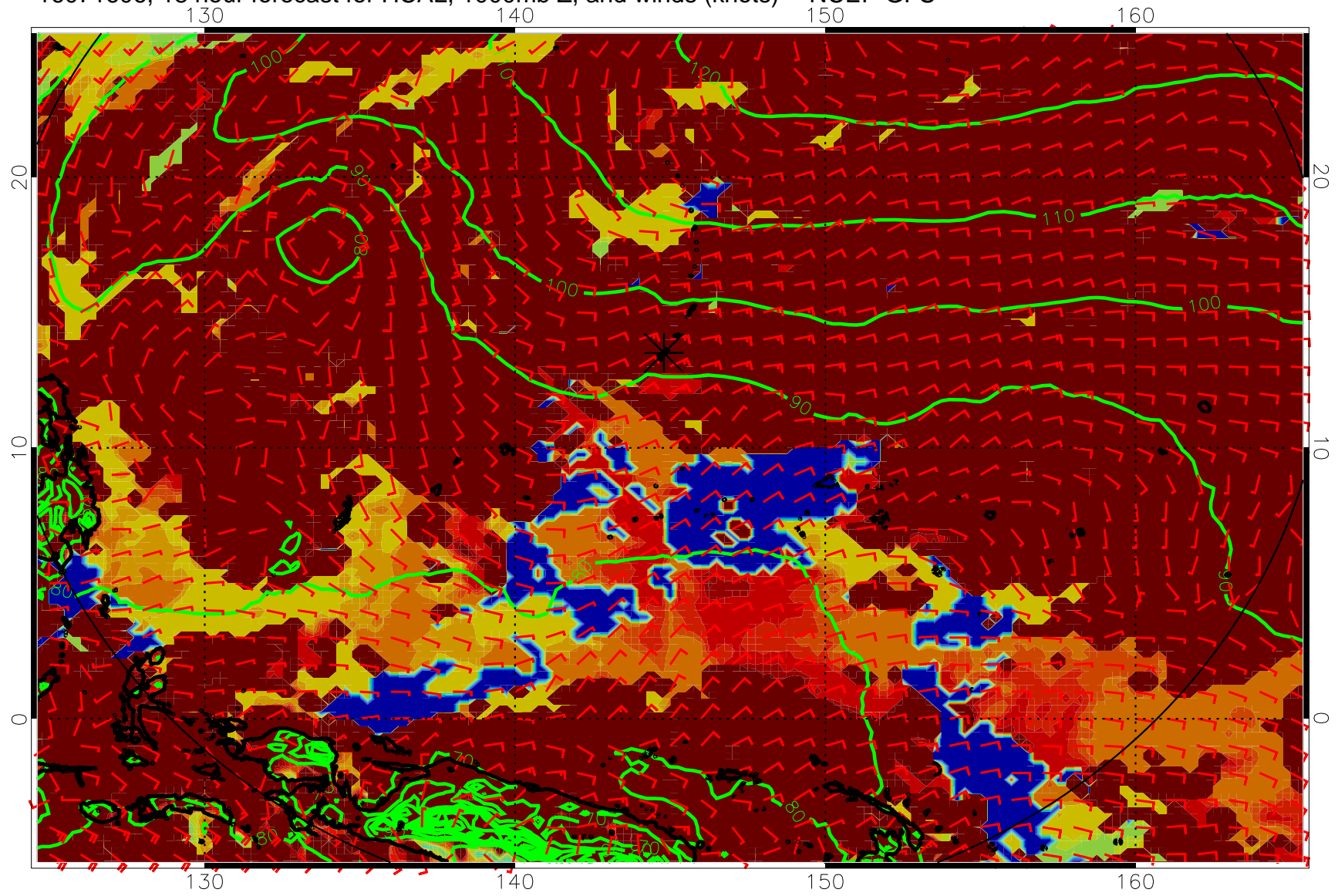
16071606, 18 hour forecast for HCAL, 1000mb Z, and winds (knots) -- NCEP GFS
