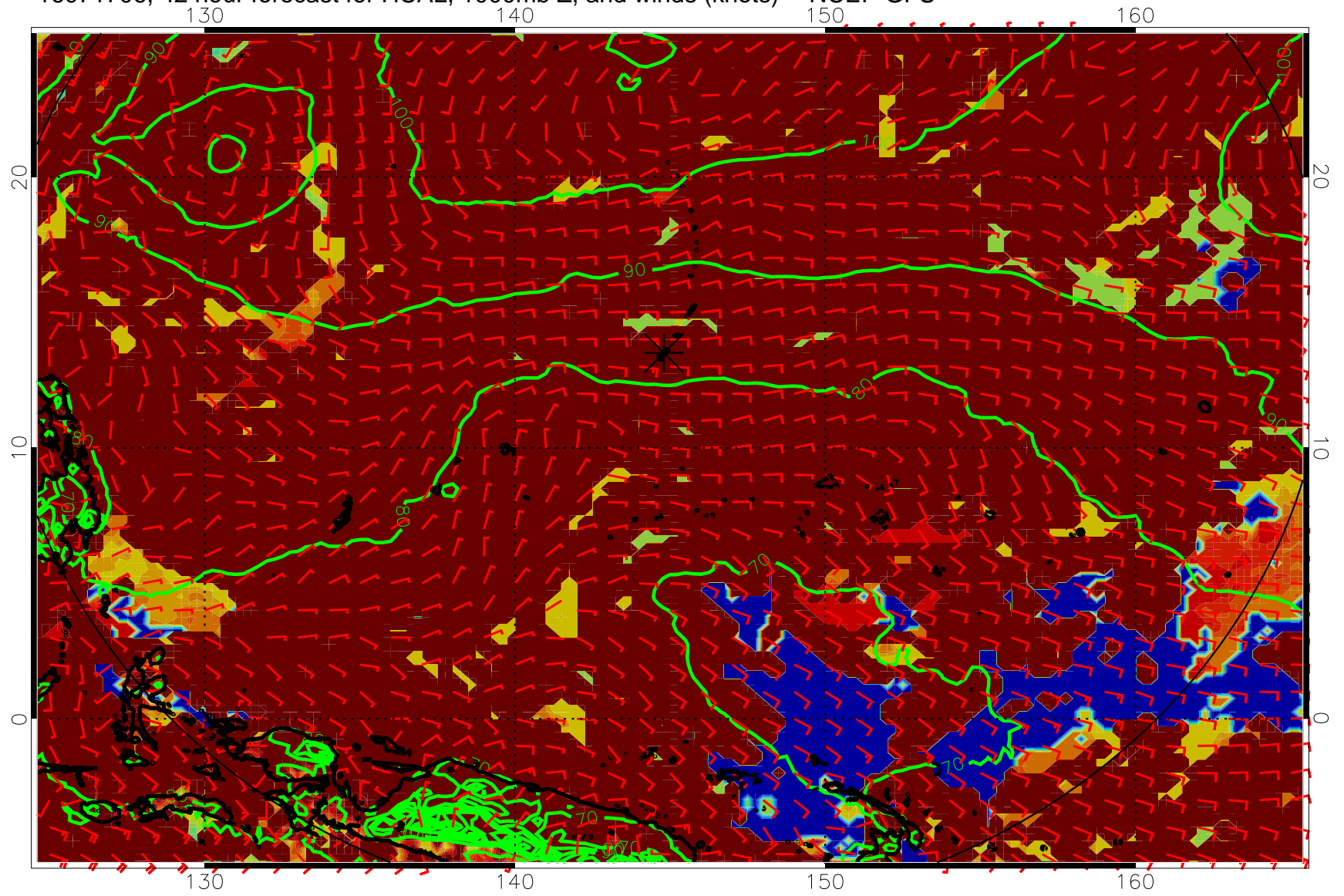
16071706, 42 hour forecast for HCAL, 1000mb Z, and winds (knots) -- NCEP GFS
