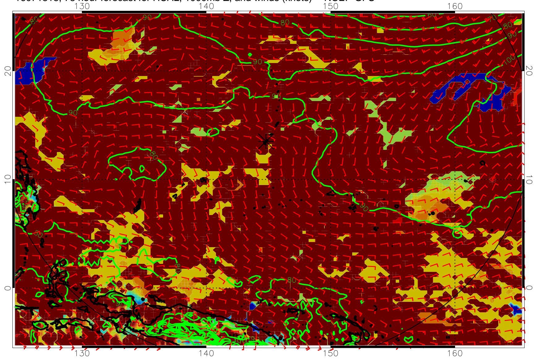
16071818, 78 hour forecast for HCAL, 1000mb Z, and winds (knots) -- NCEP GFS
