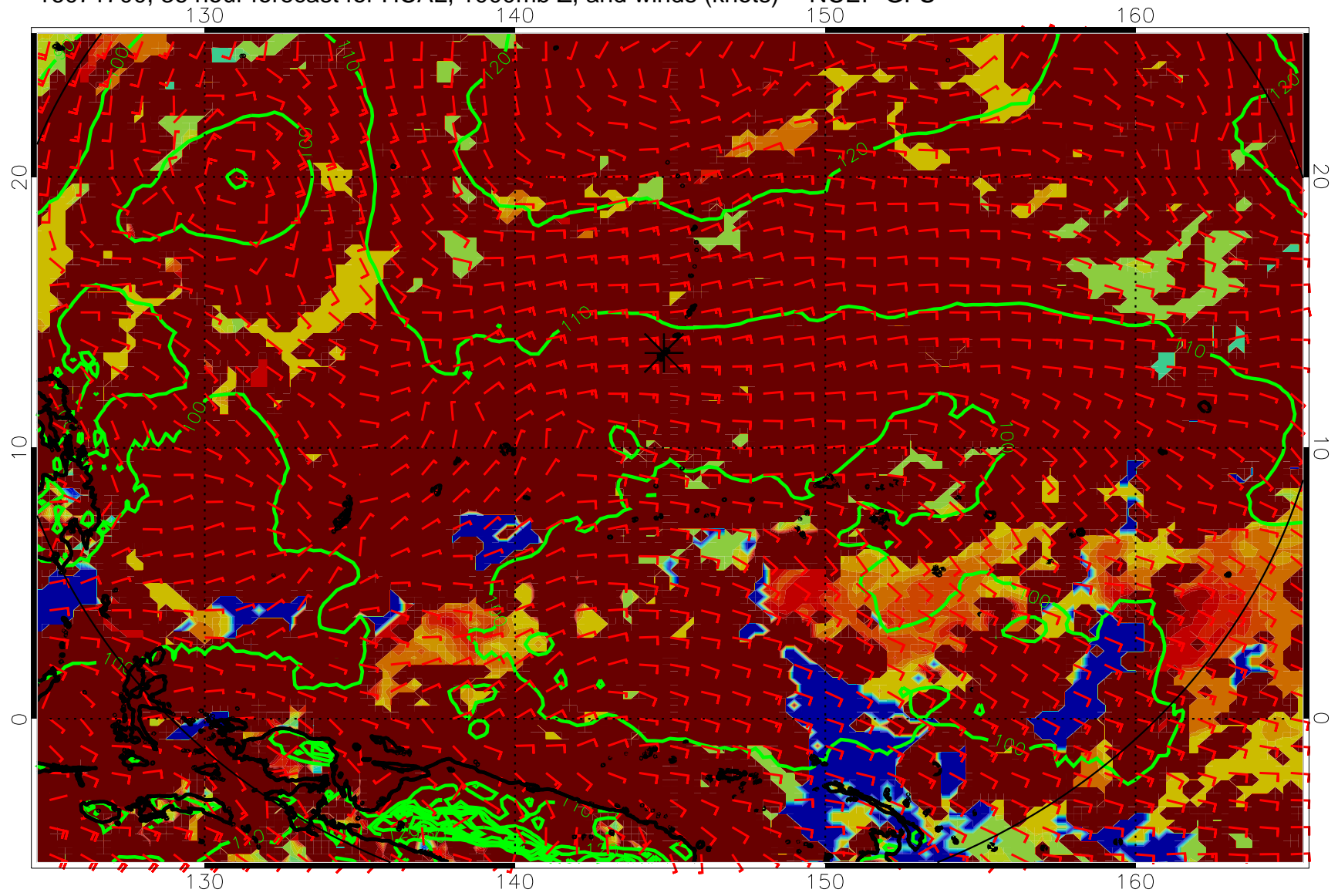
16071700, 36 hour forecast for HCAL, 1000mb Z, and winds (knots) -- NCEP GFS
