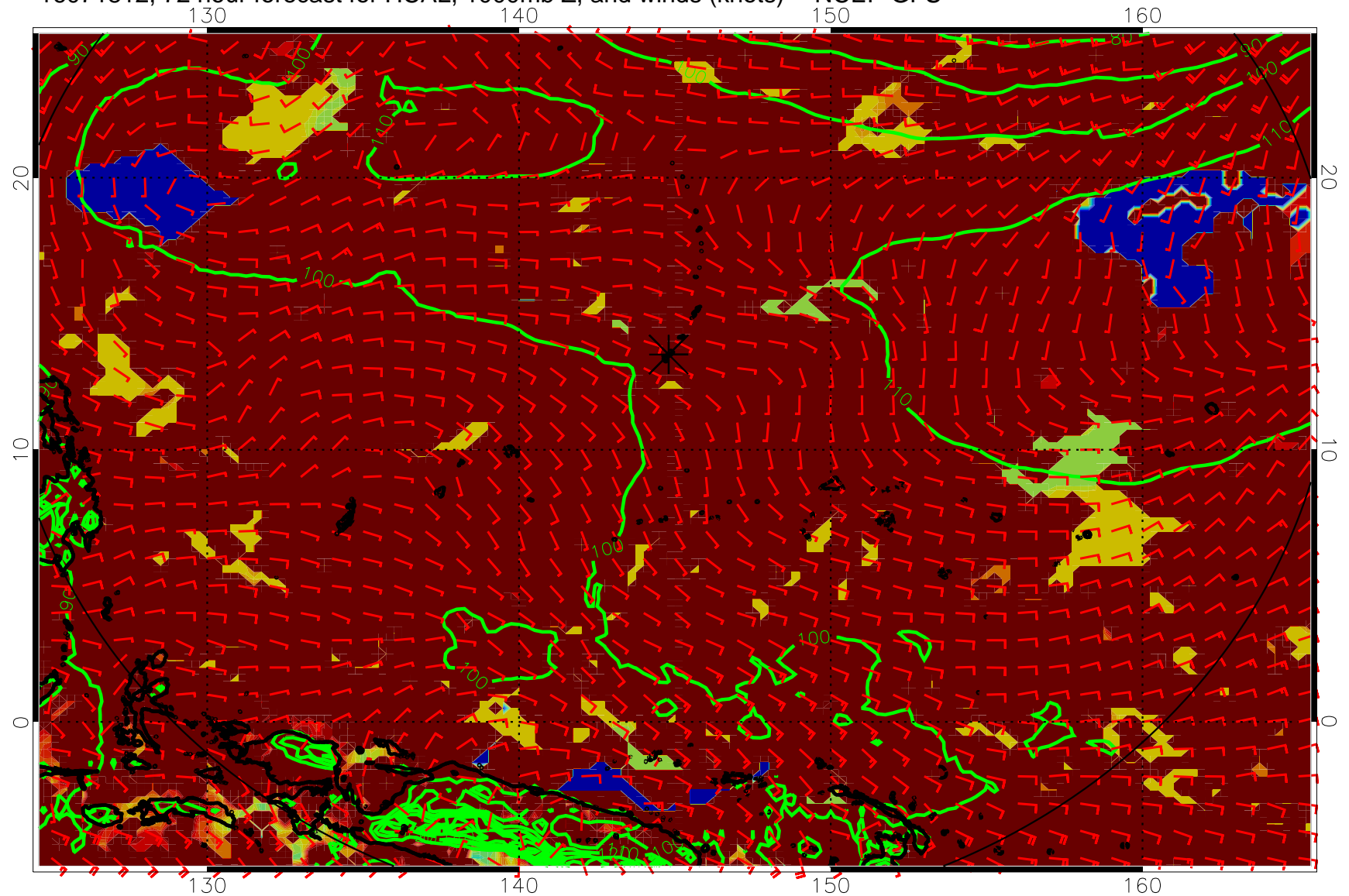
16071812, 72 hour forecast for HCAL, 1000mb Z, and winds (knots) -- NCEP GFS
