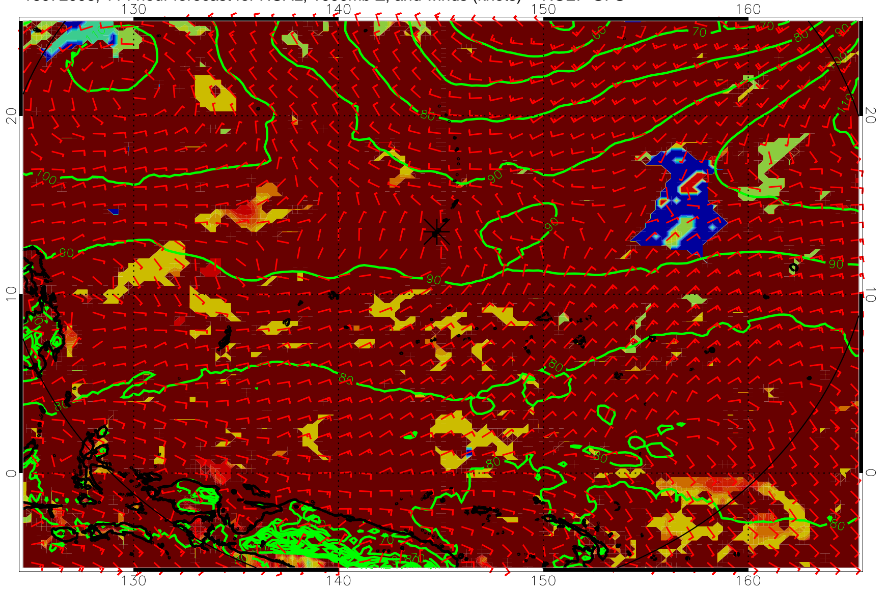
16072006, 114 hour forecast for HCAL, 1000mb Z, and winds (knots) -- NCEP GFS
