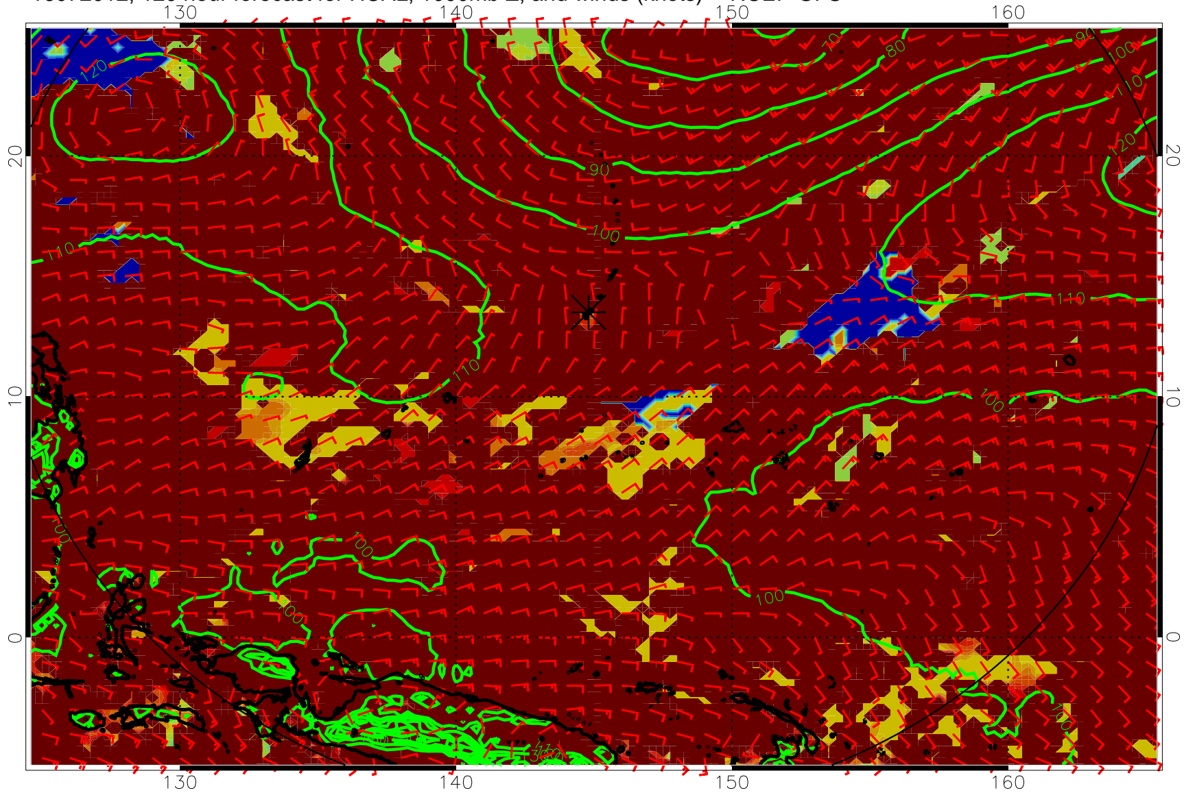
16072012, 120 hour forecast for HCAL, 1000mb Z, and winds (knots) -- NCEP GFS
