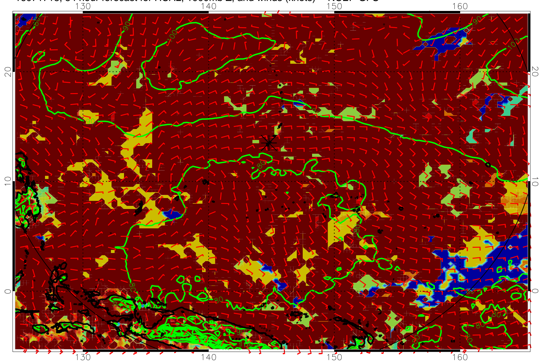
16071718, 54 hour forecast for HCAL, 1000mb Z, and winds (knots) -- NCEP GFS
