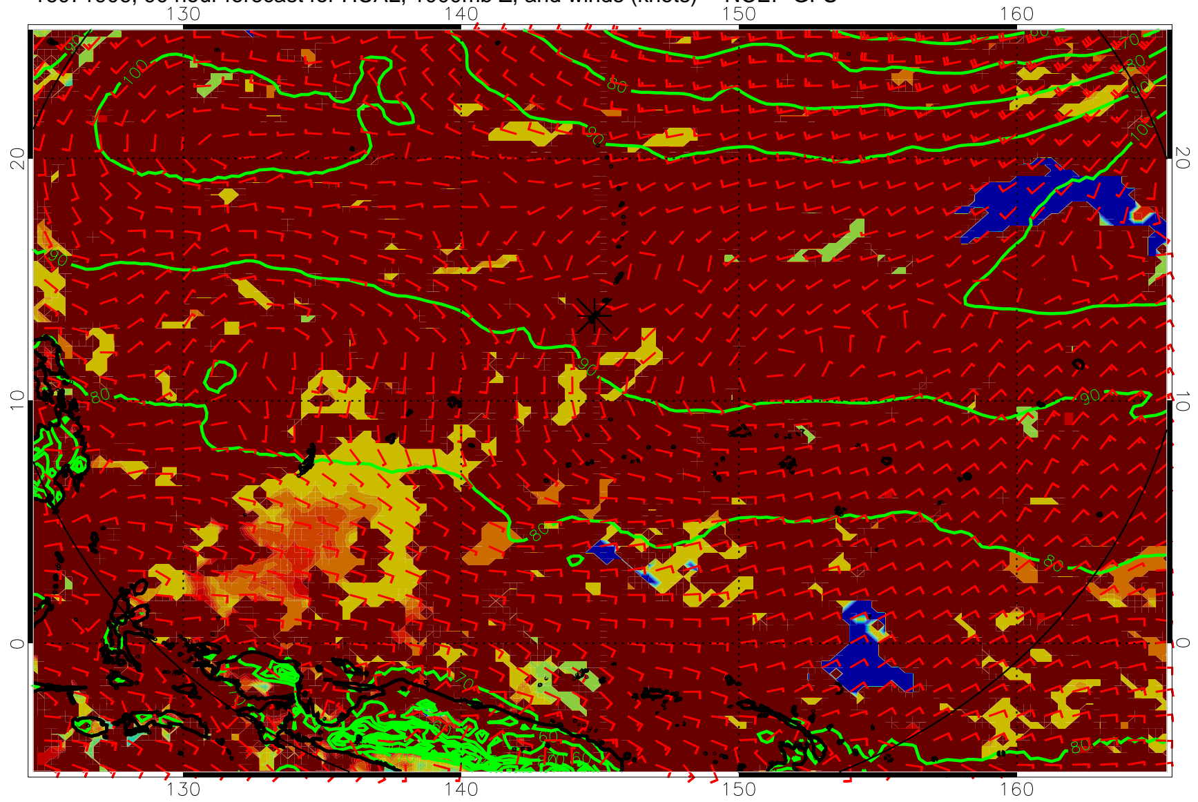
16071906, 90 hour forecast for HCAL, 1000mb Z, and winds (knots) -- NCEP GFS
