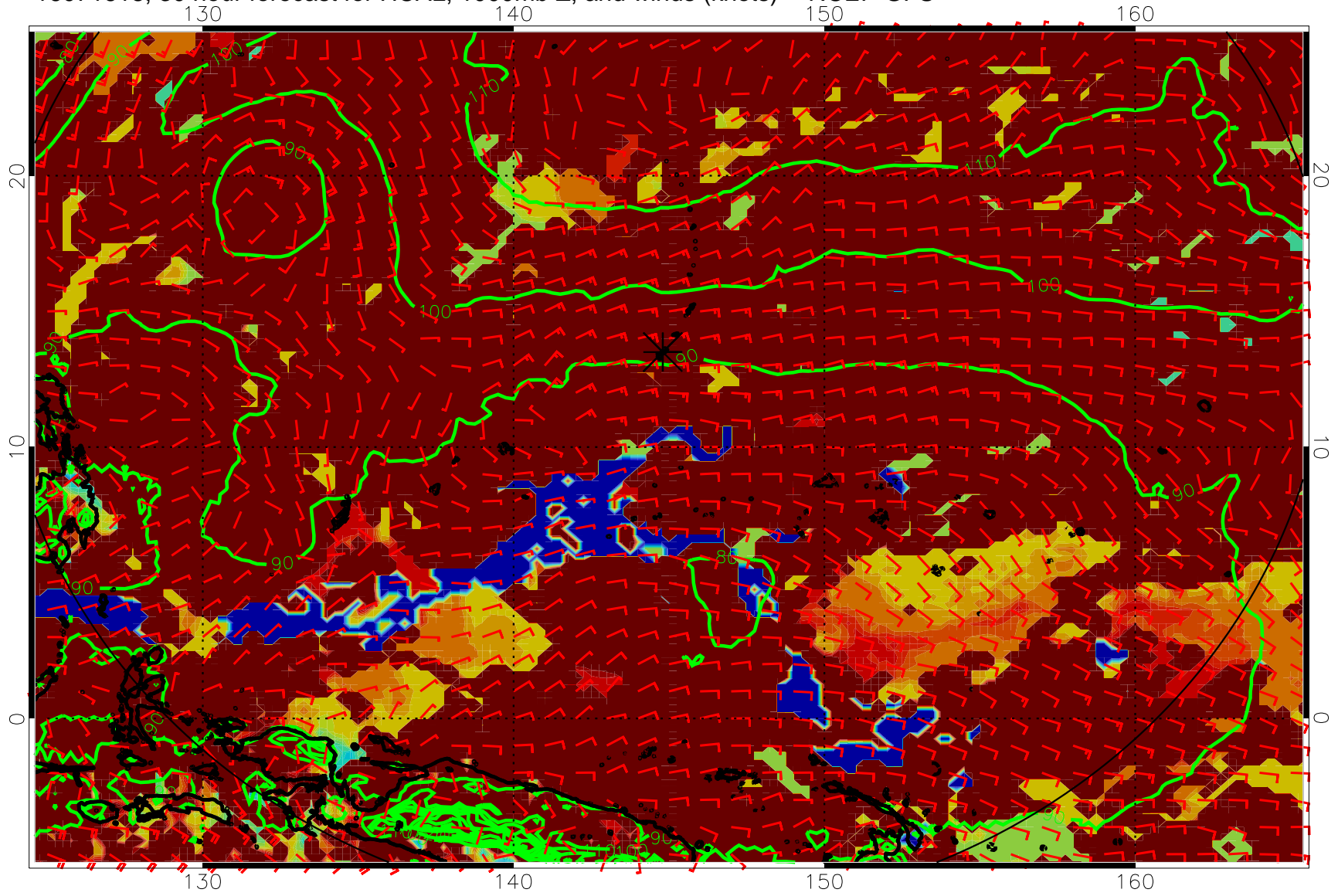
16071618, 30 hour forecast for HCAL, 1000mb Z, and winds (knots) -- NCEP GFS
