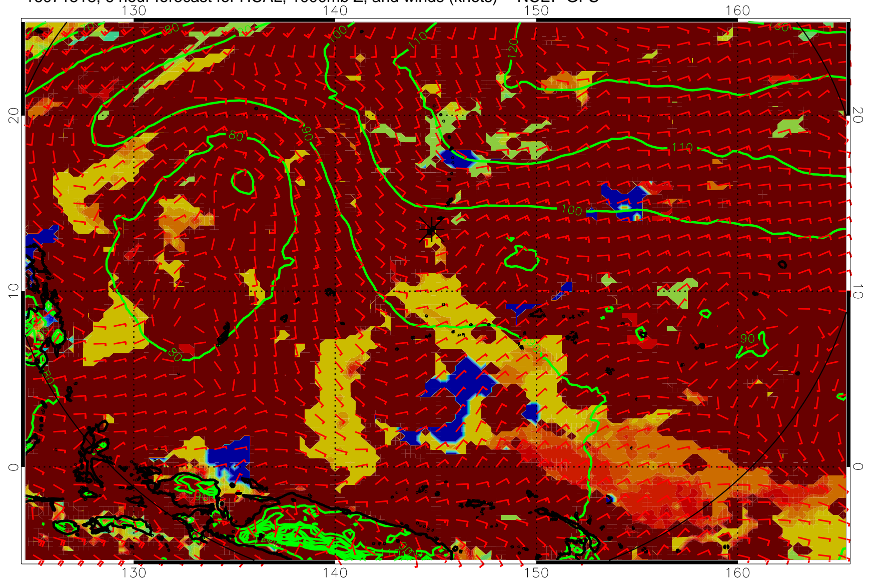
16071518, 6 hour forecast for HCAL, 1000mb Z, and winds (knots) -- NCEP GFS
