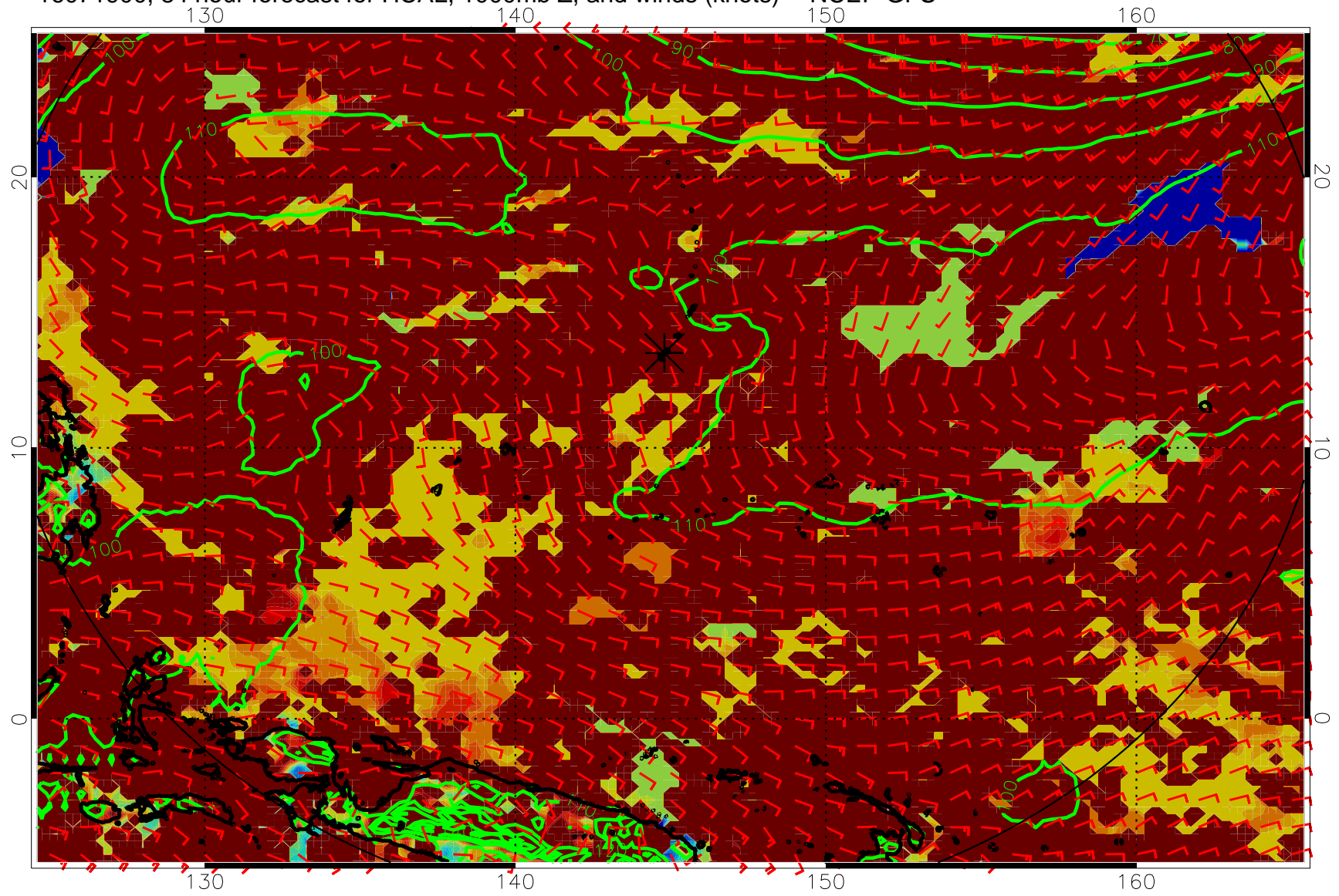
16071900, 84 hour forecast for HCAL, 1000mb Z, and winds (knots) -- NCEP GFS
