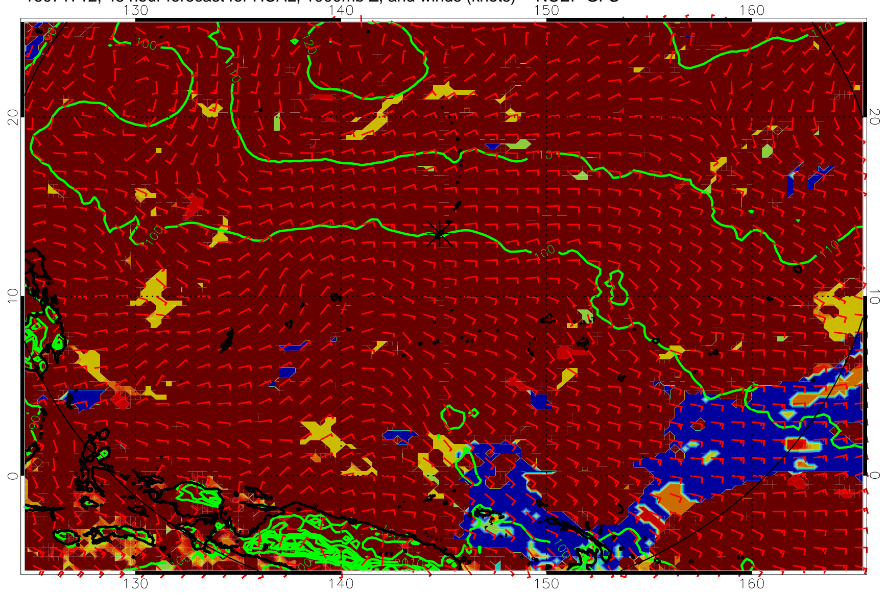
16071712, 48 hour forecast for HCAL, 1000mb Z, and winds (knots) -- NCEP GFS
