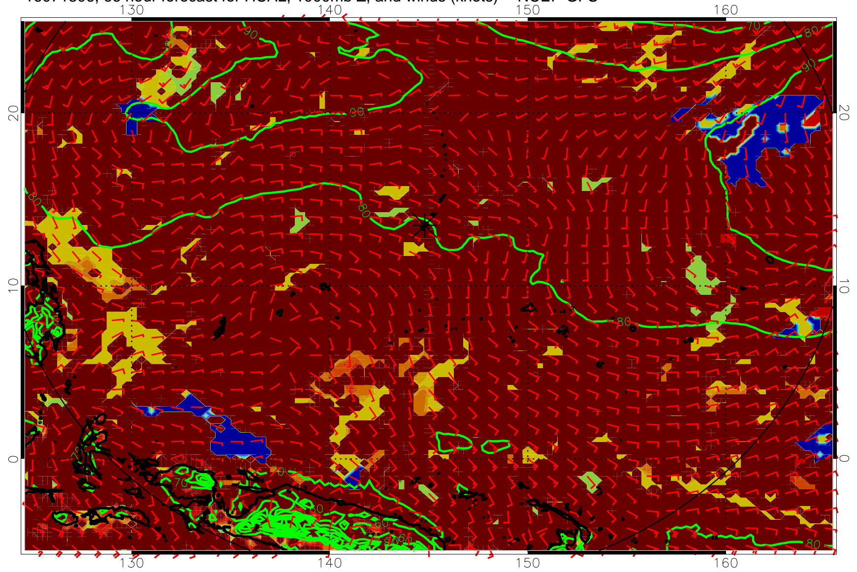
16071806, 66 hour forecast for HCAL, 1000mb Z, and winds (knots) -- NCEP GFS
