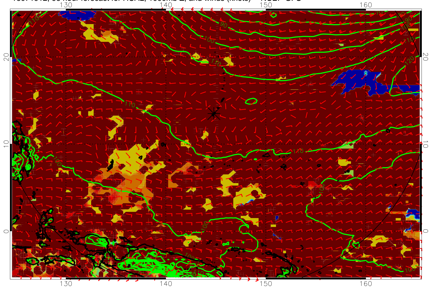
16071912, 96 hour forecast for HCAL, 1000mb Z, and winds (knots) -- NCEP GFS
