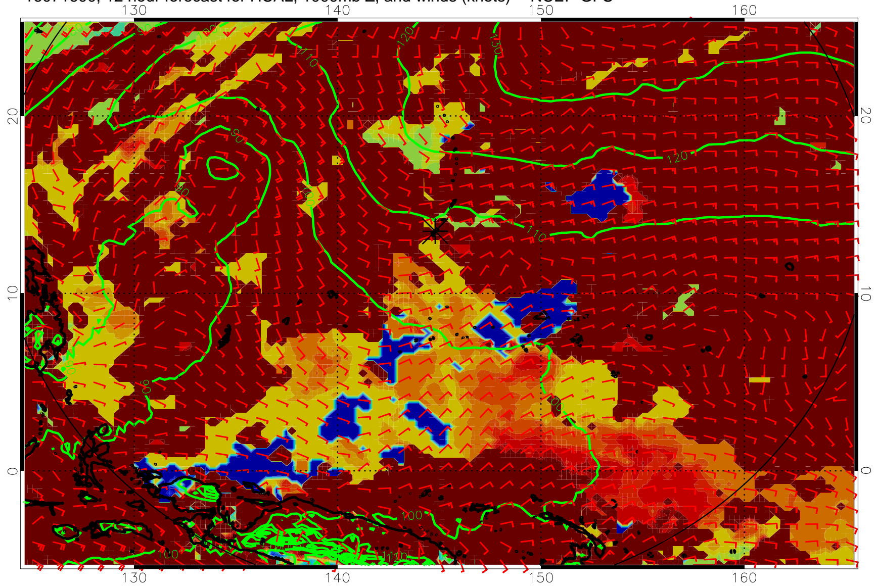
16071600, 12 hour forecast for HCAL, 1000mb Z, and winds (knots) -- NCEP GFS
