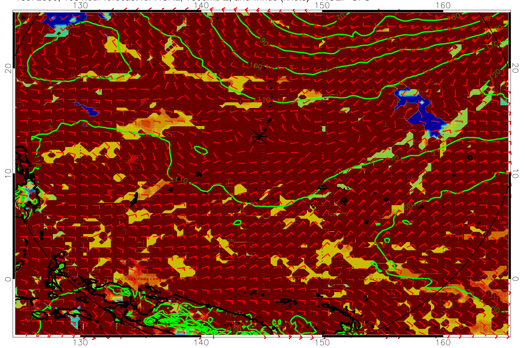
16072000, 108 hour forecast for HCAL, 1000mb Z, and winds (knots) -- NCEP GFS
