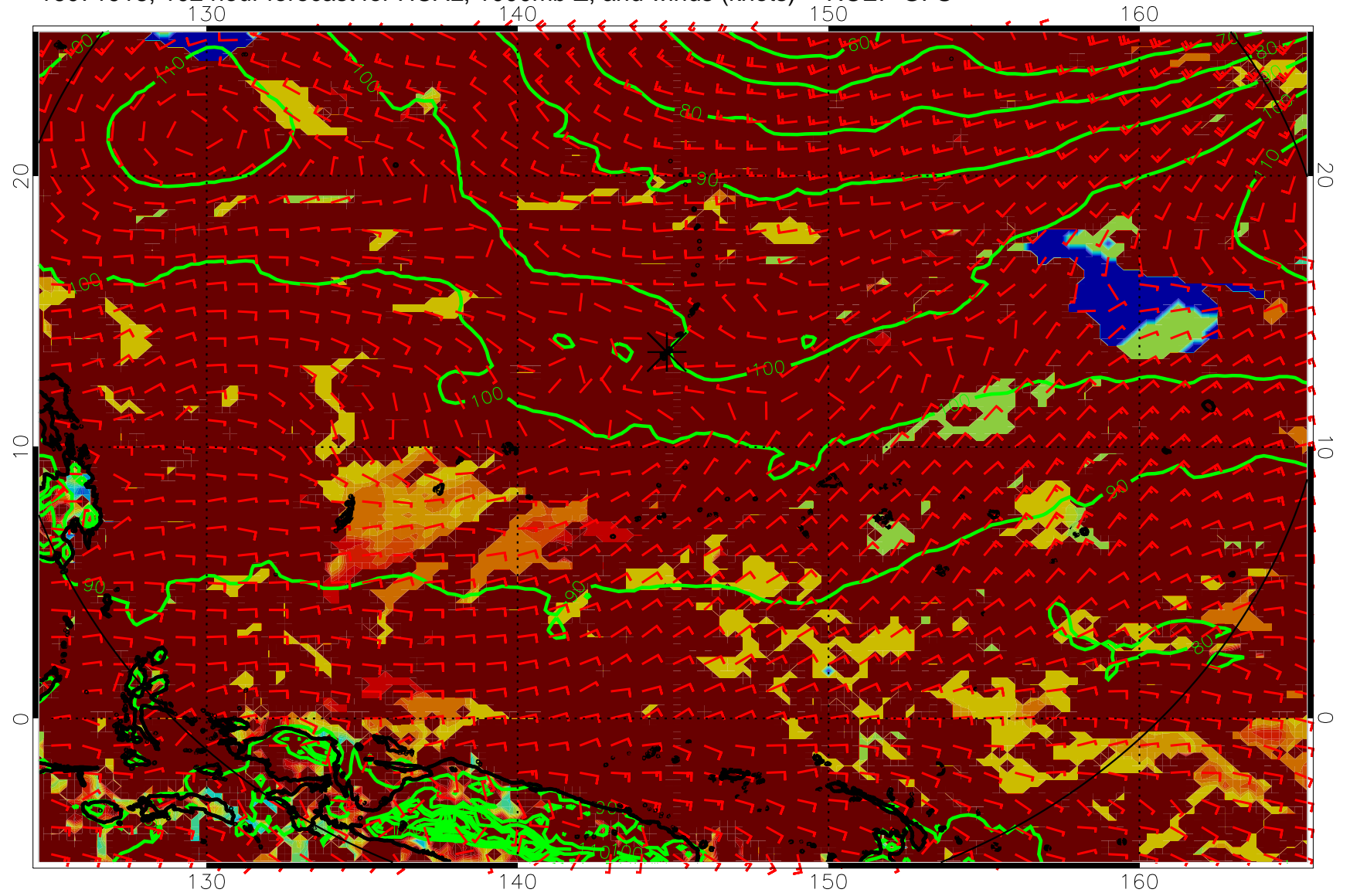
16071918, 102 hour forecast for HCAL, 1000mb Z, and winds (knots) -- NCEP GFS
