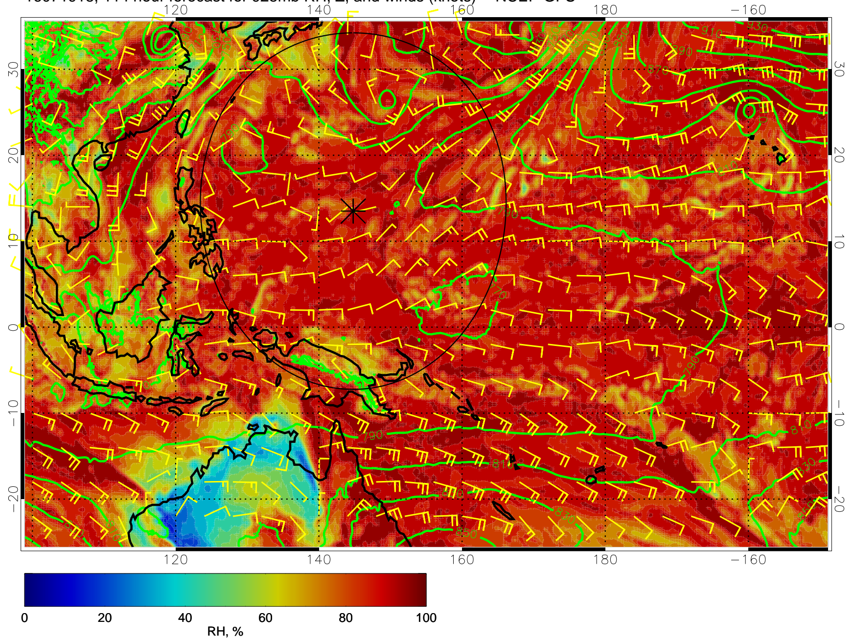
16071918, 114 hour forecast for 925mb RH, Z, and winds (knots) -- NCEP GFS
