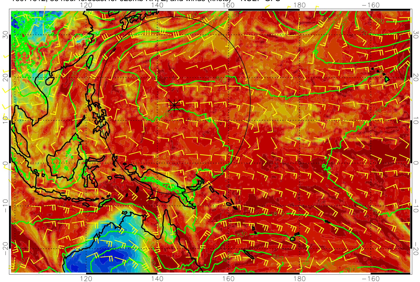
16071612, 36 hour forecast for 925mb RH, Z, and winds (knots) -- NCEP GFS
