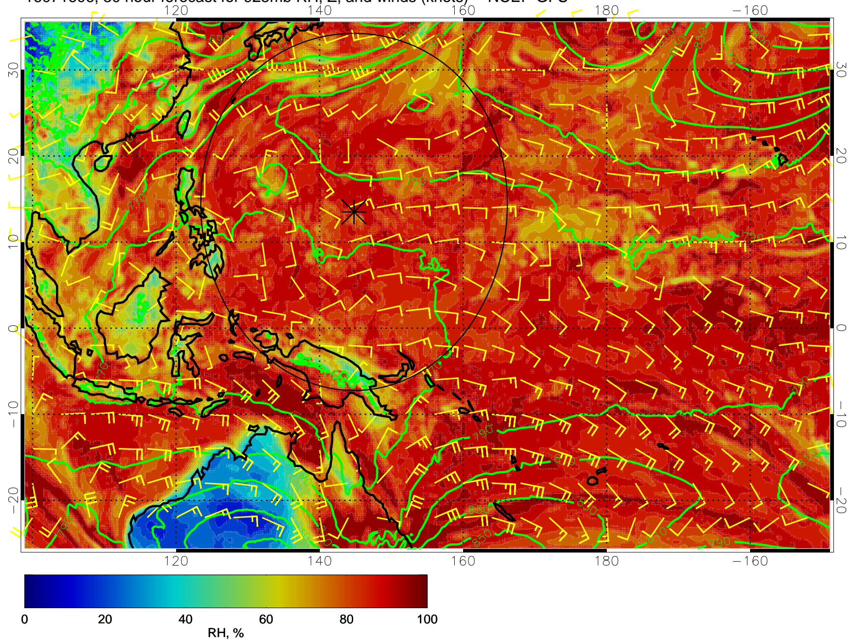
16071606, 30 hour forecast for 925mb RH, Z, and winds (knots) -- NCEP GFS
