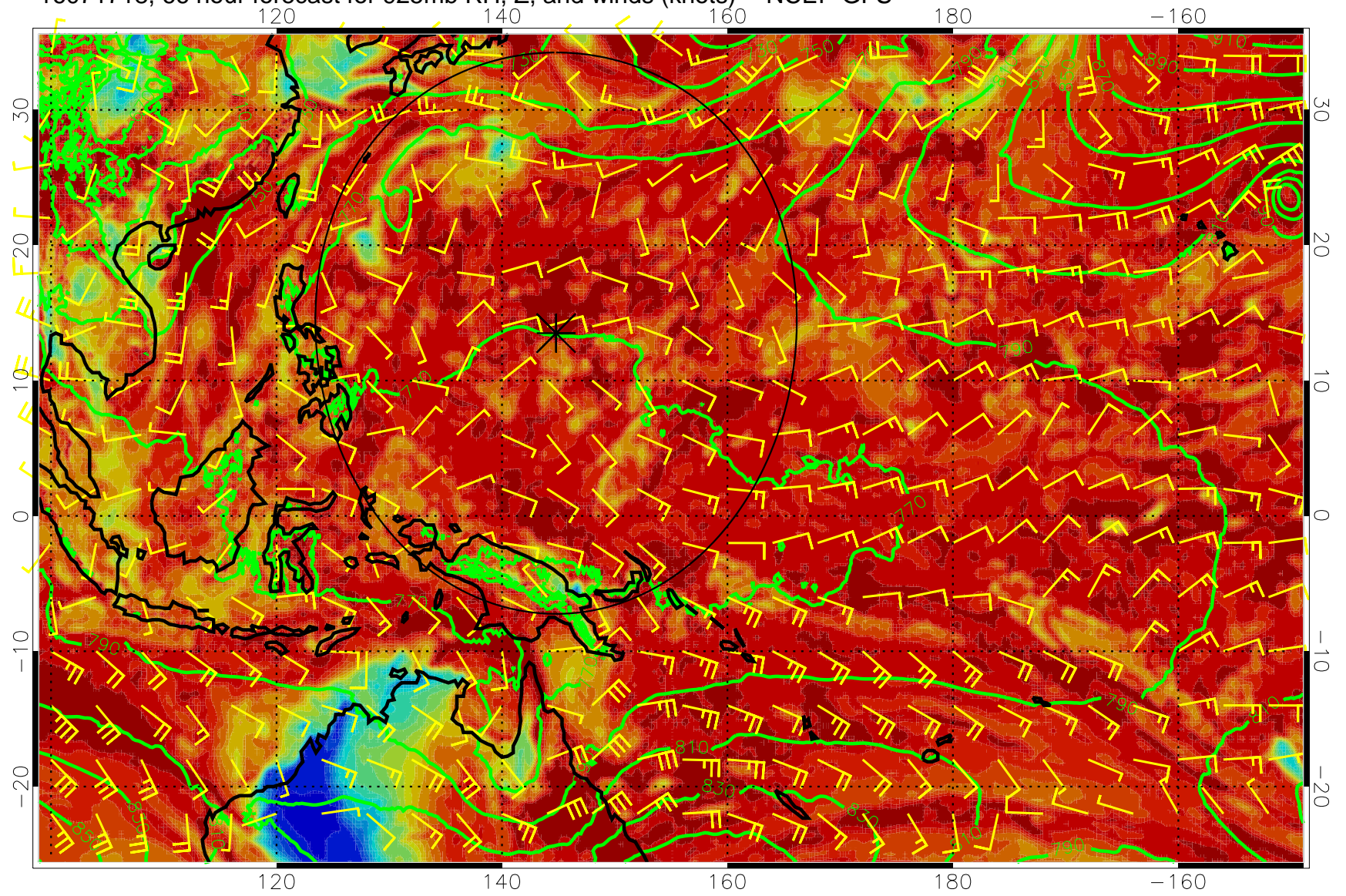
16071718, 66 hour forecast for 925mb RH, Z, and winds (knots) -- NCEP GFS
