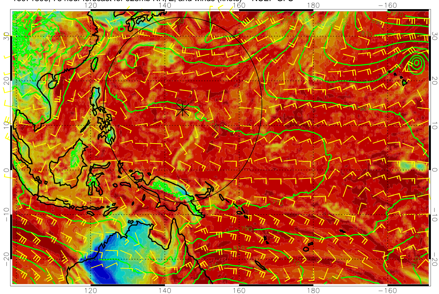
16071806, 78 hour forecast for 925mb RH, Z, and winds (knots) -- NCEP GFS
