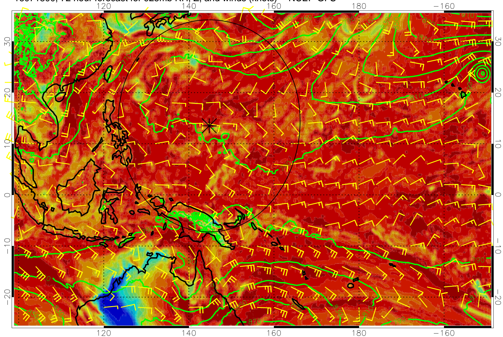
16071800, 72 hour forecast for 925mb RH, Z, and winds (knots) -- NCEP GFS
