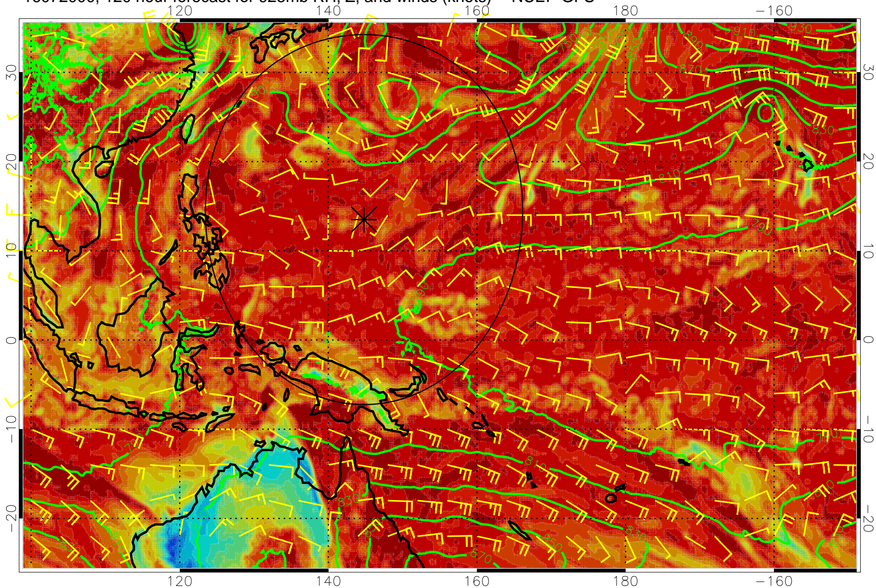
16072000, 120 hour forecast for 925mb RH, Z, and winds (knots) -- NCEP GFS
