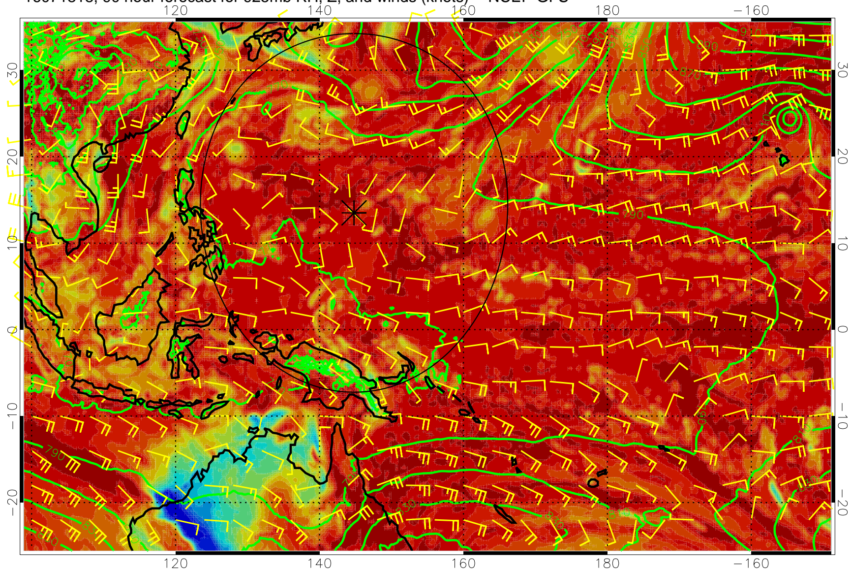
16071818, 90 hour forecast for 925mb RH, Z, and winds (knots) -- NCEP GFS
