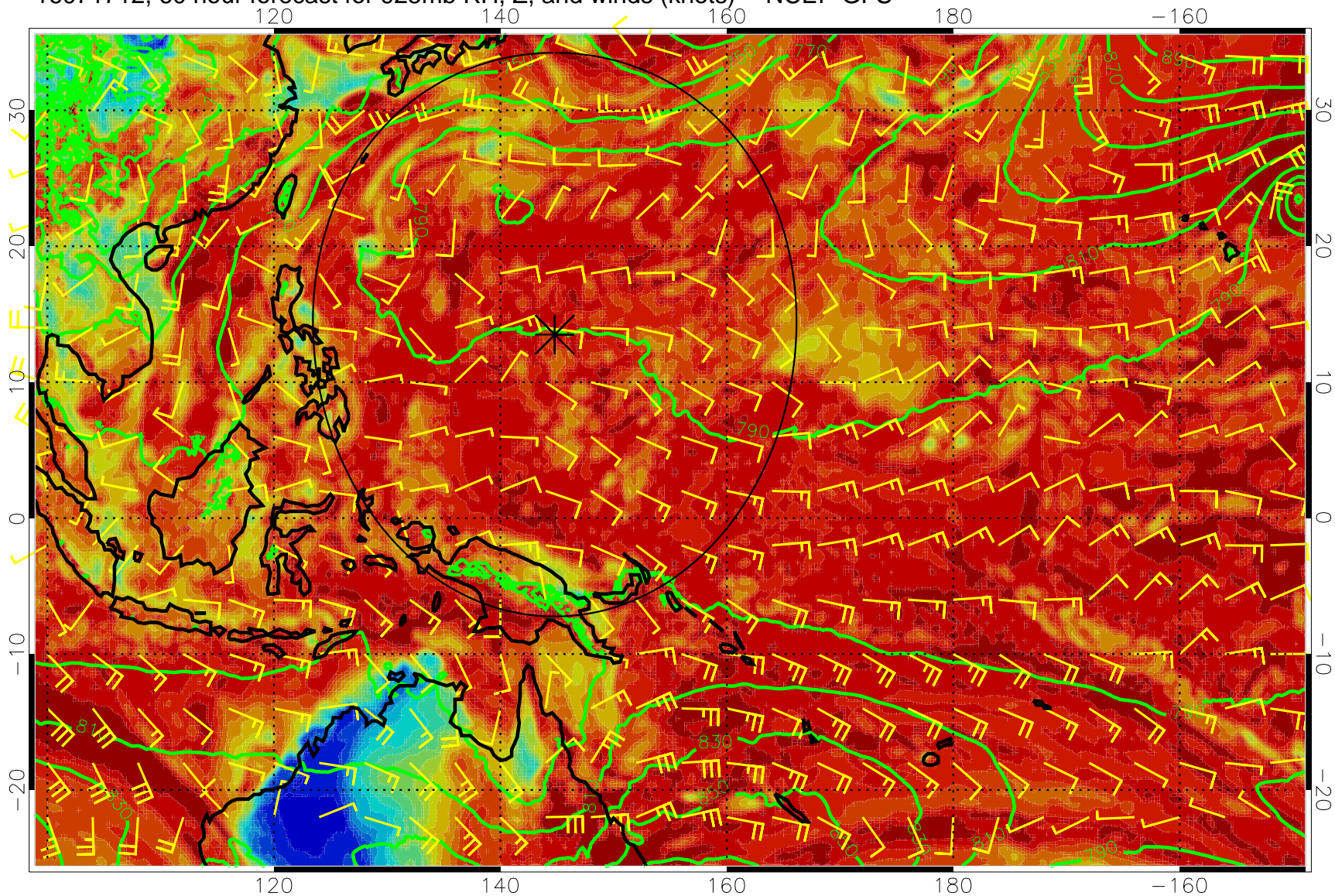
16071712, 60 hour forecast for 925mb RH, Z, and winds (knots) -- NCEP GFS
