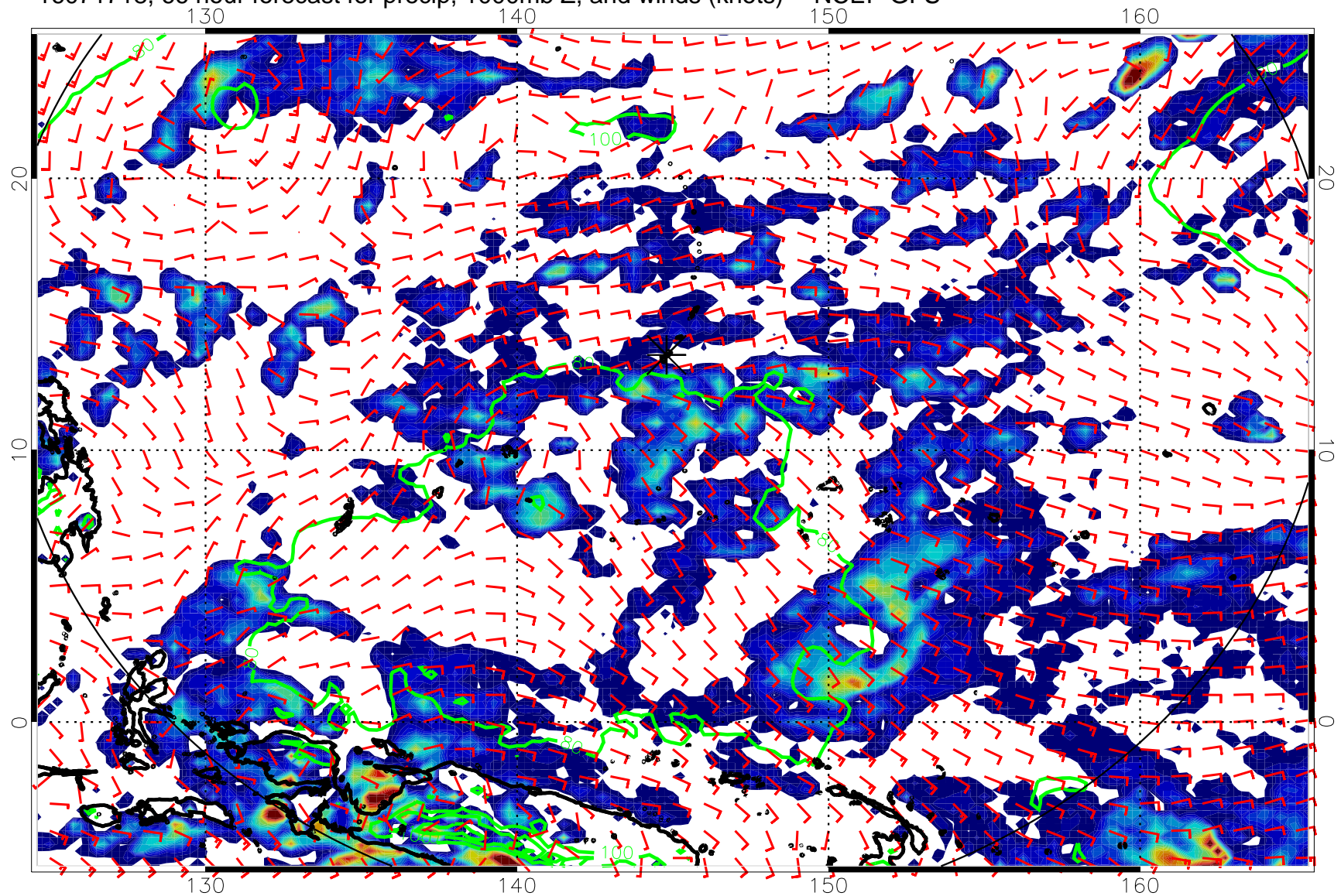
16071718, 66 hour forecast for precip, 1000mb Z, and winds (knots) -- NCEP GFS
