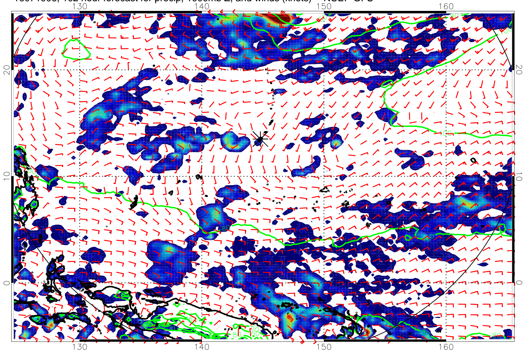
16071906, 102 hour forecast for precip, 1000mb Z, and winds (knots) -- NCEP GFS
