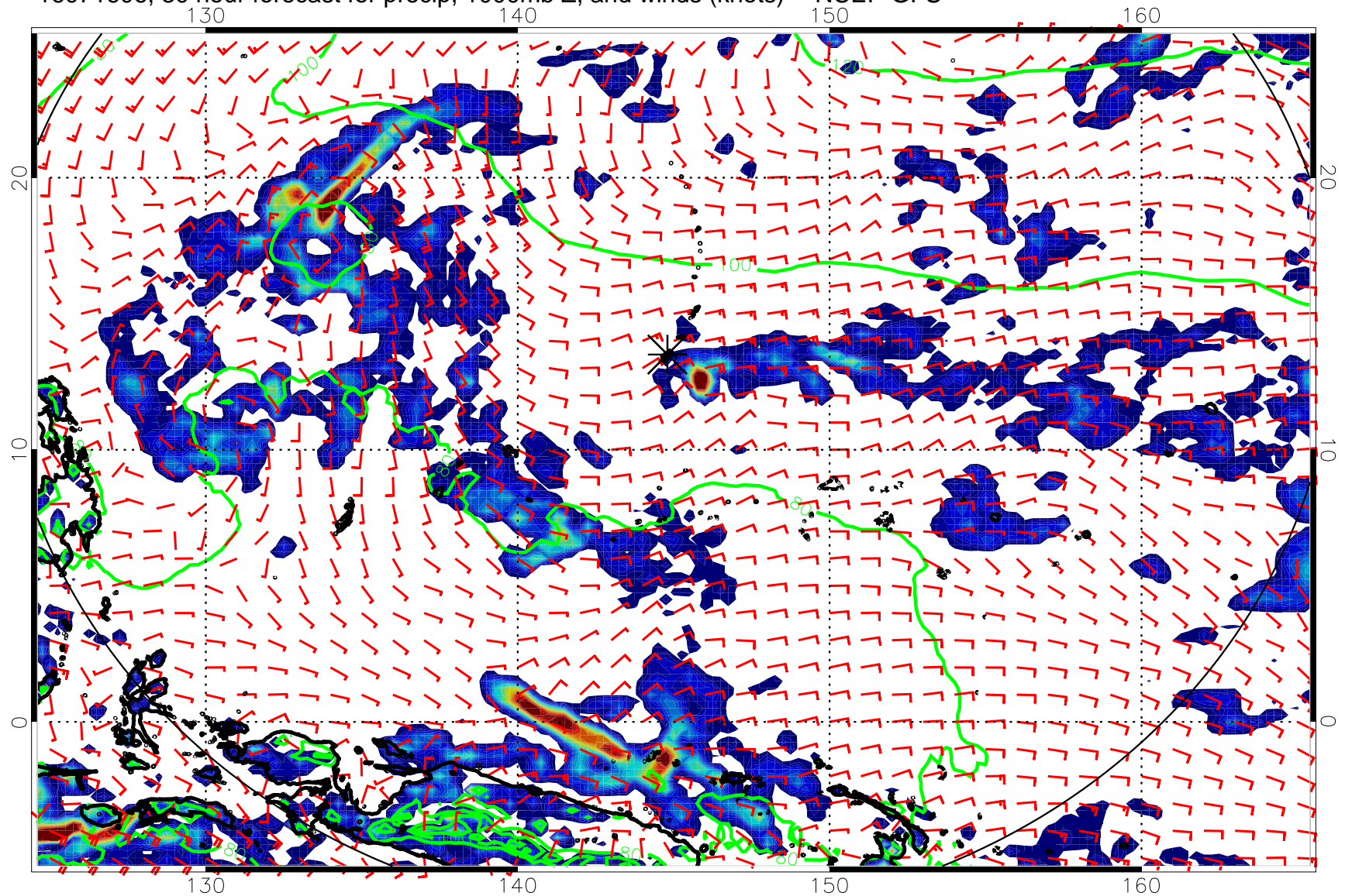
16071606, 30 hour forecast for precip, 1000mb Z, and winds (knots) -- NCEP GFS
