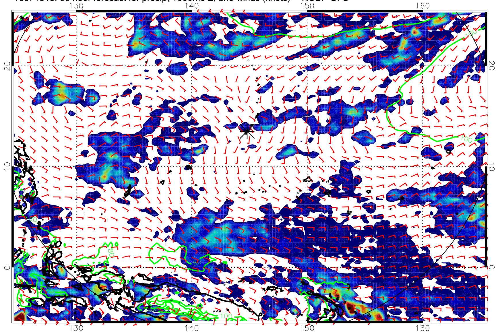
16071818, 90 hour forecast for precip, 1000mb Z, and winds (knots) -- NCEP GFS
