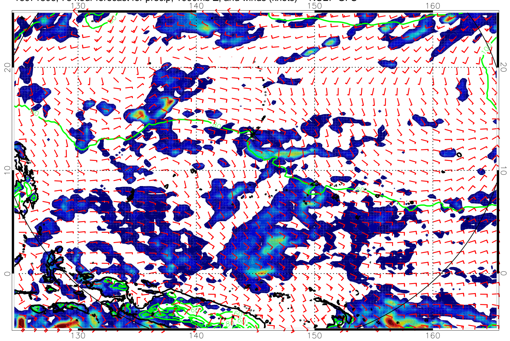
16071806, 78 hour forecast for precip, 1000mb Z, and winds (knots) -- NCEP GFS
