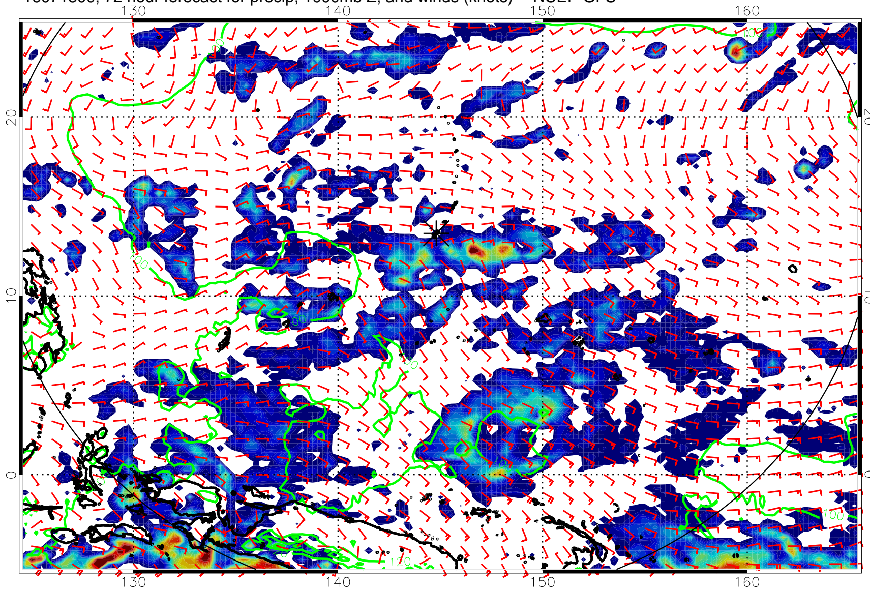
16071800, 72 hour forecast for precip, 1000mb Z, and winds (knots) -- NCEP GFS
