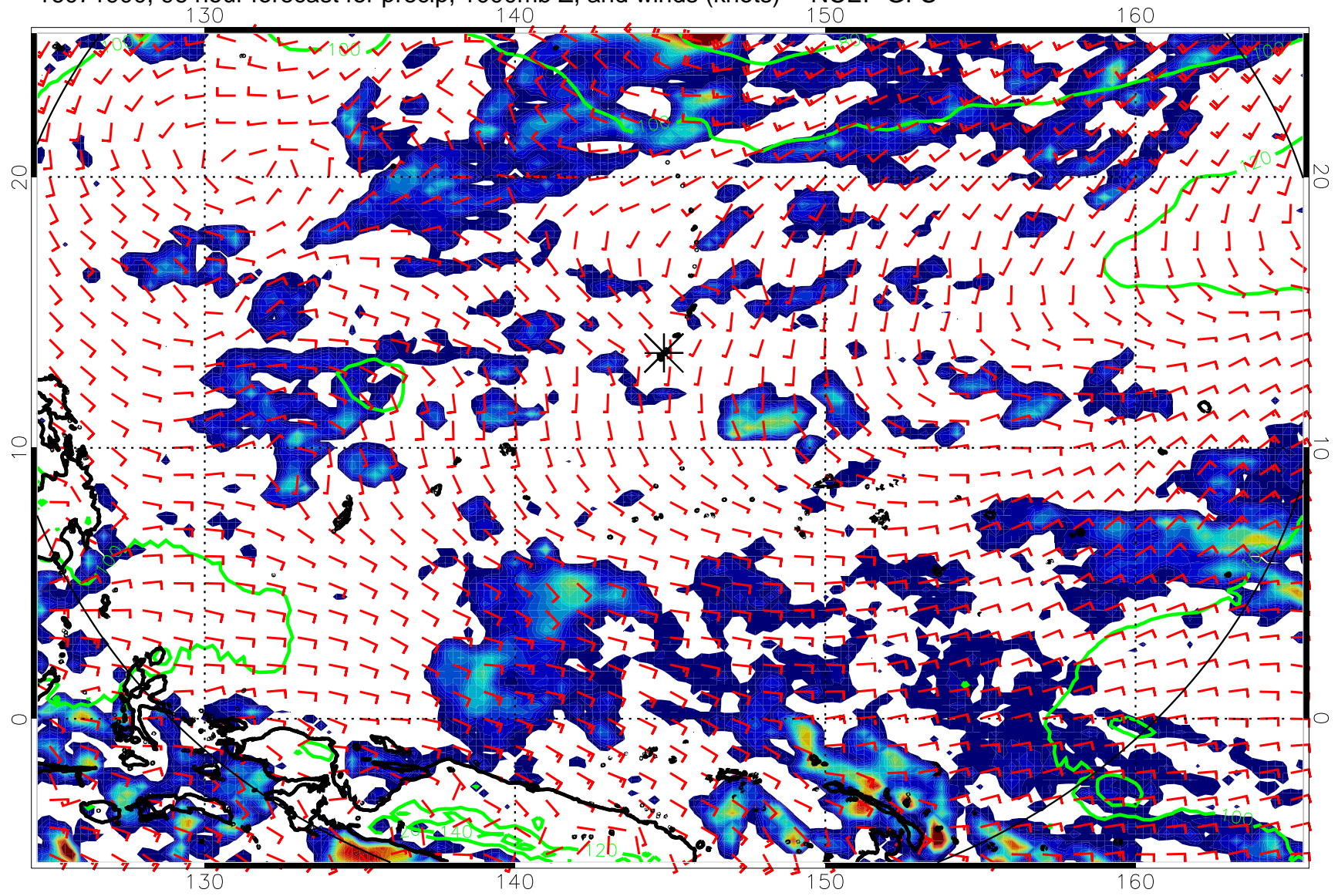
16071900, 96 hour forecast for precip, 1000mb Z, and winds (knots) -- NCEP GFS
