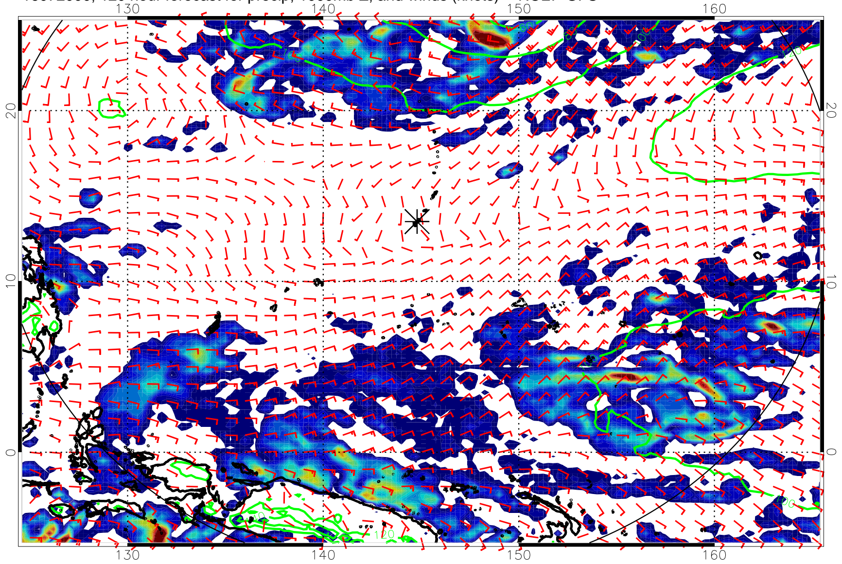
16072000, 120 hour forecast for precip, 1000mb Z, and winds (knots) -- NCEP GFS
