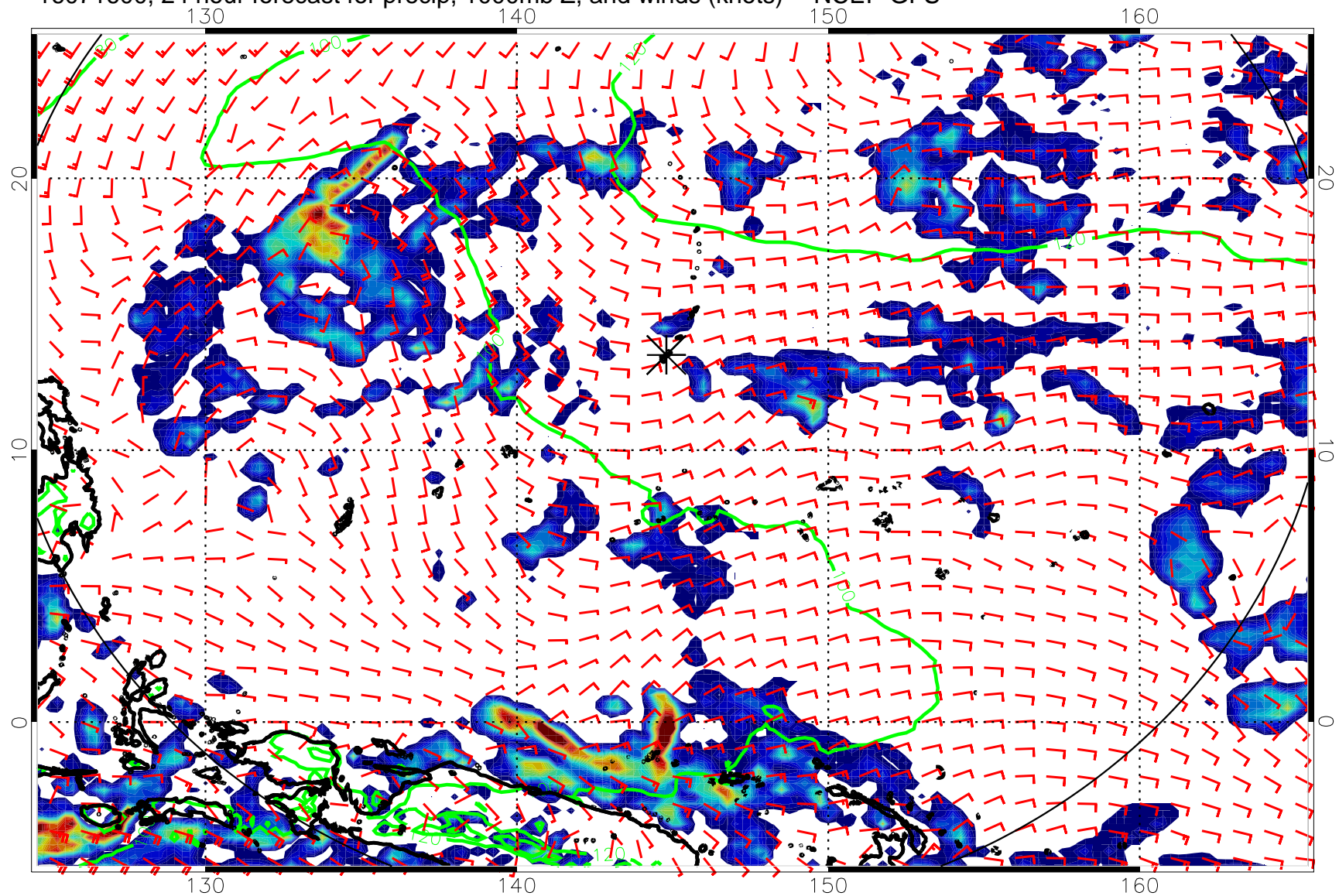
16071600, 24 hour forecast for precip, 1000mb Z, and winds (knots) -- NCEP GFS
