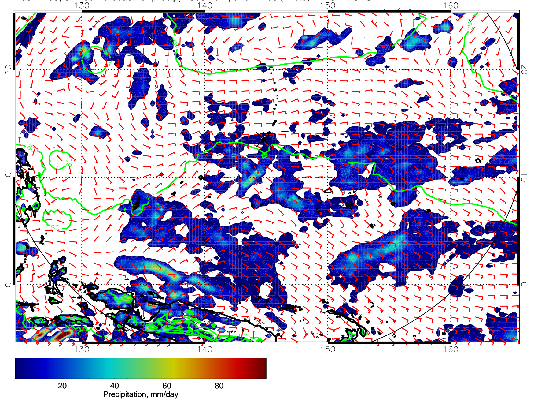
16071706, 54 hour forecast for precip, 1000mb Z, and winds (knots) -- NCEP GFS
