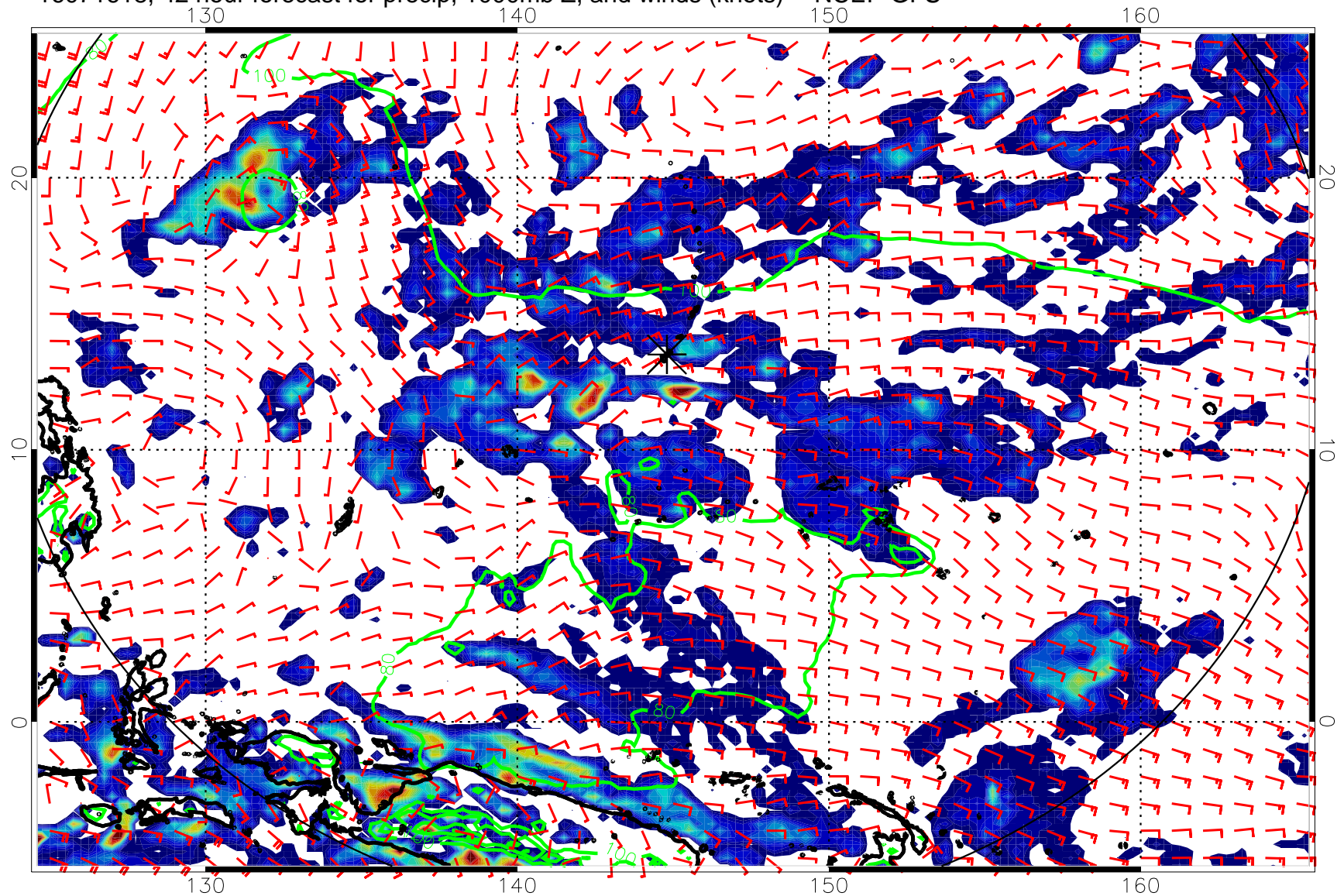
16071618, 42 hour forecast for precip, 1000mb Z, and winds (knots) -- NCEP GFS
