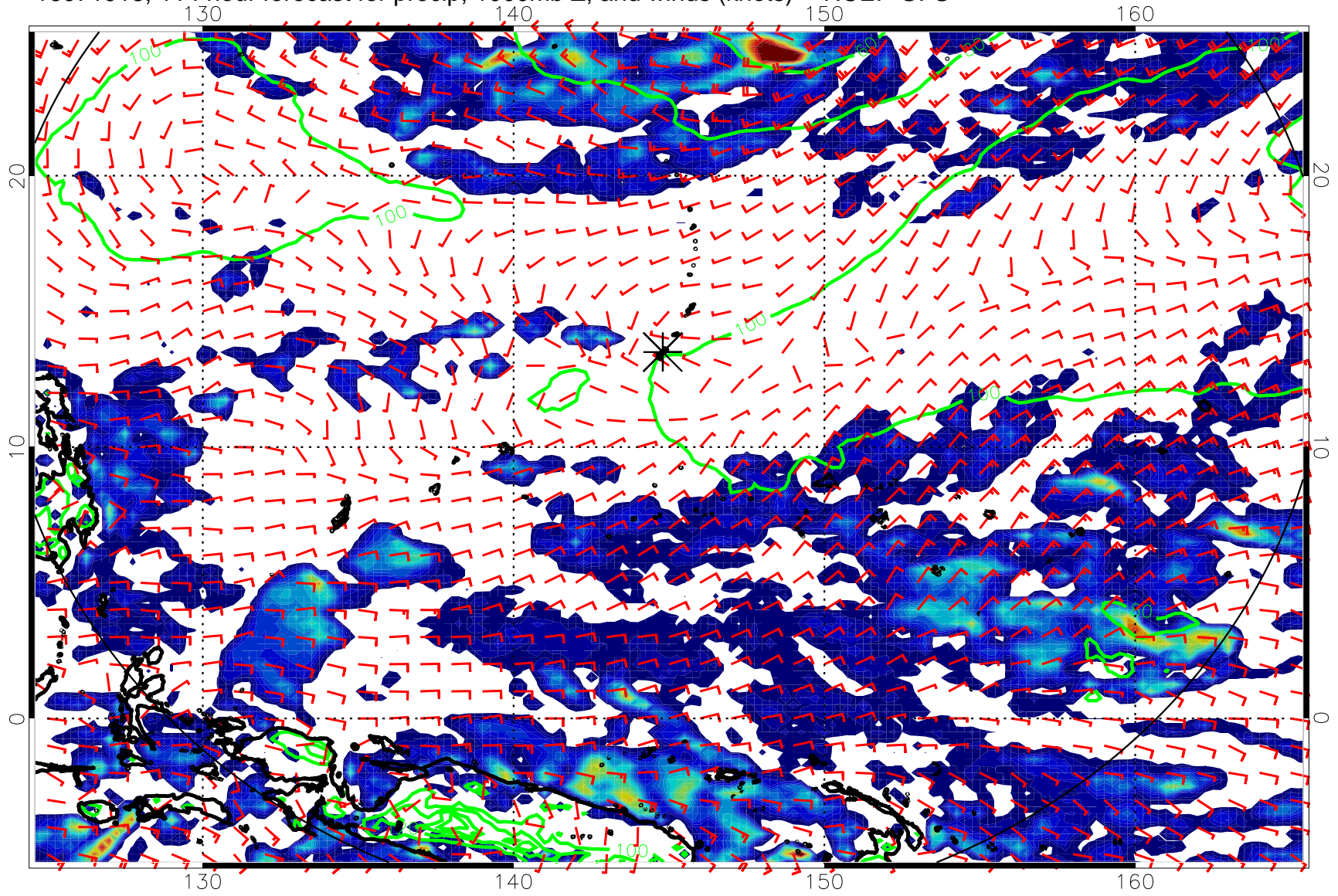
16071918, 114 hour forecast for precip, 1000mb Z, and winds (knots) -- NCEP GFS
