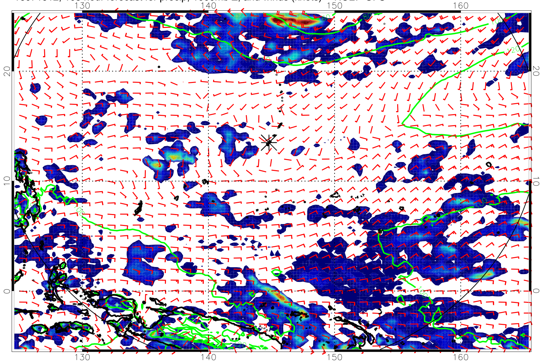
16071912, 108 hour forecast for precip, 1000mb Z, and winds (knots) -- NCEP GFS
