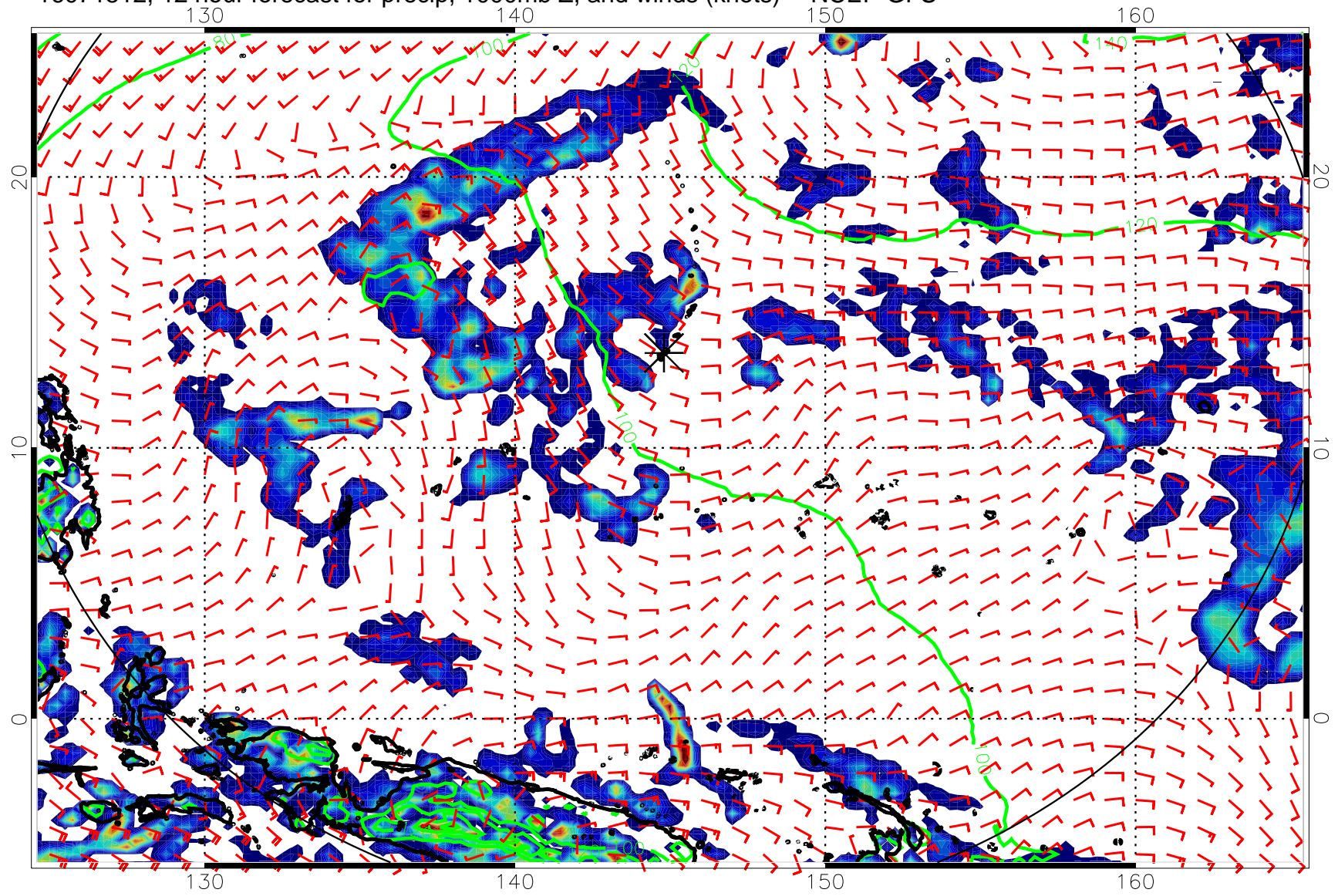
16071512, 12 hour forecast for precip, 1000mb Z, and winds (knots) -- NCEP GFS
