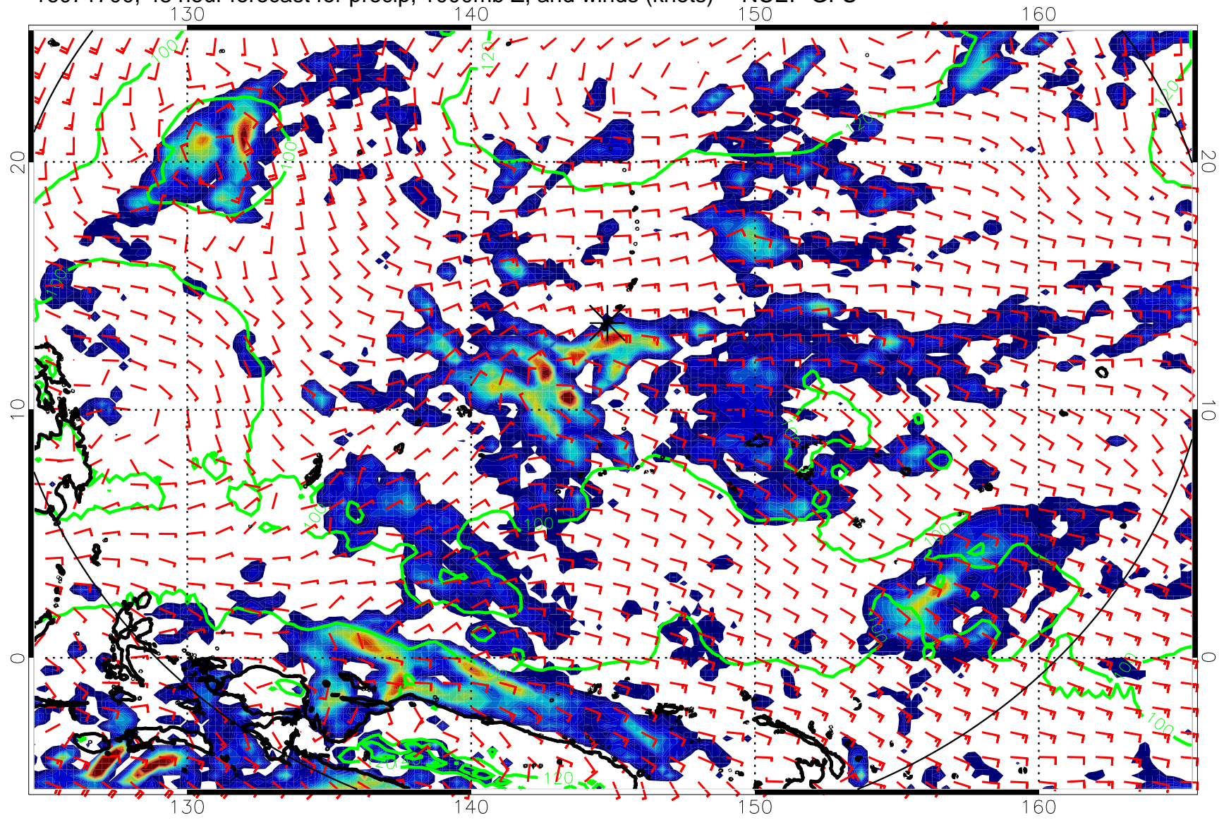
16071700, 48 hour forecast for precip, 1000mb Z, and winds (knots) -- NCEP GFS
