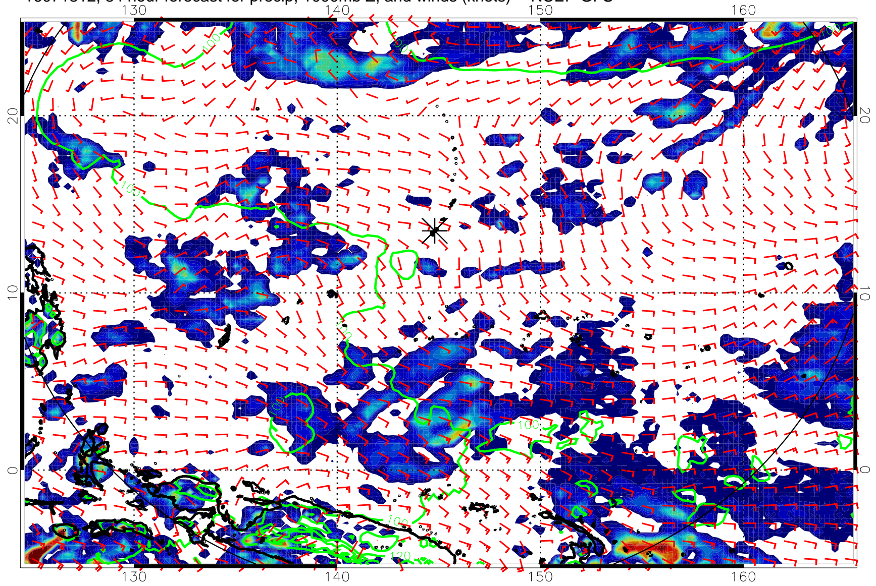
16071812, 84 hour forecast for precip, 1000mb Z, and winds (knots) -- NCEP GFS
