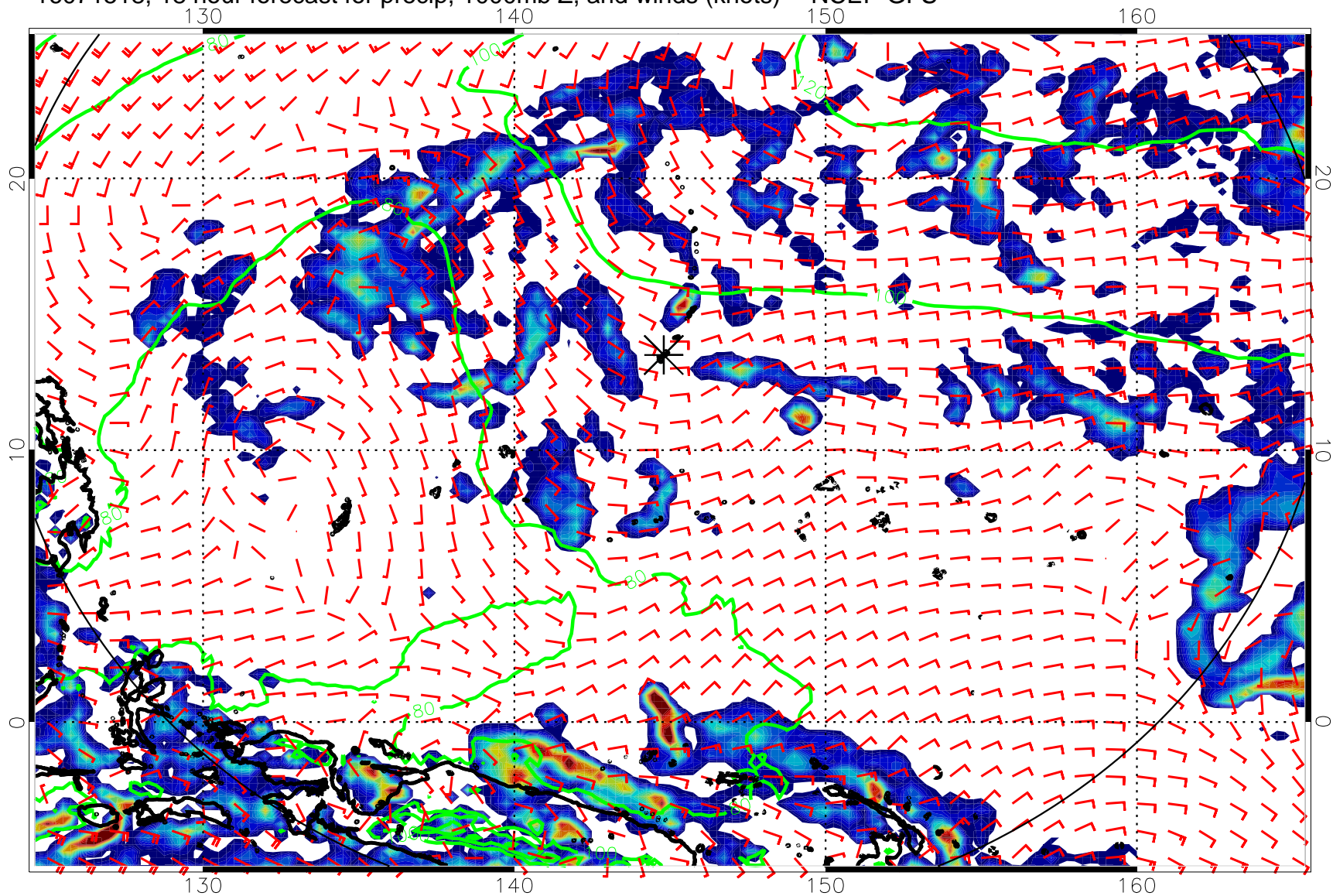
16071518, 18 hour forecast for precip, 1000mb Z, and winds (knots) -- NCEP GFS
