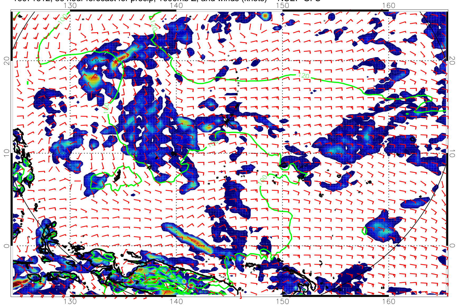
16071612, 36 hour forecast for precip, 1000mb Z, and winds (knots) -- NCEP GFS
