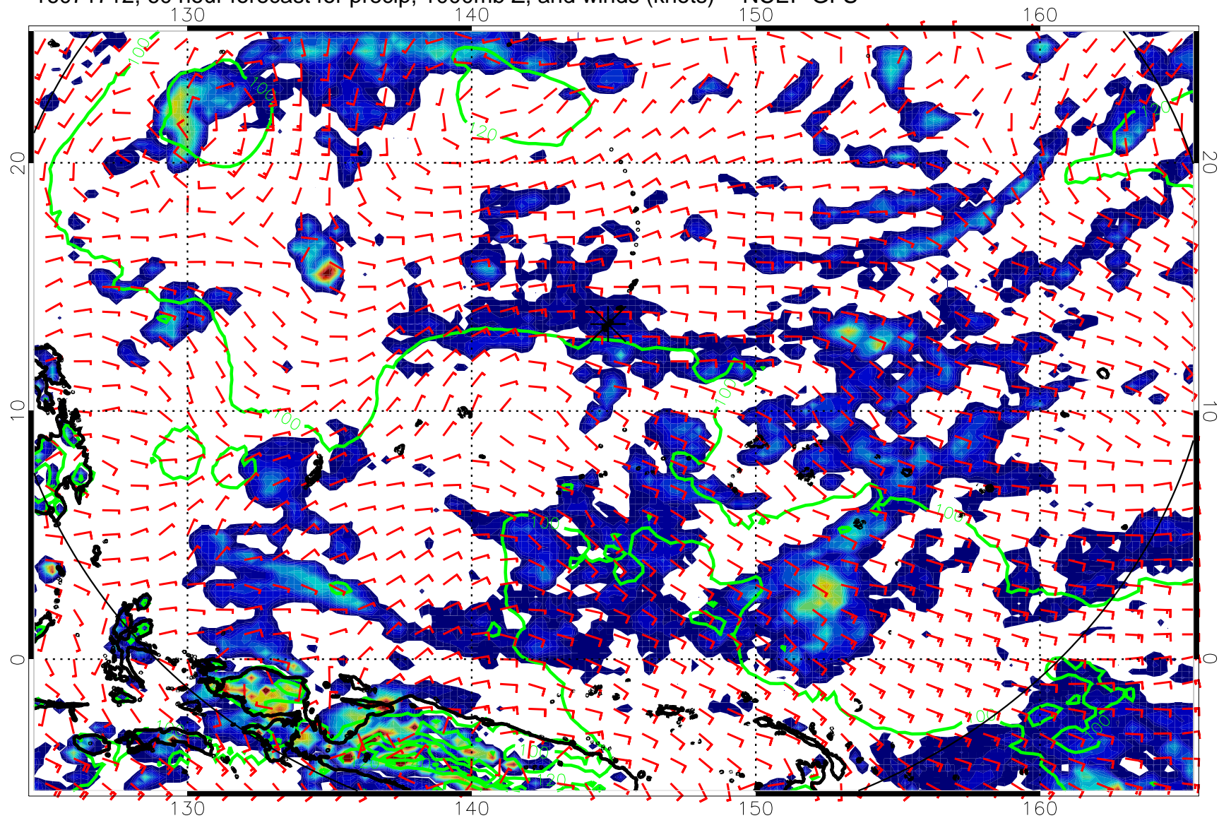
16071712, 60 hour forecast for precip, 1000mb Z, and winds (knots) -- NCEP GFS
