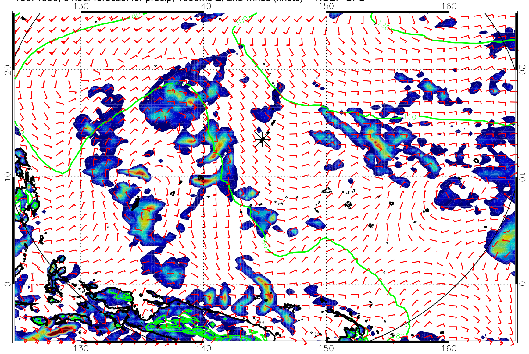
16071506, 6 hour forecast for precip, 1000mb Z, and winds (knots) -- NCEP GFS
