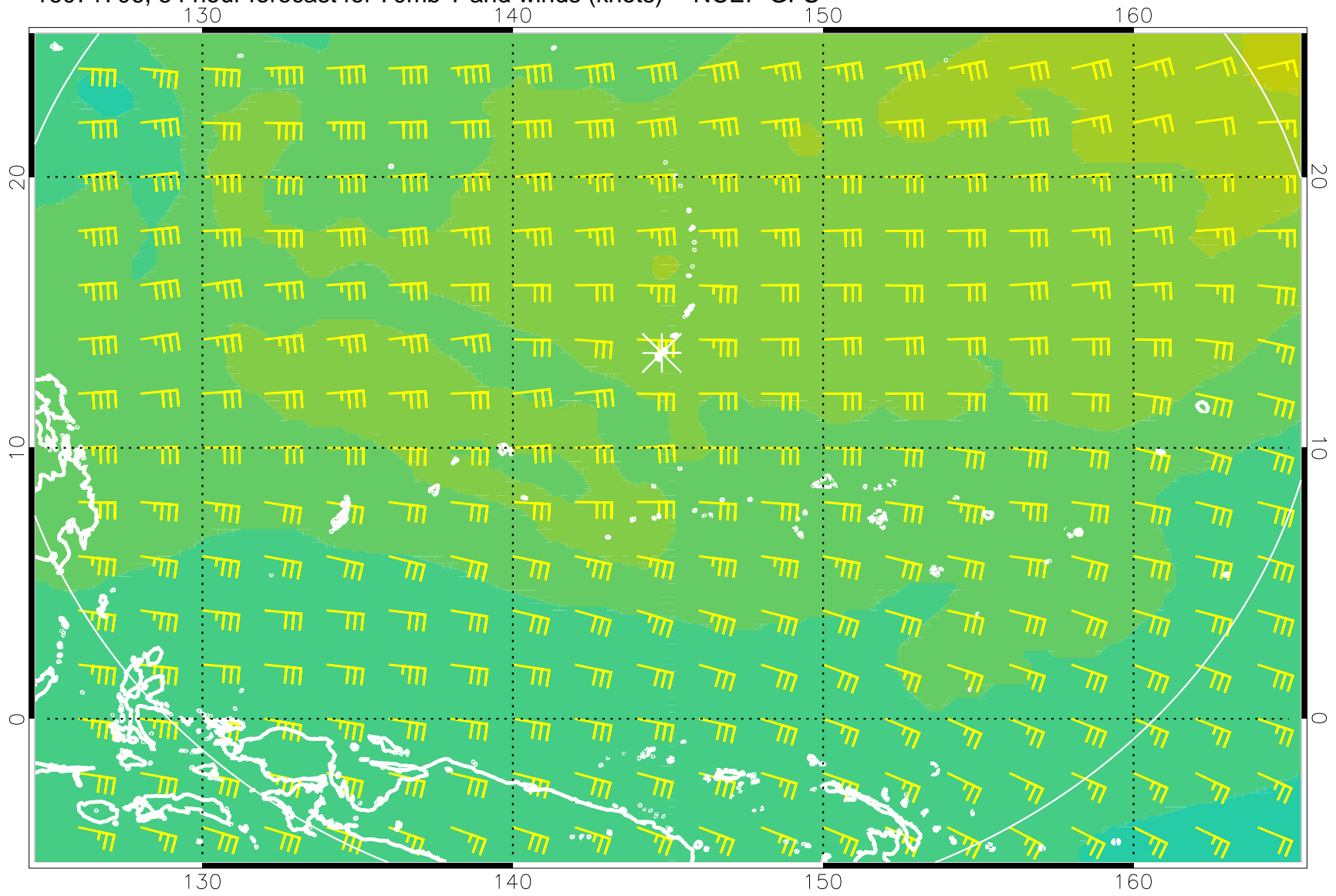
16071706, 54 hour forecast for 70mb T and winds (knots) -- NCEP GFS
