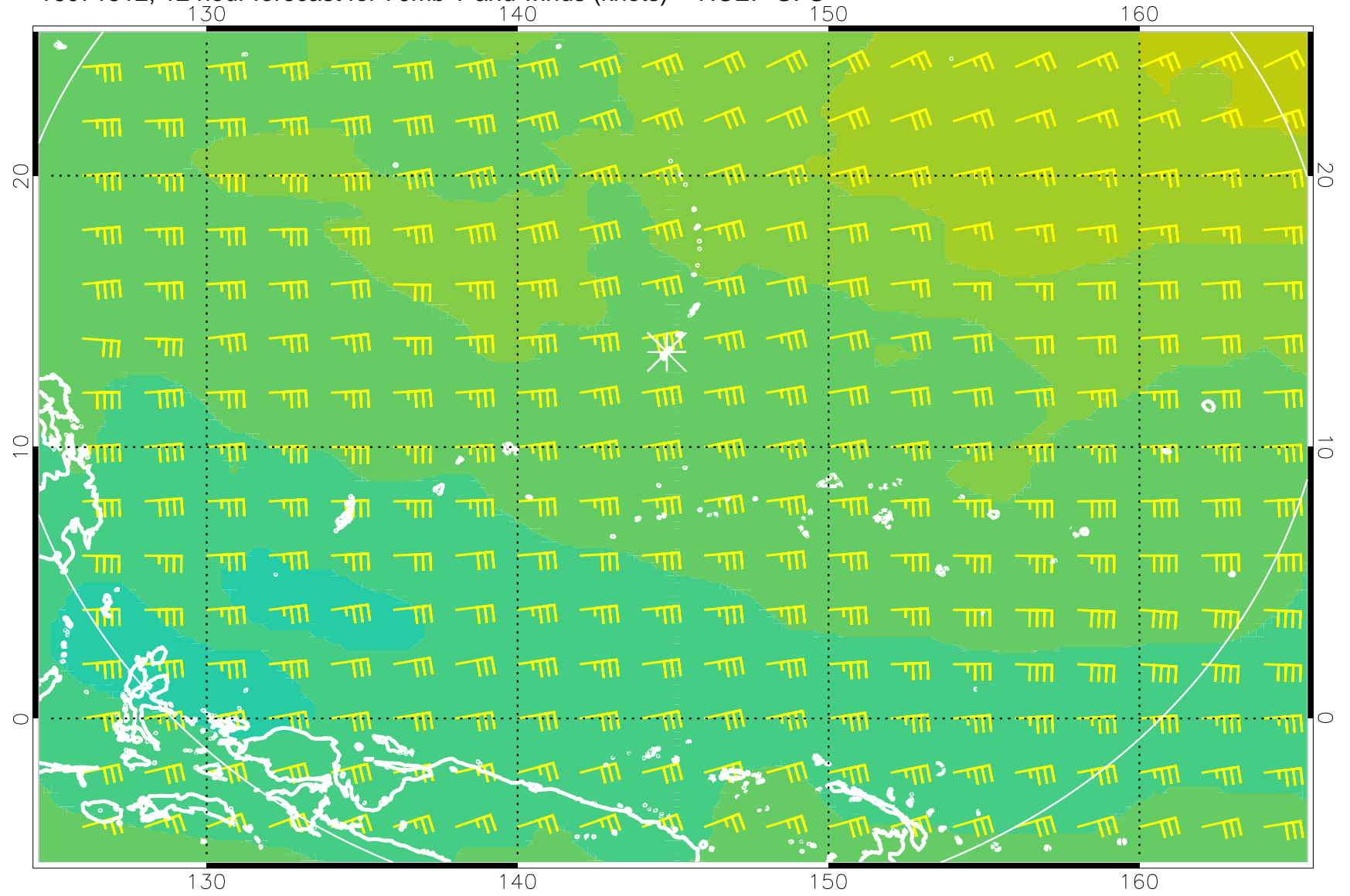
16071512, 12 hour forecast for 70mb T and winds (knots) -- NCEP GFS
