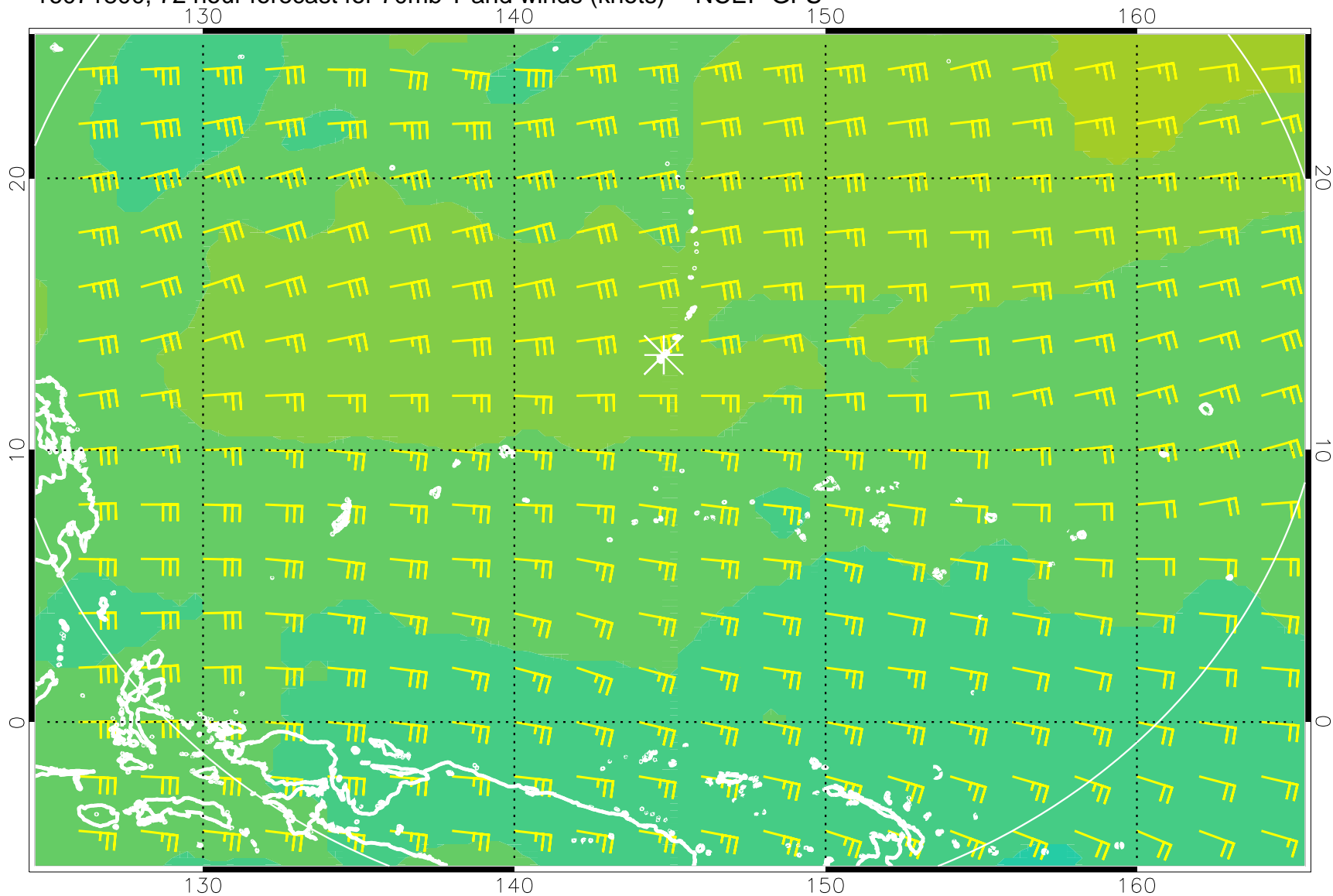
16071800, 72 hour forecast for 70mb T and winds (knots) -- NCEP GFS
