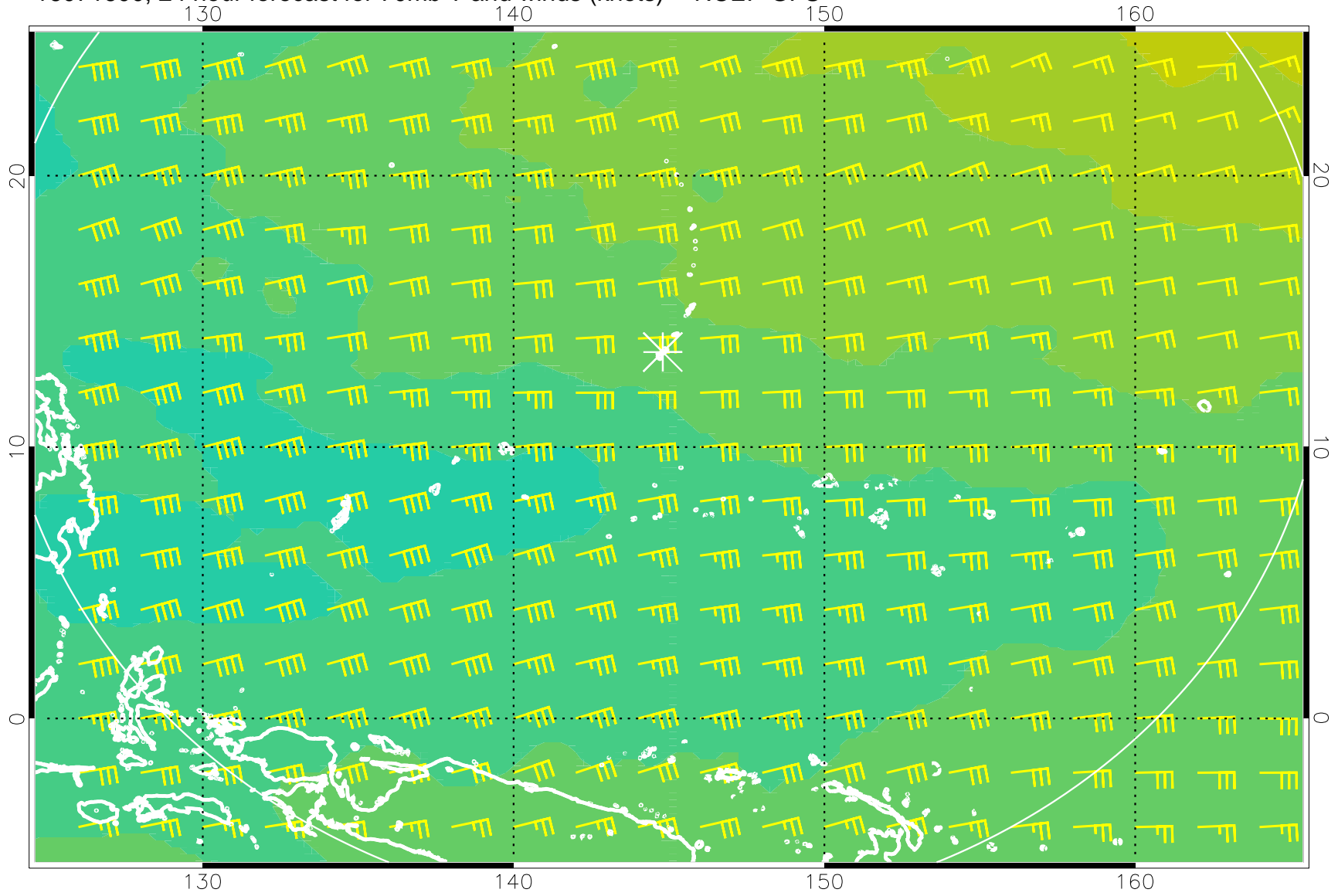
16071600, 24 hour forecast for 70mb T and winds (knots) -- NCEP GFS
