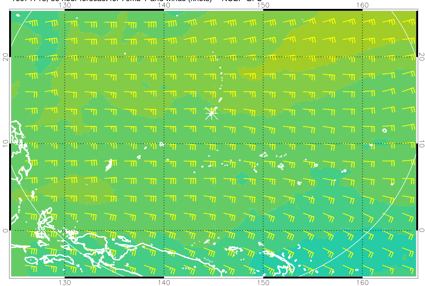
16071718, 66 hour forecast for 70mb T and winds (knots) -- NCEP GFS
