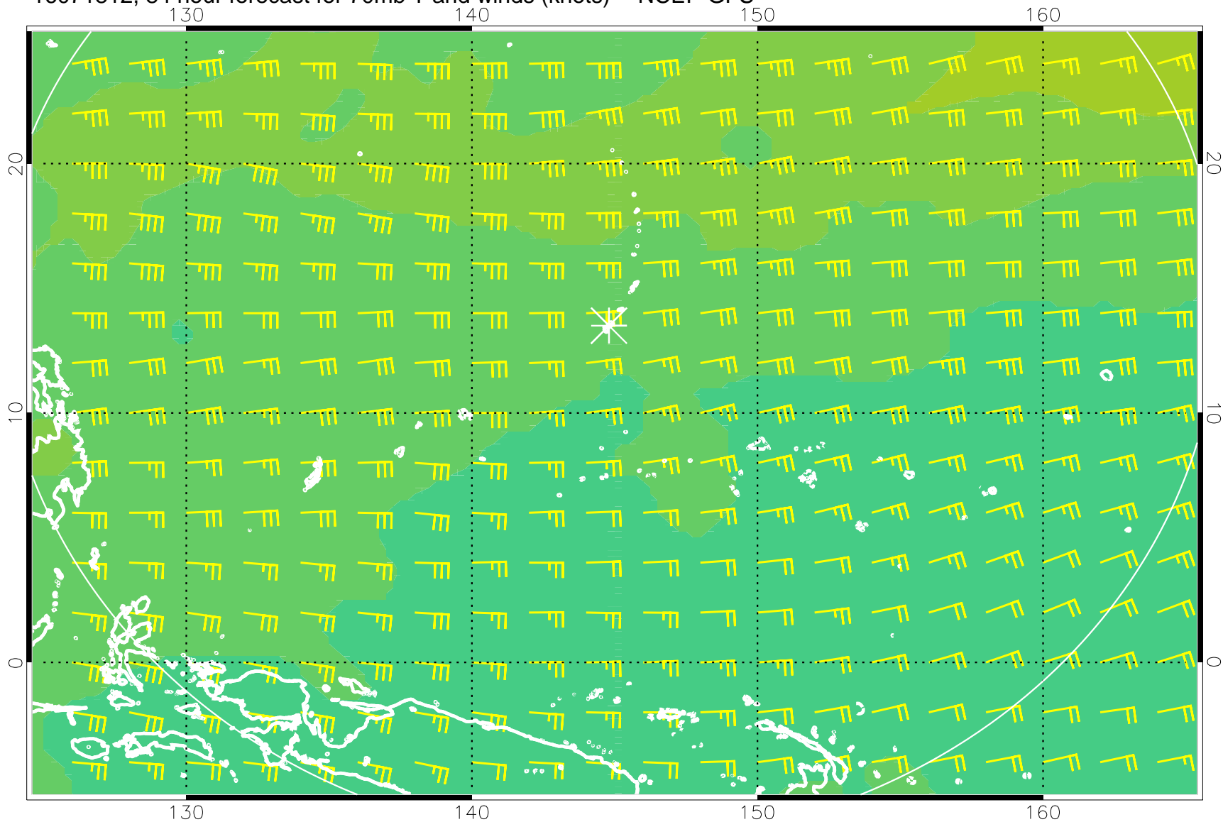
16071812, 84 hour forecast for 70mb T and winds (knots) -- NCEP GFS
