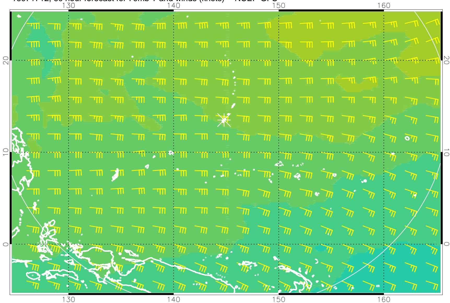
16071712, 60 hour forecast for 70mb T and winds (knots) -- NCEP GFS
