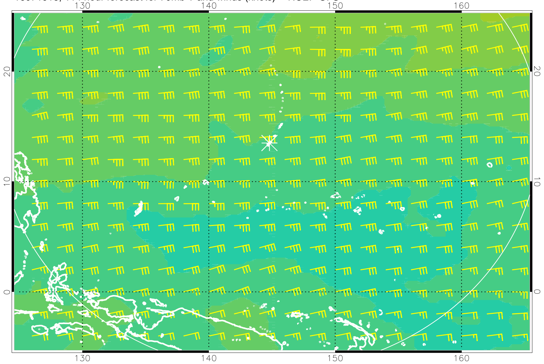
16071918, 114 hour forecast for 70mb T and winds (knots) -- NCEP GFS
