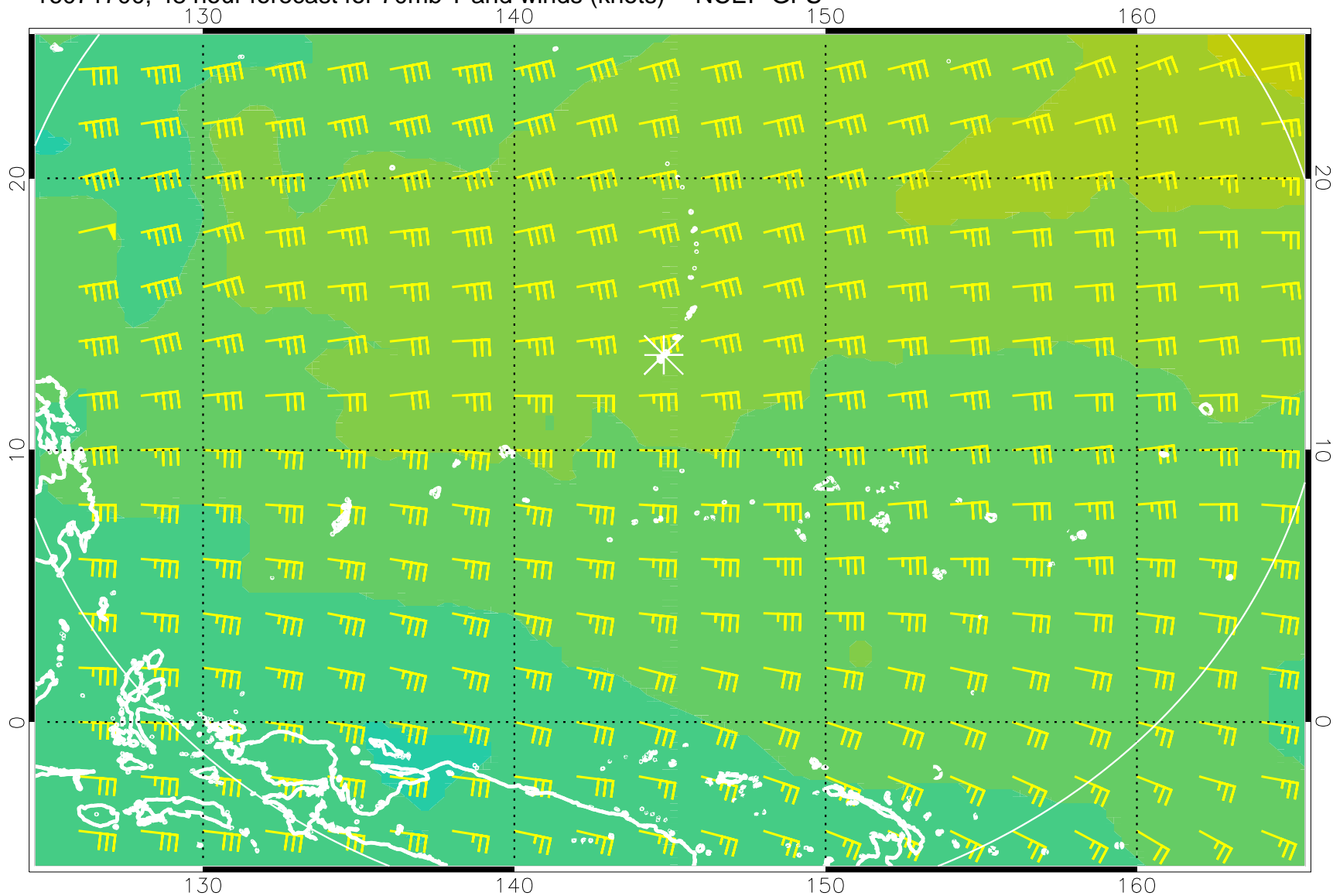
16071700, 48 hour forecast for 70mb T and winds (knots) -- NCEP GFS
