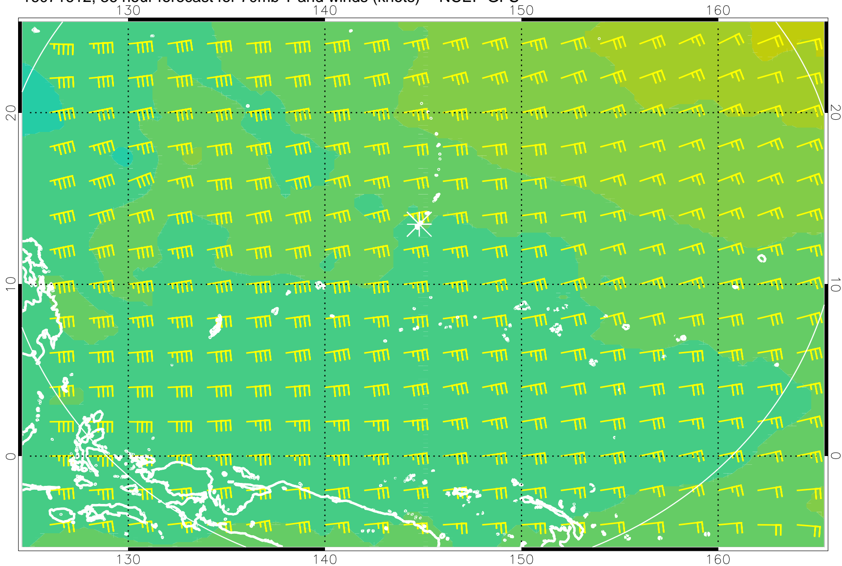
16071612, 36 hour forecast for 70mb T and winds (knots) -- NCEP GFS
