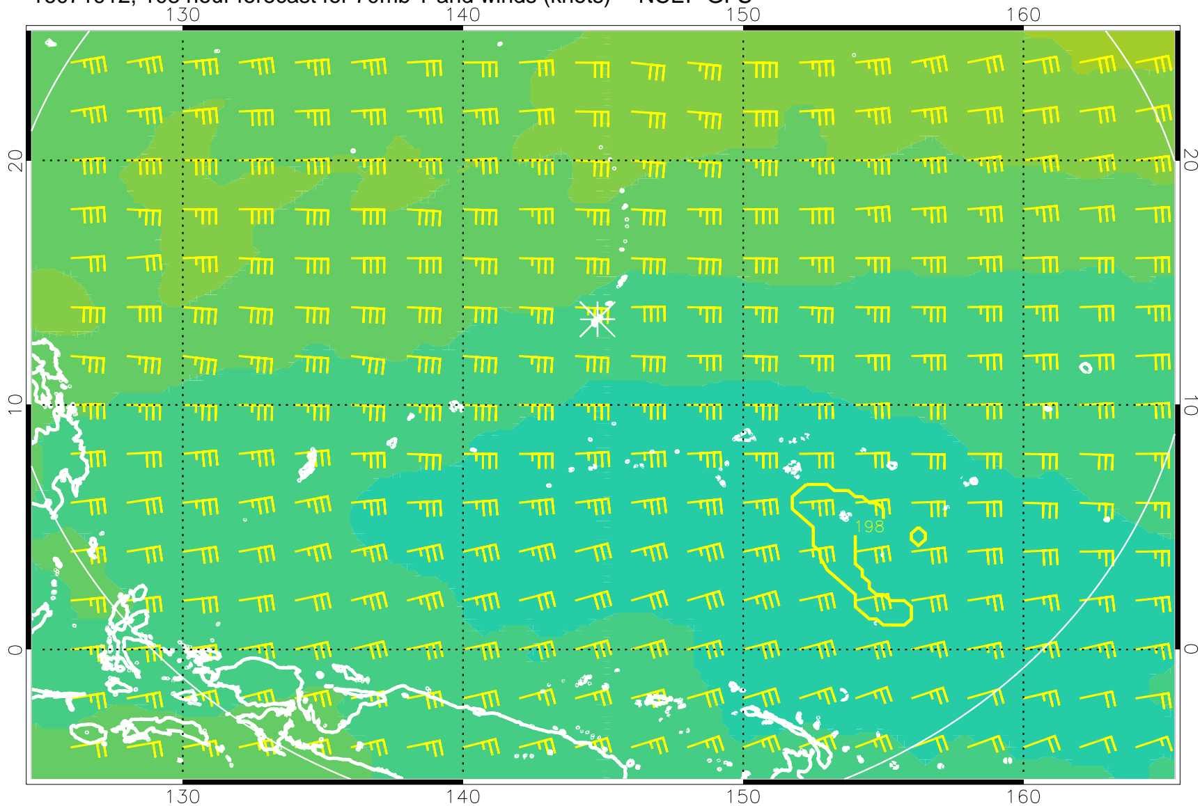
16071912, 108 hour forecast for 70mb T and winds (knots) -- NCEP GFS
