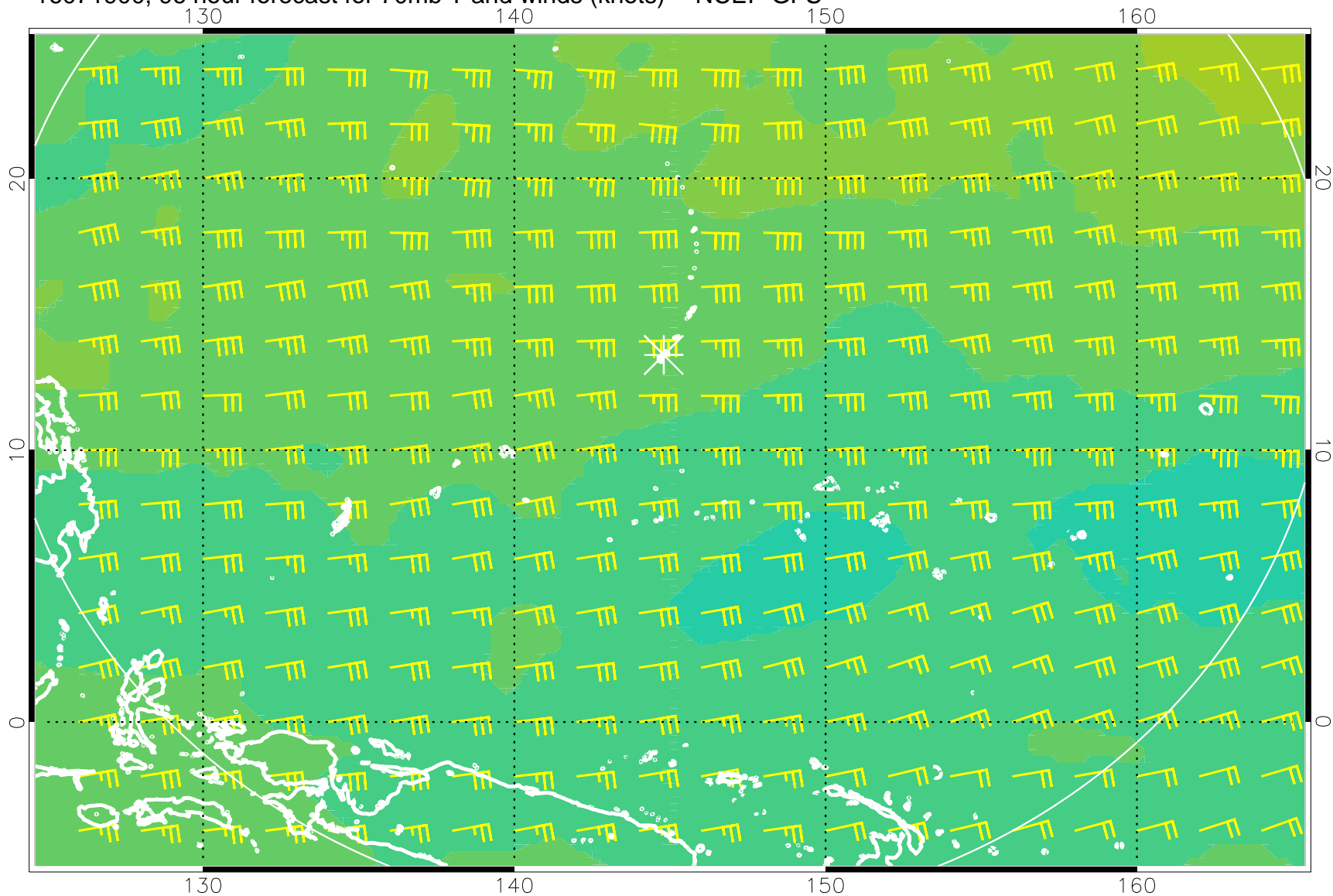
16071900, 96 hour forecast for 70mb T and winds (knots) -- NCEP GFS
