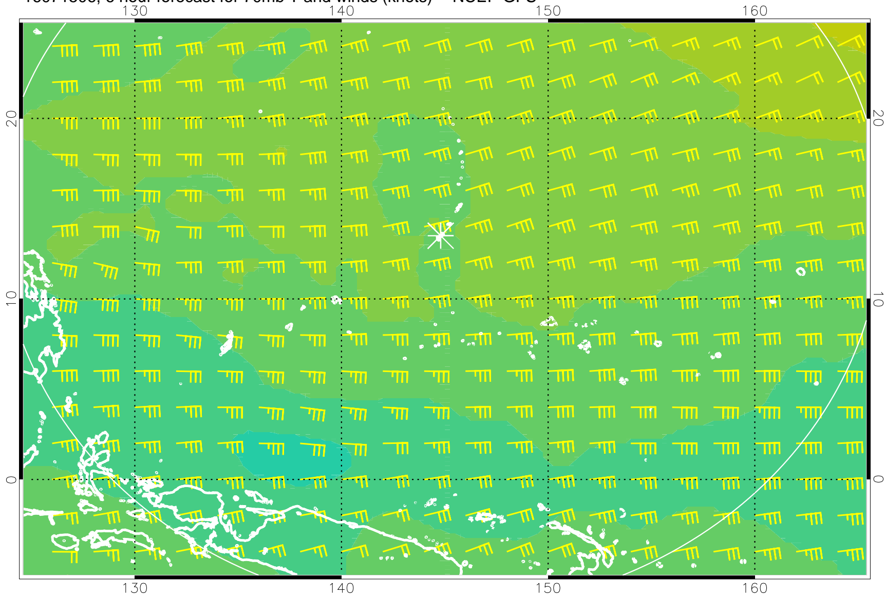
16071506, 6 hour forecast for 70mb T and winds (knots) -- NCEP GFS
