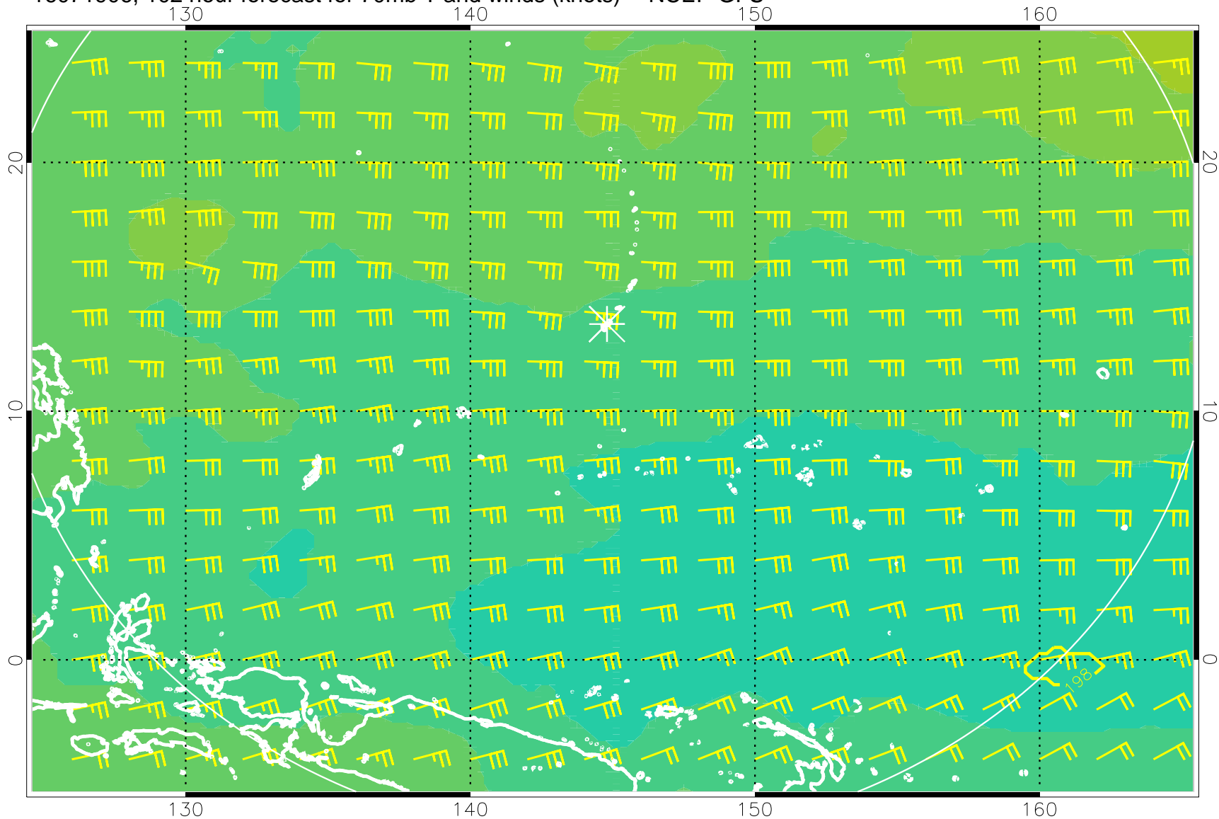
16071906, 102 hour forecast for 70mb T and winds (knots) -- NCEP GFS
