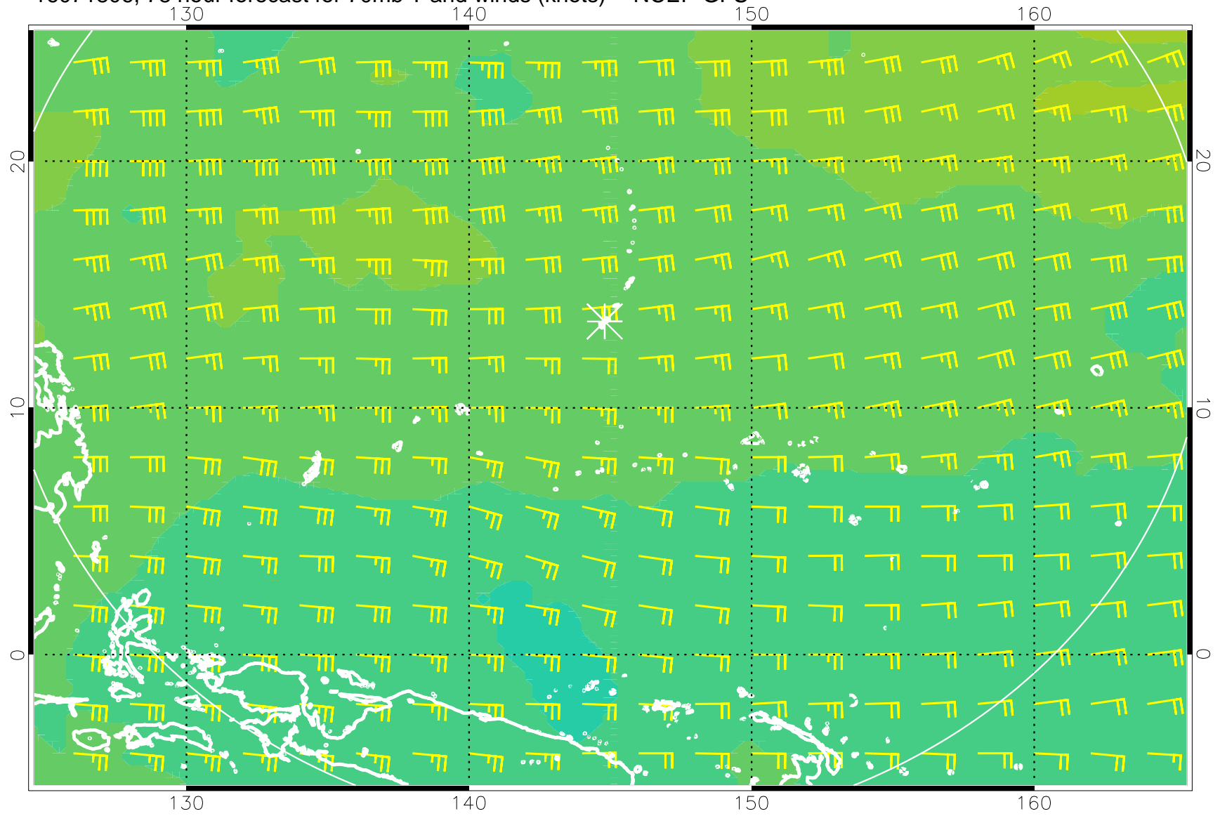
16071806, 78 hour forecast for 70mb T and winds (knots) -- NCEP GFS
