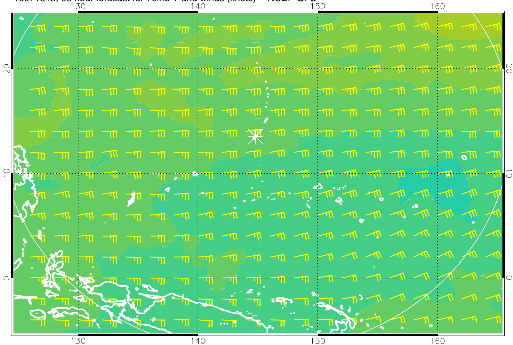
16071818, 90 hour forecast for 70mb T and winds (knots) -- NCEP GFS
