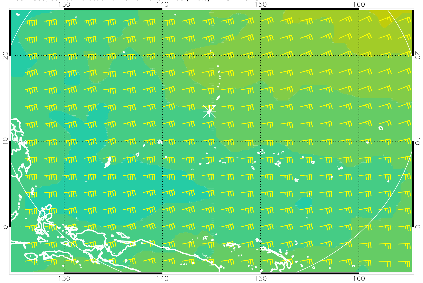
16071606, 30 hour forecast for 70mb T and winds (knots) -- NCEP GFS
