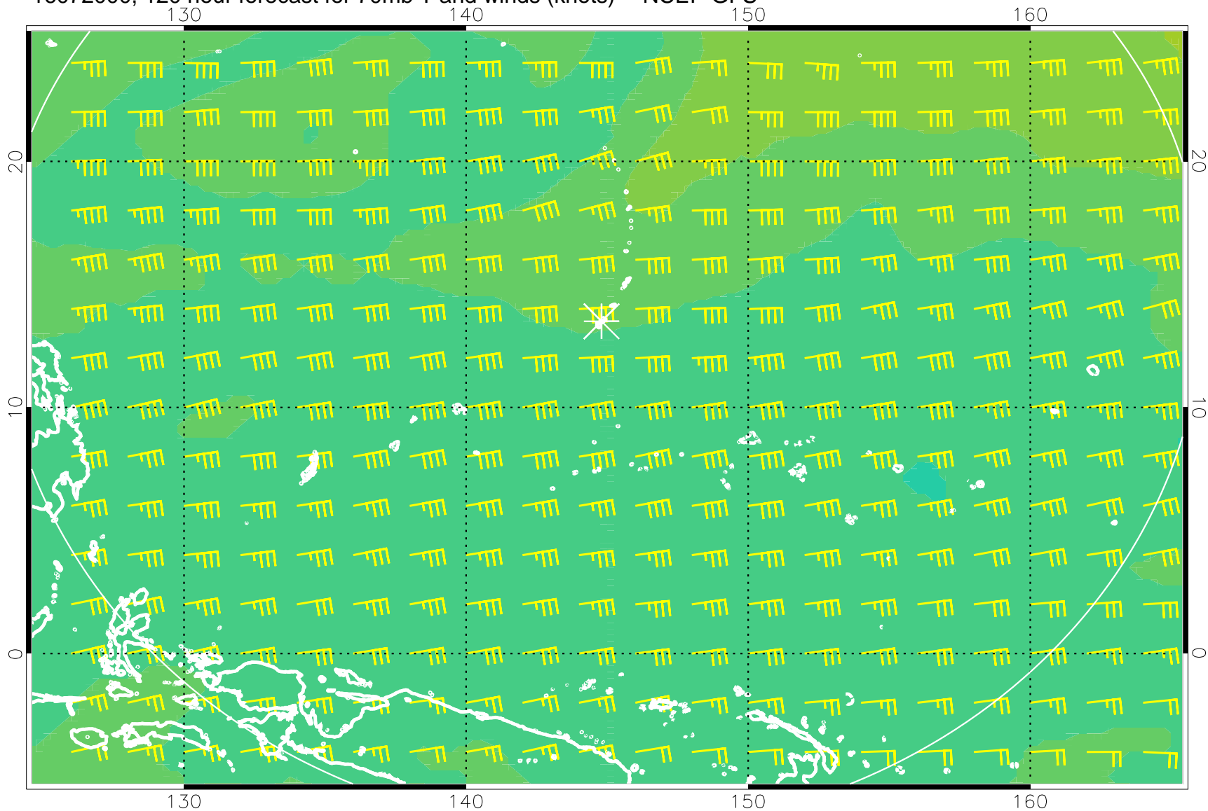
16072000, 120 hour forecast for 70mb T and winds (knots) -- NCEP GFS
