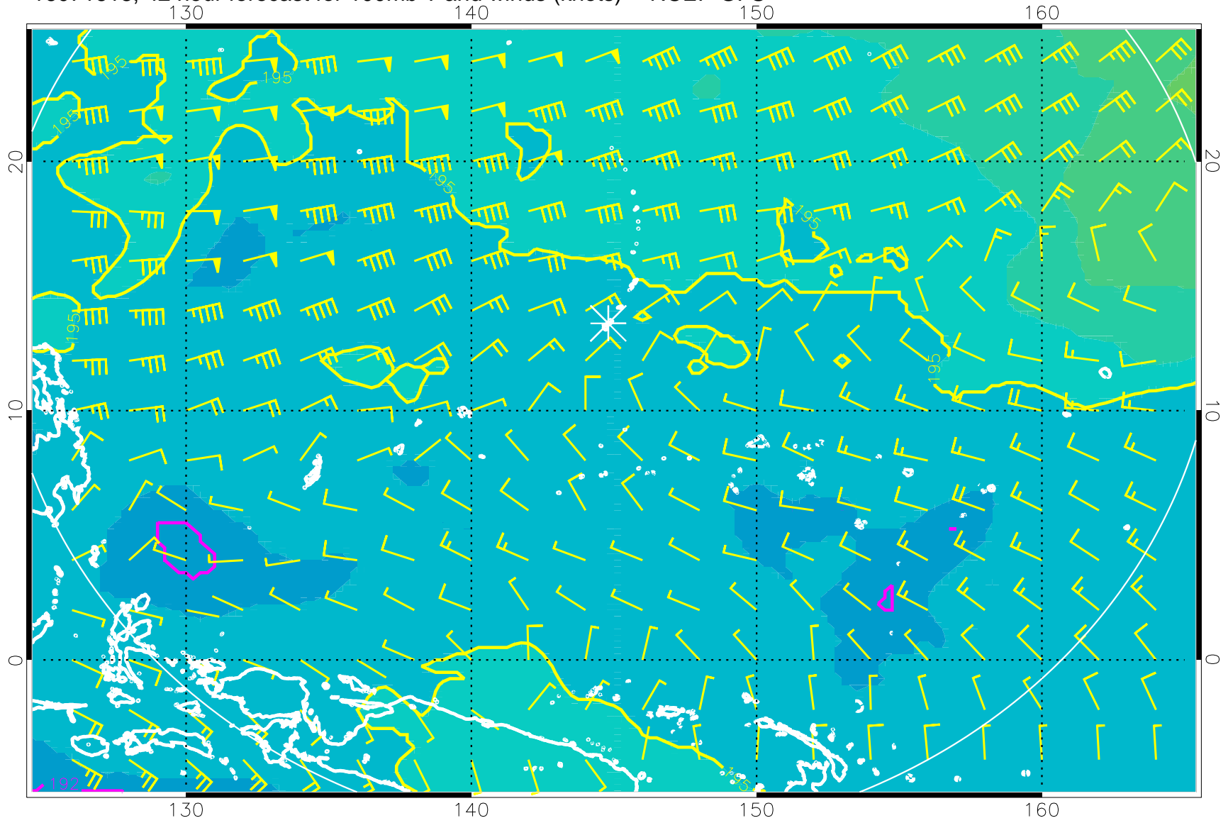
16071618, 42 hour forecast for 100mb T and winds (knots) -- NCEP GFS
