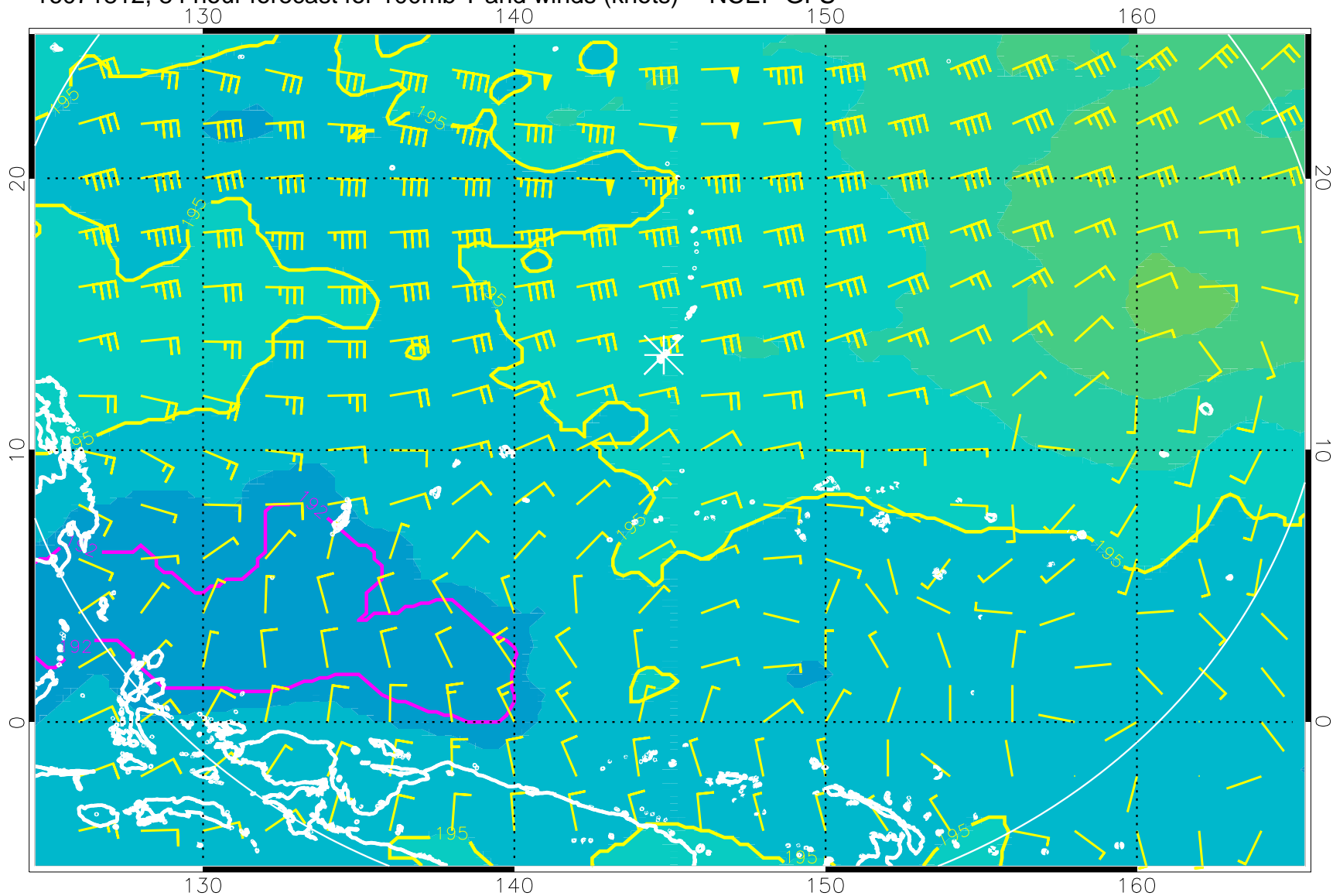
16071812, 84 hour forecast for 100mb T and winds (knots) -- NCEP GFS
