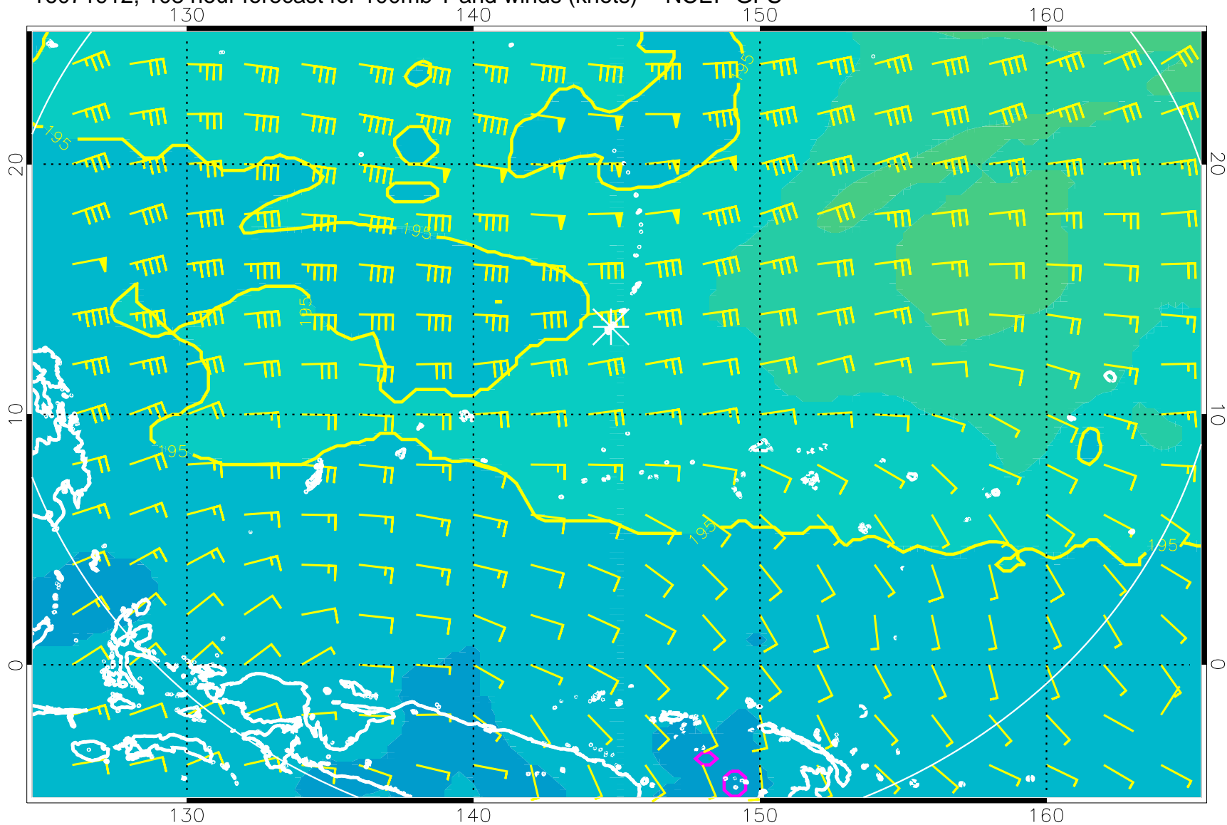
16071912, 108 hour forecast for 100mb T and winds (knots) -- NCEP GFS
