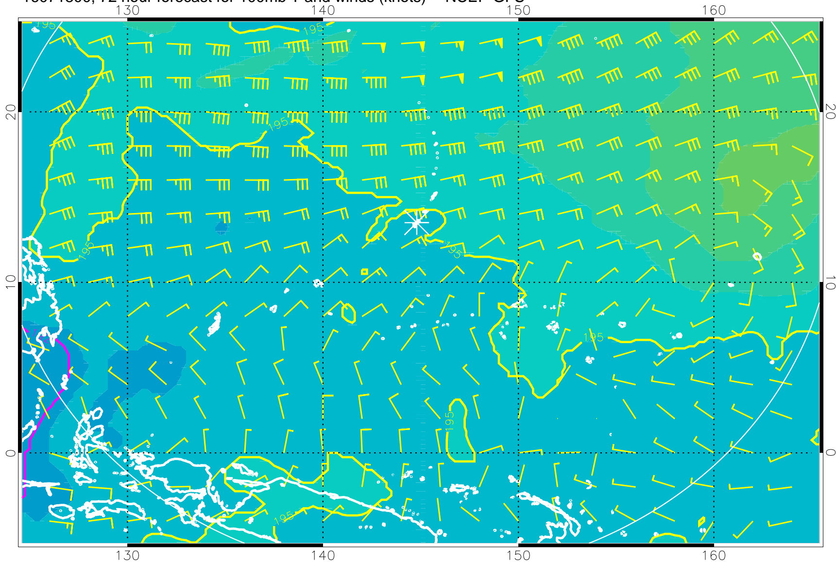
16071800, 72 hour forecast for 100mb T and winds (knots) -- NCEP GFS
