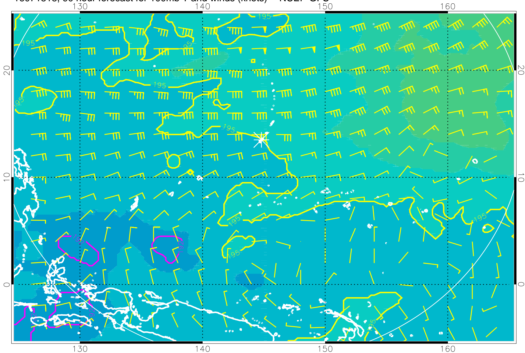
16071818, 90 hour forecast for 100mb T and winds (knots) -- NCEP GFS
