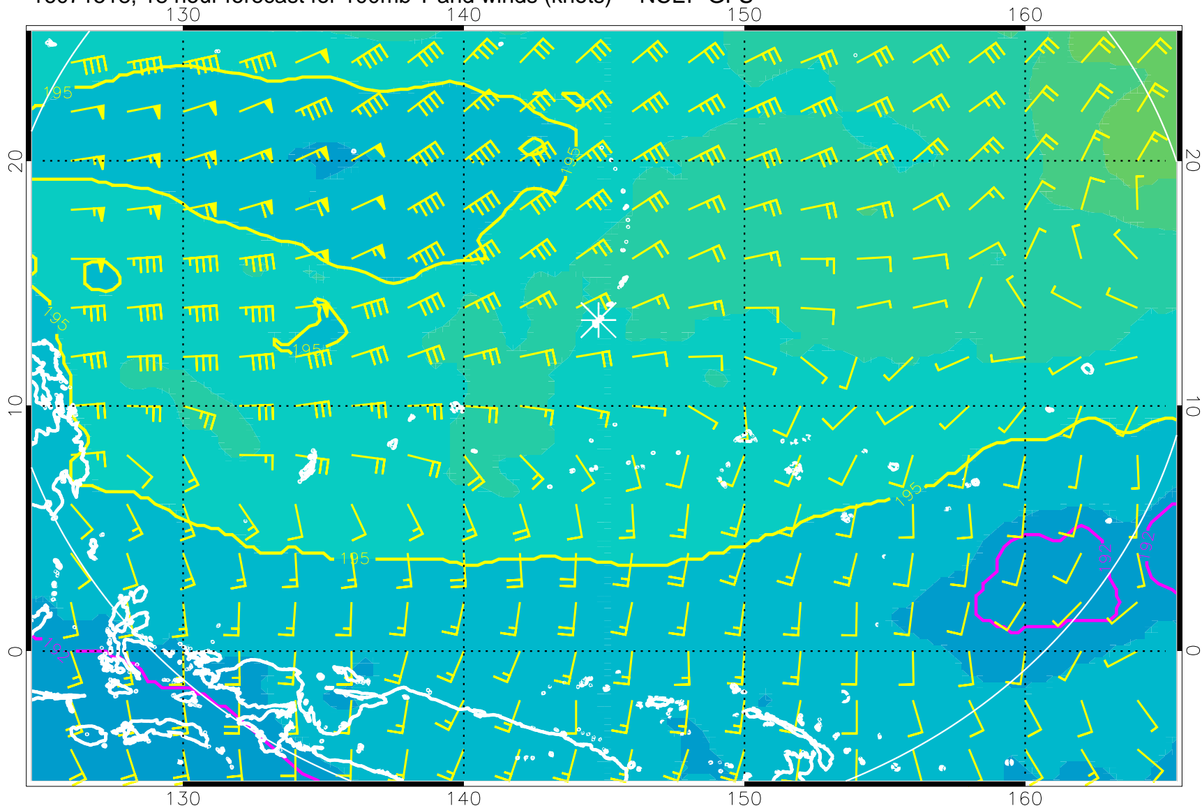
16071518, 18 hour forecast for 100mb T and winds (knots) -- NCEP GFS
