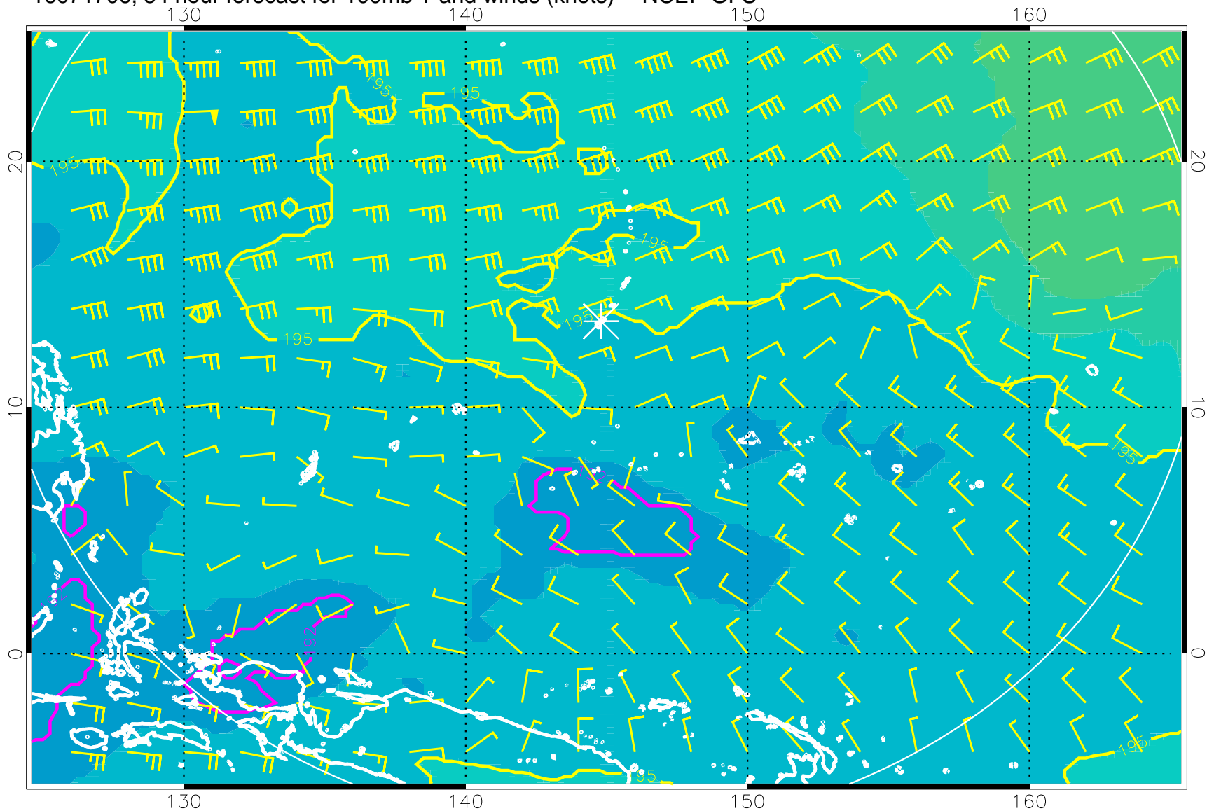
16071706, 54 hour forecast for 100mb T and winds (knots) -- NCEP GFS
