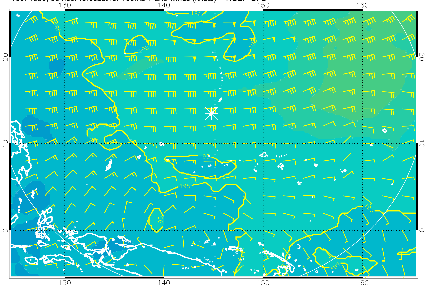
16071900, 96 hour forecast for 100mb T and winds (knots) -- NCEP GFS
