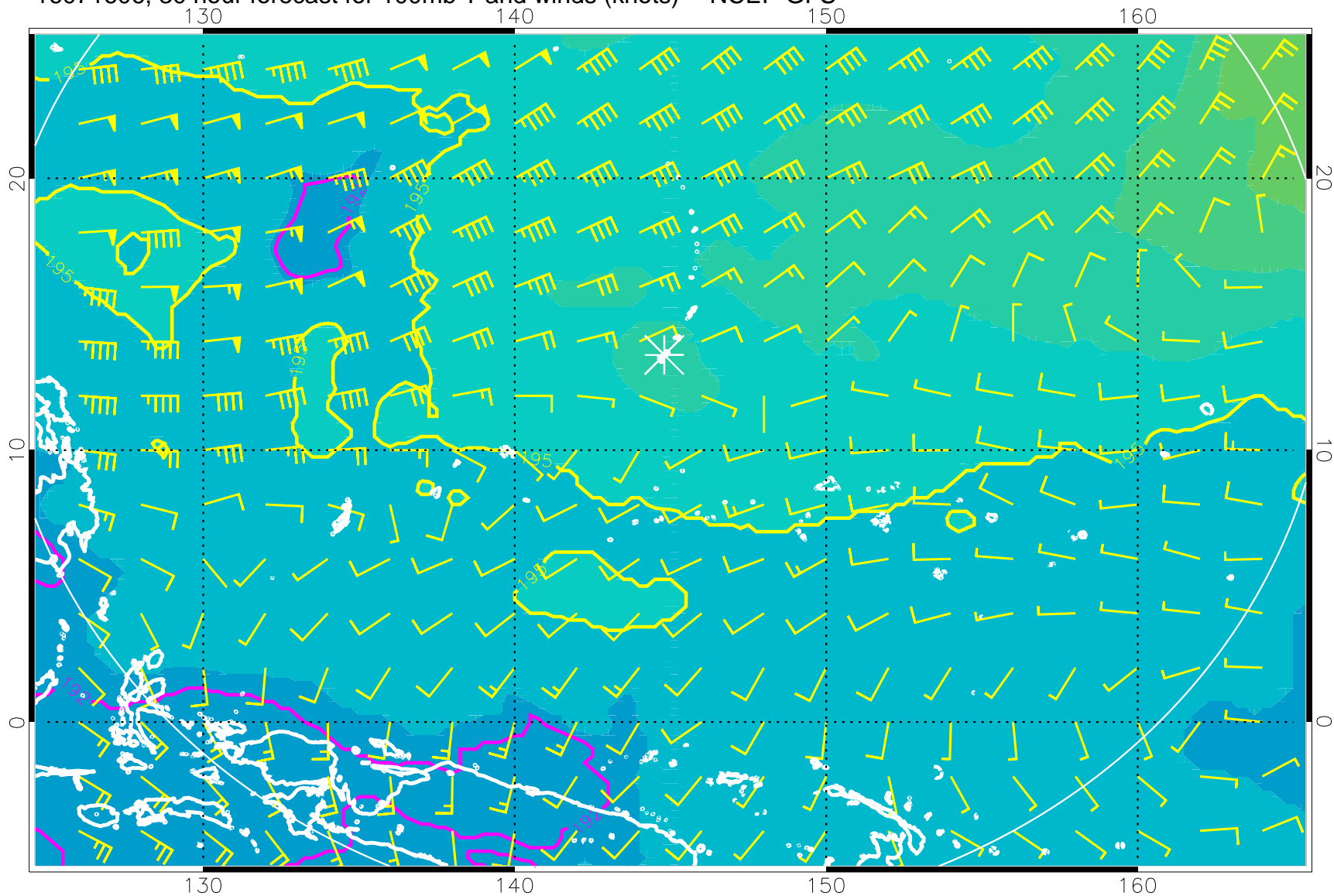
16071606, 30 hour forecast for 100mb T and winds (knots) -- NCEP GFS
