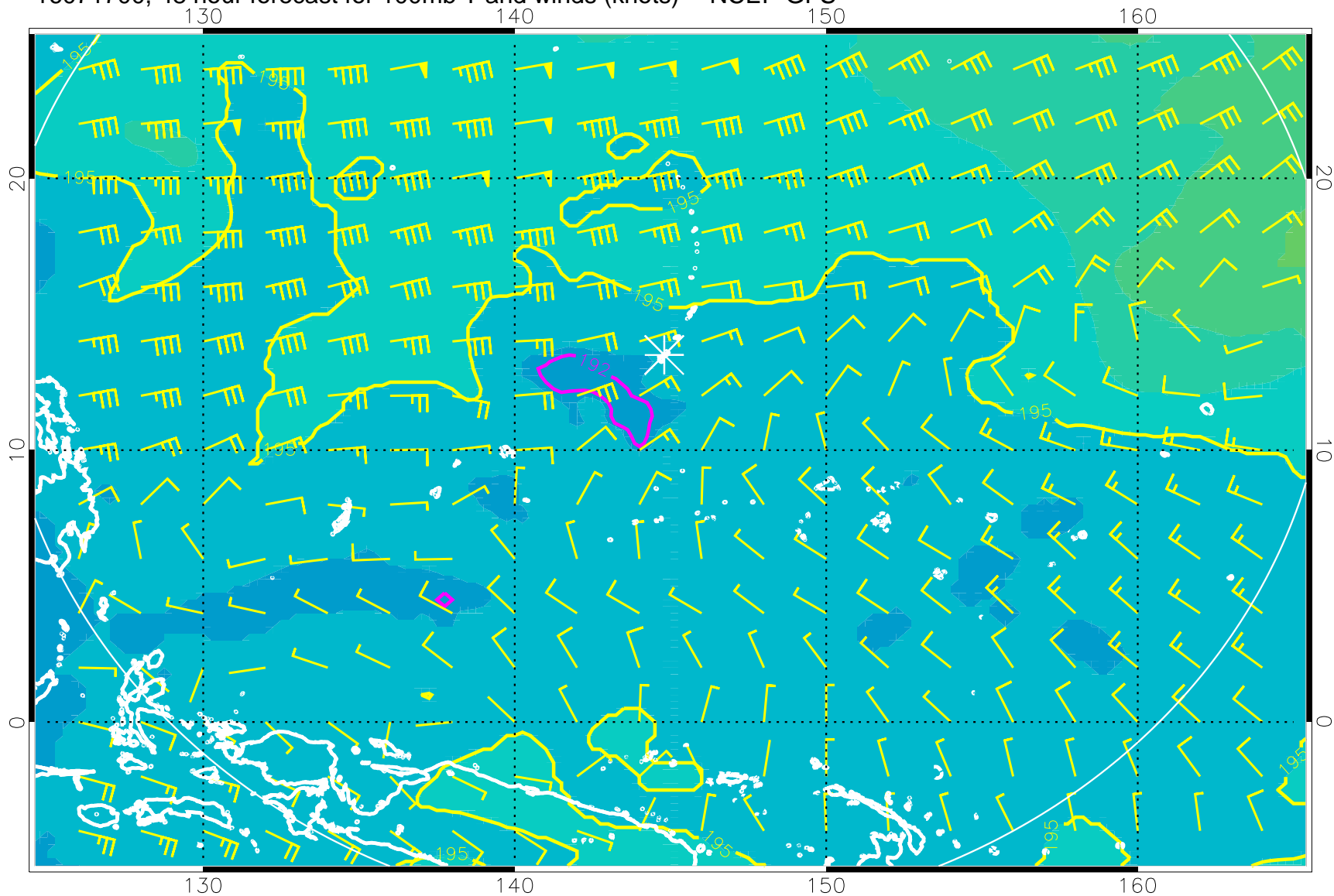
16071700, 48 hour forecast for 100mb T and winds (knots) -- NCEP GFS
