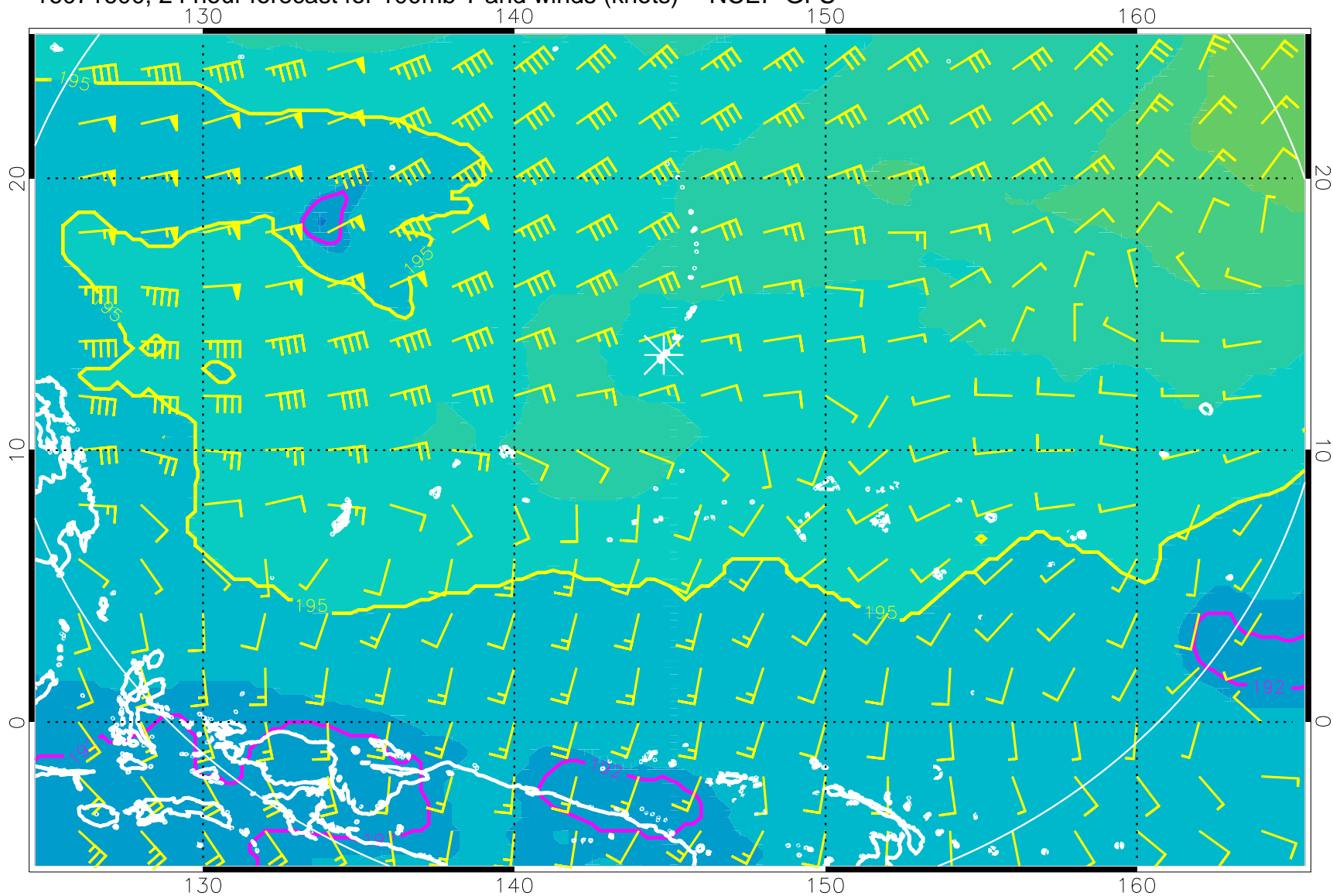
16071600, 24 hour forecast for 100mb T and winds (knots) -- NCEP GFS
