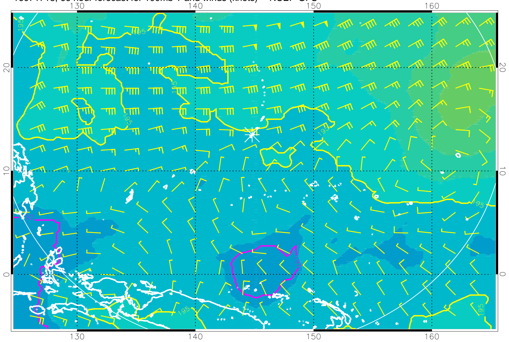
16071718, 66 hour forecast for 100mb T and winds (knots) -- NCEP GFS
