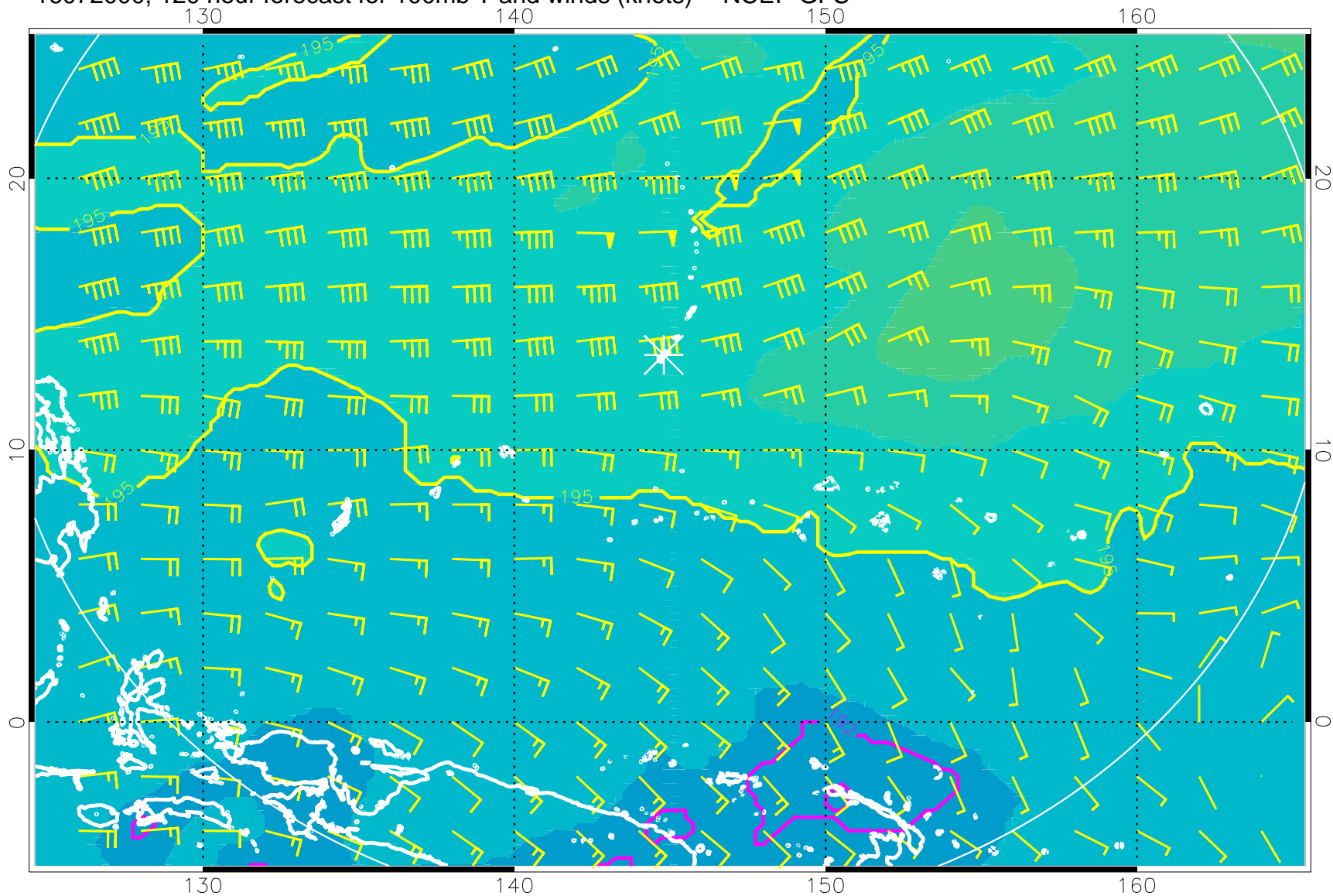
16072000, 120 hour forecast for 100mb T and winds (knots) -- NCEP GFS
