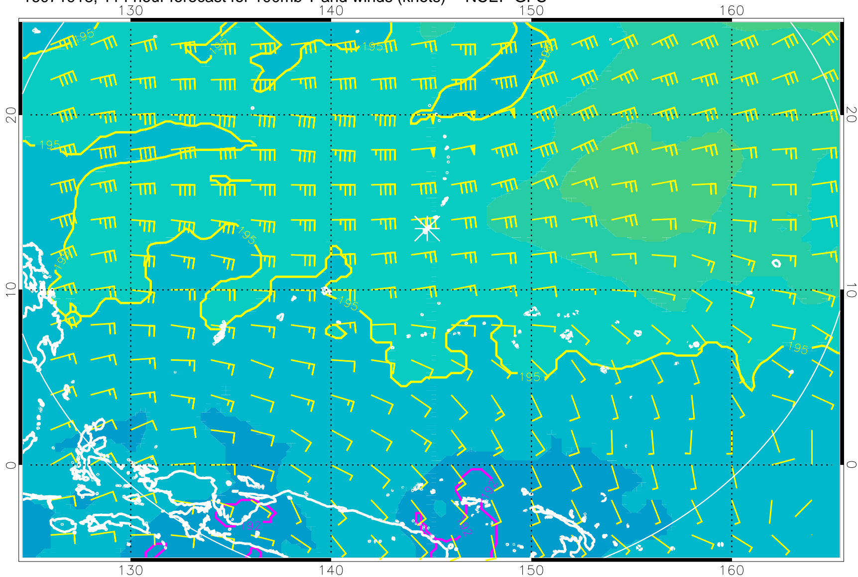
16071918, 114 hour forecast for 100mb T and winds (knots) -- NCEP GFS
