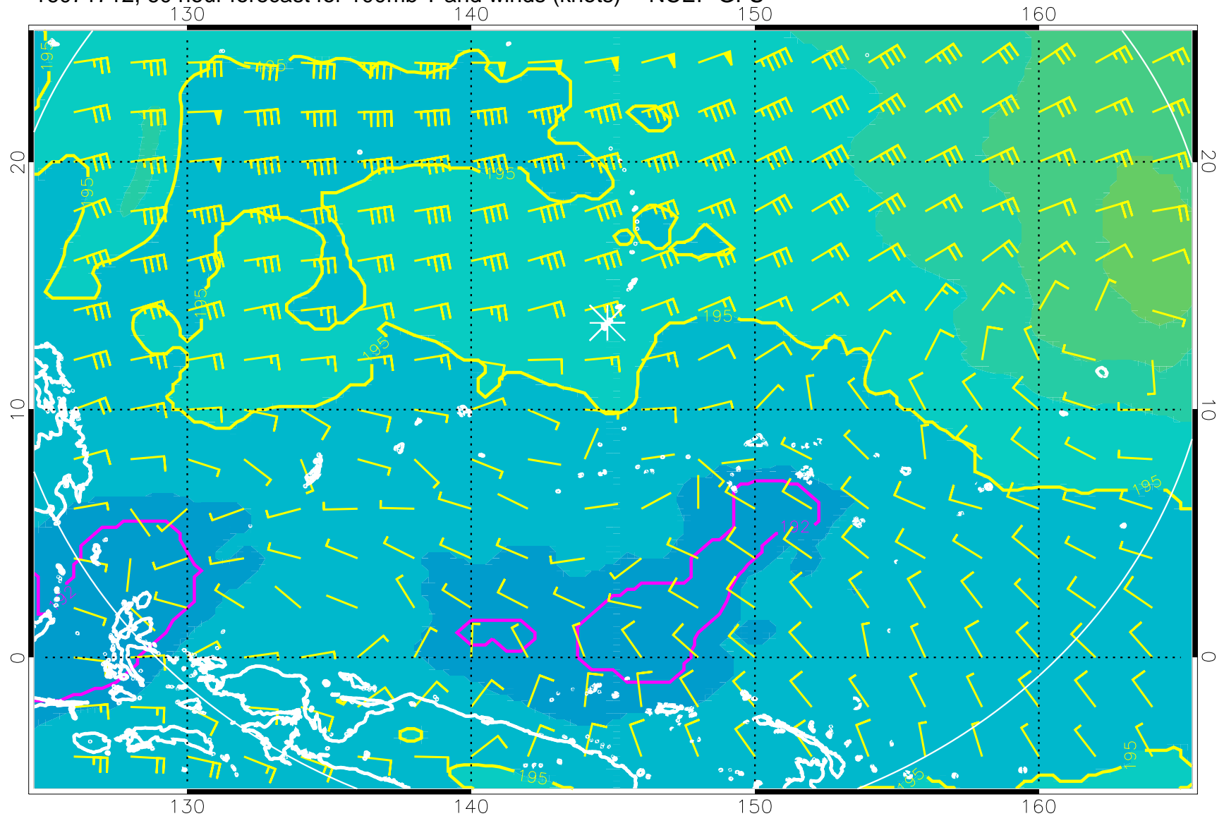
16071712, 60 hour forecast for 100mb T and winds (knots) -- NCEP GFS
