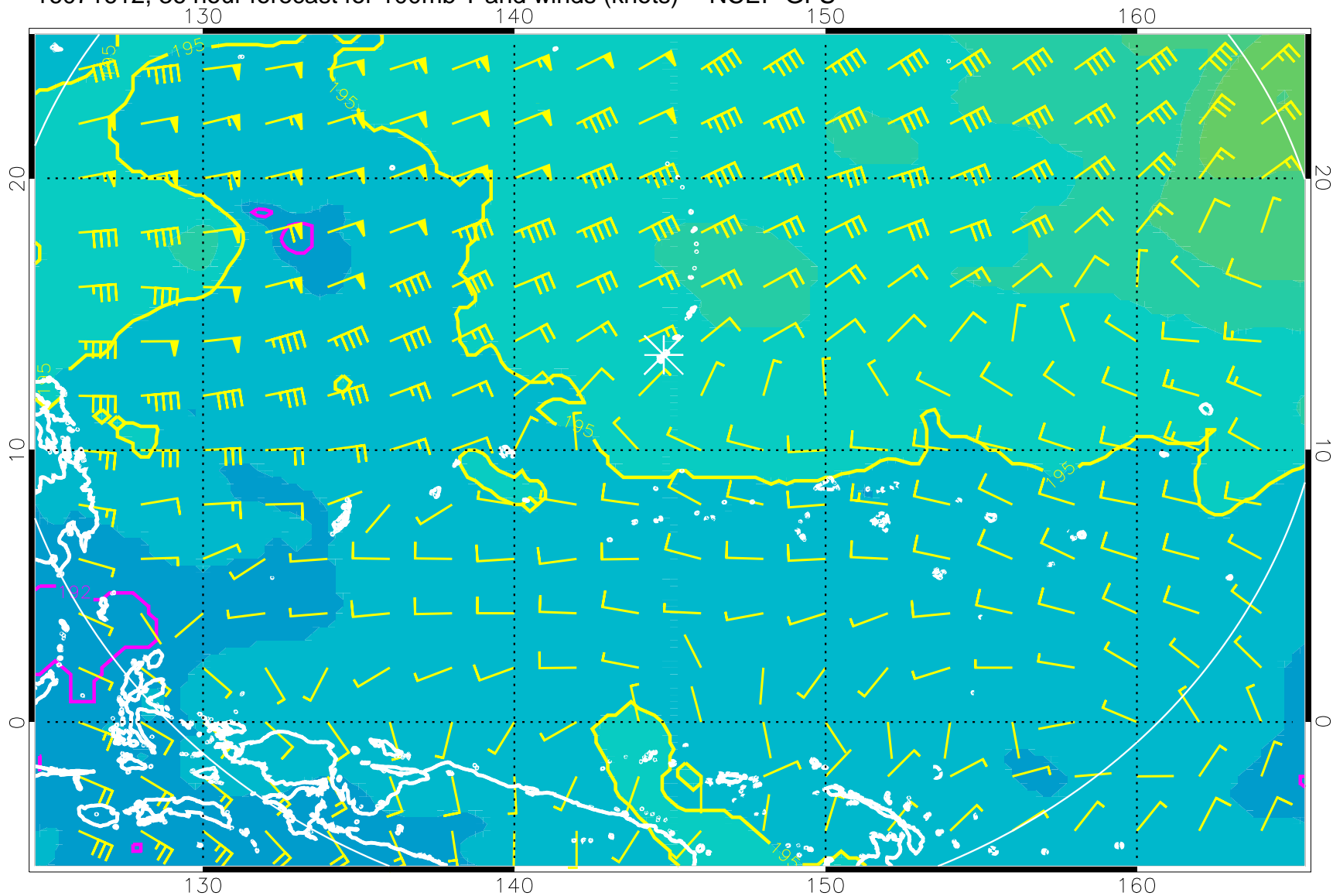
16071612, 36 hour forecast for 100mb T and winds (knots) -- NCEP GFS
