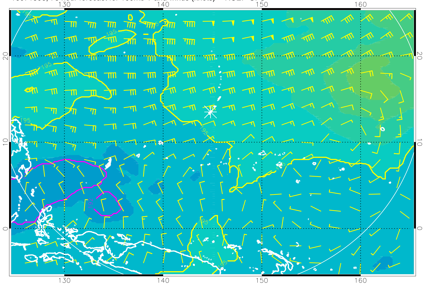
16071806, 78 hour forecast for 100mb T and winds (knots) -- NCEP GFS
