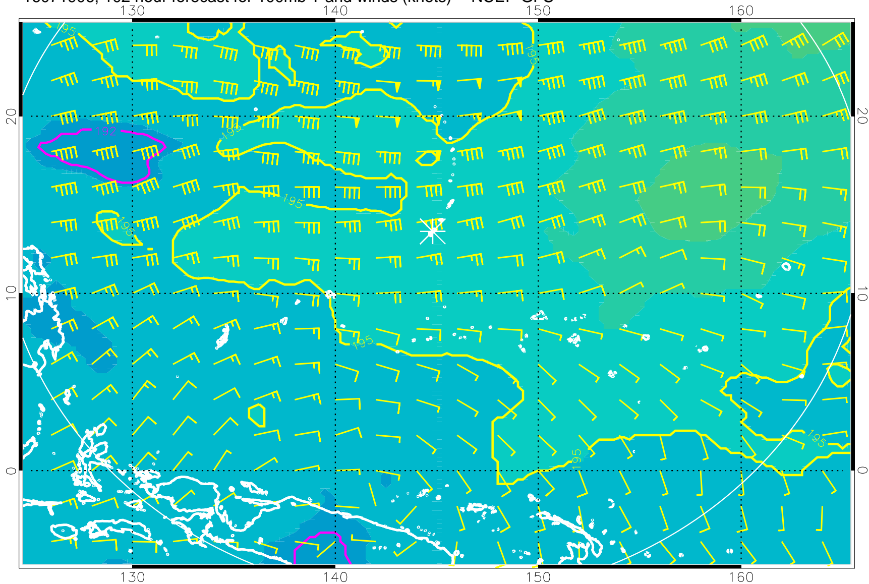
16071906, 102 hour forecast for 100mb T and winds (knots) -- NCEP GFS
