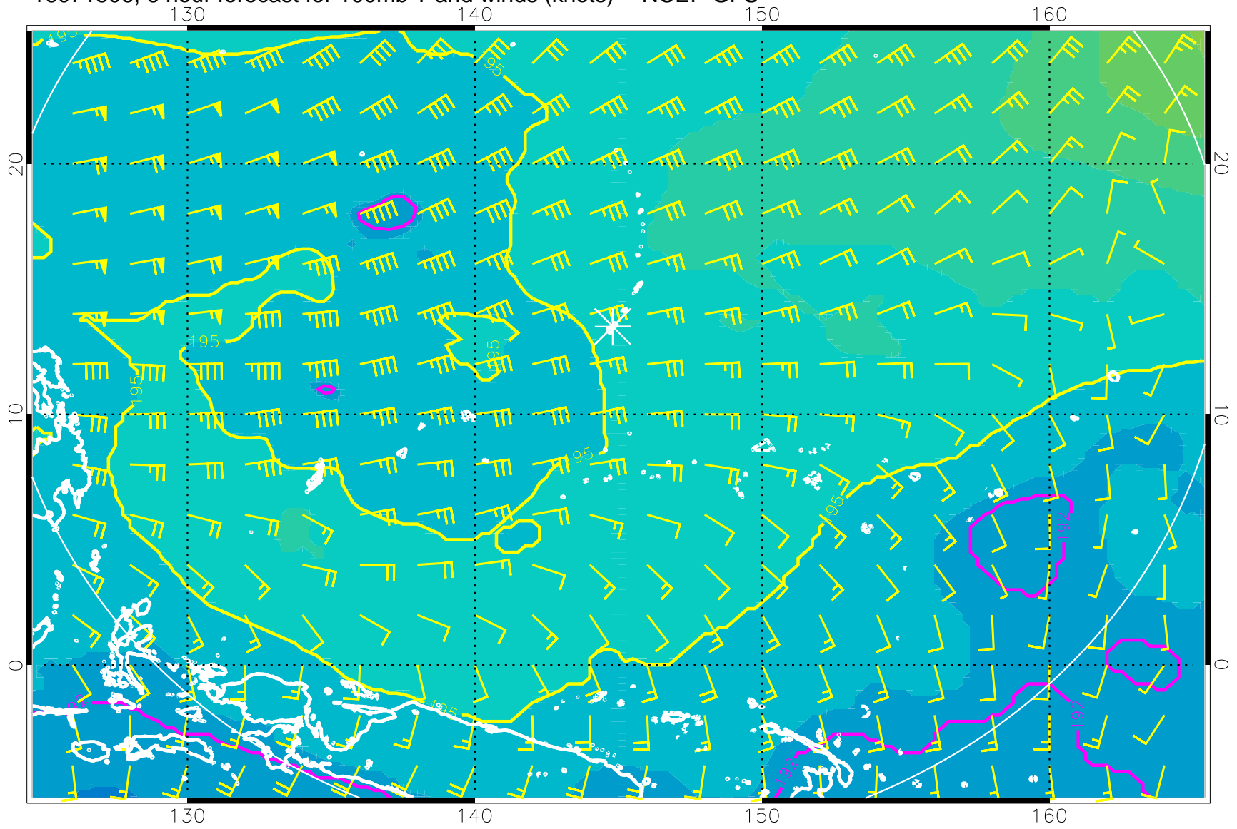
16071506, 6 hour forecast for 100mb T and winds (knots) -- NCEP GFS
