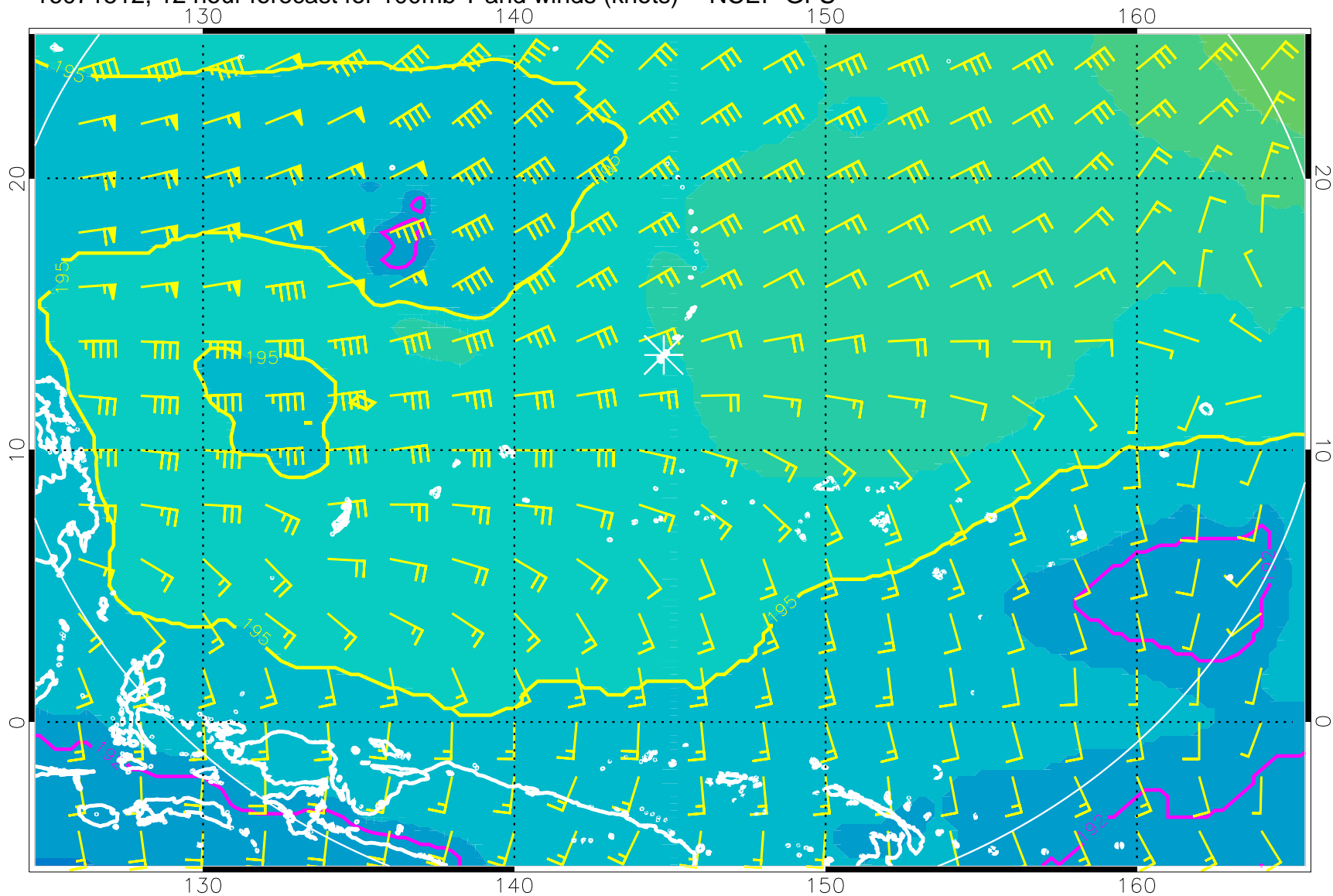
16071512, 12 hour forecast for 100mb T and winds (knots) -- NCEP GFS
