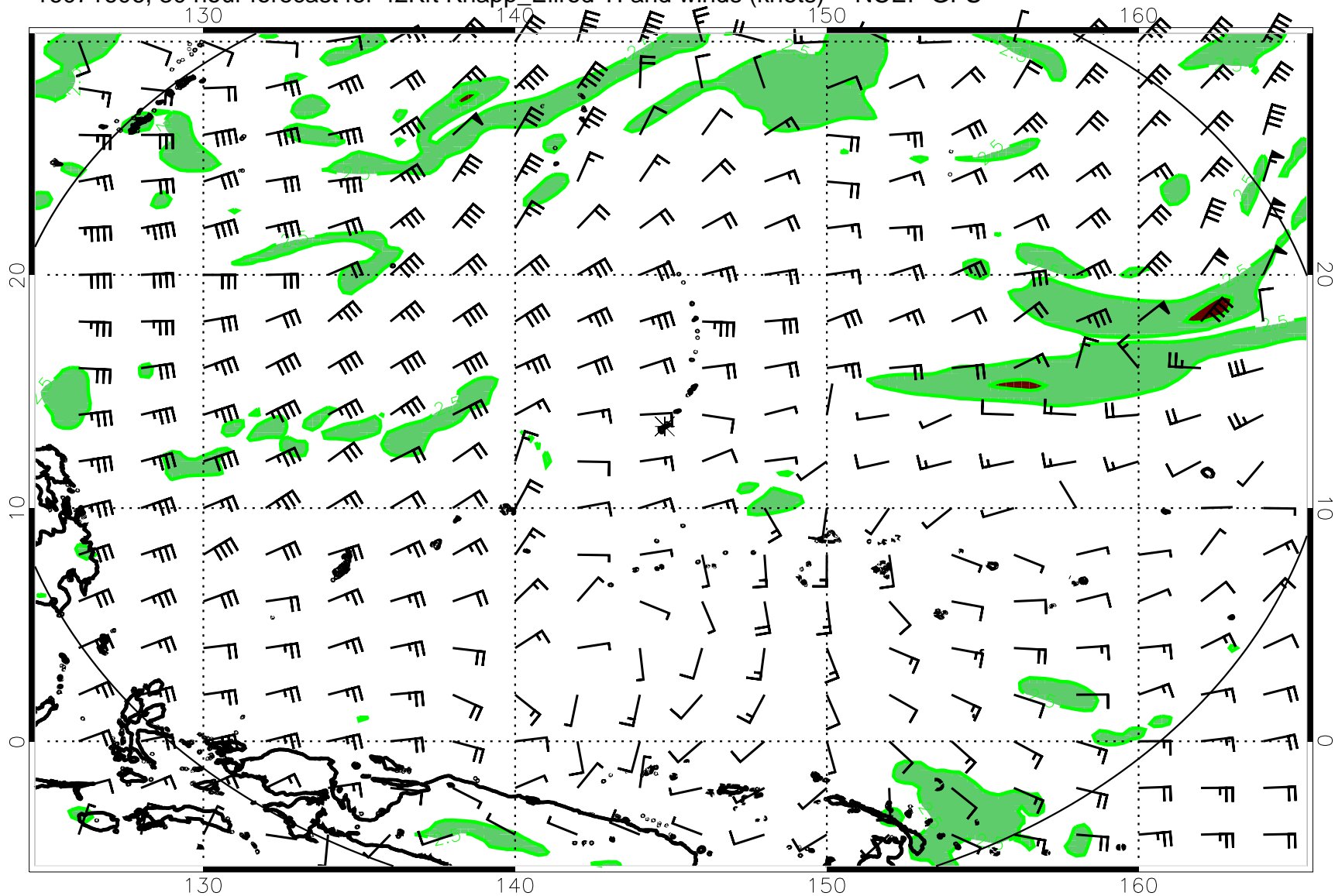
16071606, 30 hour forecast for 42Kft Knapp_Ellrod TI and winds (knots) -- NCEP GFS
