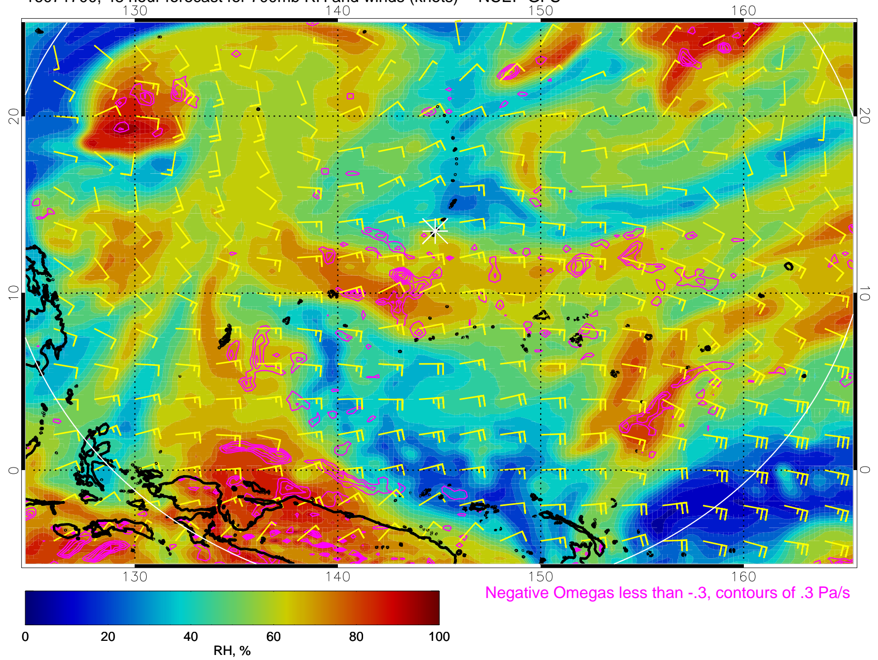
16071700, 48 hour forecast for 700mb RH and winds (knots) -- NCEP GFS
