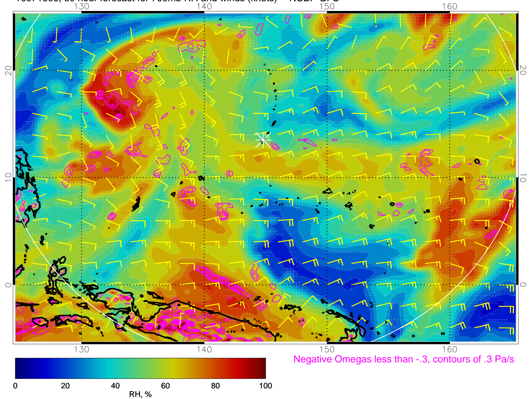
16071606, 30 hour forecast for 700mb RH and winds (knots) -- NCEP GFS
