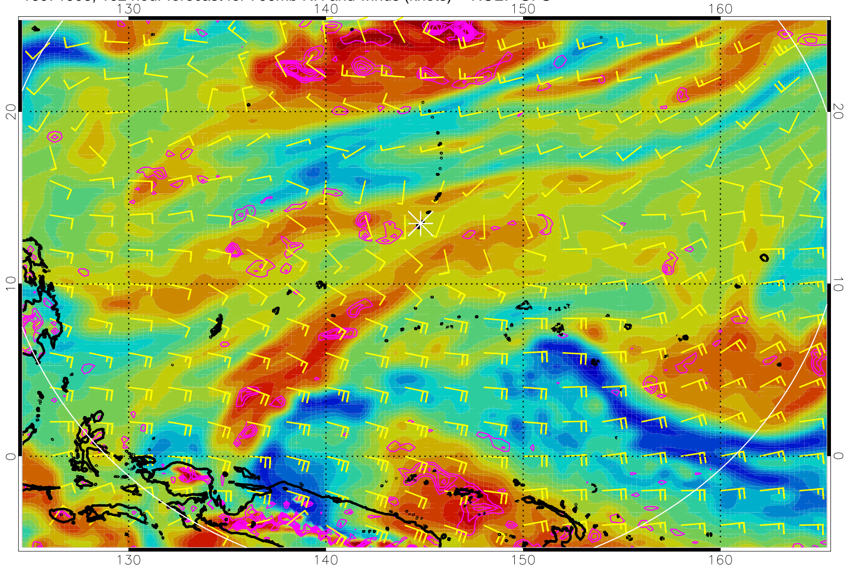
16071906, 102 hour forecast for 700mb RH and winds (knots) -- NCEP GFS
