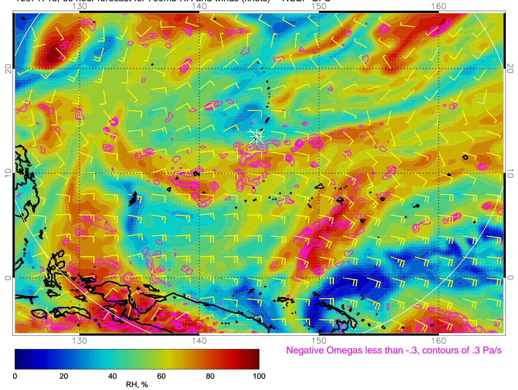
16071718, 66 hour forecast for 700mb RH and winds (knots) -- NCEP GFS
