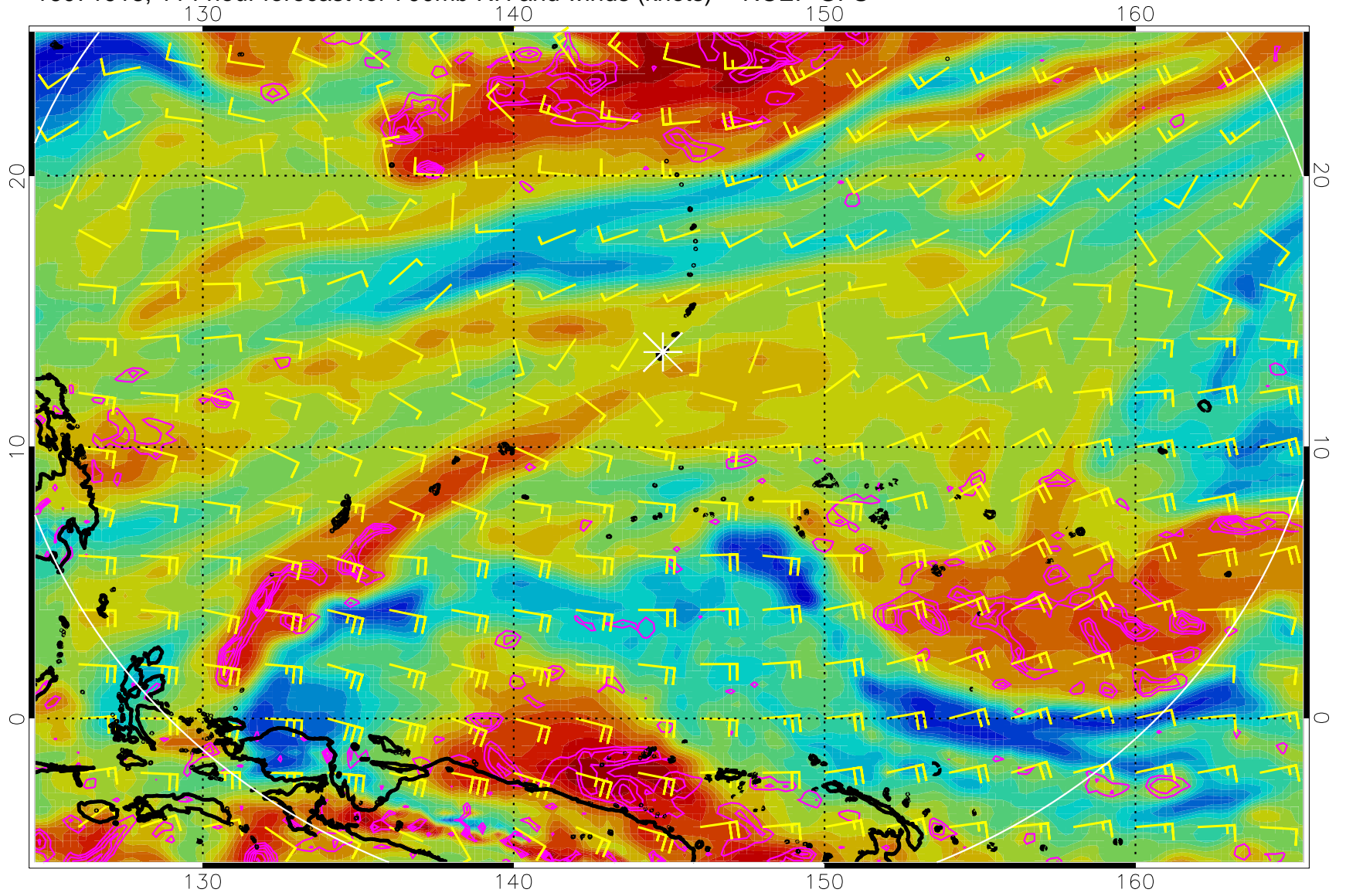
16071918, 114 hour forecast for 700mb RH and winds (knots) -- NCEP GFS
