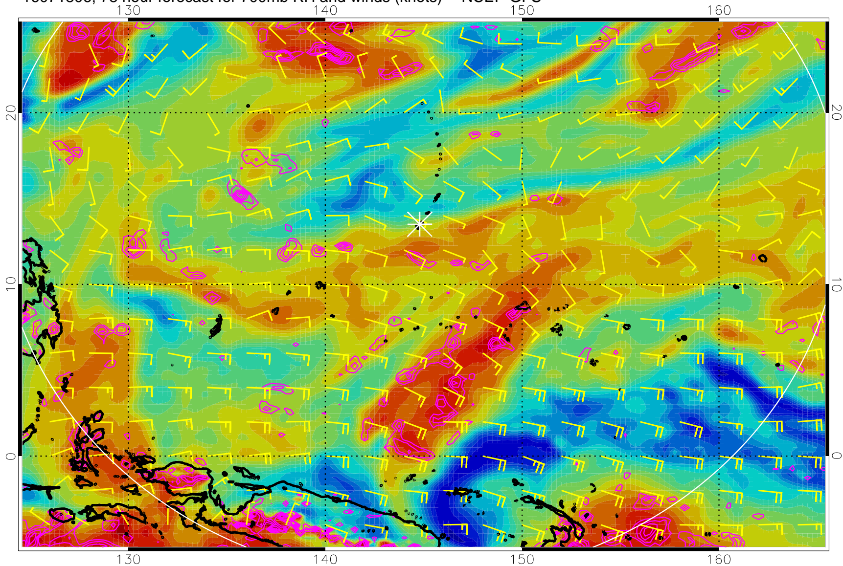
16071806, 78 hour forecast for 700mb RH and winds (knots) -- NCEP GFS
