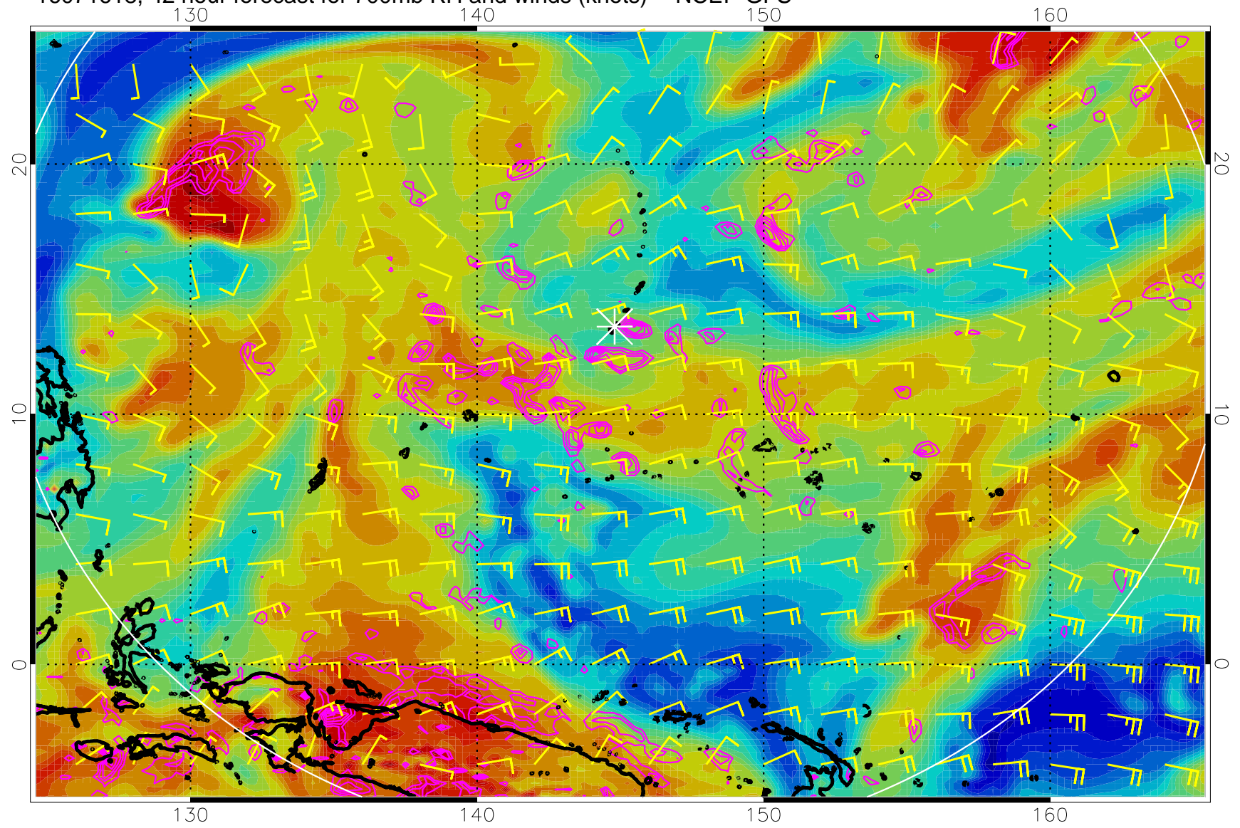
16071618, 42 hour forecast for 700mb RH and winds (knots) -- NCEP GFS
