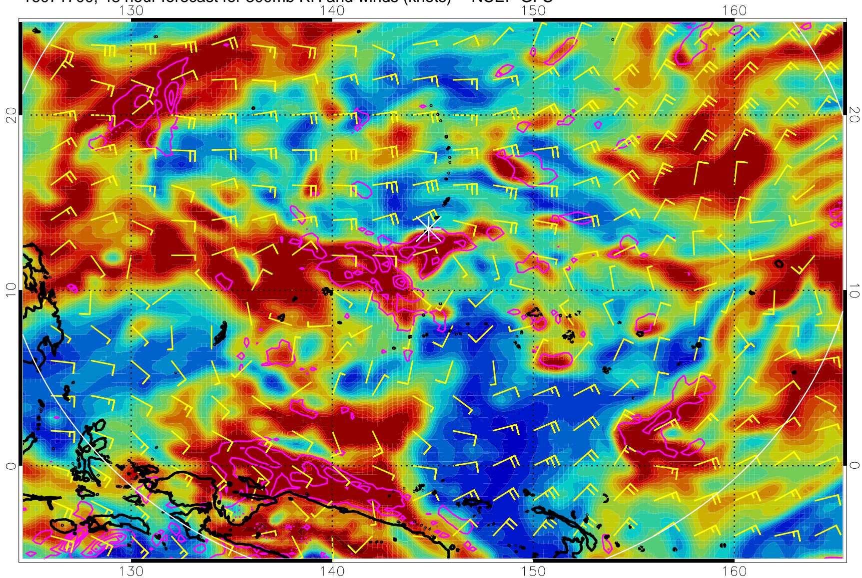
16071700, 48 hour forecast for 300mb RH and winds (knots) -- NCEP GFS
