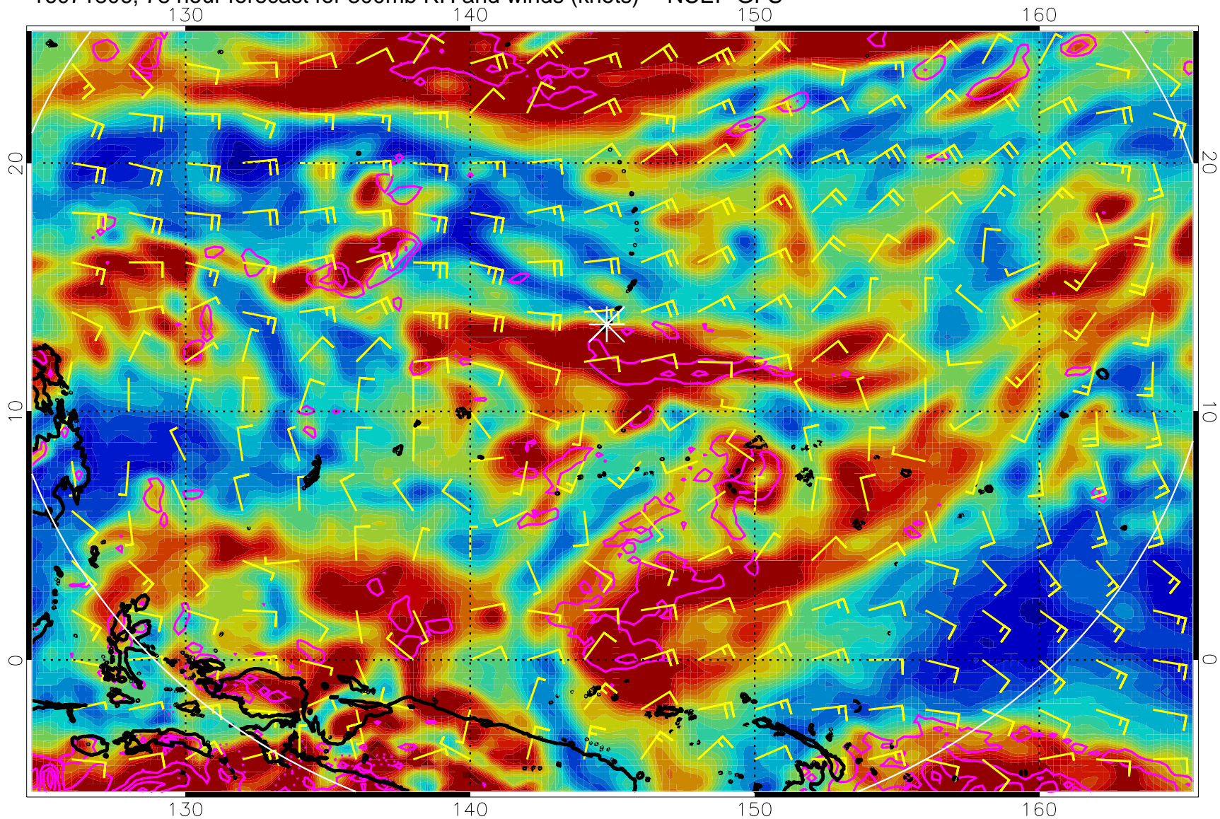
16071806, 78 hour forecast for 300mb RH and winds (knots) -- NCEP GFS
