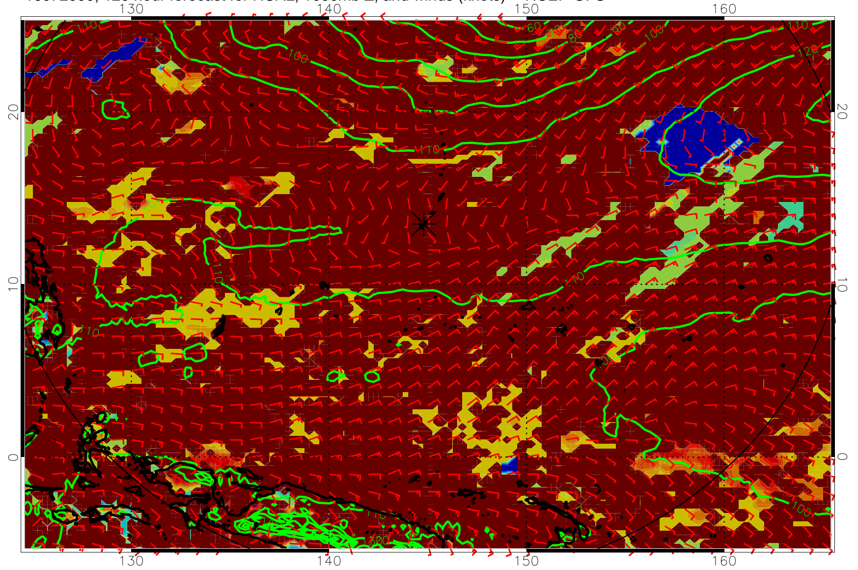
16072000, 120 hour forecast for HCAL, 1000mb Z, and winds (knots) -- NCEP GFS
