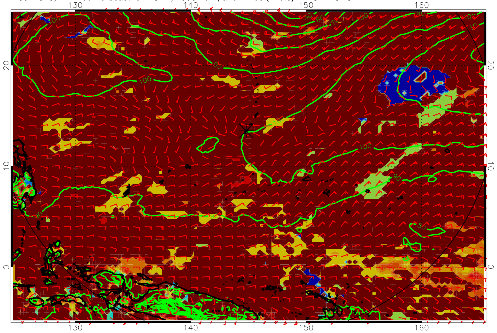
16071918, 114 hour forecast for HCAL, 1000mb Z, and winds (knots) -- NCEP GFS
