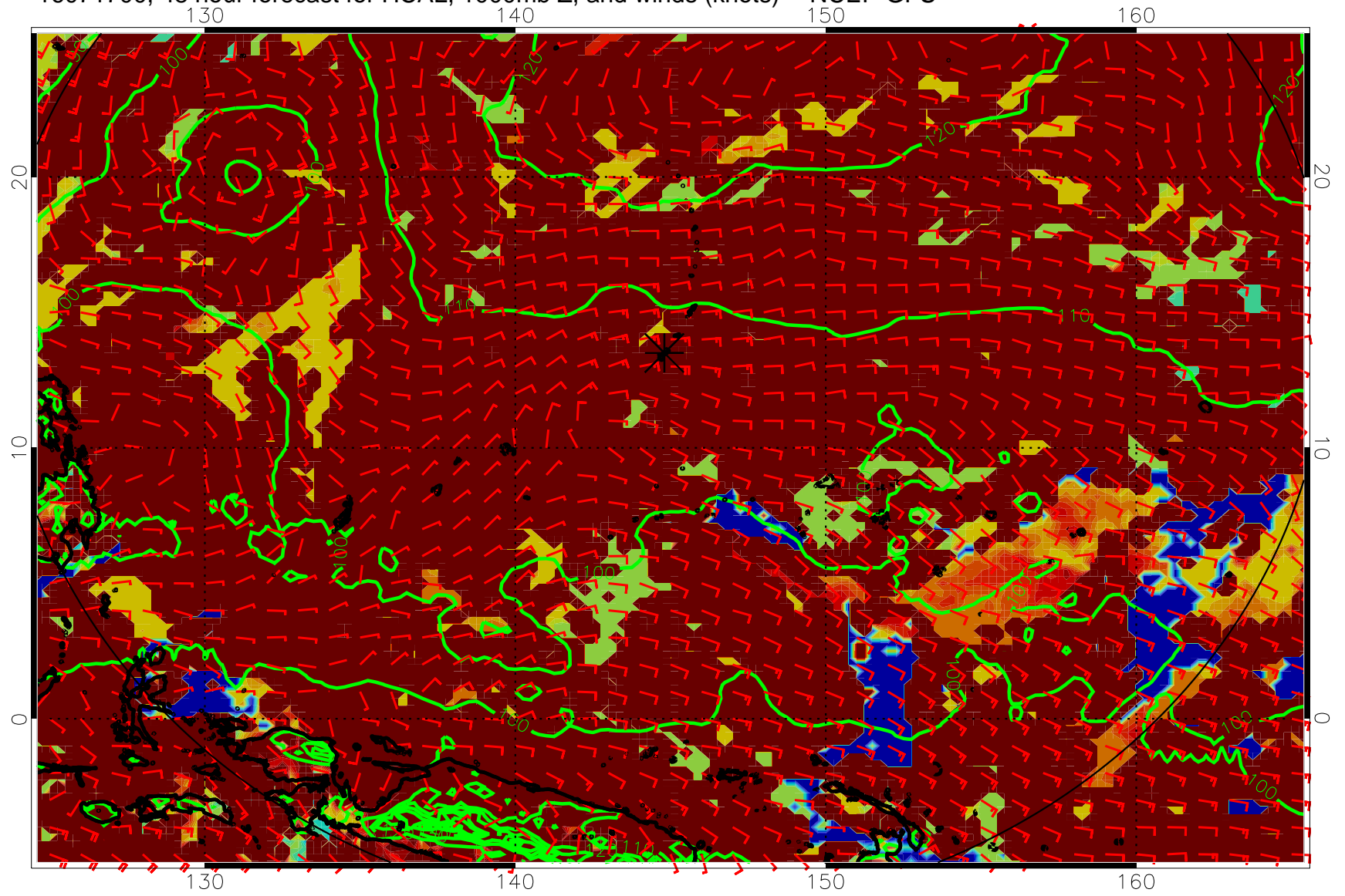
16071700, 48 hour forecast for HCAL, 1000mb Z, and winds (knots) -- NCEP GFS
