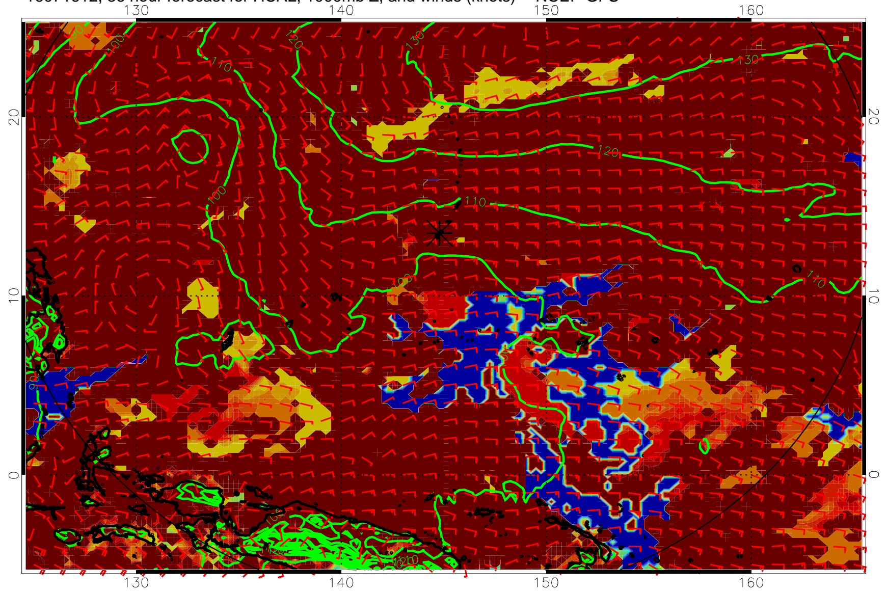
16071612, 36 hour forecast for HCAL, 1000mb Z, and winds (knots) -- NCEP GFS
