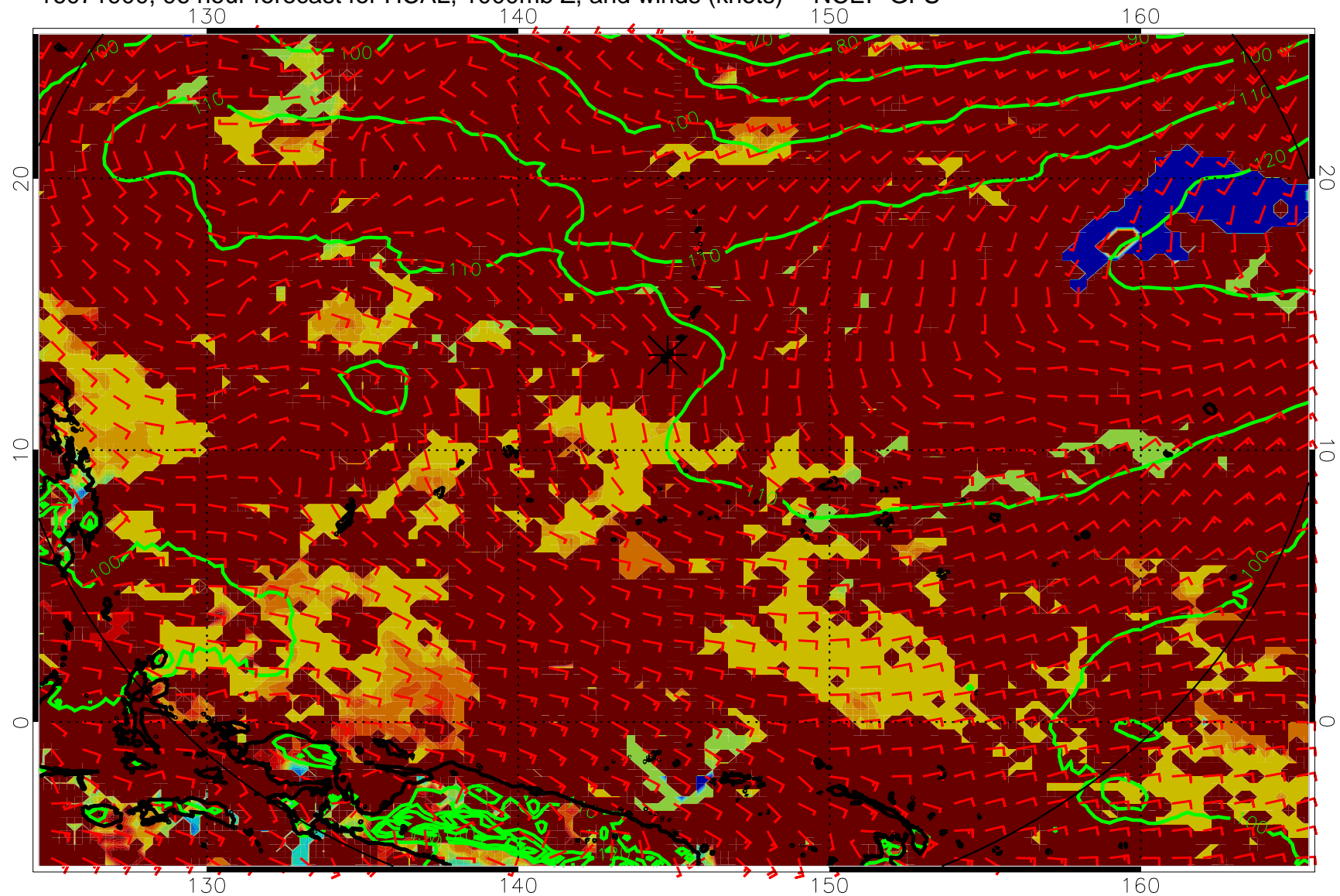
16071900, 96 hour forecast for HCAL, 1000mb Z, and winds (knots) -- NCEP GFS
