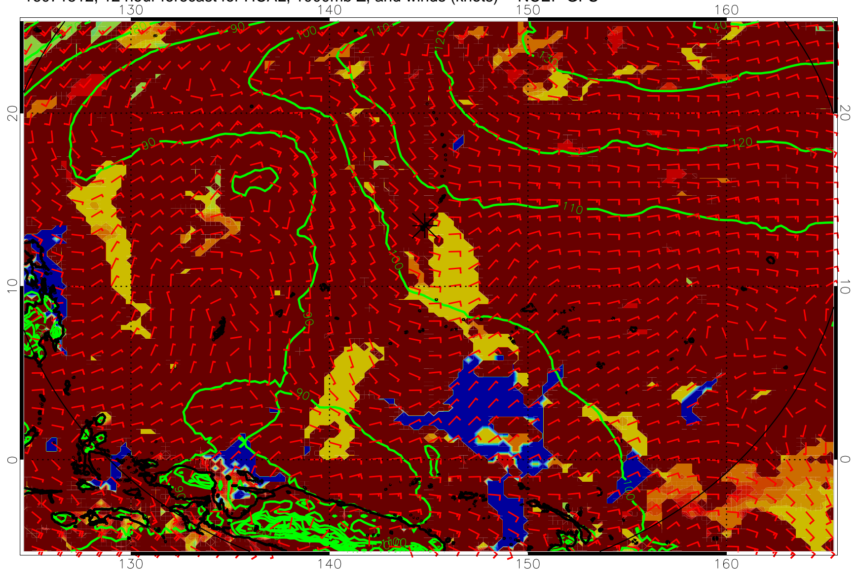
16071512, 12 hour forecast for HCAL, 1000mb Z, and winds (knots) -- NCEP GFS
