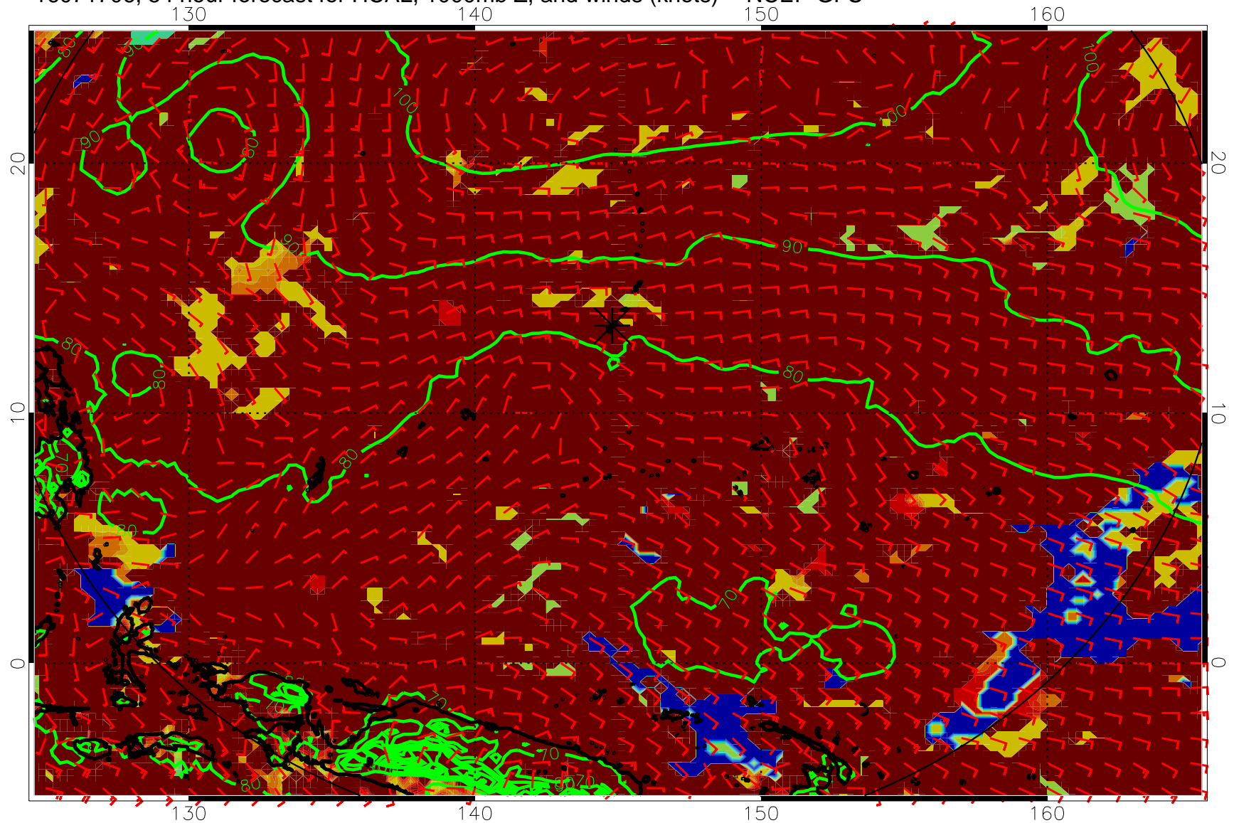
16071706, 54 hour forecast for HCAL, 1000mb Z, and winds (knots) -- NCEP GFS
