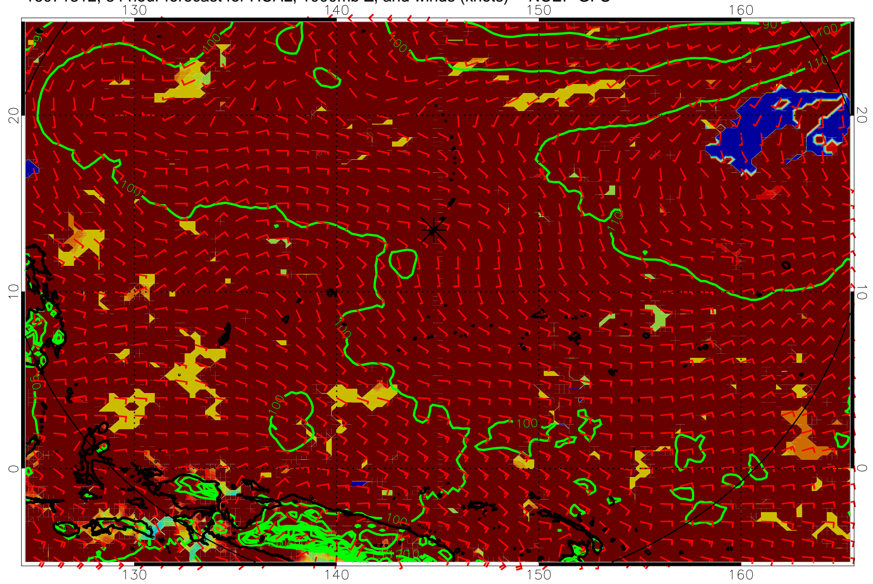
16071812, 84 hour forecast for HCAL, 1000mb Z, and winds (knots) -- NCEP GFS
