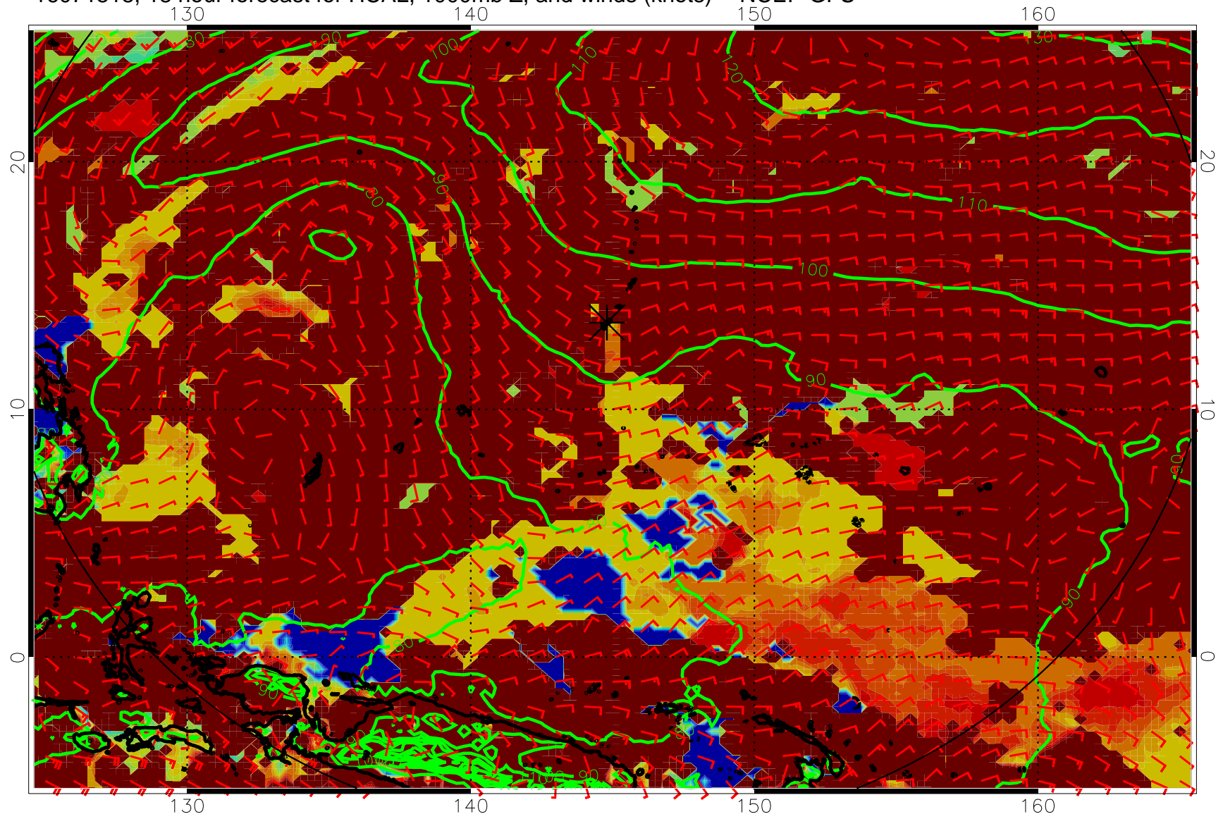
16071518, 18 hour forecast for HCAL, 1000mb Z, and winds (knots) -- NCEP GFS
