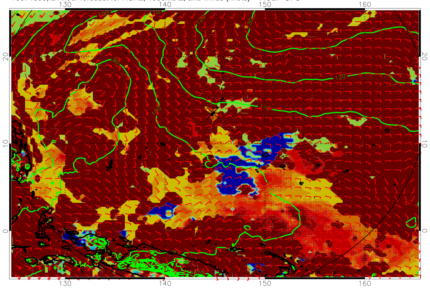
16071600, 24 hour forecast for HCAL, 1000mb Z, and winds (knots) -- NCEP GFS
