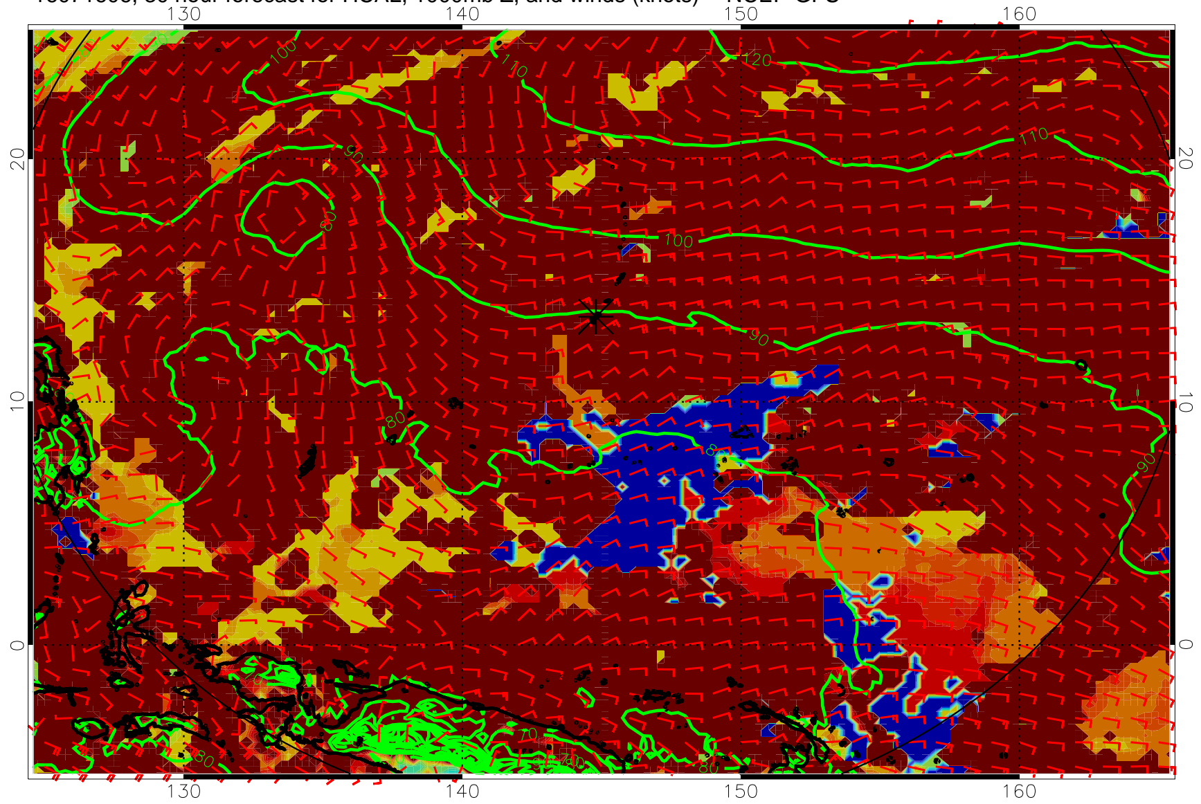
16071606, 30 hour forecast for HCAL, 1000mb Z, and winds (knots) -- NCEP GFS
