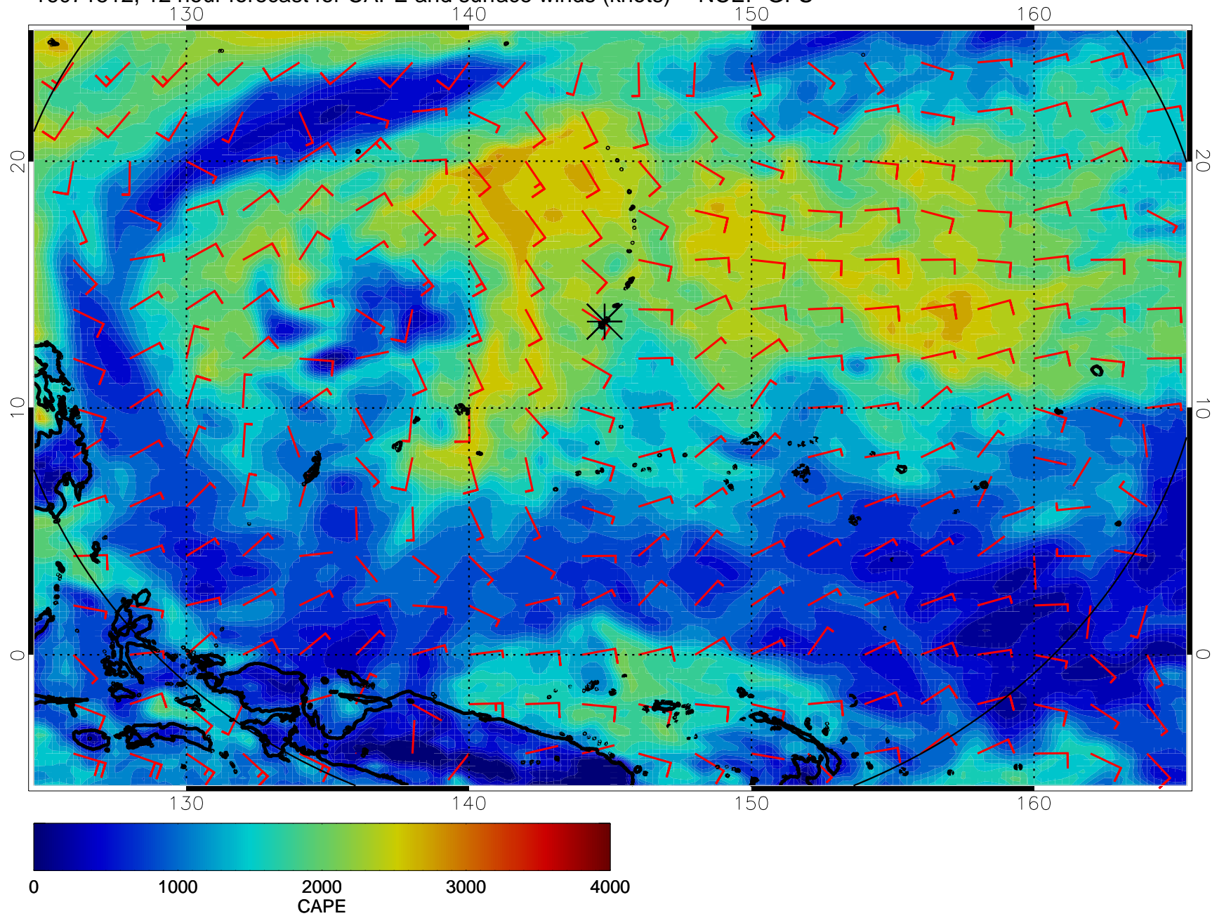
16071512, 12 hour forecast for CAPE and surface winds (knots) -- NCEP GFS
