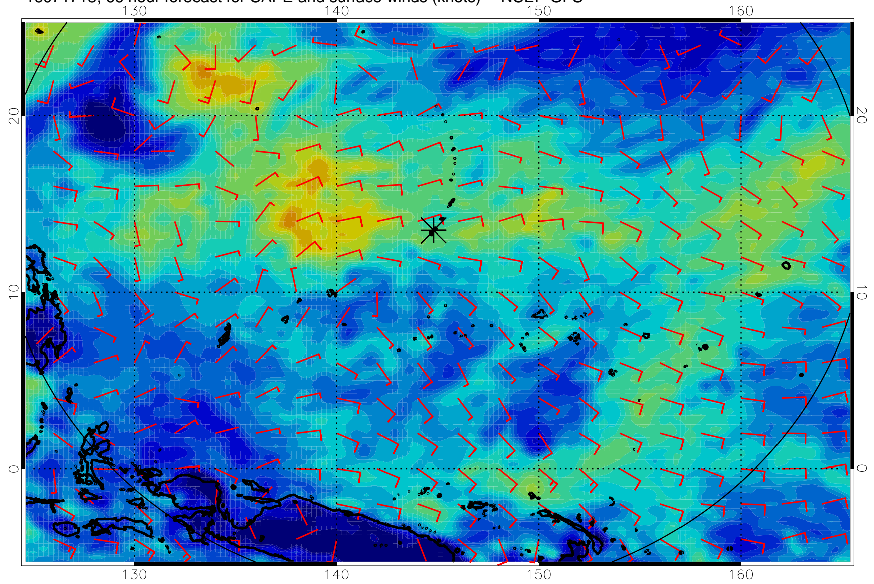
16071718, 66 hour forecast for CAPE and surface winds (knots) -- NCEP GFS
