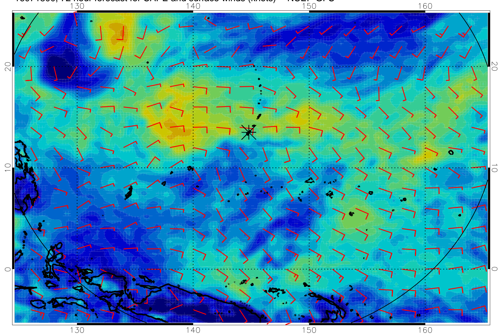
16071800, 72 hour forecast for CAPE and surface winds (knots) -- NCEP GFS
