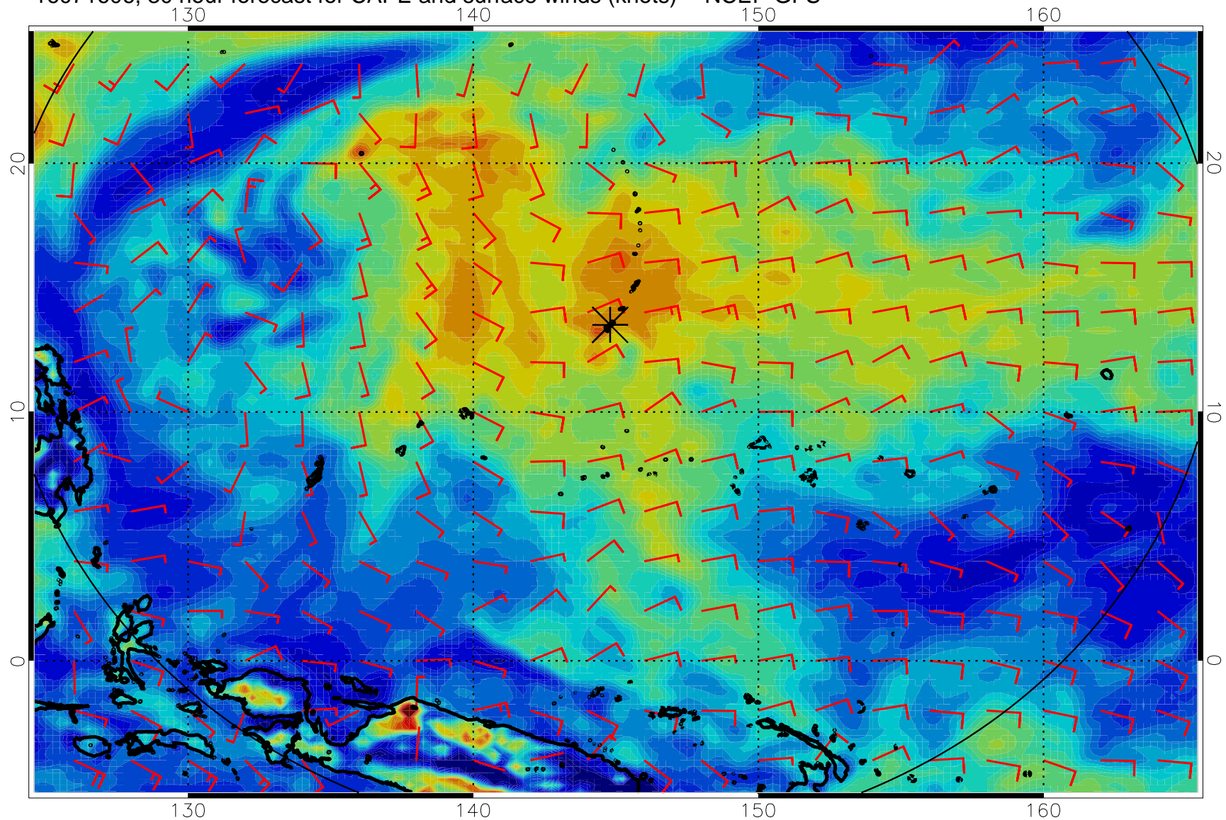
16071606, 30 hour forecast for CAPE and surface winds (knots) -- NCEP GFS
