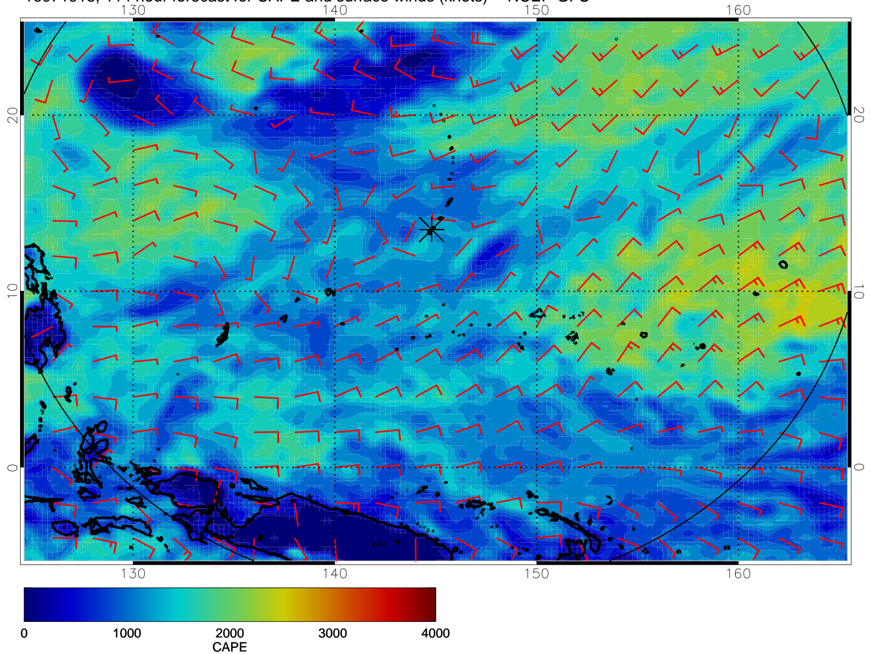
16071918, 114 hour forecast for CAPE and surface winds (knots) -- NCEP GFS
