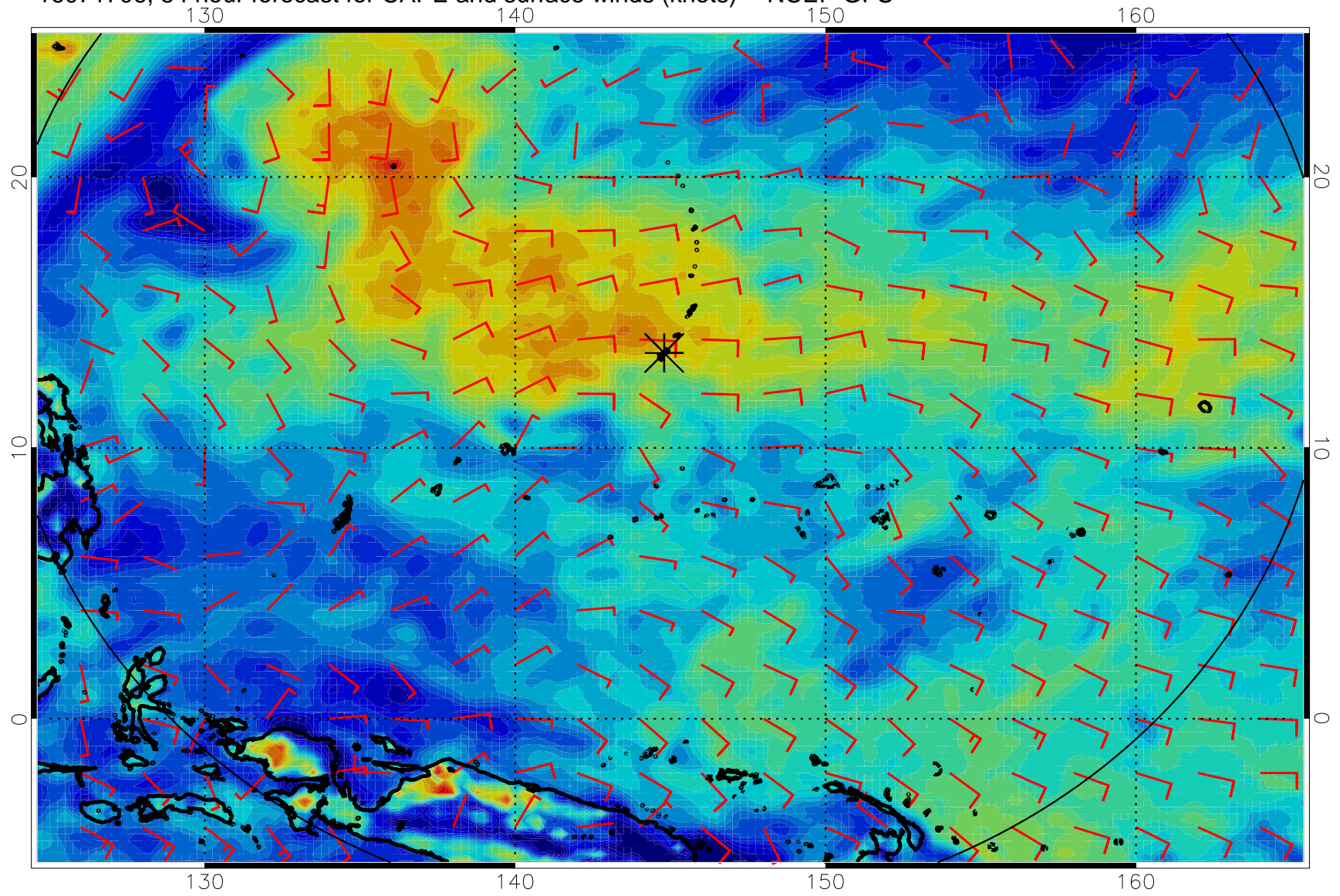
16071706, 54 hour forecast for CAPE and surface winds (knots) -- NCEP GFS
