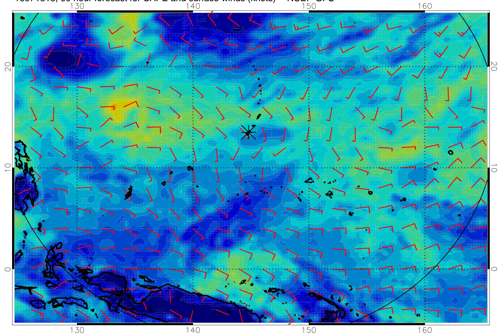
16071818, 90 hour forecast for CAPE and surface winds (knots) -- NCEP GFS
