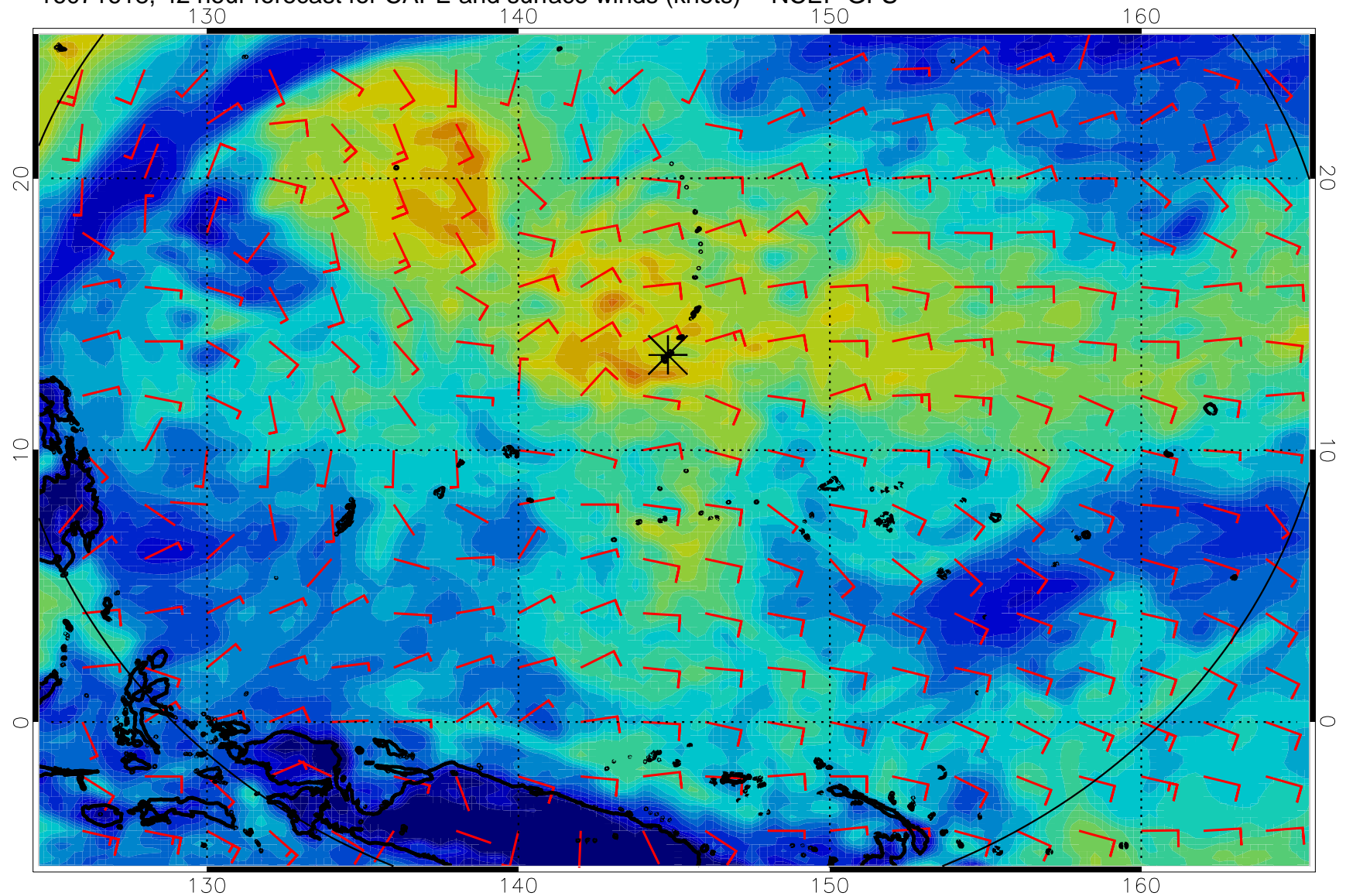
16071618, 42 hour forecast for CAPE and surface winds (knots) -- NCEP GFS
