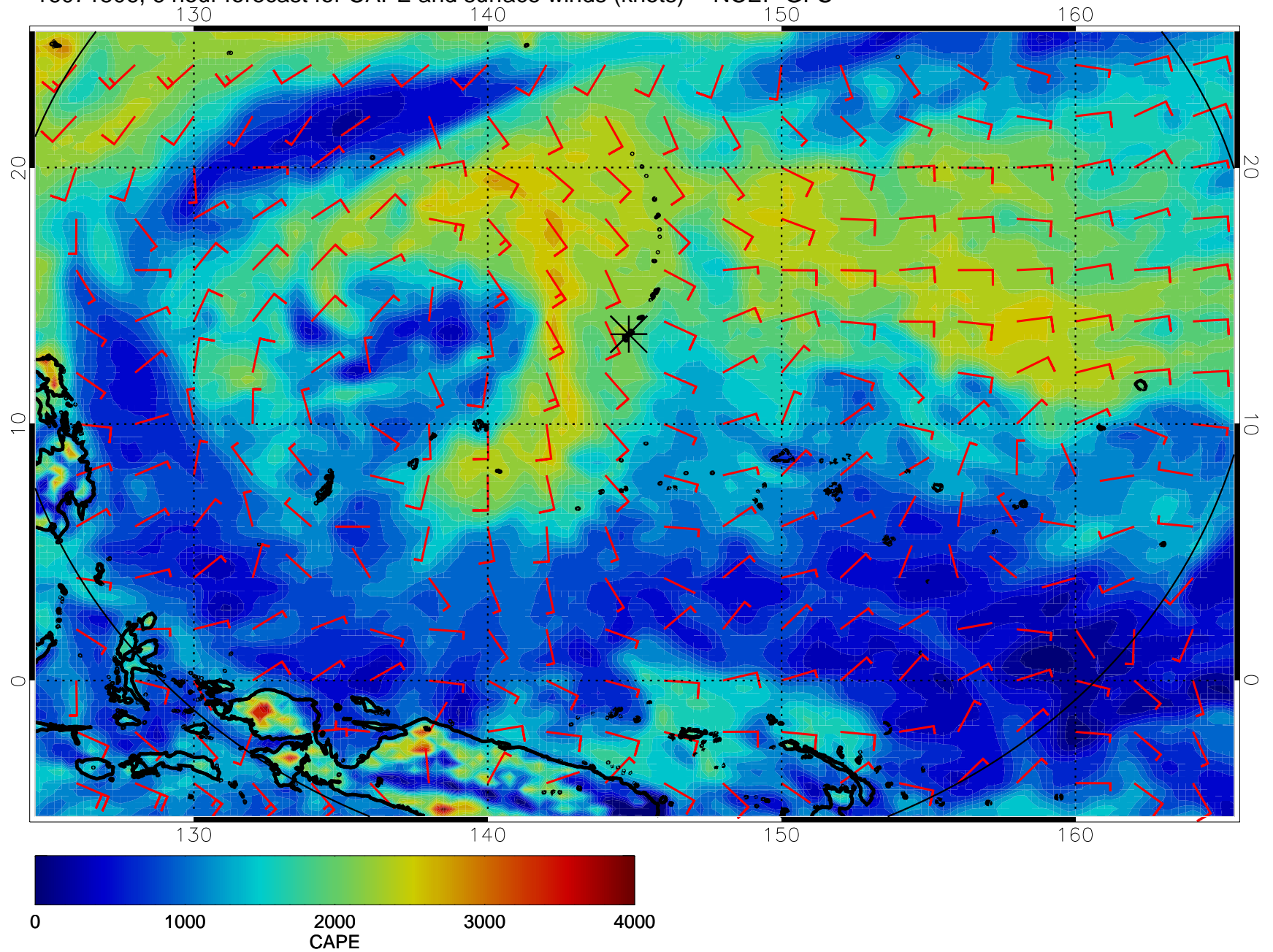
16071506, 6 hour forecast for CAPE and surface winds (knots) -- NCEP GFS
