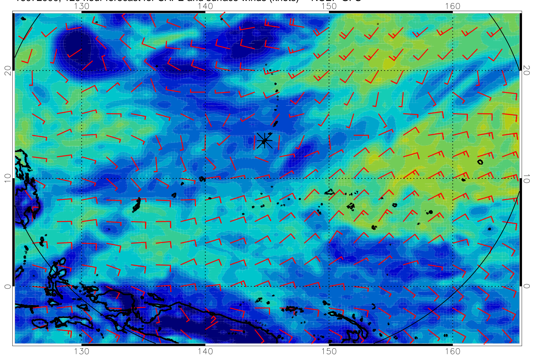
16072000, 120 hour forecast for CAPE and surface winds (knots) -- NCEP GFS
