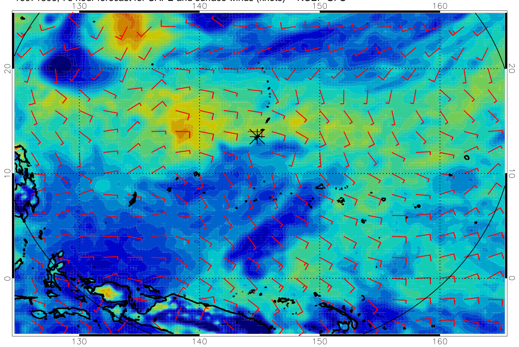
16071806, 78 hour forecast for CAPE and surface winds (knots) -- NCEP GFS
