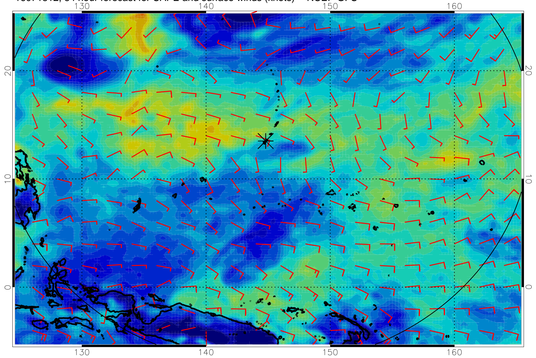
16071812, 84 hour forecast for CAPE and surface winds (knots) -- NCEP GFS
