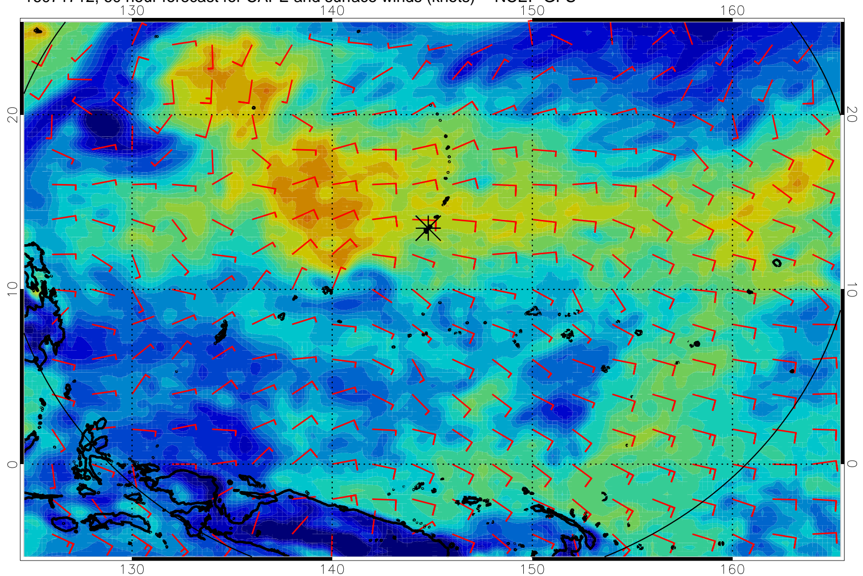
16071712, 60 hour forecast for CAPE and surface winds (knots) -- NCEP GFS
