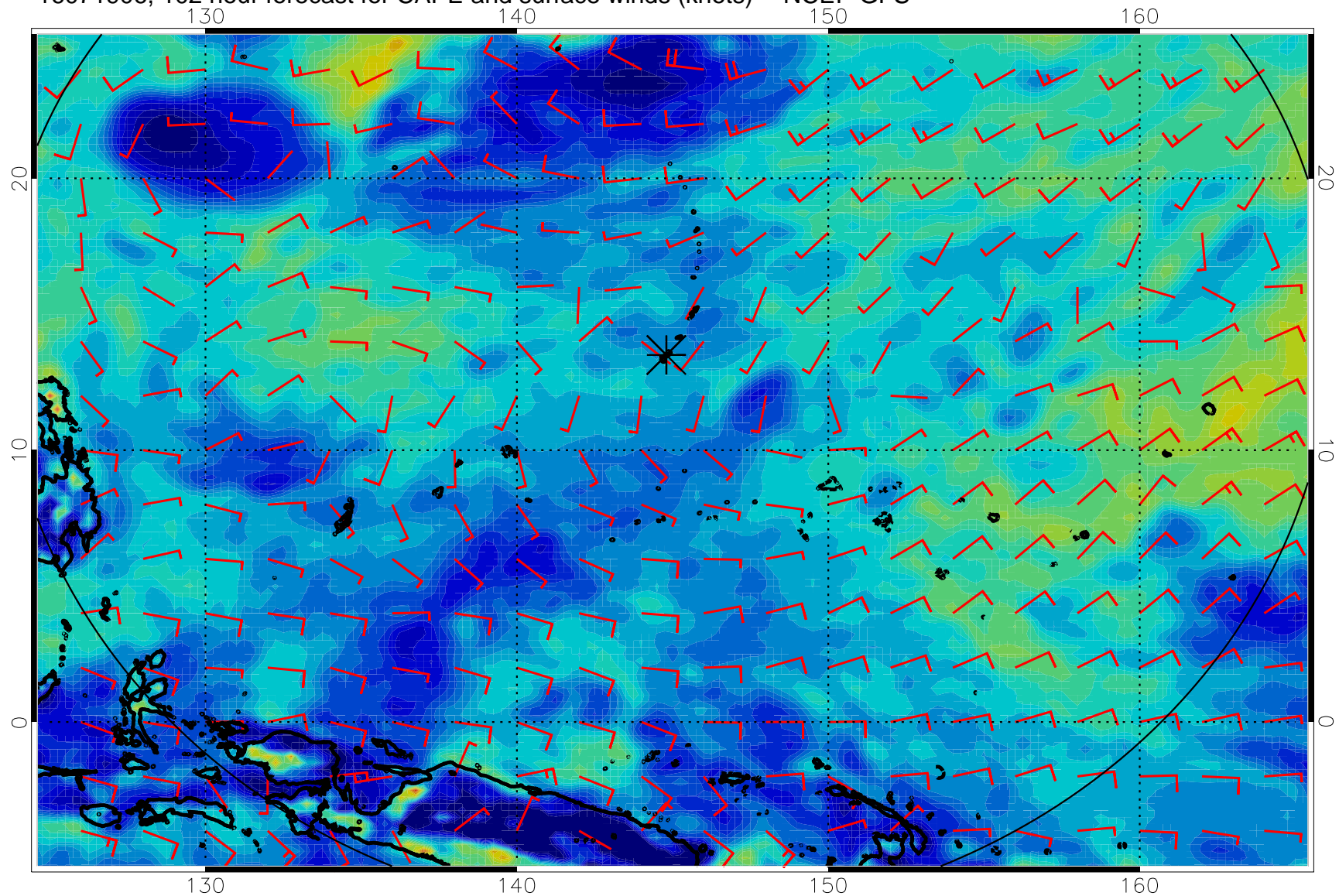
16071906, 102 hour forecast for CAPE and surface winds (knots) -- NCEP GFS
