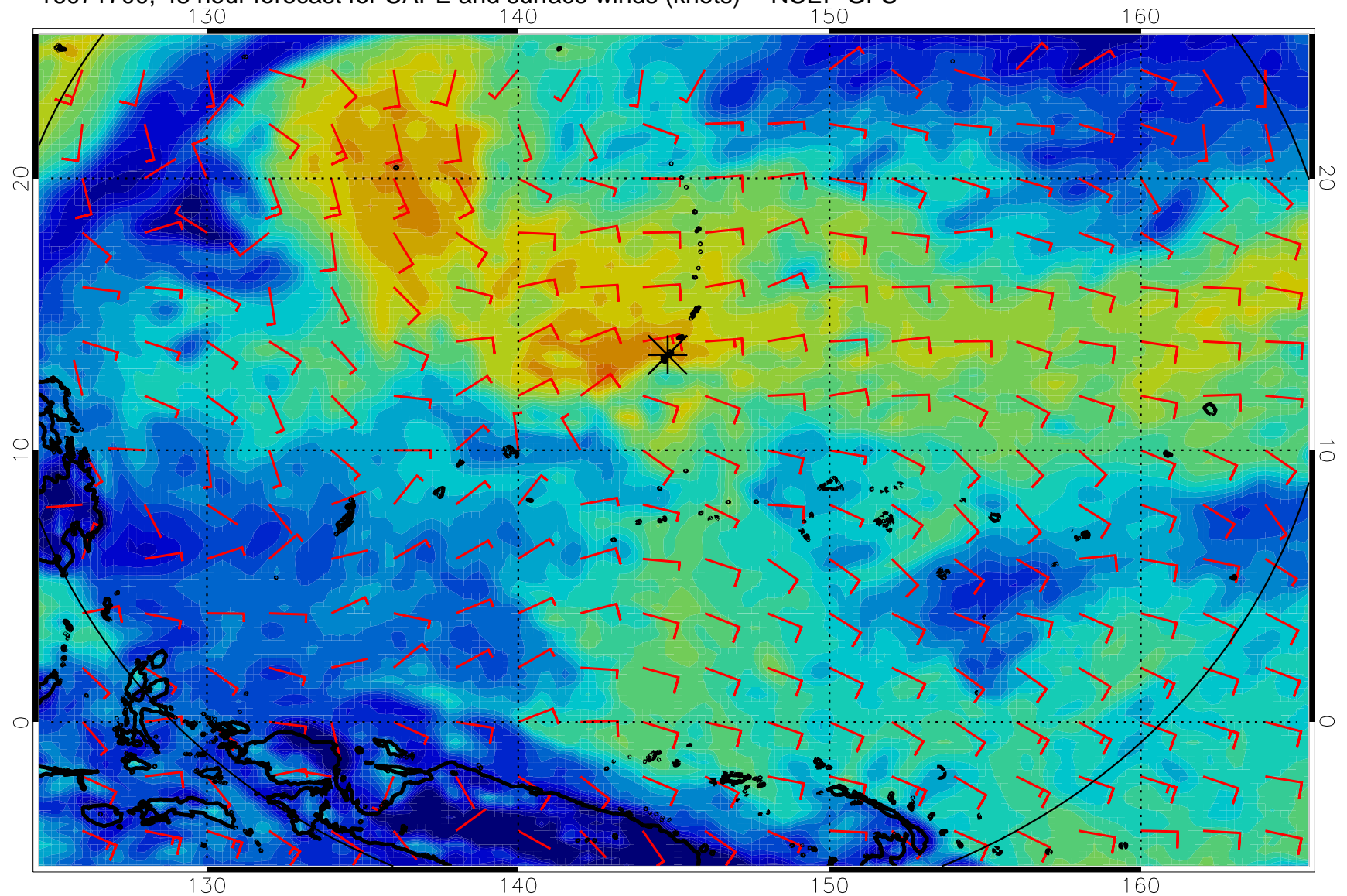
16071700, 48 hour forecast for CAPE and surface winds (knots) -- NCEP GFS
