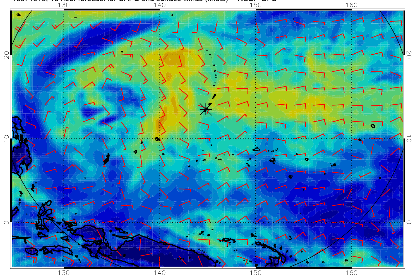
16071518, 18 hour forecast for CAPE and surface winds (knots) -- NCEP GFS
