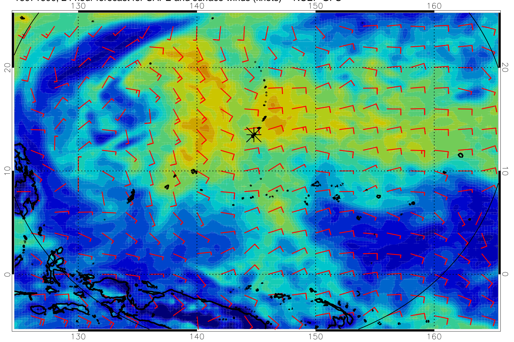
16071600, 24 hour forecast for CAPE and surface winds (knots) -- NCEP GFS
