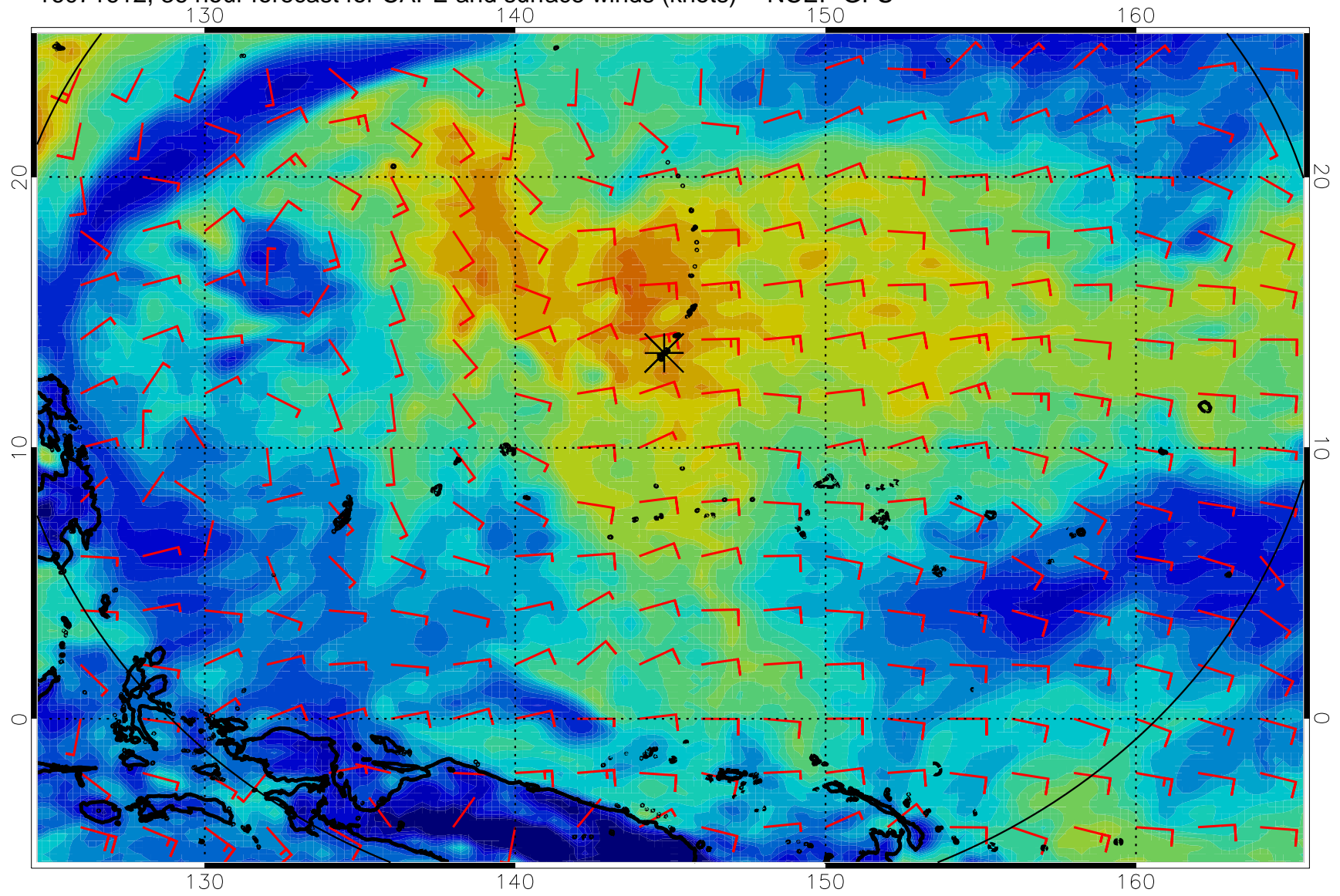
16071612, 36 hour forecast for CAPE and surface winds (knots) -- NCEP GFS
