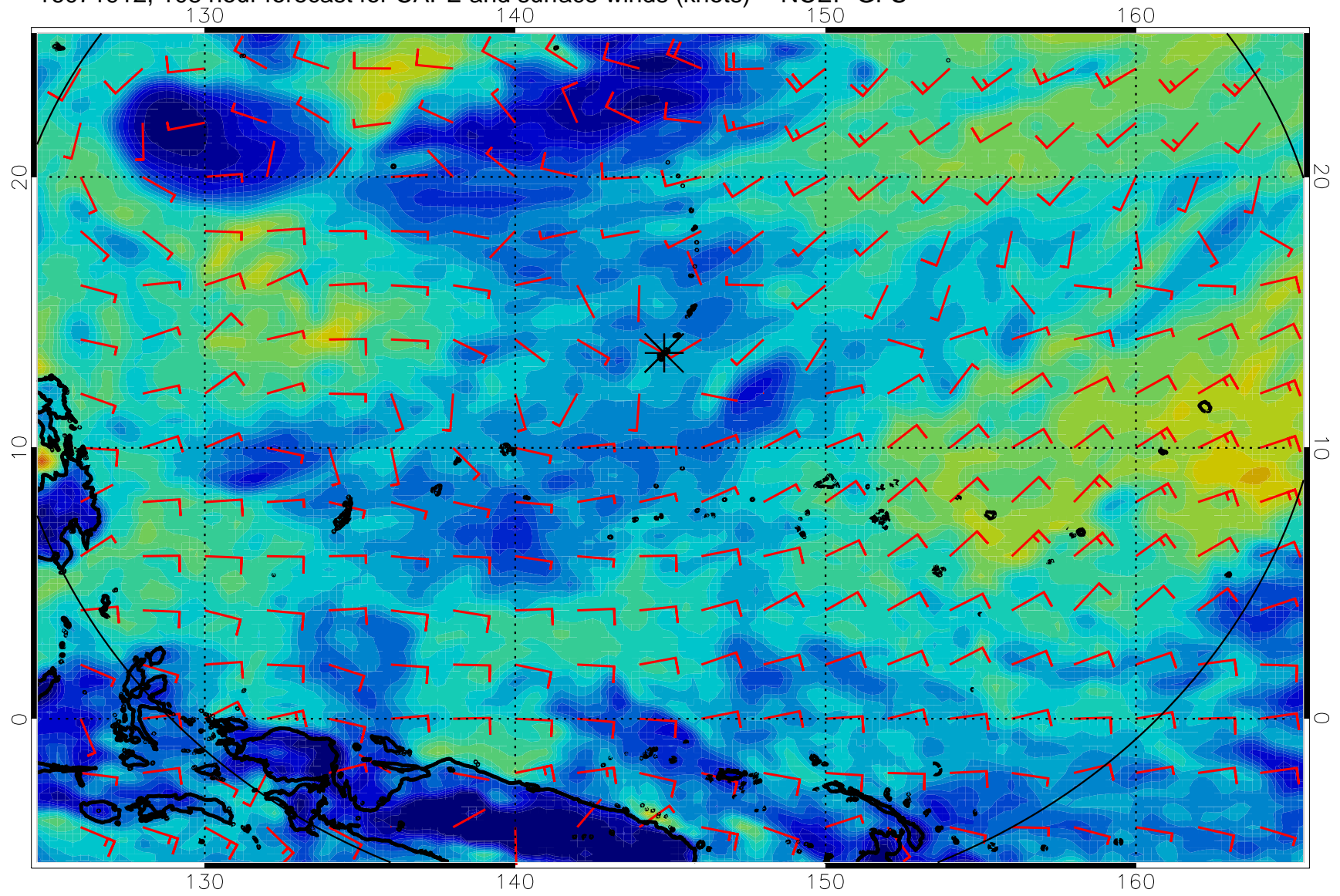
16071912, 108 hour forecast for CAPE and surface winds (knots) -- NCEP GFS
