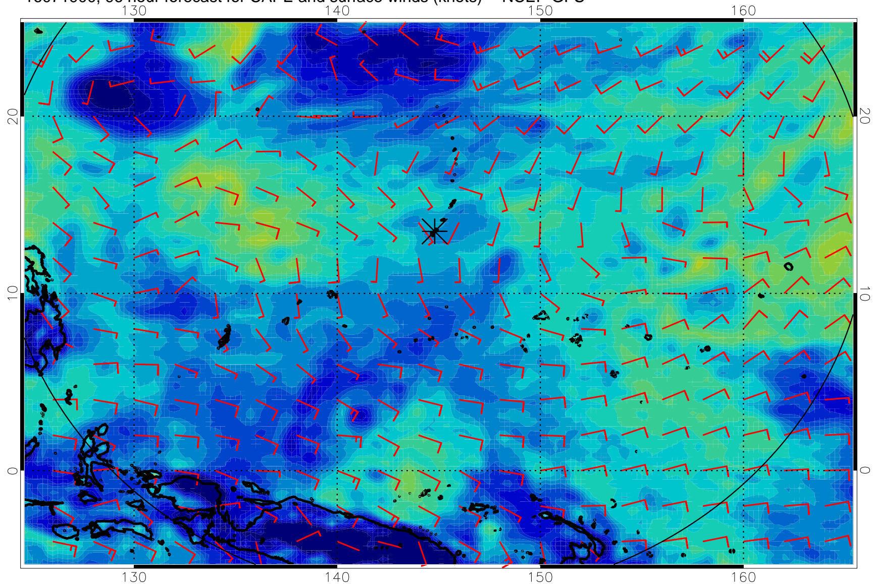
16071900, 96 hour forecast for CAPE and surface winds (knots) -- NCEP GFS
