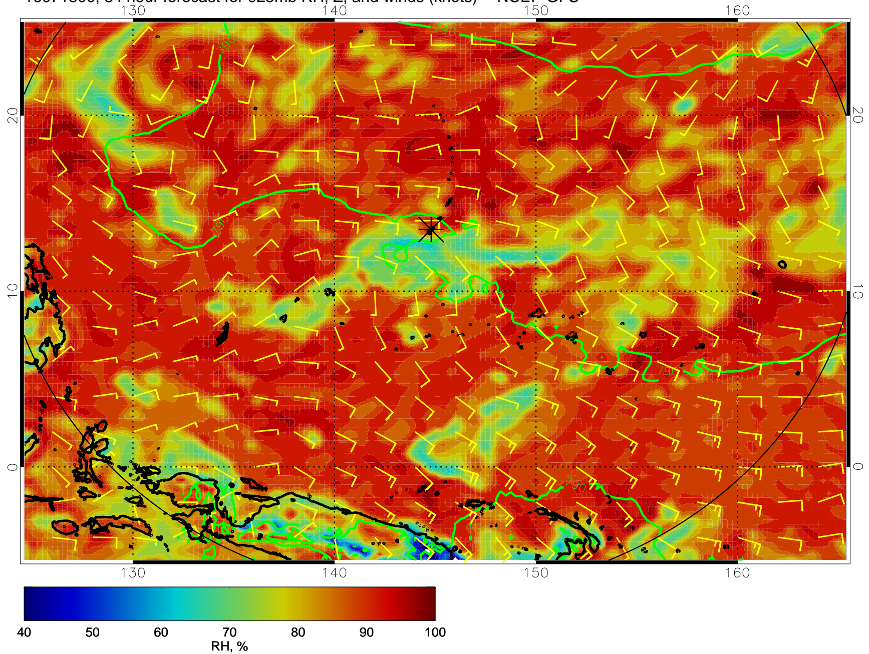
16071800, 84 hour forecast for 925mb RH, Z, and winds (knots) -- NCEP GFS
