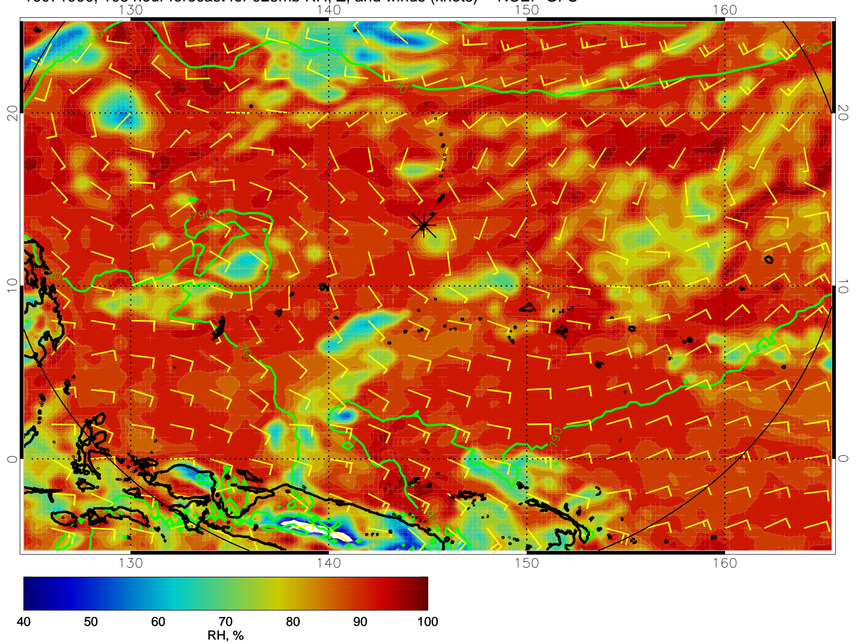
16071900, 108 hour forecast for 925mb RH, Z, and winds (knots) -- NCEP GFS
