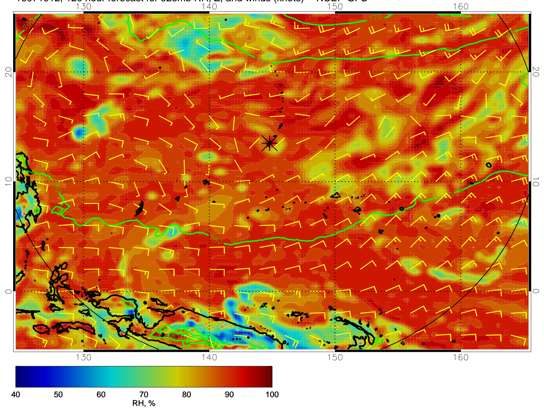
16071912, 120 hour forecast for 925mb RH, Z, and winds (knots) -- NCEP GFS
