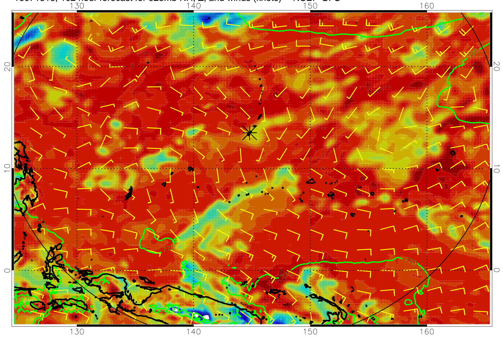
16071818, 102 hour forecast for 925mb RH, Z, and winds (knots) -- NCEP GFS
