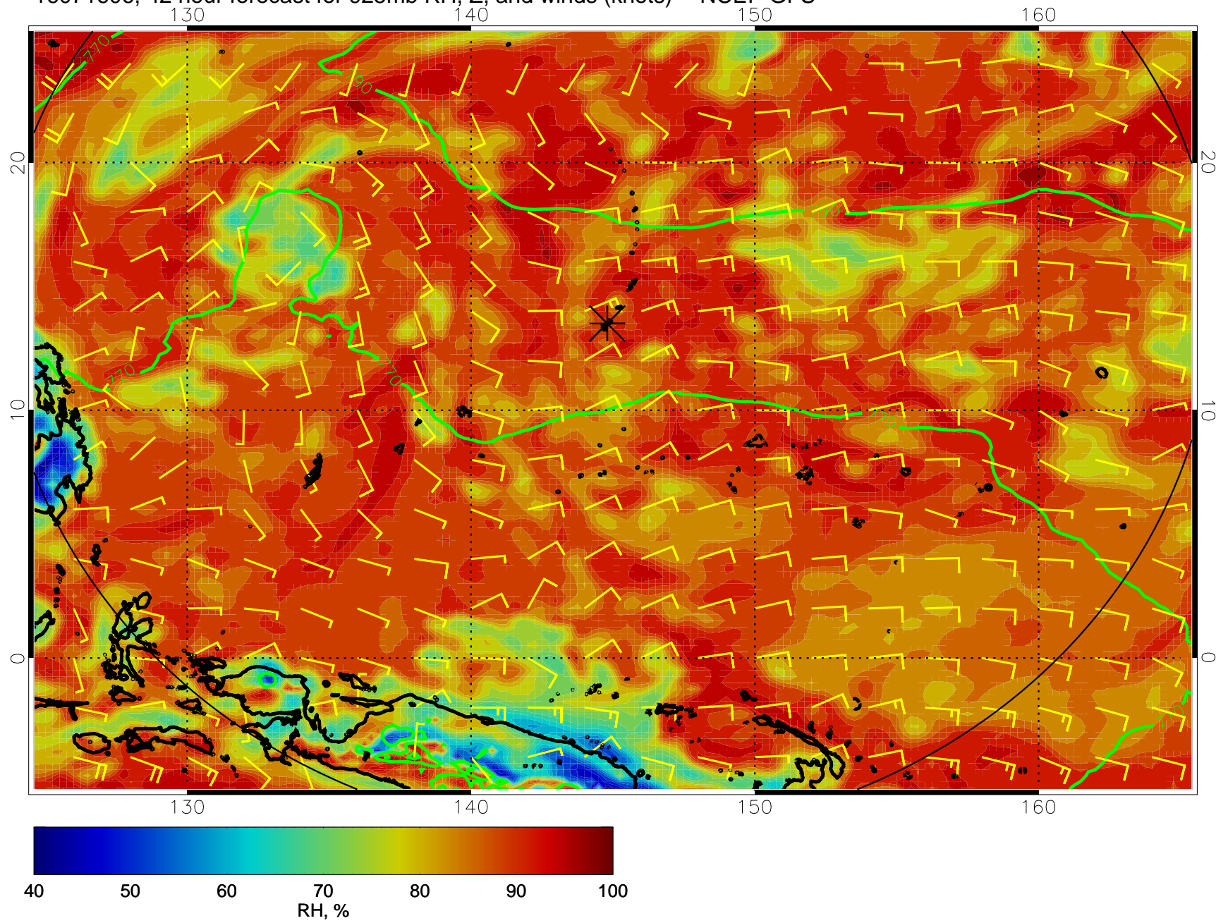
16071606, 42 hour forecast for 925mb RH, Z, and winds (knots) -- NCEP GFS
