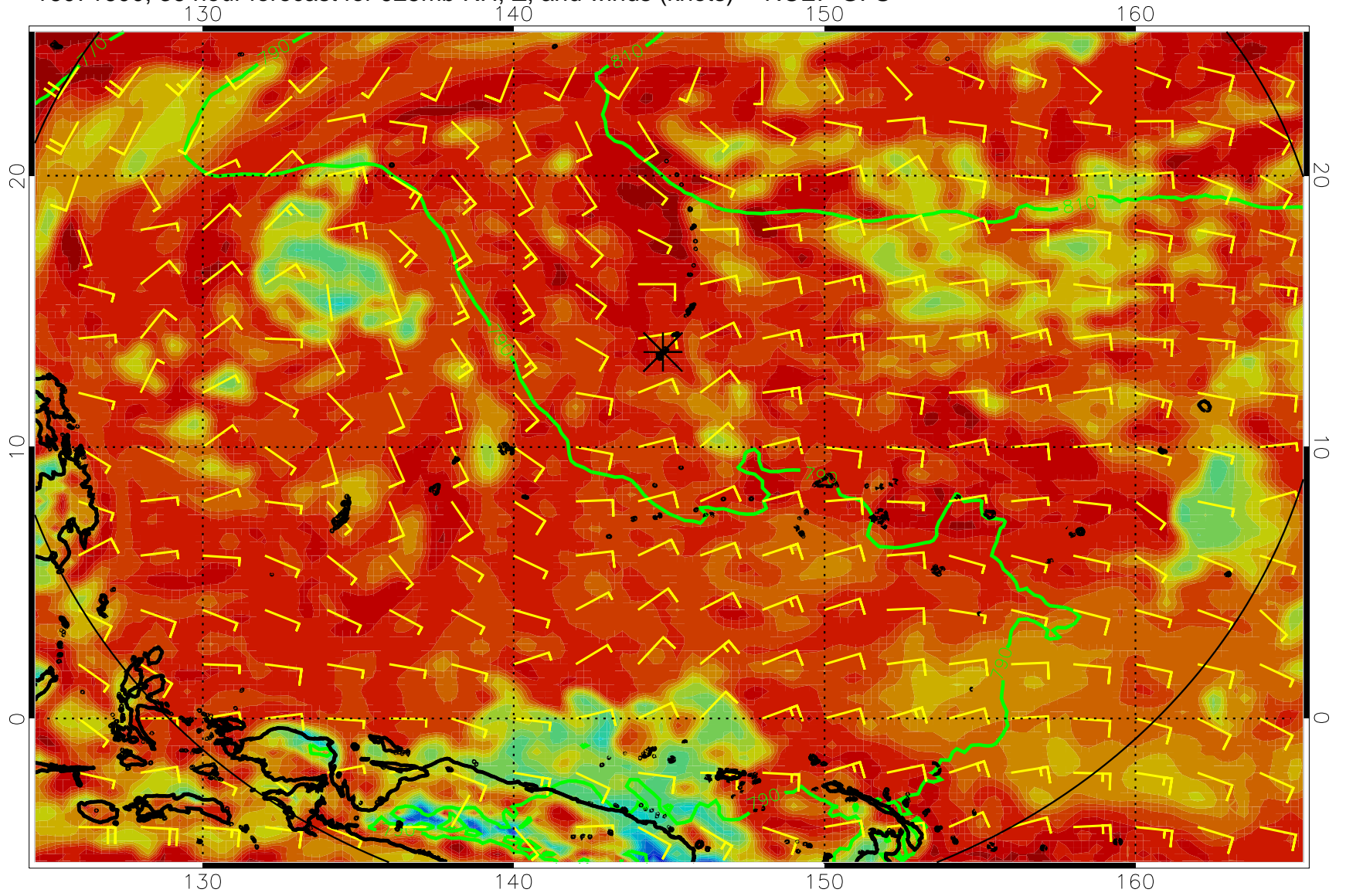
16071600, 36 hour forecast for 925mb RH, Z, and winds (knots) -- NCEP GFS
