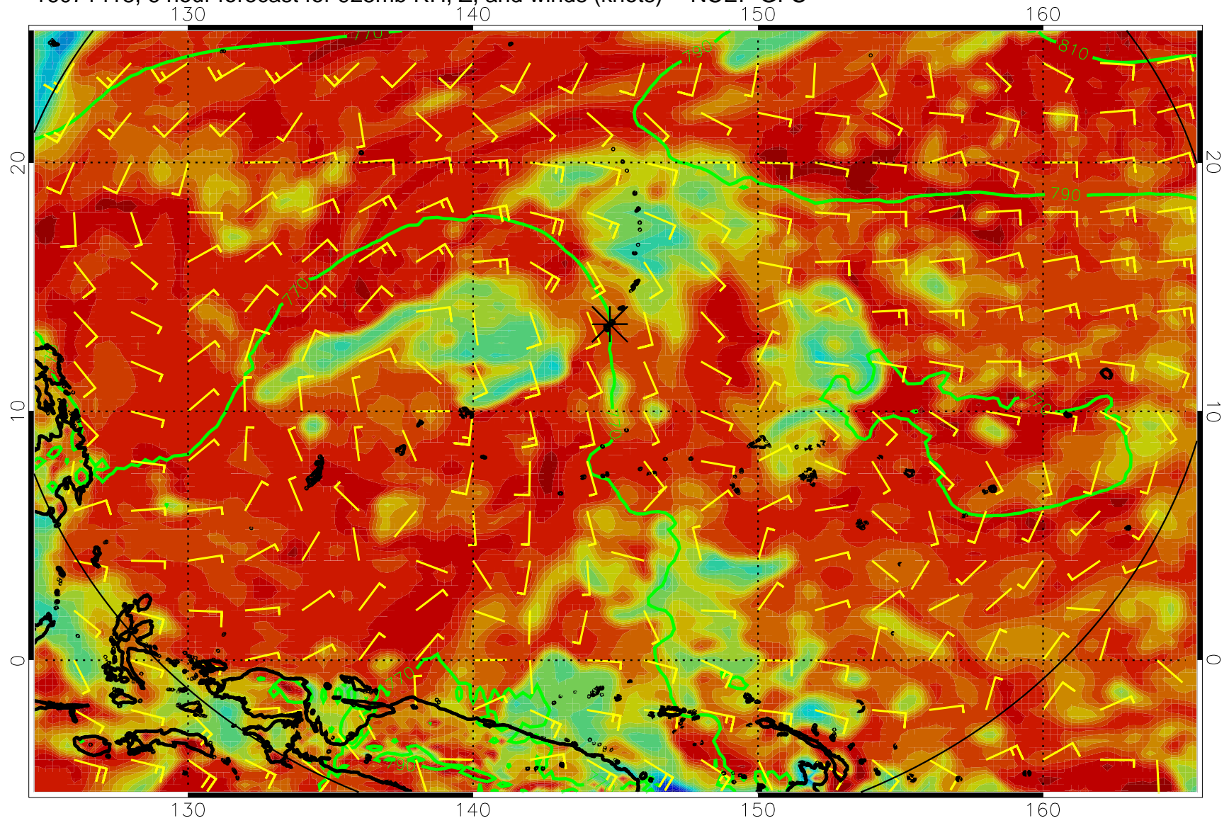
16071418, 6 hour forecast for 925mb RH, Z, and winds (knots) -- NCEP GFS
