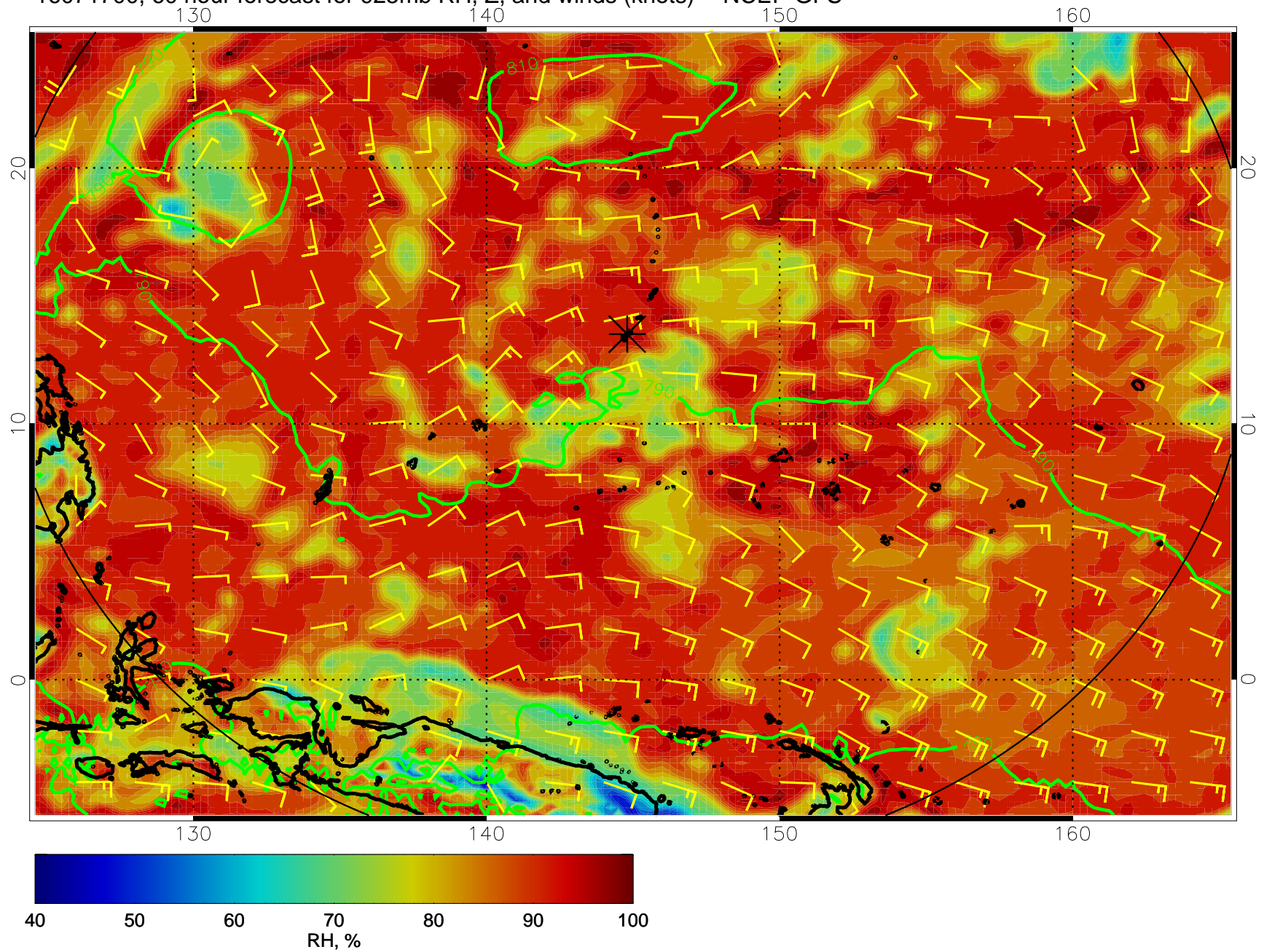
16071700, 60 hour forecast for 925mb RH, Z, and winds (knots) -- NCEP GFS
