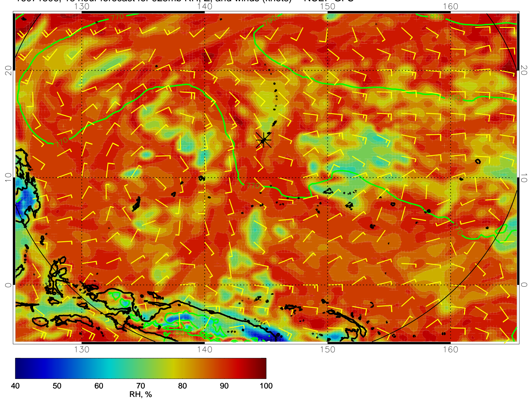
16071506, 18 hour forecast for 925mb RH, Z, and winds (knots) -- NCEP GFS
