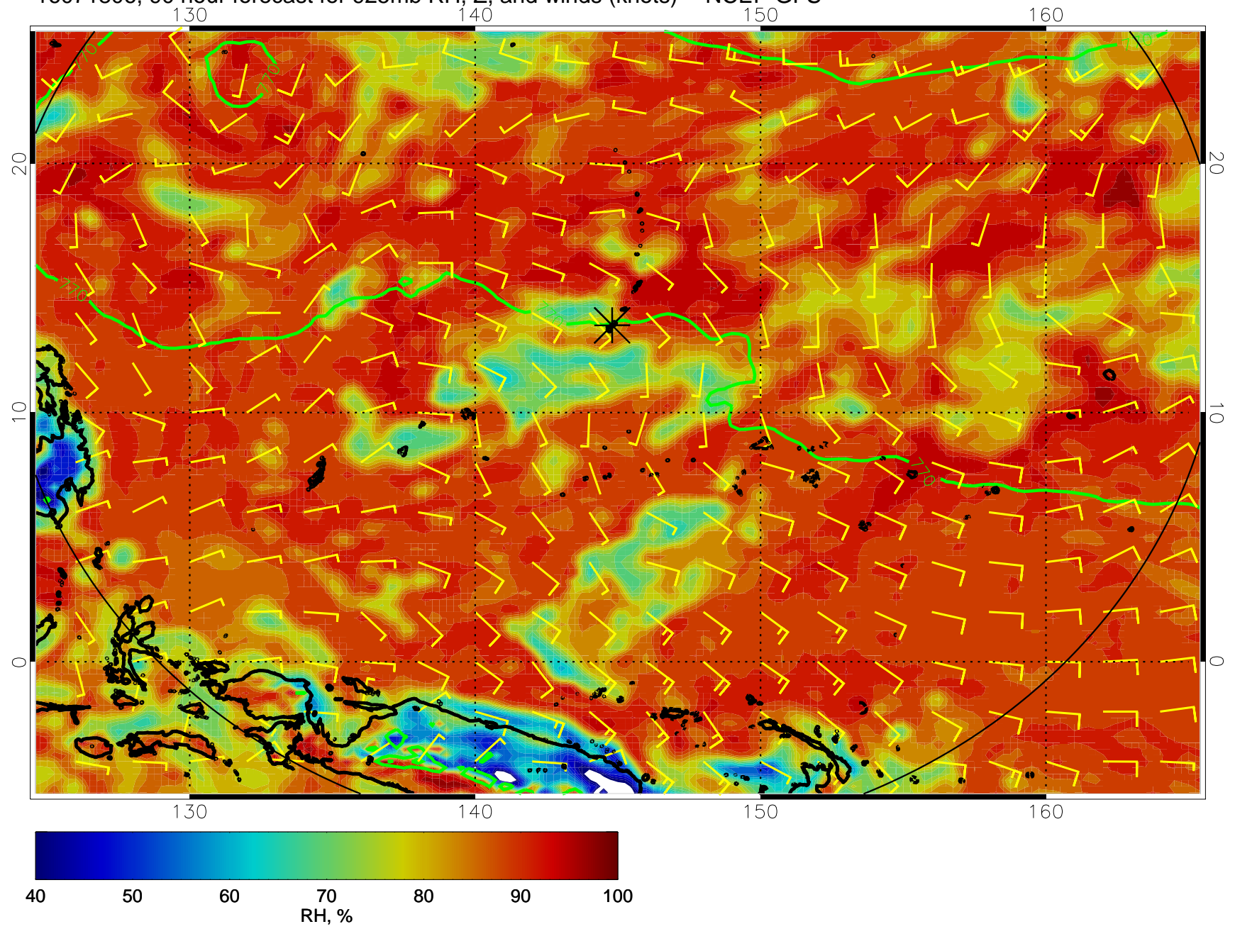
16071806, 90 hour forecast for 925mb RH, Z, and winds (knots) -- NCEP GFS
