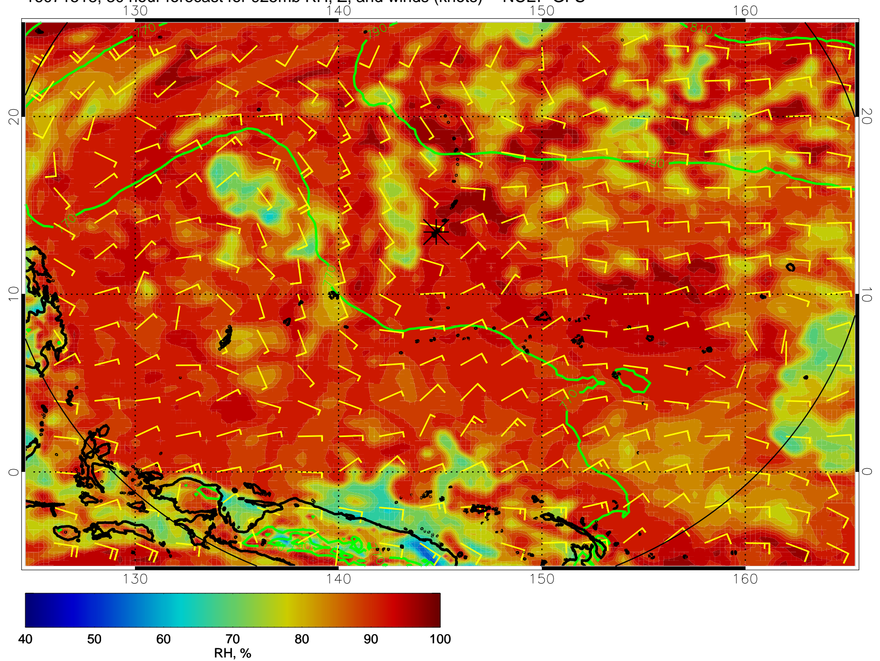
16071518, 30 hour forecast for 925mb RH, Z, and winds (knots) -- NCEP GFS
