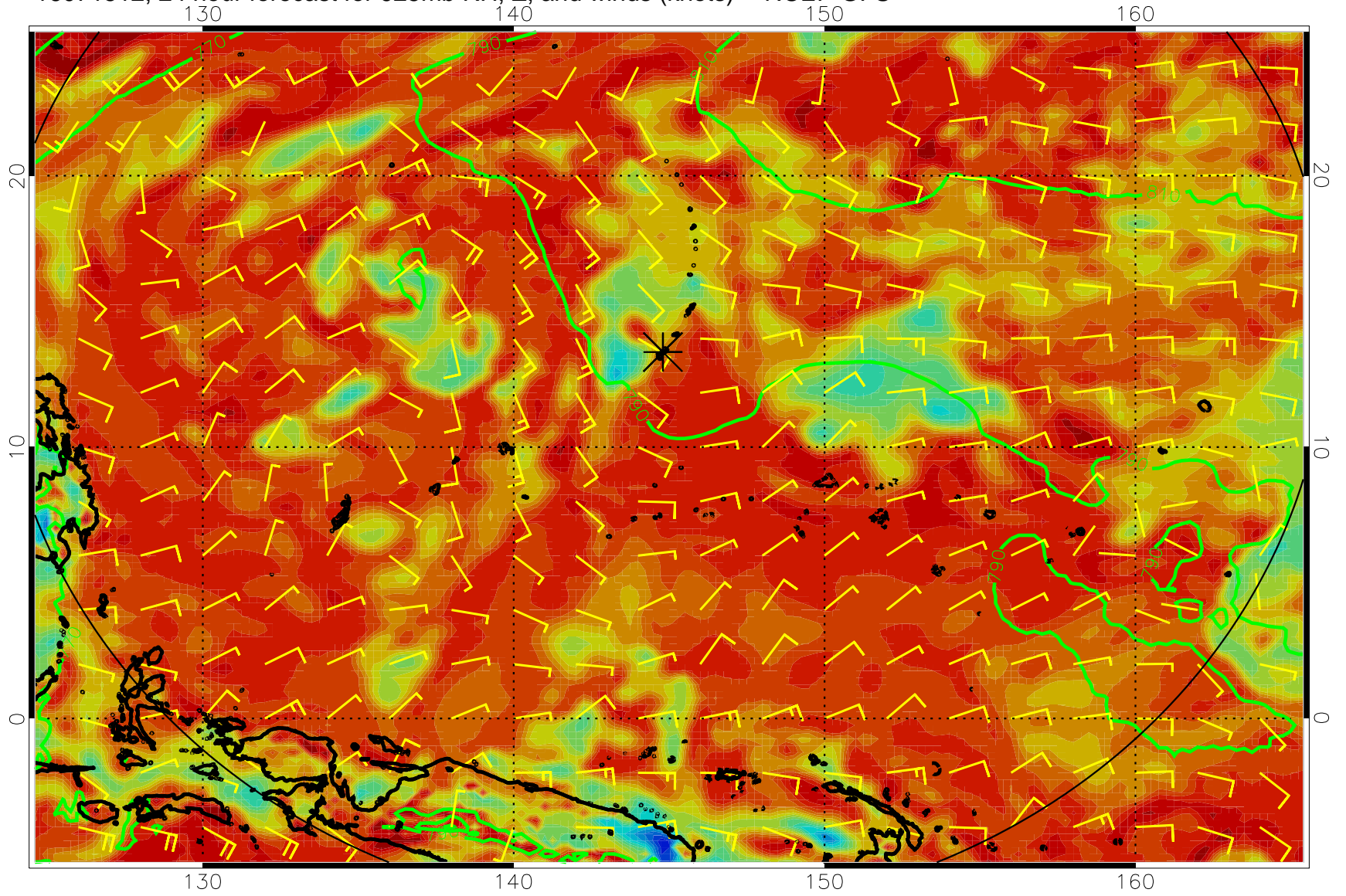
16071512, 24 hour forecast for 925mb RH, Z, and winds (knots) -- NCEP GFS
