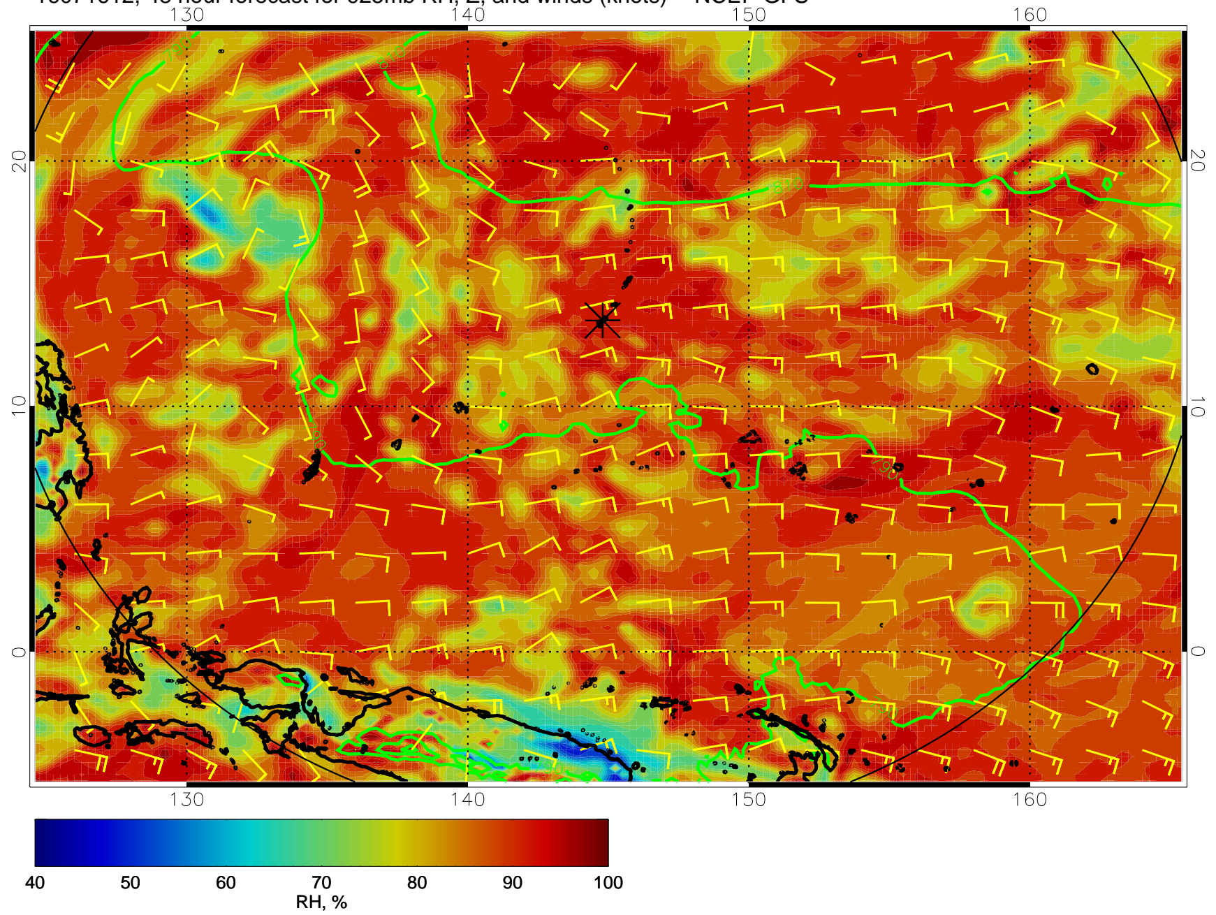
16071612, 48 hour forecast for 925mb RH, Z, and winds (knots) -- NCEP GFS
