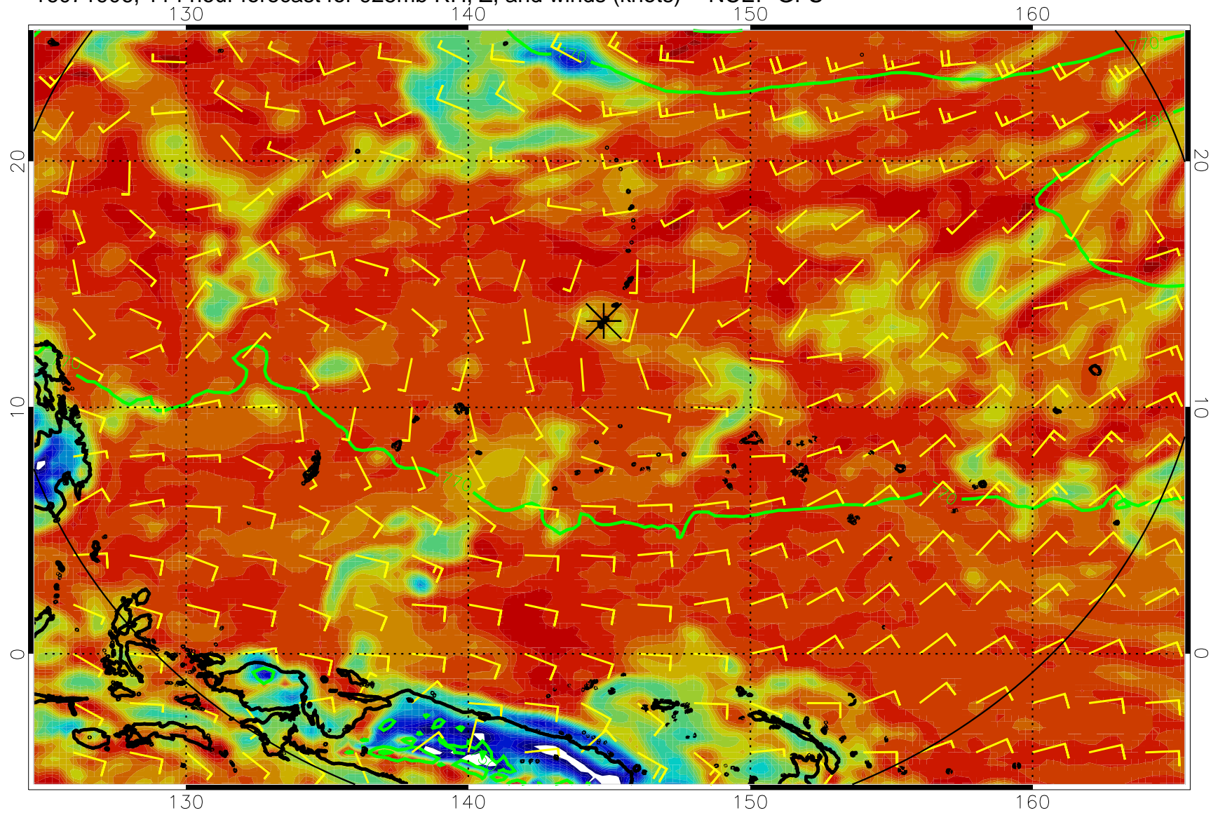
16071906, 114 hour forecast for 925mb RH, Z, and winds (knots) -- NCEP GFS
