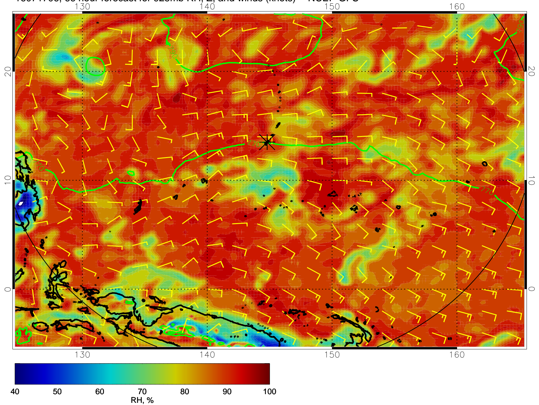
16071706, 66 hour forecast for 925mb RH, Z, and winds (knots) -- NCEP GFS
