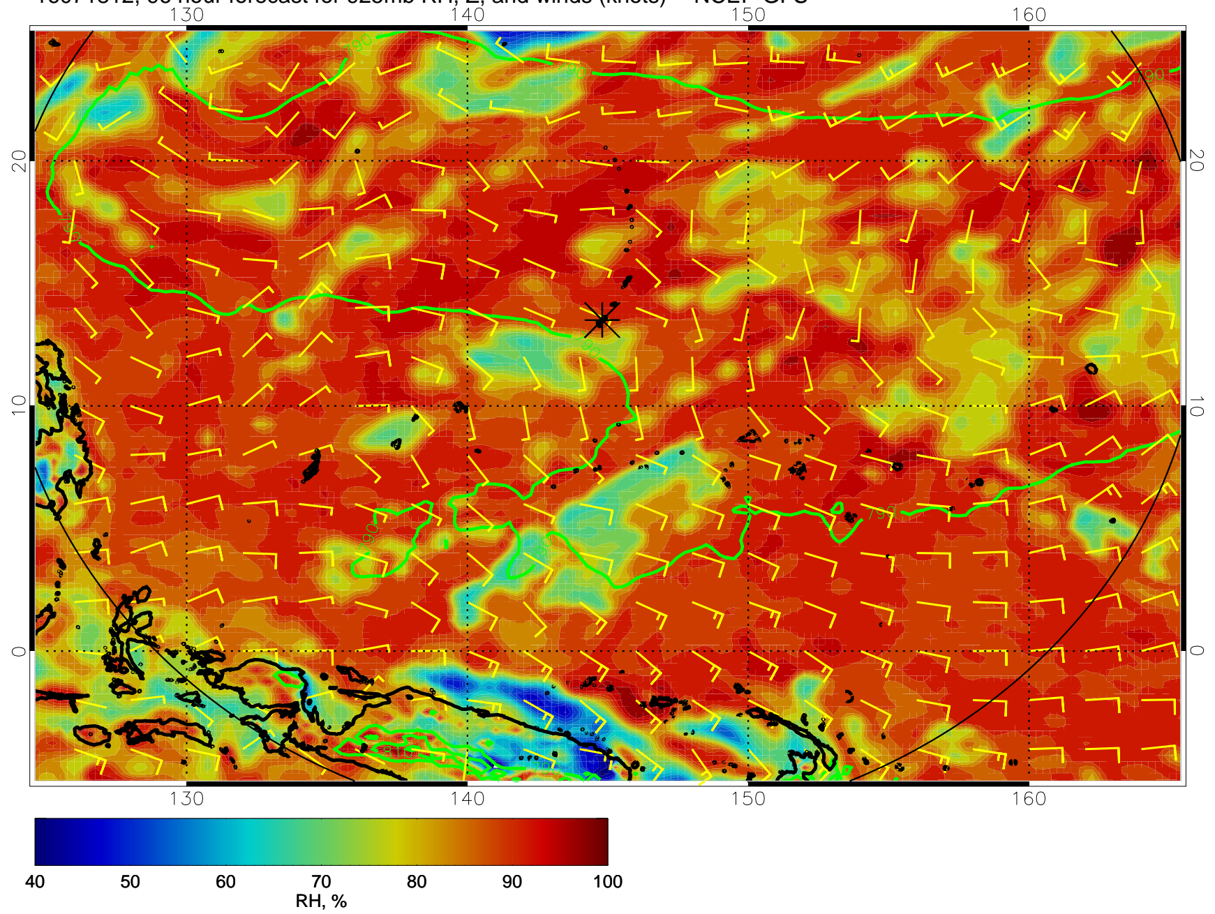
16071812, 96 hour forecast for 925mb RH, Z, and winds (knots) -- NCEP GFS
