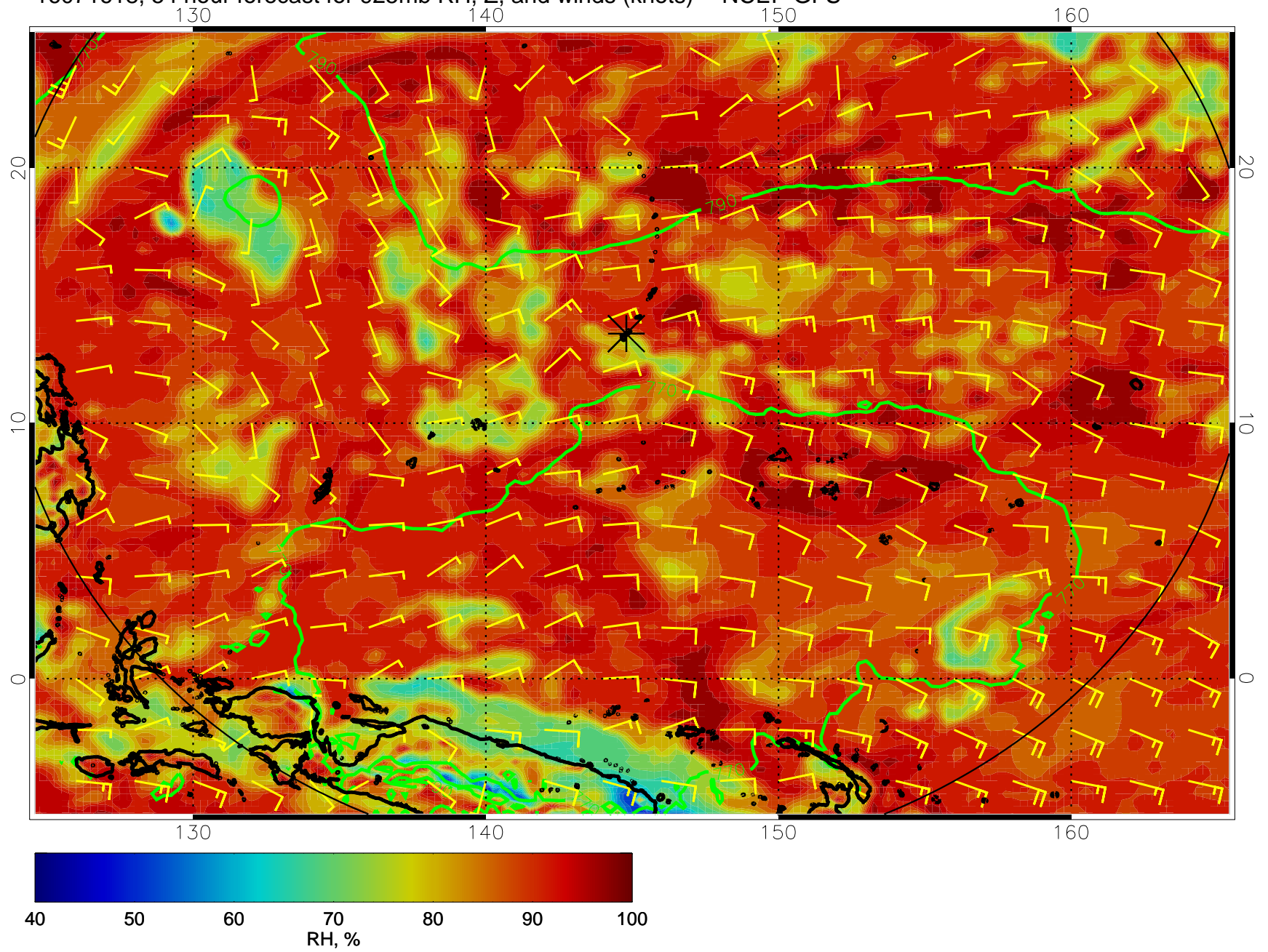
16071618, 54 hour forecast for 925mb RH, Z, and winds (knots) -- NCEP GFS
