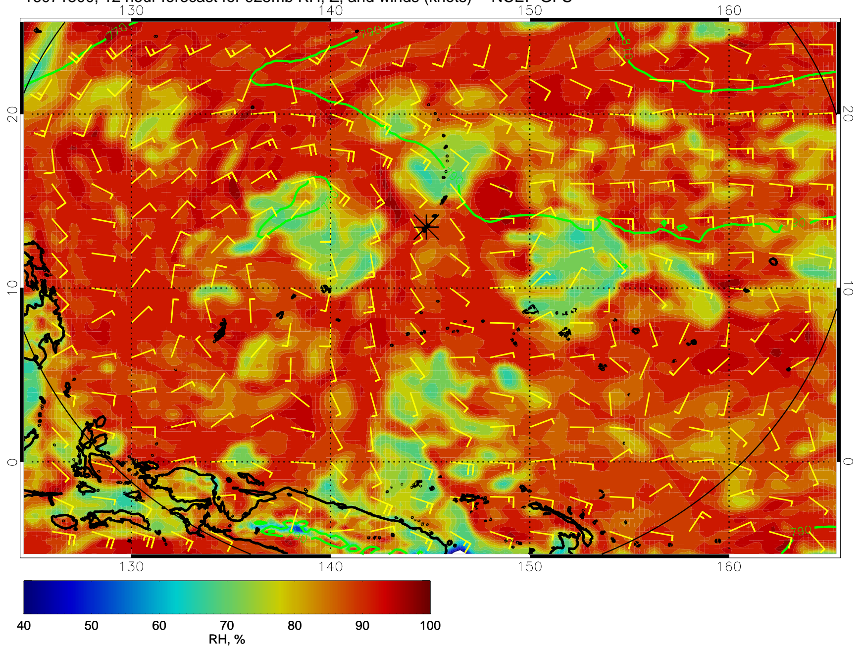
16071500, 12 hour forecast for 925mb RH, Z, and winds (knots) -- NCEP GFS
