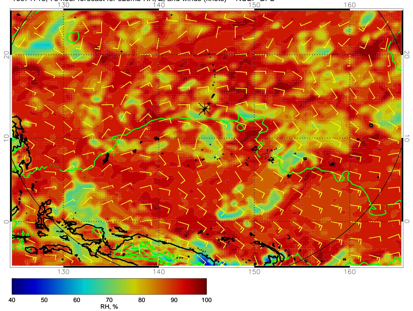
16071718, 78 hour forecast for 925mb RH, Z, and winds (knots) -- NCEP GFS
