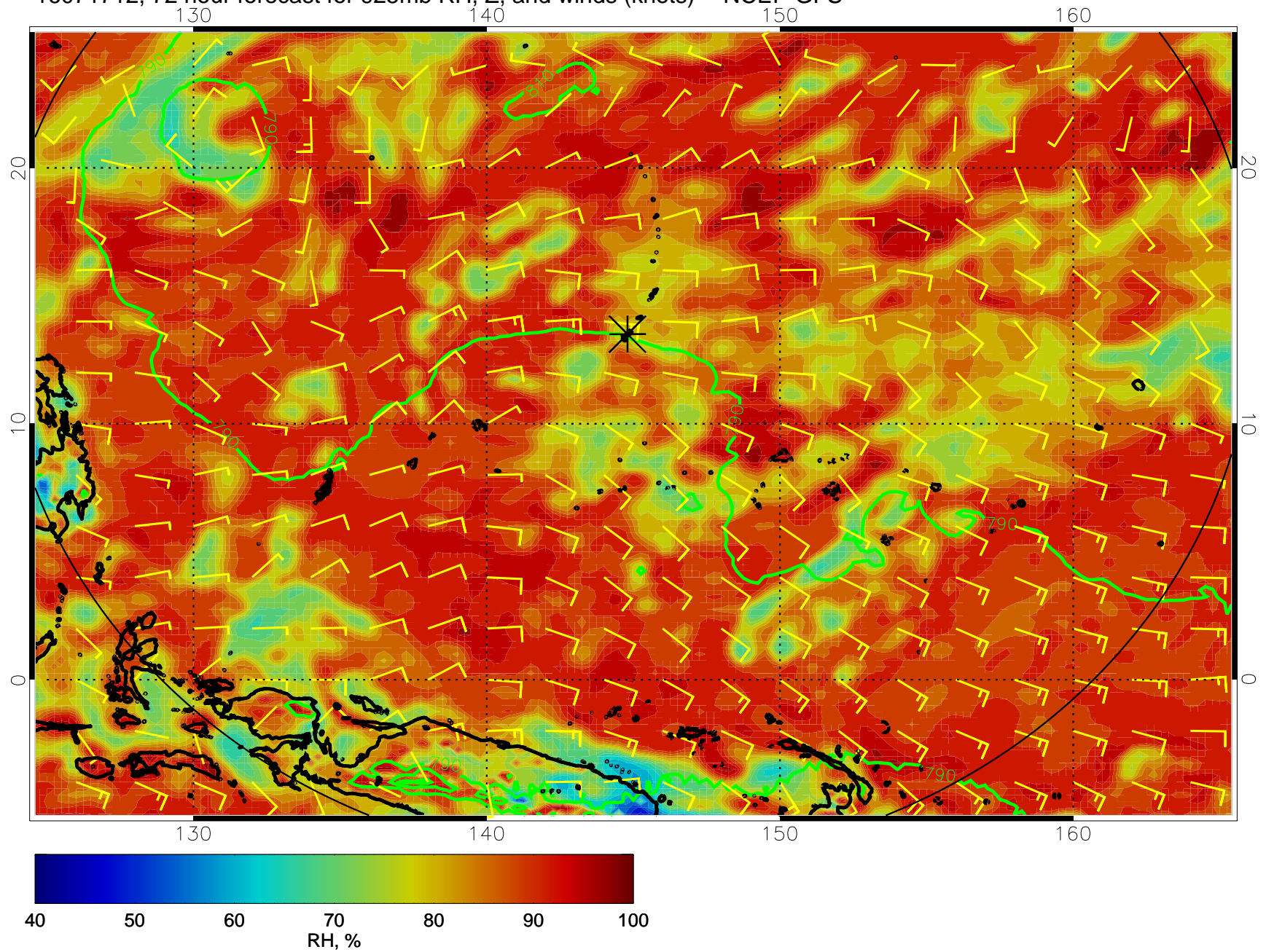
16071712, 72 hour forecast for 925mb RH, Z, and winds (knots) -- NCEP GFS
