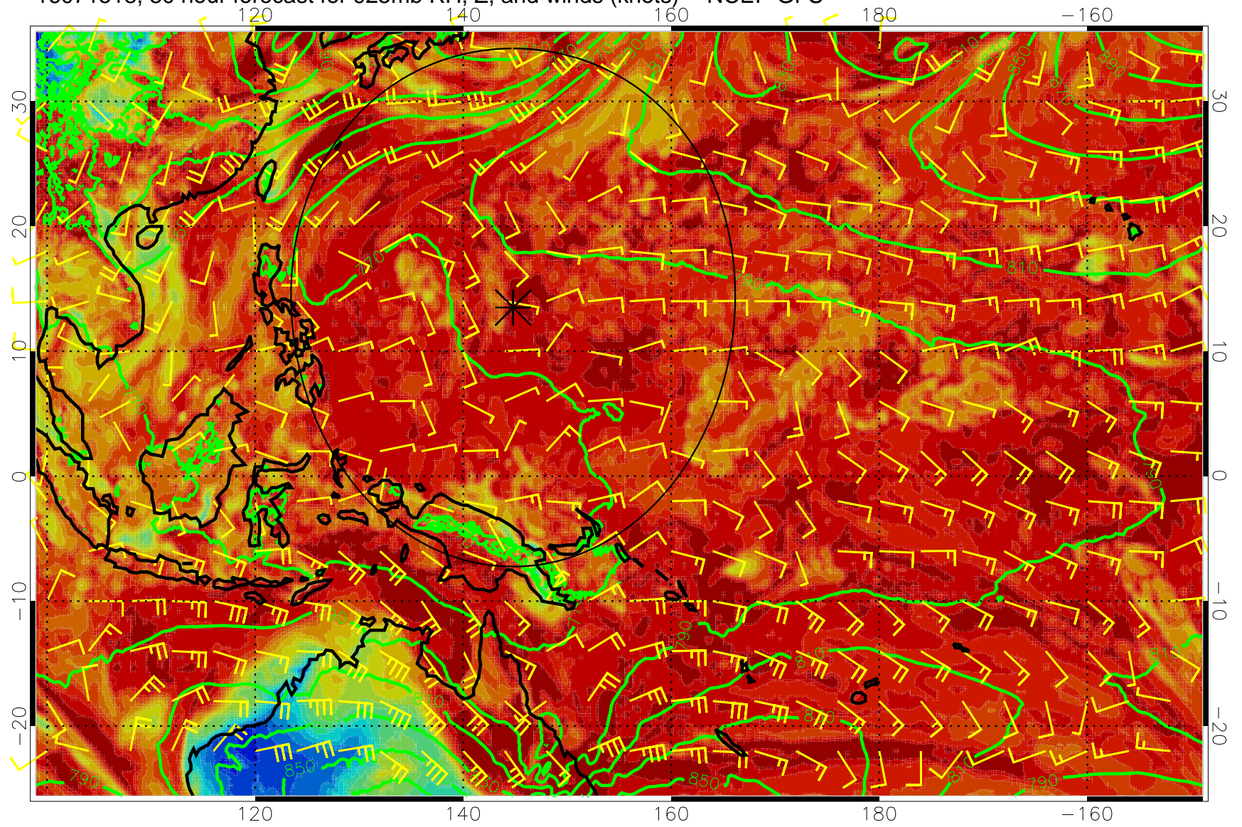
16071518, 30 hour forecast for 925mb RH, Z, and winds (knots) -- NCEP GFS
