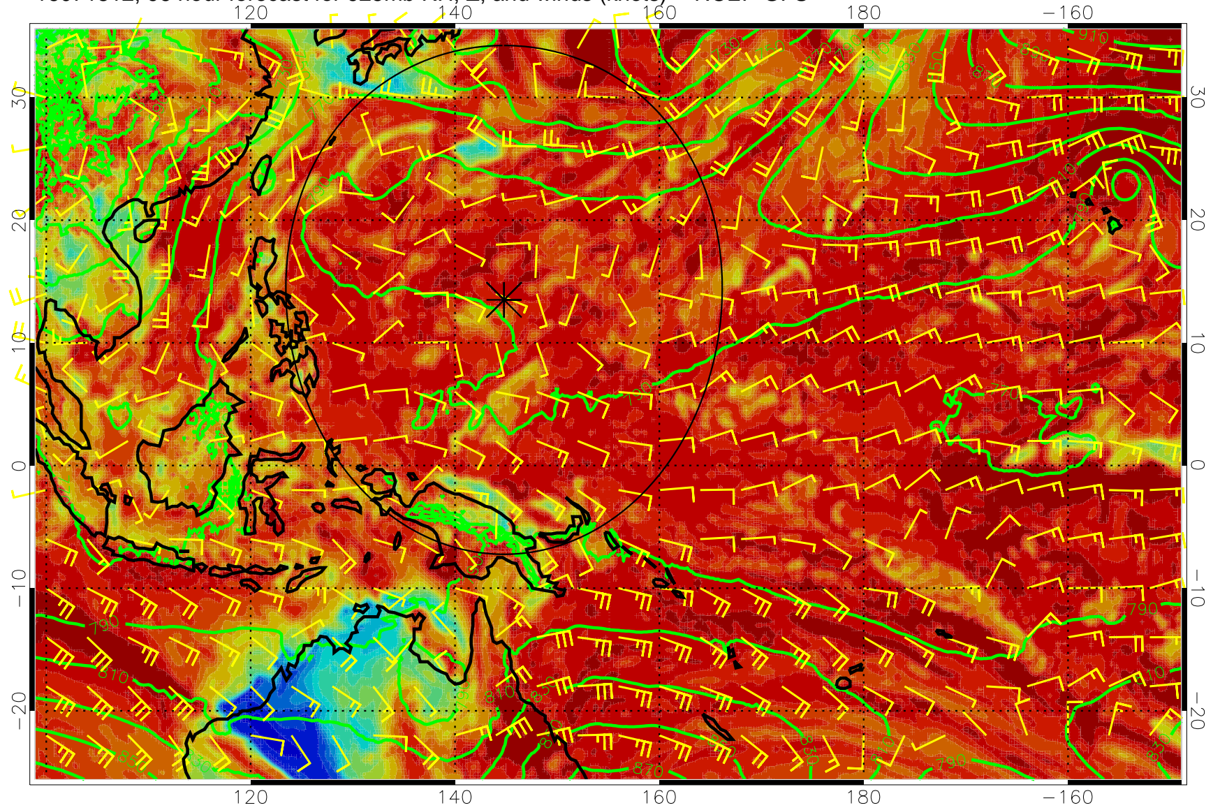
16071812, 96 hour forecast for 925mb RH, Z, and winds (knots) -- NCEP GFS
