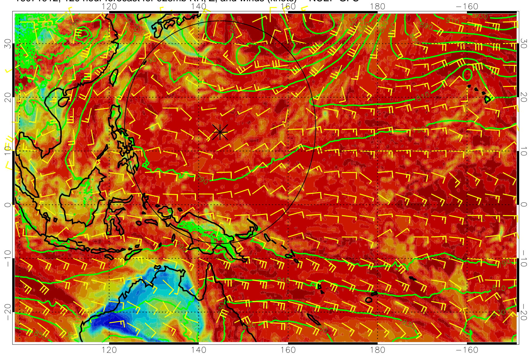
16071912, 120 hour forecast for 925mb RH, Z, and winds (knots) -- NCEP GFS
