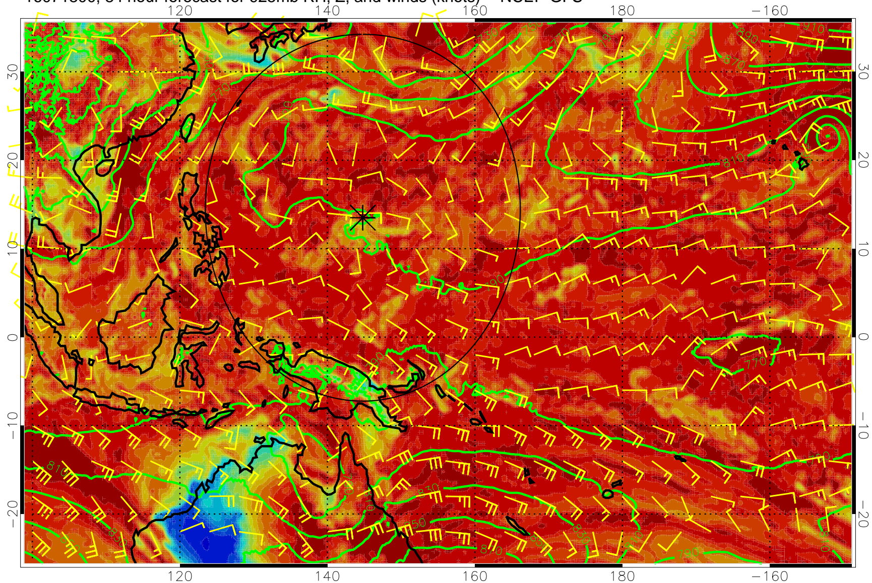
16071800, 84 hour forecast for 925mb RH, Z, and winds (knots) -- NCEP GFS
