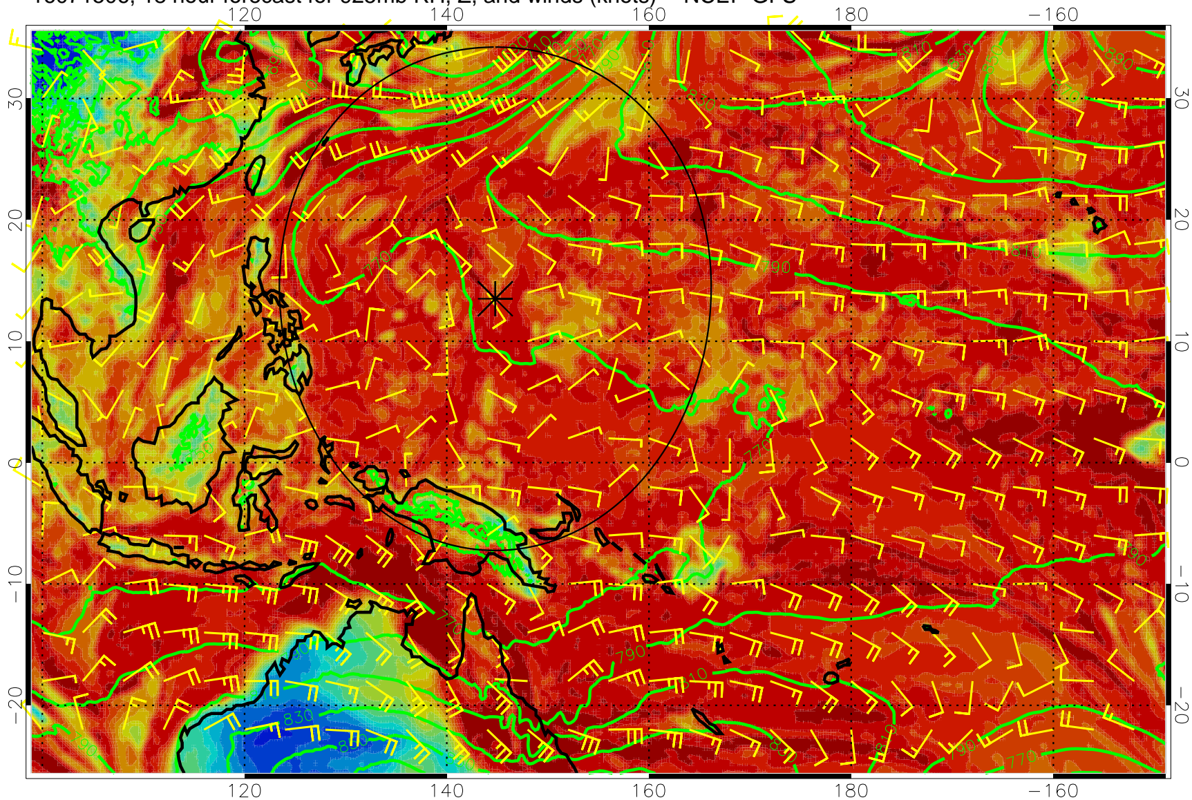
16071506, 18 hour forecast for 925mb RH, Z, and winds (knots) -- NCEP GFS
