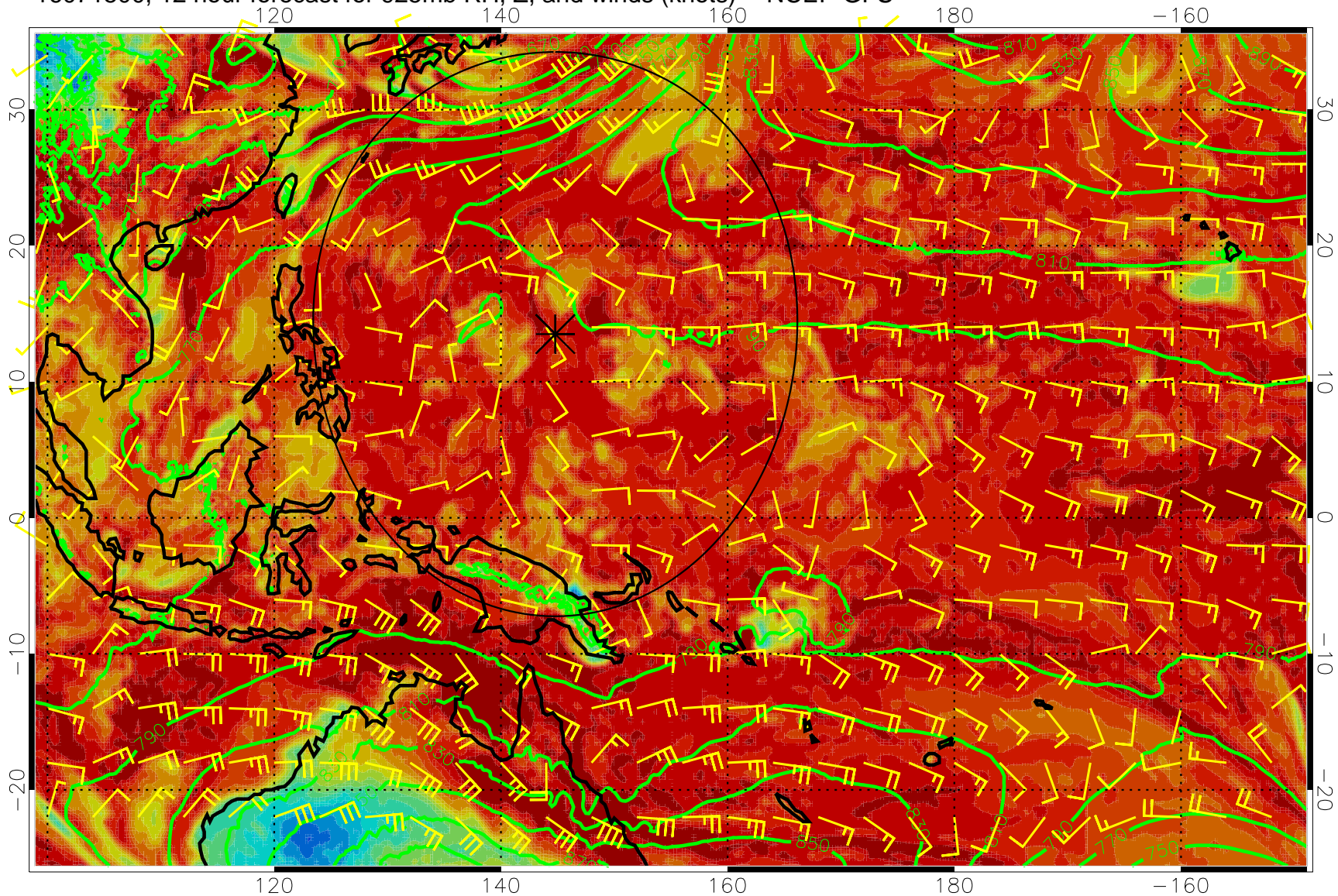
16071500, 12 hour forecast for 925mb RH, Z, and winds (knots) -- NCEP GFS
