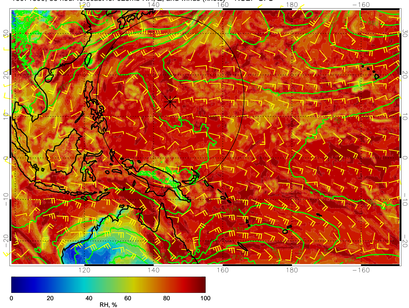
16071600, 36 hour forecast for 925mb RH, Z, and winds (knots) -- NCEP GFS
