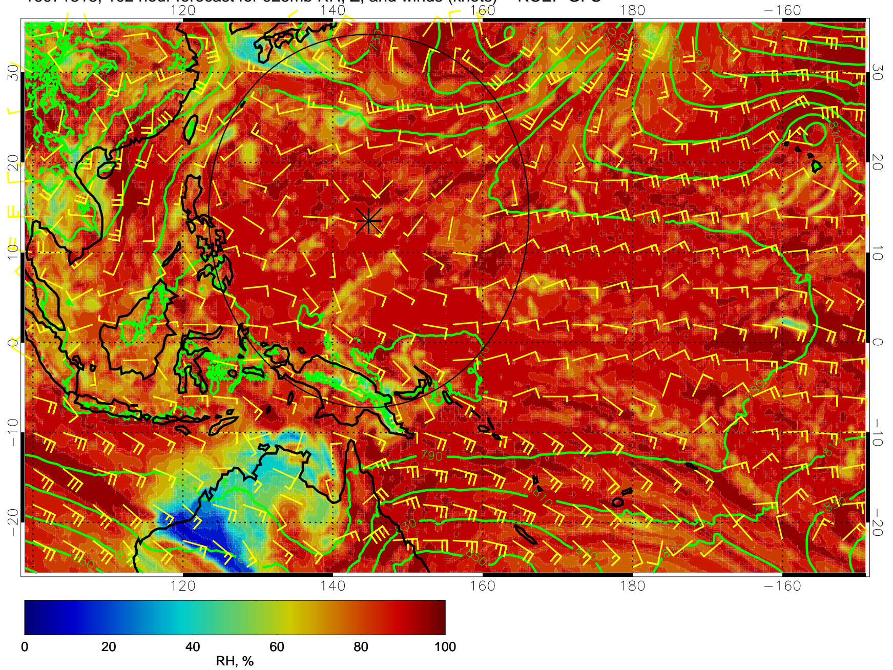
16071818, 102 hour forecast for 925mb RH, Z, and winds (knots) -- NCEP GFS
