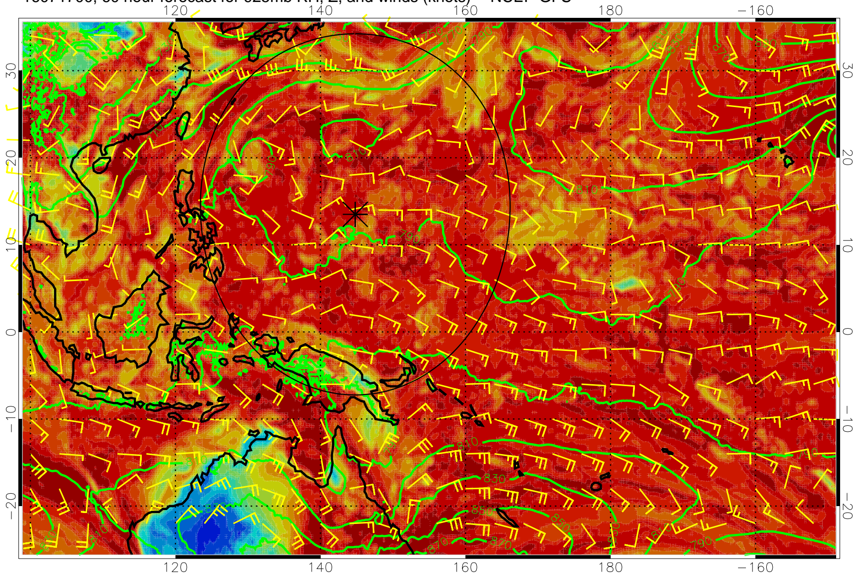
16071700, 60 hour forecast for 925mb RH, Z, and winds (knots) -- NCEP GFS
