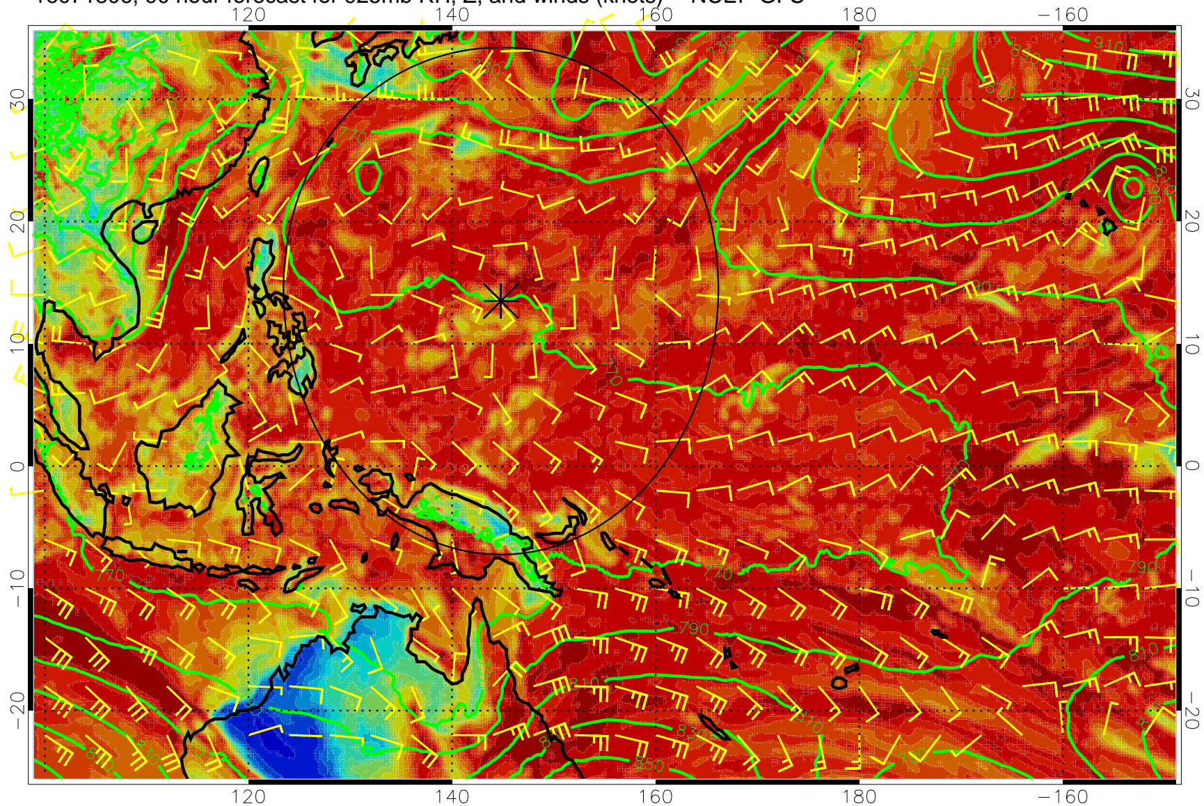
16071806, 90 hour forecast for 925mb RH, Z, and winds (knots) -- NCEP GFS
