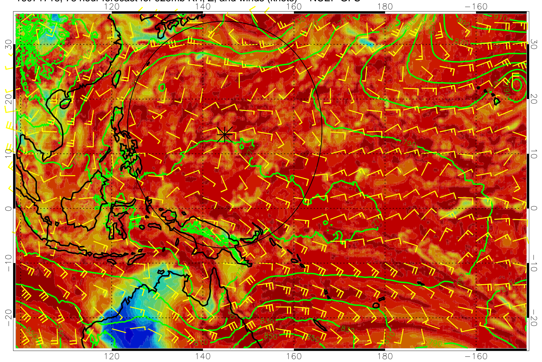
16071718, 78 hour forecast for 925mb RH, Z, and winds (knots) -- NCEP GFS
