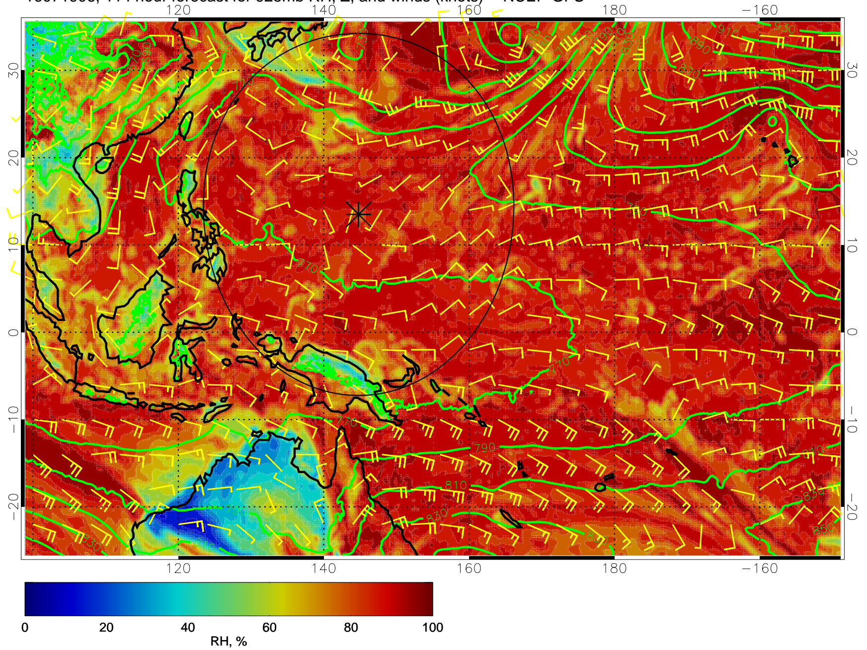
16071906, 114 hour forecast for 925mb RH, Z, and winds (knots) -- NCEP GFS
