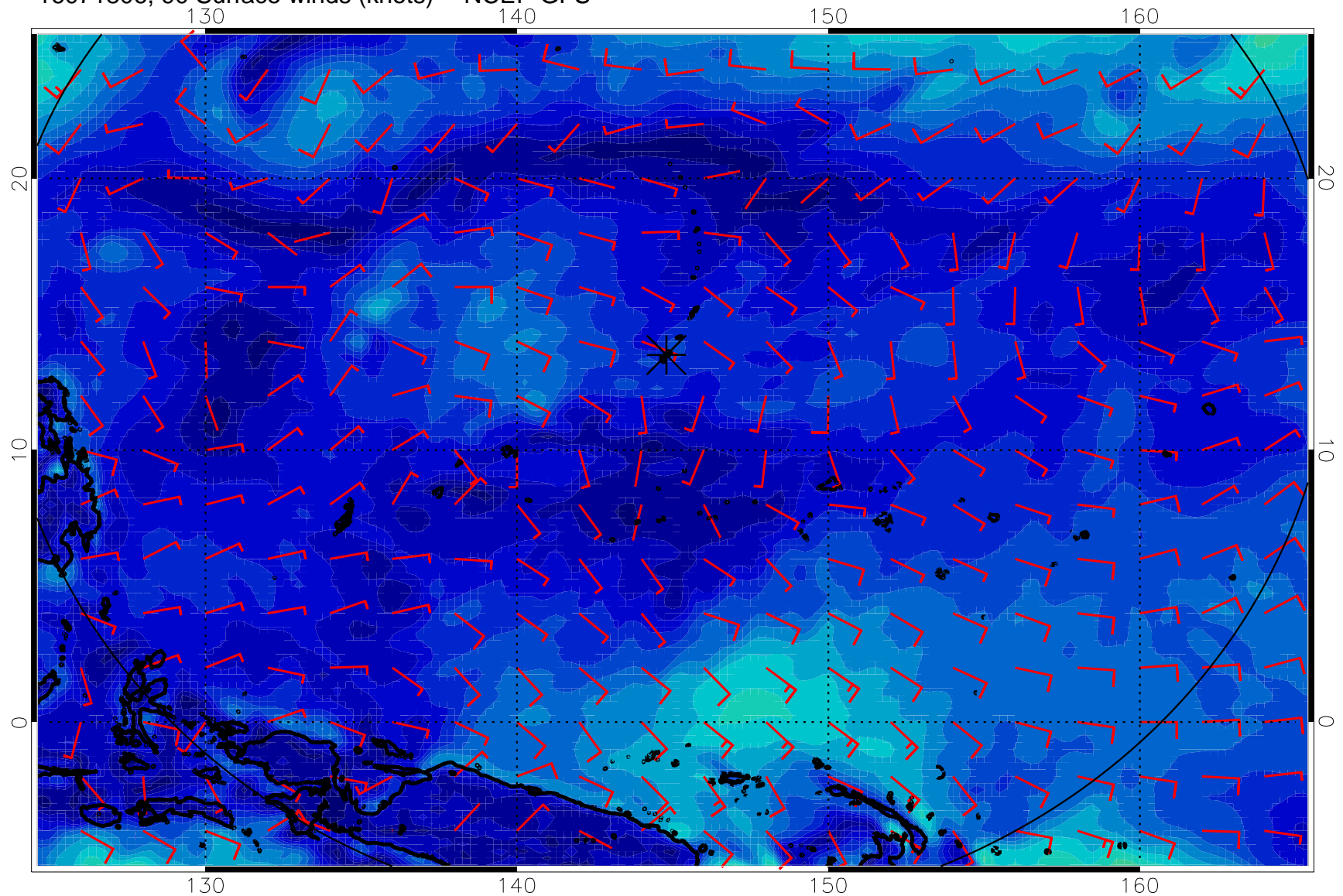
16071806, 90 Surface winds (knots) -- NCEP GFS
