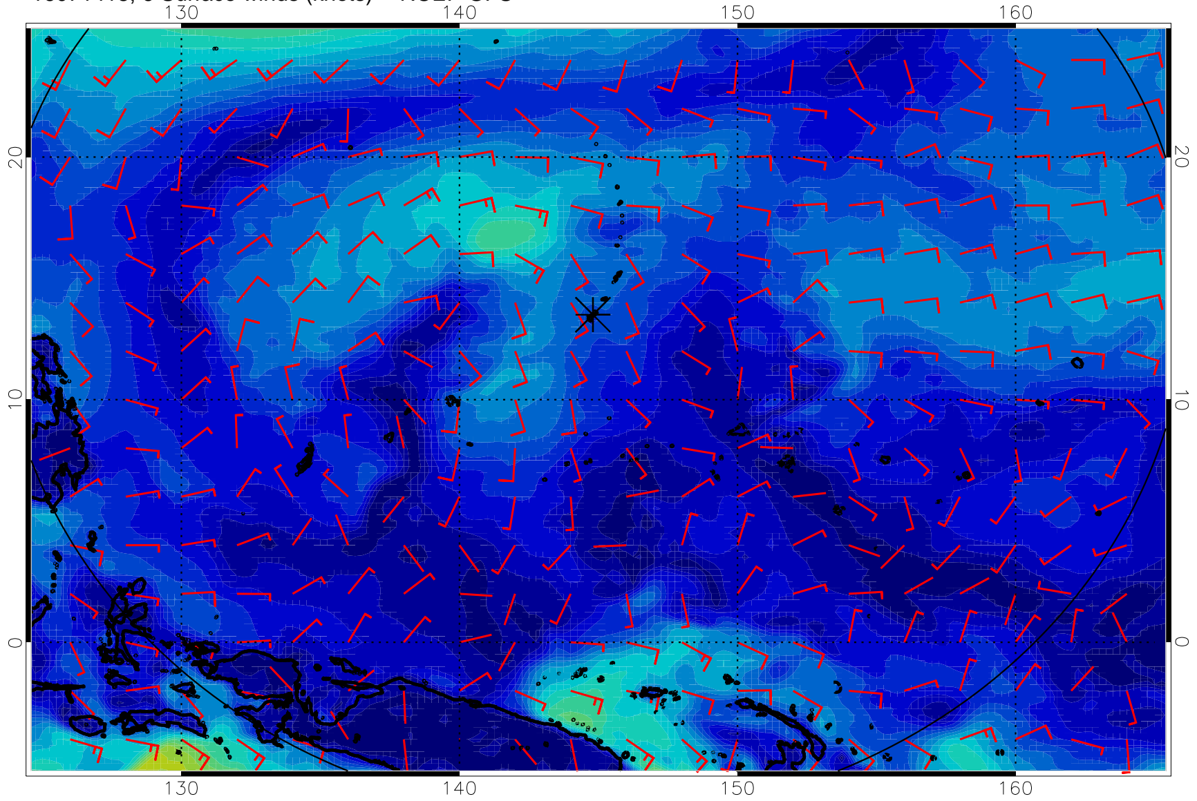
16071418, 6 Surface winds (knots) -- NCEP GFS
