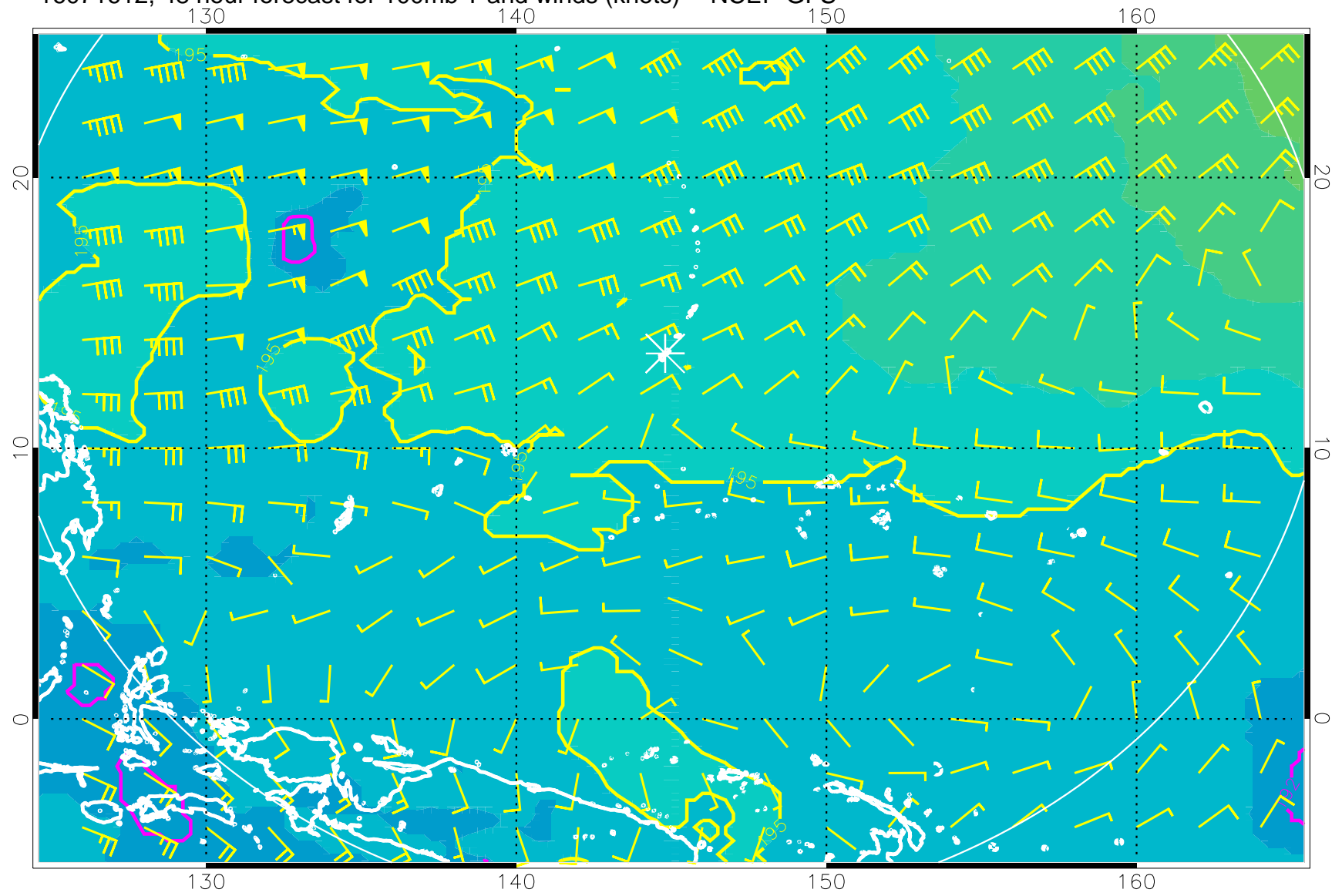
16071612, 48 hour forecast for 100mb T and winds (knots) -- NCEP GFS
