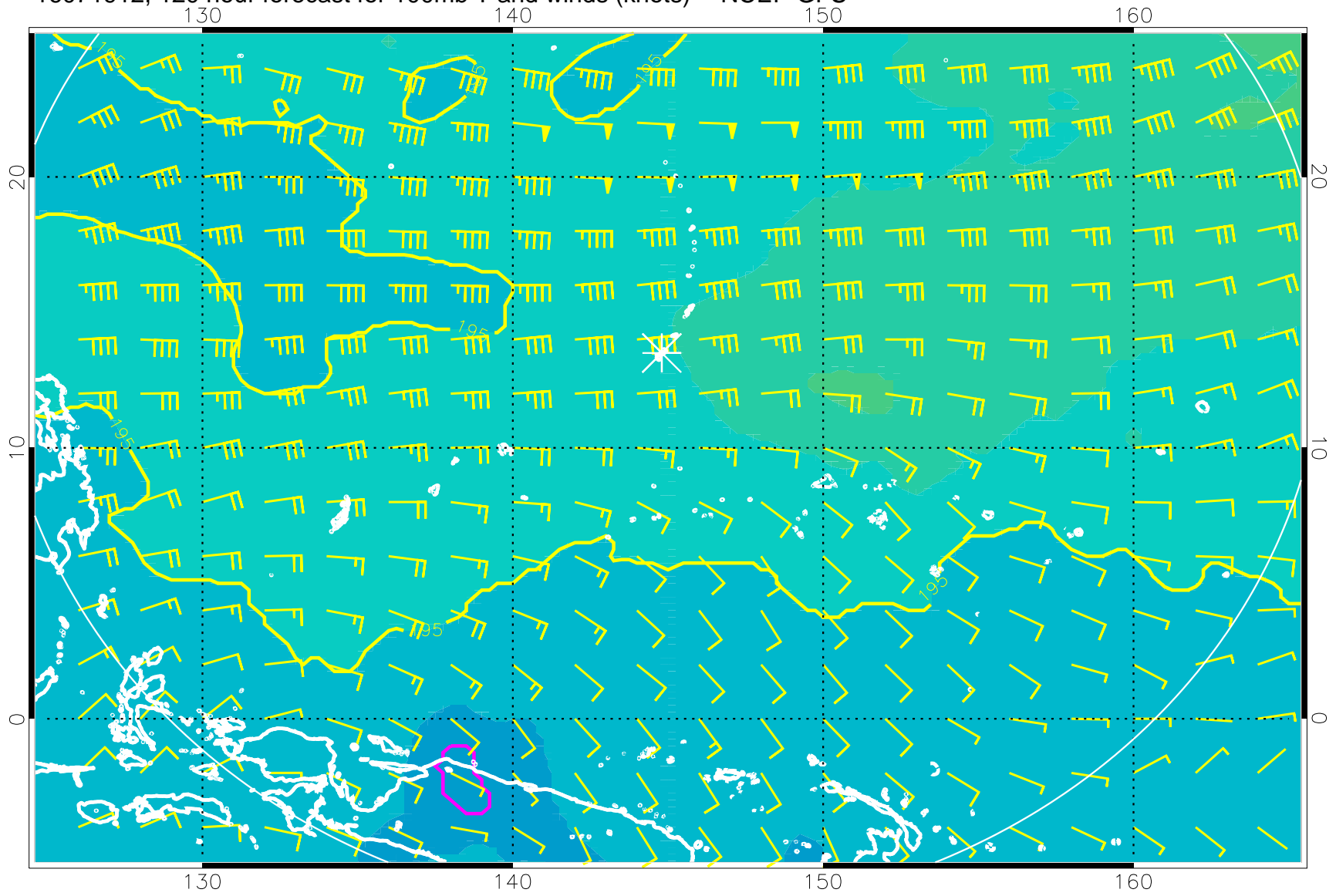
16071912, 120 hour forecast for 100mb T and winds (knots) -- NCEP GFS
