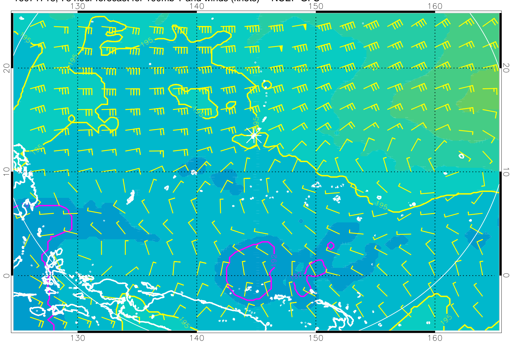
16071718, 78 hour forecast for 100mb T and winds (knots) -- NCEP GFS
