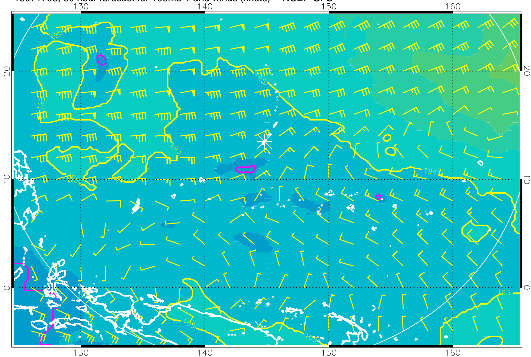
16071700, 60 hour forecast for 100mb T and winds (knots) -- NCEP GFS
