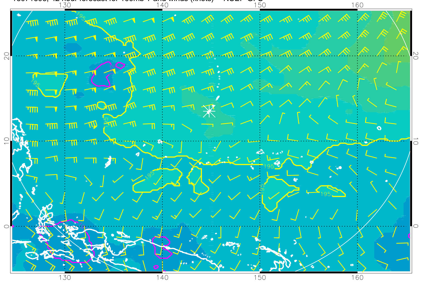
16071606, 42 hour forecast for 100mb T and winds (knots) -- NCEP GFS
