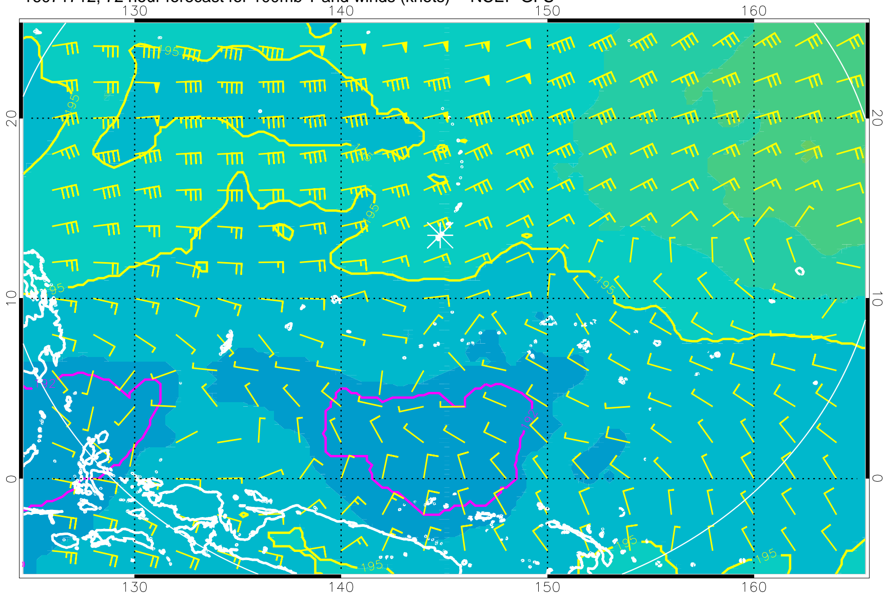
16071712, 72 hour forecast for 100mb T and winds (knots) -- NCEP GFS
