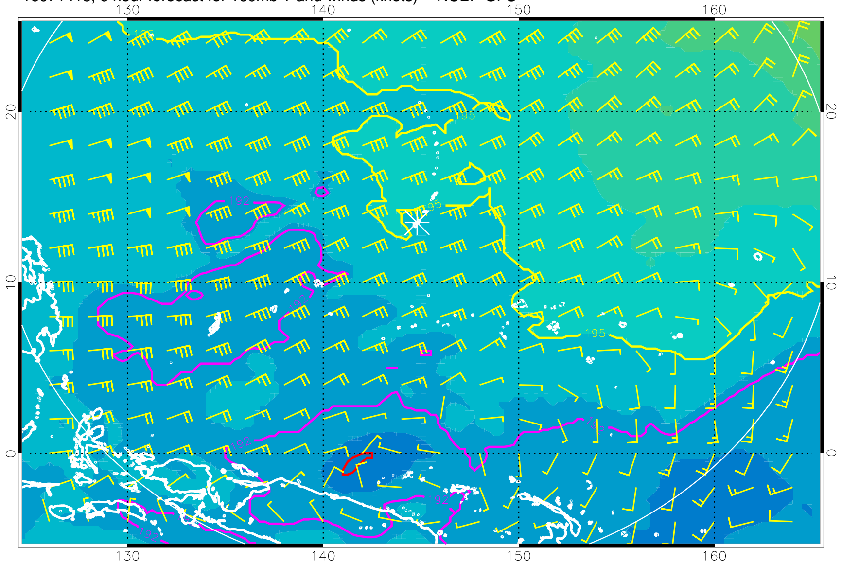
16071418, 6 hour forecast for 100mb T and winds (knots) -- NCEP GFS
