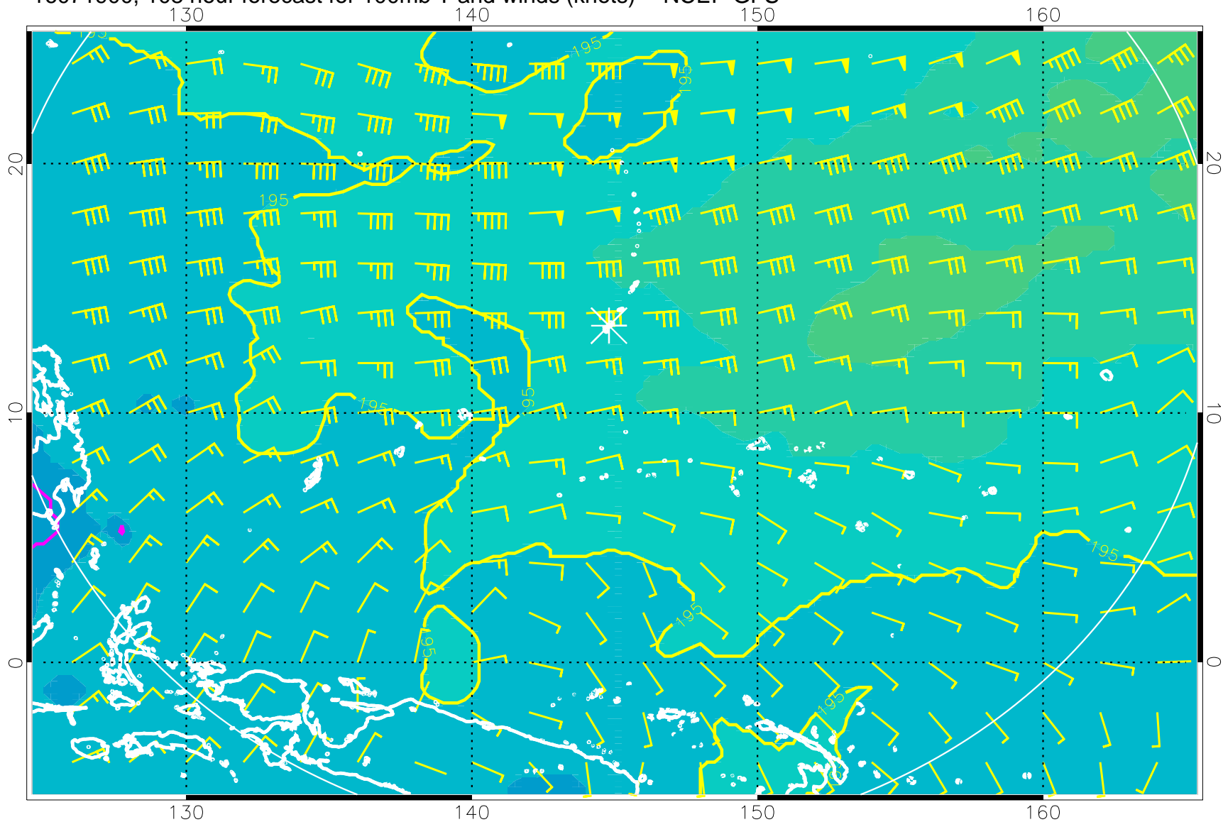
16071900, 108 hour forecast for 100mb T and winds (knots) -- NCEP GFS
