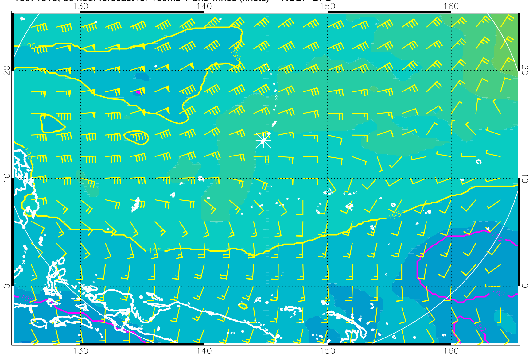
16071518, 30 hour forecast for 100mb T and winds (knots) -- NCEP GFS
