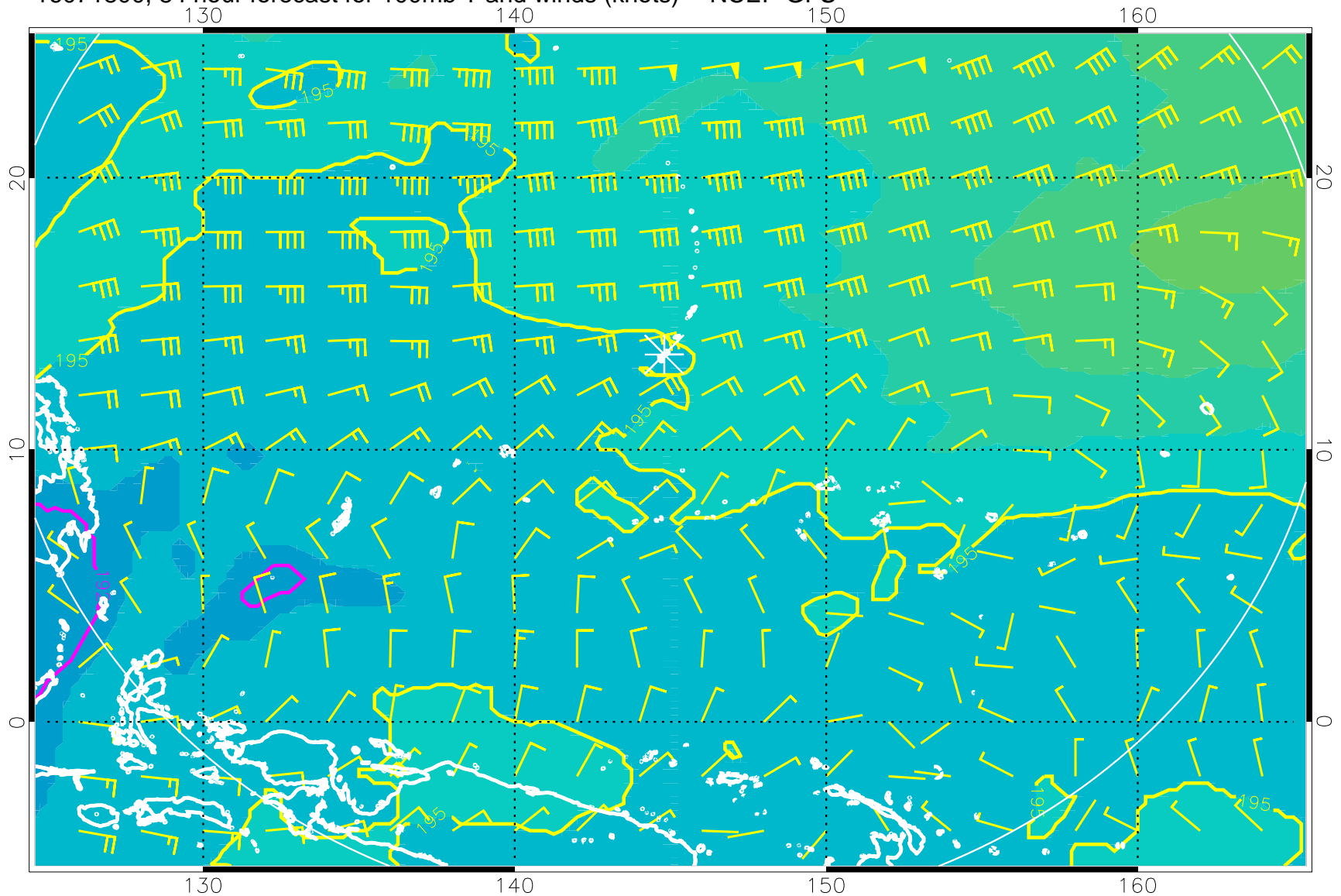
16071800, 84 hour forecast for 100mb T and winds (knots) -- NCEP GFS
