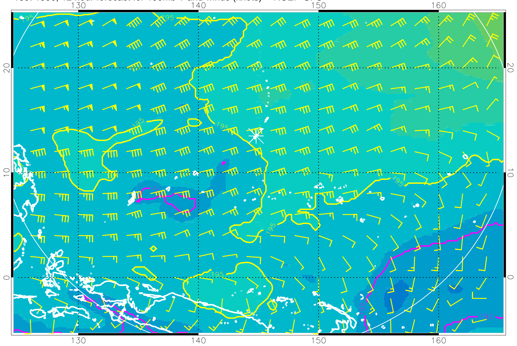
16071500, 12 hour forecast for 100mb T and winds (knots) -- NCEP GFS
