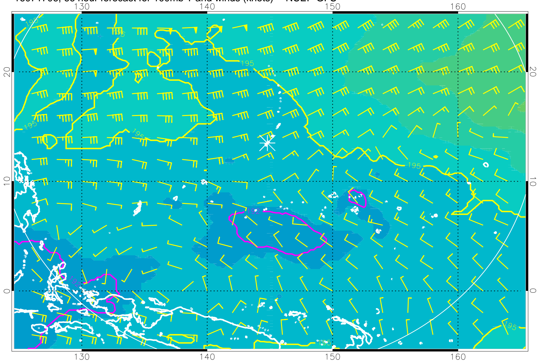
16071706, 66 hour forecast for 100mb T and winds (knots) -- NCEP GFS
