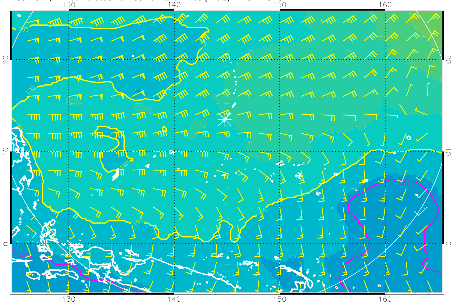
16071512, 24 hour forecast for 100mb T and winds (knots) -- NCEP GFS
