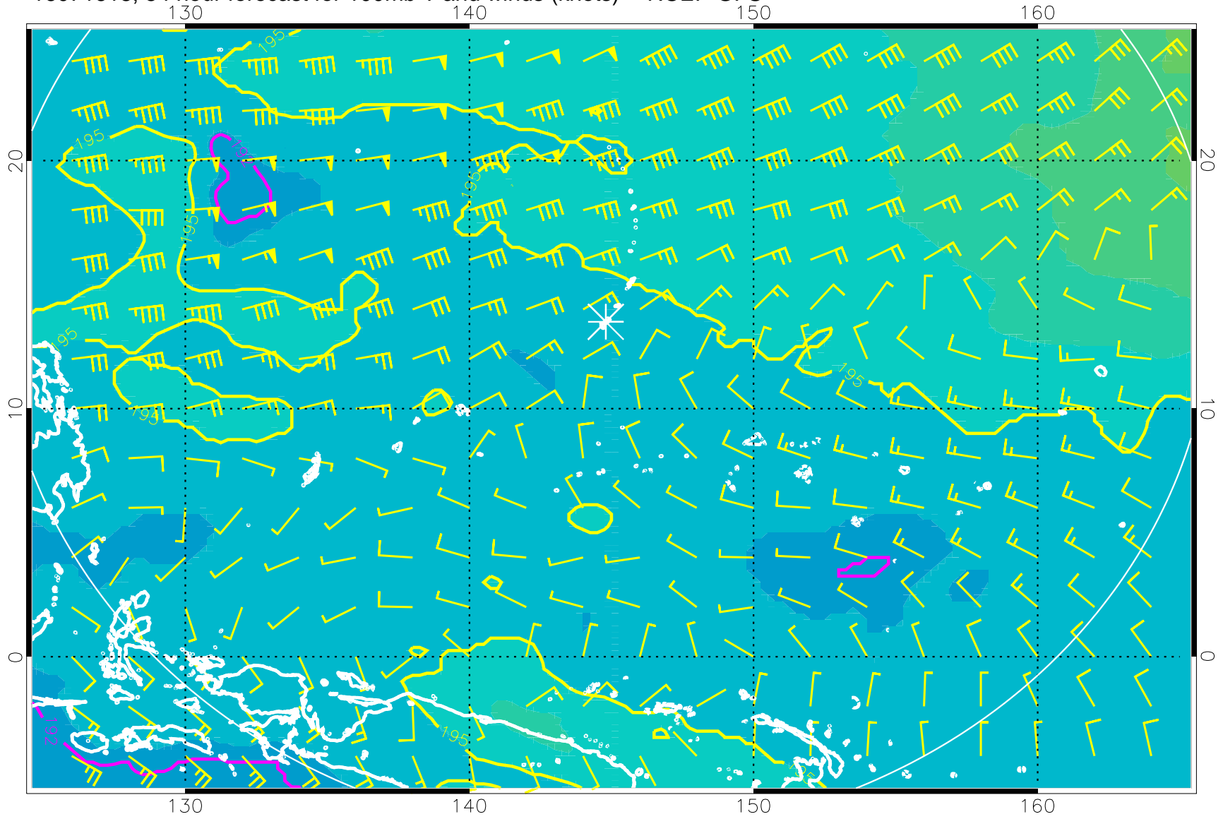
16071618, 54 hour forecast for 100mb T and winds (knots) -- NCEP GFS
