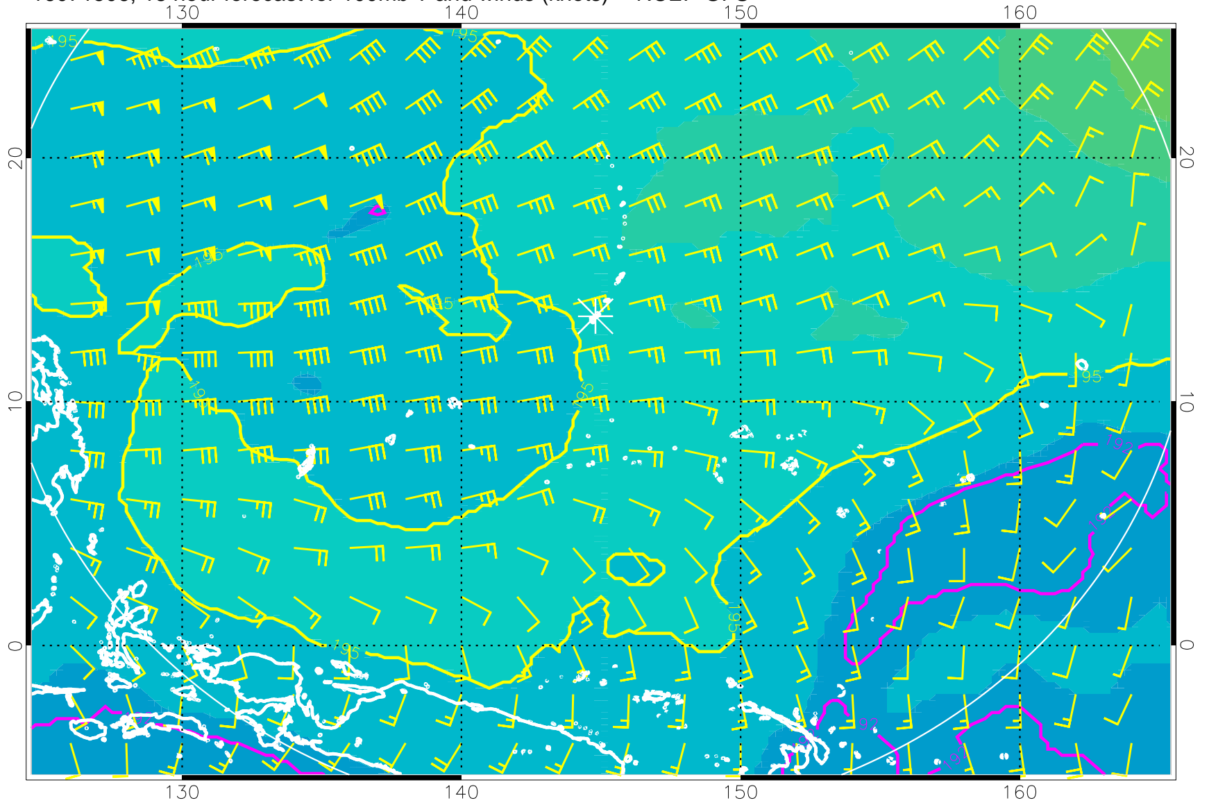
16071506, 18 hour forecast for 100mb T and winds (knots) -- NCEP GFS
