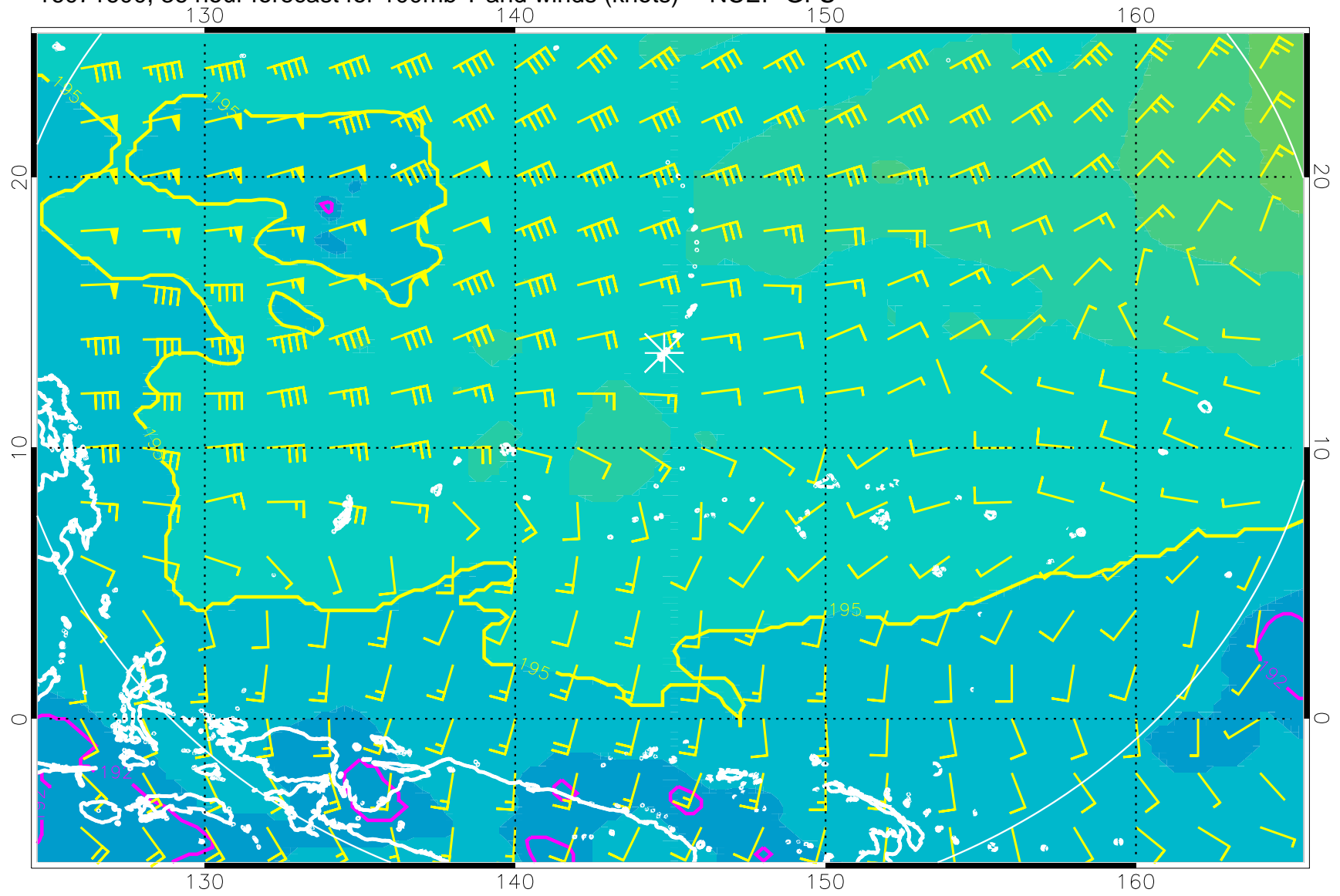
16071600, 36 hour forecast for 100mb T and winds (knots) -- NCEP GFS
