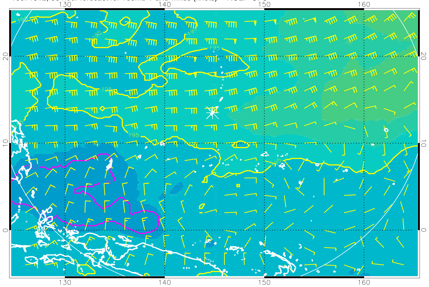
16071812, 96 hour forecast for 100mb T and winds (knots) -- NCEP GFS
