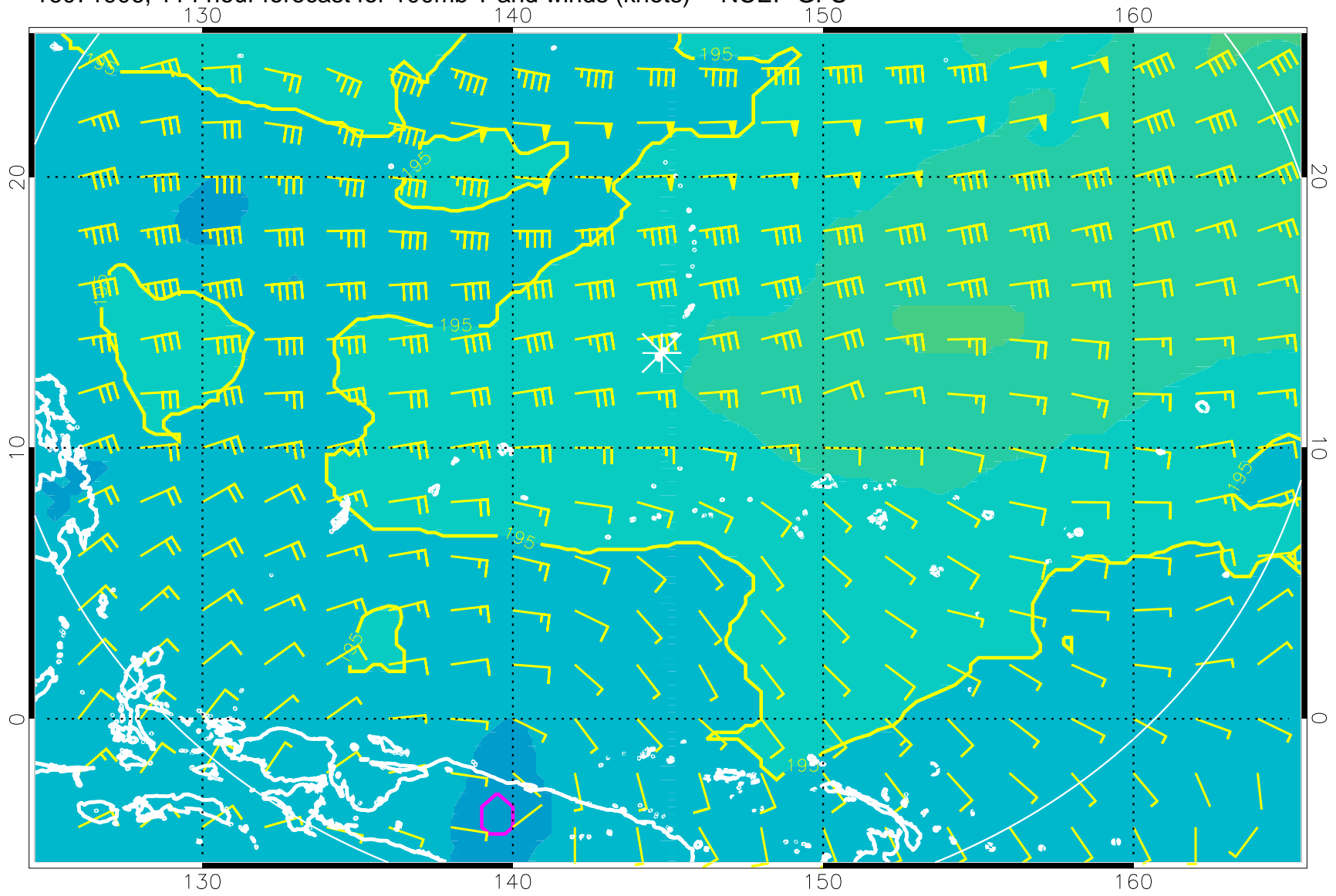
16071906, 114 hour forecast for 100mb T and winds (knots) -- NCEP GFS
