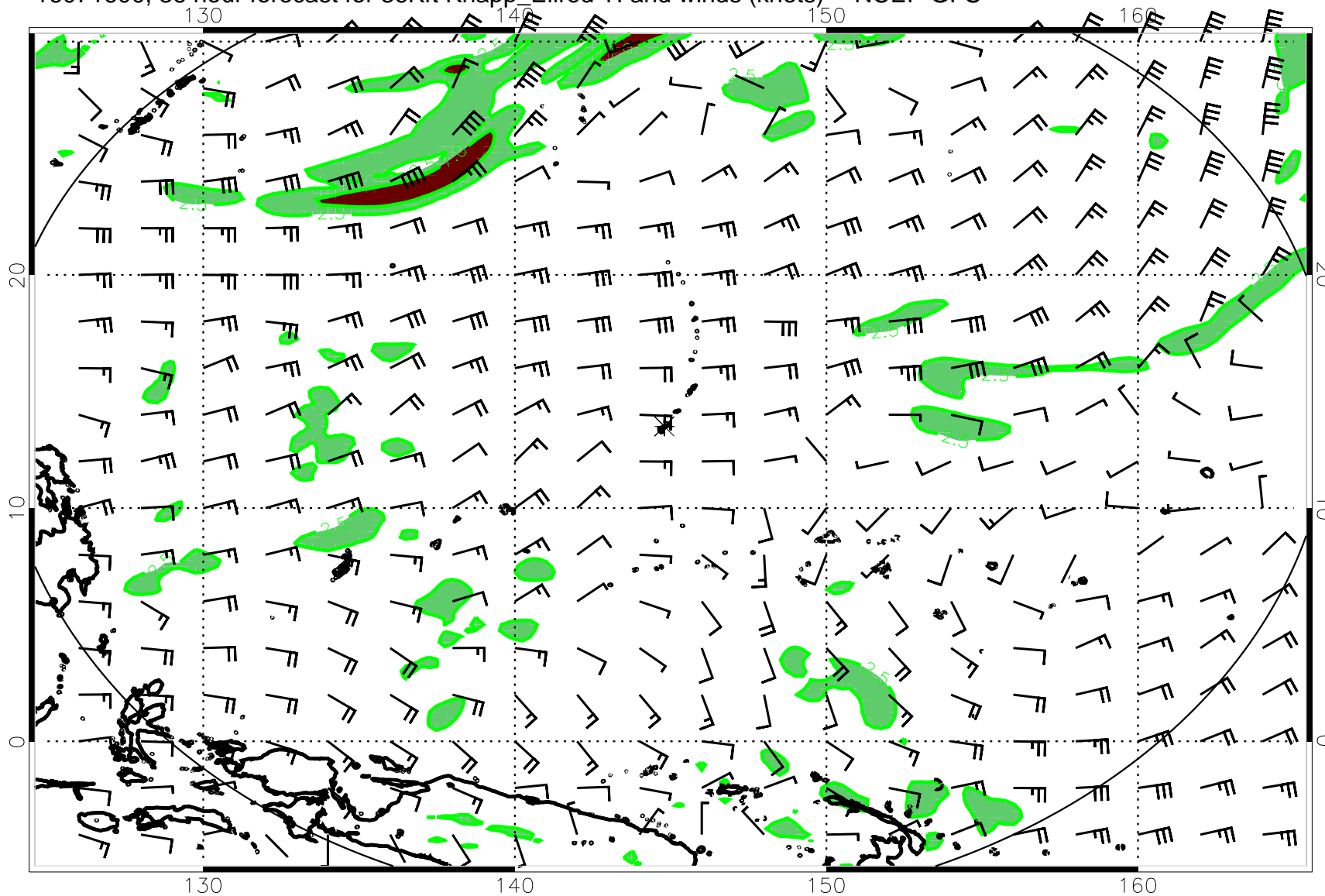
16071600, 36 hour forecast for 36Kft Knapp_Ellrod TI and winds (knots) -- NCEP GFS
