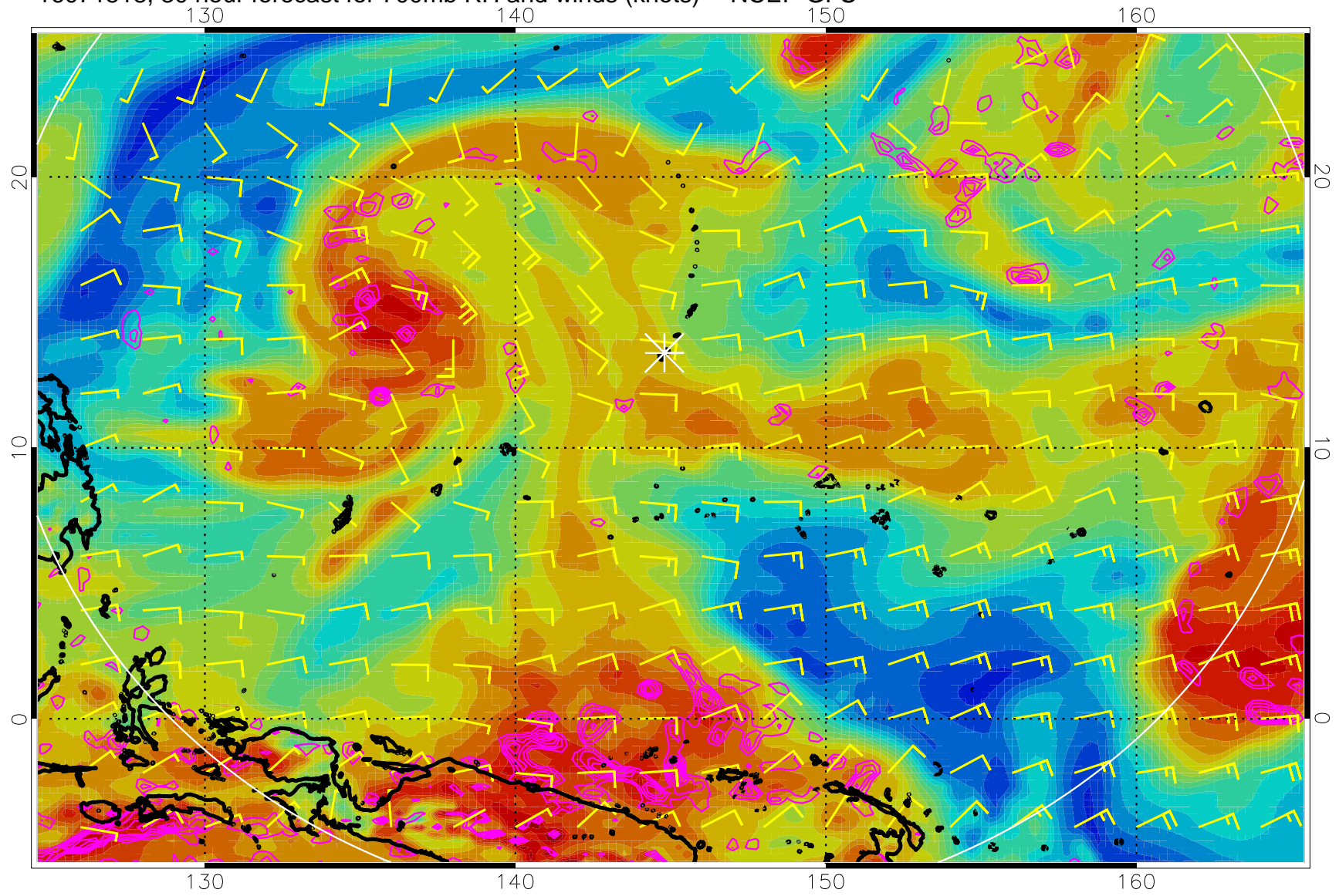
16071518, 30 hour forecast for 700mb RH and winds (knots) -- NCEP GFS
