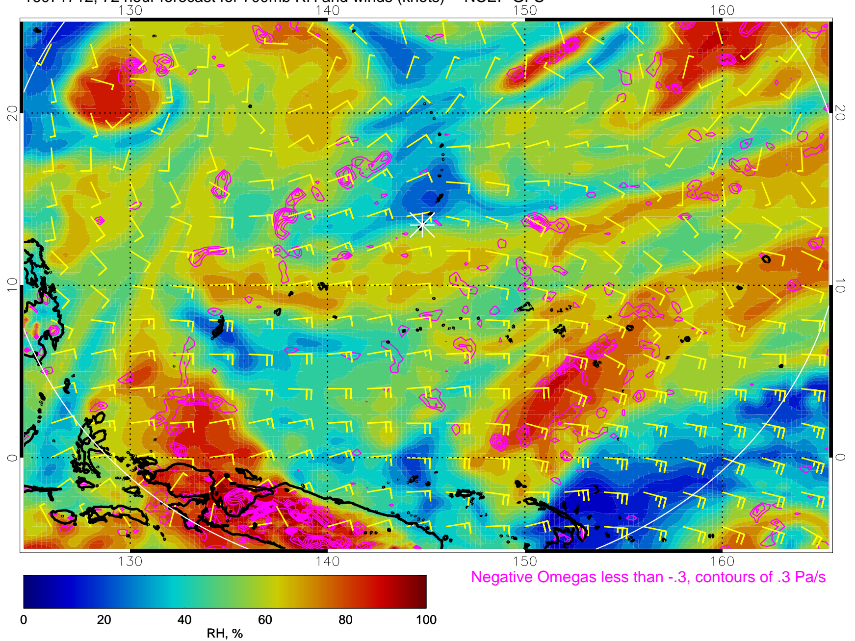
16071712, 72 hour forecast for 700mb RH and winds (knots) -- NCEP GFS
