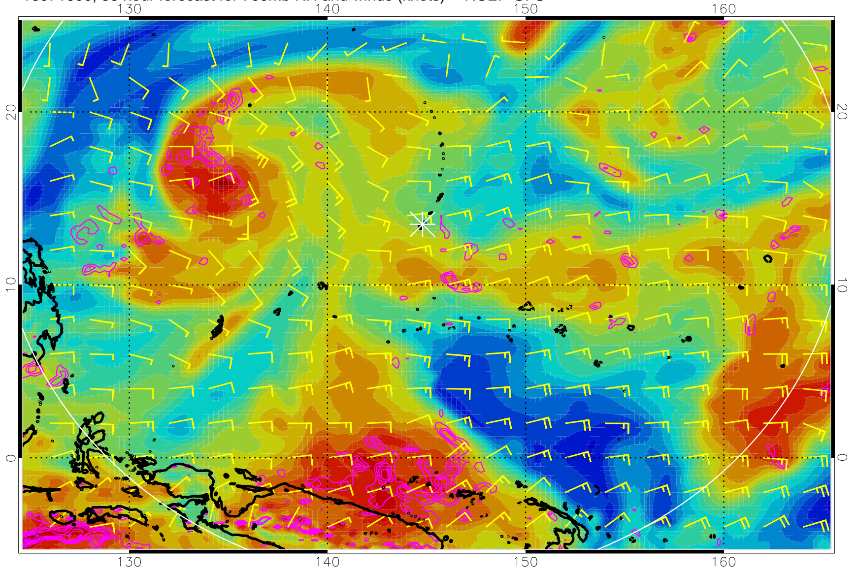
16071600, 36 hour forecast for 700mb RH and winds (knots) -- NCEP GFS
