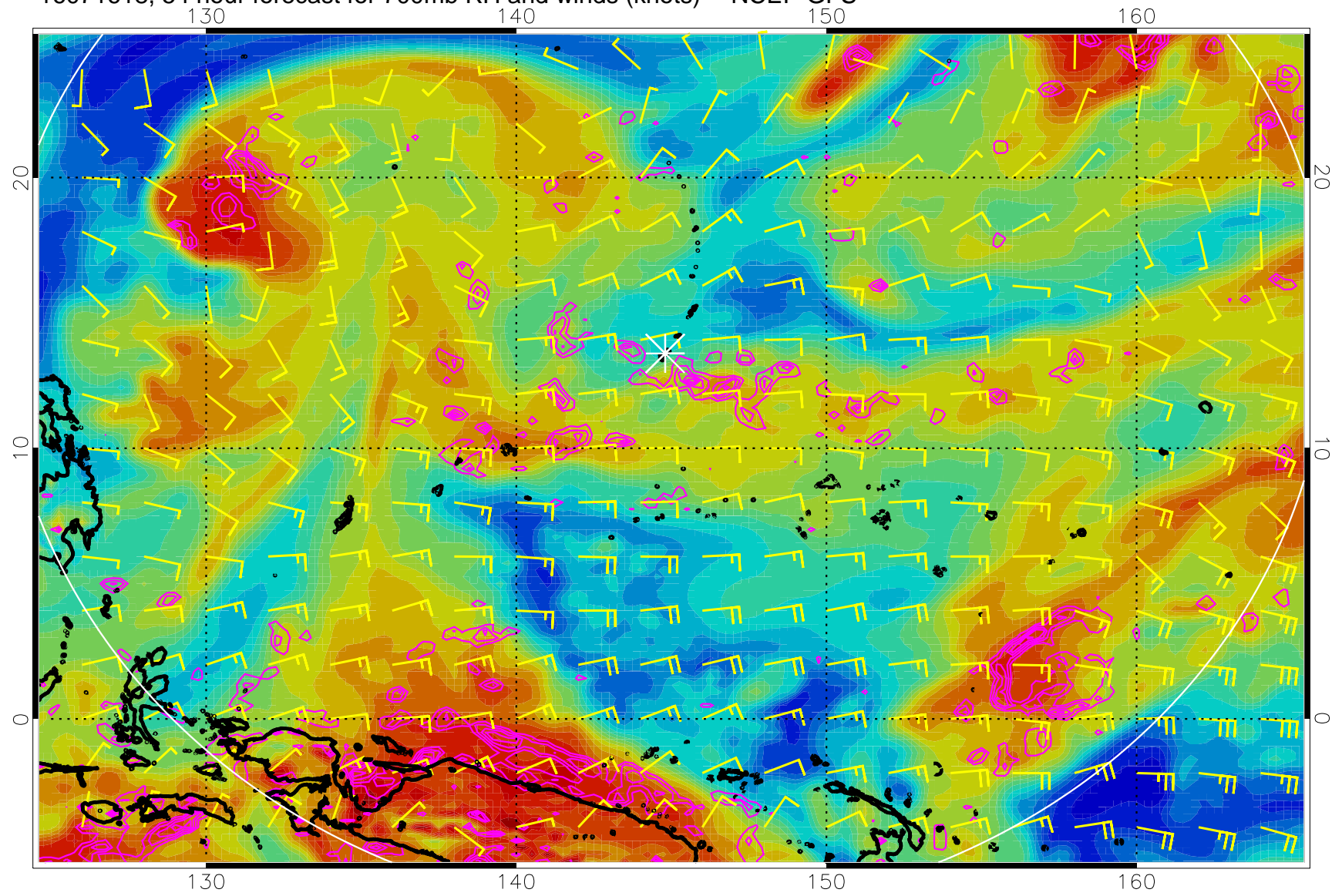
16071618, 54 hour forecast for 700mb RH and winds (knots) -- NCEP GFS
