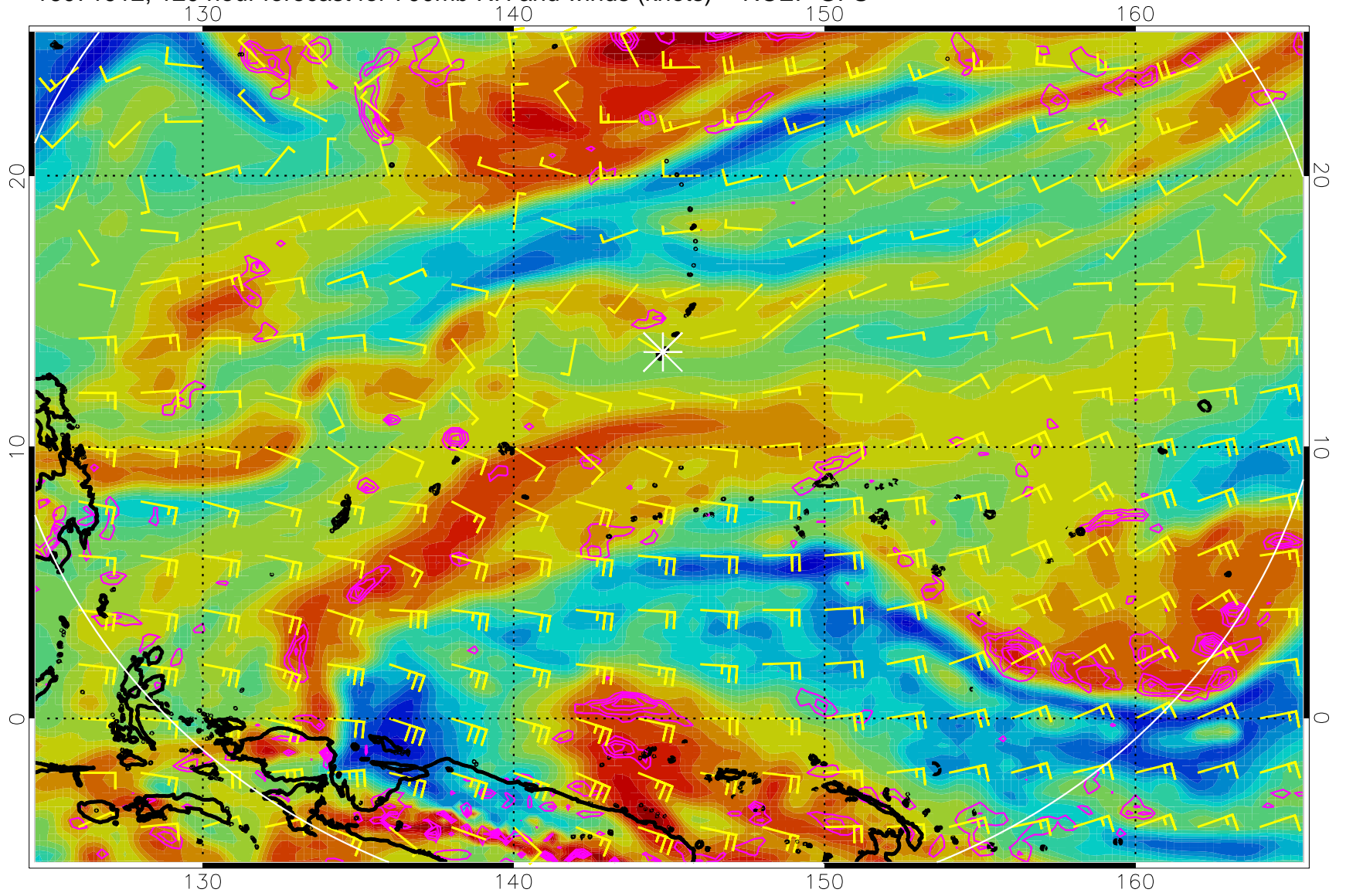
16071912, 120 hour forecast for 700mb RH and winds (knots) -- NCEP GFS
