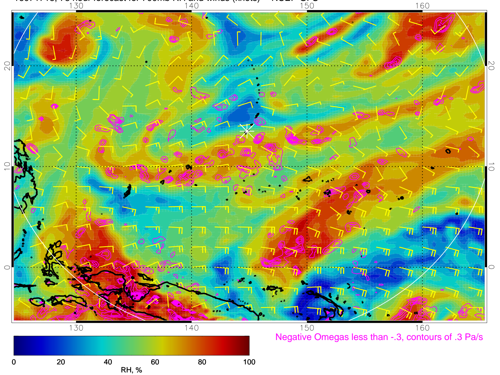
16071718, 78 hour forecast for 700mb RH and winds (knots) -- NCEP GFS
