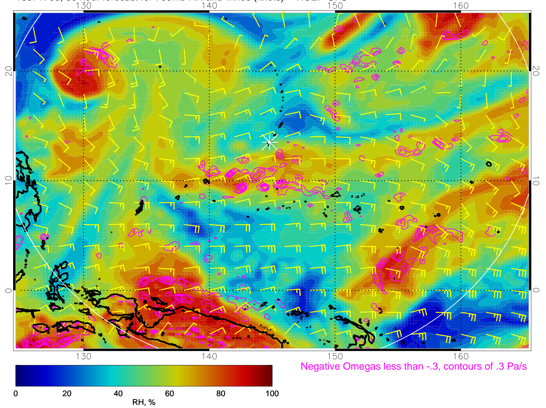
16071700, 60 hour forecast for 700mb RH and winds (knots) -- NCEP GFS
