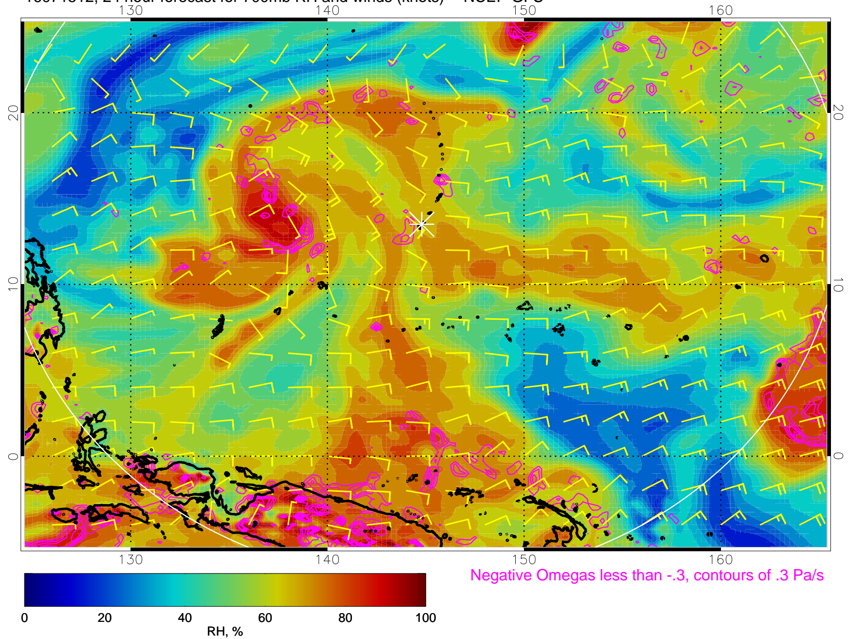
16071512, 24 hour forecast for 700mb RH and winds (knots) -- NCEP GFS
