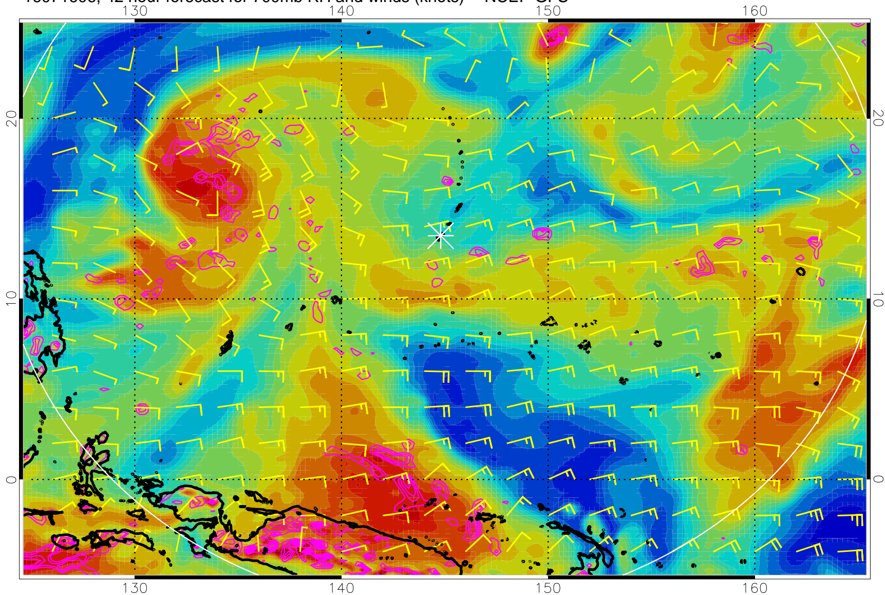
16071606, 42 hour forecast for 700mb RH and winds (knots) -- NCEP GFS
