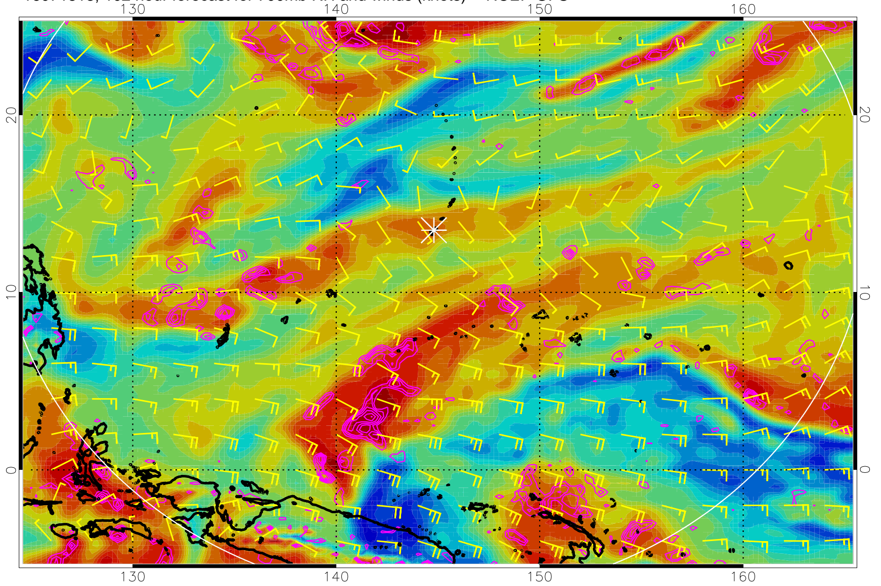
16071818, 102 hour forecast for 700mb RH and winds (knots) -- NCEP GFS
