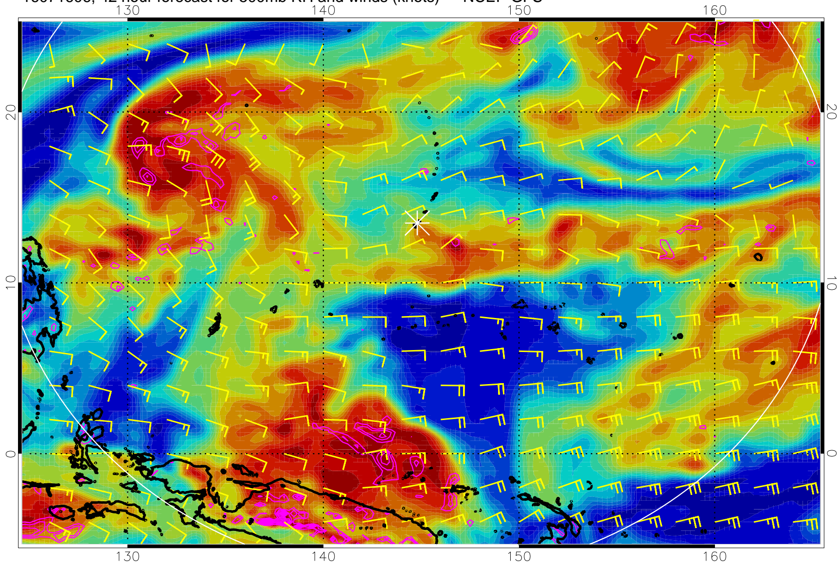
16071606, 42 hour forecast for 500mb RH and winds (knots) -- NCEP GFS
