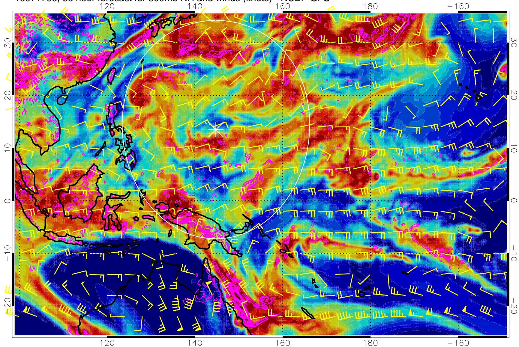
16071706, 66 hour forecast for 500mb RH and winds (knots) - NCEP GFS
