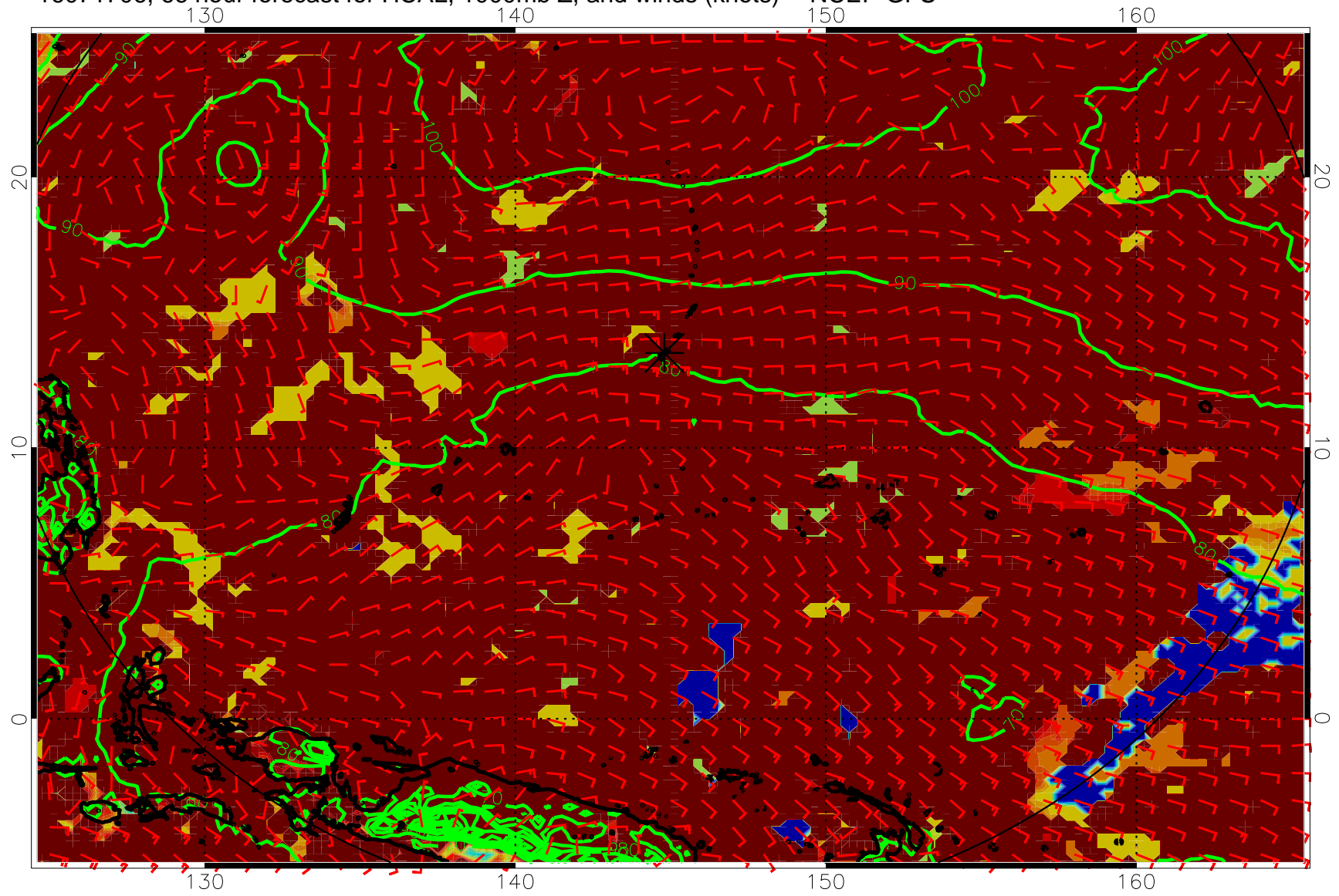
16071706, 66 hour forecast for HCAL, 1000mb Z, and winds (knots) -- NCEP GFS
