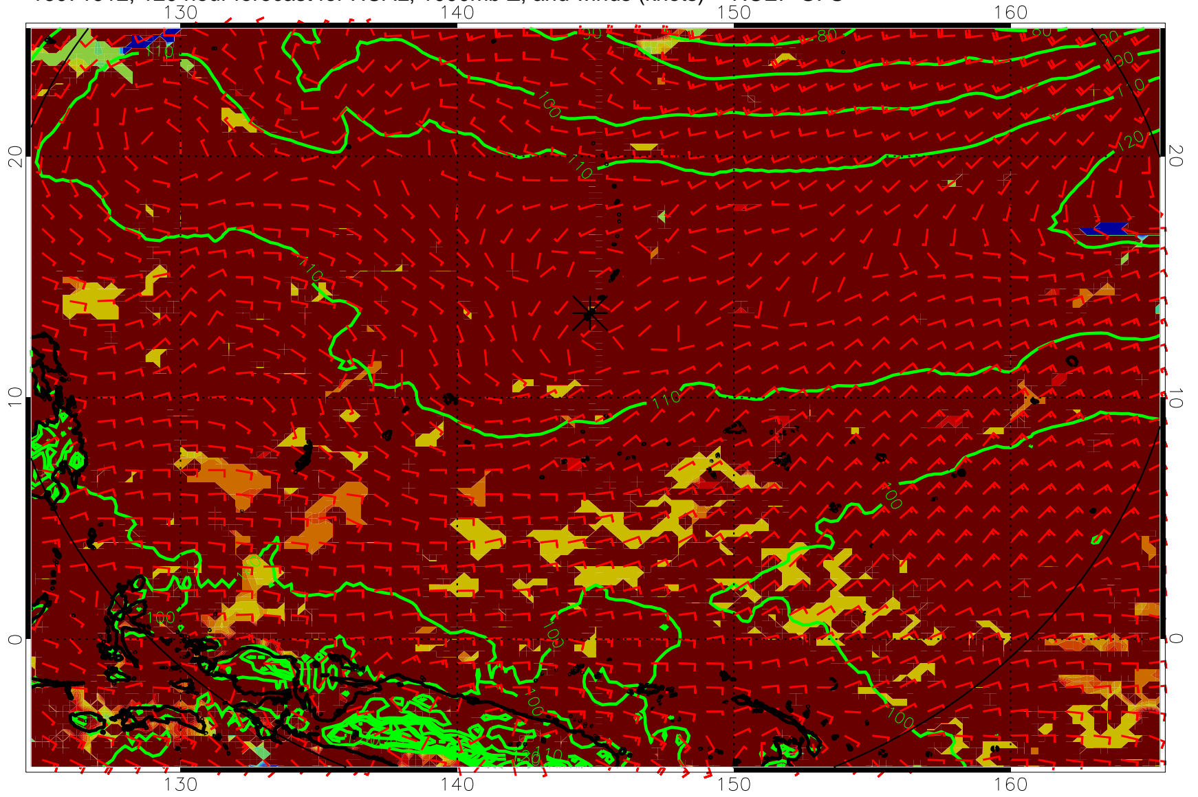
16071912, 120 hour forecast for HCAL, 1000mb Z, and winds (knots) -- NCEP GFS
