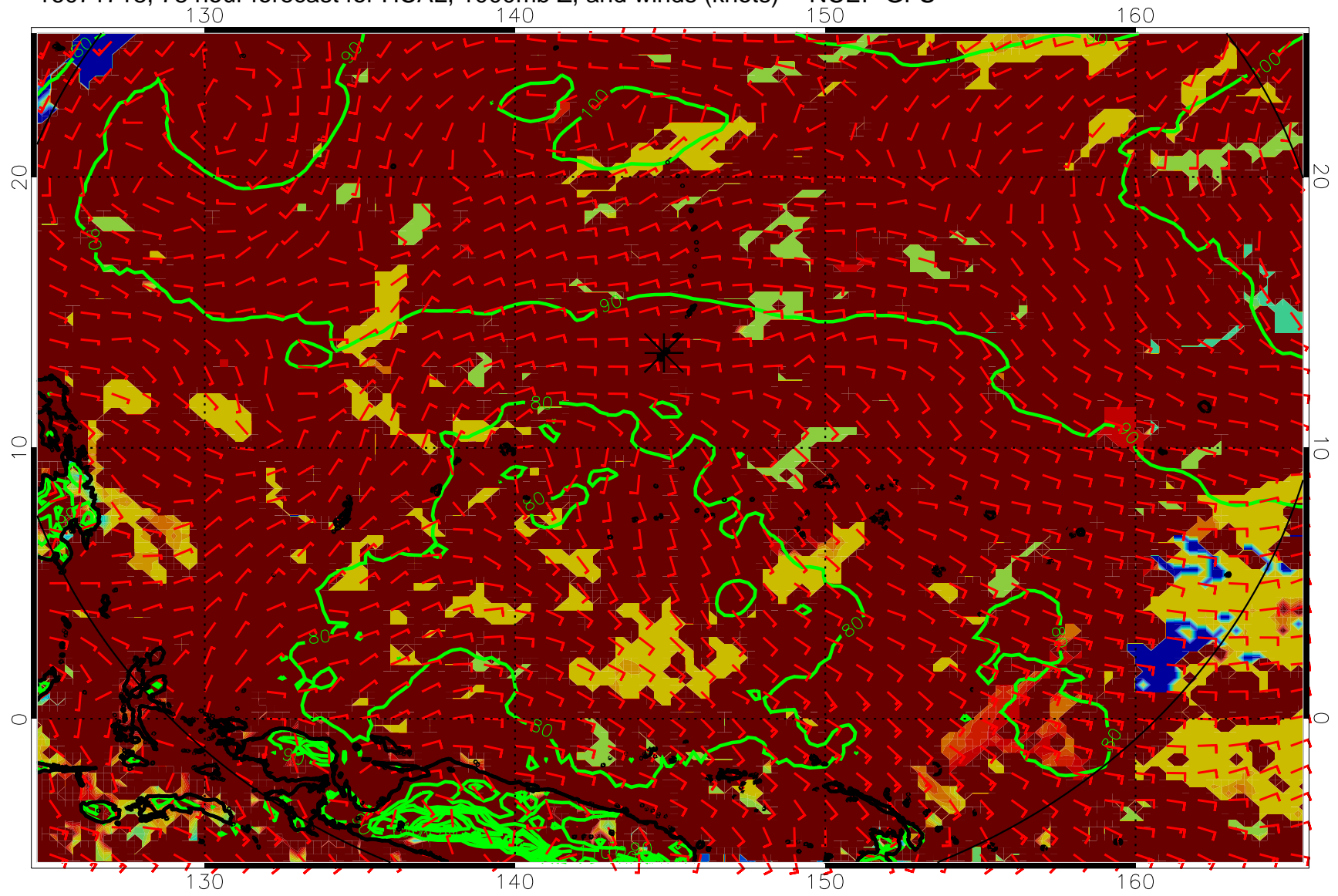
16071718, 78 hour forecast for HCAL, 1000mb Z, and winds (knots) -- NCEP GFS
