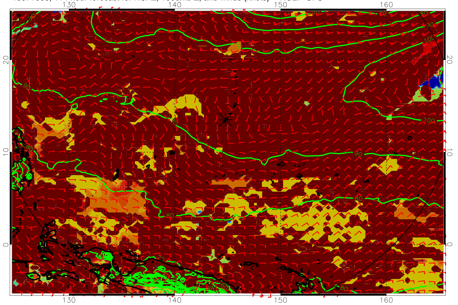
16071906, 114 hour forecast for HCAL, 1000mb Z, and winds (knots) -- NCEP GFS
