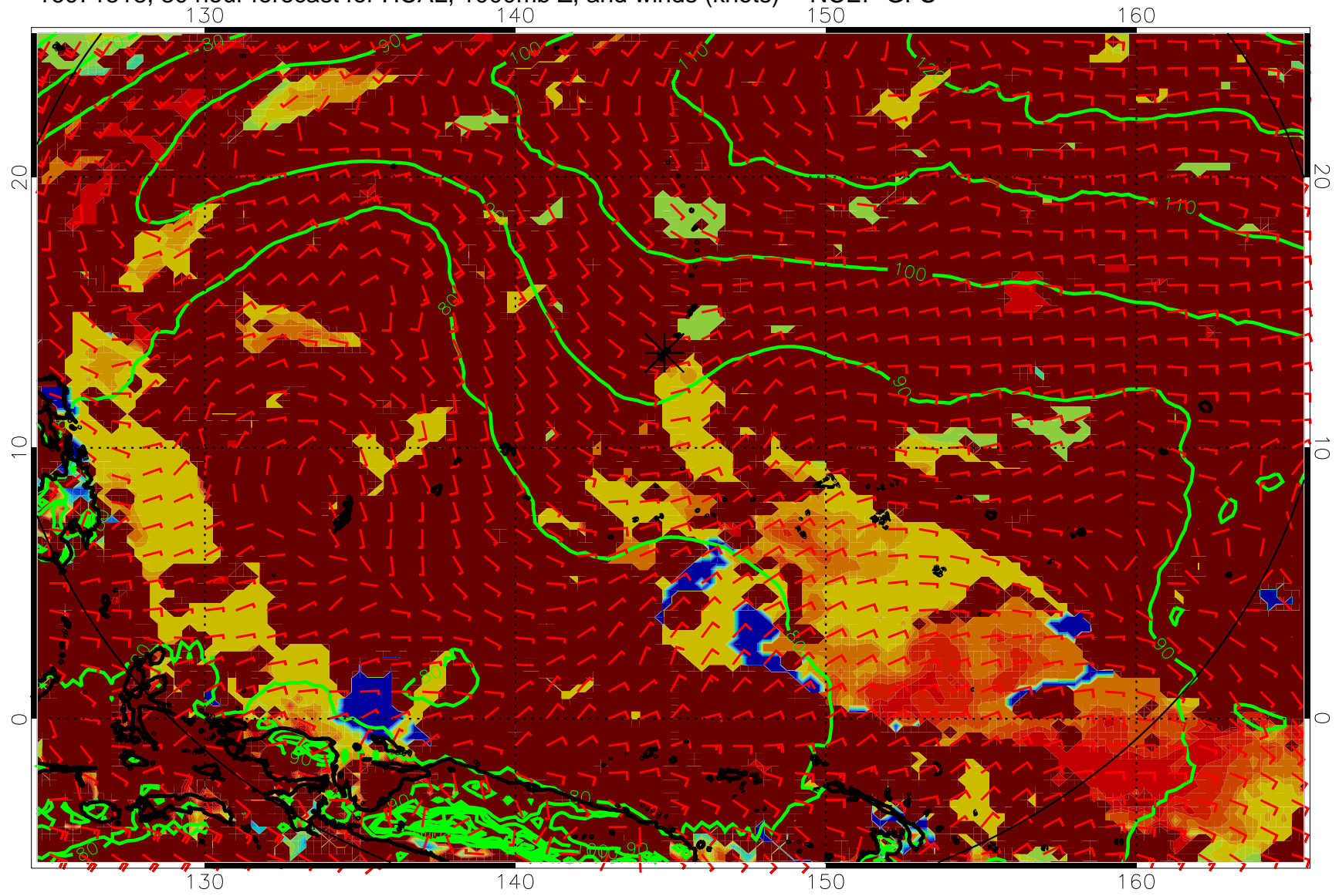
16071518, 30 hour forecast for HCAL, 1000mb Z, and winds (knots) -- NCEP GFS
