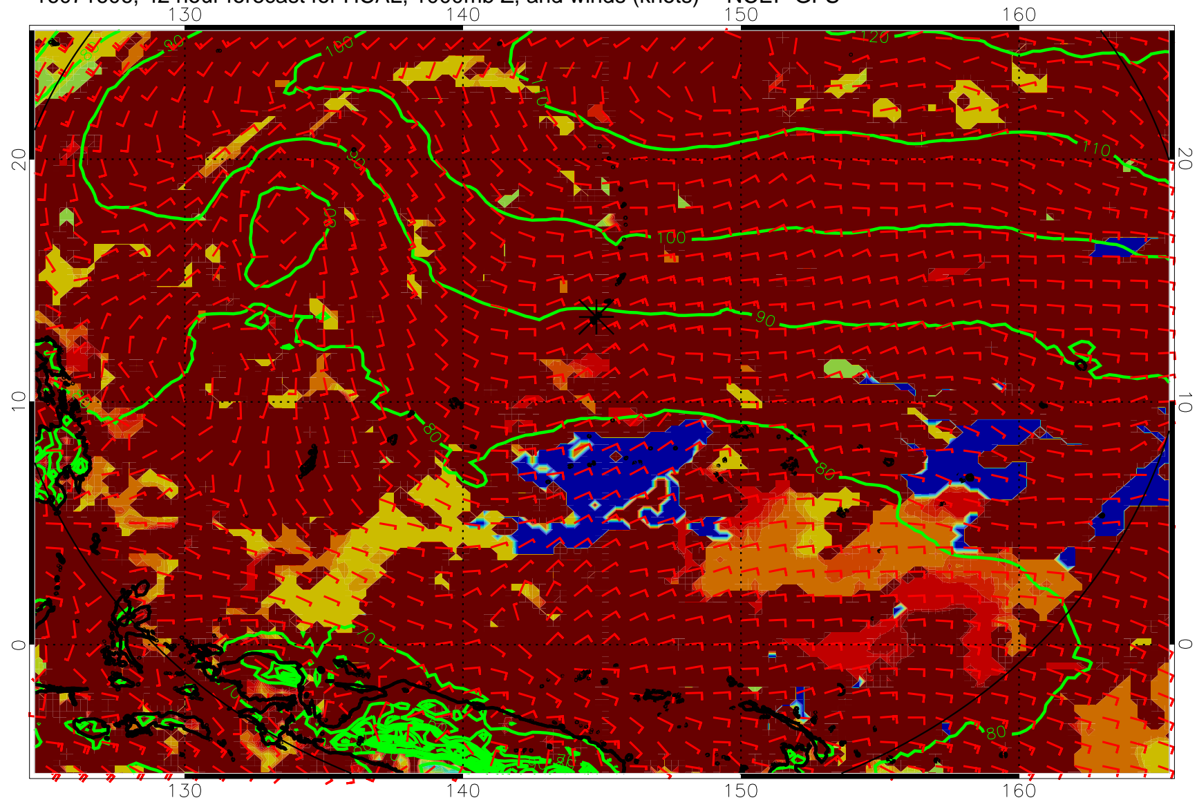
16071606, 42 hour forecast for HCAL, 1000mb Z, and winds (knots) -- NCEP GFS
