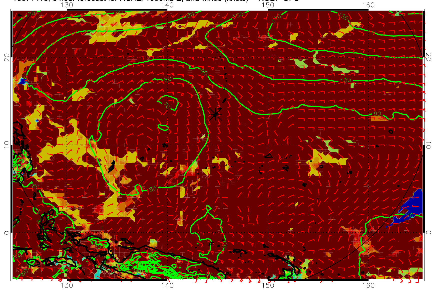
16071418, 6 hour forecast for HCAL, 1000mb Z, and winds (knots) -- NCEP GFS
