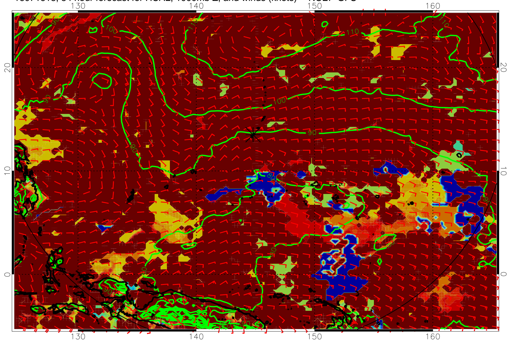
16071618, 54 hour forecast for HCAL, 1000mb Z, and winds (knots) -- NCEP GFS
