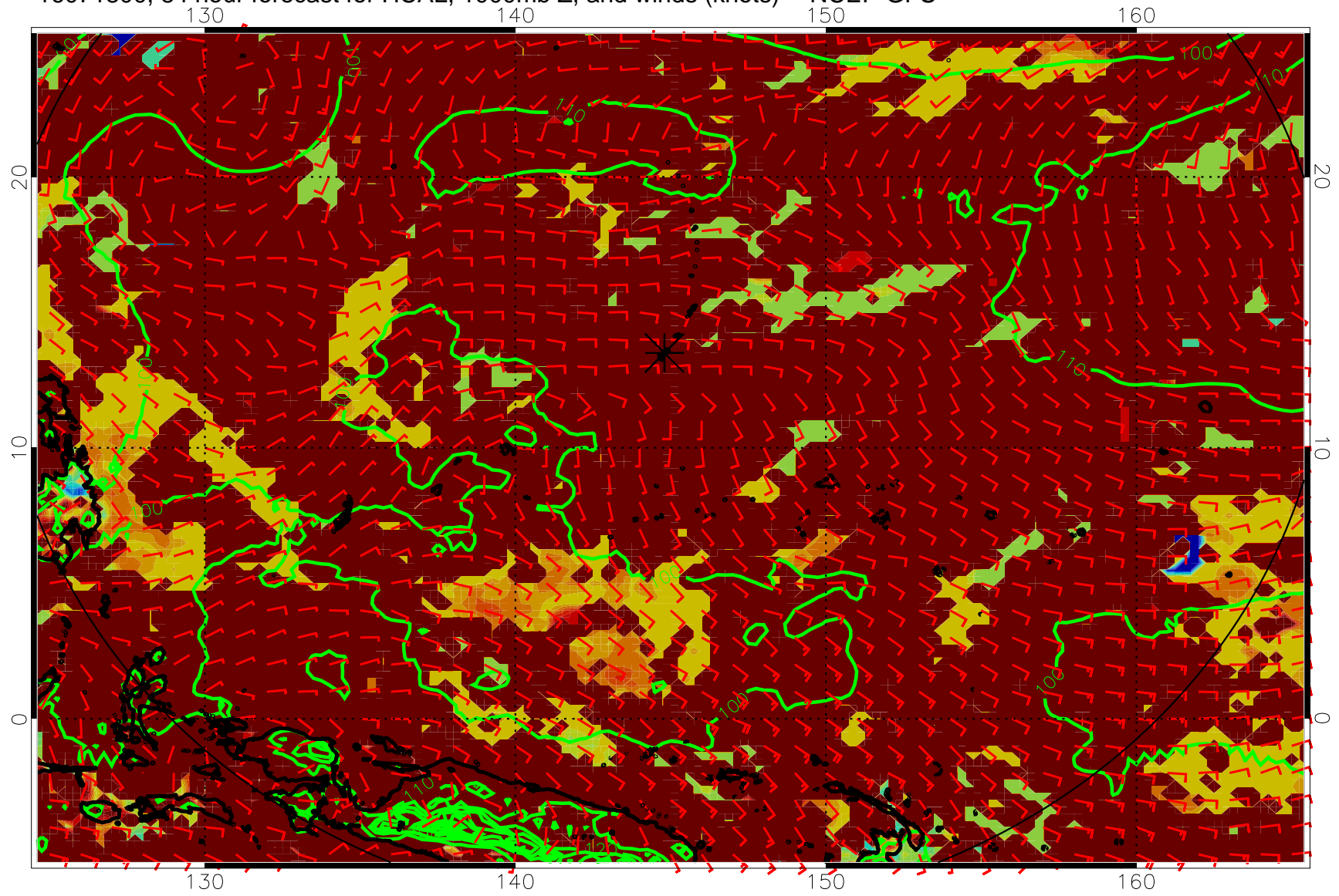
16071800, 84 hour forecast for HCAL, 1000mb Z, and winds (knots) -- NCEP GFS
