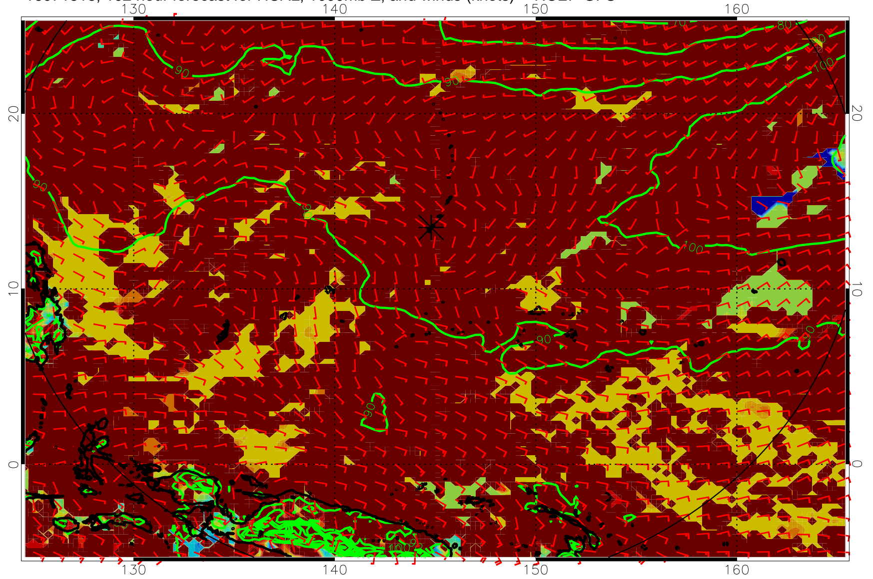
16071818, 102 hour forecast for HCAL, 1000mb Z, and winds (knots) -- NCEP GFS
