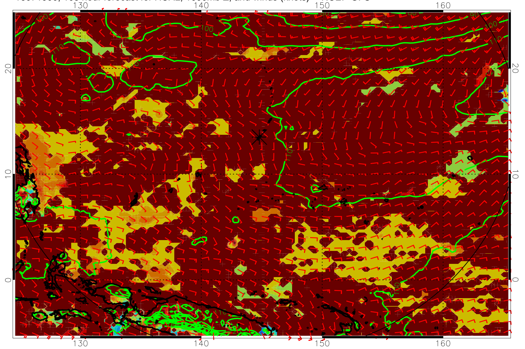
16071900, 108 hour forecast for HCAL, 1000mb Z, and winds (knots) -- NCEP GFS
