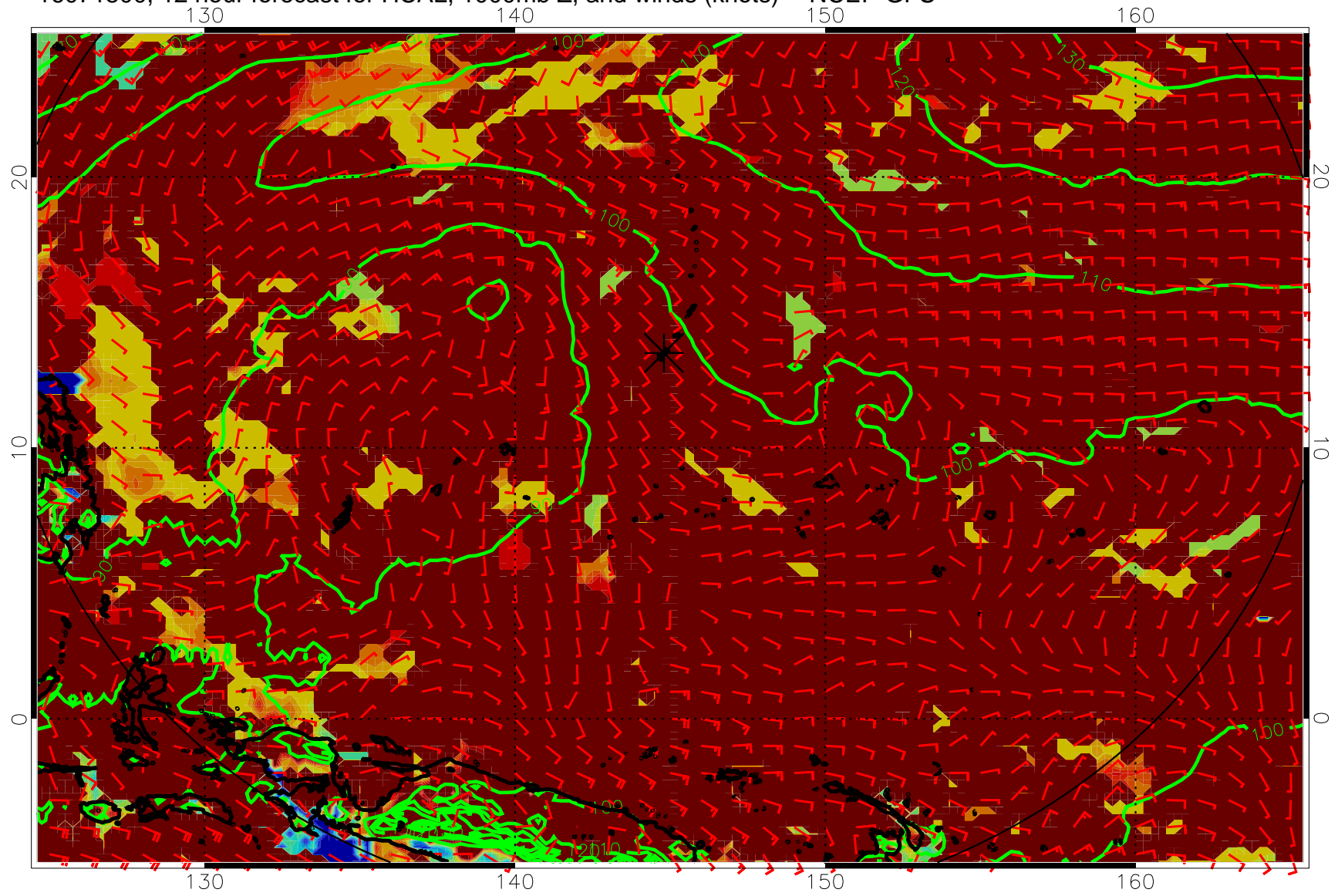
16071500, 12 hour forecast for HCAL, 1000mb Z, and winds (knots) -- NCEP GFS
