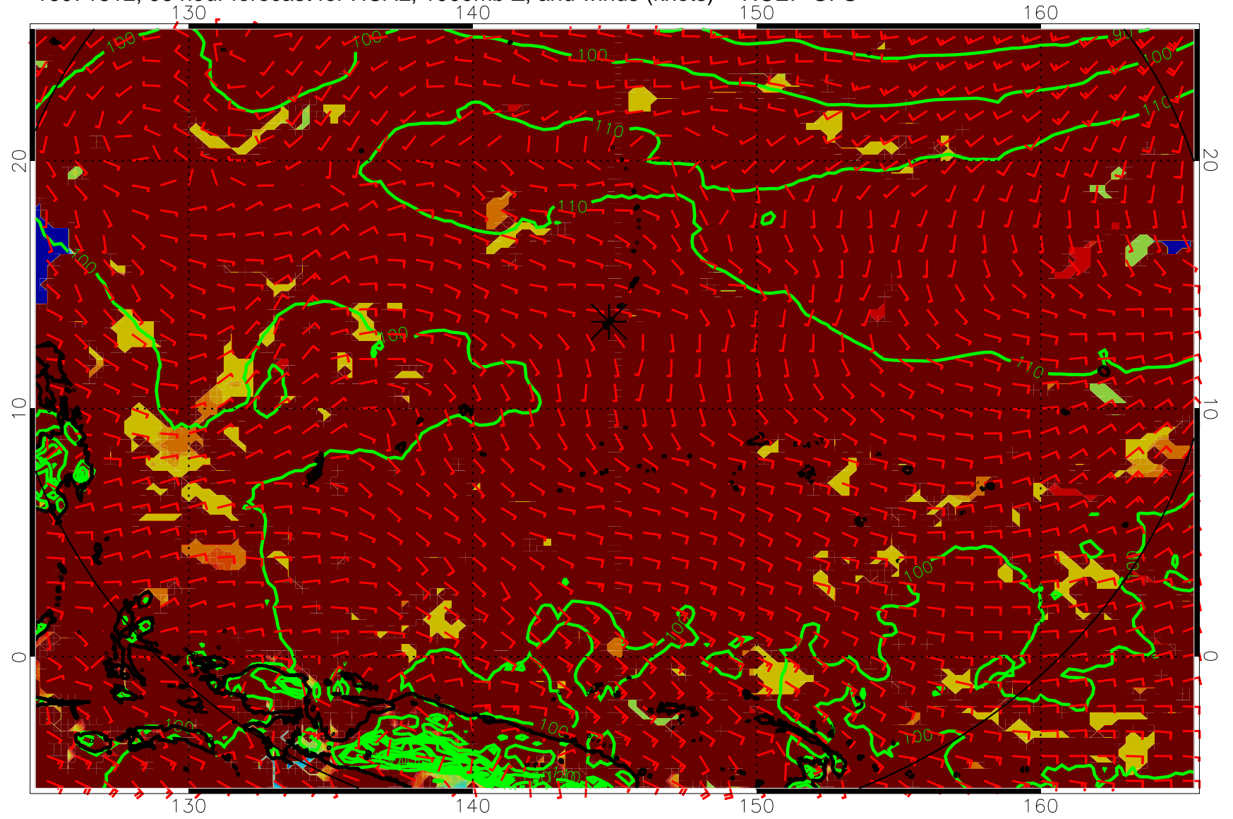
16071812, 96 hour forecast for HCAL, 1000mb Z, and winds (knots) -- NCEP GFS
