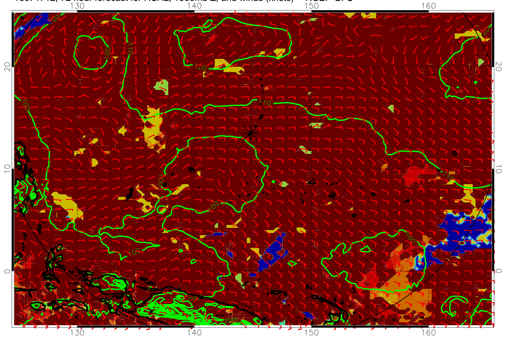
16071712, 72 hour forecast for HCAL, 1000mb Z, and winds (knots) -- NCEP GFS
