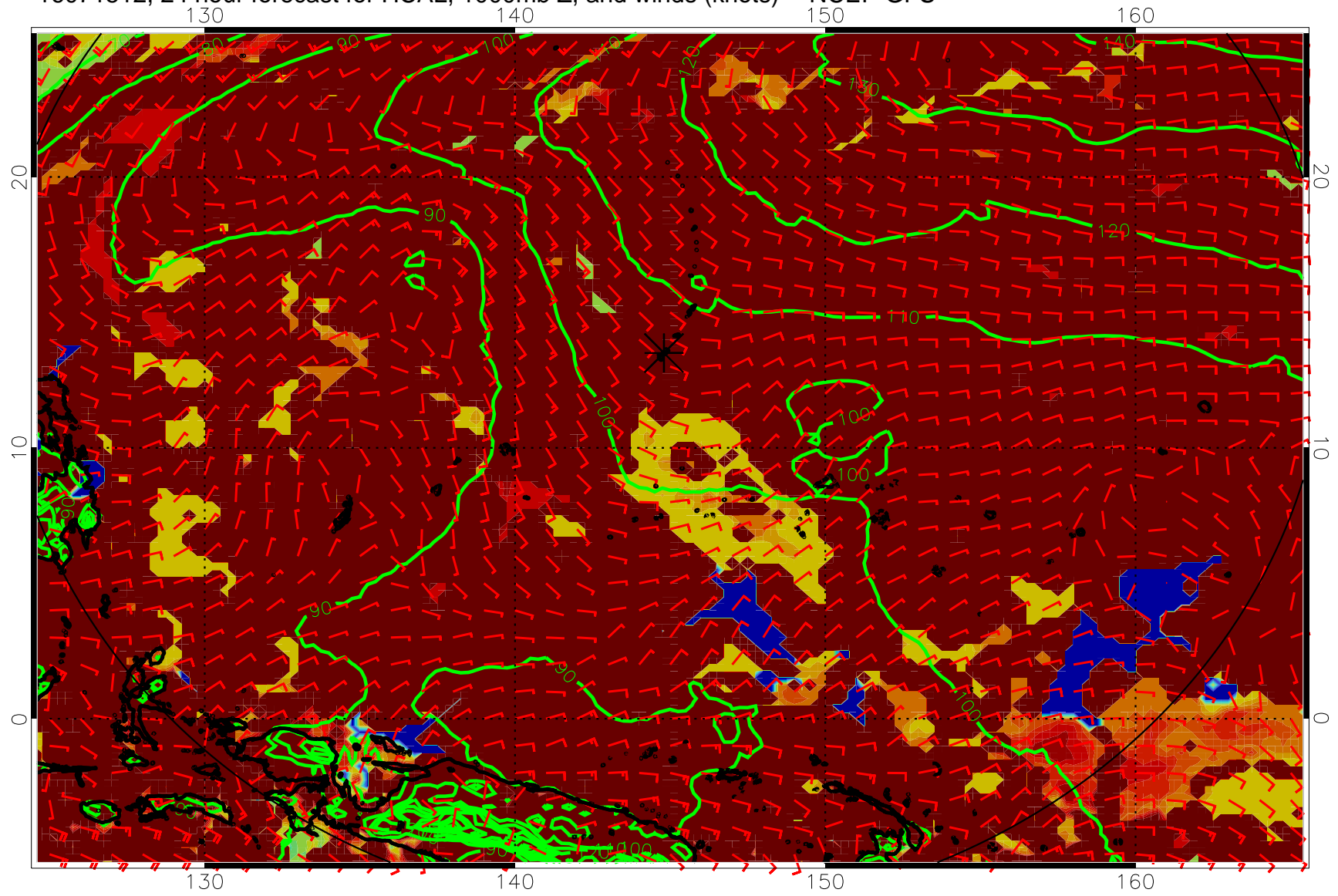
16071512, 24 hour forecast for HCAL, 1000mb Z, and winds (knots) -- NCEP GFS
