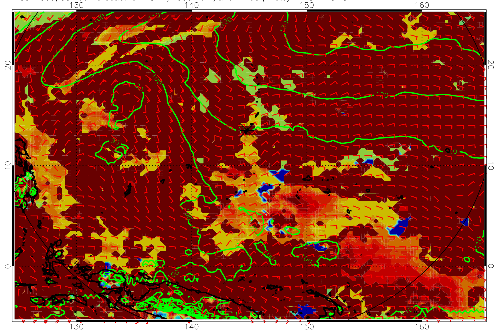
16071600, 36 hour forecast for HCAL, 1000mb Z, and winds (knots) -- NCEP GFS
