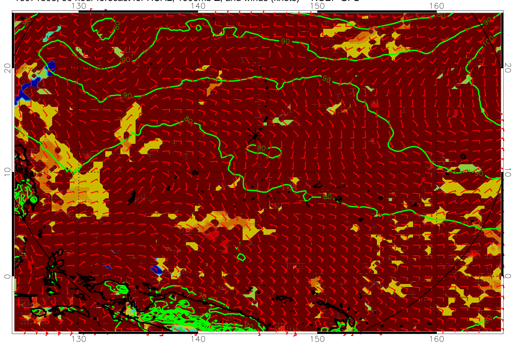
16071806, 90 hour forecast for HCAL, 1000mb Z, and winds (knots) -- NCEP GFS
