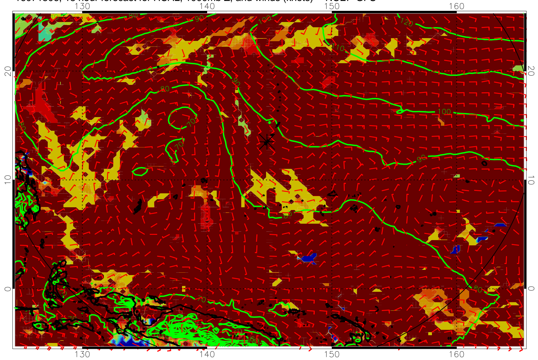
16071506, 18 hour forecast for HCAL, 1000mb Z, and winds (knots) -- NCEP GFS
