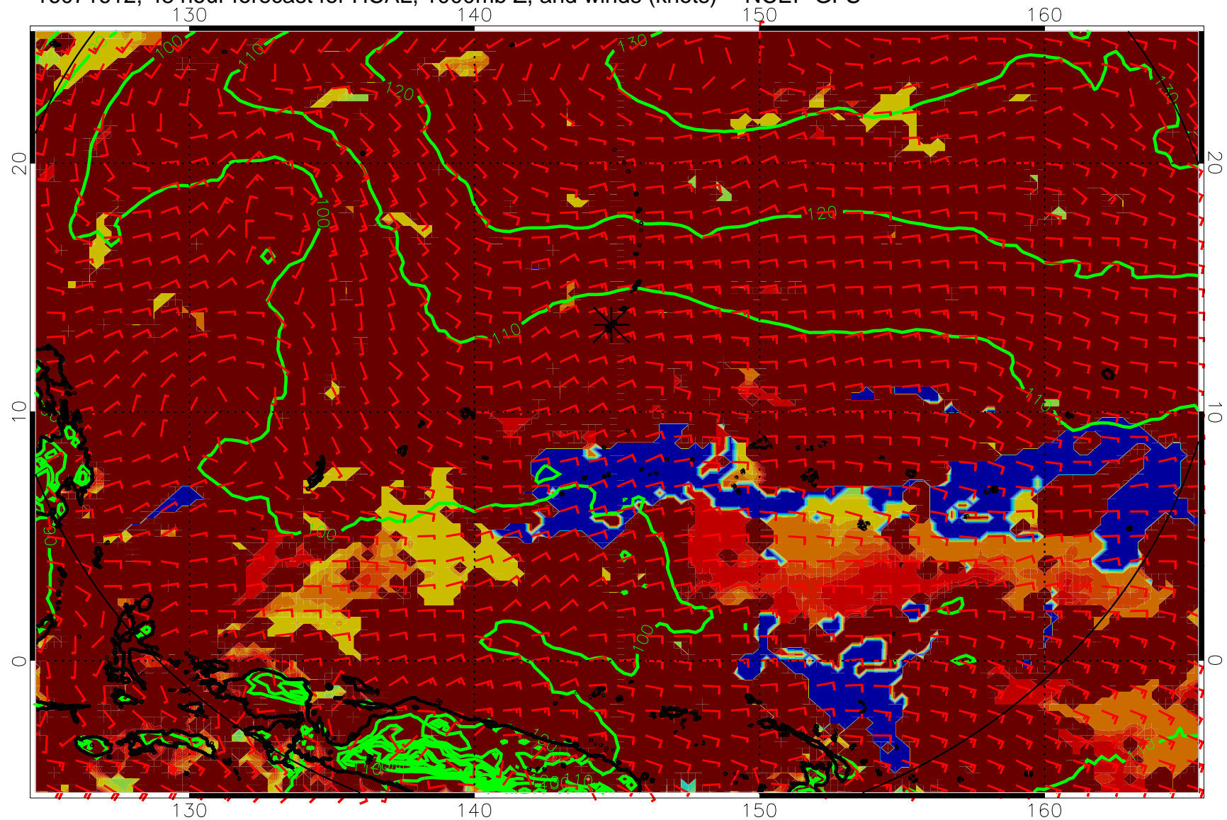
16071612, 48 hour forecast for HCAL, 1000mb Z, and winds (knots) -- NCEP GFS
