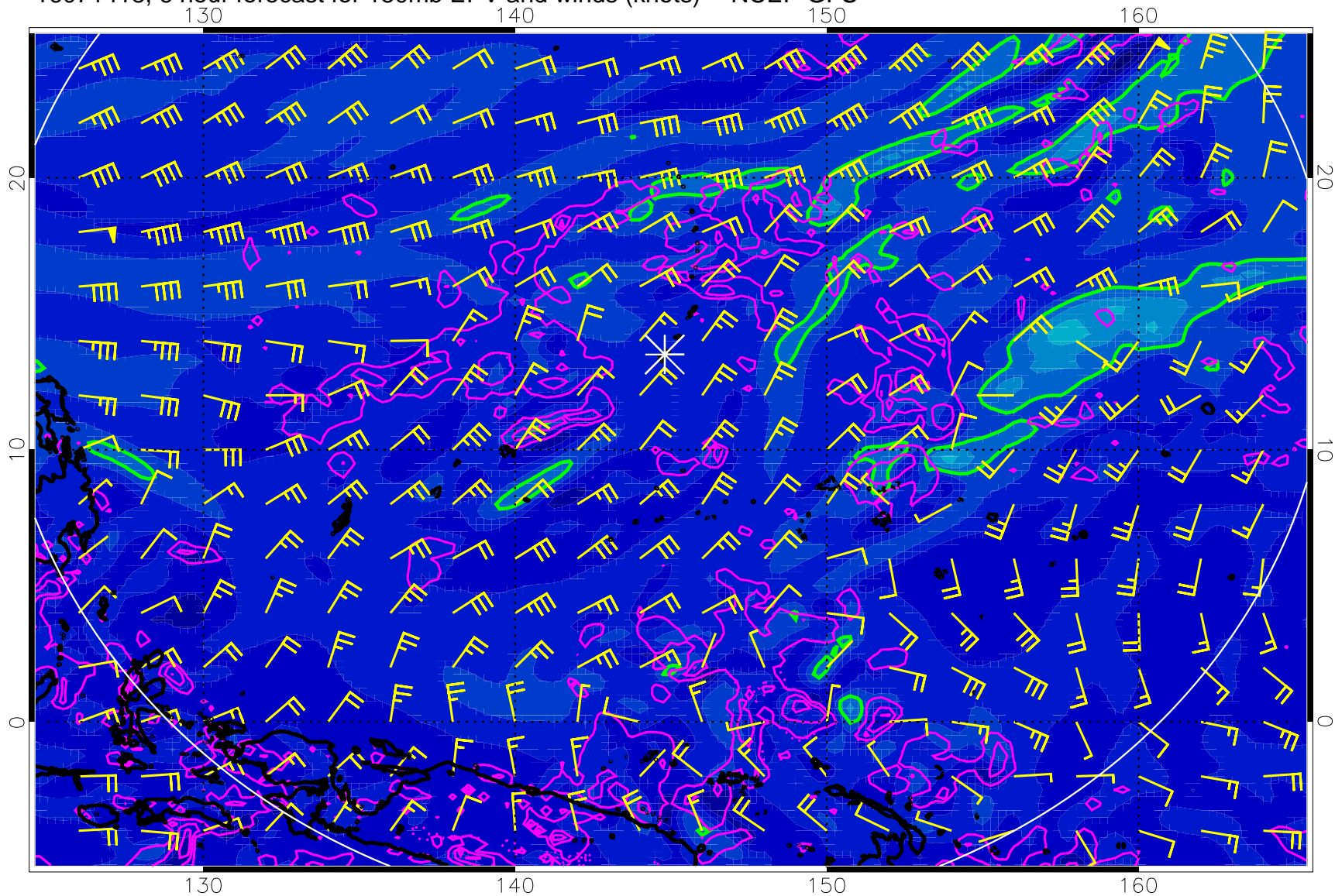
16071418, 6 hour forecast for 150mb EPV and winds (knots) -- NCEP GFS
