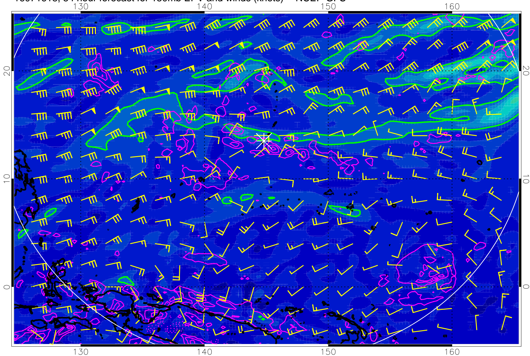
16071618, 54 hour forecast for 150mb EPV and winds (knots) -- NCEP GFS
