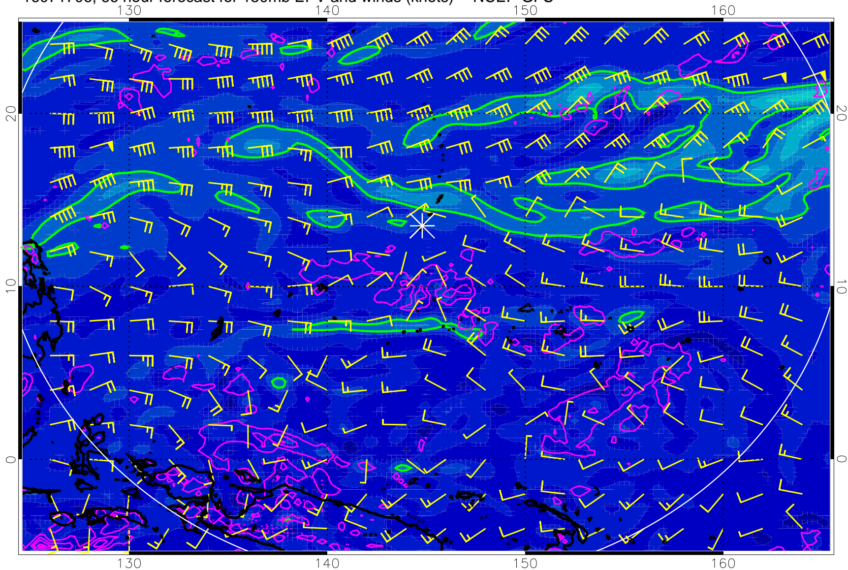
16071706, 66 hour forecast for 150mb EPV and winds (knots) -- NCEP GFS
