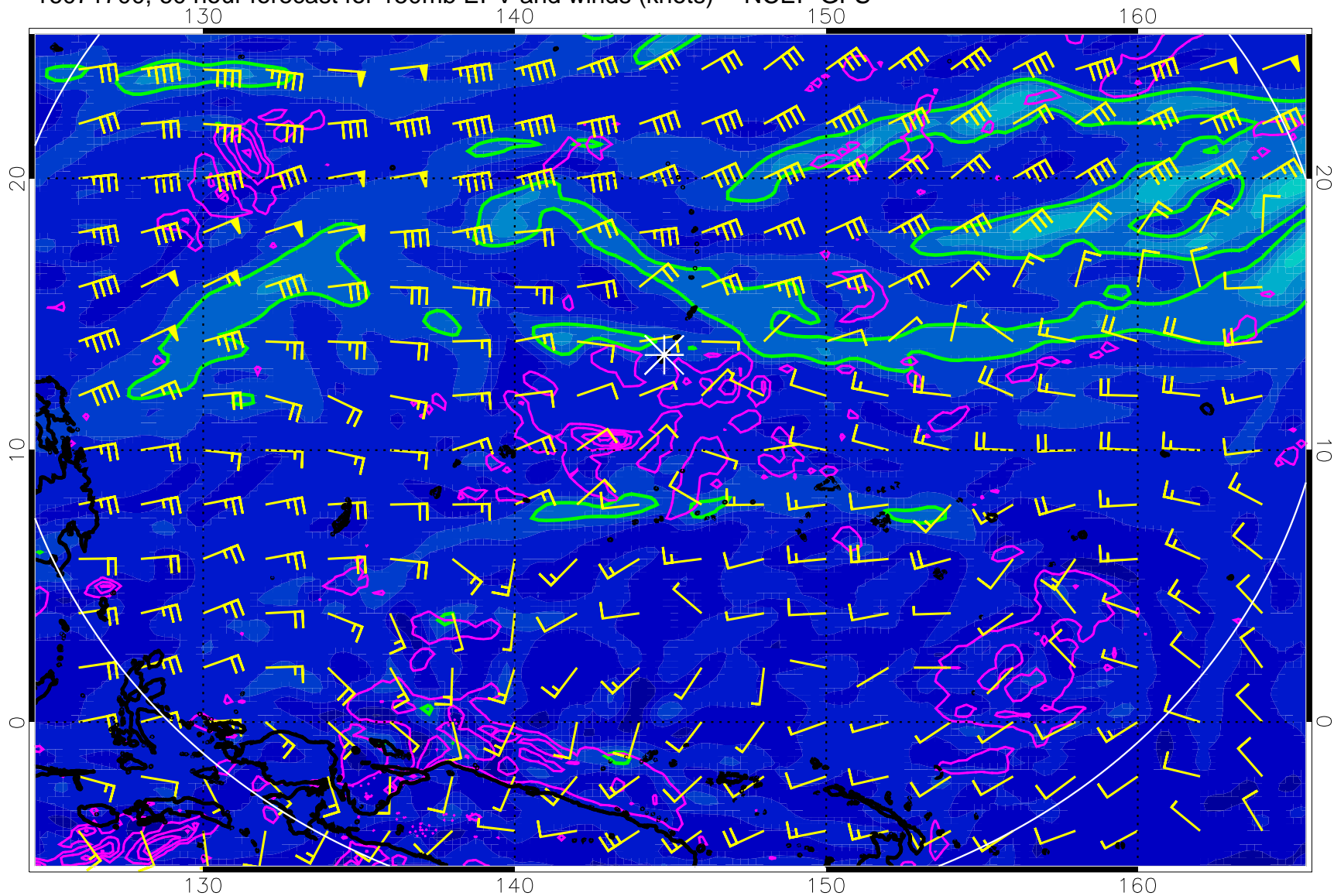
16071700, 60 hour forecast for 150mb EPV and winds (knots) -- NCEP GFS
