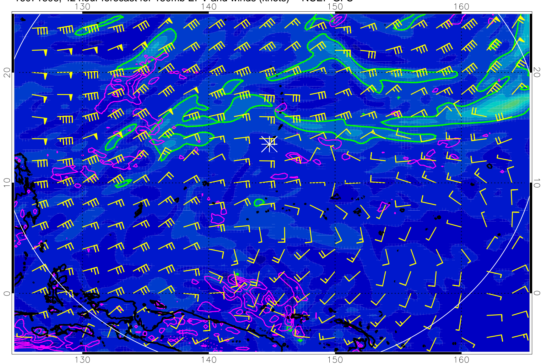
16071606, 42 hour forecast for 150mb EPV and winds (knots) -- NCEP GFS
