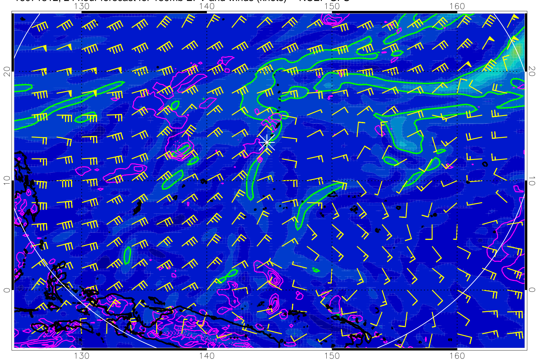
16071512, 24 hour forecast for 150mb EPV and winds (knots) -- NCEP GFS
