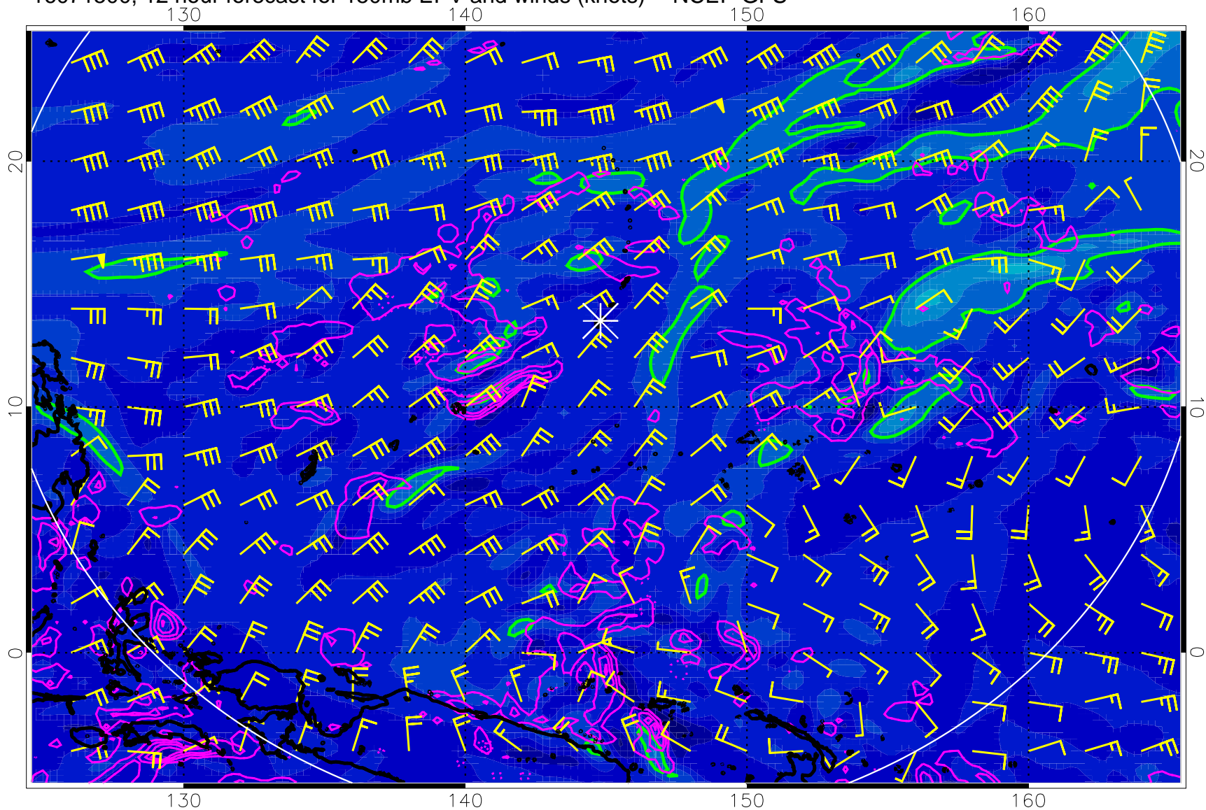
16071500, 12 hour forecast for 150mb EPV and winds (knots) -- NCEP GFS
