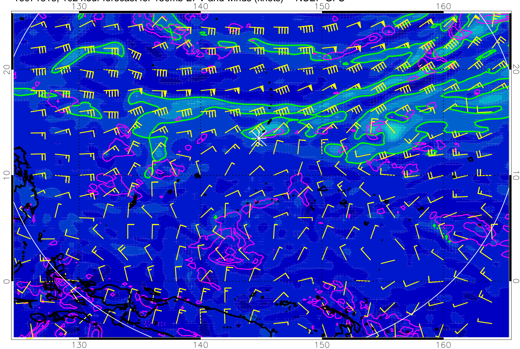
16071818, 102 hour forecast for 150mb EPV and winds (knots) -- NCEP GFS
