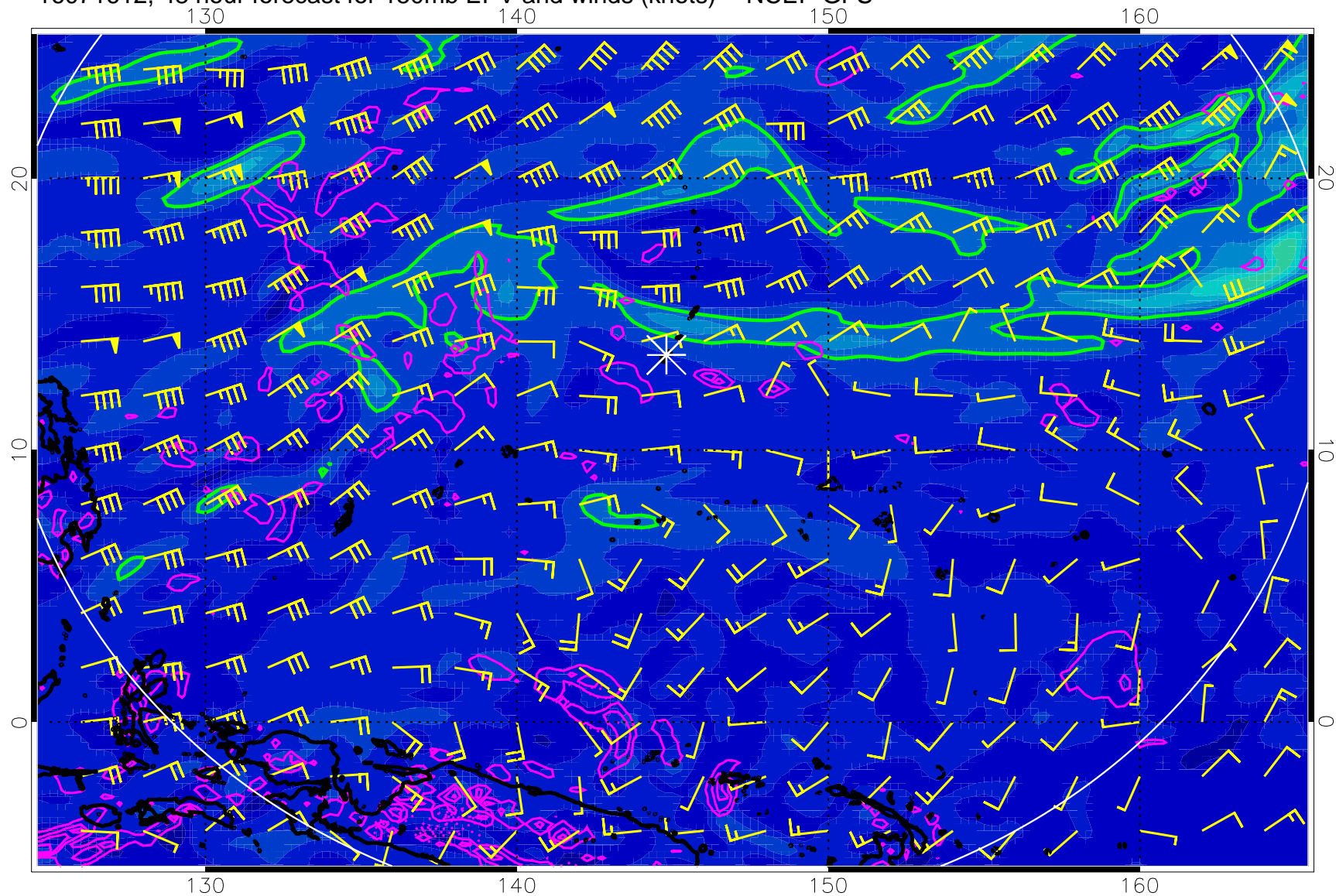
16071612, 48 hour forecast for 150mb EPV and winds (knots) -- NCEP GFS
