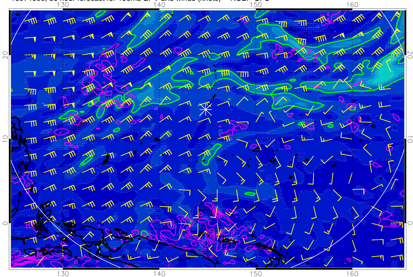
16071600, 36 hour forecast for 150mb EPV and winds (knots) -- NCEP GFS
