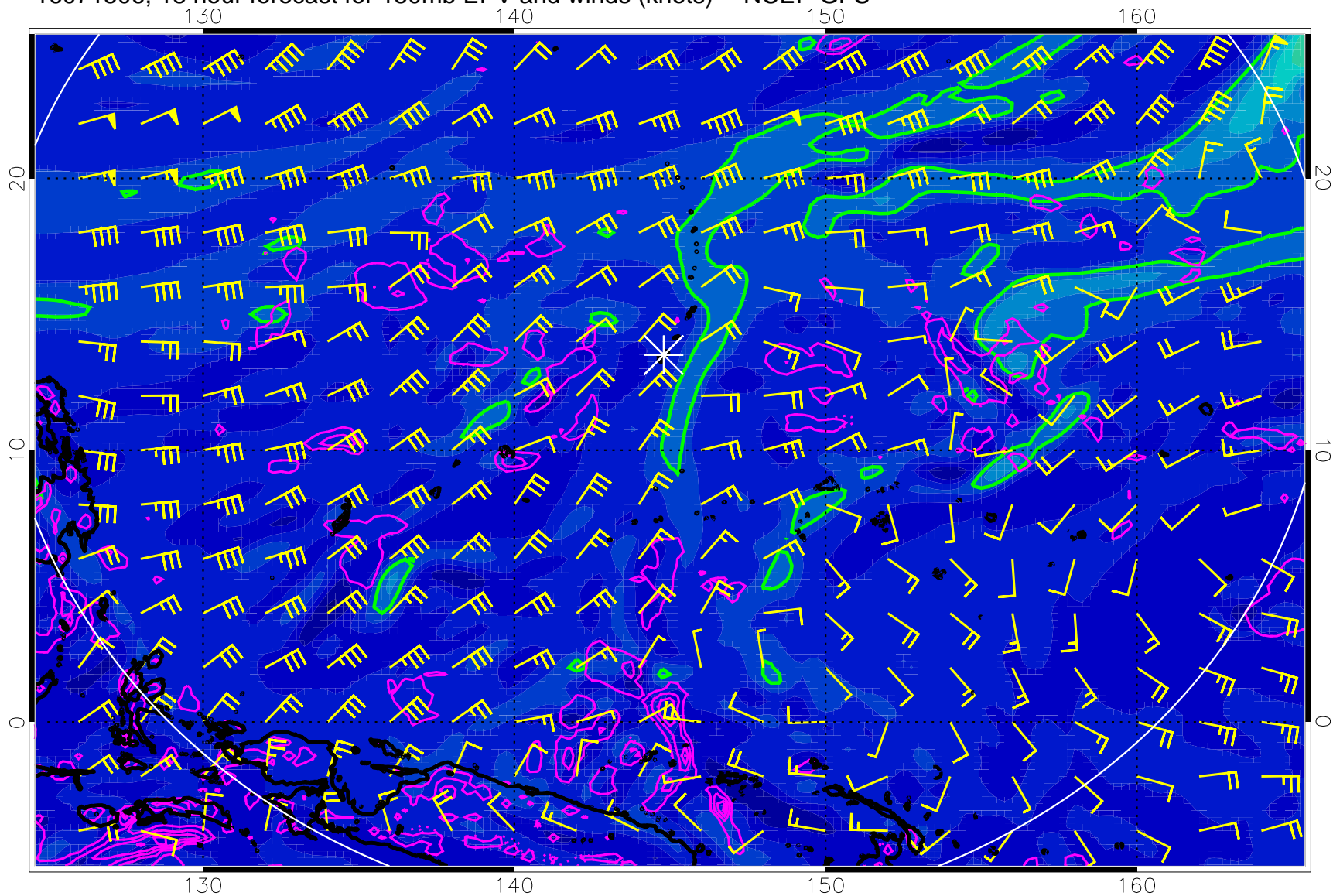
16071506, 18 hour forecast for 150mb EPV and winds (knots) -- NCEP GFS
