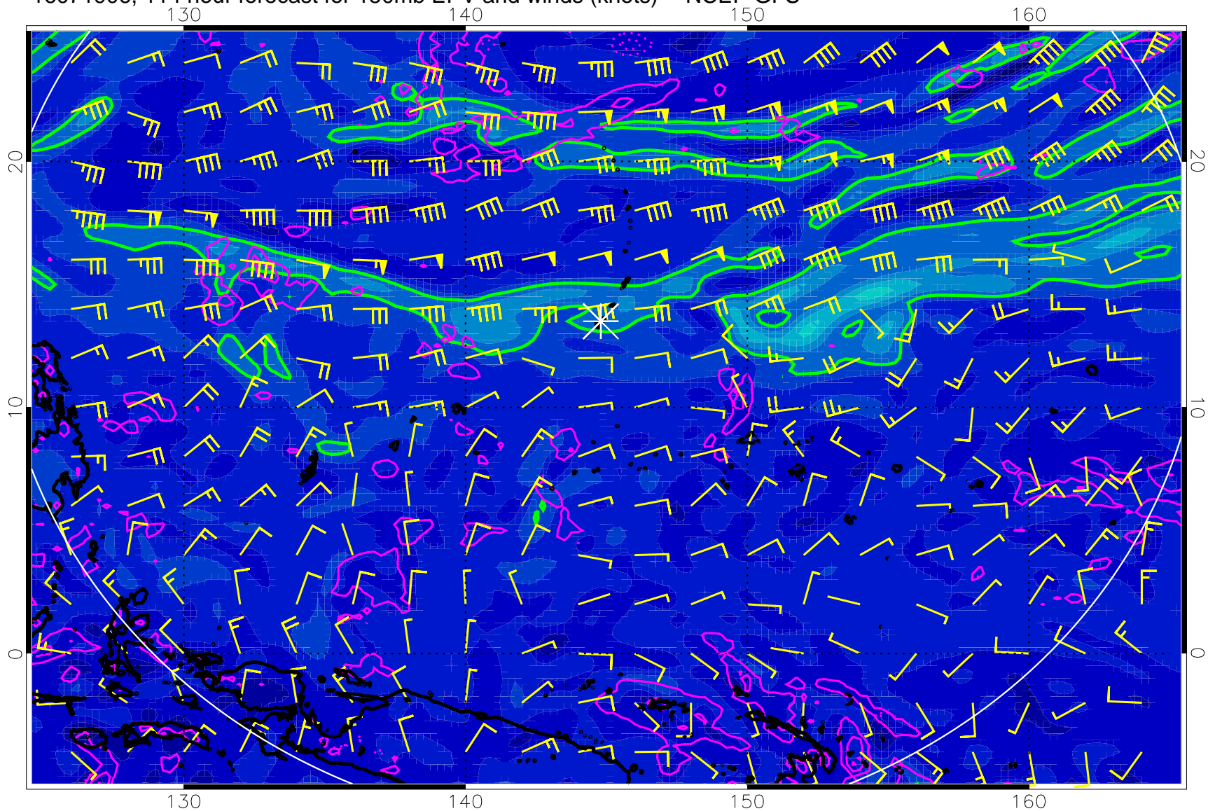
16071906, 114 hour forecast for 150mb EPV and winds (knots) -- NCEP GFS
